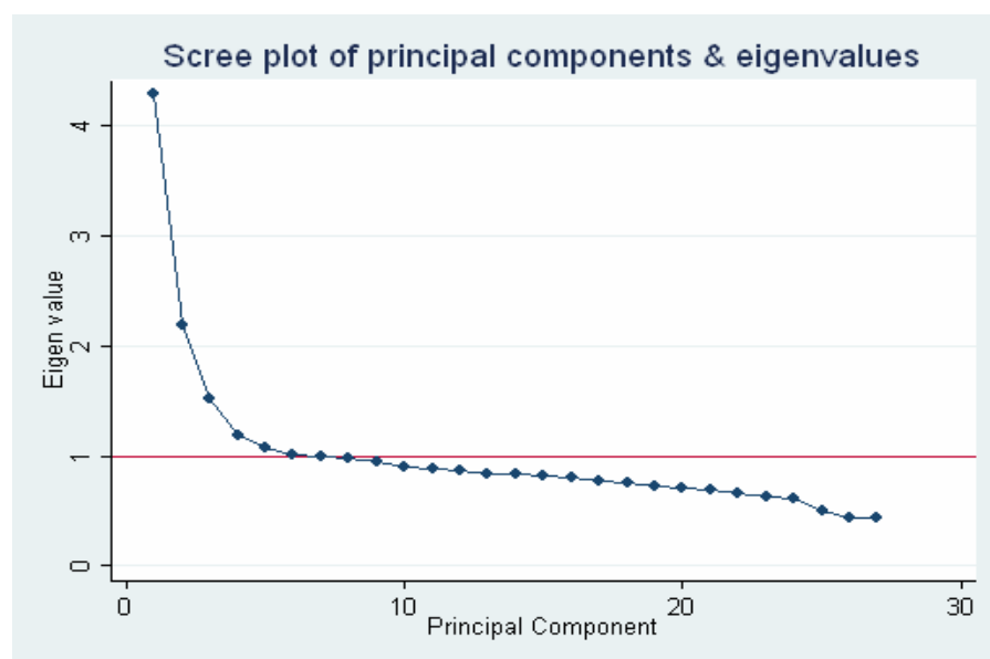
Figure 2: Scree plot of principal components and eigen values
