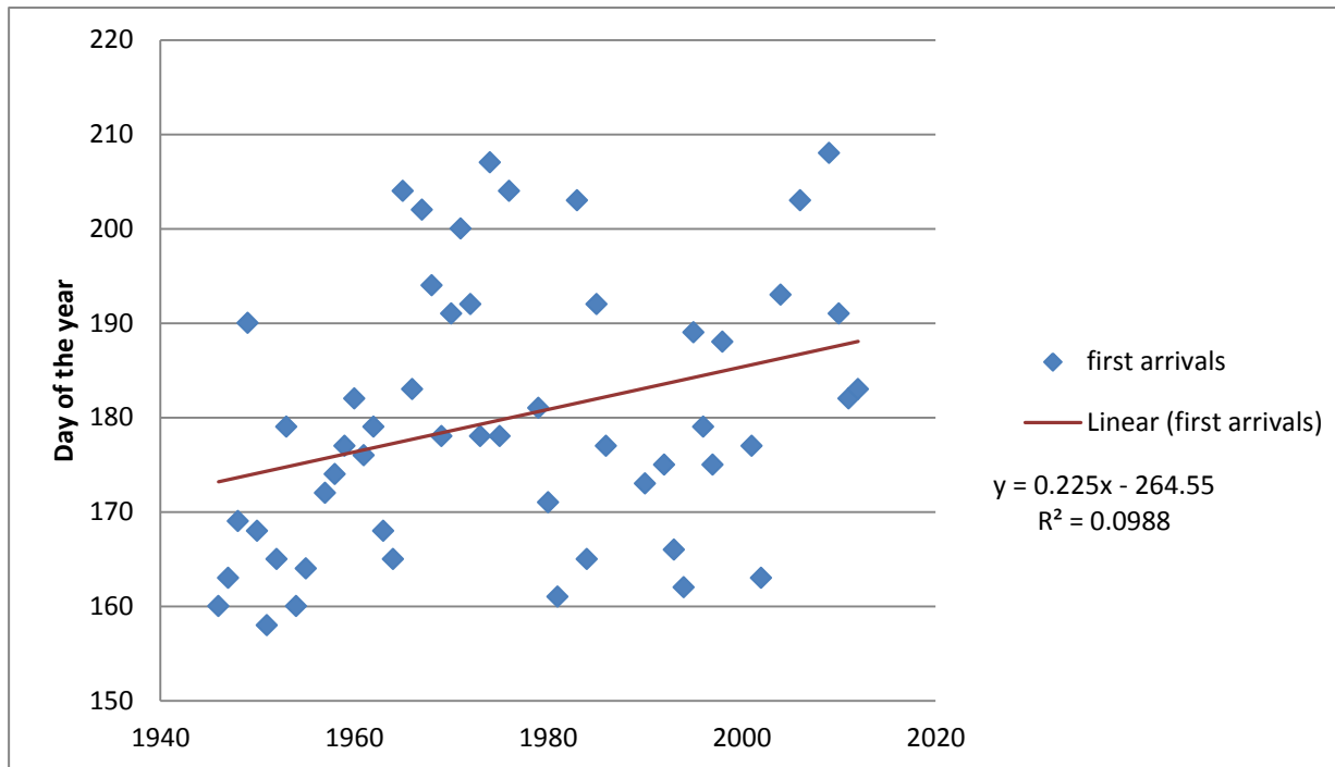
Figure 20: Graphical representation of the first arrival times of the main shoal on the lower south coast of KZN, the period observed was between 1946 and 2012. Similarly to figure 17 in some years the main shoal failed to appear along the lower south coast and therefore were classified as a non-run, therefore there are fewer listed points as in figure 16.
