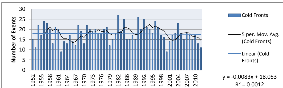
Figure 12: Total amount of mid latitude disturbances of each winter period from 1952-2010
