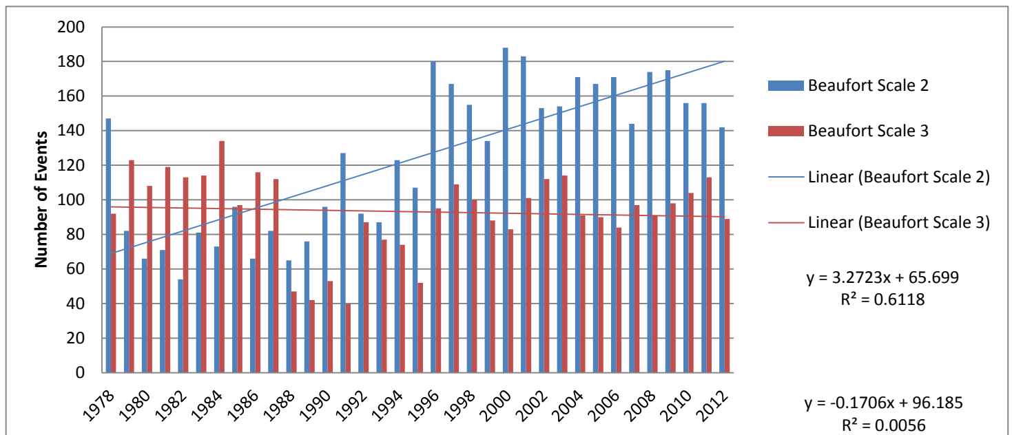
Figure 15: Category 2 and winter wind speed variability, Port Shepstone 1978-2012
