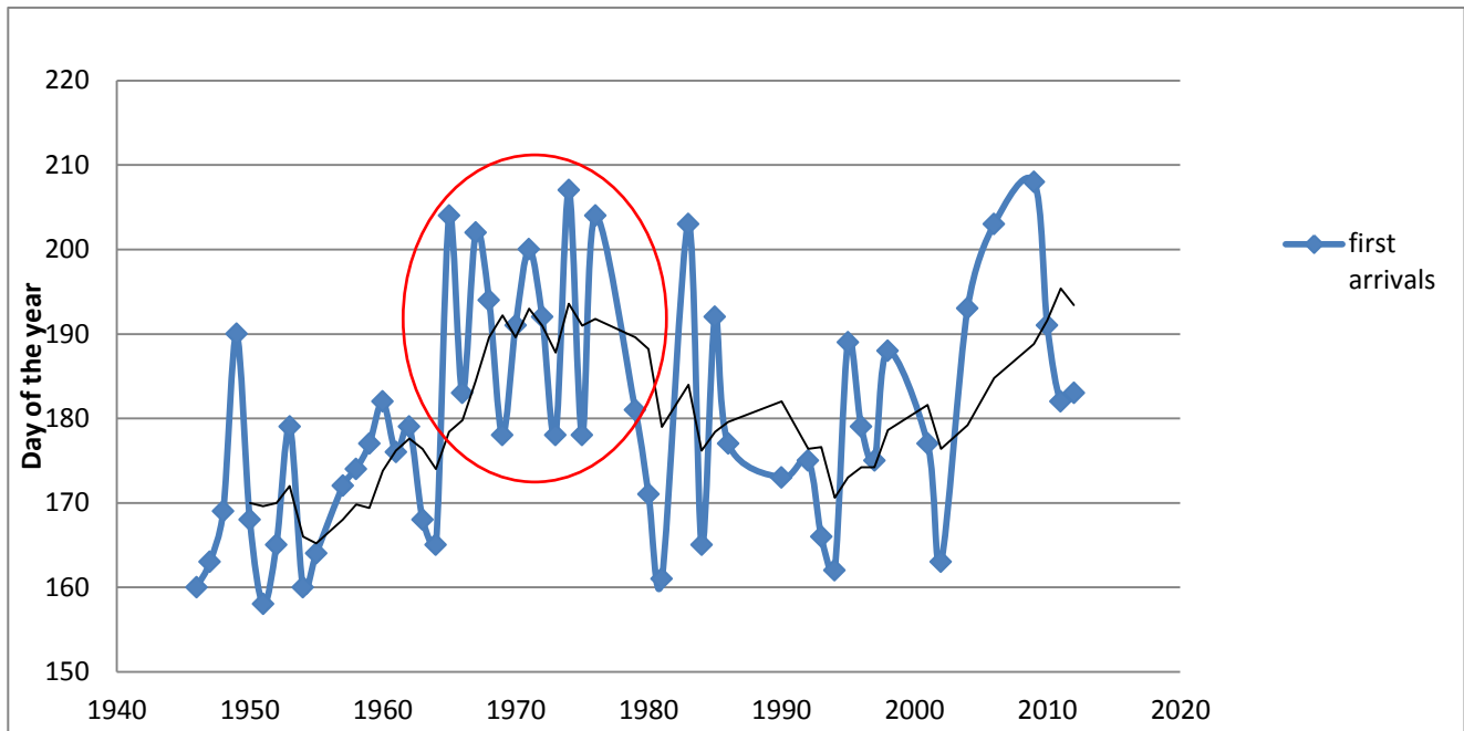
Figure24: Arrival times of the main shoal illustrating an important period between 1965-1979.
