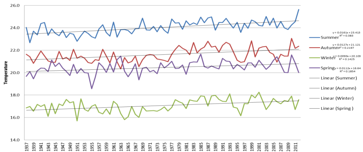
Figure 2: Seasonal changes in average temperature for Durban for the period between 1937 and 2012,
