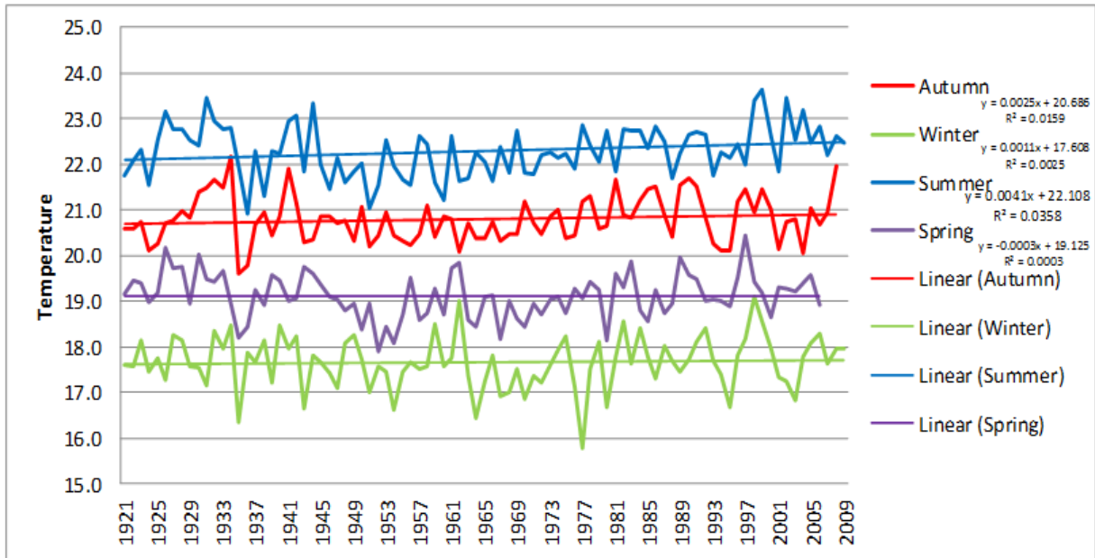
Figure 5: Seasonal changes in average temperature for Port St. Johns for the period between 1921 and 2012
