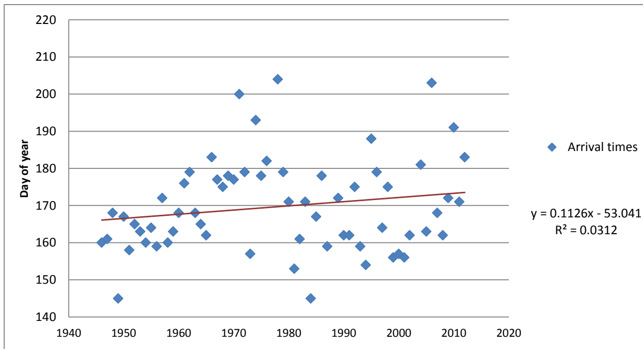
Figure 18: Graphical representation of the first arrival times of the sardine shoals that include the main and the pilot shoals. The runs were examined over a period of 66 years and started in 1946 and ended in 2012. The dates were selected based on which shoal arrived along the south coast of KZN first, whether it was the pilot or the main shoal and thus graphically depicted.
