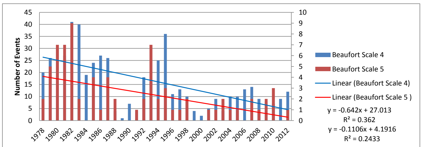
Figure 17: Category 4 and 5 annual winter wind speed variability, Port Shepstone 1978-2012
