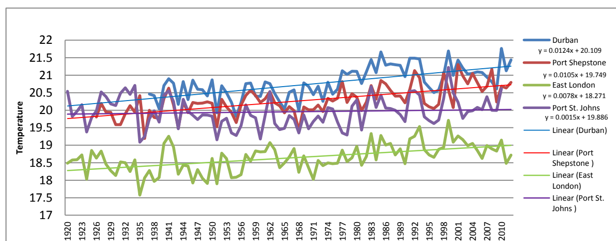
Figure 4: Annual average long term temperatures trends for the four climatic zones with a running mean of 11 years
