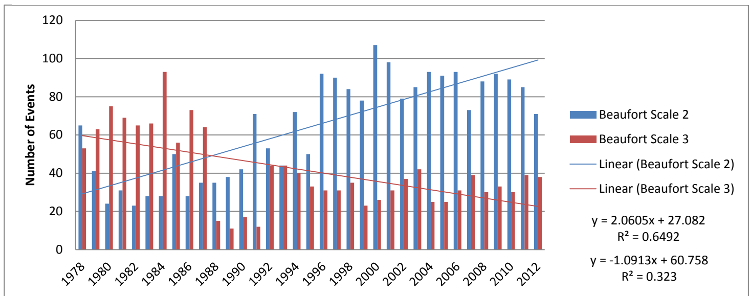
Figure 15: Category 2 and winter wind speed variability, Port Shepstone 1978-2012
