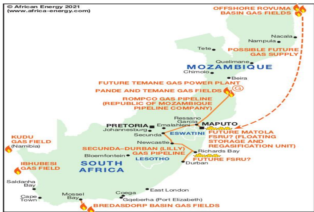
Figure 2.2: Cross border gas pipeline network
