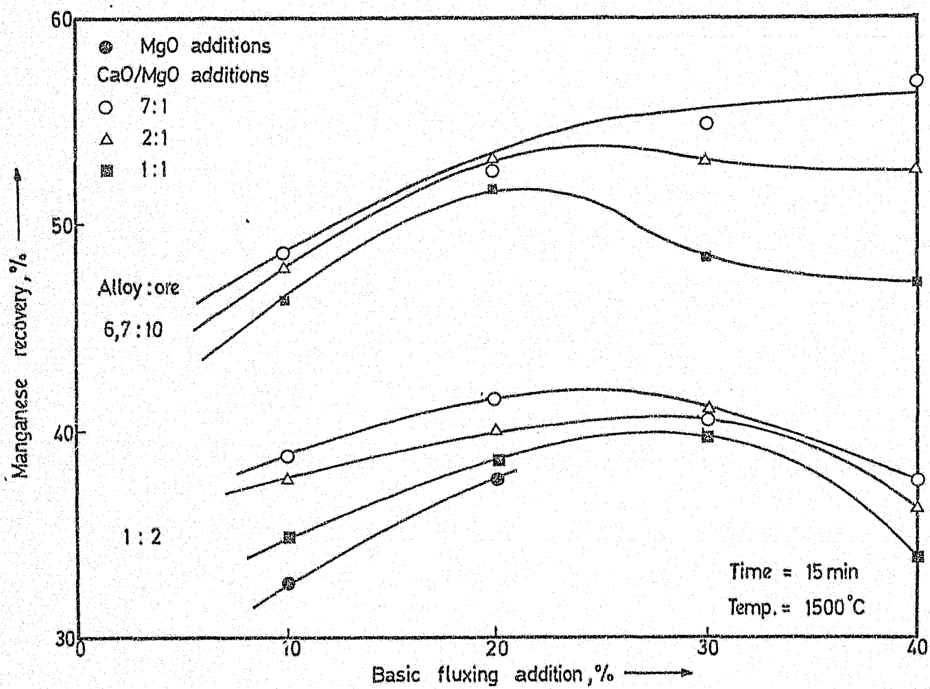
Figure 40. Effect of CaO-to-MgO ratio on manganese recovery.
