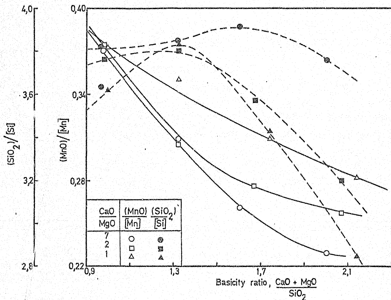
Figure 55. Effect of the replacement of CaO by MgO on the manganese distribution and silicon distribution ratios for a reaction with an alloy-to-ore ratio of 6,7 to 10.
