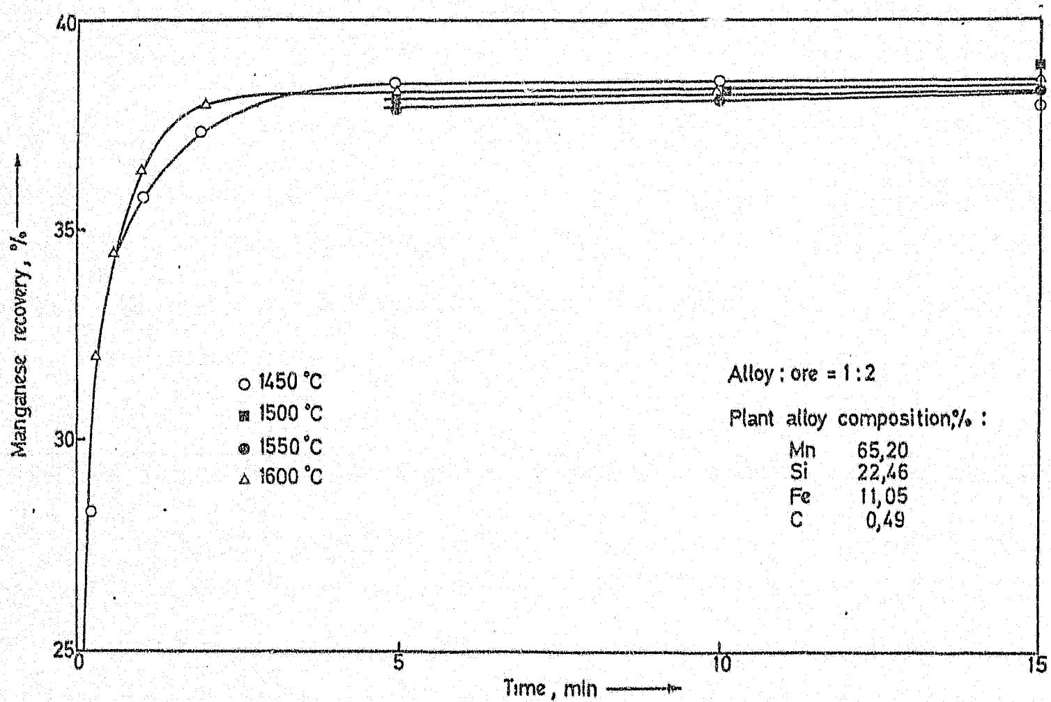
Figure 35 Manganese recovery with time for various initial reaction temperatures.
