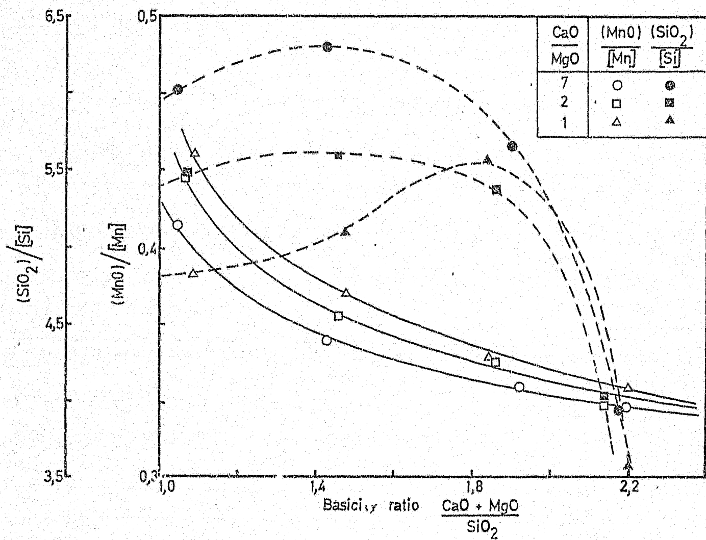
Figure 56. Effect of the replacement of CaO by MgO on the manganese distribution and silicon distribution ratios for a reaction with an alloy-to-ore ratio of 1 to 2.
