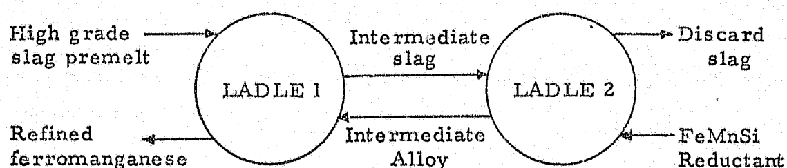
Figure 59. A two-stage refining process after Barcza (67) .
