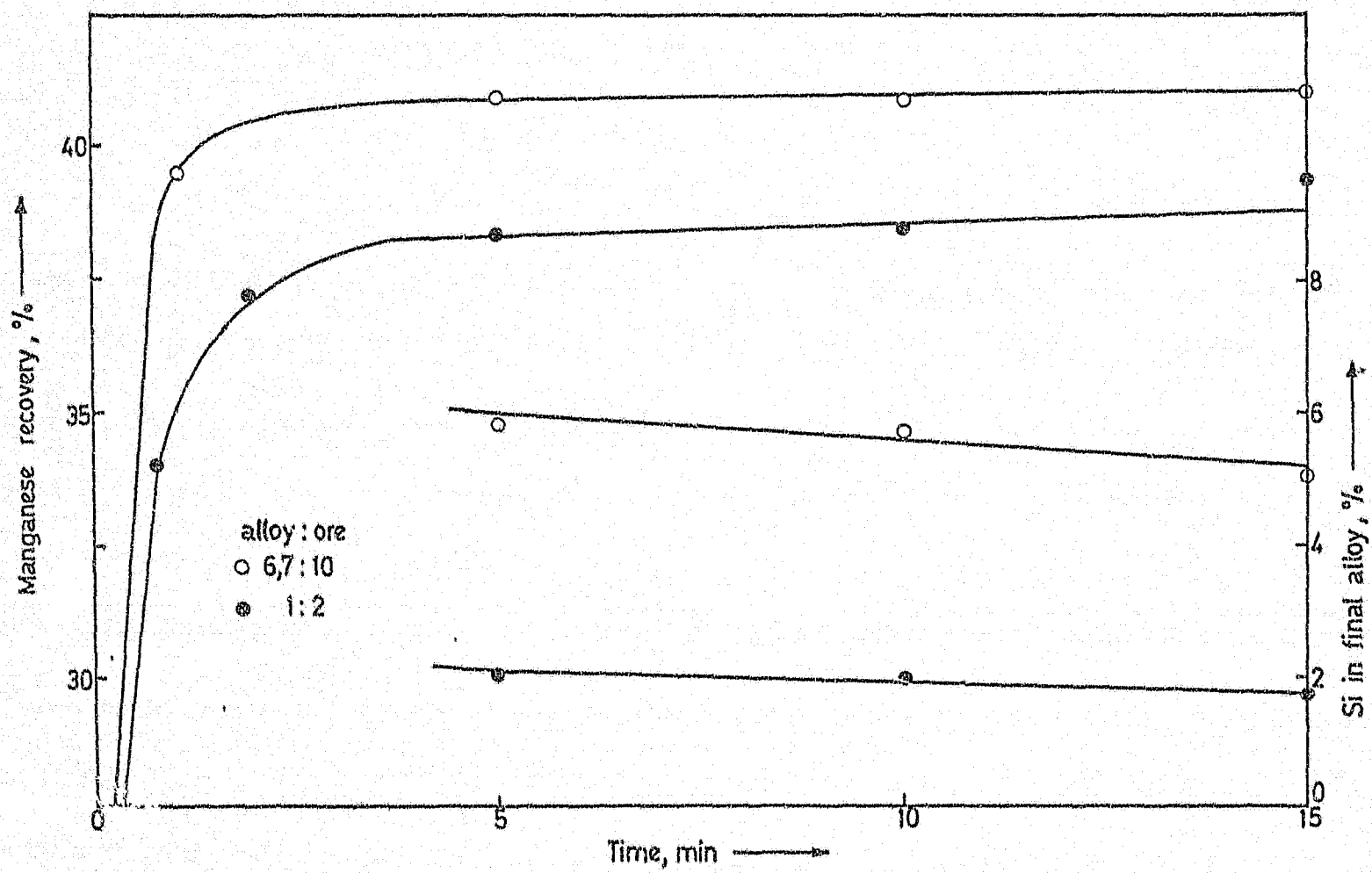
Figure 36. Effects of variations in the alloy:ore ratio on the change in manganese recovery with time at 1500°C.
