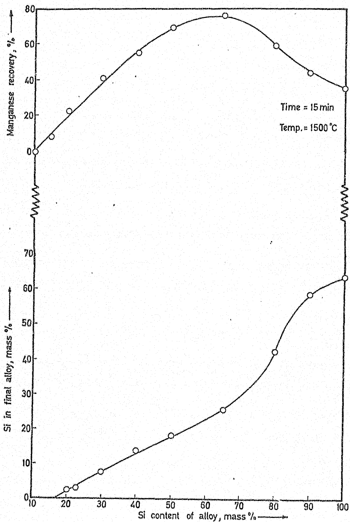
Figure 44 Manganese recovery and final alloy silicon content using a 1 to 2 alloy-to-ore ratio.
