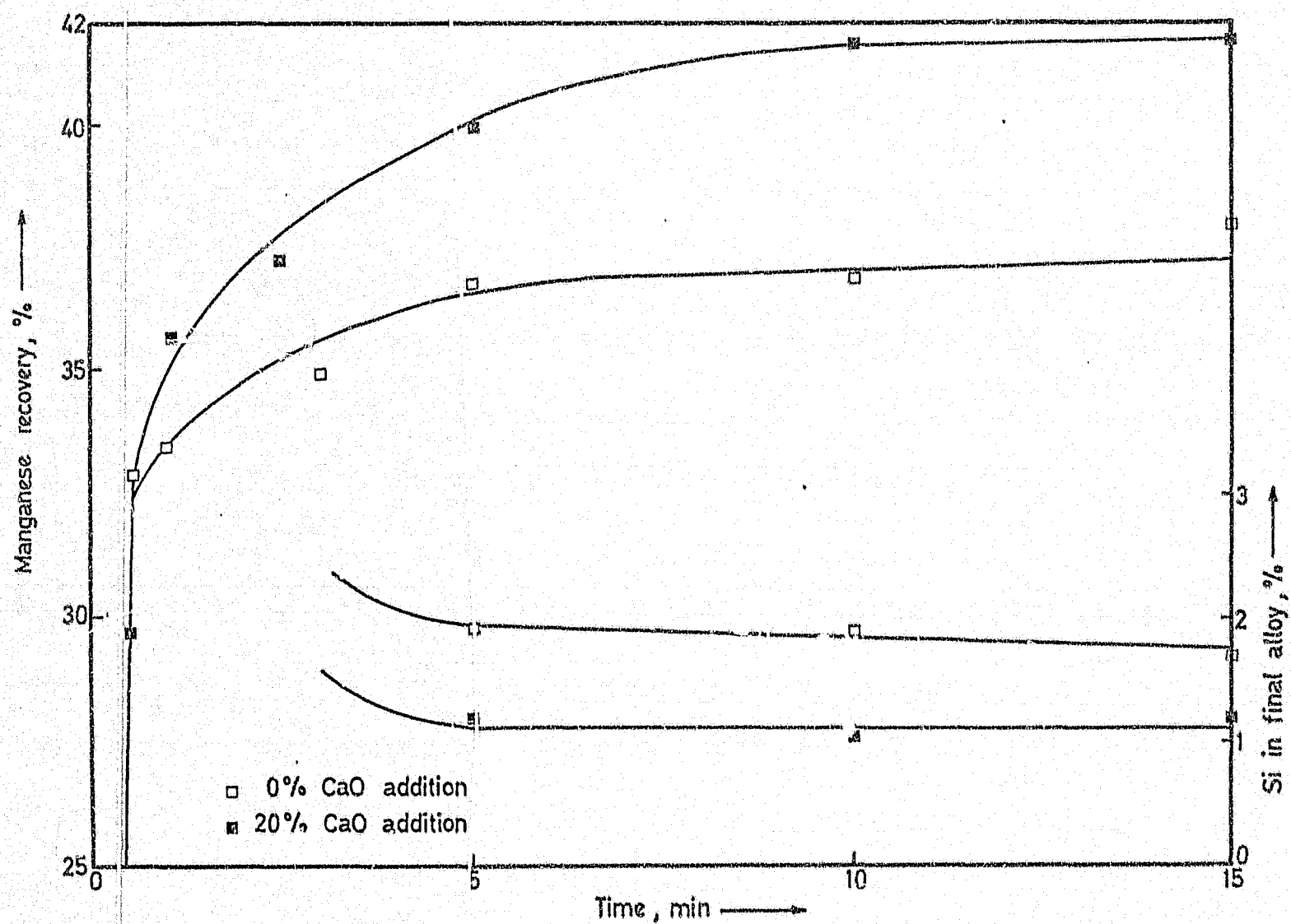
Figure 37. Reactions at 1500°C for a plant alloy-to-ore ratio of 1 to 2
