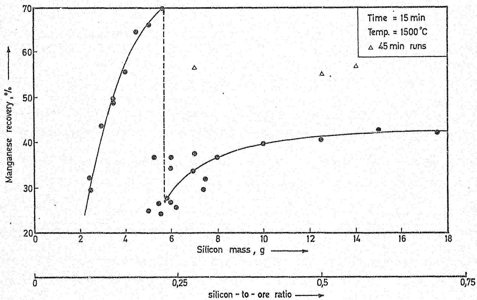
Figure 49. The variation of manganese recovery when silicon is used as reducing agent.
