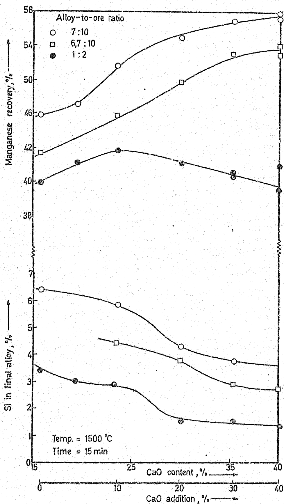
Figure 39. Effect of CaO on manganese recovery and the silicon content of the final alloy.
