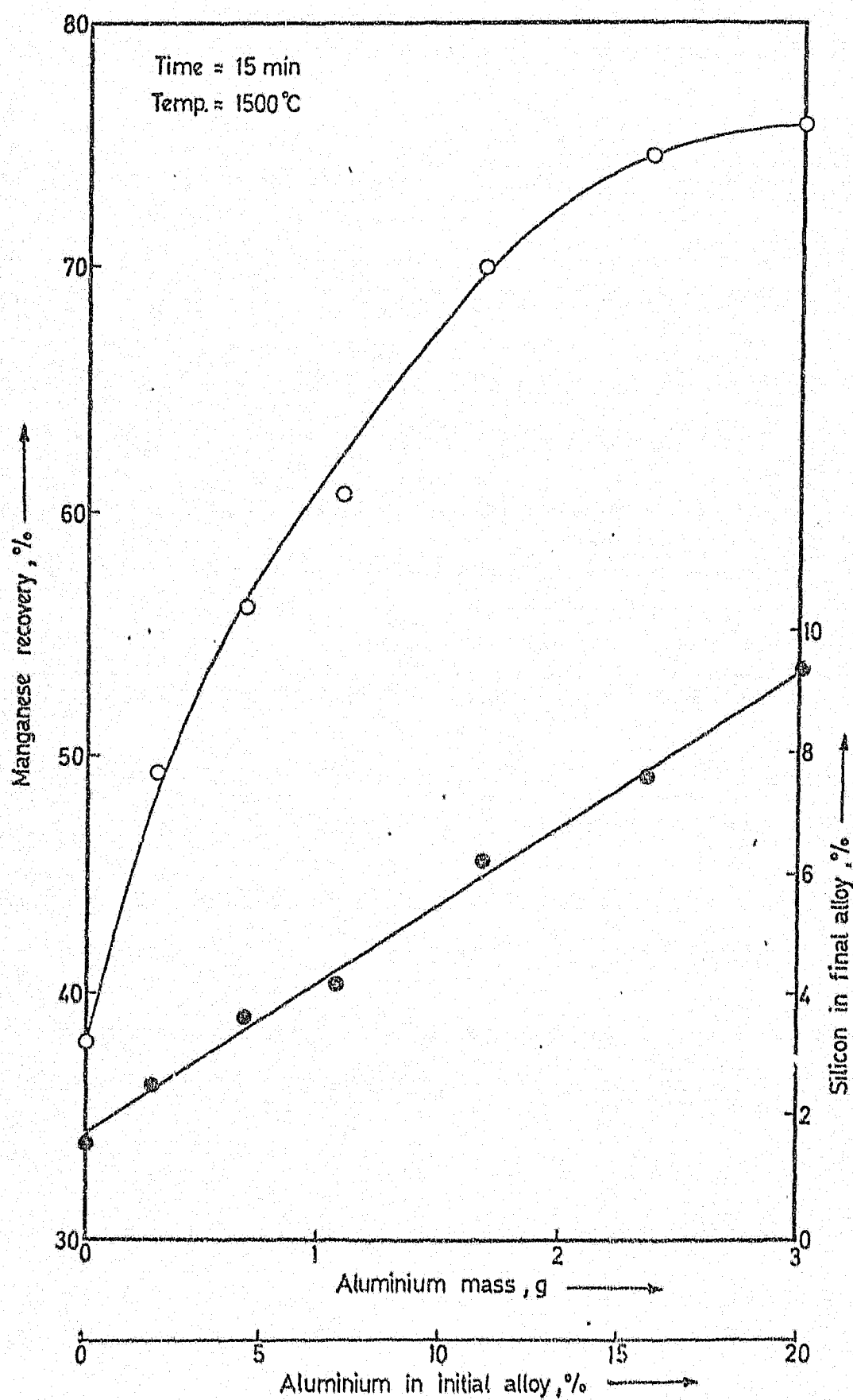
Figure 51. Manganese recovery related to aluminium addition. Samples contained the mass of silicon as used in the experiments with a 1 to 2 alloy-to-ore ratio where a plant alloy was utilized (22, 46% Si).
