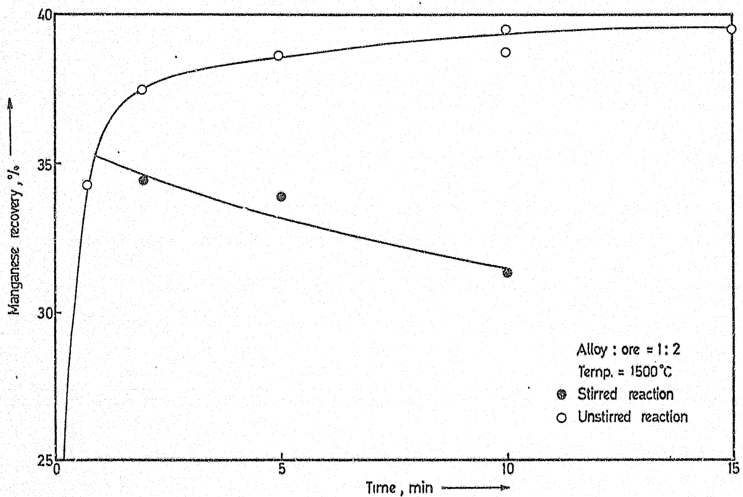
Figure 52. Effect of stirring on the non-fluxed reaction using plant ferromanganese-silicide.
