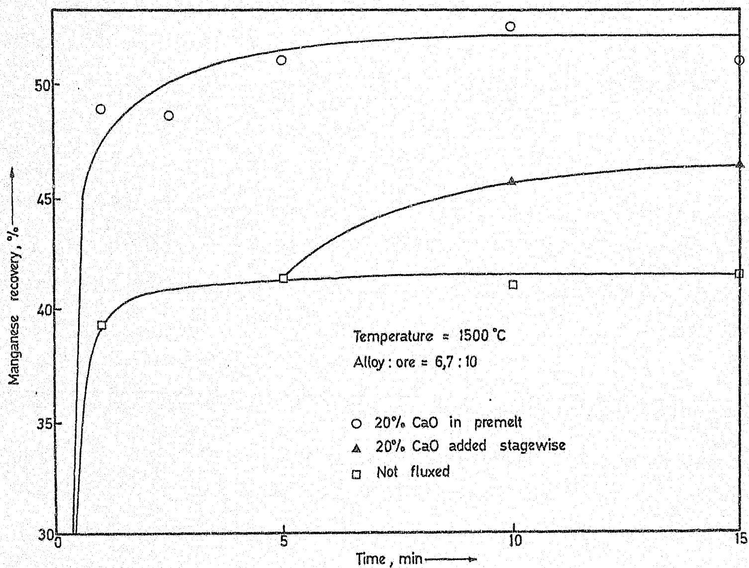
Figure 38. Variation of manganese recovery with time using a stoichiometric amount of FeMnSi.
