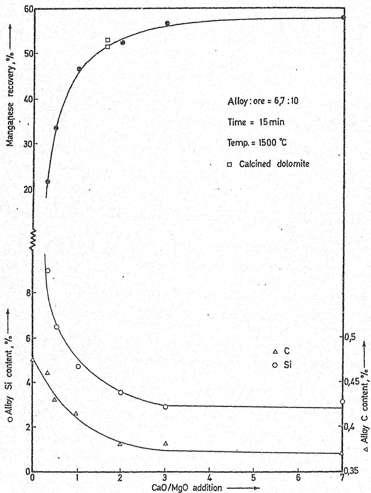
Figure 41. Silicon and carbon content of the final alloy corresponding to the manganese recovery shown.
