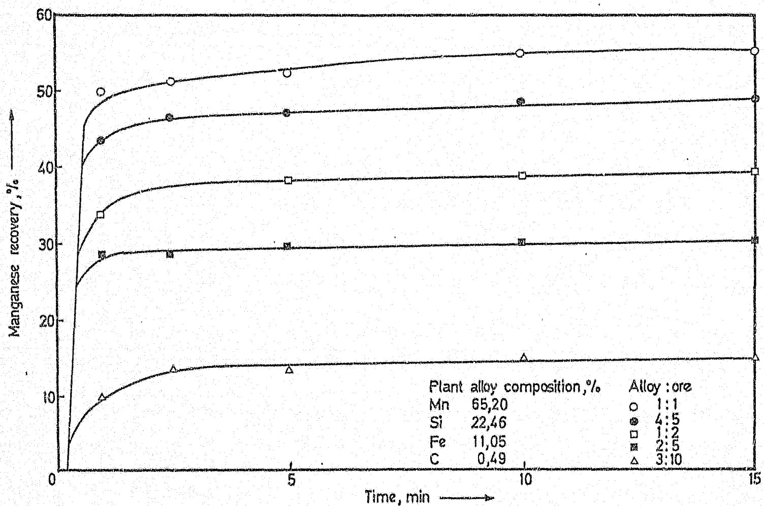
Figure 43. Increase in manganese recovery with time for increases in plant alloy-to-ore ratio without fluxing additions at 1500°C.
