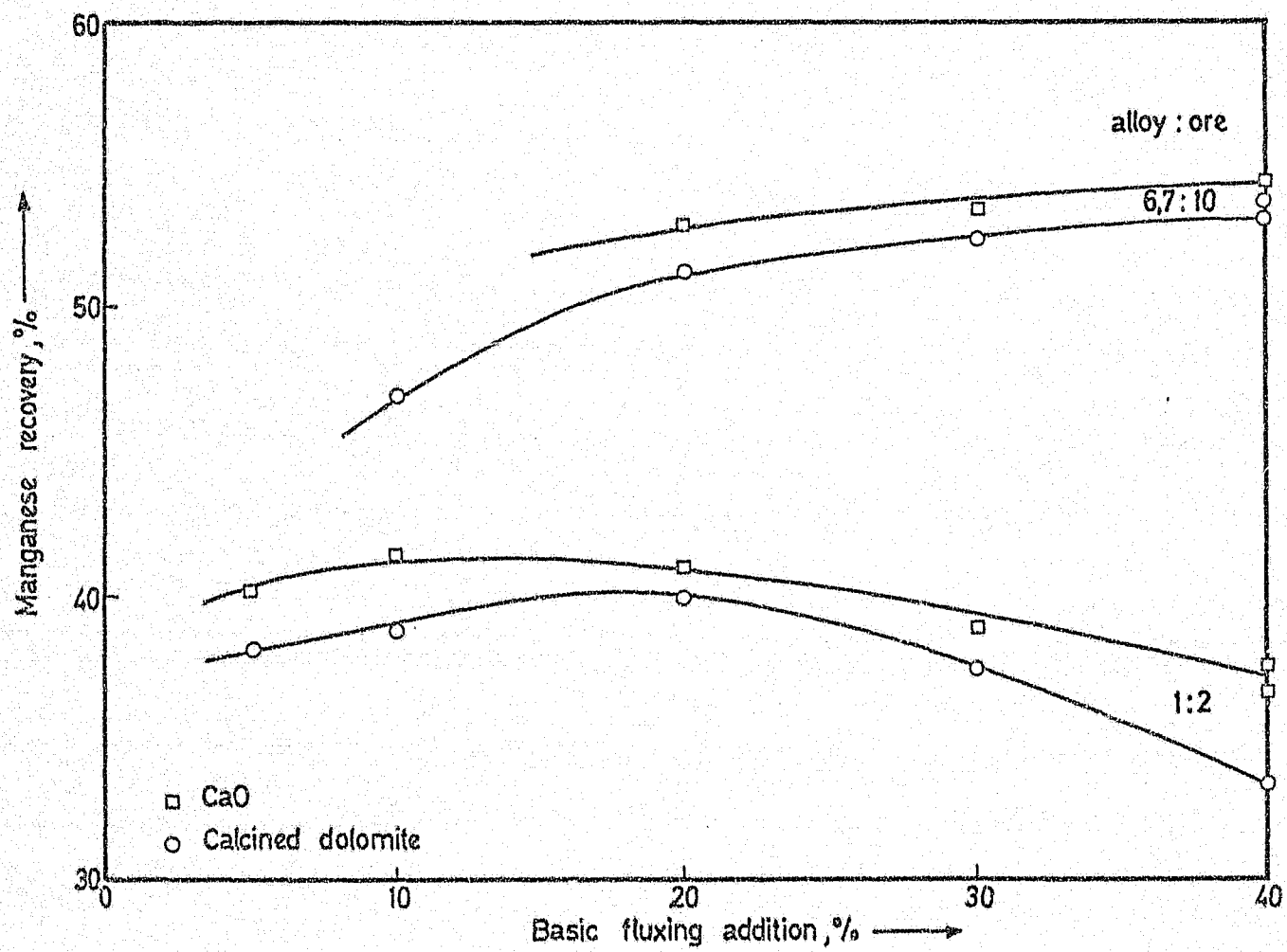
Figure 42. Comparisons of manganese recoveries when lime and calcined dolomite are used as fluxes.
