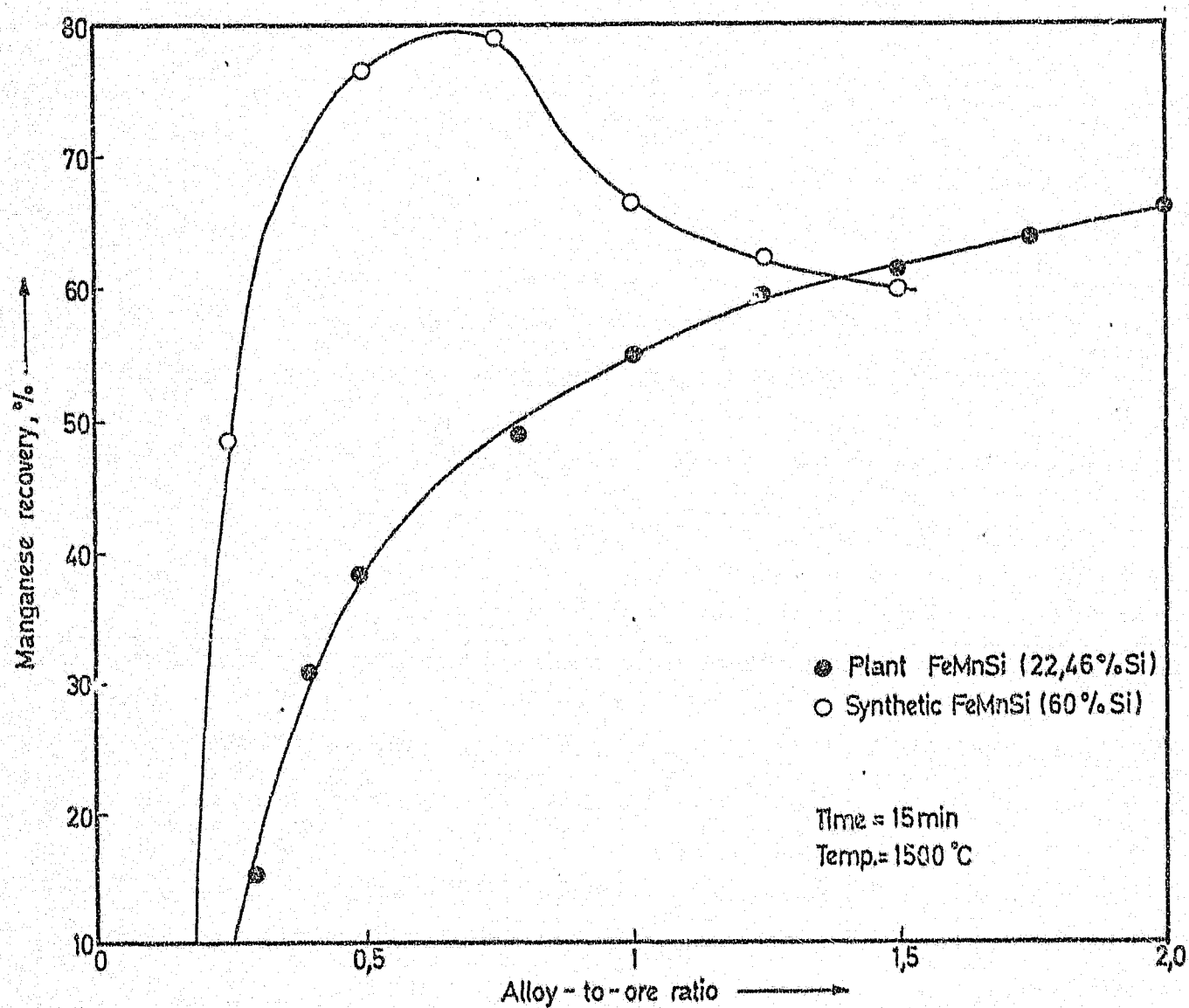
Figure 45. Comparison of manganese recovery using two ferromanganese-silicide reducing alloys.
