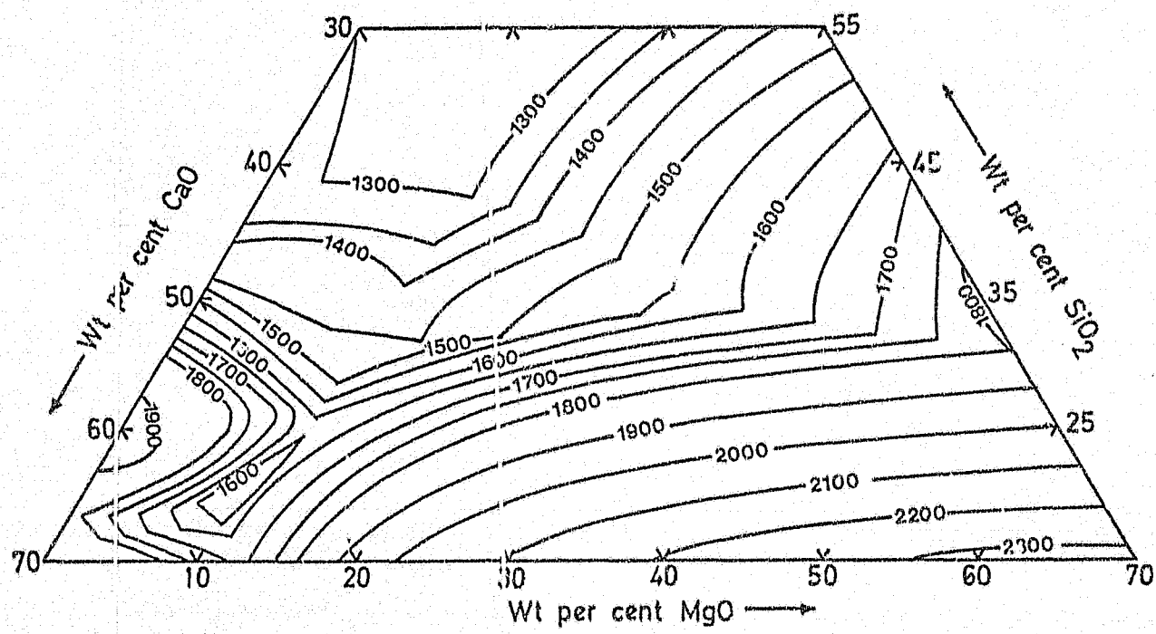
Figure 57. Liquidus diagram for the 15 mass per cent \text{Al}_2\text{O}_3 plane in the \text{CaO-MgO-Al}_2\text{O}_3\text{-SiO}_2 system after Osborn et al (134) .
