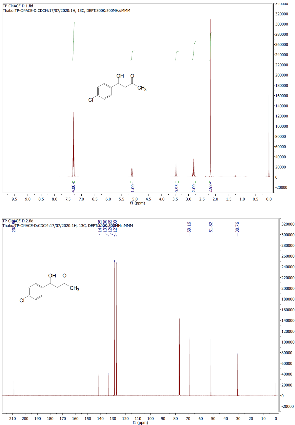
Figure S.4-3: ^1\text{H} and ^{13}\text{C} NMR spectra of the aldol product TP_A3Cl4ACE
