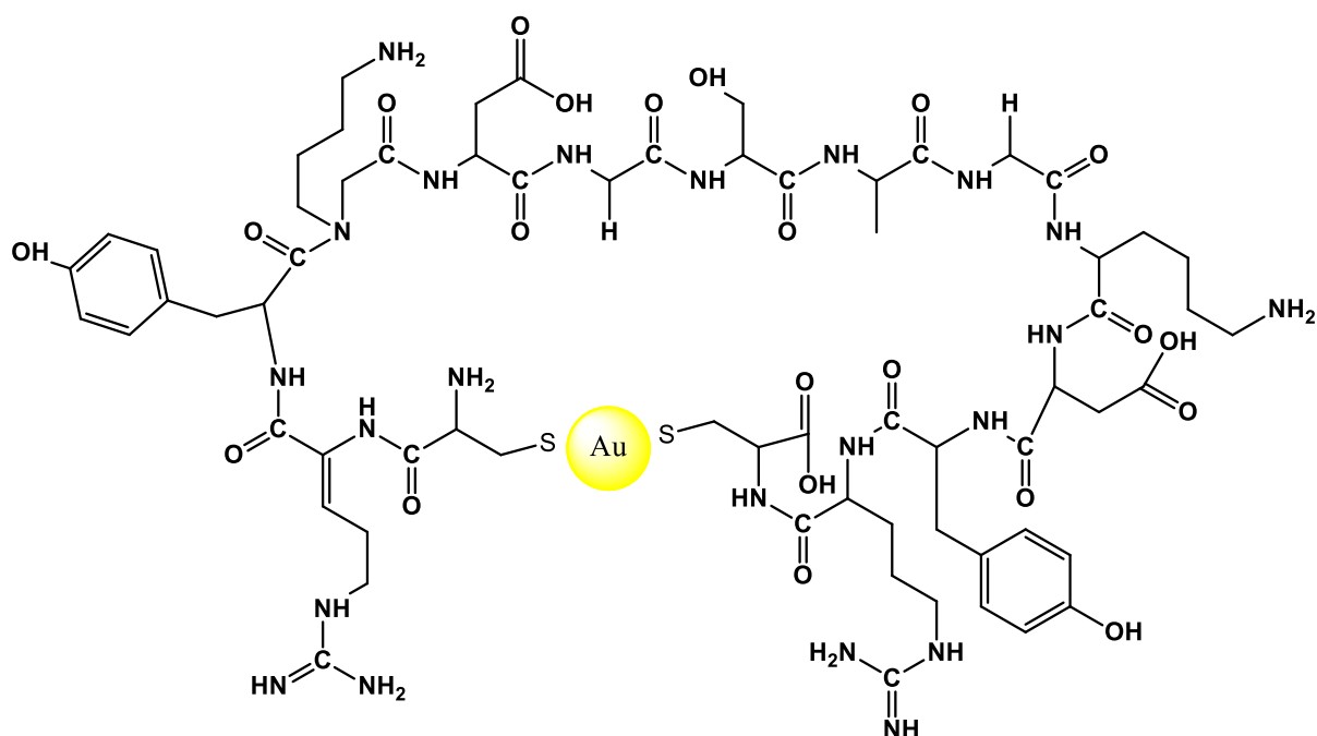
Figure 5- 1: Proposed structure of TP_ADLys peptide bounded to AuNP with its two cysteine residues.
