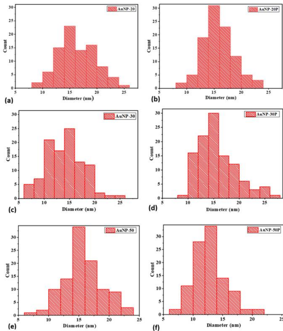
Figure 5- 5: Particle size distribution of citrate capped AuNPs and peptide-functionalised AuNPs obtained from TEM images.
