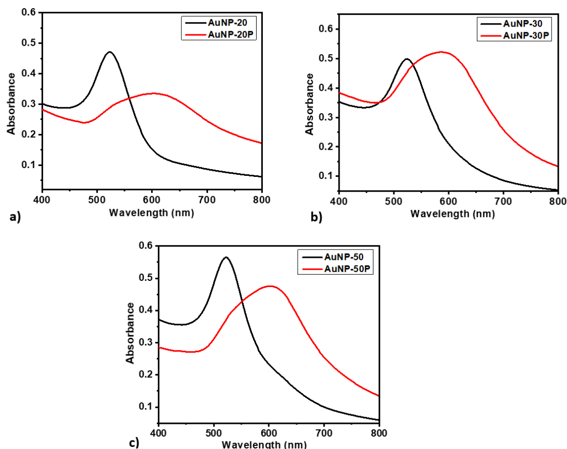
Figure 5- 3: UV-vis absorption spectra showing LSPR band for citrate-capped AuNP (black line) and peptide-AuNPs (red line).
