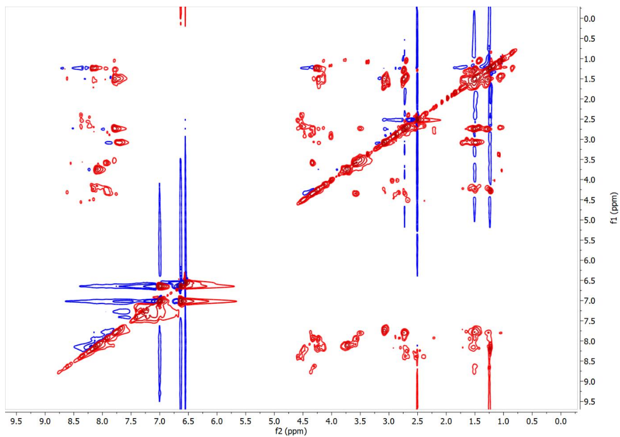
Figure S.3-18: 2D ^1\text{H} ROESY NMR spectrum of TP_ADlys peptide
