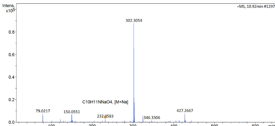
Figure 4- 2: LC-MS chromatograph depicting the formation of A1 product in 3 hours.
