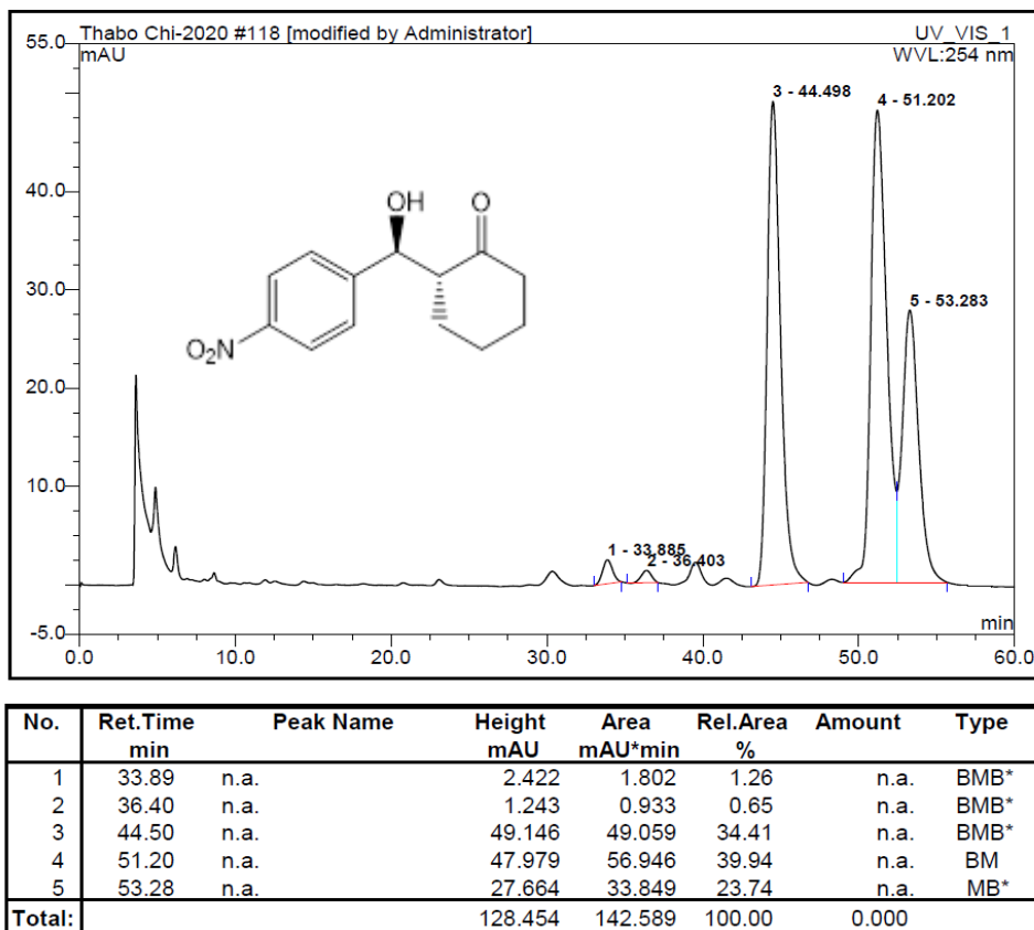
Figure S.4-20: Chiral HPLC chromatogram of TP_A4.10N4CY (entry 5)
