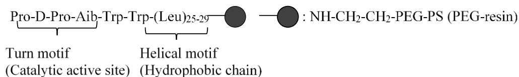
Figure 1- 8: Resin-supported peptide catalyst. 11
