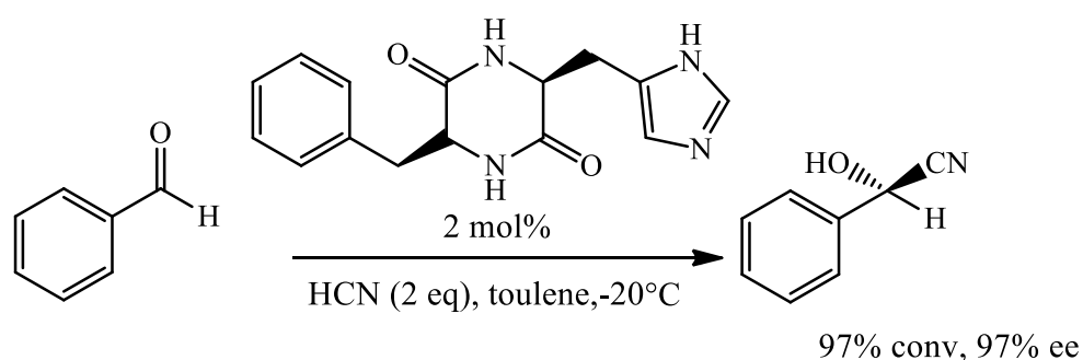
Scheme 1- 6: The asymmetric cyanation of benzaldehyde to a cyanohydrine. 84
