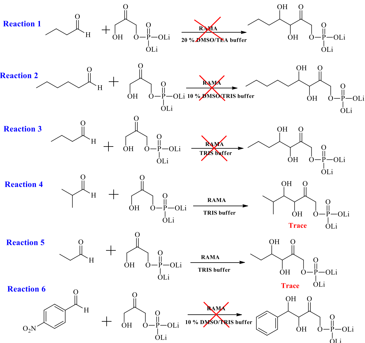
Scheme 4- 2: Aldol reactions catalyzed by RAMA using DHAP as a donor ketone: Reaction 1 , 1 mg RAMA, 20 % DMSO/TEA buffer (pH 7.0); Reaction 3-6 , 3 mg ( 9.5 \times 10^{-5} mol) RAMA, DHAP (0.05 mmol, 8.5 mg), TRIS-buffer pH 7.6, rt for 24-72 h.
