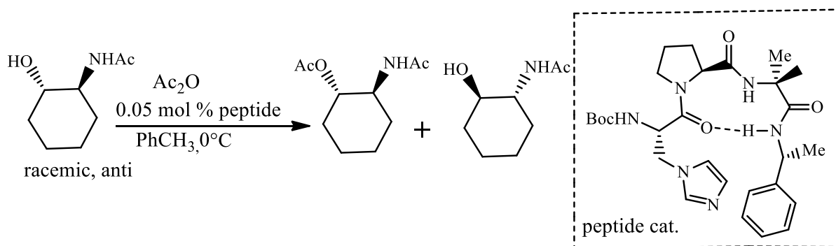
Scheme 1- 7: Peptide mediated kinetic resolution of functionalized racemic alcohols. 85
