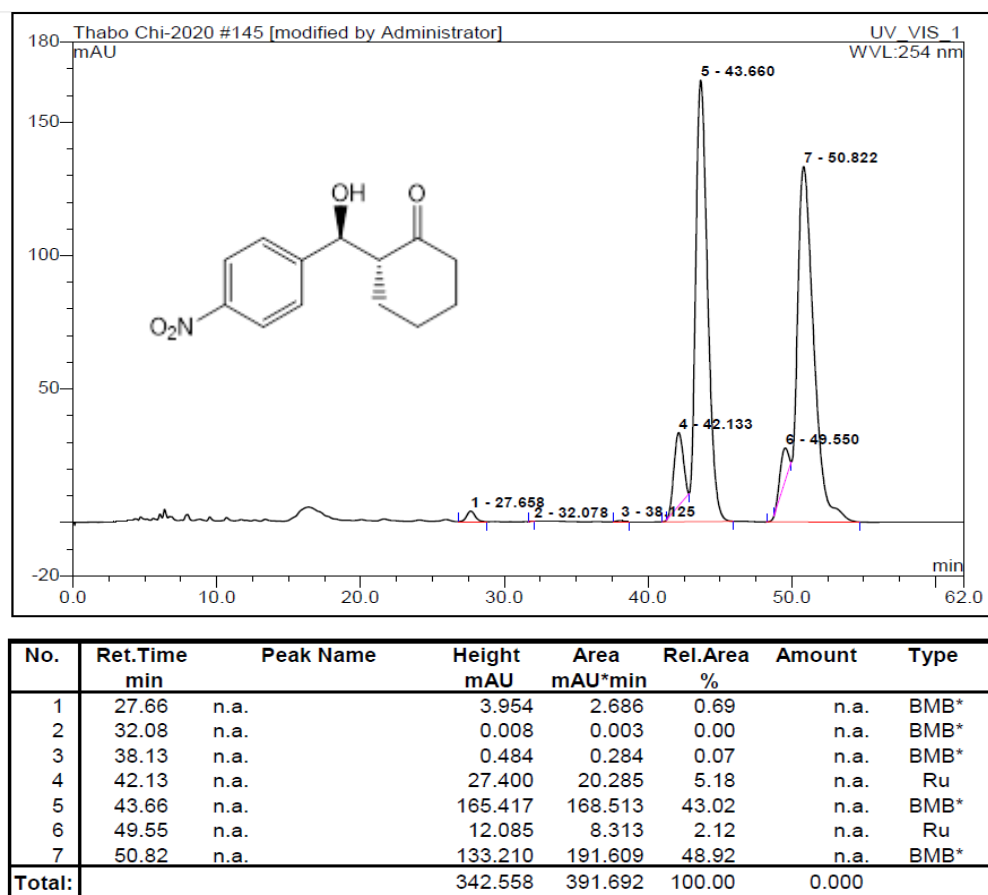
Figure S.4-23: Chiral HPLC chromatogram of TP_A4.14N4CY (entry 6)
