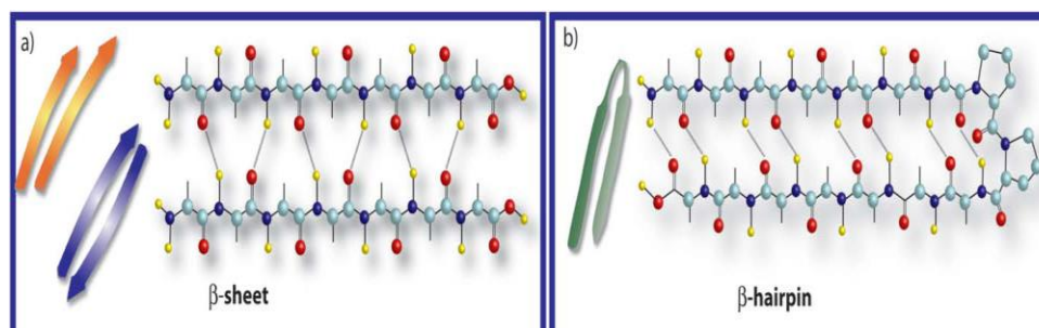
Figure 2- 7: Common peptide secondary structure conformations 54
