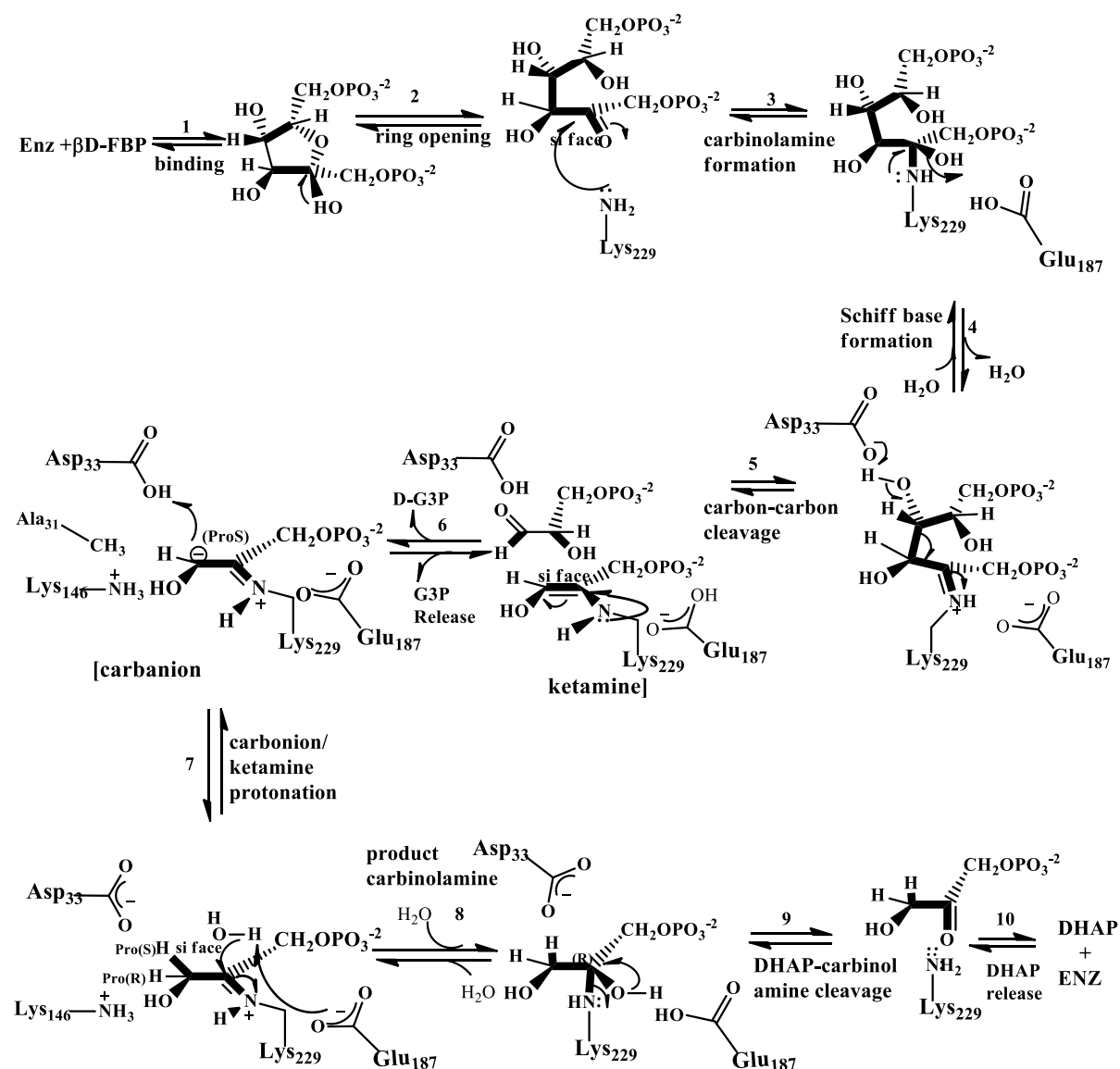
Scheme 1- 4: Mechanism of Fructose-1, 6-bisphosphate aldolase based on the structure of the DHAP Schiff-base intermediate. 62
