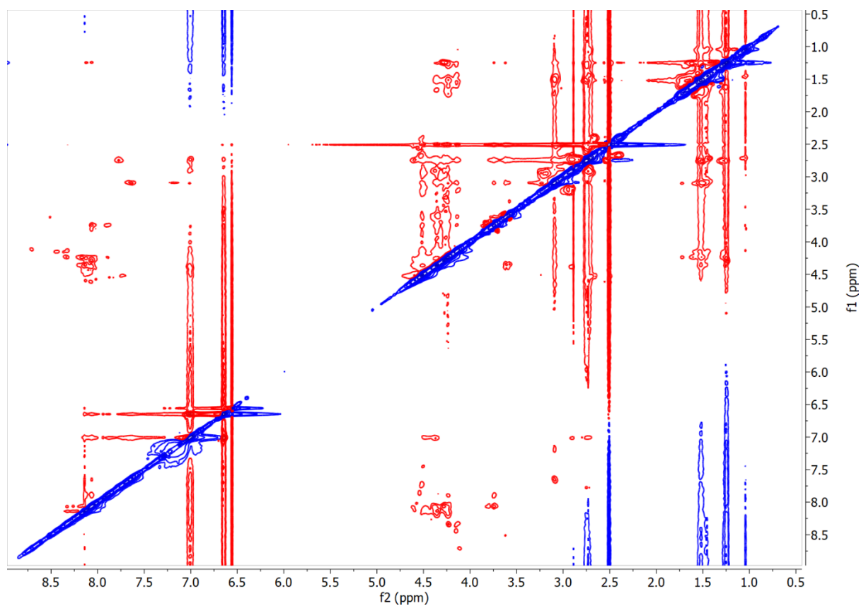
Figure-S.3-22: 2D ^1\text{H} ROESY spectrum of TP_ADlys peptide at 308K
