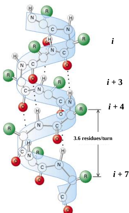
Figure 1- 3: An \alpha -helix that is stabilized by internal hydrogen bonding. 40
