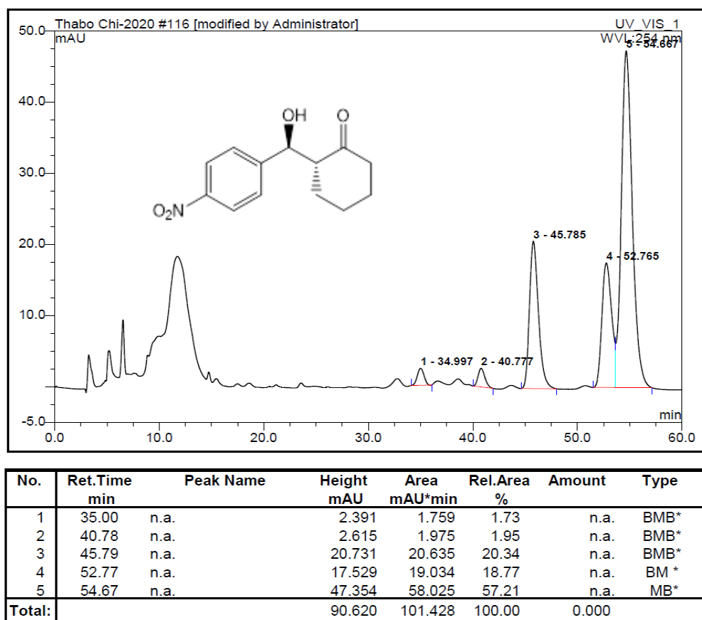
Figure S.4-22: Chiral HPLC chromatogram of TP_A4.13N4CY (entry 4)
