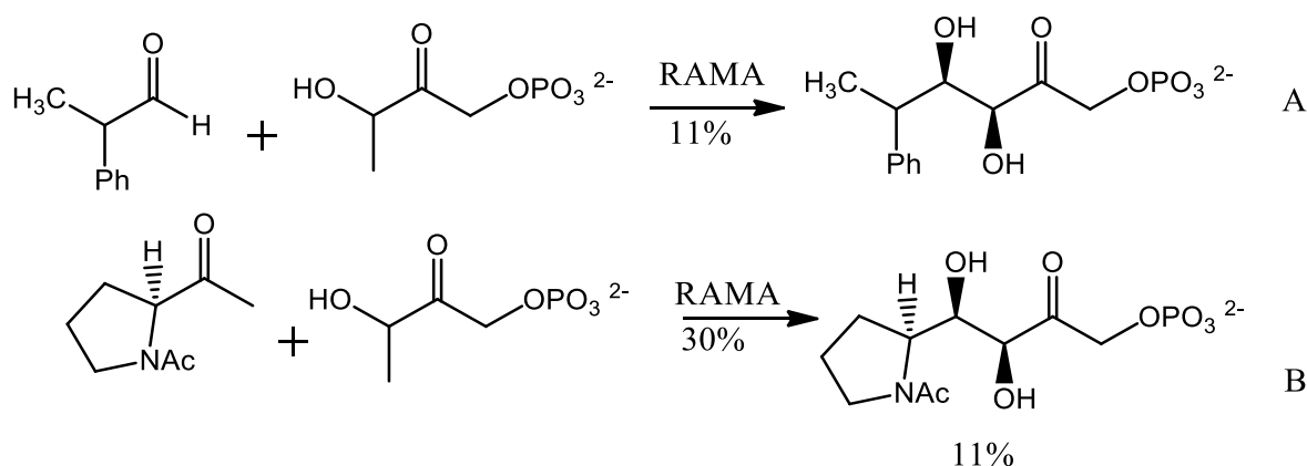
Scheme 4- 1: Aldol reaction between cyclic and linear aldehyde and DHAP using RAMA. 19
