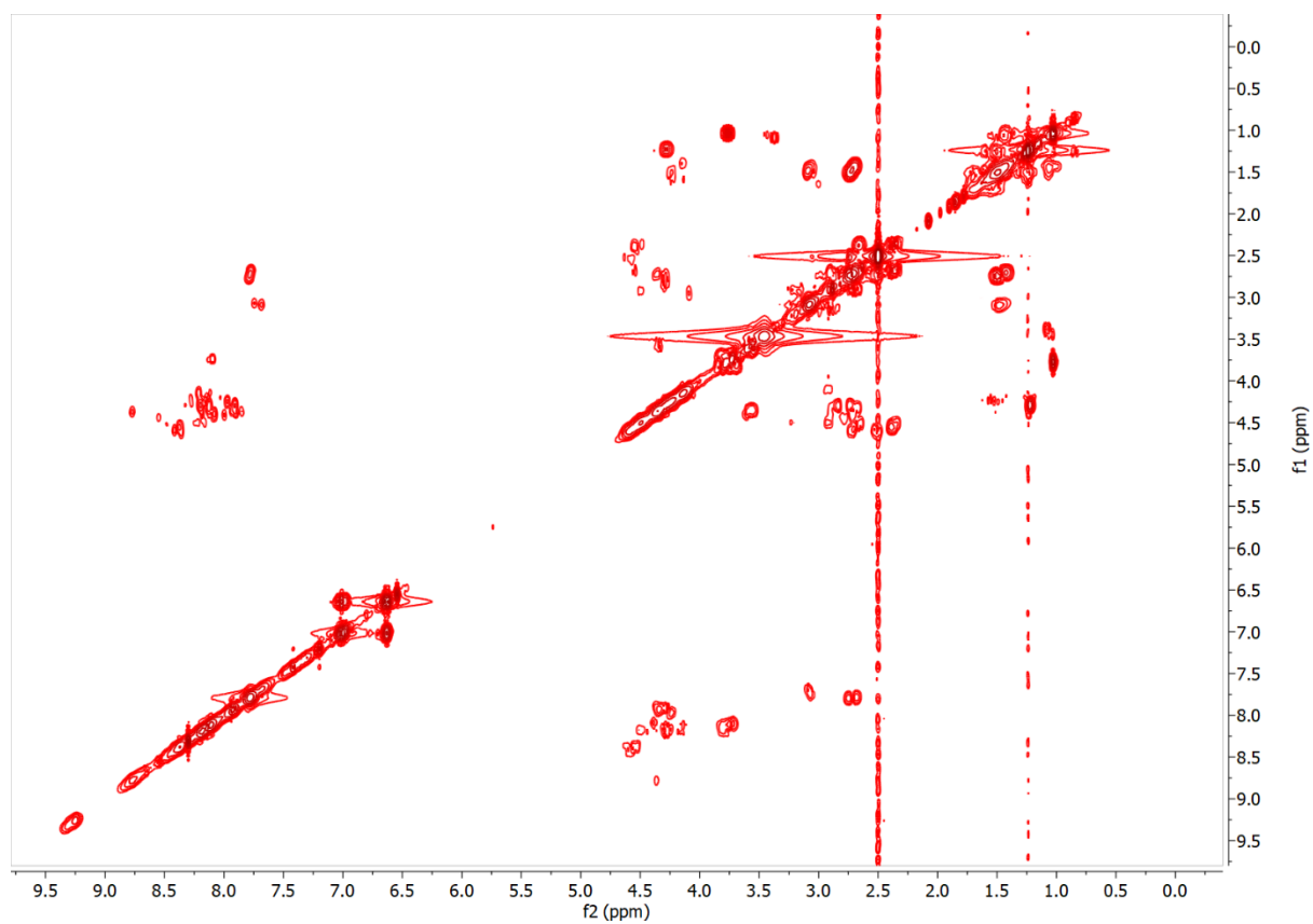
Figure S.3-4: 2D ^1\text{H} COSY NMR spectrum of TP_Asp peptide
