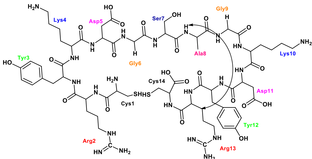
Figure 3- 6: TP_Asp peptide structure with arrows indicating long correlation using ROESY
