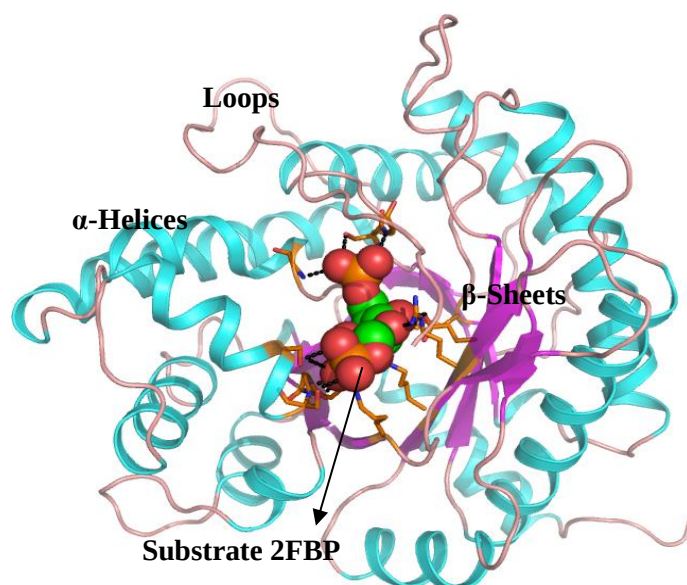
Figure 1- 2: Ribbon diagram of the crystal structure of aldolase enzyme depicting the \alpha -alpha helices (cerulean), \beta -sheets (purple), and active site residues bonded to the substrate (shown as spheres) [PDB code: 2ALD]
