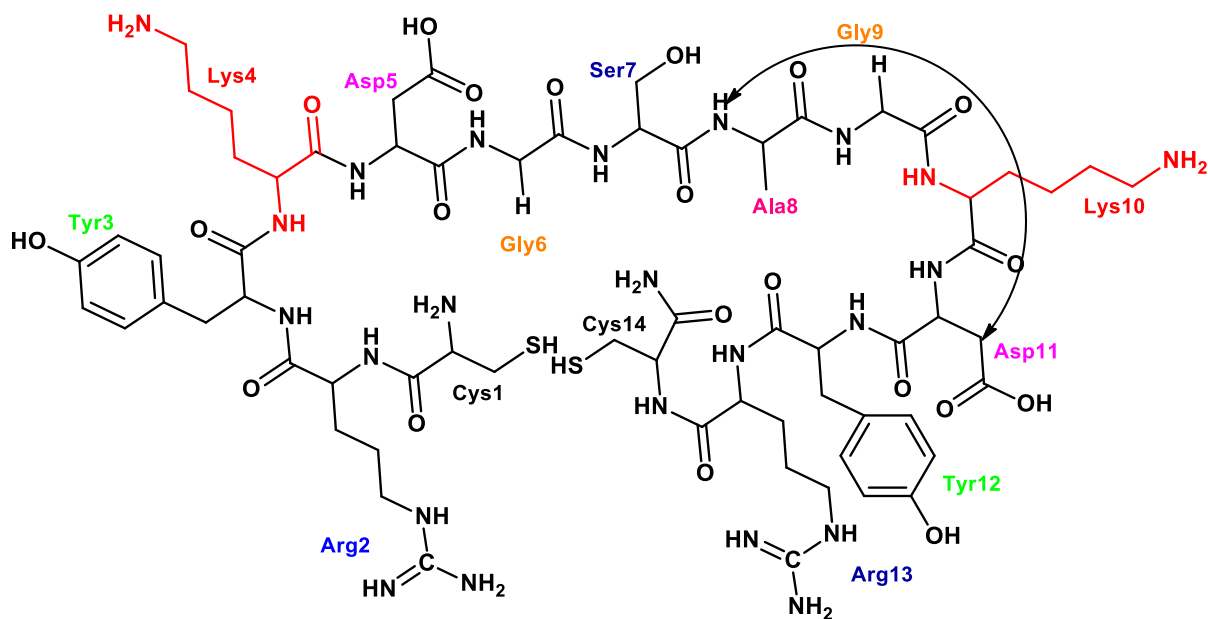
Figure 3-7: TP_ADLYs peptide structure with arrows indicating long correlations using ROESY NOEs (black lines)
