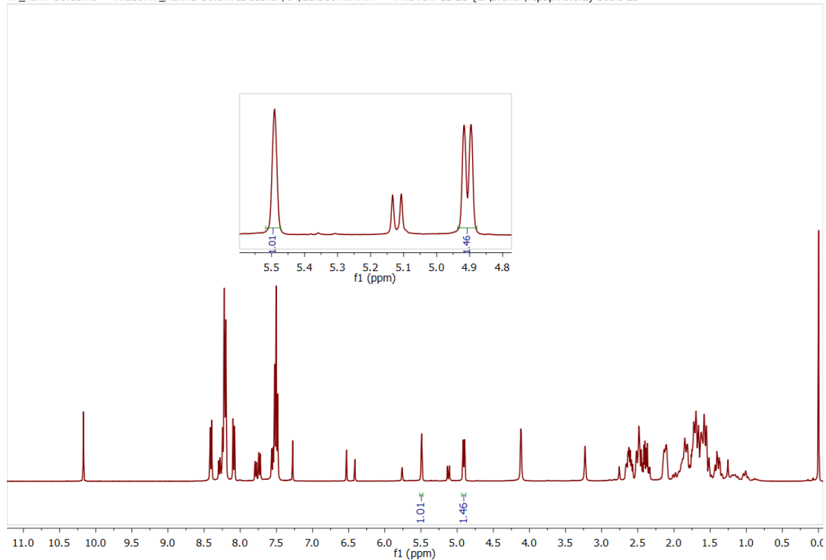
Figure S.4-53: ^1\text{H} NMR spectrum of the crude product TP_A4.24N4CY
