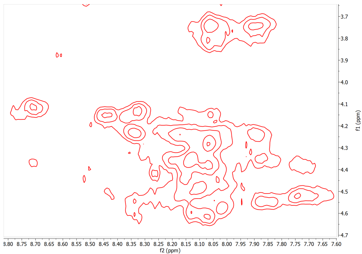
Figure S.3-23: 2D ^1\text{H} ROESY spectrum of TP_ADlys peptide, ^1\text{H} N fingerprint region at 308K.
