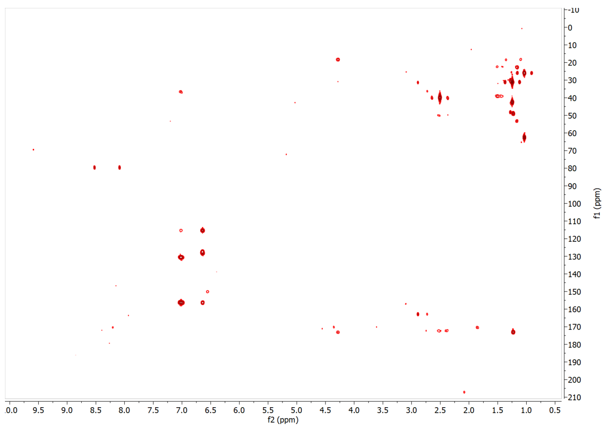
Figure S.3-7: HMBC NMR spectrum of TP_Asp peptide
