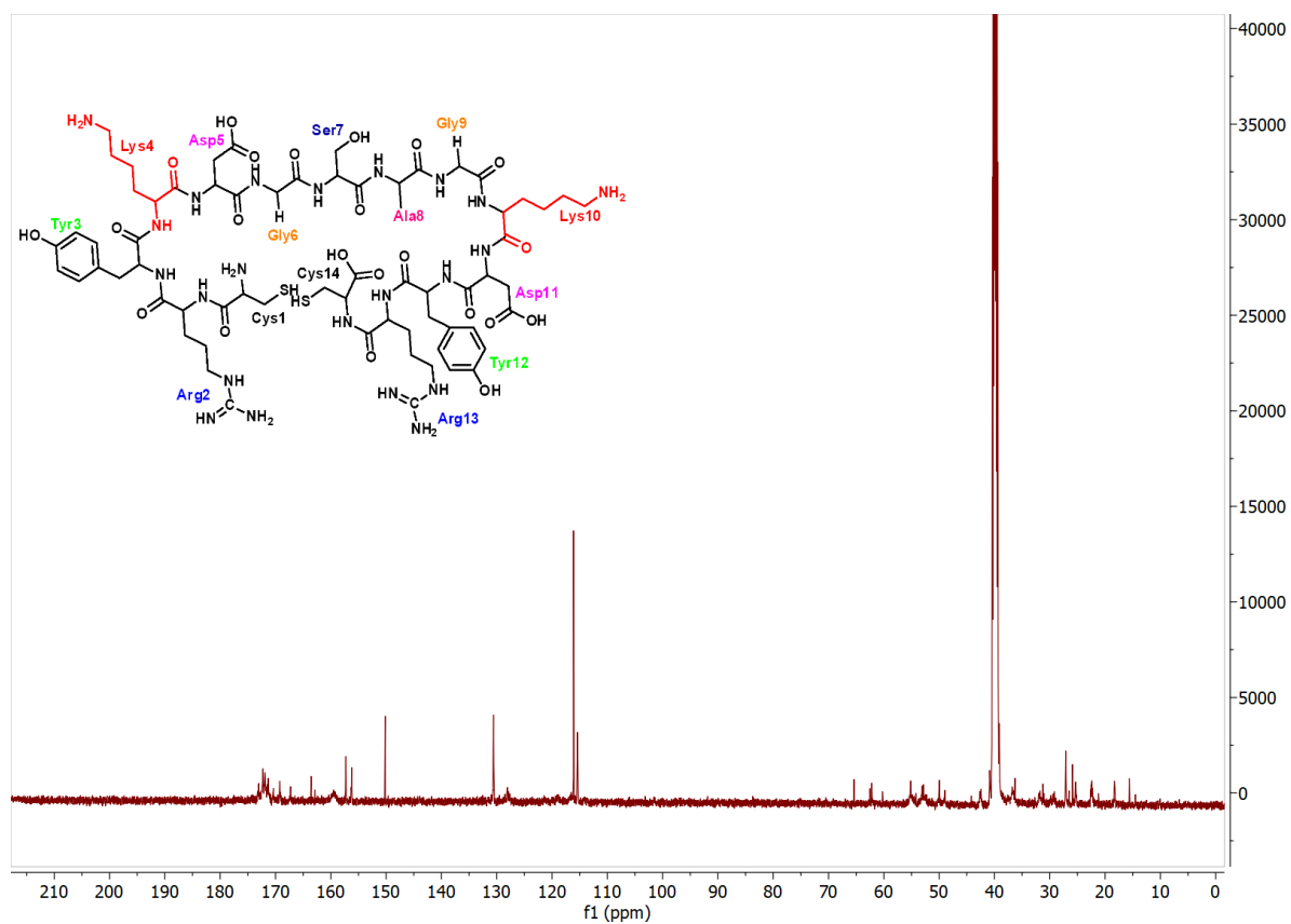
Figure S.3-11: ^{13}\text{C} NMR spectrum of TP_ADLYs peptide
