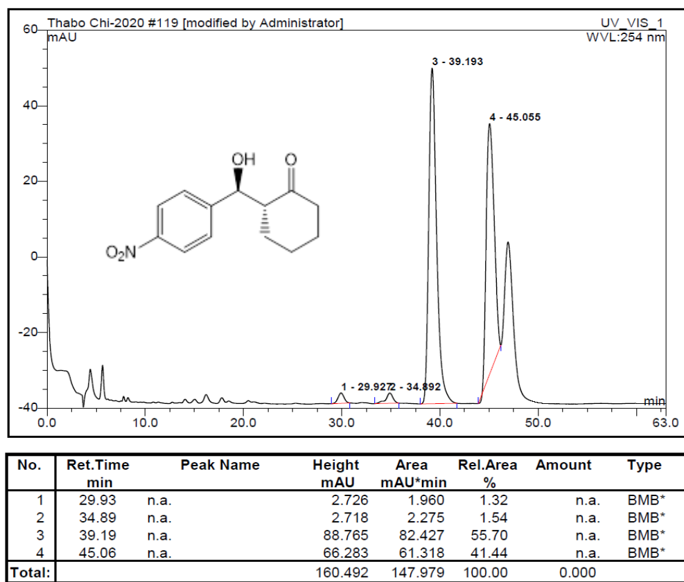
Figure S.4-16: Chiral HPLC chromatogram of TP_A4.4N4CY (entry 6)
