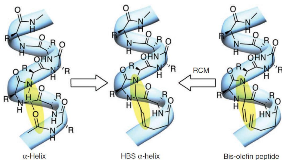
Figure 1- 9: An N-terminal hydrogen bond replace with C-C bond obtained from a ring closing metathesis (RCM) reaction. 95
