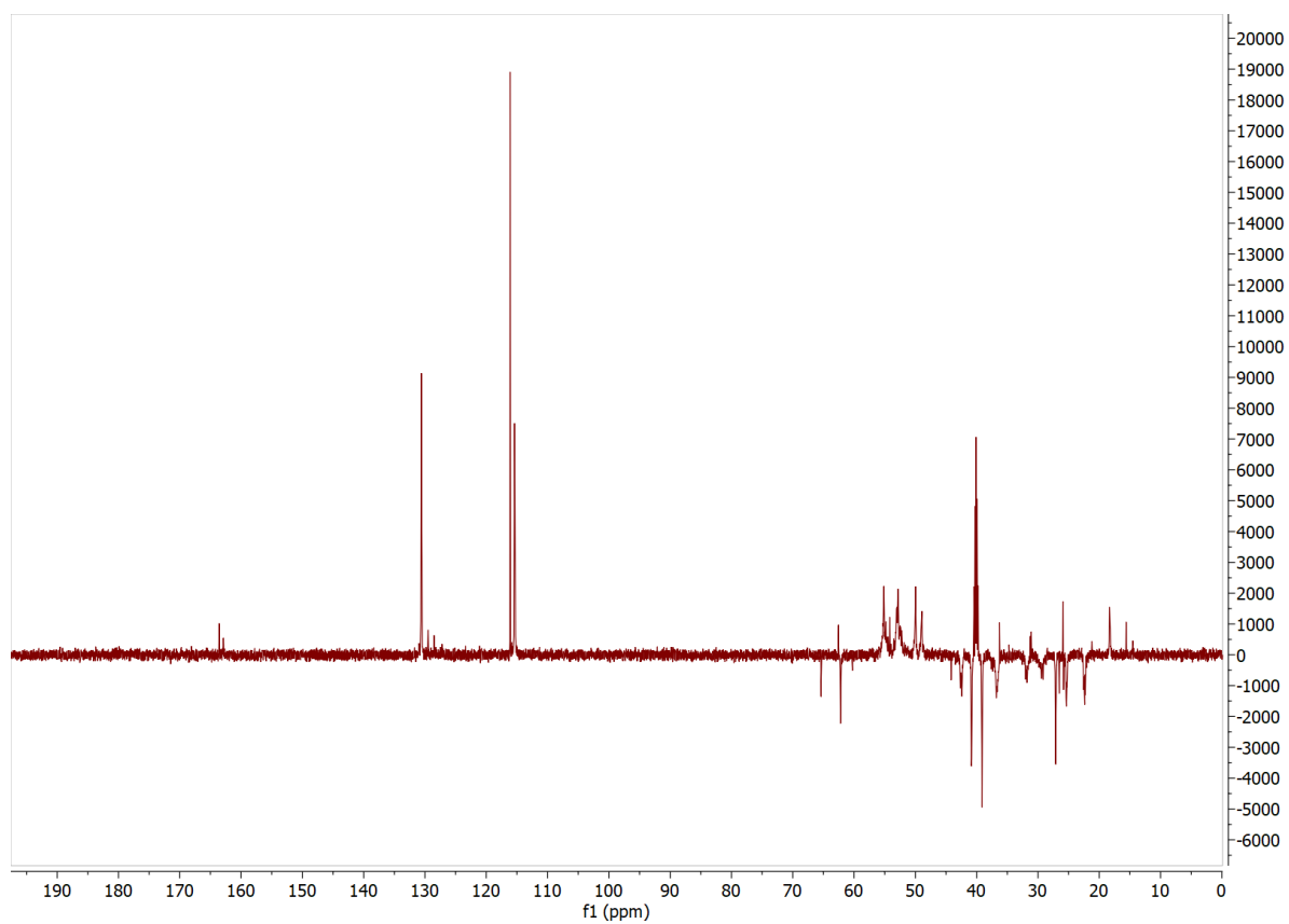
Figure S.3-12: DEPT 135 NMR spectrum of TP_ADLYs peptide
