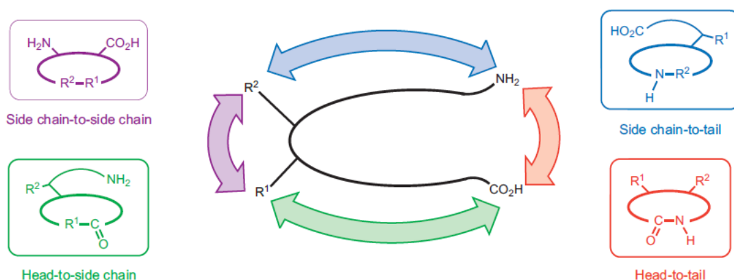
Figure 2- 9: Different ways of peptide cyclization. 59
