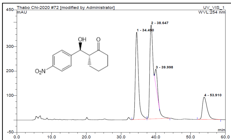
Figure S.4-R: Chiral HPLC chromatogram of racemate TP_A4N4CY-R12
