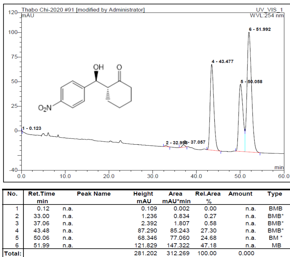
Figure S.4-31: Chiral HPLC chromatogram of TP_A4.22N4CY (entry 8)
