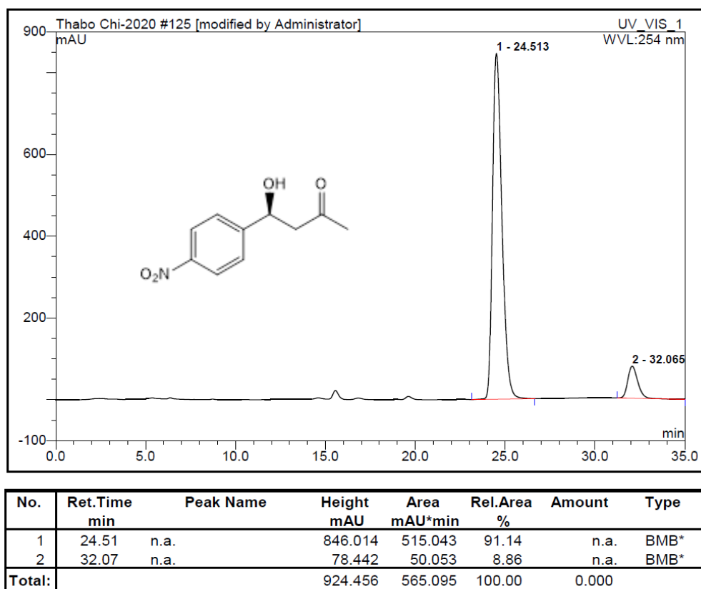
Figure S.4-8: Chiral HPLC chromatogram of TP_A1.2N4ACE (entry 4)
