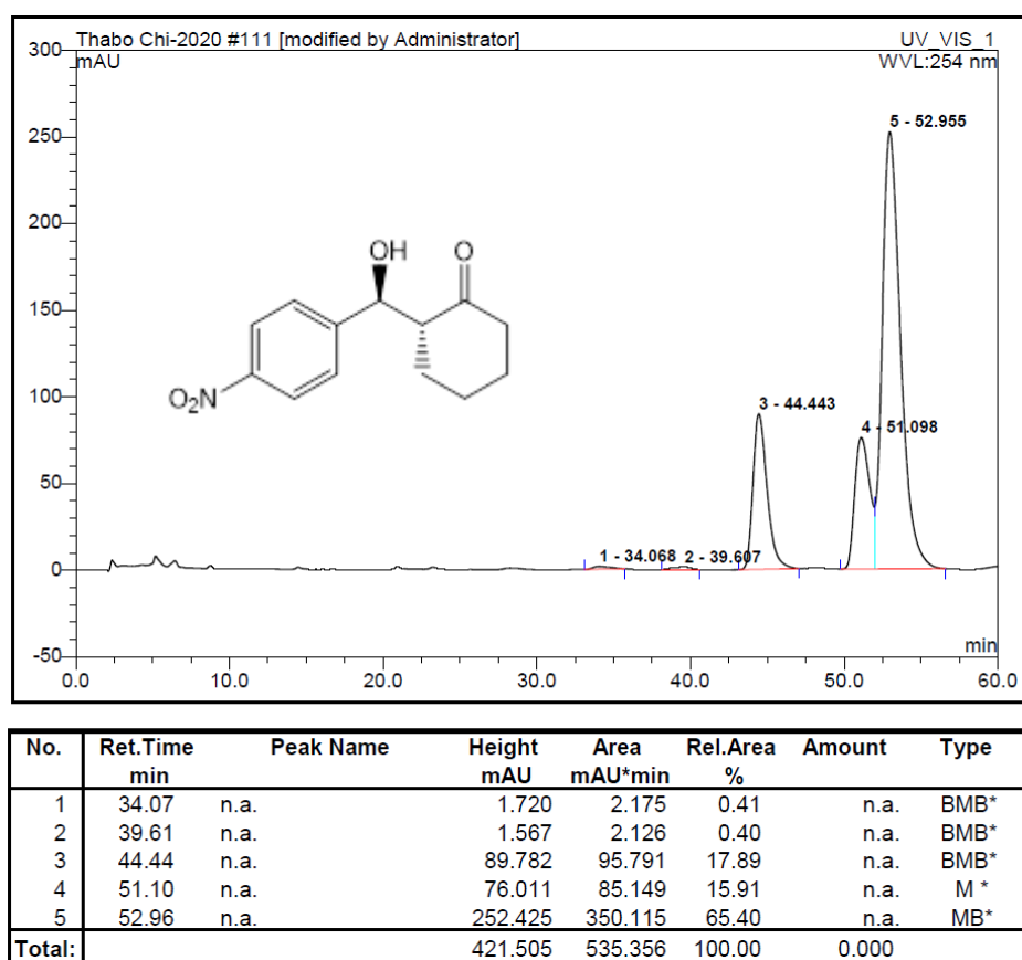
Figure S.4-30: Chiral HPLC chromatogram of TP_A4.21N4CY (entry 7)
