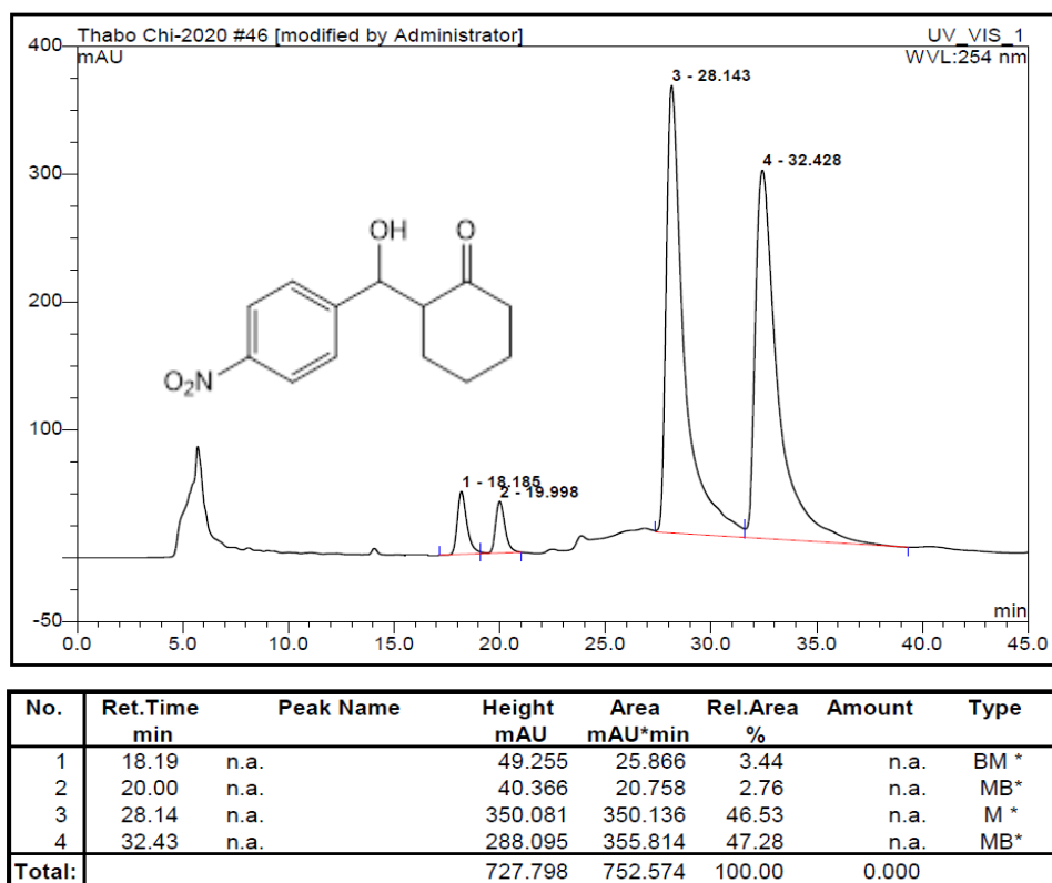
Figure S.4-R: Chiral HPLC chromatogram of racemate TP_A4N4CY-R10
