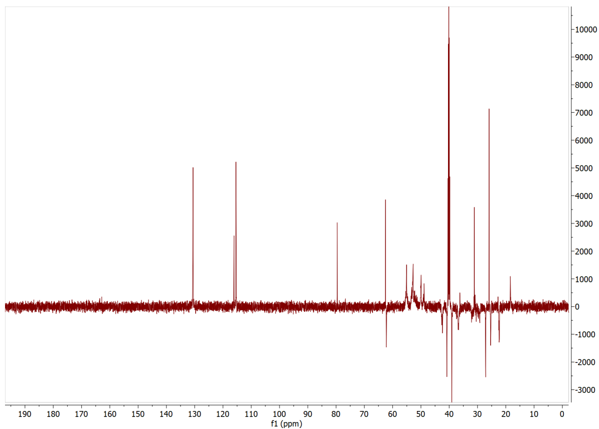
Figure S.3-3: DEPT 135 NMR spectrum of TP_Asp peptide
