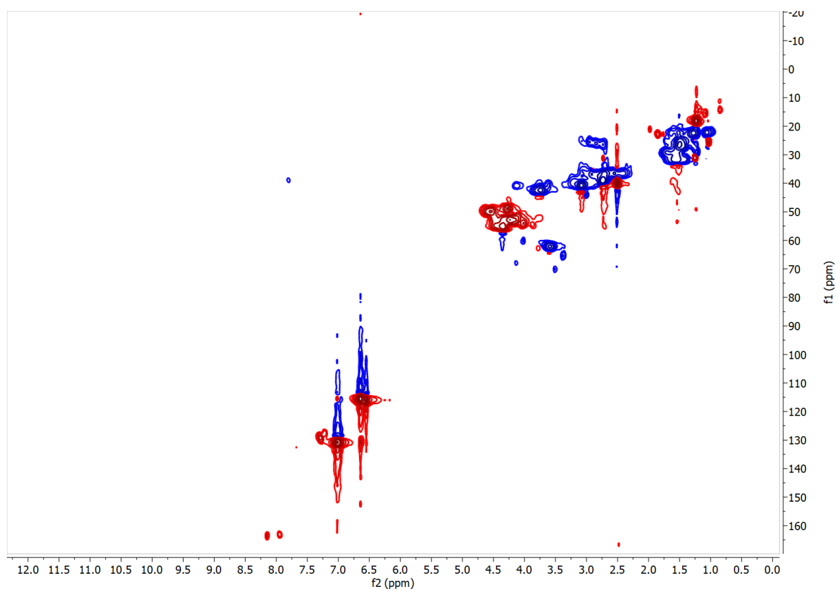
Figure S.3-14: HSQC NMR spectrum of TP_ADLYs peptide
