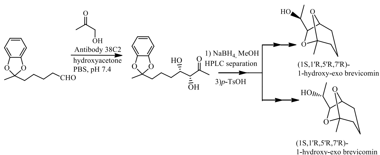
Scheme 2- 1: Total synthesis of hydroxybrevicomins from aldol reaction catalyzed by an antibody 38C2. 14
