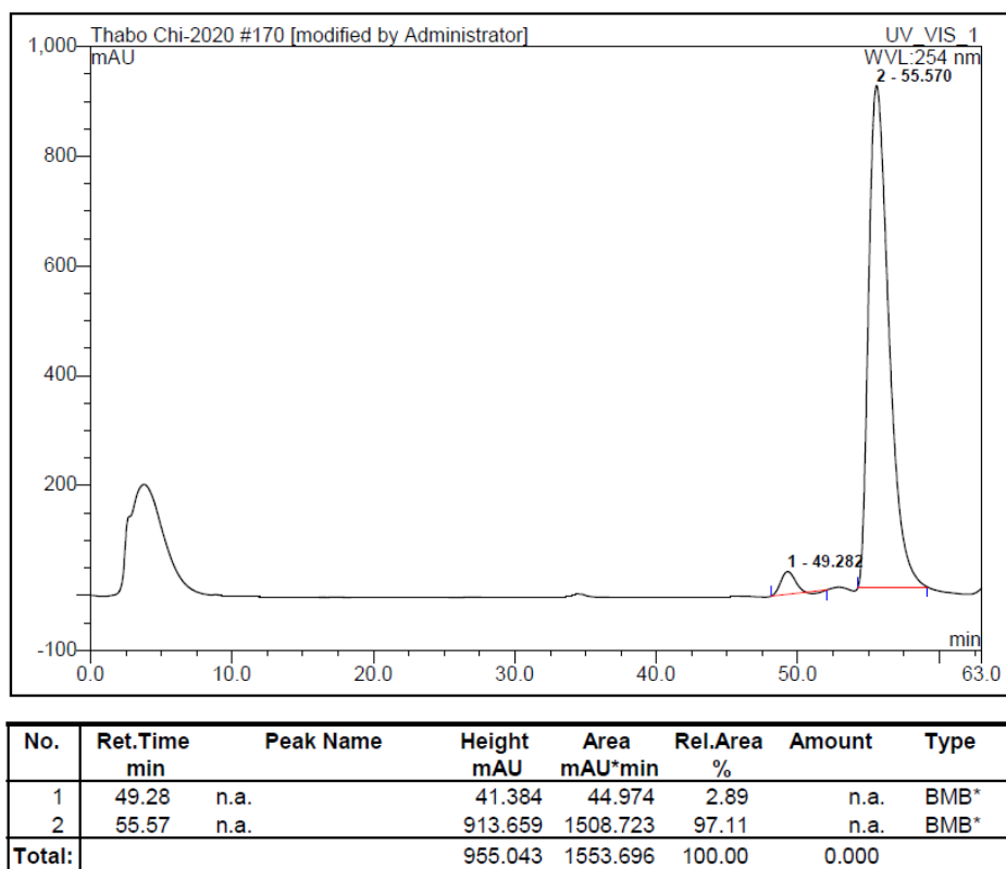
Figure S.4-33: Chiral HPLC chromatogram of TP_A4.24N4CY (entry 10)
