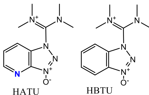
Figure 2- 4: Illustration of the difference between HATU and HBTU
