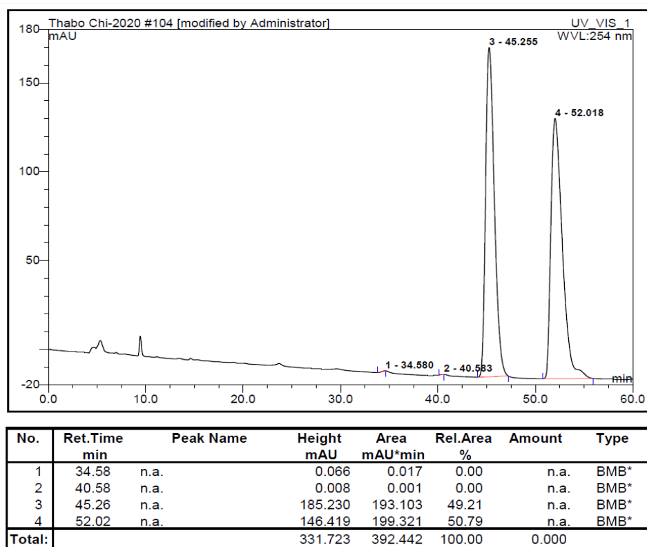
Figure S.4-R: Chiral HPLC chromatogram of racemate TP_A4N4CY-R13
