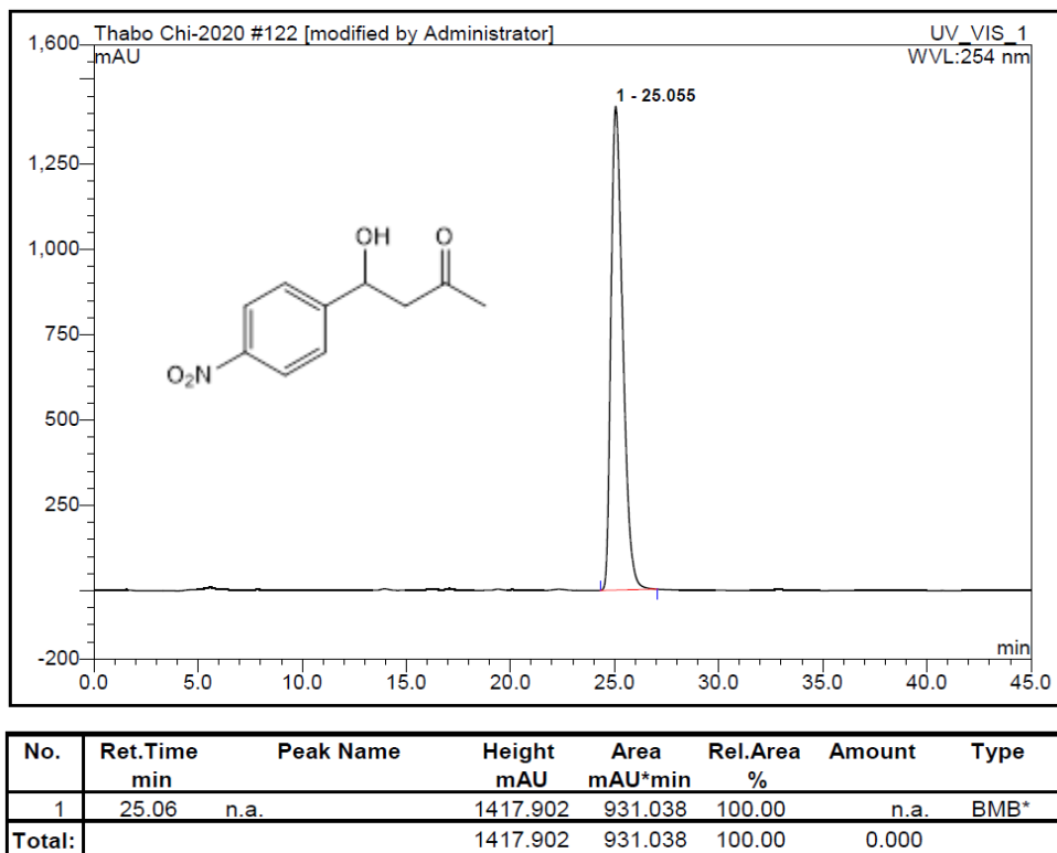
Figure S.4-S: Chiral HPLC chromatogram of TP_A1N4ACE –standard
