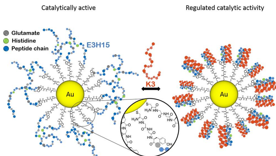
Figure 1- 11: Peptide sequence of E3H15 conjugated to Gold nanoparticles. 111
