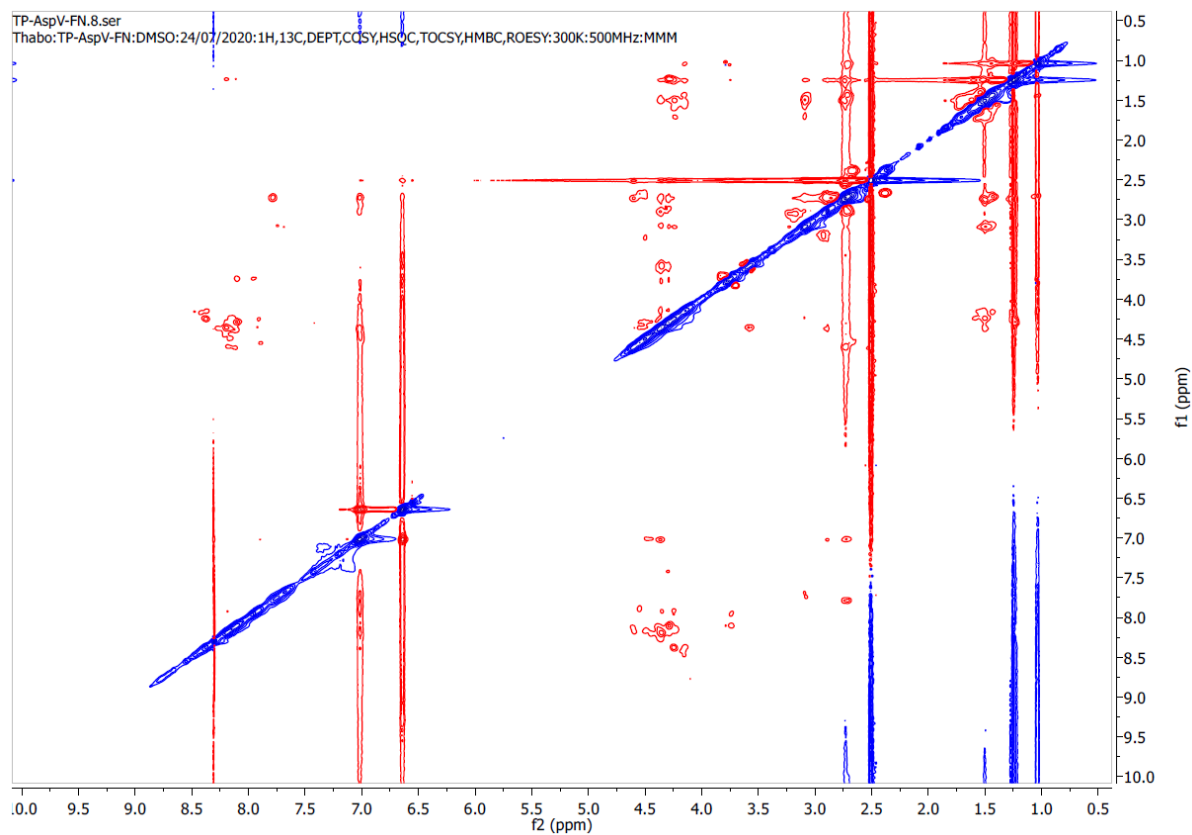
Figure S.3-8: 2D ^1\text{H} ROESY NMR spectrum of TP_Asp peptide
