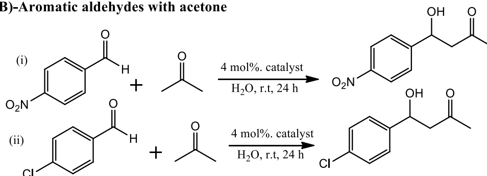
Scheme 4- 4: Aldol test reactions for selected peptides, using (A) linear aldehydes and (B) aromatic aldehydes with acetone.
