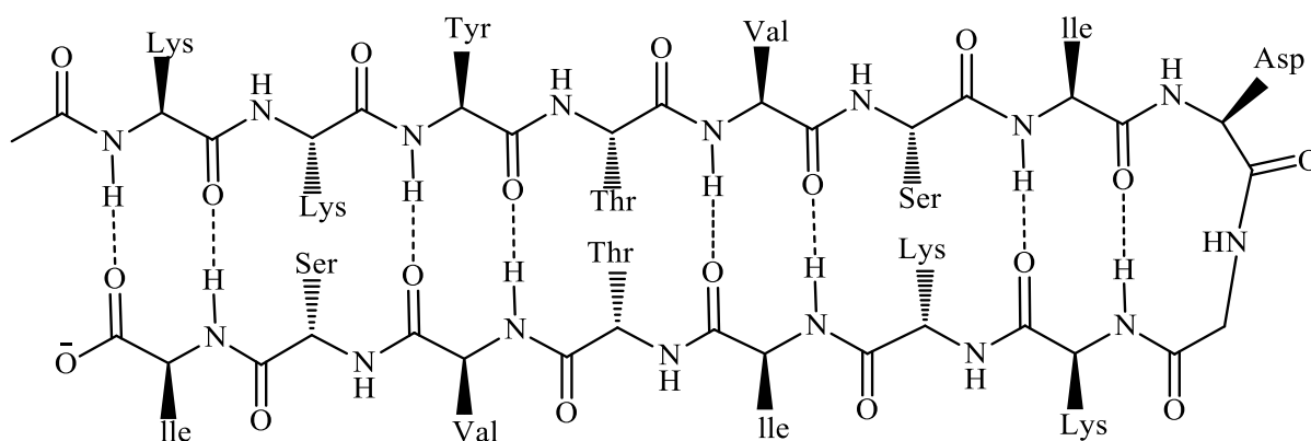
Figure 1- 10: \beta -hairpin with Asp-Gly \beta -turn promoter done by Ramírez-Alvarado et al. 100
