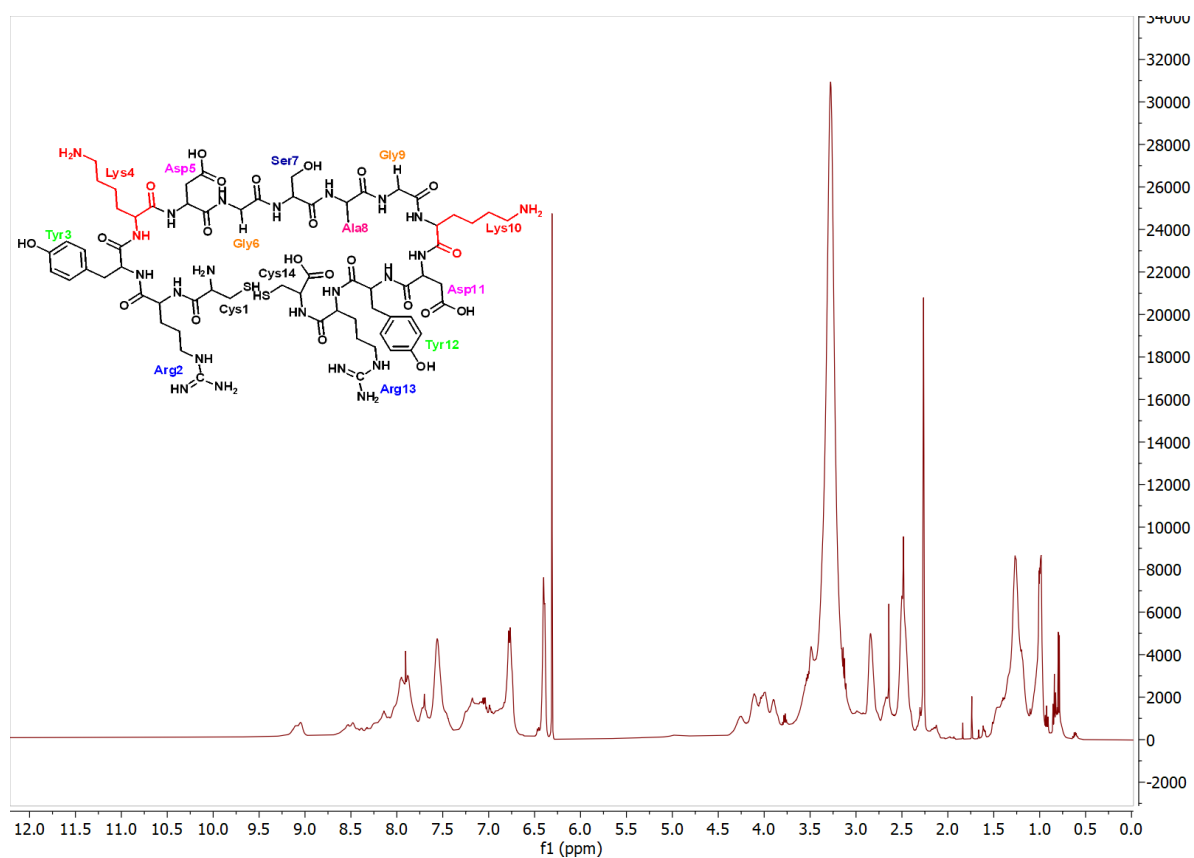
Figure S.3-10: ^1\text{H} NMR spectrum of TP_ADLYs peptide
