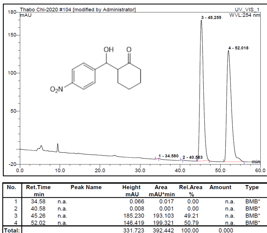
Figure S.4-R: Chiral HPLC chromatogram of racemate TP_A4N4CY-R21
