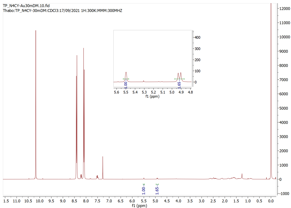
Figure S.4-49: ^1\text{H} NMR spectrum of the crude product TP_A4.20N4CY
