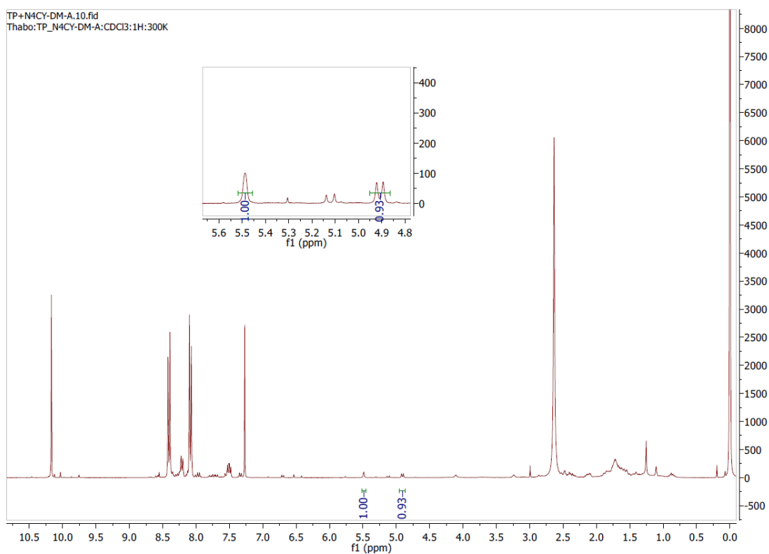
Figure S.4-35: ^1\text{H} NMR spectrum of the crude product of TP_A4.3N4CY
