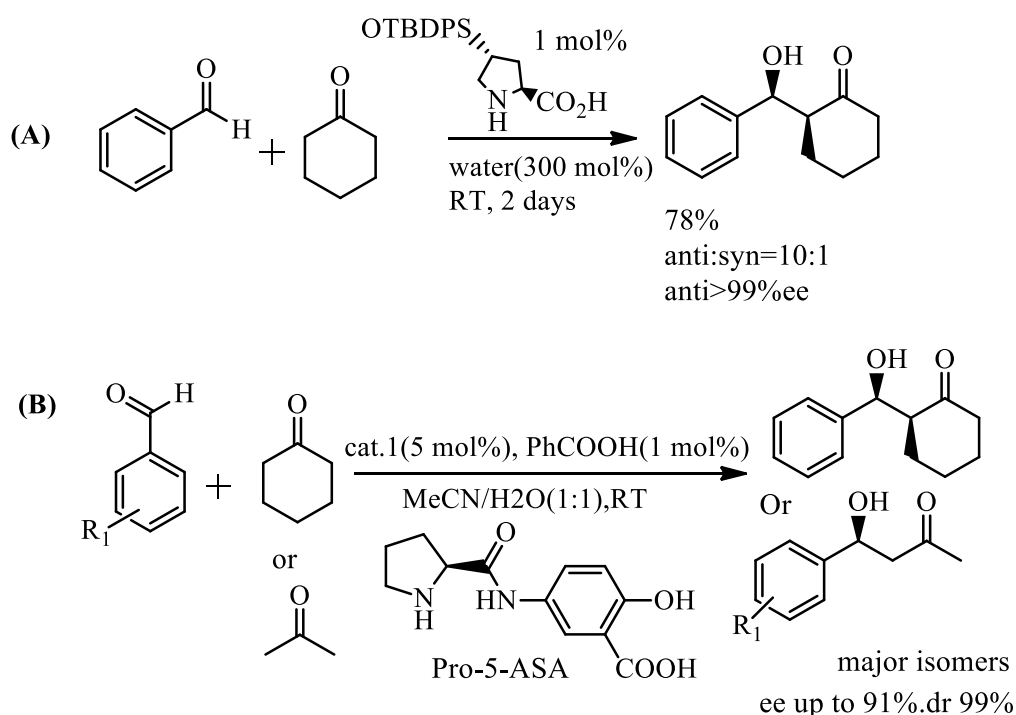
Scheme 4- 3: Water as solvent in organocatalytic asymmetric aldol reactions, (A) Hayashi's proline catalyzed aldehyde–ketone aldol reaction in water, 23 (B) Rahman's small proline-based dipeptide in aqueous medium. 5
