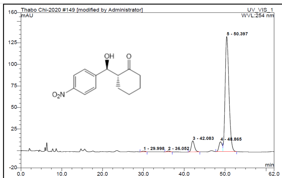
Figure S.4-R: Chiral HPLC chromatogram of racemate TP_A4N4CY-R17
