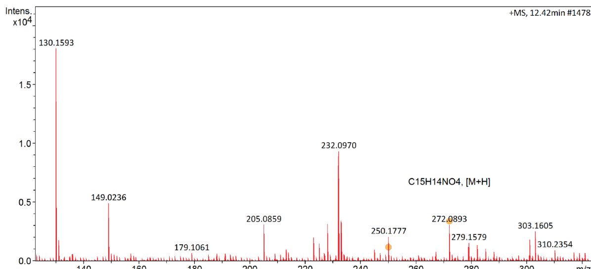
Figure 4- 3: LC-MS chromatograph depicting the formation of A2 product in 30 minutes.
