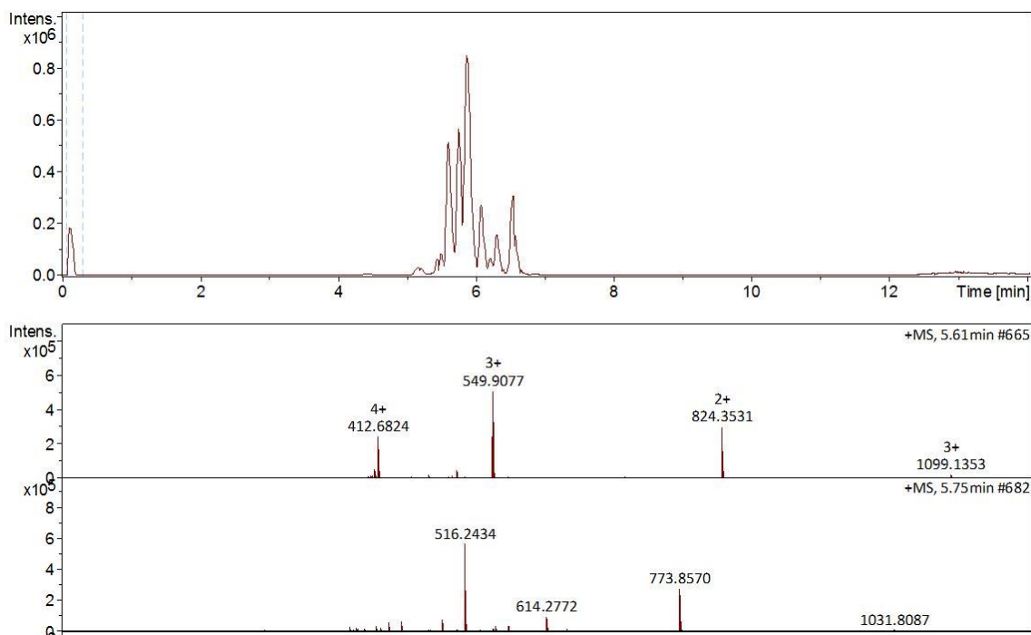
Figure 2- 11: LC-MS spectrum for the 1 st purification of TP_Glu peak 1
