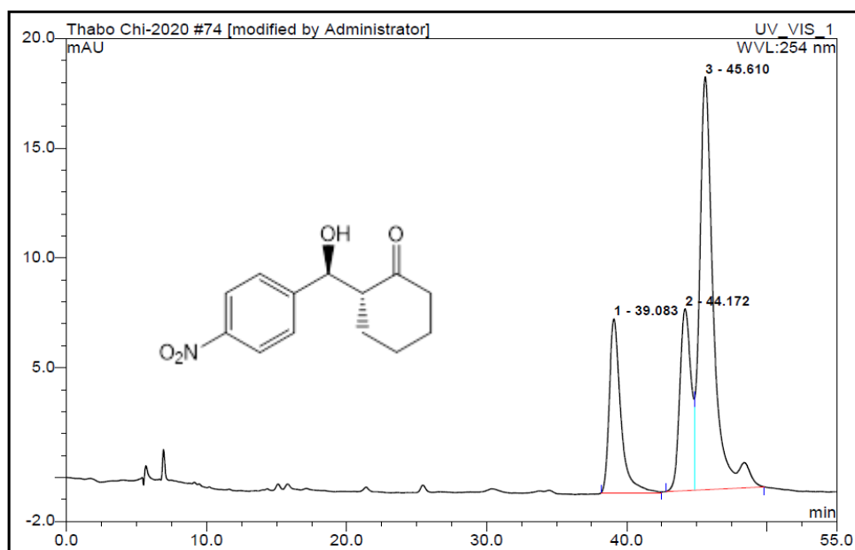
Figure S.4-R: Chiral HPLC chromatogram of racemate TP_A4N4CY-R7
