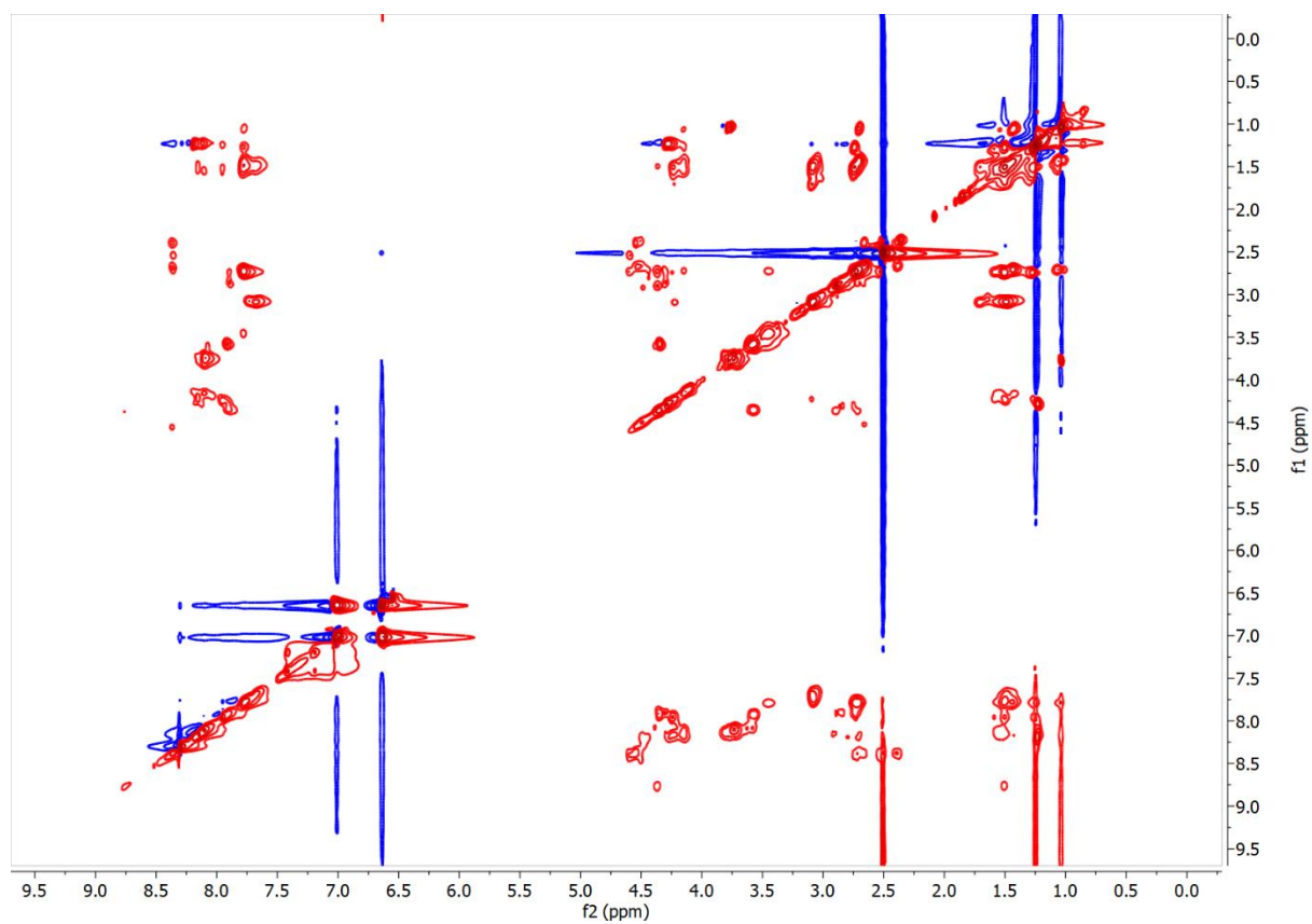
Figure S.3-6: 2D ^1\text{H} TOCSY NMR spectrum of TP_Asp peptide
