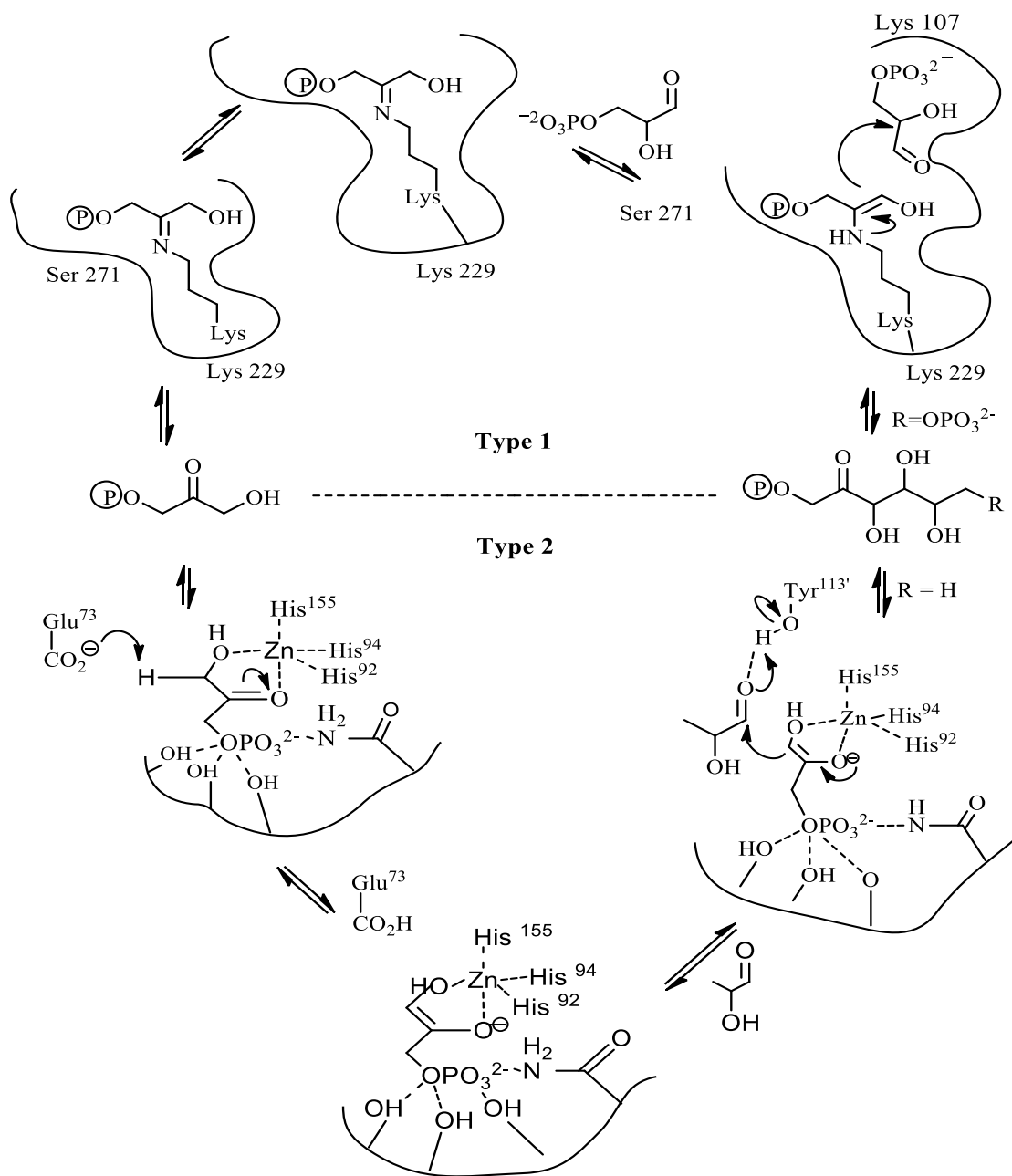
Scheme 1- 3: Mechanism of Type I Schiff base forming aldolase represented by the RAMA (Rabbit muscle aldolase ) and the Type II zinc enolate mechanism represented by the fucose-1-phosphate enzyme aldolase, bottom. \text{P} = \text{OPO}_3^{2-} . 20
