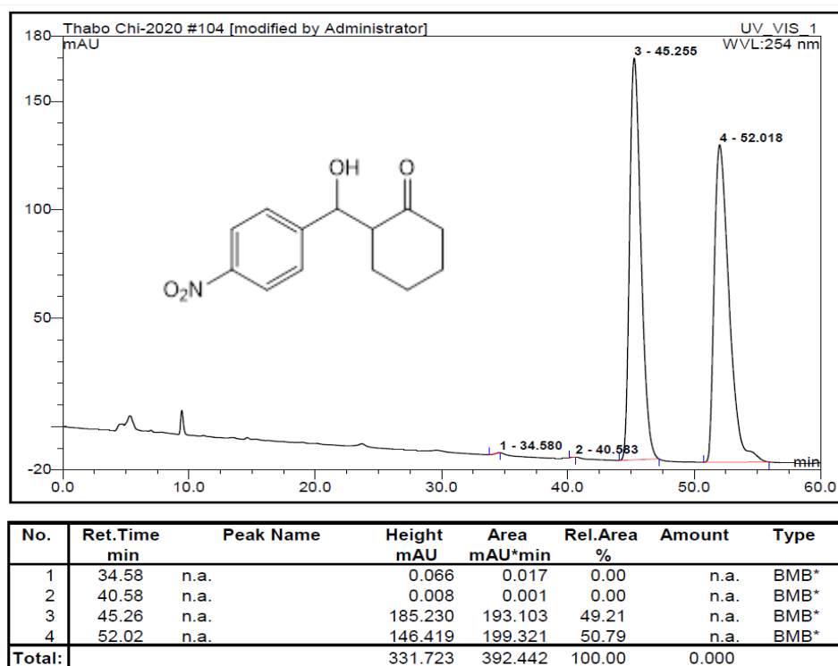
Figure S.4-R: Chiral HPLC chromatogram of racemate TP_A4N4CY-R19
