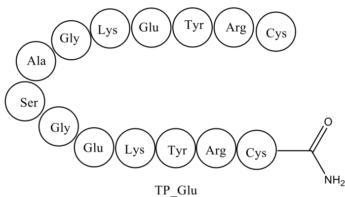
Figure 2- 10: Amino acid sequence for peptide catalyst TP_Glu
