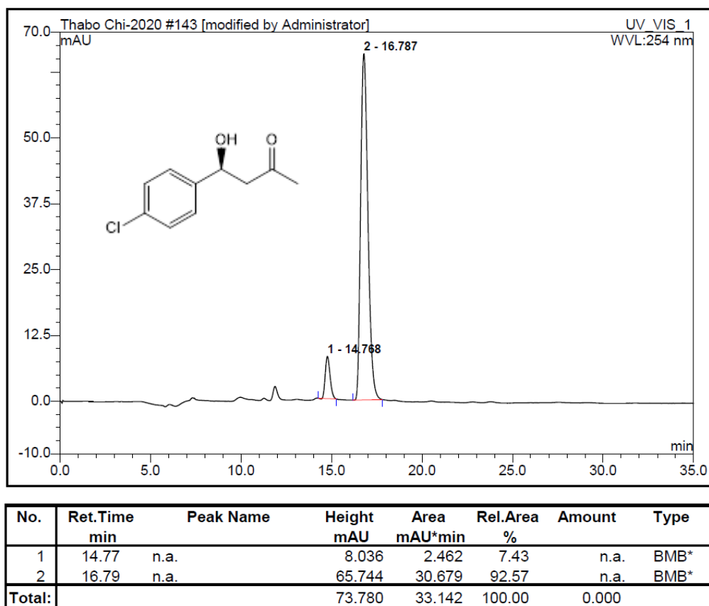
Figure S.4-9: Chiral HPLC chromatogram of TP_A3Cl4ACE (entry 5)
