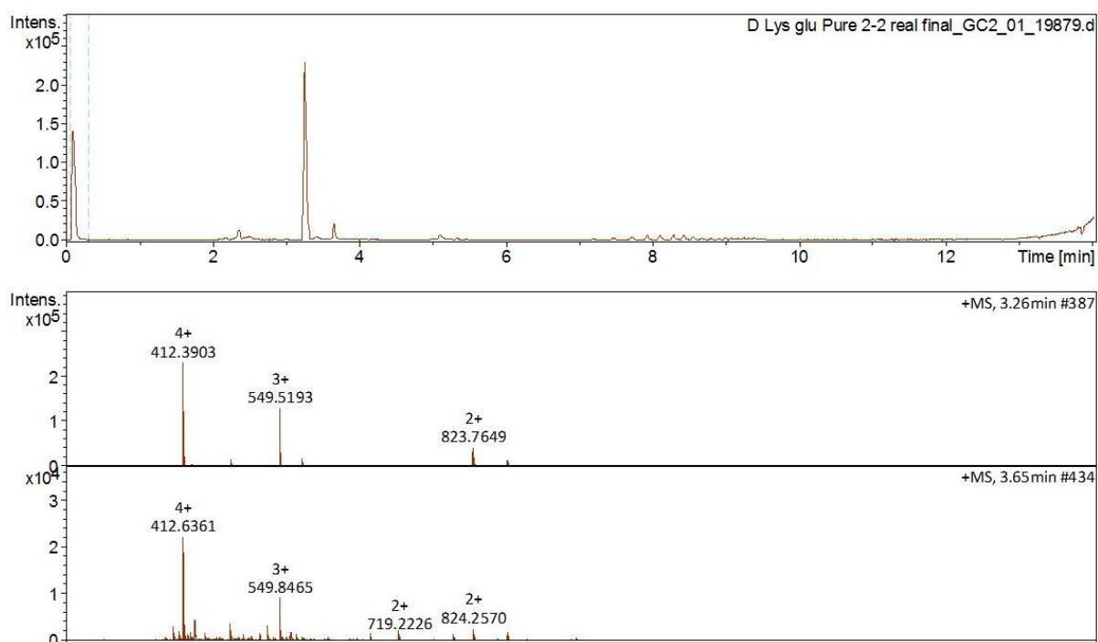
Figure 2- 15: LC-MS spectrum for TP_GDLys peak 2 after 2 nd purification
