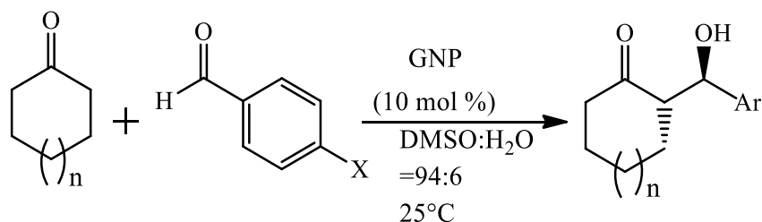
Scheme 1- 9: AuNPs-supported proline-catalyzed asymmetric aldol reactions. 112
