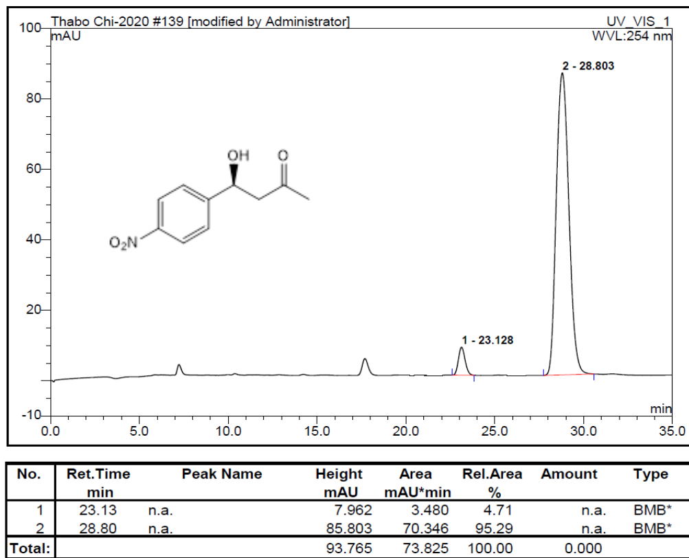
Figure S.4-11: Chiral HPLC chromatogram of TP-A1.4N4ACE (entry 2)
