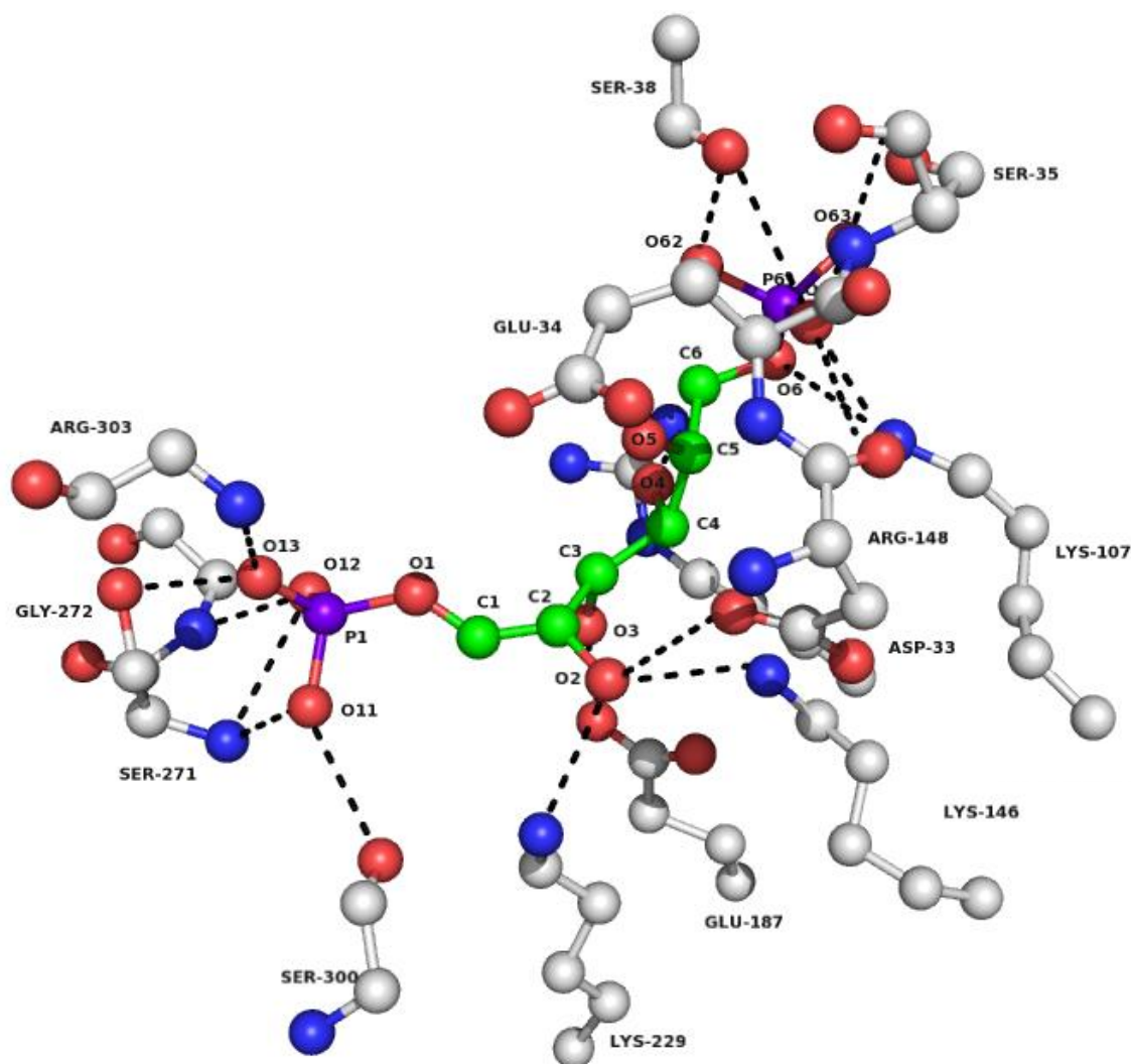
Figure 1- 6: 3D Structure depicting the FBPA active site residues interaction with the substrate molecule (2FBP) [some residues chains (side or main) are omitted for picture clarity]
