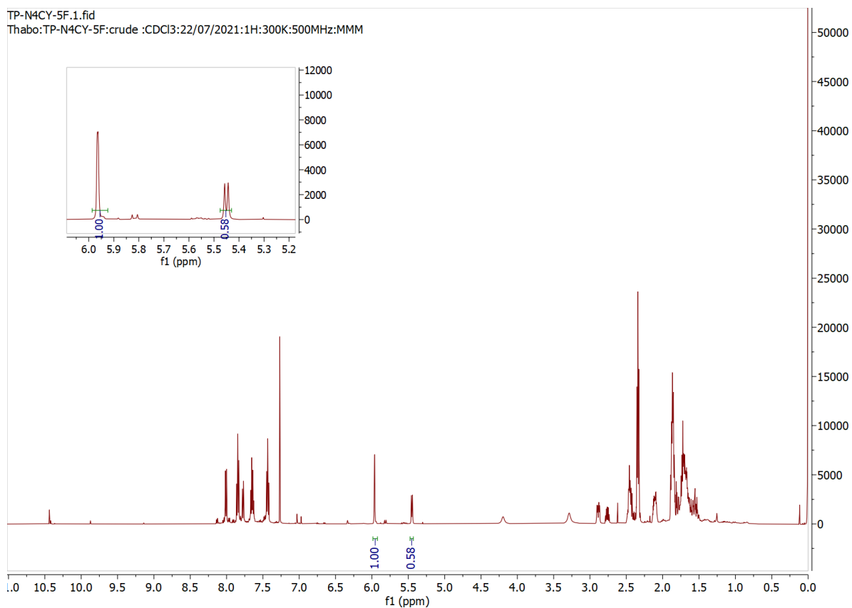
Figure S.4-39: ^1\text{H} NMR spectrum of the crude product of TP_A4.8N4CY
