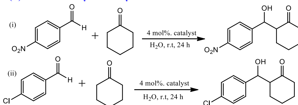
Scheme 4- 5: Aldol test reaction for selected peptides, using (A) linear aldehydes with cyclopentanone and (B) aromatic aldehydes cyclopentanone, (C) linear aldehydes with cyclohexanone, (D) aromatic aldehydes with cyclohexanone.
