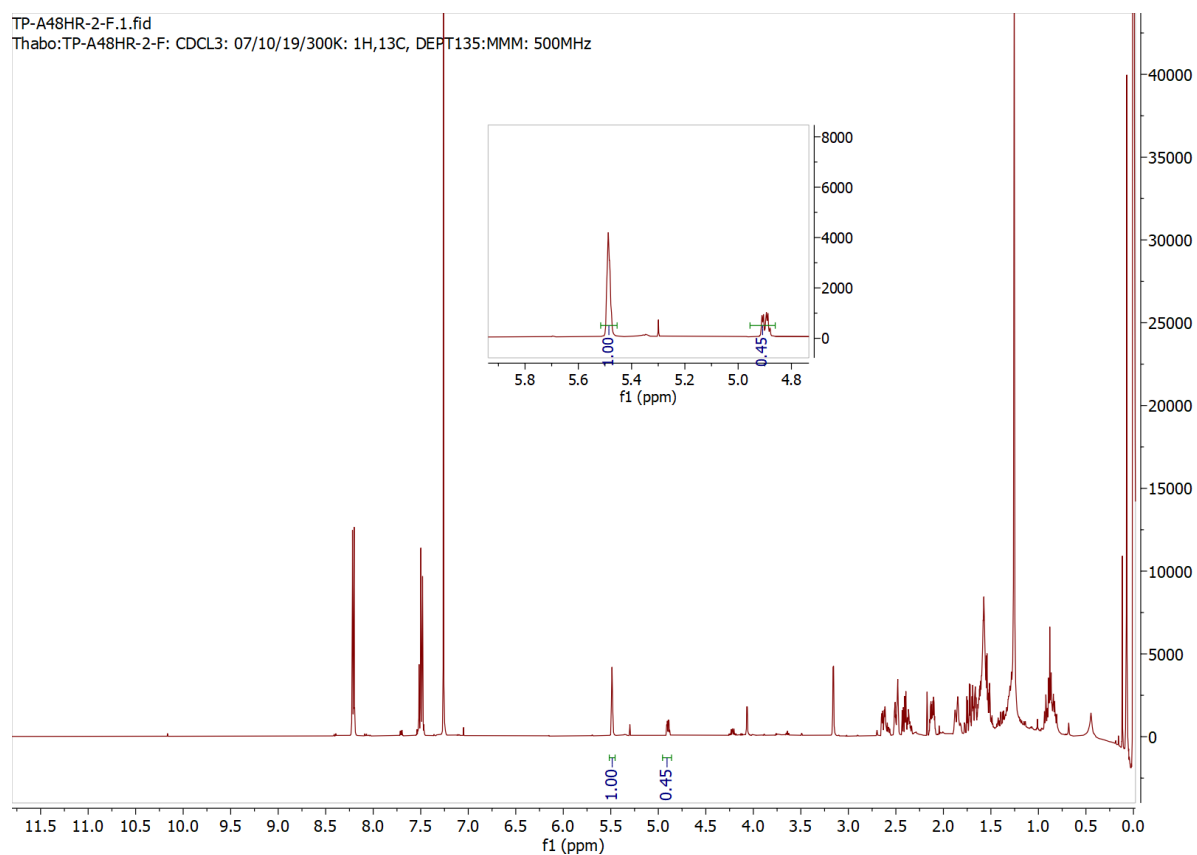
Figure S.4-37: ^1\text{H} NMR spectrum of the crude product TP_A4.5N4CY
