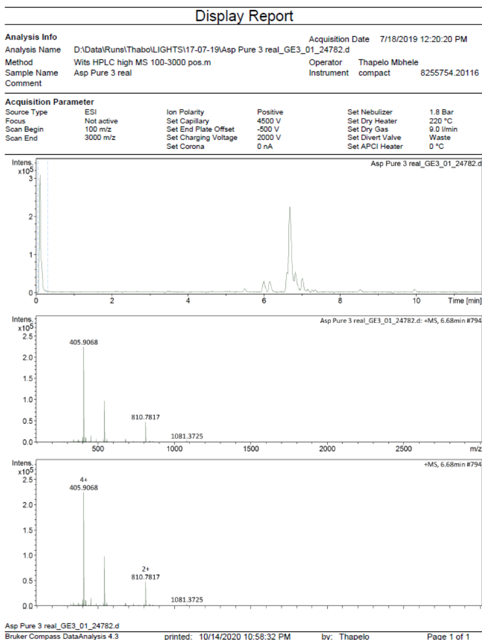
Figure S.2-3: LC-MS spectrum of TP_Asp conformation 3 (peak 3)
