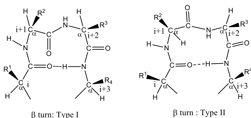
Scheme 1- 2: Types of beta turn motifs. 48
