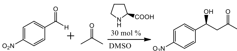
Scheme 1- 5: Asymmetric aldol reaction reported by List et al. 71
