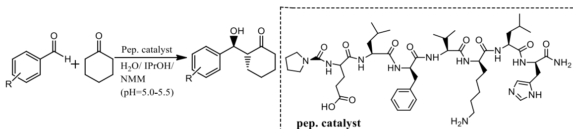
Scheme 2- 3: Bayat's rational design of mimetic peptides based on the AKR active site. 21
