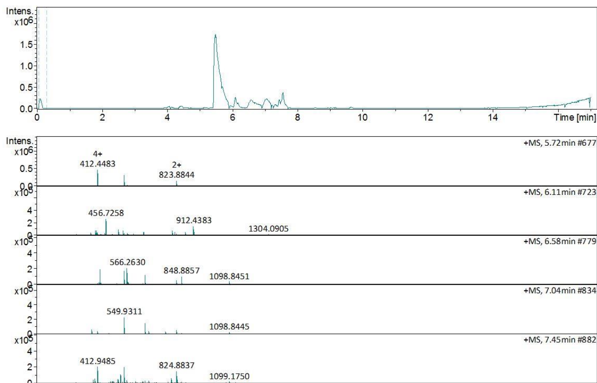
Figure 2- 14: LC-MS spectrum for TP_GDLys peak 2 after 1 st purification
