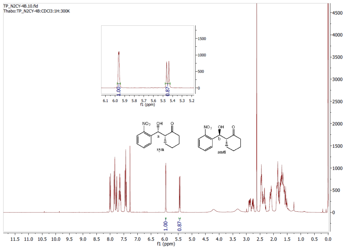
Figure S.4-40: ^1\text{H} NMR spectrum of the crude product of TP_A5.1N2CY
