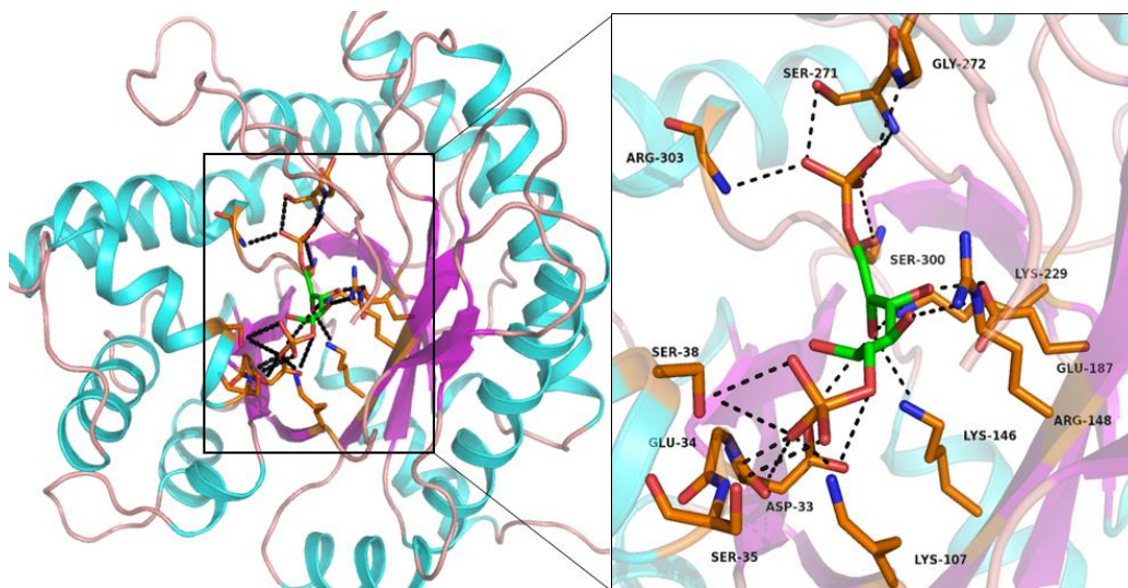
Figure 1- 5: The active sites residues of FBPA shown as stick form (on the right)
