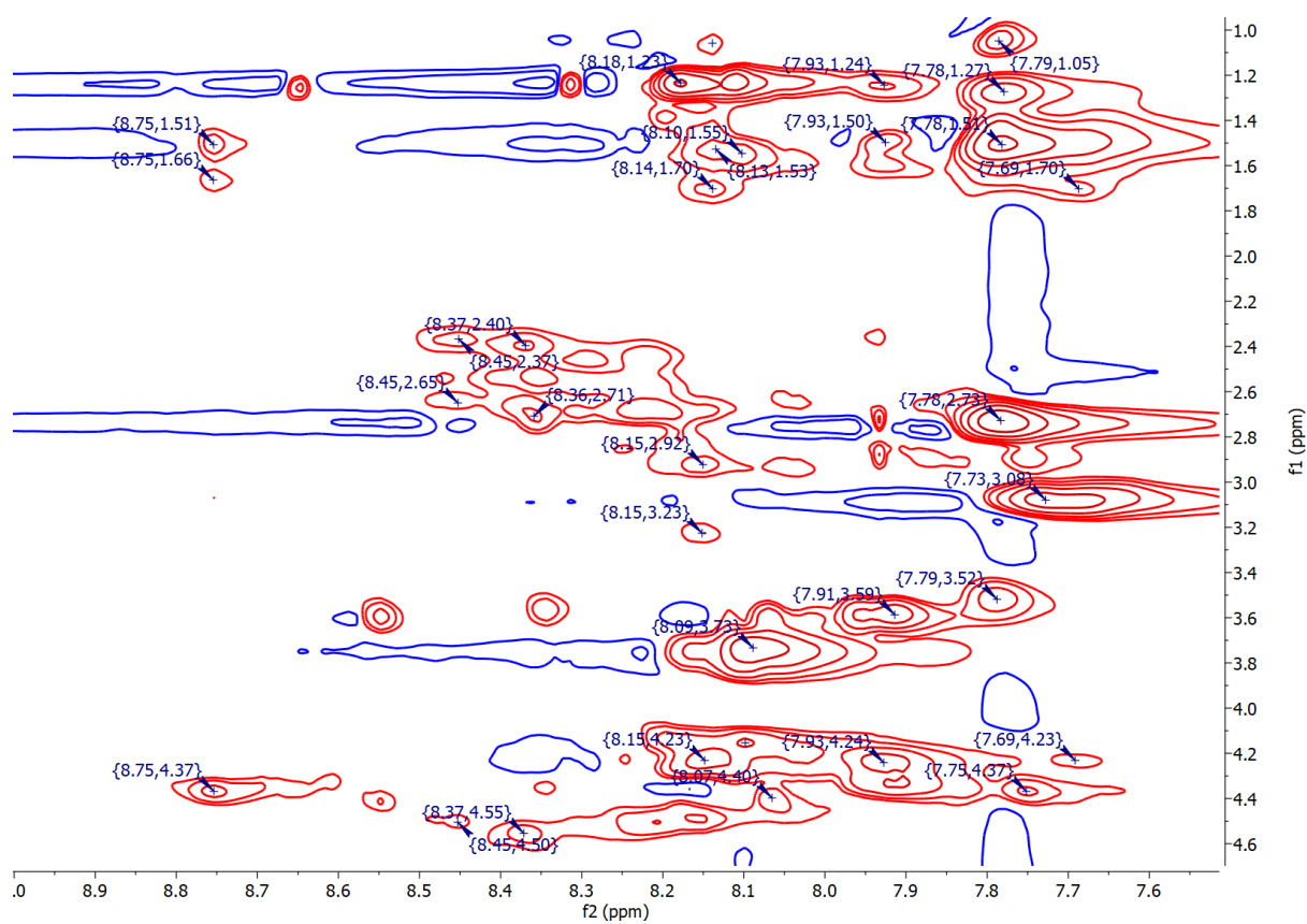
Figure S.3-16: 2D ^1\text{H} TOCSY spectrum of TP_ADLYs peptide, ^1\text{HN} fingerprint region
