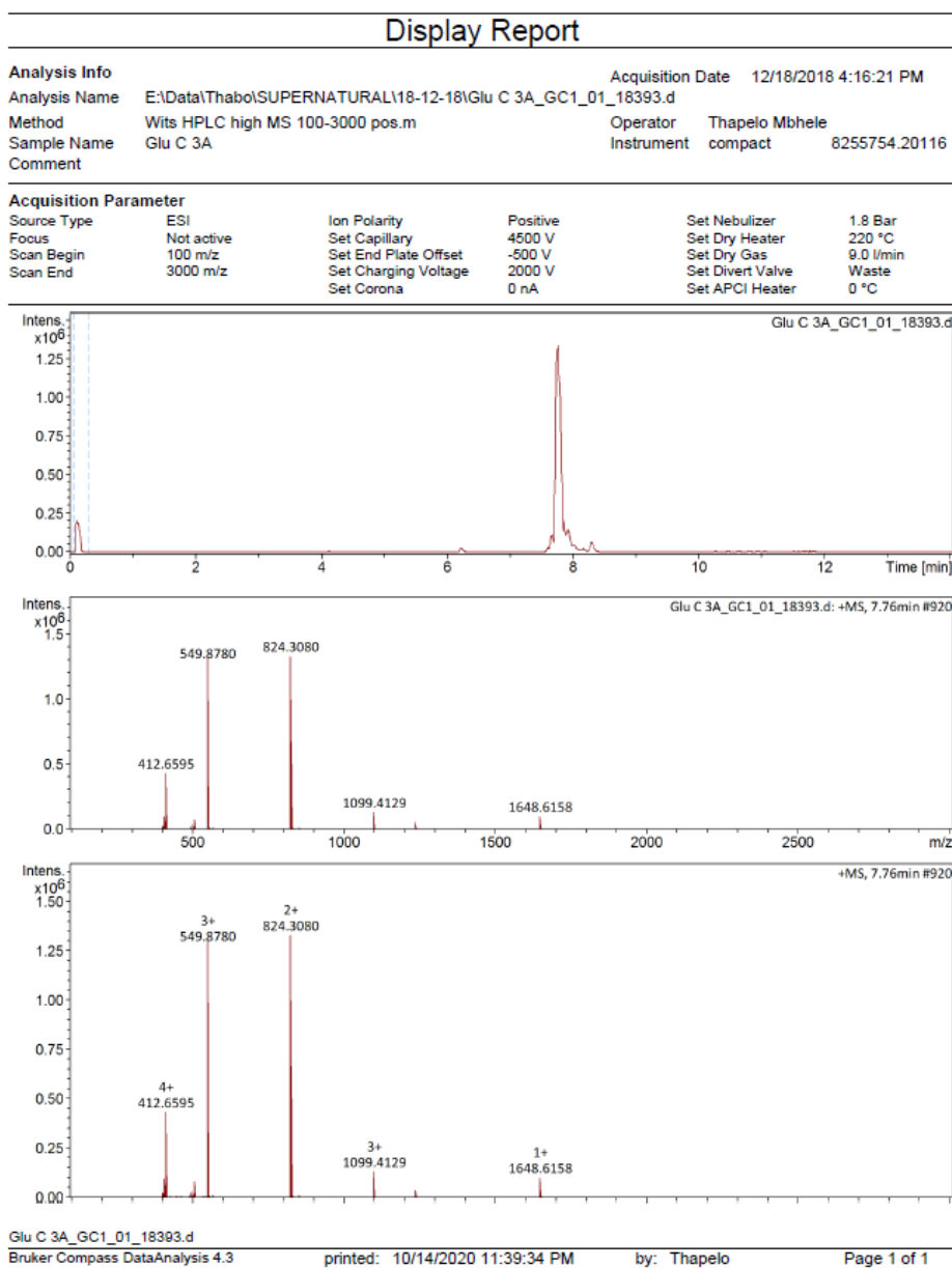
Figure S.2-11: LC-MS spectrum of TP_Glu conformation 3 (peak 3)
