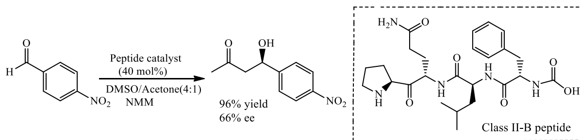
Scheme 1- 8: Kofoed's peptide catalyzed enantioselective aldol reaction of p -nitrobenzaldehyde and acetone. 93
