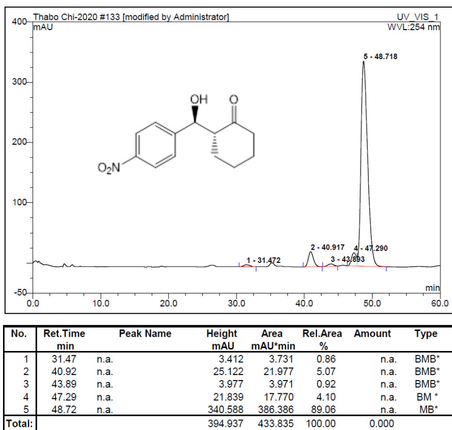
Figure S.4-27: Chiral HPLC chromatogram of TP_A4.18N4CY (entry 5)
