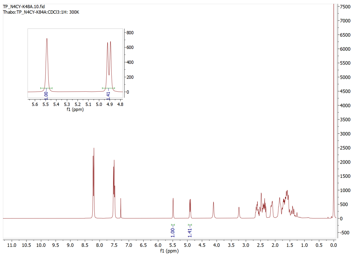
Figure S.4-43: 1 H NMR spectrum of the crude product TP_A4.10N4CY
