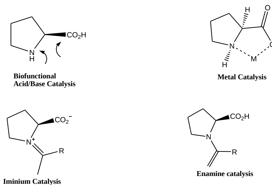
Figure 1- 7: Modes of action of proline catalysis. 77
