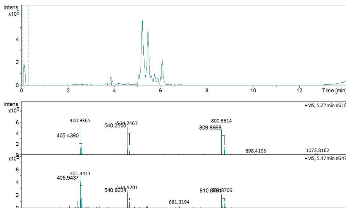
Figure 2- 8 : LC-MS spectrum for 1 st purification of peak 1 for TP_ADA peptide
