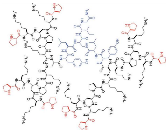
Scheme 2- 2: A) Peptide dendrimer catalyzed aldol reaction, B) L2D1 Peptide dendrimer used. 15
