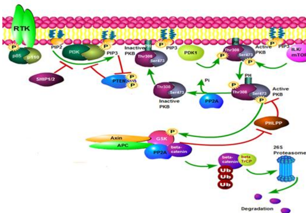
Figure 4. 1: PP2A signalling. As highlighted within the text, PP2A antagonizes the activation of PKB by dephosphorylating its Thr308 residue that is phosphorylated by PDK1. This dephosphorylation, in turn, leads to the dephosphorylation of PKB on its Ser473 residue, or alternatively, can be directly dephosphorylated by PP2A, leading to its inactivation. PP2A also enhances the stabilization of the \beta -catenin degradation complex (GSK3 \beta -Axin-APC) by regulating the Ser9 phosphorylation status of GSK3 \beta . Figure generated using the Pathway Builder Tool. 2.0.
