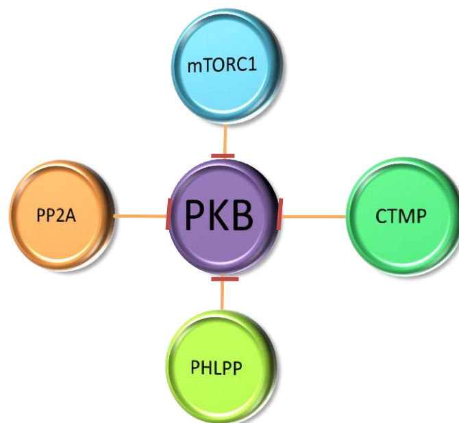
Figure 1.14: Termination of the PI3K/PKB signalling pathway through PKB inactivation. mTORC1, CTMP, PP2A and PHLPP are able to dephosphorylate the Ser473 residue of PKB.
