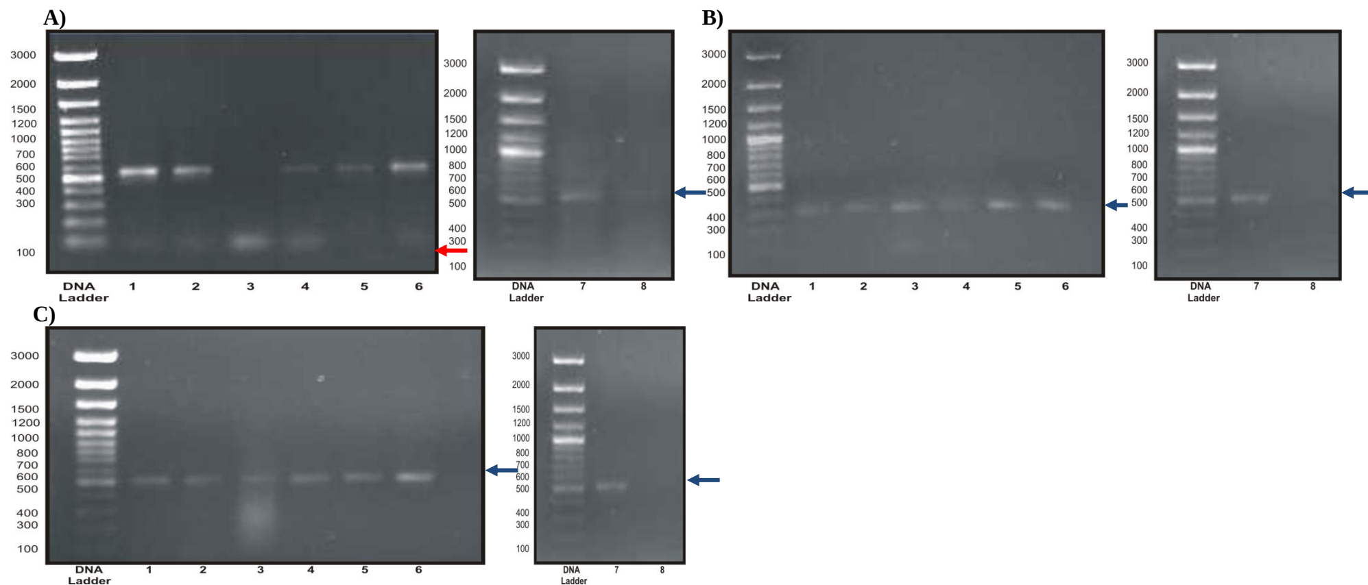
Figure B4: Amplification of Exon 4 (C2 domain) and Exon 20 (kinase domain) of the PIK3CA gene in HOSCC cells. A) The presence of a PCR fragment at 550 bp is indicative of a positive amplification of the larger splice fragment of Exon 4 (Exon 4A), indicated by the blue arrow, and the smaller splice fragment, Exon 4B ( B ), at 350 bp. The absence of a PCR fragment in lane 8 or the template-free control confirms the specificity of the reaction. Red arrow indicates primer dimer formation. C) The presence of a 500 bp PCR amplified fragment is indicative of Exon 20. The absence of a PCR fragment in lane 8 or the template-free control confirms the specificity of the reaction. Lanes 1-8: WHCO1, WHCO3, WHCO5, WHCO6, SNO, MCF7, HT29 and template-free control.
