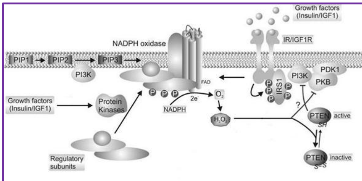
Figure 4. 2: Regulation of PTEN through Oxidation. RTK activation (illustrated here as the Insulin Tyrosine Receptor/IR), leads to the production of H_2O_2 through the membrane-bound NADPH oxidase. The recruitment of PTEN to the membrane, results in the H_2O_2 -mediated oxidation of its catalytic cysteine residues, leading to its reversible inhibition. See test for further details. Figure adapted from Szypowska 584 .
