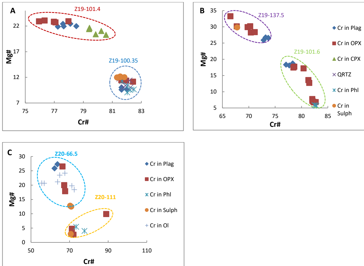
Figure 8-17: Cr# vs Mg# variation diagrams for chromites from the southwestern portion of the Uitloop farm magmatic lithologies.
