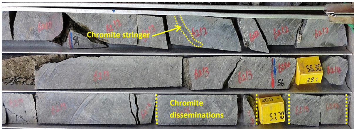
Figure 6-2: A photograph of borehole core samples showing a chromite stringer in harzburgite and fine-grained chromite disseminations in feldspathic harzburgite at a depth of 54.25 m and 57.5 m respectively in borehole Z20.
