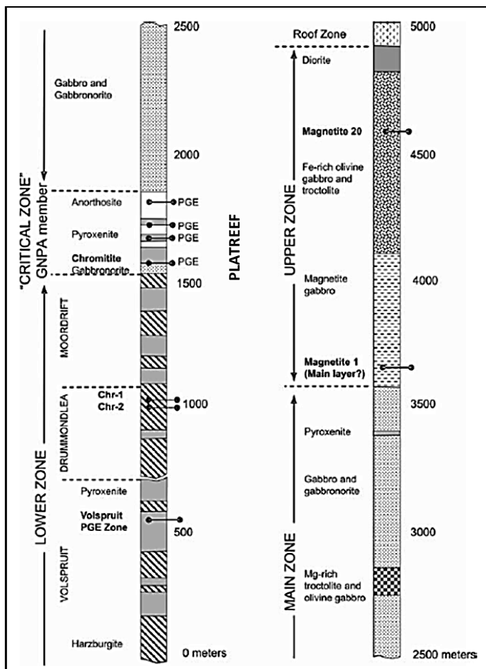
Figure 3-3: The stratigraphy of the northern limb indicating the occurrence of economic mineralisation within different Zones (McDonald et al., 2005).
