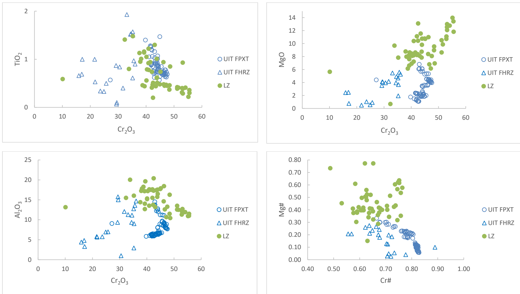
Figure 8-19: Compositional variation diagrams comparing the compositions of chromites from the southwestern portion of the Uitloop farm magmatic lithologies to those from the Lower Zone lithologies south of Mokopane (Hulbert, 1983) in the northern limb. (UIT FPXT = Uitloop feldspathic pyroxenite, UIT FHRZ = Uitloop feldspathic harzburgite, LZ = Lower Zone).
