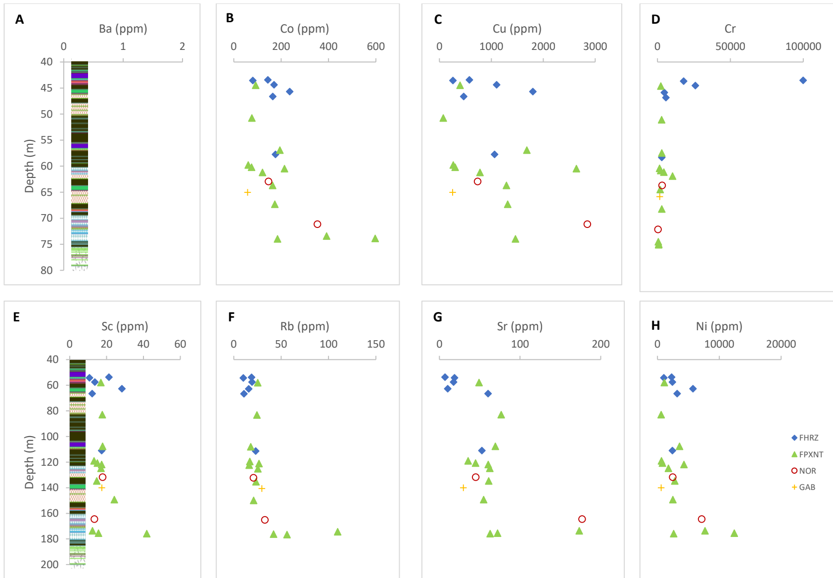
Figure 7-6: Variation in selected trace element concentrations (ppm) with stratigraphic height in borehole Z20 from the Uitloop farm. (FHRZ = Feldspathic harzburgite, FPXNT = Feldspathic pyroxene, NOR = Norite, GAB = Gabbro).
