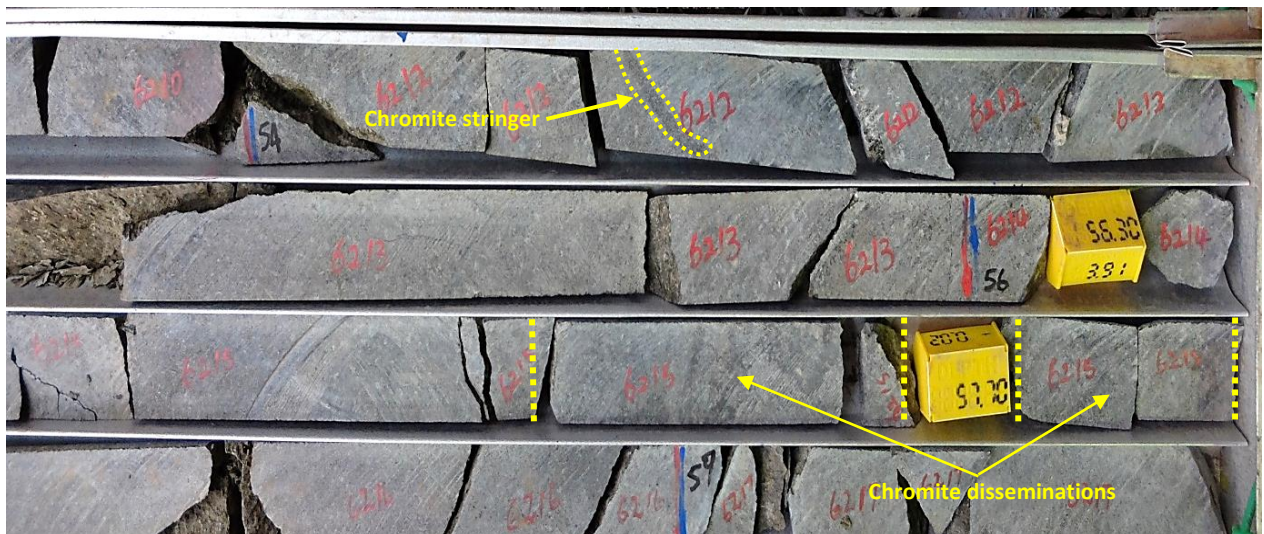
Figure 8-2: A photograph of borehole core sample showing a chromite stringer and chromite disseminations in feldspathic harzburgite at depths of 54.25 m and 57.5 m respectively in borehole Z20.
