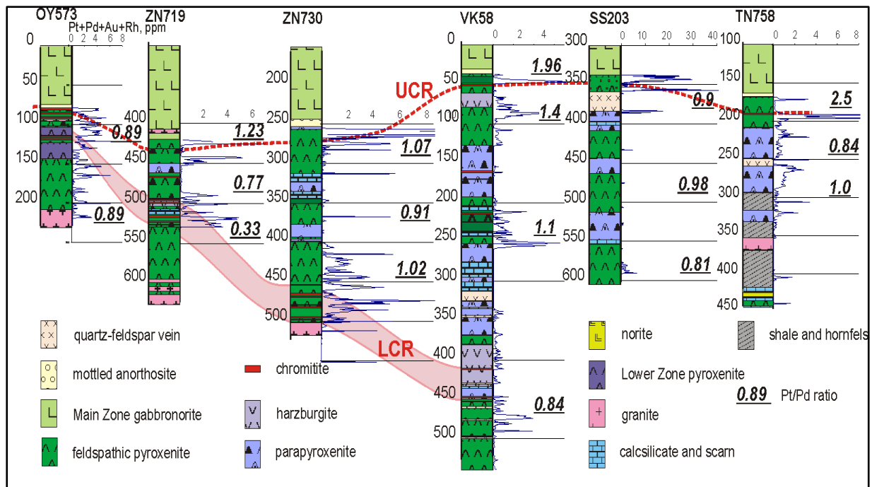
Figure 3-7: Stratigraphic logs showing persistent chromite-bearing horizons; termed the Upper Chromite Zones (UCR) and Lower Chromite Zone (LCR), within the Platreef along strike on Overysel (OY), Zwartfontein (ZN), Vaalkop (VK), Sandsloot (SS) and Tweefontein (TN) farms (Yudovskaya & Kinnaird, 2010).
