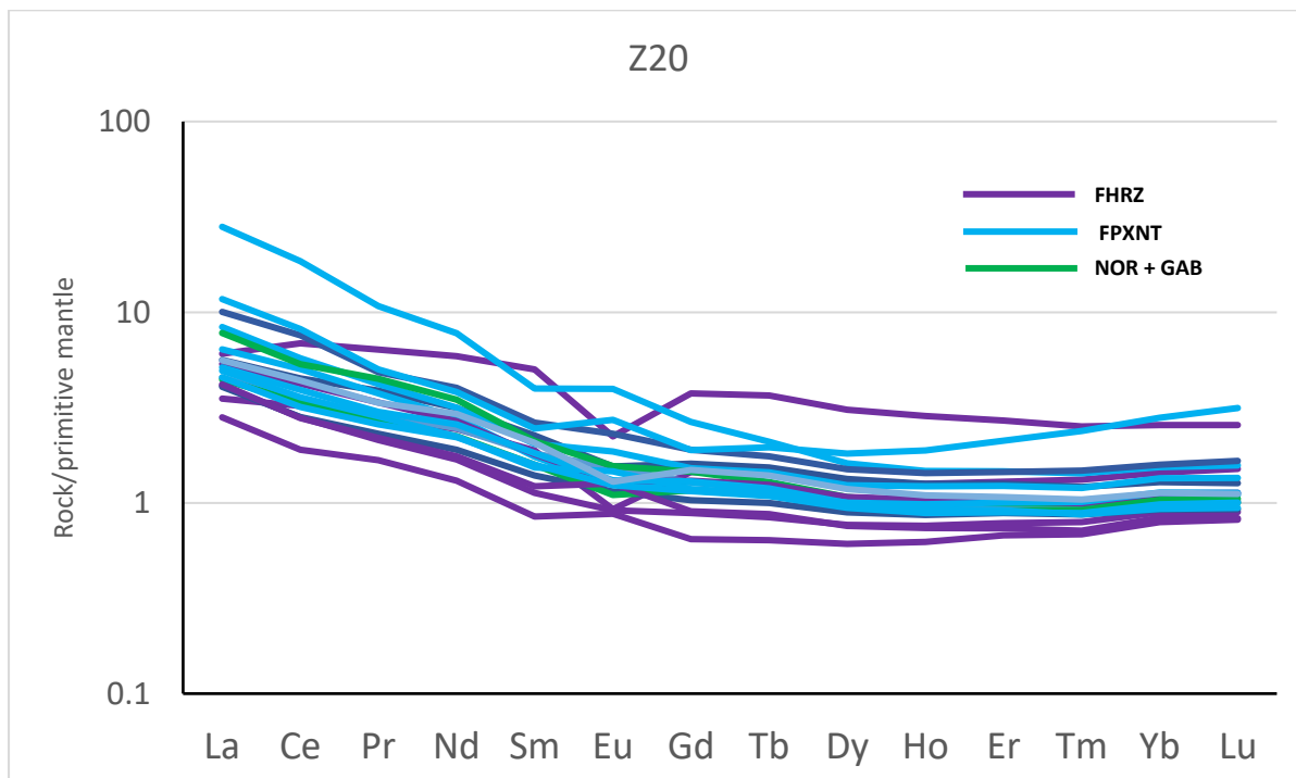
Figure 7-11: Primitive mantle normalized REE graphs (normalised to data by Hoffman (1988)) of the feldspathic pyroxenite (FPXNT) and feldspathic harzburgite (FHRZ) and Norite (NOR) + gabbro (GAB) from borehole Z20 of the southwestern portion of Uitloop farm.
