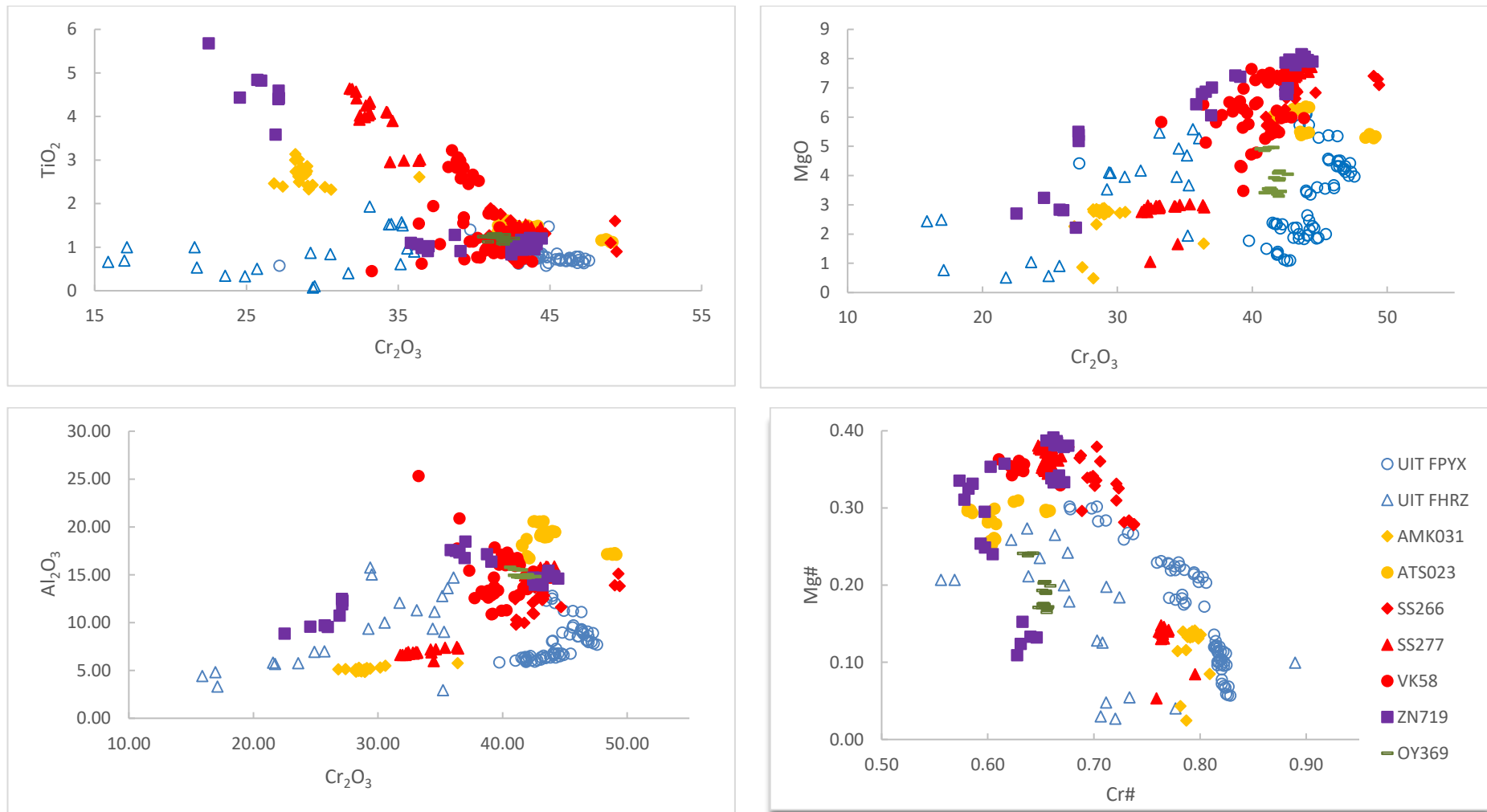
Figure 8-18: Compositional variation diagrams comparing the compositions of chromites from the southwestern portion of the Uitloop farm magmatic lithologies to those from different parts of the Platreef (Yudovskaya & Kinnaird, 2010) in the northern limb. (UIT = Uitloop, AMK = Macalacaskop, ATS = Turfspruit, SS = Sandsloot, VK = Vaalkop, ZN = Zwartfontein and OY = Overysel).
