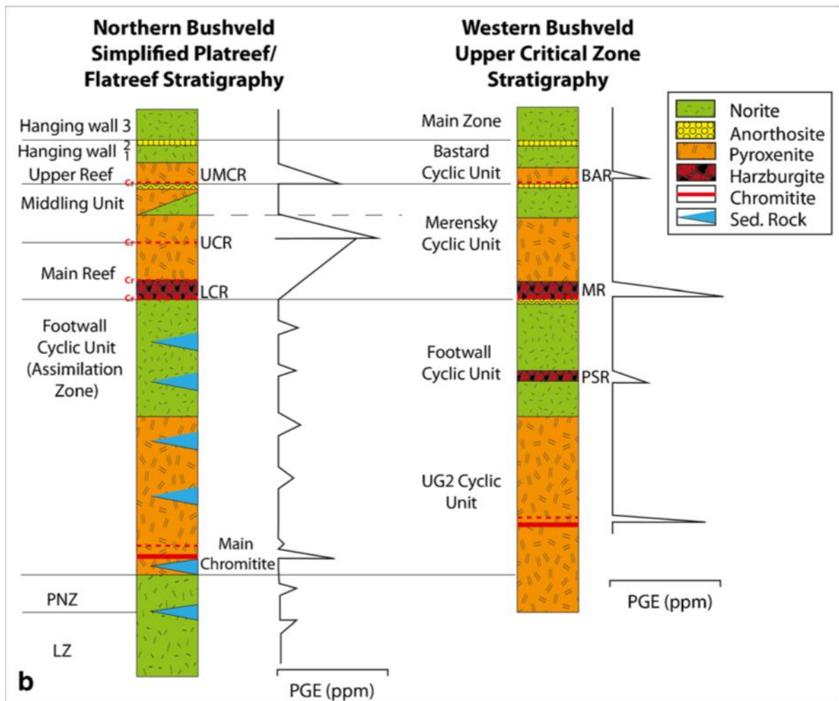
Figure 3-6: The stratigraphical correlation between the Platreef/Flatreef and the Upper Critical Zone of the western limb of the Bushveld Complex (Grobler et al., 2018).
