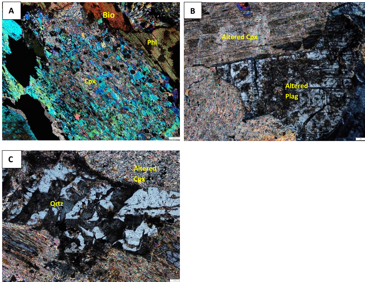
Figure 5-5: Photomicrographs (under XPL) of Gabbro, sample Z20-140.1, from the local magmatic stratigraphy in borehole Z20 at the southwestern portion of the Uitloop farm. (A) Altered clinopyroxene phenocryst. (B) Altered clinopyroxene and sericitized twinned plagioclase. (C) Interstitial quartz with a granophyric texture.
