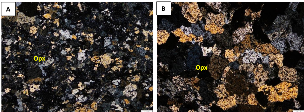
Figure 5-2: Photomicrographs (taken under XPL) of orthopyroxenite from the local magmatic lithologies at the southwestern portion of the Uitloop farm. (A) Fine-grained cumulus orthopyroxene crystals, sample Z19-174.9. (B) Coarse-grained cumulus orthopyroxene crystals, sample Z19-199.
