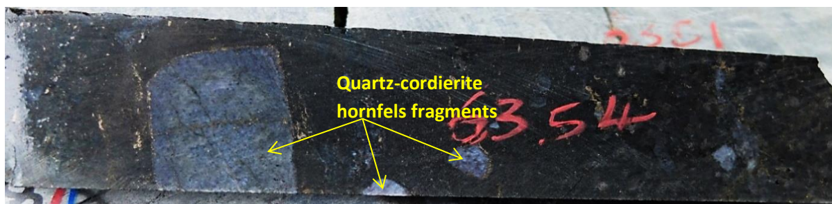
Figure 4-16: A photograph of borehole core sample showing hornfels (Sedimentary breccia) (sample Z20183.5) with various quartz-cordierite hornfels fragments rimmed by base metal sulphides.
