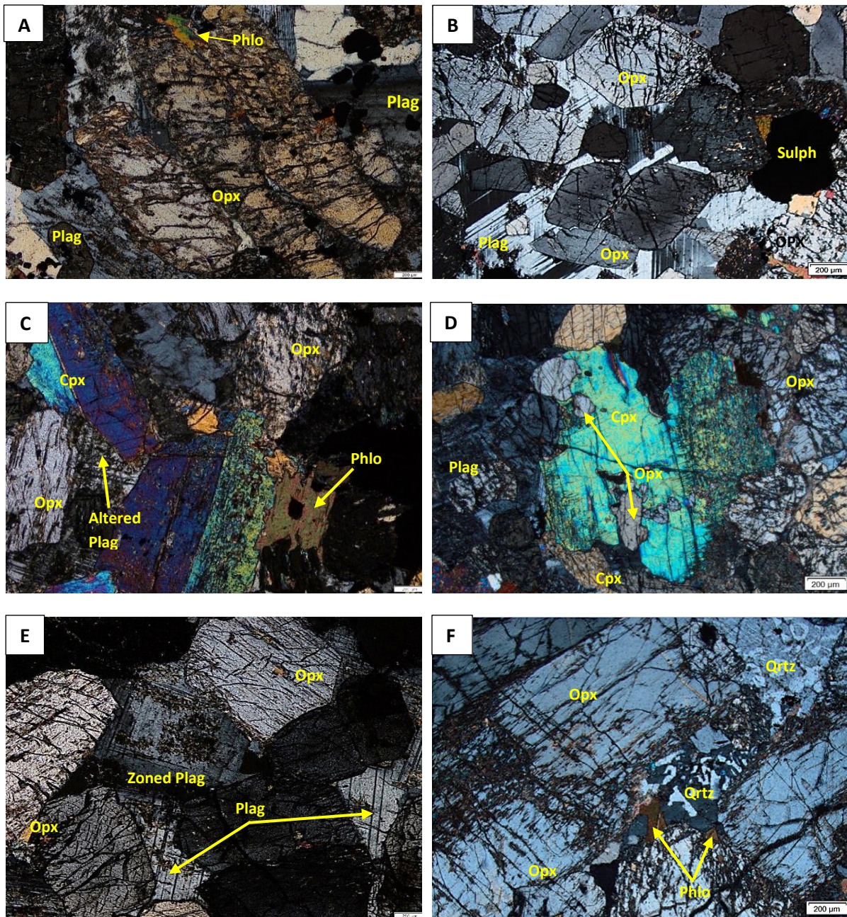
Figure 5-1: Photomicrographs (taken under XPL) of feldspathic pyroxenites under XPL from the southwestern portion of the Uitloop farm. (A) Cumulus orthopyroxene laths, sample Z19-100.35, (B) Cumulus orthopyroxene with intercumulus plagioclase, sample Z20-134.8, (C) Twinned clinopyroxene (D) Clinopyroxene oikocryst enclosing orthopyroxene, sample Z20-121.9, (E) Zoned and twinned intercumulus plagioclase, sample Z20-121.9 and (F) Granophyric quartz, sample Z20-120.75.
