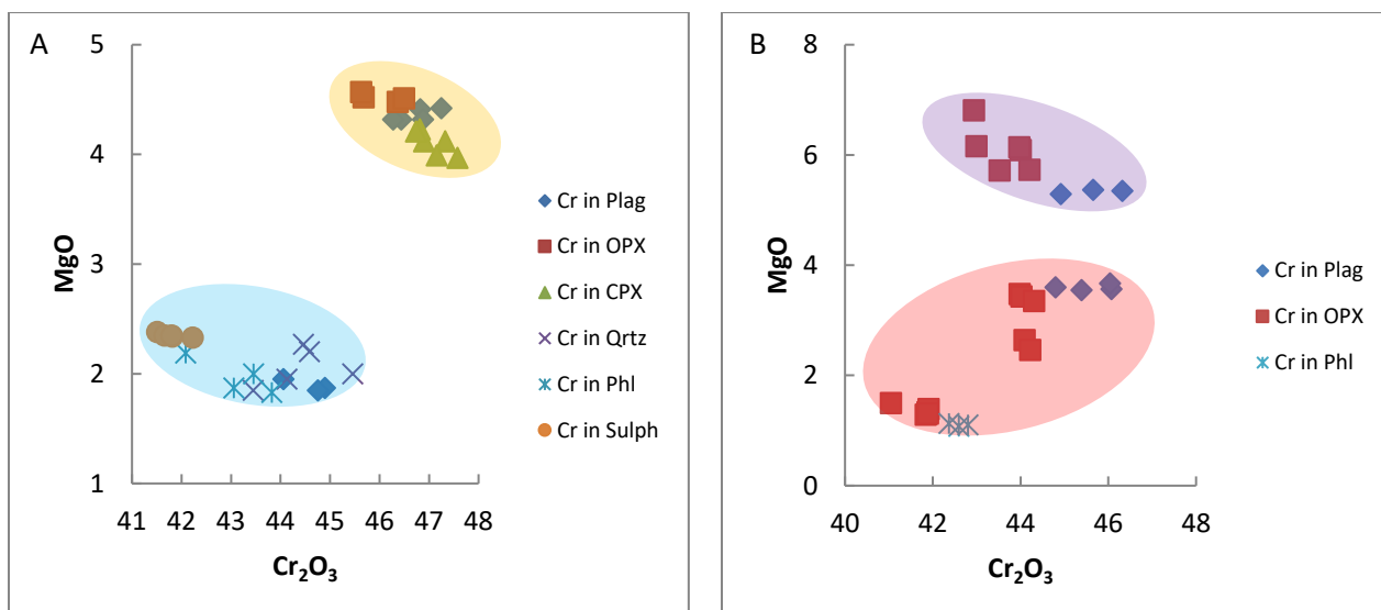
Figure 8-11: Geochemical graphs of chromite composition from feldspathic pyroxenite lithologies from the southwestern portion of the Uitloop farm; (A) \text{Cr}_2\text{O}_3 vs MgO (Blue: Z19-100.35, Orange: Z19-101.4) (B) \text{Cr}_2\text{O}_3 vs MgO (Red: Z19-101.6, Purple: Z19-137.5).
