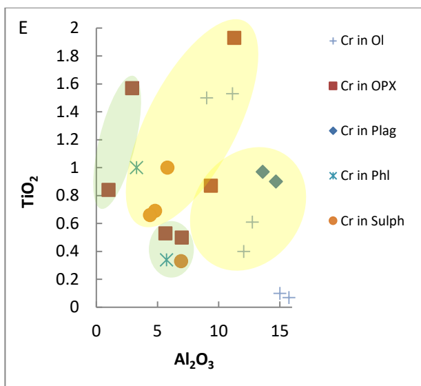
Figure 8-16: Geochemical graphs of chromite composition from feldspathic harzburgite (Yellow: Z20-66.5 & Green: Z20-111) lithologies from the southwestern portion of the Uitloop farm; (a) \text{Cr}_2\text{O}_3 vs \text{MgO} (b) \text{Cr}_2\text{O}_3 vs \text{Al}_2\text{O}_3 c) \text{Al}_2\text{O}_3 vs \text{MgO} D) \text{Cr}_2\text{O}_3 vs \text{TiO}_2 E) \text{Al}_2\text{O}_3 vs \text{TiO}_2 .
