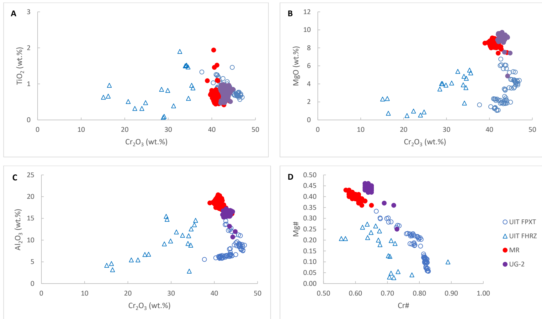
Figure 8-20: Compositional variation diagrams comparing the compositions of chromites from the southwestern portion of the Uitloop farm to those of the Merensky Reef (Li et al., 2005) and the UG-2 chromitite layer (Mondal & Mathez, 2007). (UIT FPXT = Uitloop feldspathic pyroxenite, UIT FHRZ = Uitloop feldspathic harzburgite, MR = Merensky Reef, UG-2 = UG-2 = Chromitite layer).
