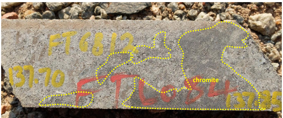
Figure 11-7: A photograph of sample Z19-137.7 (feldspathic pyroxenite).
