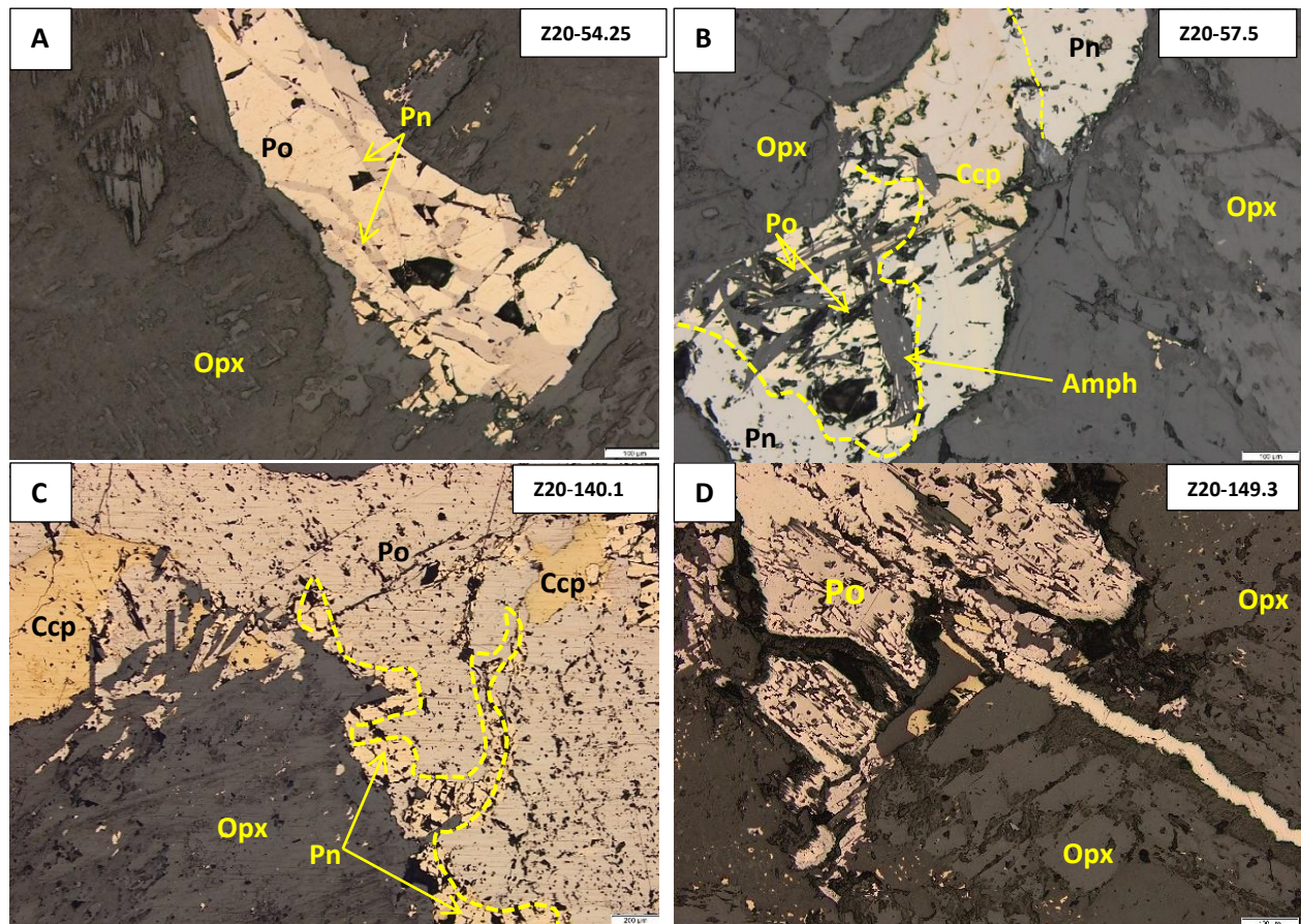
Figure 6-10: Photomicrographs under reflected light, of base metal sulphides observed within the magmatic rocks at the southwestern portion of the Uitloop farm. (A) Pentlandite exsolution in pyrrhotite. (B & C) Pyrrhotite replaced by needle-like amphibole (tremolite). (D) Pyrrhotite vein truncating orthopyroxene crystals. (Mgt= magnetite, Po= pyrrhotite, Pn = pentlandite, Ccp = chalcopyrite).
