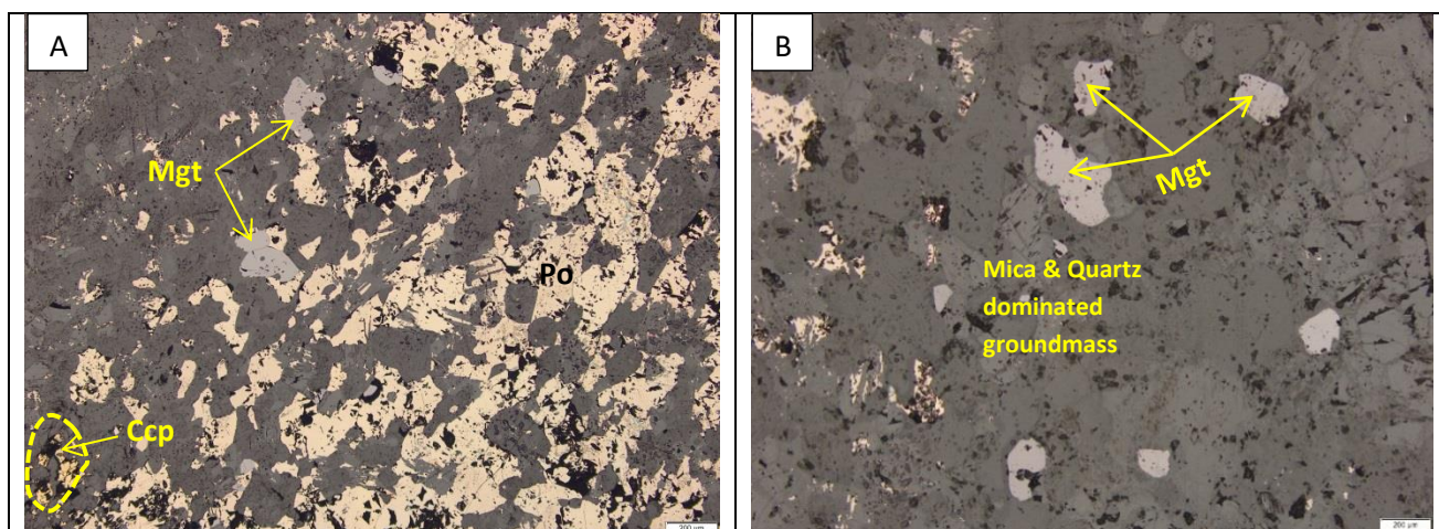
Figure 11-82: Photomicrographs, under reflected light, of mica-rich hornfels (sample Z20-184.4) from footwall rocks to the southwestern part of the Uitloop farm.
