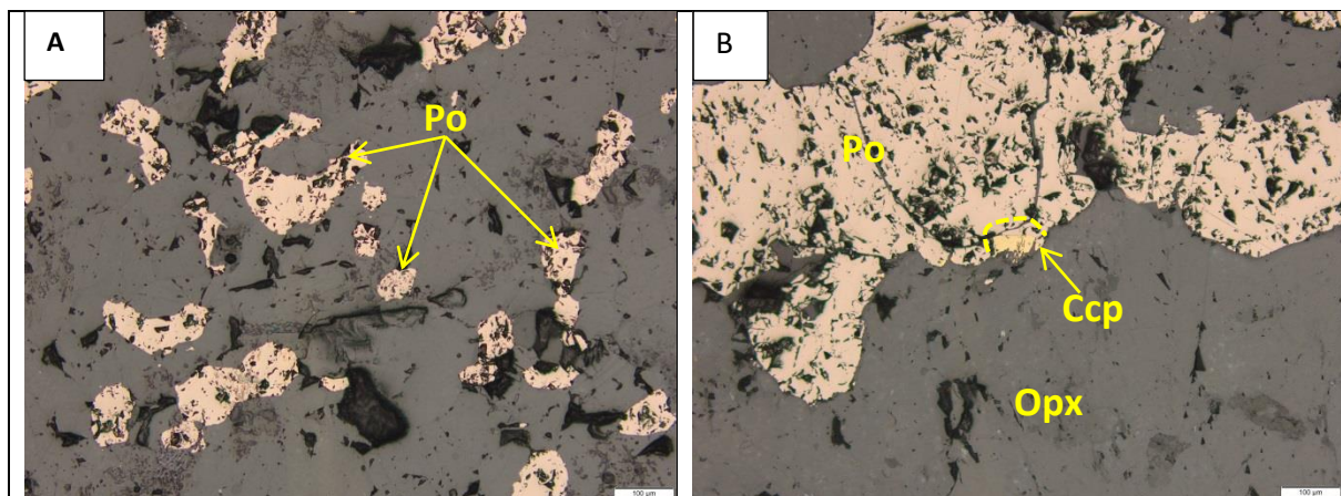
Figure 11-58: Photomicrographs, under reflected light, of sample Z19-195.5 (orthopyroxenite) from the southwestern part of Uitloop farm.
