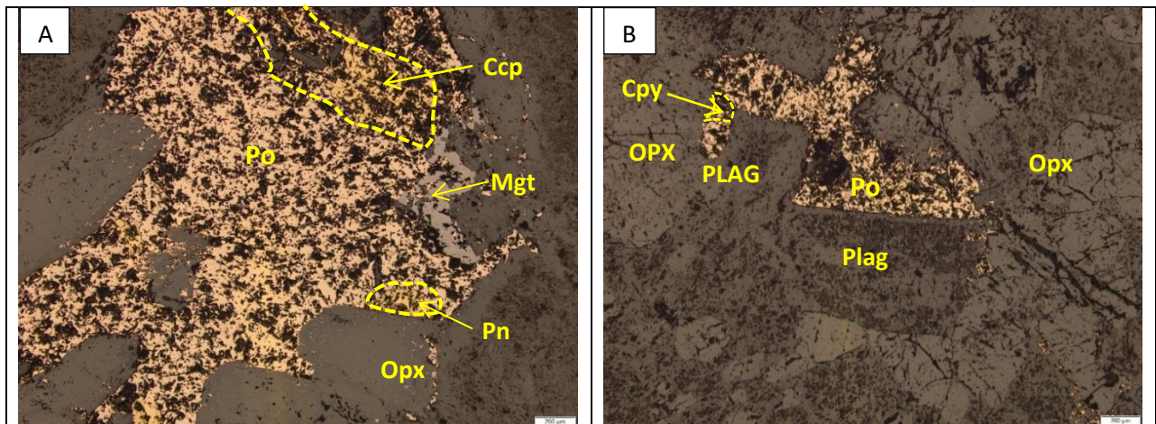
Figure 11-76: Photomicrographs, under reflected light, of feldspathic pyroxenite (sample Z20-173.7) from southwestern part of the Uitloop farm.
