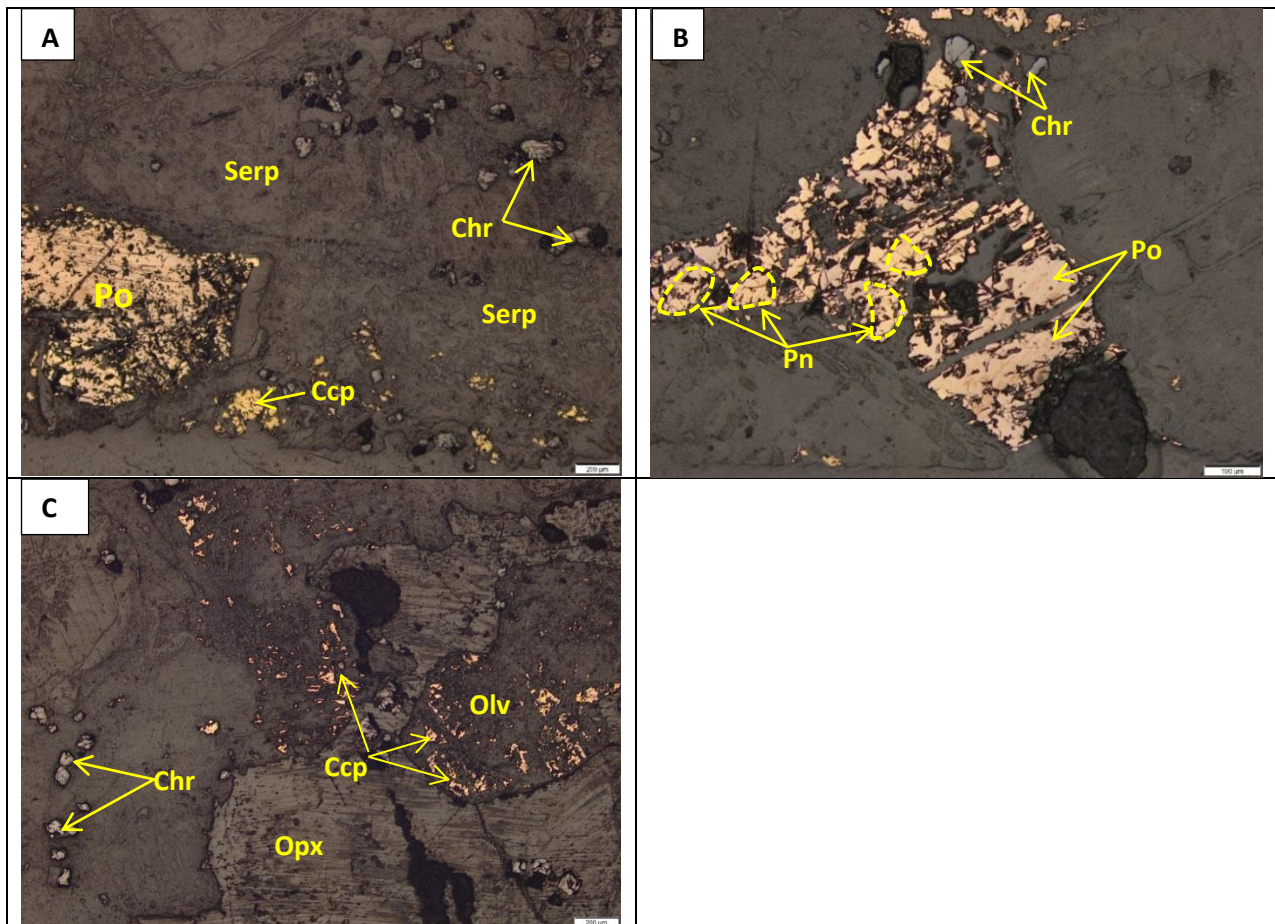
Figure 11-59: Photomicrographs, under reflected light, of sample Z20-53.7 (harzburgite) from the southwestern part of Uitloop farm.
