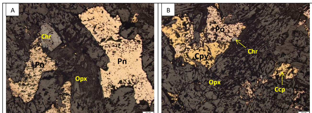
Figure 11-62: Photomicrographs, under reflected light, of sample Z20-57.9 (feldspathic pyroxenite) from the southwestern part of the Uitloop farm.
