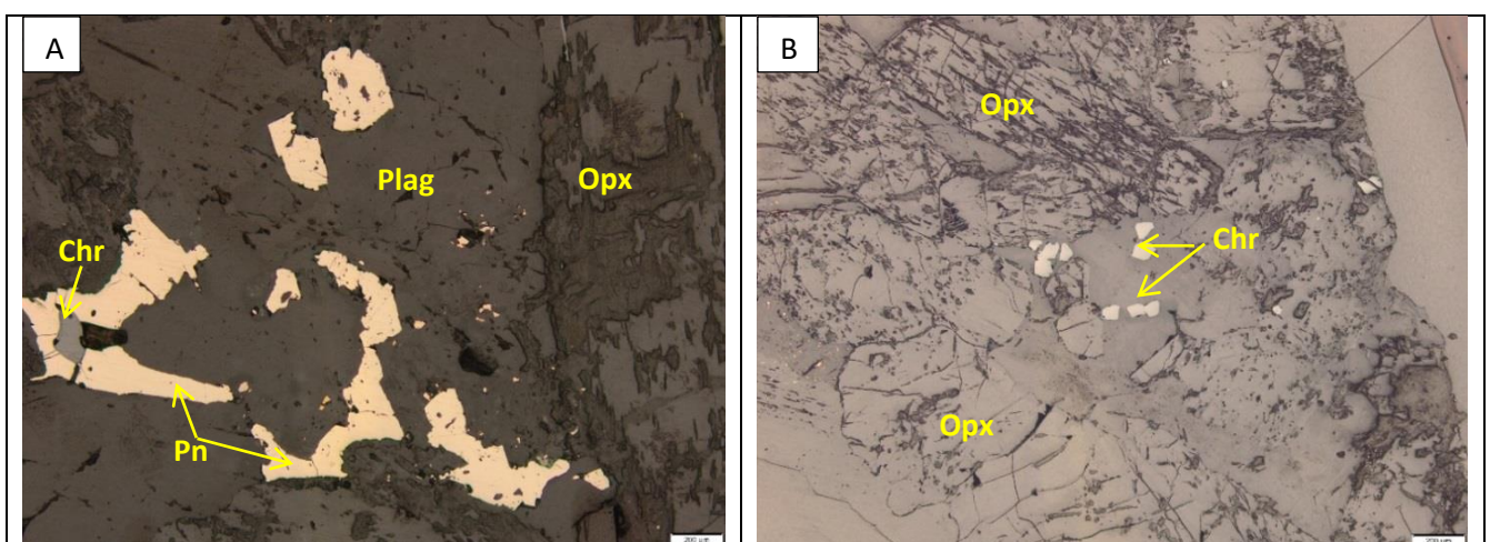
Figure 11-65: Photomicrographs, under reflected light, of sample Z20-83.2 (feldspathic pyroxenite) from the southwestern part of the Uitloop farm.
