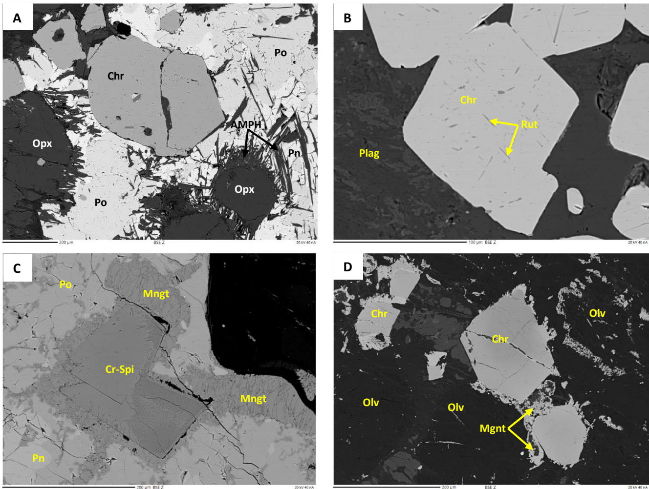
Figure 8-4: The morphology of chromite crystals from the southwestern part of the Uitloop farm. (A) Z20-100.35-3_9, subrounded chromite crystals enclosed by sulphides with needle-like amphibole intergrowths. (B) Z19-101.4_29, cumulus euhedral chromite with rutile exsolution in plagioclase. (C) Z20-66.5_23, BSE; Cr-Spinel with secondary magnetite along crystals boundaries enclosed by sulphide minerals. (D) Z20-66.5_26, BSE; chromite crystals rimmed by magnetite hosted by olivine. (Chr= chromite, Opx= orthopyroxene, Amph = Amphibole, Plag = plagioclase, Phl = phlogopite, Po = pyrrhotite, Pn = pentlandite, Mgnt = magnetite, Cr-Spi = Chromium-spinel, Rut = rutile).
