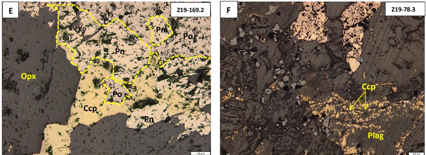
Figure 6-9: Photomicrographs under reflected light, of base metal sulphides observed within magmatic rocks at the southwestern portion of the Uitloop farm. (A & B) Sulphides associated with chromite grains. (C) Pyrrhotite rims around plagioclase and orthopyroxene. (D & E) Evidence of sulphide liquid fractionation. (F) Chalcopyrite remobilization into inclusions in plagioclase. (Chr = chromite, Mgt= magnetite, Po= pyrrhotite, Pn = pentlandite, Ccp = chalcopyrite).
