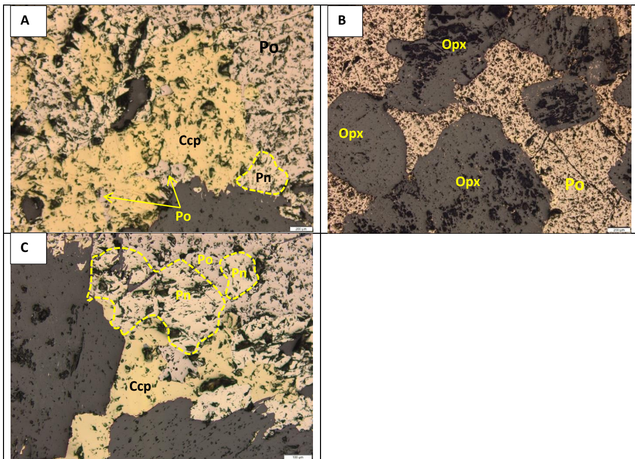
Figure 11-55: Photomicrographs, under reflected light, of sample Z19-169.2 (feldspathic pyroxenite) from the southwestern part of Uitloop farm.
