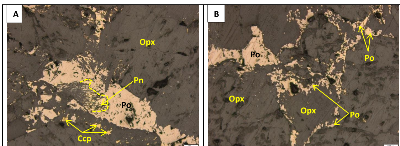
Figure 11-52: Photomicrographs, under reflected light, of sample Z19-101.6 (feldspathic pyroxenite) from the southwestern part of Uitloop farm.
