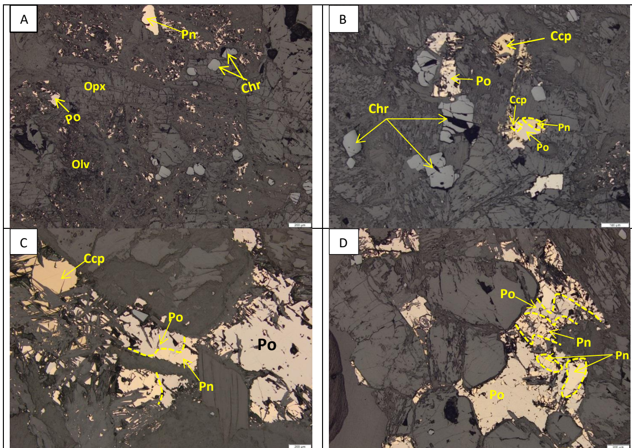
Figure 11-61: Photomicrographs, under reflected light, of sample Z20-57.5 (feldspathic harzburgite) from the southwestern part of the Uitloop farm.
