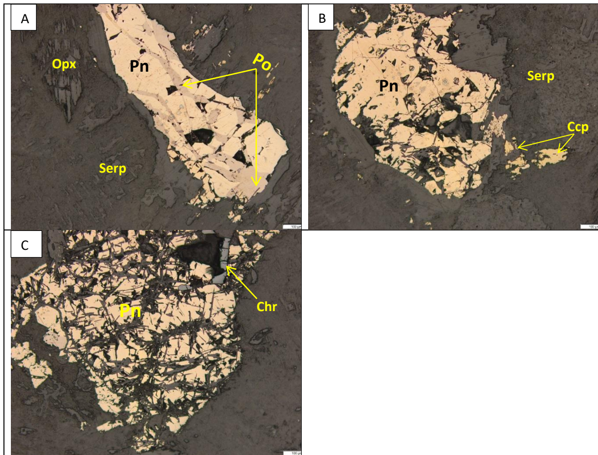
Figure 11-60: Photomicrographs, under reflected light, of sample Z20-54.25 (harzburgite) from the southwestern part of Uitloop farm.
