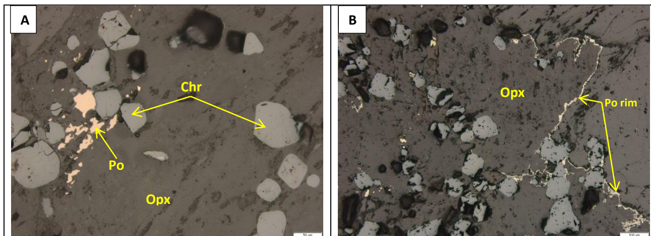
Figure 11-50: Photomicrographs, under reflected light, of sample Z19-101 (feldspathic pyroxenite) from the southwestern part of Uitloop farm.
