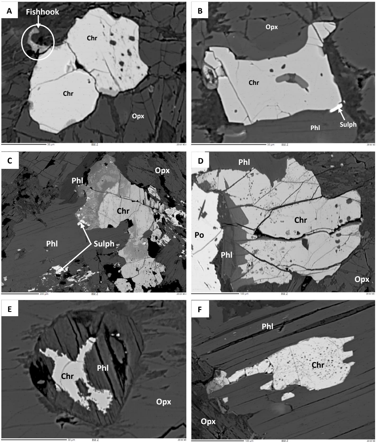
Figure 8-5: The morphology of the chromite crystals from the southwestern part of the Uitloop farm. (A) Z20-111-1_46, BSE; coarse interstitial anhedral chromite crystals with fish-hook, magnetite along crystals boundaries and silicate inclusions. (B) Z20-111-1_47, BSE; fish-hook chromite set between orthopyroxene and corroded by phlogopite, this chromite crystal also has silica inclusions. (C) Z20-111-2_48, BSE; amoeboidal chromite corroded by phlogopite, with sulphides and secondary magnetite (a fine-grained spinel phase) along crystals boundaries. (D) Z20-111-2_49, BSE; corroded sieve-textured chromite replaced by phlogopite and magnetite, (E) Z20-111-2_50, BSE; chromite relic within secondary phlogopite. (F) Z20-111-1_45, BSE; sieve textured chromite relic within secondary phlogopite. (Chr= chromite, Opx= orthopyroxene, Plag = plagioclase, Sulph = sulphide, Phl = phlogopite).
