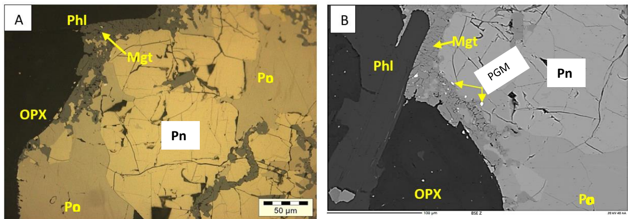
Figure 6-12: Photomicrographs under reflected light (A) and BSE (B), of base metal sulphides associated with feldspathic harzburgite, sample Z20-66.5. (A) Pyrrhotite and pentlandite rimmed by secondary magnetite. (B) Platinum group minerals (PGM) associated with secondary magnetite. (Mgt= magnetite, Po= pyrrhotite, Pn = pentlandite).
