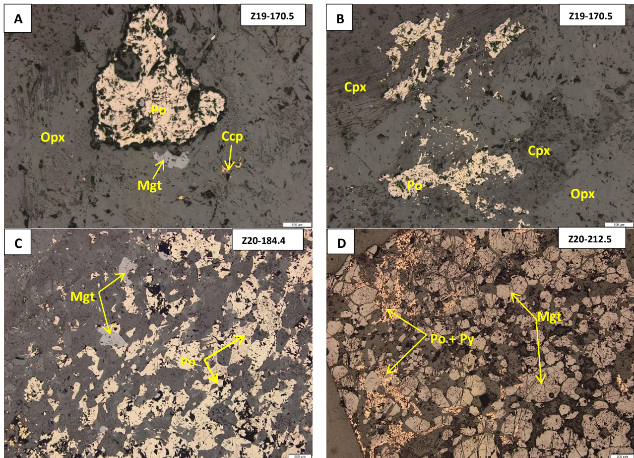
Figure 6-11: Photomicrographs under reflected light, of base metal sulphides in the footwall lithologies at the southwestern portion of the Uitloop farm; (A & B) parapyroxenite, (C) hornfels and (D) magnetite-rich calcsilicate. (Mgt= magnetite, Po= pyrrhotite, Py = Pyrite).
