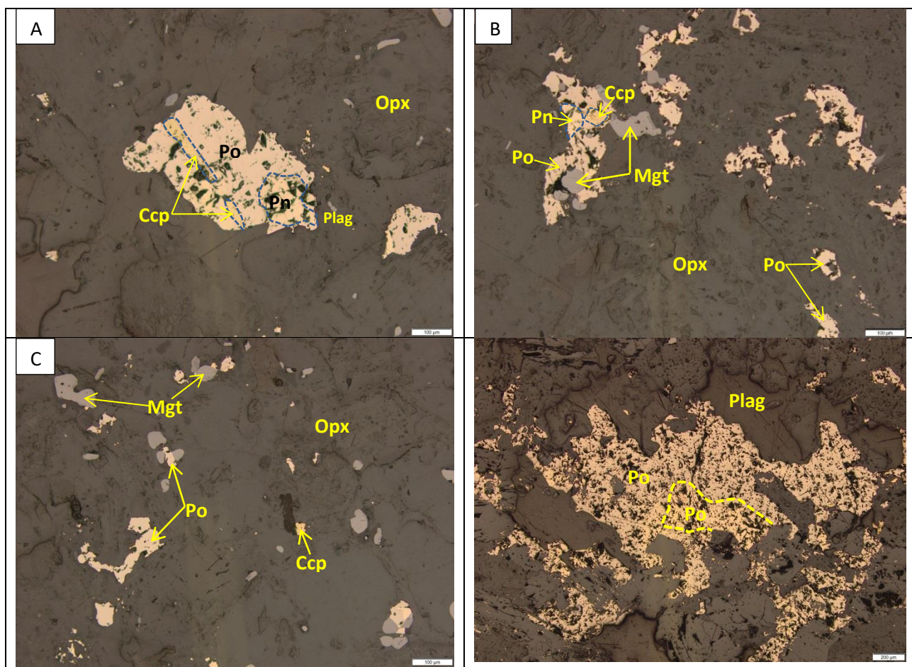
Figure 11-80: Photomicrographs, under reflected light, of feldspathic pyroxenite (sample Z2-176.1) from the southwestern part of the Uitloop farm.
