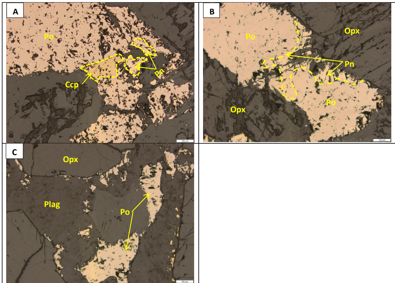
Figure 11-71: Photomicrographs, under reflected light, of feldspathic pyroxenite (Sample Z20-134.8) from the southwestern part of the Uitloop farm.
