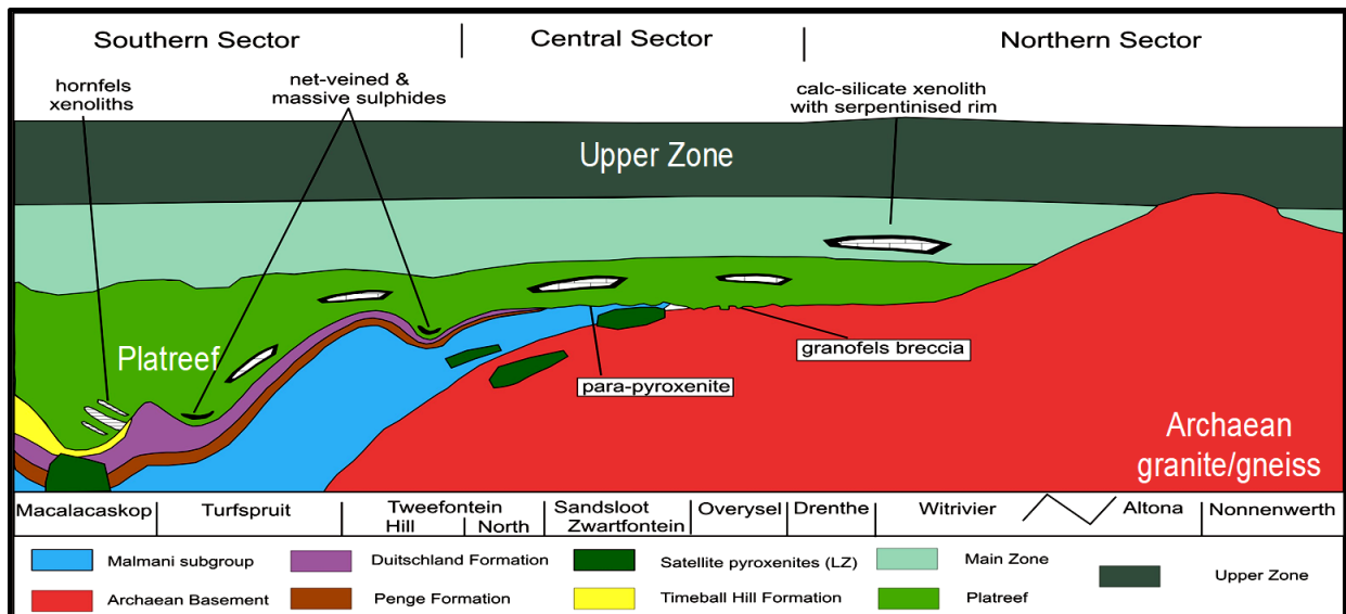
Figure 3-4: A schematic cross-section through the entire strike length of the Platreef (Kinnaid et al., 2005).
