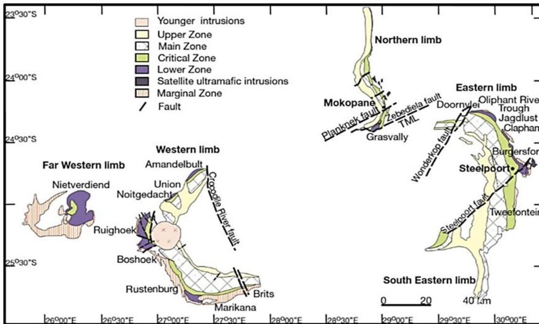
Figure 2-1: Geological map indicating different segments of the Rustenburg Layered Suite of the Bushveld Complex (Yudovskaya et al., 2013).
