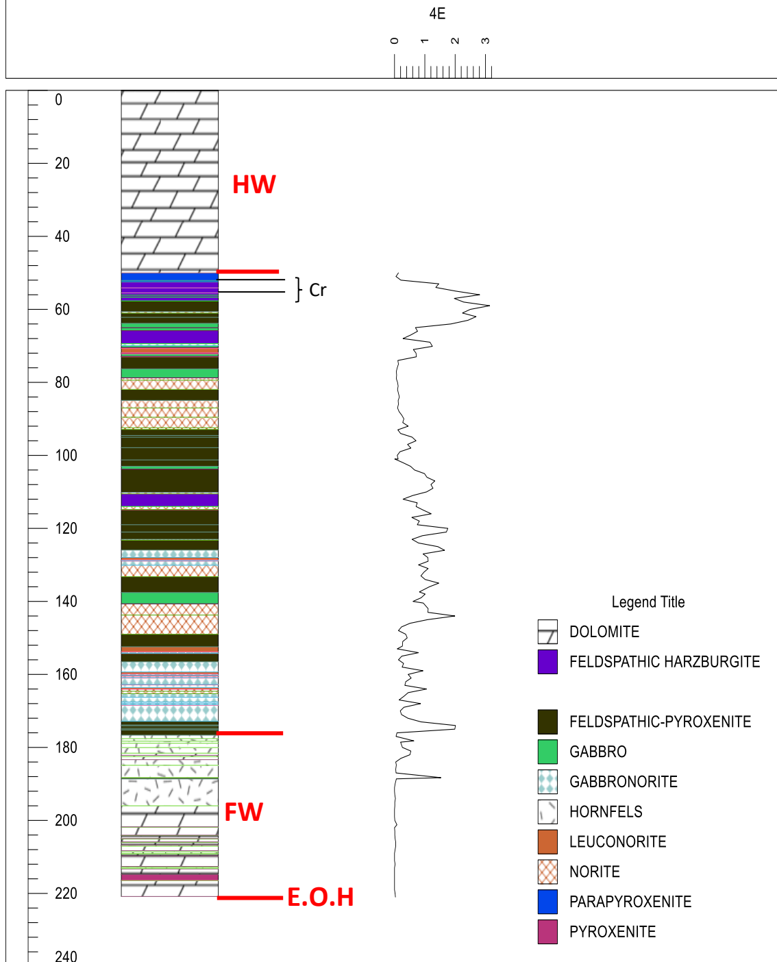
Figure 4-20: Simplified geological log of borehole Z20 indicating major stratigraphic positions; HW = hanging wall, Cr = chromite mineralisation, FW = footwall, E.O.H = end of hole, a graph displaying the down-hole 4E grade profile is also included.
