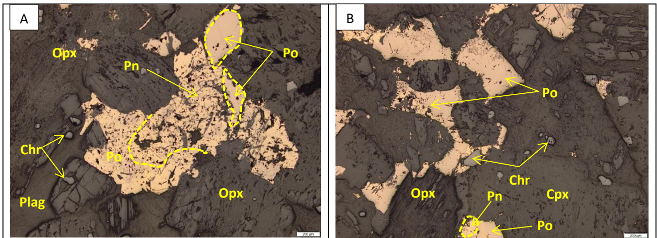
Figure 11-63: Photomicrographs, under reflected light, of sample Z20-62.7 (feldspathic pyroxenite) from the southwestern part of the Uitloop farm.
