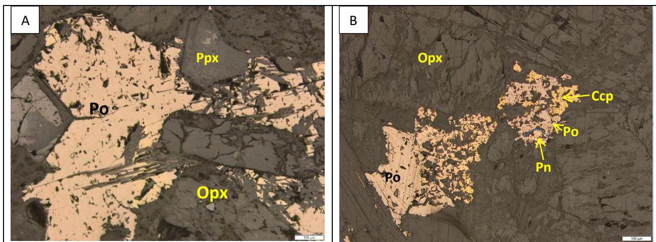
Figure 11-67: Photomicrographs, under reflected light, of sample Z20-111 (feldspathic harzburgite) from the southwestern part of the Uitloop farm.
