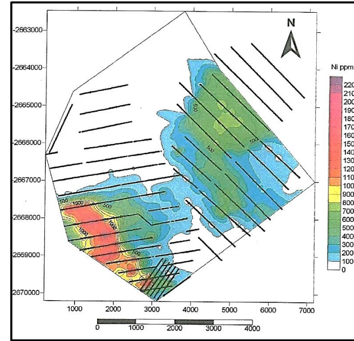
Figure 1-4: Southern Era soil geochemical contour maps indicating nickel (Ni) anomalies on the Uitloop farm (Lowman, 2007)
