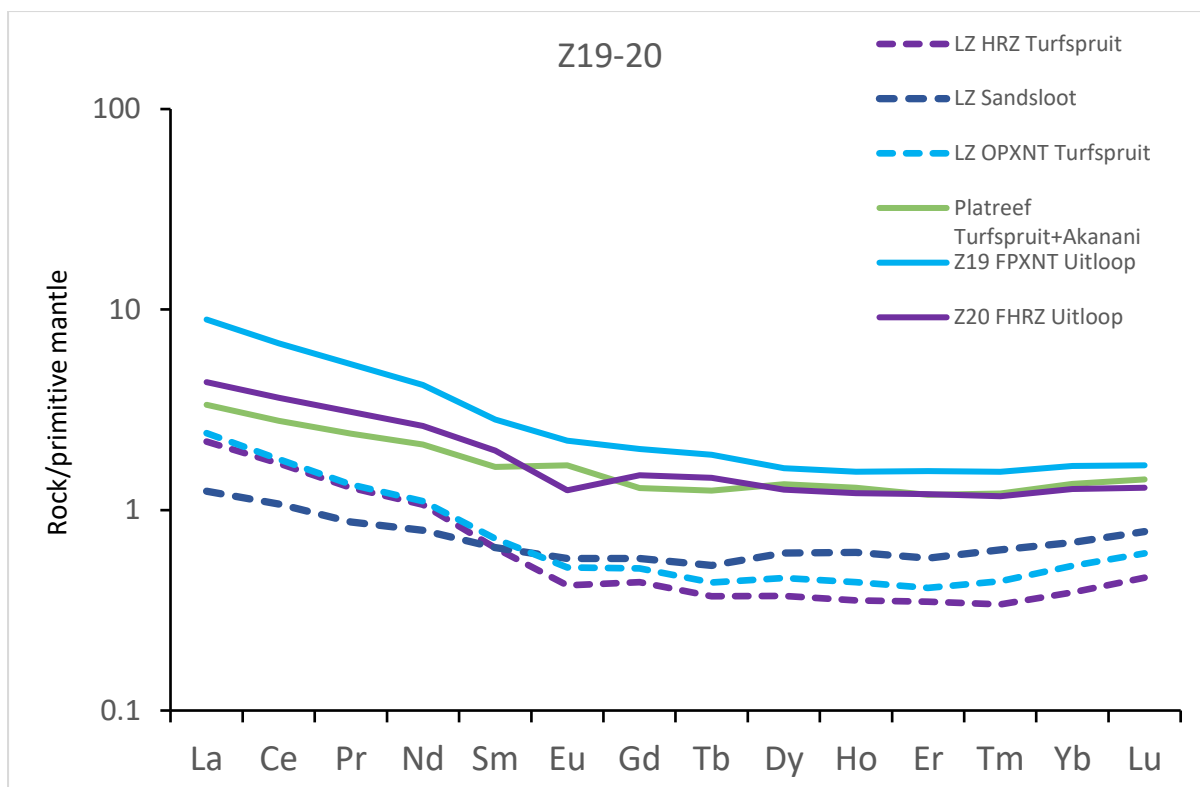
Figure 7-12: Primitive mantle normalized REE graphs (normalised to data by Hoffman (1988)) of the ultramafic rocks from the southwestern part of the Uitloop farm compared to the Lower Zone data from Turfspruit and Sandsloot and Platreef data from Turfspruit and Akanani (data supplied by Dr M. Yudovskaya).
