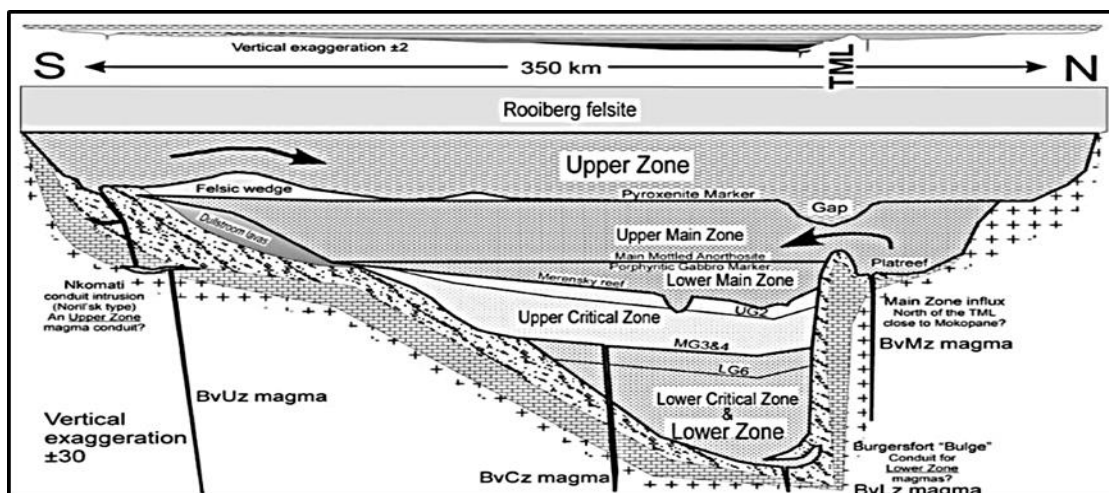
Figure 2-2: A north-south cross section through the Rustenburg Layered Suite of the Bushveld Complex (Kruger, 2005).
