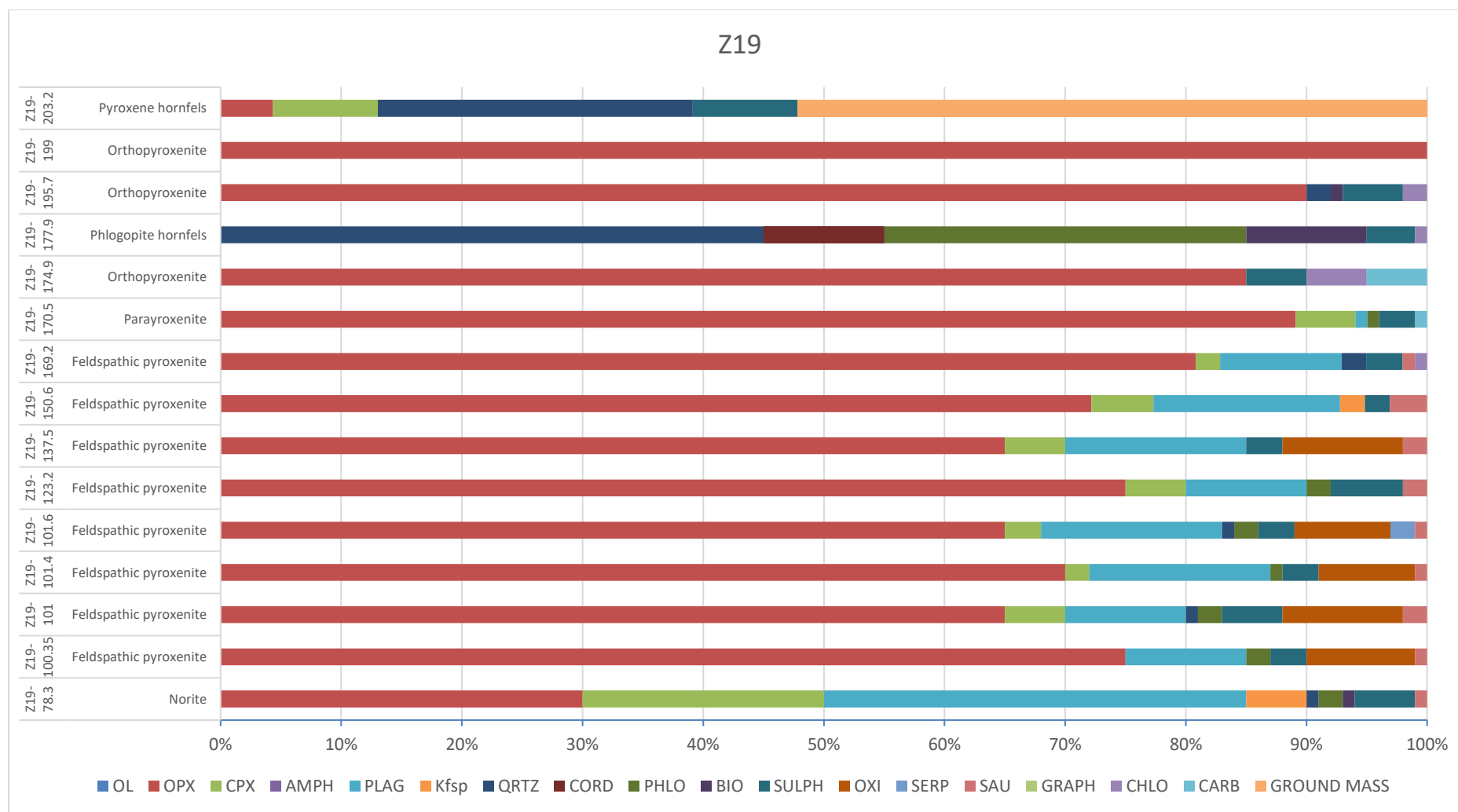
Figure 11-46: Modal mineralogy estimation bar chart for borehole Z19 thin sections.
