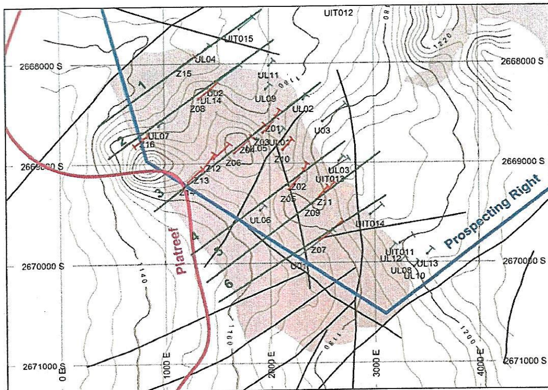
Figure 1-5: Map showing the historical boreholes across the Uitloop II body. (Croll et al., 2012).
