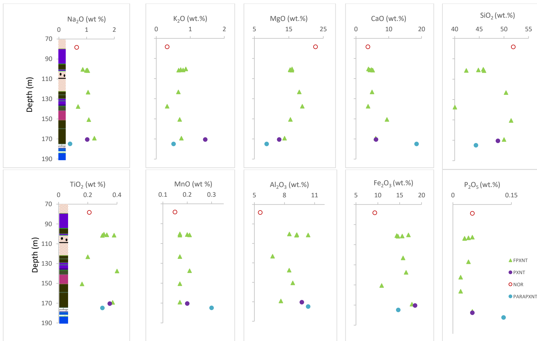
Figure 7-7-1: Variation in major element concentrations with stratigraphic height in borehole Z19. (FPXNT = feldspathic pyroxene, PXNT = pyroxenite, NOR = norite, PARAPXNT = parapyroxenite).
