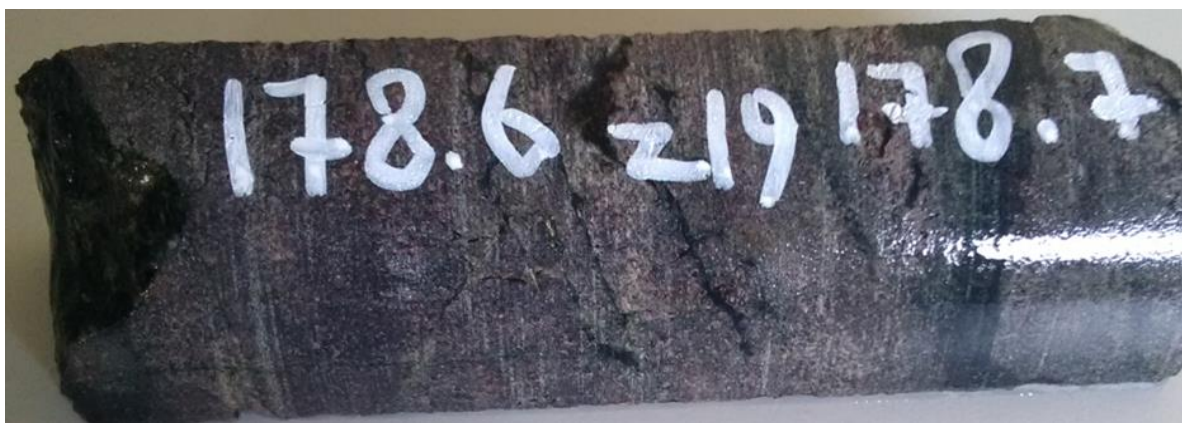
Figure 11-14: A photograph of sample Z19-178.6 (hornfels).
