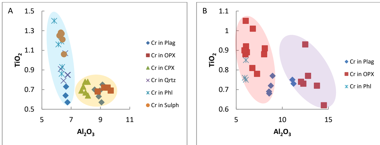
Figure 8-15: Geochemical plots of chromite composition from feldspathic pyroxenite lithologies from the southwestern portion of the Uitloop farm; (A) \text{Al}_2\text{O}_3 vs \text{TiO}_2 (Blue: Z19-100.35, Orange: Z19-101.4) (B) \text{Al}_2\text{O}_3 vs \text{TiO}_2 (Red: Z19-101.6, Purple: Z19-137.5).
