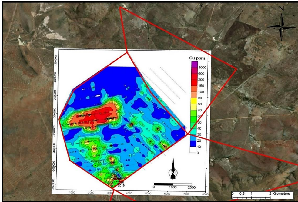
Figure 1-3: SouthernEra soil geochemical contour map indicating Copper (Cu) anomalies on the Uitloop farm (Lowman, 2007).
