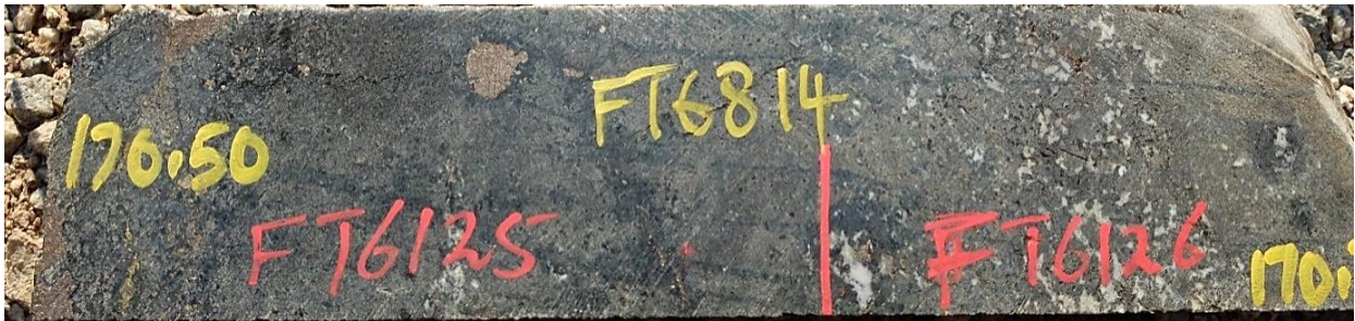
Figure 6-6: A photograph of borehole core samples showing parapyroxenite with sulphide blebs, sample Z19-170.5.
