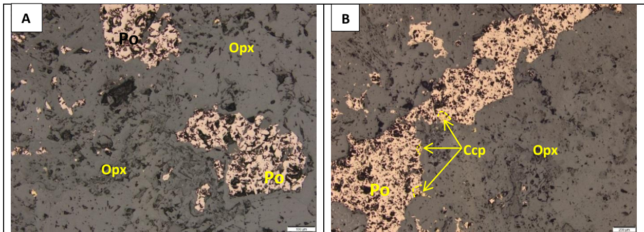
Figure 11-57: Photomicrographs, under reflected light, of sample Z19-174.9 (parapyroxenite) from the southwestern part of Uitloop farm.
