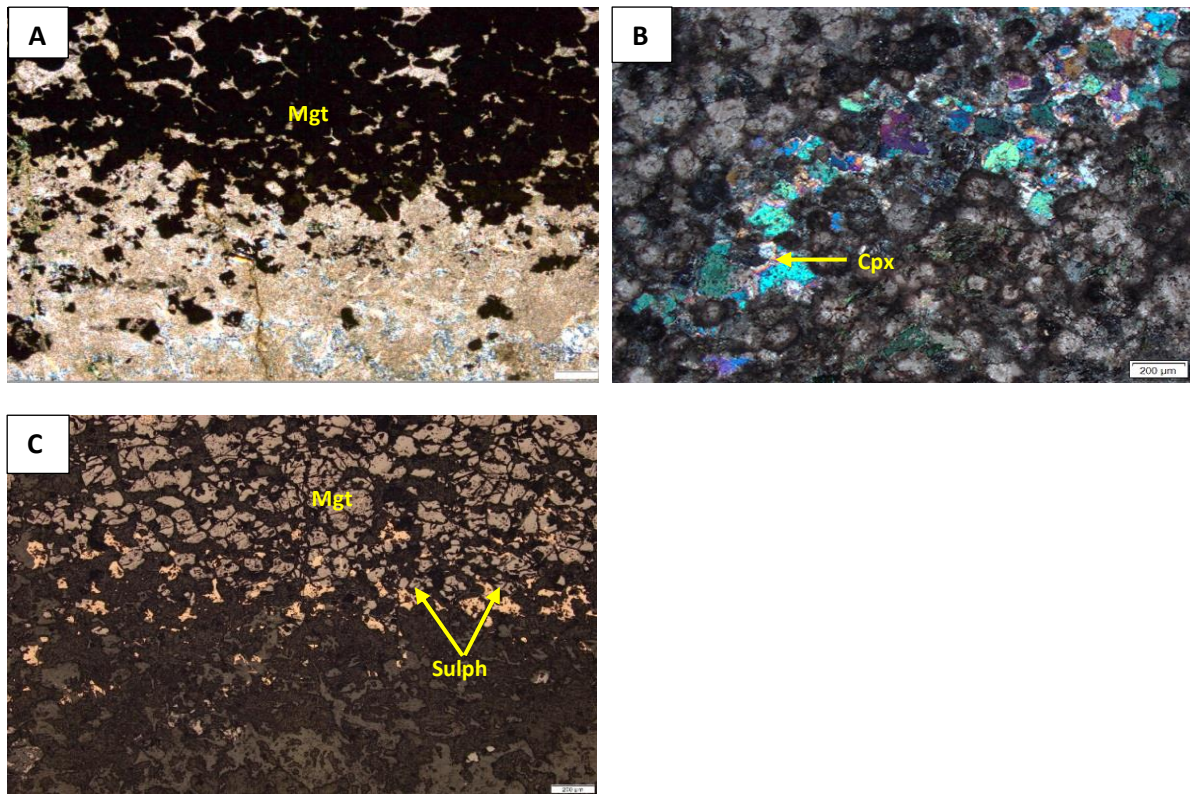
Figure 5-9: Photomicrographs, taken under XPL in transmitted light (A-B) and taken in reflected light (C), of calcsilicate with magnetite bands, sample Z20-212.5, from footwall lithologies at the southwestern portion of the Uitloop farm. (A) Magnetite grains in an altered calcsilicate. (B) Clinopyroxene crystals within altered brown crystal mush. (C) Magnetite and Base Metal Sulphides.
