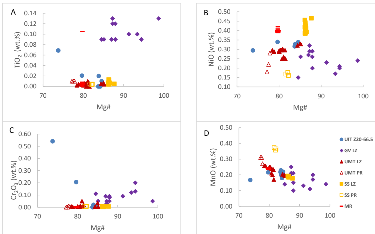
Figure 8-23: Compositional variation diagrams comparing the compositions of olivine crystals from the southwestern portion of the Uitloop farm (UIT) magmatic lithologies to those of the Lower Zone (LZ) and Platreef (PR) olivine crystals from Turfspruit (UMT), Sandsloot (SS) (Yudovskaya & Kinnaird, 2013), Grasvalley farms (GV) (Hulbert, 1983) and Merensky Reef (MR) (Naldrett et al., 2009).
