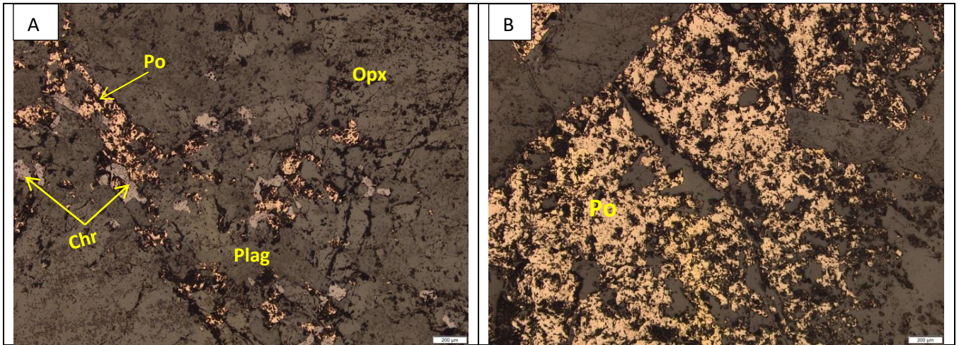
Figure 11-75: Photomicrographs, under reflected light, of norite (sample Z20-153.5) from the southwestern part of the Uitloop farm.
