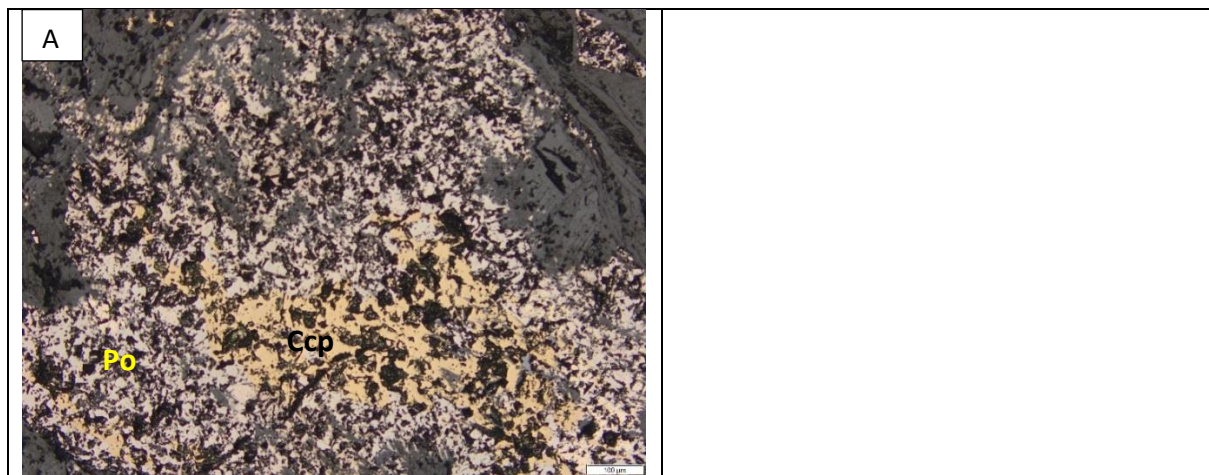
Figure 11-79: Photomicrographs, under reflected light, of feldspathic pyroxenite (sample Z20-176) from the southwestern part of the Uitloop farm.
