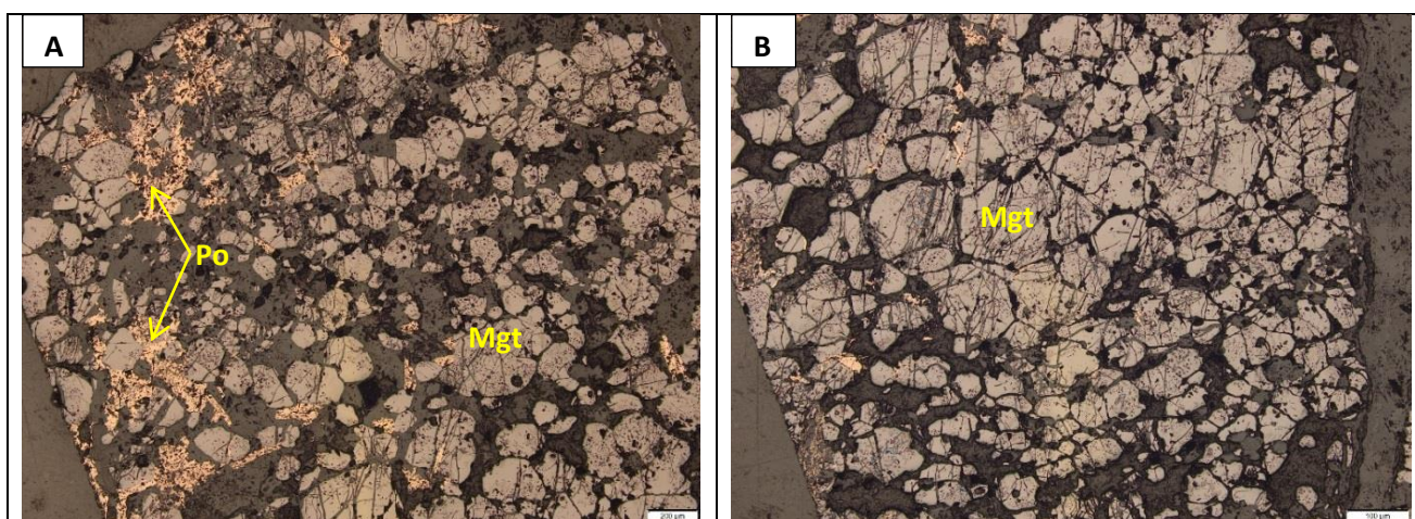
Figure 11-84: Photomicrographs, under reflected light, of dolomite with alternating magnetite bands (sample Z20-212.5) from footwall rocks southwestern part of the Uitloop farm.
