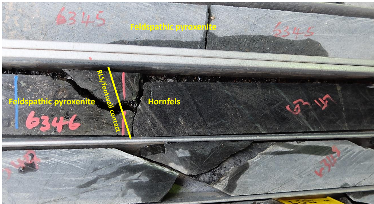
Figure 4-15: A photograph of borehole core sample showing a sharp contact between the Feldspathic pyroxenite and the metasedimentary footwall lithologies (mica-rich hornfels) of the Transvaal Supergroup at a depth of 176.1m in borehole Z20.
