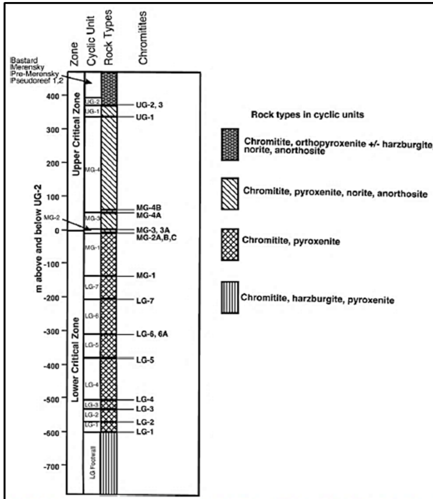
Figure 2-4: The stratigraphic positions of the chromitite layers within the Critical Zone (Naldrett et al., 2009).
