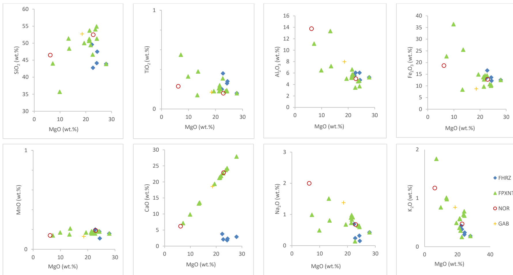
Figure 7-4: Binary variation diagrams showing major elements concentrations (wt. %) versus MgO content (wt. %) in borehole Z20 lithologies. (FHRZ = Feldspathic harzburgite, FPXNT = Feldspathic pyroxene, NOR = Norite, GAB = Gabbro).
