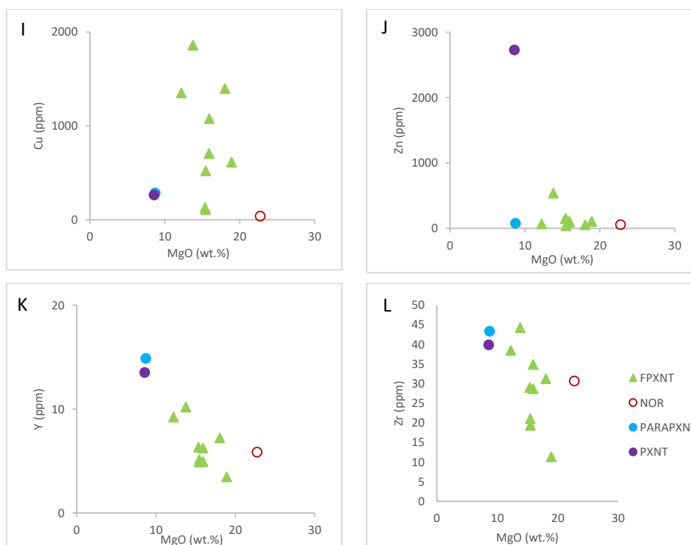
Figure 7-7: Binary variation diagrams showing selected trace elements (Rb, Sr, Ba, Sc, V, Cr, Co, Ni, Cu, Zn, Y, Zr & Ga) concentrations (ppm) versus MgO content (wt.%) in borehole Z19 lithologies.
