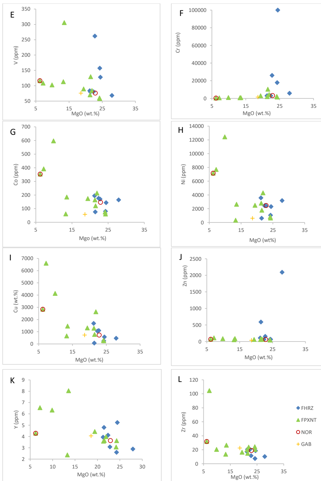
Figure 7-8: Binary variation diagrams showing selected trace elements (Rb, Sr, Ba, Sc, V, Cr, Co, Ni, Cu, Zn, Y & Zr) concentrations (ppm) versus MgO content (wt.%) in borehole Z20 lithologies.
