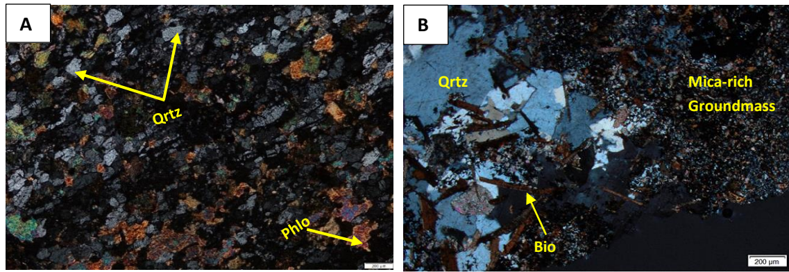
Figure 5-8: Photomicrographs, under XPL, of phlogopite hornfels from footwall lithologies at the southwestern portion of the Uitloop farm. (A) Fine-grained phlogopite hornfels, sample Z19-177.9. (B) Randomly orientated biotite laths associated with quartz grains in biotite hornfels, sample Z20-194.4.
