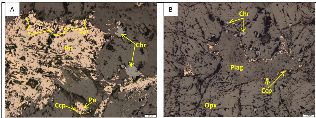
Figure 11-66: Photomicrographs, under reflected light, of sample Z20-107.7 (feldspathic pyroxenite) from the southwestern part of the Uitloop farm.
