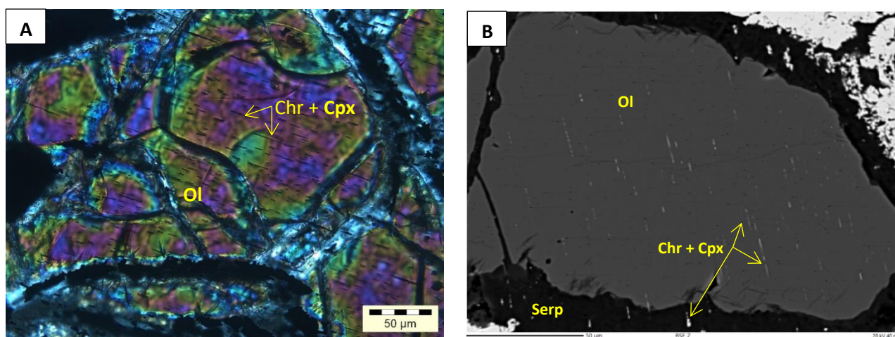
Figure 8-21: Photomicrographs of olivine crystals under XPL (A) and BSE (B). (A) Z20-66.5, transmitted cross polarized light; chromite and clinopyroxene lamellae in olivine. (B) Z20-66.5-3_44, BSE; chromite and clinopyroxene lamellae in olivine. (Ol = Olivine, Serp = Serpentine, Chr = Chromite, Cpx = Clinopyroxene).
