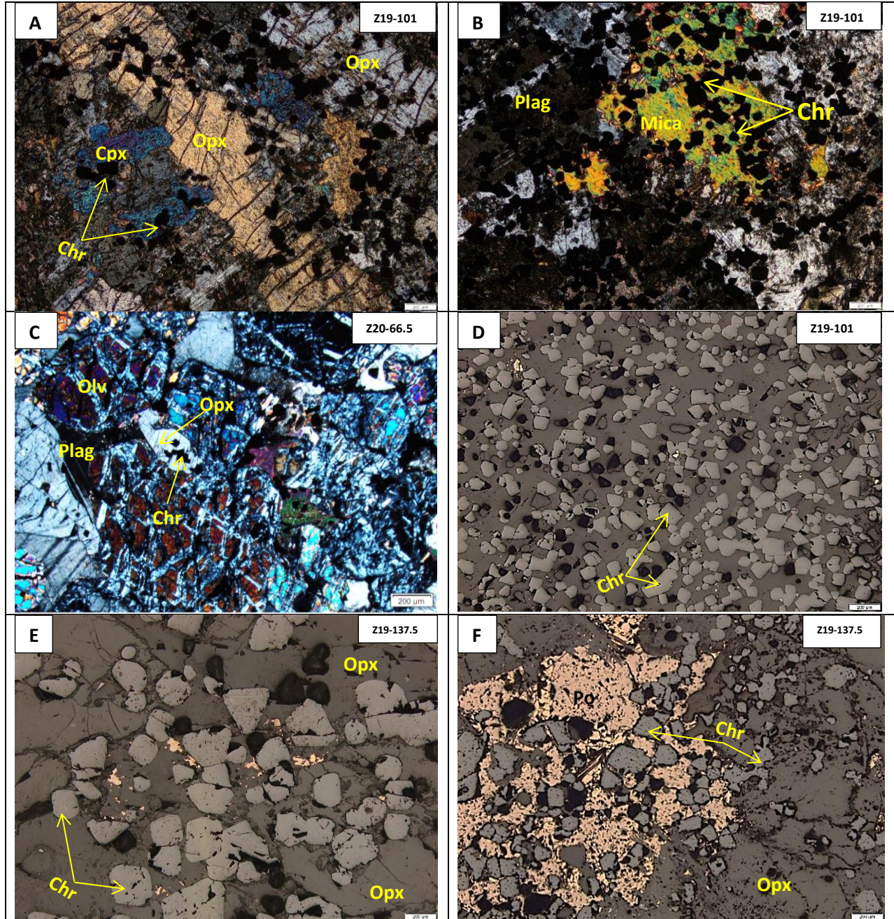
Figure 6-3: Photomicrographs of chromite under XPL in transmitted light (A, B & C) and reflected light (D, E & F). (A) Chromite disseminations within cumulus pyroxene, (B) plagioclase (B) and mica in feldspathic pyroxenite. (C) Chromite inclusions within olivine in feldspathic harzburgite and (D) feldspathic pyroxenite. (E) Annealing chromite crystals. (F) Chromite crystals in close association with pyrrhotite.
