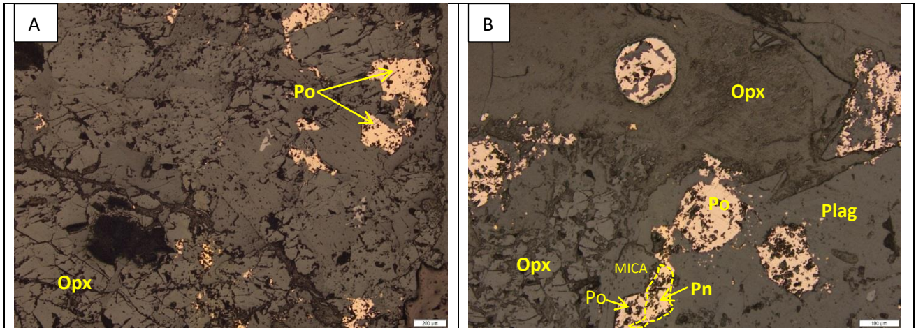
Figure 11-78: Photomicrographs, under reflected light, of feldspathic pyroxenite (sample Z20-175.9) from the southwestern part of the Uitloop farm.
