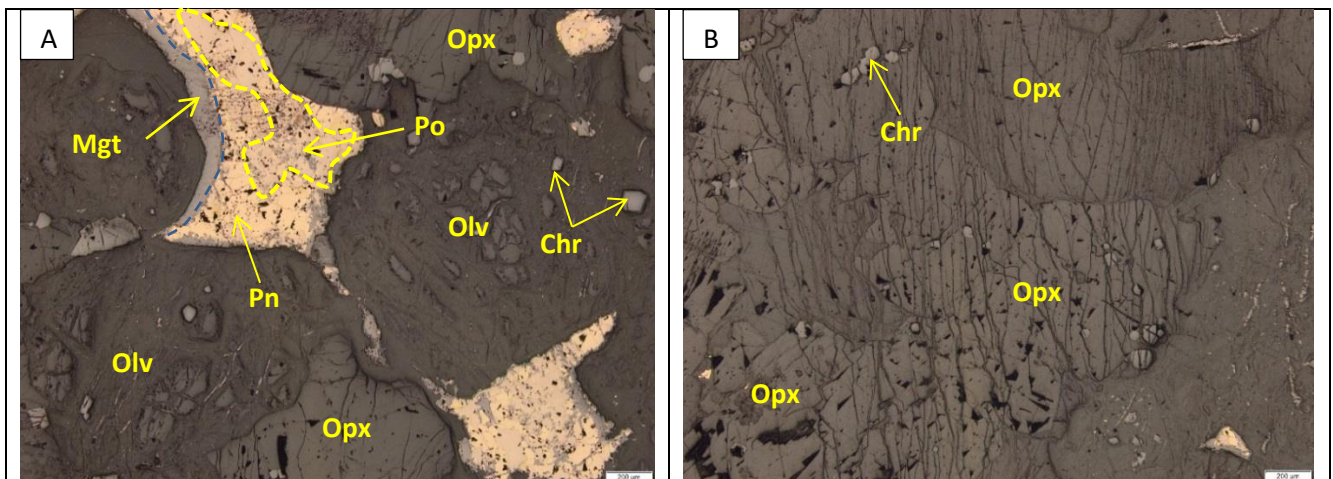
Figure 11-64: Photomicrographs, under reflected light, of sample Z20-66.5 (feldspathic harzburgite) from the southwestern part of the Uitloop farm.
