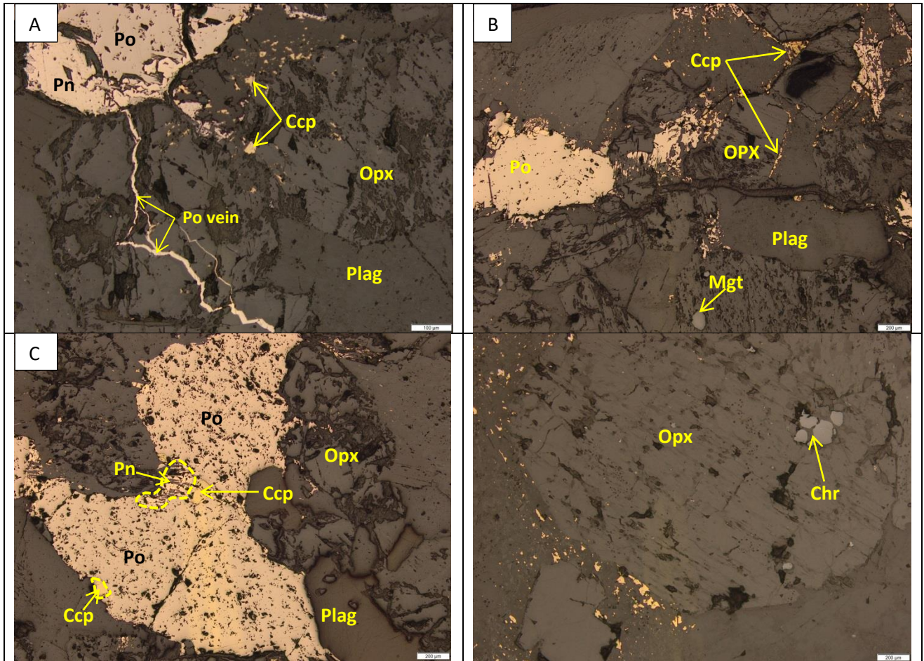
Figure 11-73: Photomicrographs, under reflected light, of feldspathic pyroxenite (sample Z20-149.3) from the southwestern part of the Uitloop farm.
