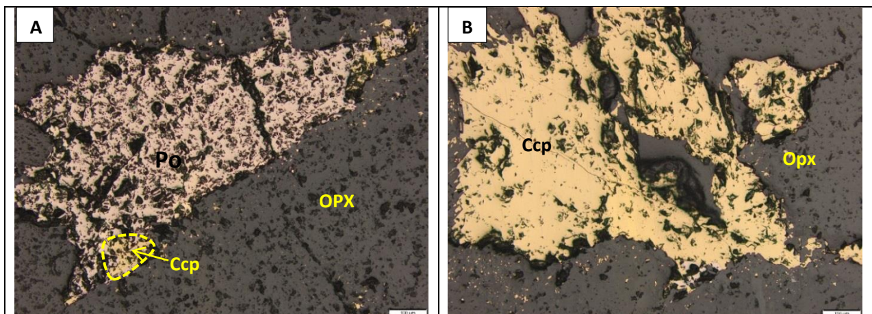
Figure 11-54: Photomicrographs, under reflected light, of sample Z19-150.6 (feldspathic pyroxenite) from the southwestern part of Uitloop farm.
