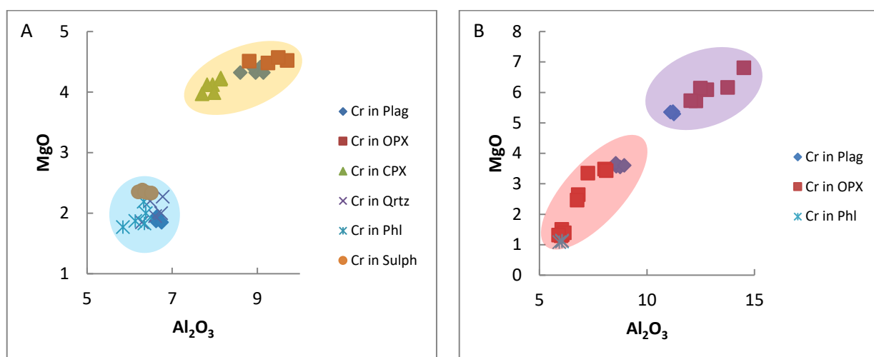
Figure 8-13: Geochemical graphs of chromite composition from feldspathic pyroxenite lithologies from the southwestern portion of the Uitloop farm; (A) \text{Al}_2\text{O}_3 vs \text{MgO} (Blue: Z19-100.35, Orange: Z19-101.4) (B) \text{Al}_2\text{O}_3 vs \text{MgO} Red: Z19-101.6, Purple: Z19-137.5).
