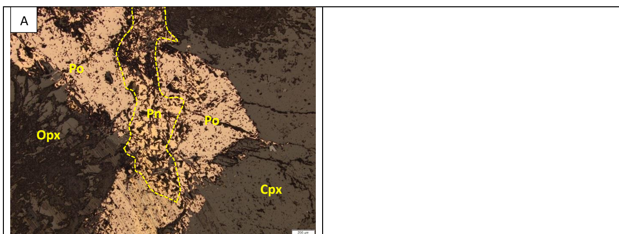
Figure 11-68: Photomicrographs, under reflected light, of sample Z20-120.75 (feldspathic pyroxenite) from the southwestern part of the Uitloop farm.
