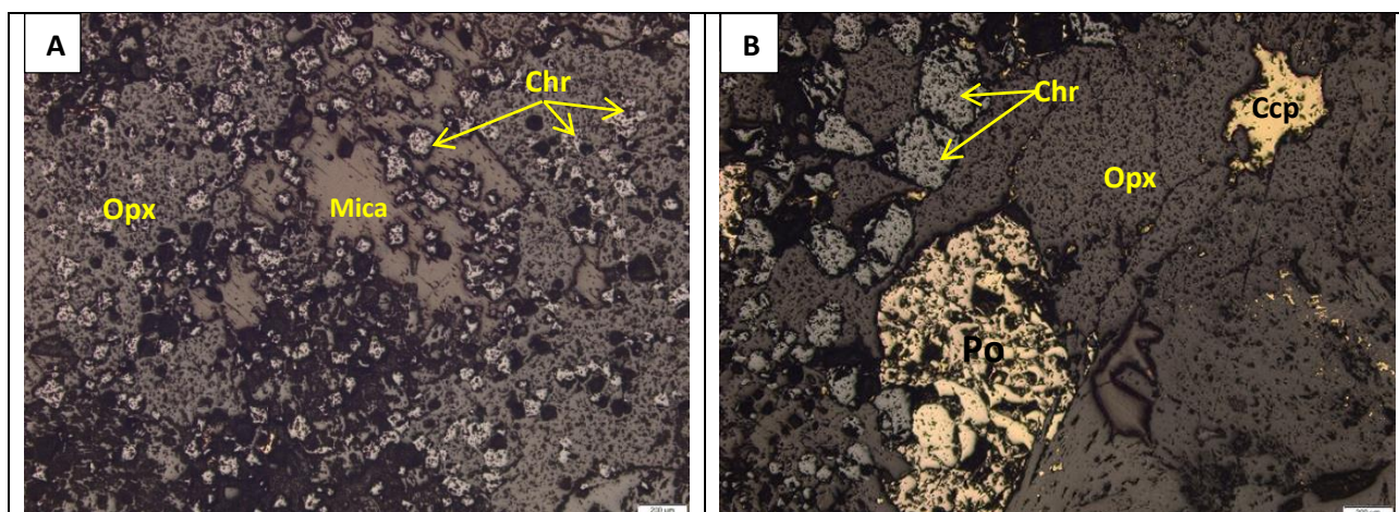
Figure 11-49: Photomicrographs, under reflected light, of sample Z19-100.35 (feldspathic pyroxenite) from the southwestern part of Uitloop farm.
