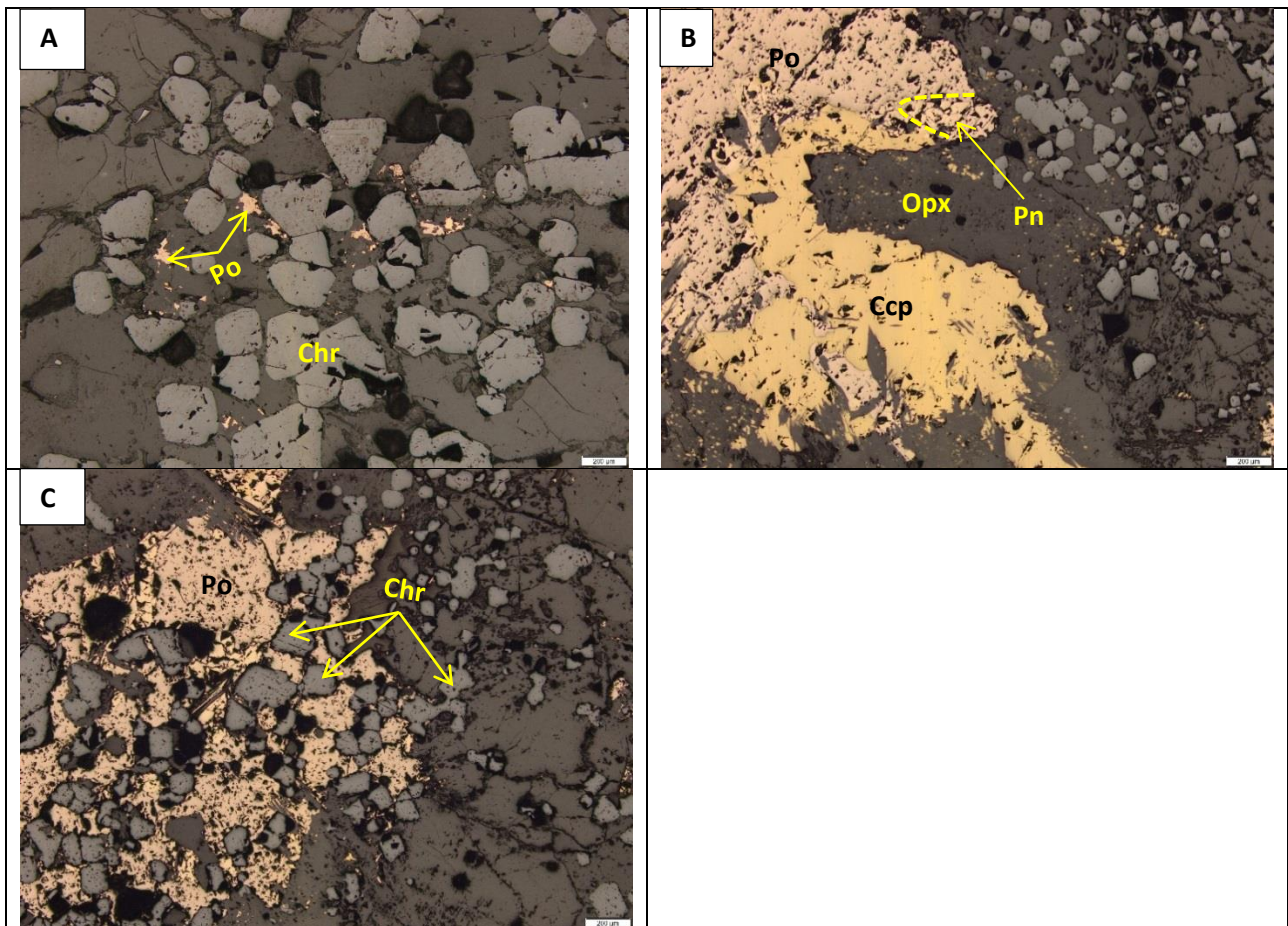
Figure 11-53: Photomicrographs, under reflected light, of sample Z19-123.2 (feldspathic pyroxenite) from the southwestern part of Uitloop farm.
