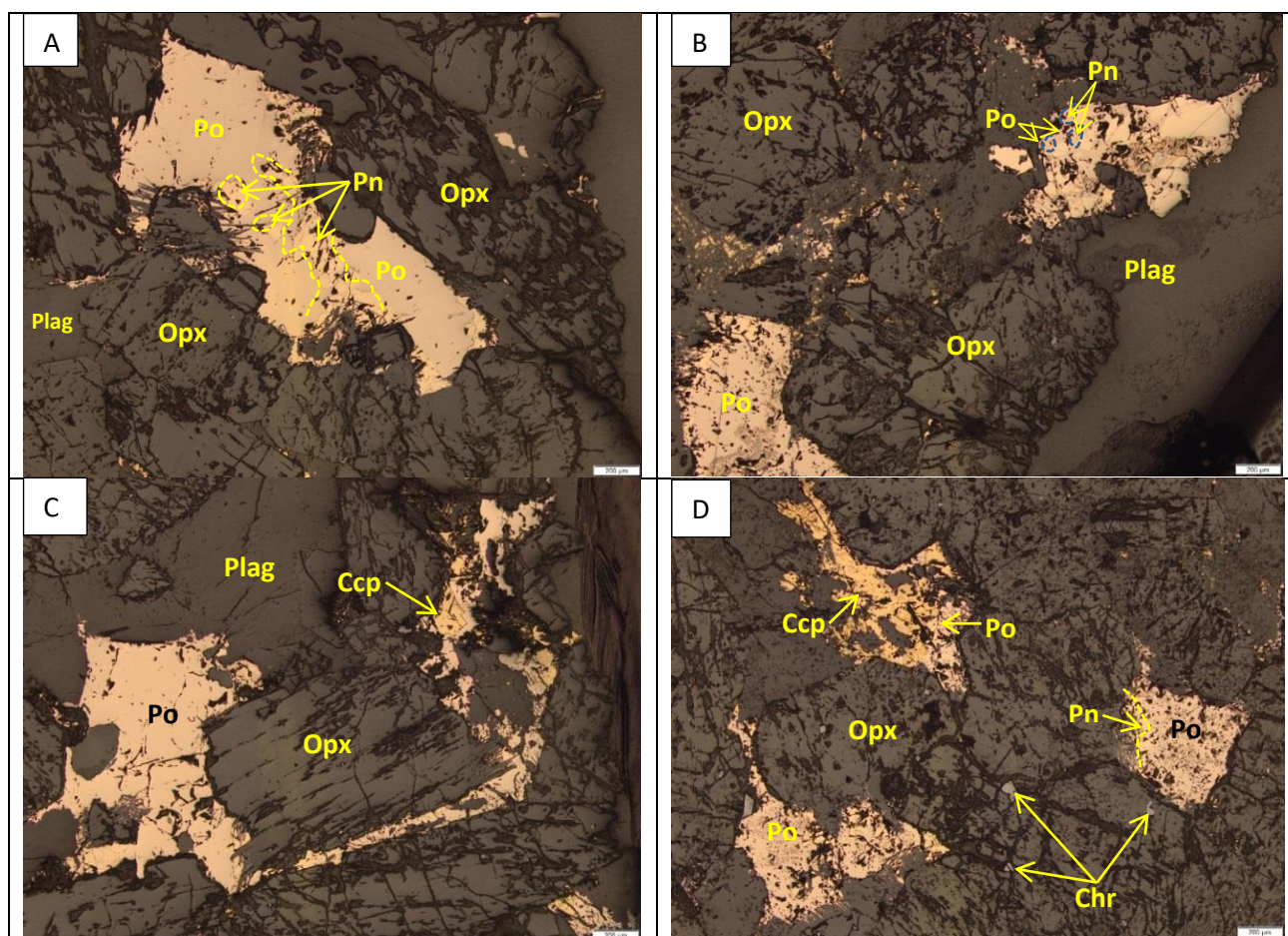
Figure 11-70: Photomicrographs, under reflected light, of feldspathic pyroxenite (Sample Z20-124.8) from the southwestern part of the Uitloop farm.
