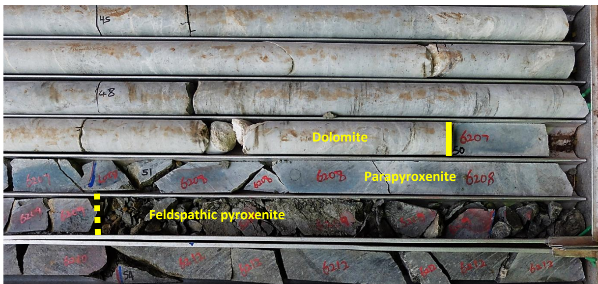
Figure 4-1: In borehole Z20, a 2.5 m thick assimilation zone (parapyroxenite) separates the dolomite hanging wall from the underlying feldspathic pyroxenite of the Bushveld Complex.
