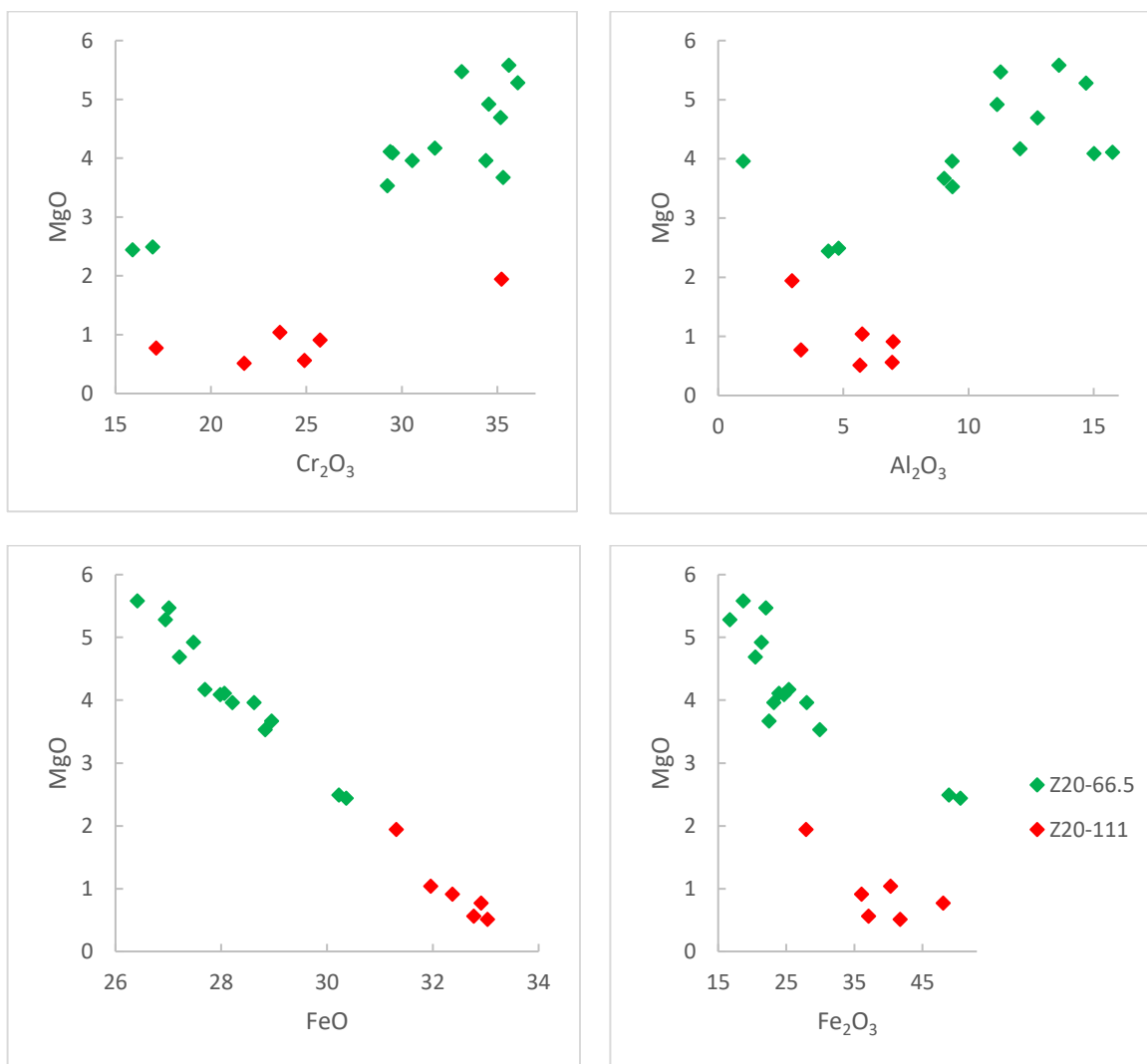
Figure 8-8: Geochemical graphs of chromite composition from feldspathic harzburgite lithologies from the southwestern portion of the Uitloop farm; (A) \text{Cr}_2\text{O}_3 vs MgO (B) \text{Al}_2\text{O}_3 vs MgO (C) FeO vs MgO (D) \text{Fe}_2\text{O}_3 vs MgO
