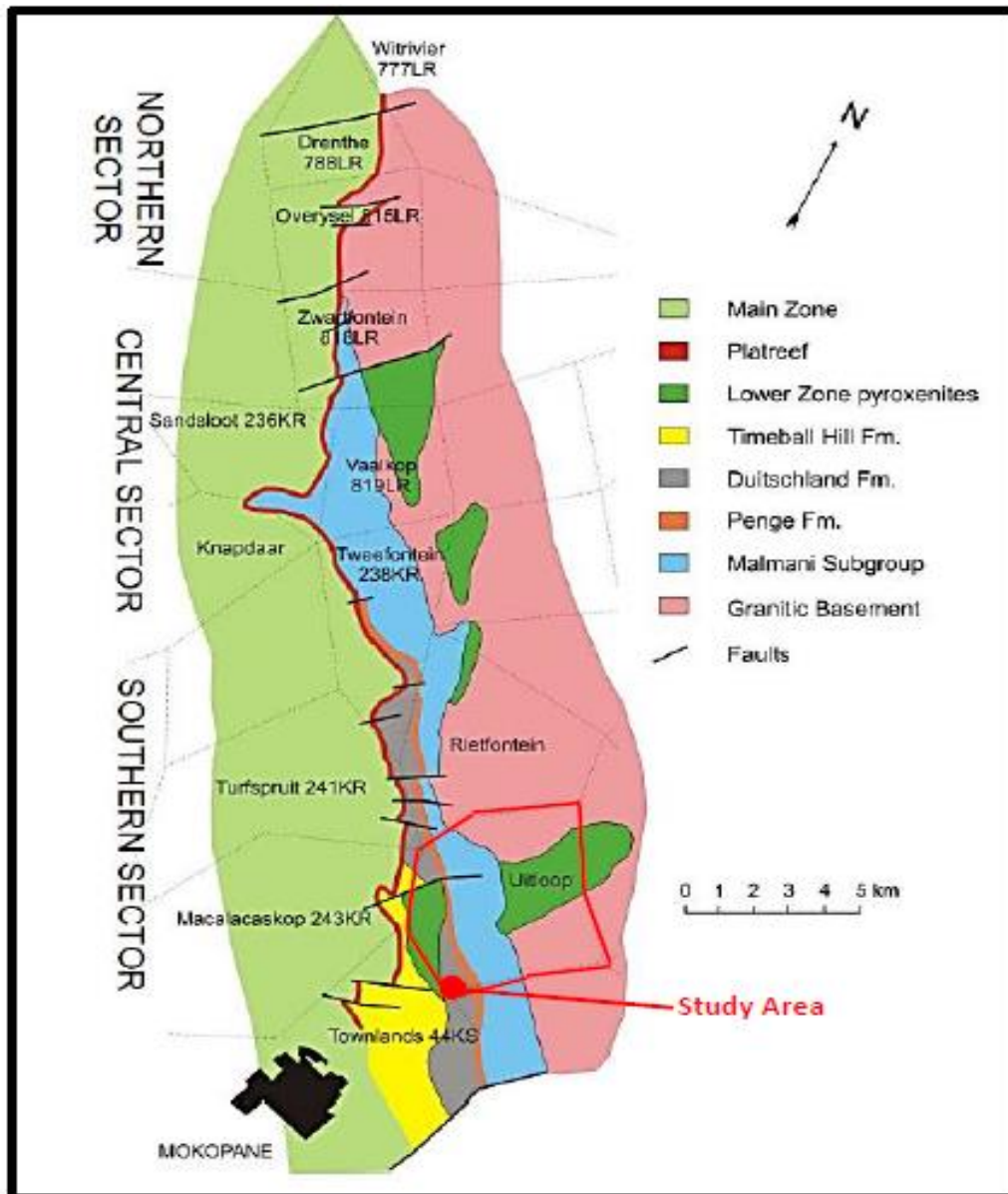
Figure 1-1: Geological map of the northern limb of the Bushveld Complex indicating the northern, central and southern sectors (Modified by Nex and Kinnaird, 2004 after van der Merwe, 1978). The red line indicates the outline of the farm Uitloop 3KS while the red circle shows the location of the studied area on the farm.
