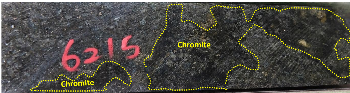
Figure 4-7: A photograph of borehole core sample showing coarse-grained feldspathic harzburgite (sample Z20-57.5) with chromite disseminations.
