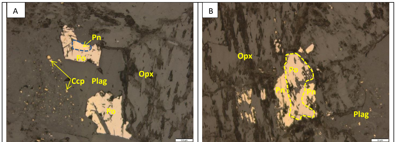
Figure 11-74: Photomicrographs, under reflected light, of feldspathic pyroxenite (sample Z20-155.7) from the southwestern part of the Uitloop farm.
