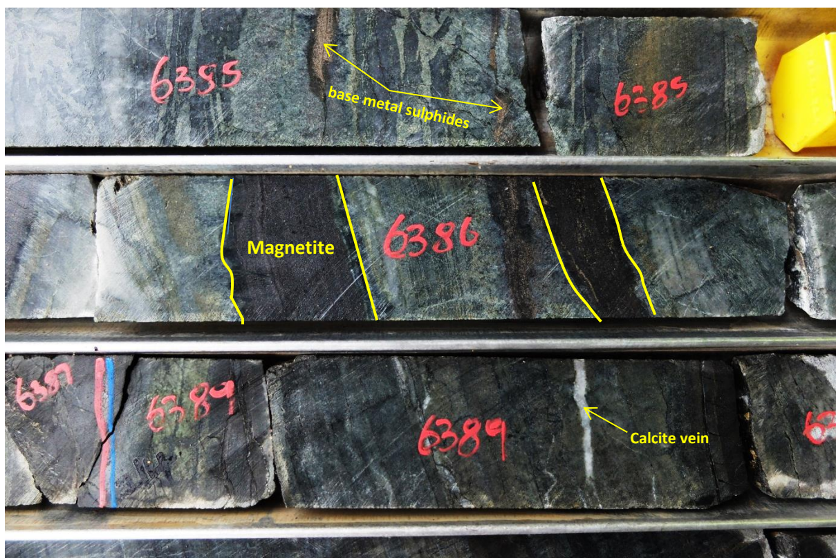
Figure 4-18: A photograph of borehole core sample showing dolomite with bands of magnetite and minor base metal sulphides as well as calcite veins.
