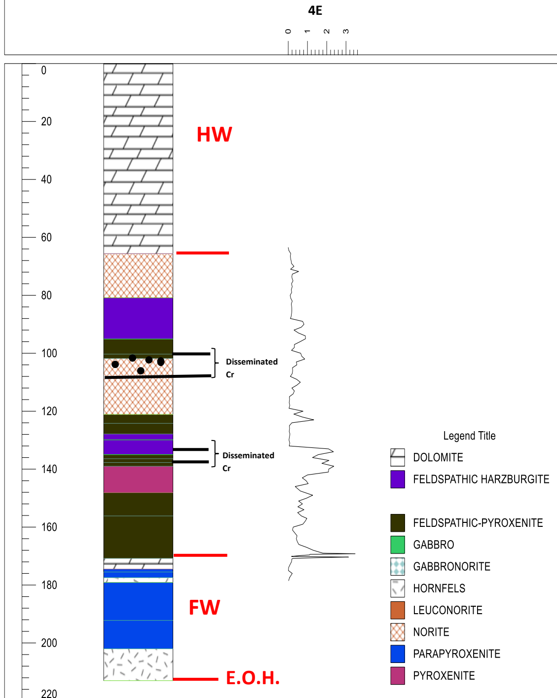
Figure 4-19: Simplified geological log of borehole Z19 indicating major stratigraphic positions; HW = hanging wall, Cr = chromite mineralisation, FW = footwall, E.O.H = end of hole, a graph displaying the down-hole 4E grade profile is also included.
