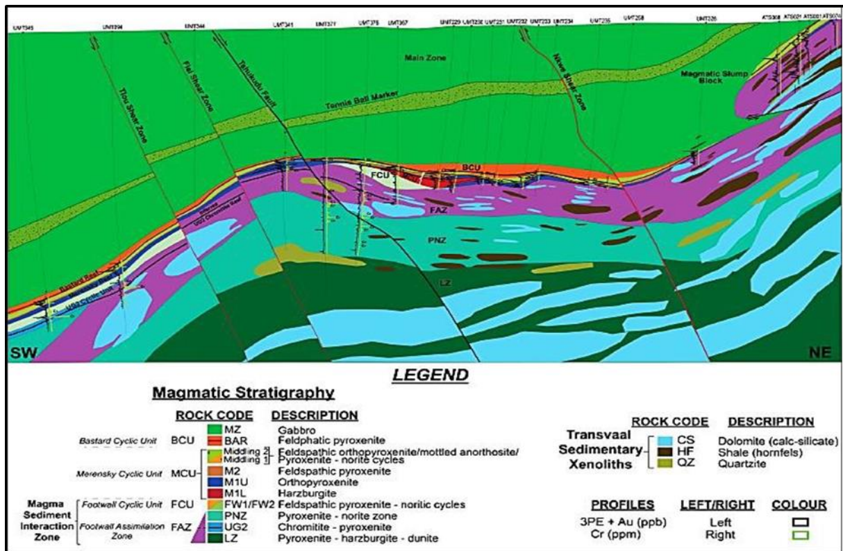
Figure 3-5: A NE-SW cross-section across the Flatreef and its down-dip extension on Turfspruit farm (Grobler et al., 2018).
