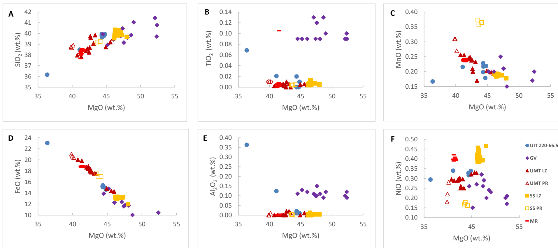
Figure 8-22: Compositional variation diagrams comparing the compositions of olivine crystals from the southwestern portion of the Uitloop farm magmatic lithologies to the Lower Zone olivine crystals from Turfspruit, Sandsloot (Yudovskaya & Kinnaird, 2010), Grasvally farms (Hulbert, 1983) and the Merensky Reef (Naldrett et al., 2009). (UIT = Uitloop, LZ = Lower Zone, PR = Platreef, GV = Grasvally, UMT = Turfspruit, SS = Sandsloot, MR = Merensky Reef).
