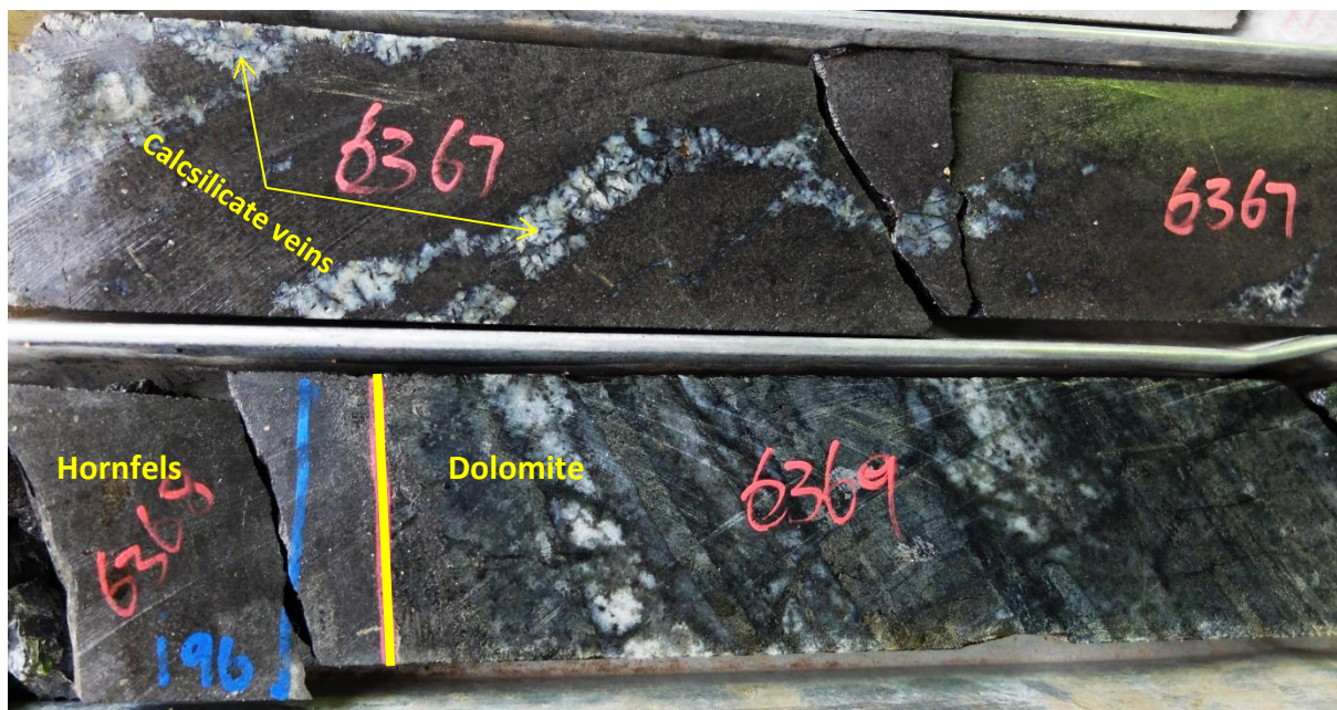
Figure 4-17: A photograph of borehole core samples showing a sharp contact between the hornfels and the underlying dolomitic unit at a depth of 196 m below surface.
