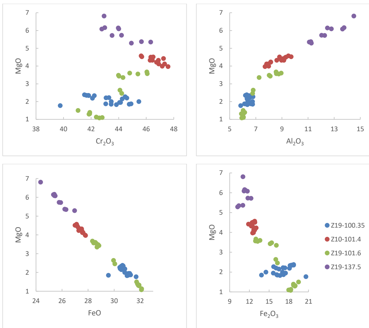
Figure 8-6: Geochemical graphs of chromite composition from feldspathic pyroxenite lithologies from the southwestern portion of the Uitloop farm; (A) Cr 2 O 3 vs MgO (B) Al 2 O 3 vs MgO (C) FeO vs MgO (D) Fe 2 O 3 vs MgO.
