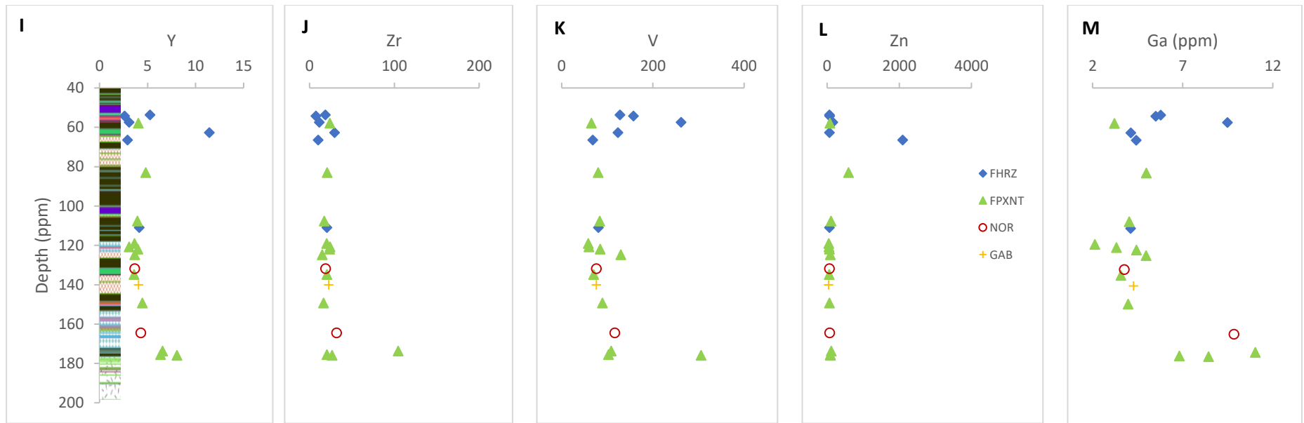
Fig 7-6 cont.) (FHRZ = Feldspathic harzburgite, FPXNT = Feldspathic pyroxene, NOR = Norite, GAB = Gabbro).
