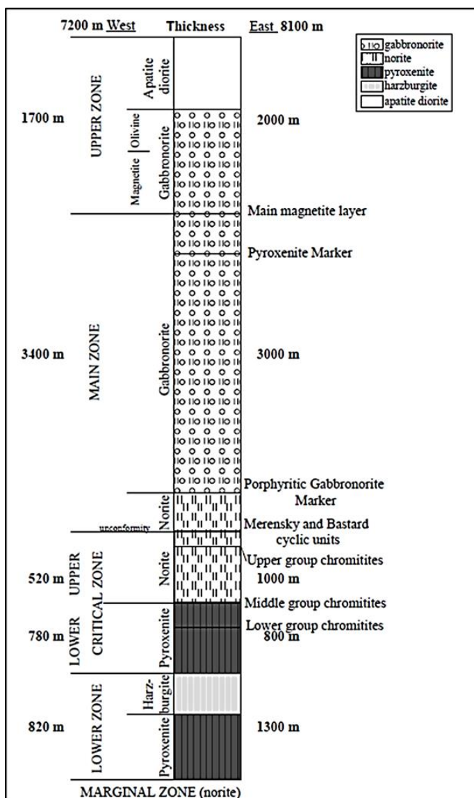
Figure 2-3: The stratigraphy of the Rustenburg layered suit of the Bushveld Complex (After Eales & Cawthorn, 1996).
