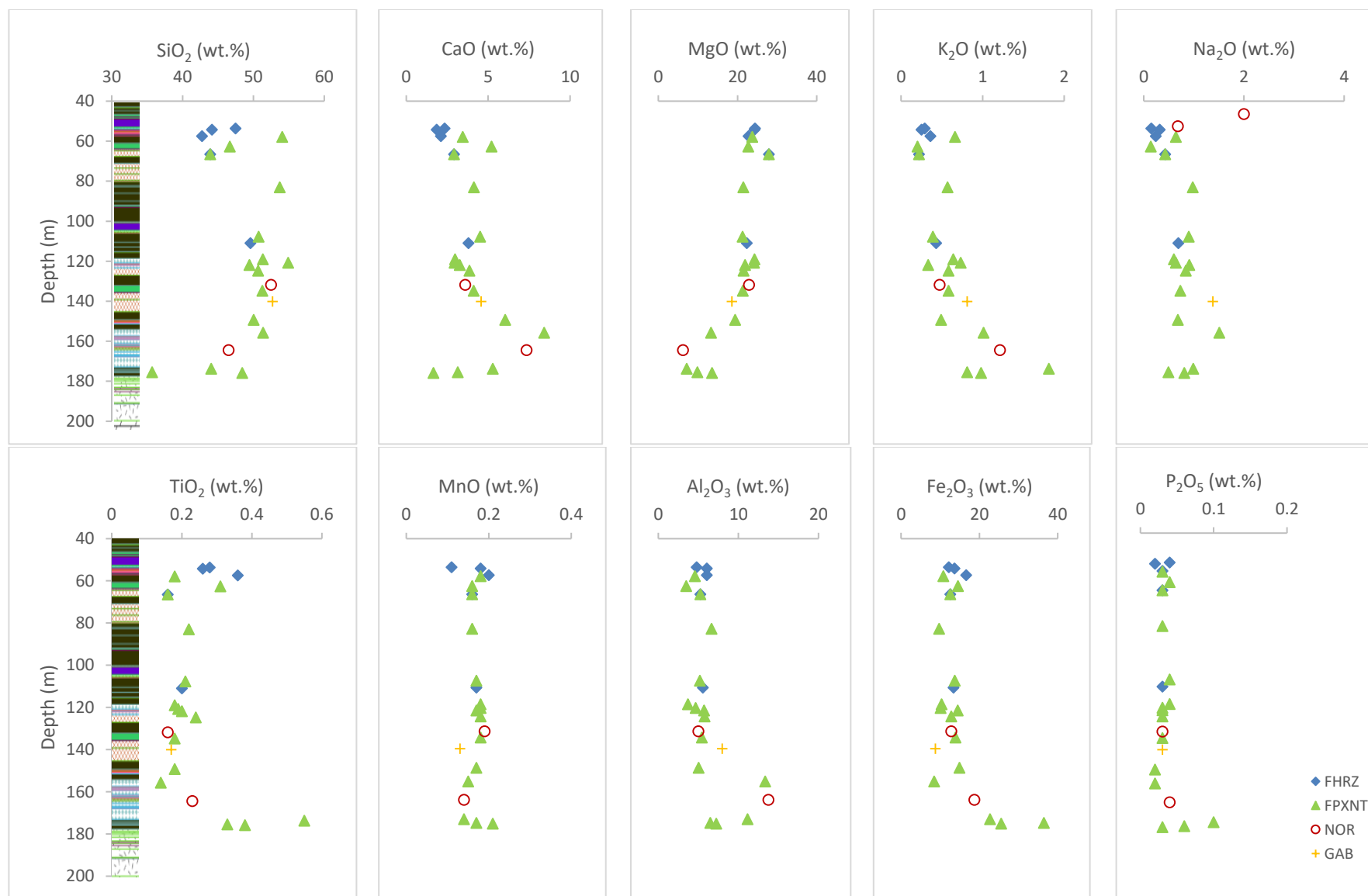
Figure 7-2: Variation in major element concentrations with stratigraphic height in borehole Z20. (FHRZ = feldspathic harzburgite, FPXNT = Feldspathic pyroxene, NOR = norite, GAB = gabbro).
