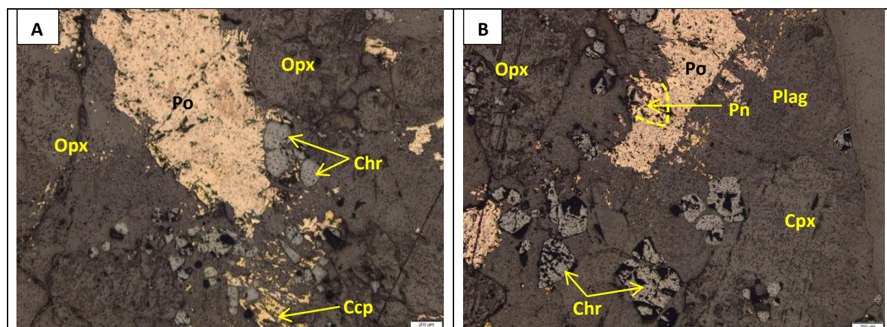
Figure 11-51: Photomicrographs, under reflected light, of sample Z19- 101.4 (feldspathic pyroxenite) from the southwestern part of Uitloop farm.
