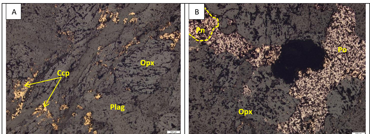
Figure 11-77: Photomicrographs, under reflected light, of feldspathic pyroxenite (sample Z20-175.5) from the southwestern part of the Uitloop farm.
