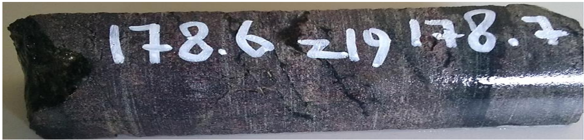
Figure 4-13: A photograph of borehole core sample showing fine-grained mica-rich hornfels (sample Z19-178.6).
