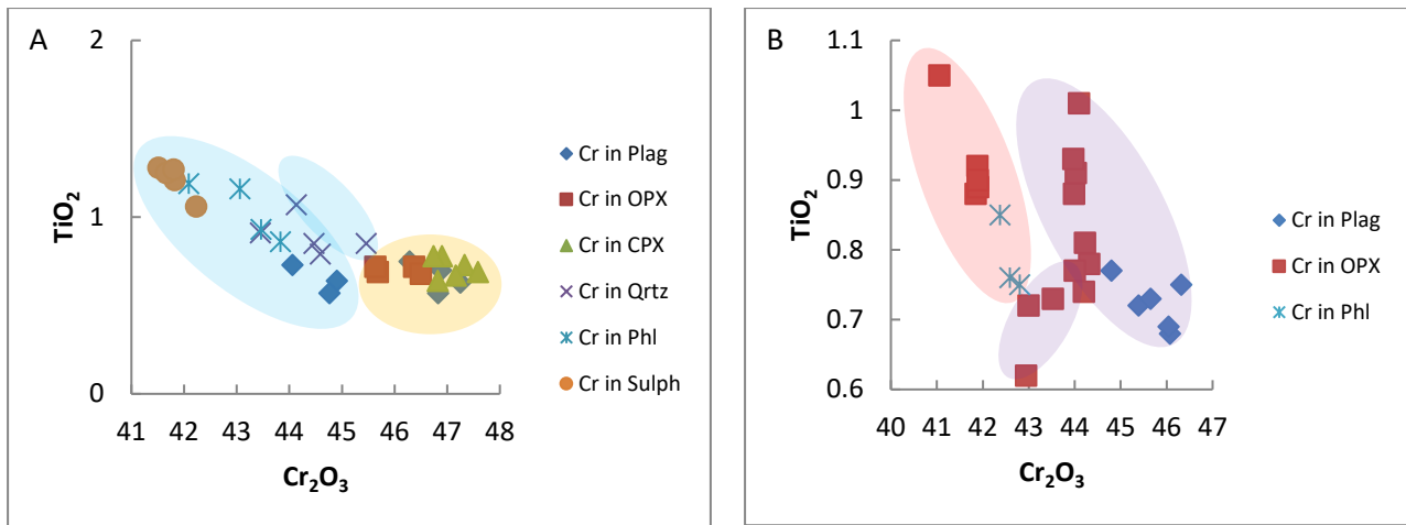
Figure 8-14: Geochemical graphs of chromite composition from feldspathic pyroxenite lithologies from the southwestern portion of the Uitloop farm; (A) \text{Cr}_2\text{O}_3 vs \text{TiO}_2 (Blue: Z19-100.35, Orange: Z19-101.4) (B) \text{Cr}_2\text{O}_3 vs \text{TiO}_2 (Red: Z19-101.6, Purple: Z19-137.5).
