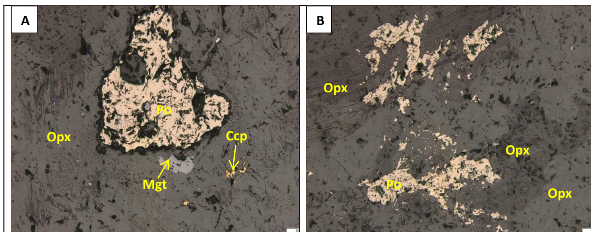
Figure 11-56: Photomicrographs, under reflected light, of sample Z19-170.5 (parapyroxenite) from the southwestern part of Uitloop farm.
