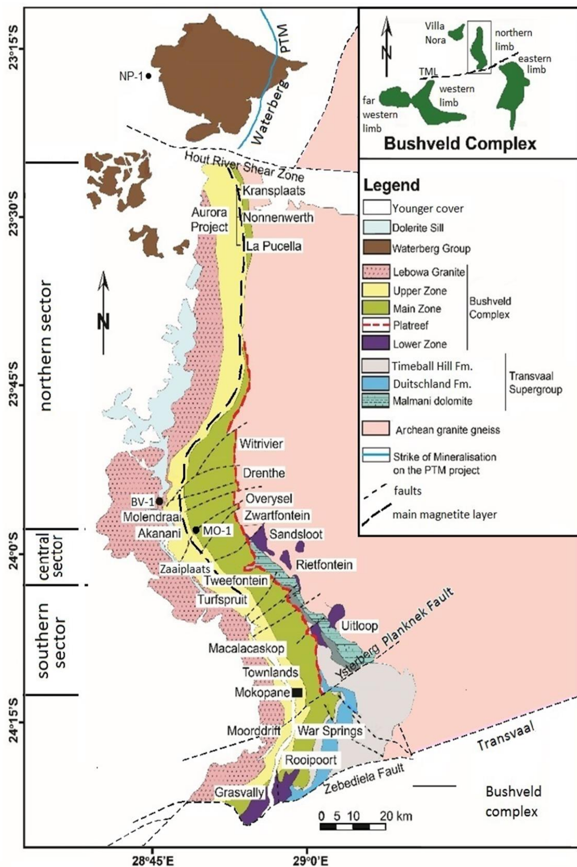
Figure 3-1: Geological map of the northern limb of the Bushveld Complex (Kinnaird & McDonald, 2018).
