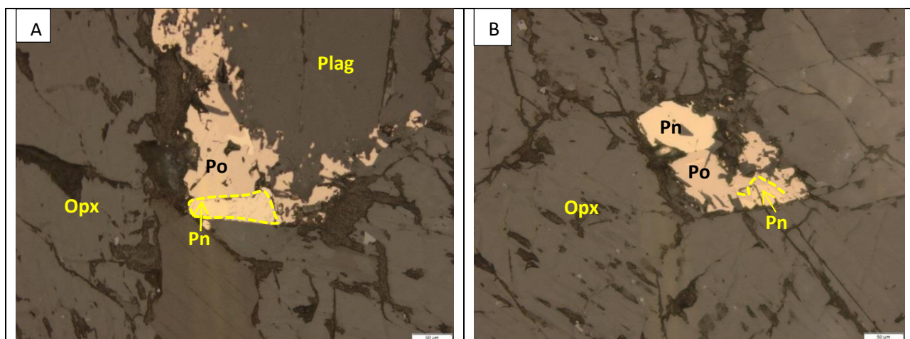
Figure 11-69: Photomicrographs, under reflected light, of Sample Z20-121.9 (feldspathic pyroxenite) from the southwestern part of the Uitloop farm.
