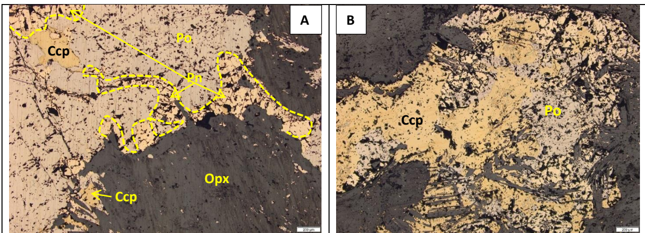
Figure 11-72: Photomicrographs, under reflected light, of gabbro (sample Z20-140.1) from the southwestern part of the Uitloop farm.
