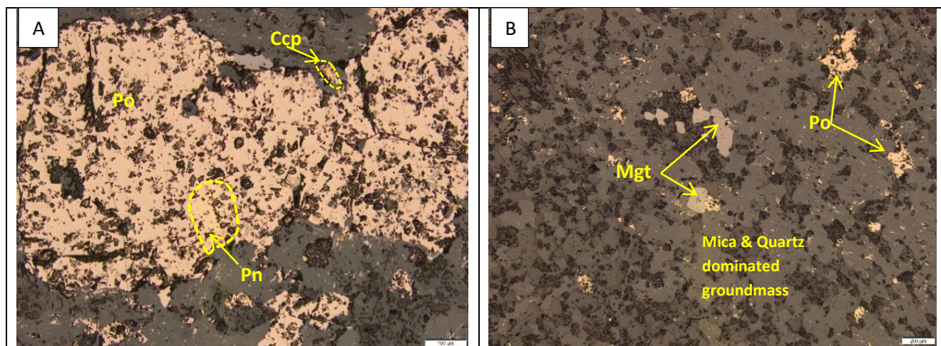
Figure 11-81: Photomicrographs, under reflected light, of mica-rich hornfels (sample Z20-183.5) from footwall rocks to the southwestern part of the Uitloop farm.
