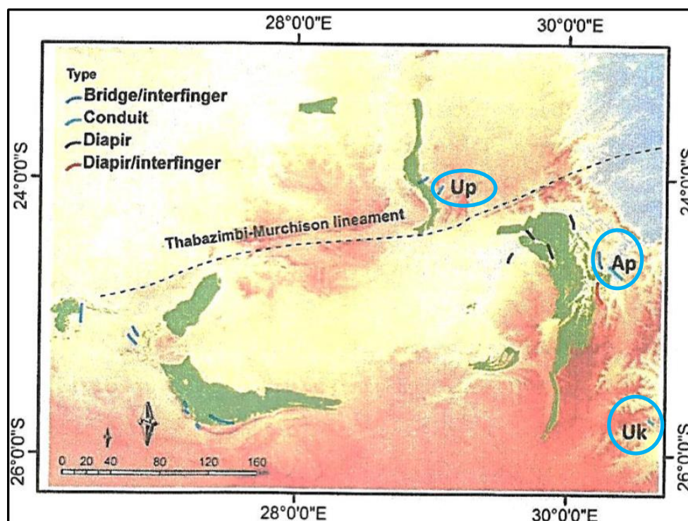
Figure 1-6: Location and orientation of conduit-type intrusions in the Bushveld Complex. Up=Uitloop, Ap= Apiesdooringdraai, Uk=Uitkomst (Modified after Clarke et al., 2009a).
