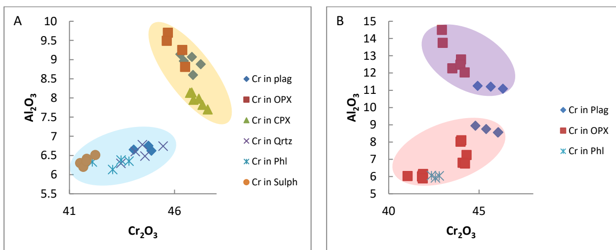
Figure 8-12: Geochemical plots of chromite composition from feldspathic pyroxenite lithologies from the southwestern portion of the Uitloop farm; (A) \text{Cr}_2\text{O}_3 vs \text{Al}_2\text{O}_3 (Blue: Z19-100.35, Orange: Z19-101.4) (B) \text{Cr}_2\text{O}_3 vs \text{Al}_2\text{O}_3 . (Red: Z19-101.6, Purple: Z19-137.5).
