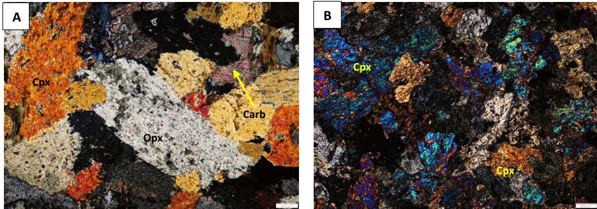
Figure 5-6: Photomicrographs (taken under XPL) of parapyroxenite (sample Z19-170.5) from footwall lithologies at the southwestern portion of the Uitloop farm in borehole Z19. (A & B) Granular pyroxene crystals.
