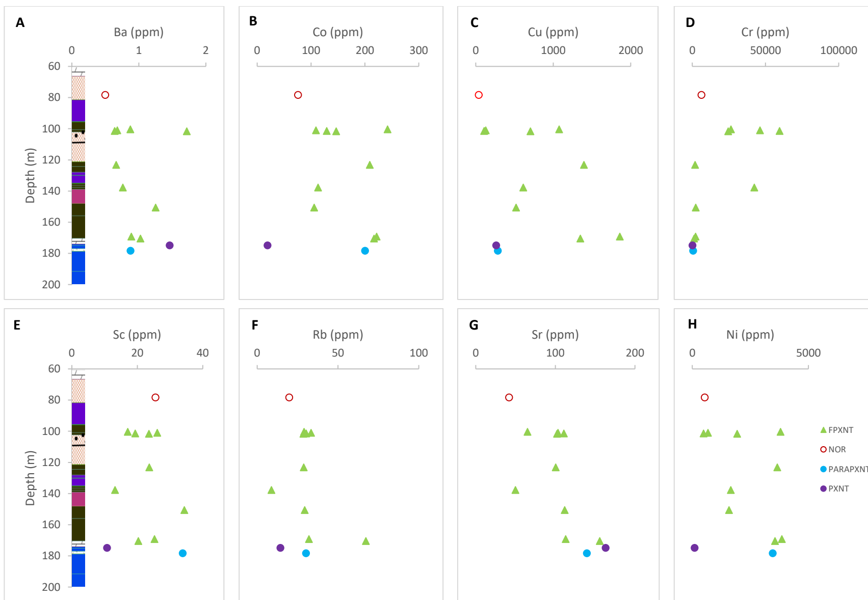
Figure 7-5: Variation in selected trace element concentrations (ppm) with stratigraphic height in borehole Z19 from the Uitloop farm. (FHRZ = Feldspathic harzburgite, FPXNT = Feldspathic pyroxene, NOR = Norite, PXNT = Pyroxenite, PARAPXNT = Parapyroxenite).
