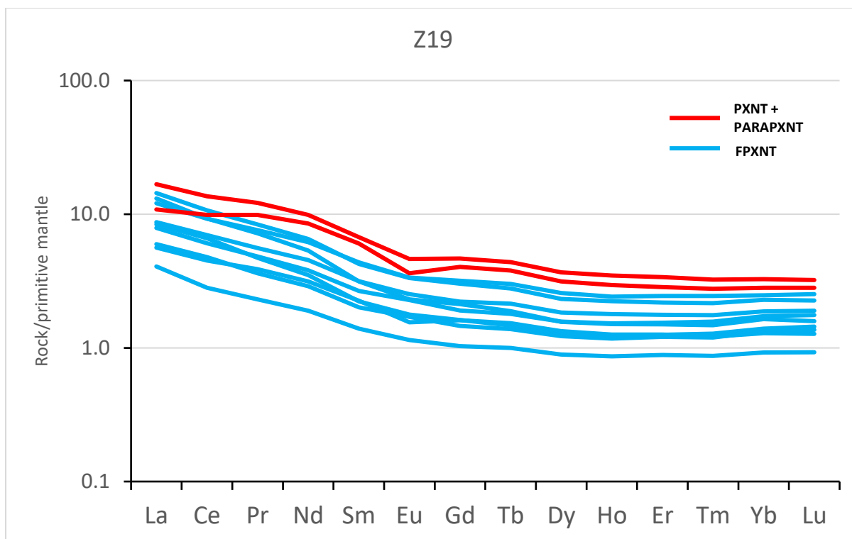
Figure 7-10: Primitive mantle normalized REE graphs (normalised to data by Hoffman (1988)) of the feldspathic pyroxenite (FPXNT) and pyroxenite (PXNT) + parapyroxenites (PARAPXNT) from borehole Z19 of the southwestern portion of Uitloop farm.
