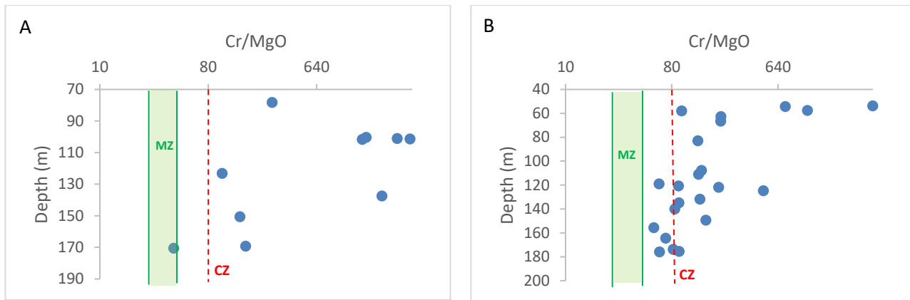
Figure 7-9: Cr/MgO vs depth for boreholes Z19 (A) and Z20 (B) showing that majority of the mafic/ultramafic rocks from the southwestern part of the Uitloop farm have Cr/MgO >80 and thus are of Critical Zone affinity. (MZ = Main Zone, CZ = Critical Zone).
