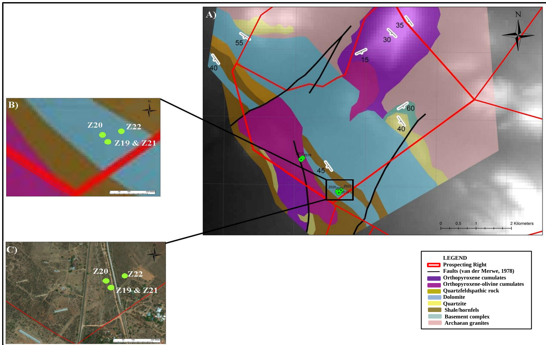
Figure 1-2: Location of the study area in the Uitloop farm indicating position of the boreholes use on this study A) & B) simplified geological map of the Uitloop farm (study area) (After van der Merwe, 1978), indicating the licenced area. C) Google earth image of Figure B.
