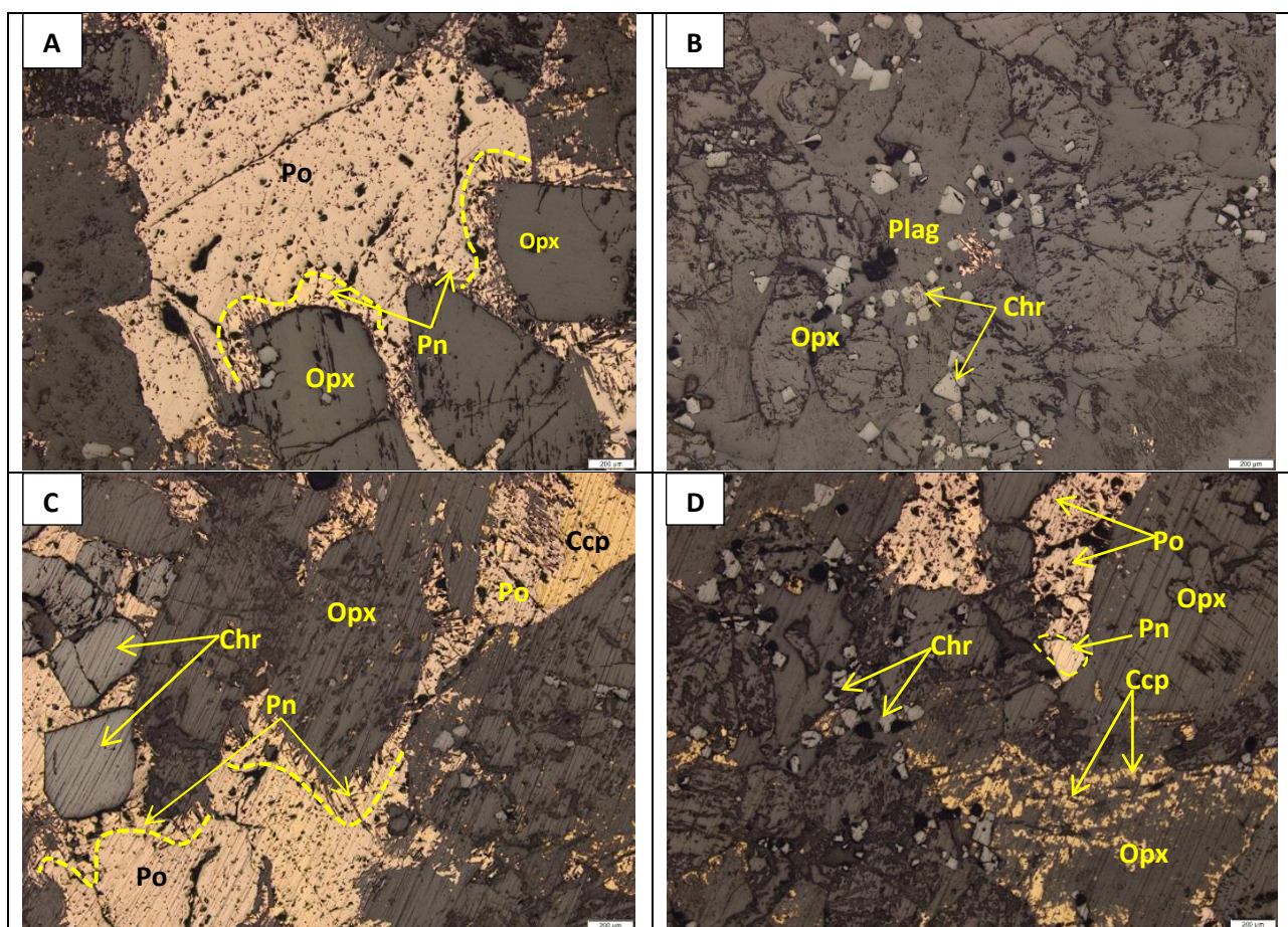
Figure 11-48: Photomicrographs, under reflected light, of sample Z19-78.3 (feldspathic pyroxenite) from the southwestern part of Uitloop farm.
