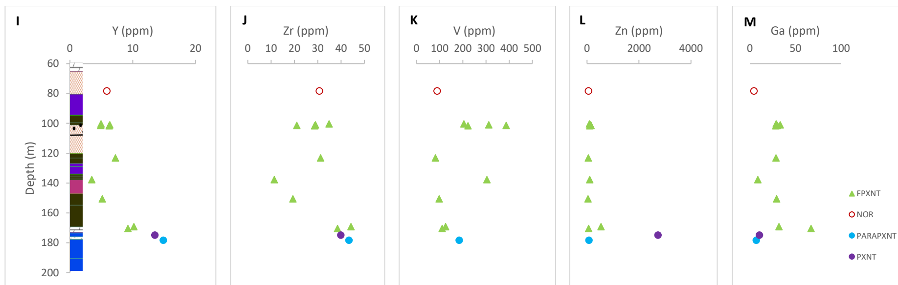
(Figure 7-5 cont.) (FHRZ = Feldspathic harzburgite, FPXNT = Feldspathic pyroxene, NOR = Norite, PXNT = Pyroxenite, PARAPXNT = Parapyroxenite).
