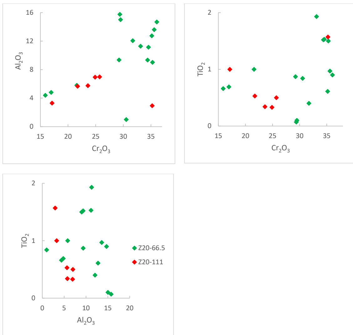
Figure 8-9: Geochemical graphs of chromite composition from feldspathic harzburgite lithologies from the southwestern portion of the Uitloop farm; (A) Cr_2O_3 vs Al_2O_3 (B) Cr_2O_3 vs TiO_2 (C) Al_2O_3 vs TiO_2 .
