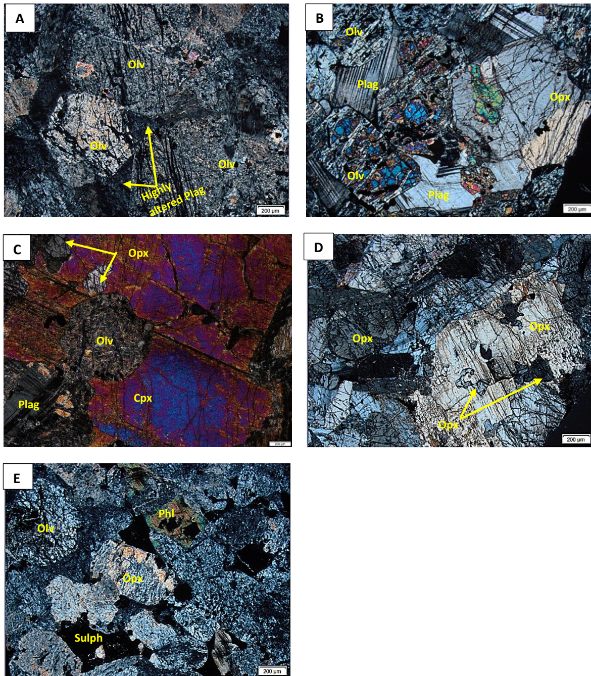
Figure 5-3: Photomicrographs (taken under XPL) of feldspathic harzburgite from the magmatic lithologies at the southwestern portion of the Uitloop farm. (A) Serpentinised olivine with characteristic fractures filled with magnetite, sample Z20 – 54.25, (B) Cumulus olivine and interstitial twinned plagioclase, sample Z20 – 66.5, (C) Clinopyroxene oikocryst enclosing olivine and orthopyroxene, sample Z20–111, (D) Orthopyroxene phenocryst with orthopyroxene inclusions, sample Z20–111, and (E) Olivine with characteristic fractures filled by magnetite, altered orthopyroxene crystals, phlogopite with chromite inclusions, sample Z20-53.7.
