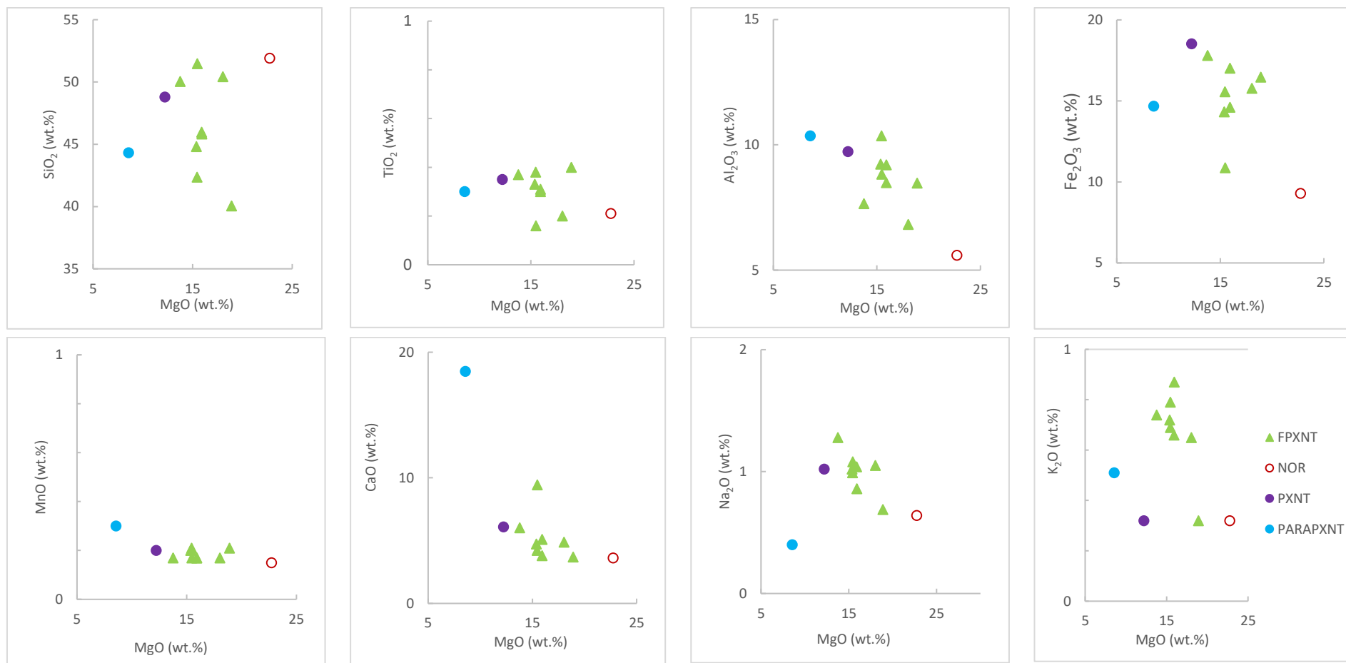
Figure 7-3: Binary variation diagrams showing selected major elements concentrations (wt.%) versus MgO content (wt.%) in borehole Z19 lithologies. (FHRZ = Feldspathic harzburgite, FPXNT = Feldspathic pyroxene, NOR = Norite, PXNT = Pyroxenite, PARAPXNT = Parapyroxenite).
