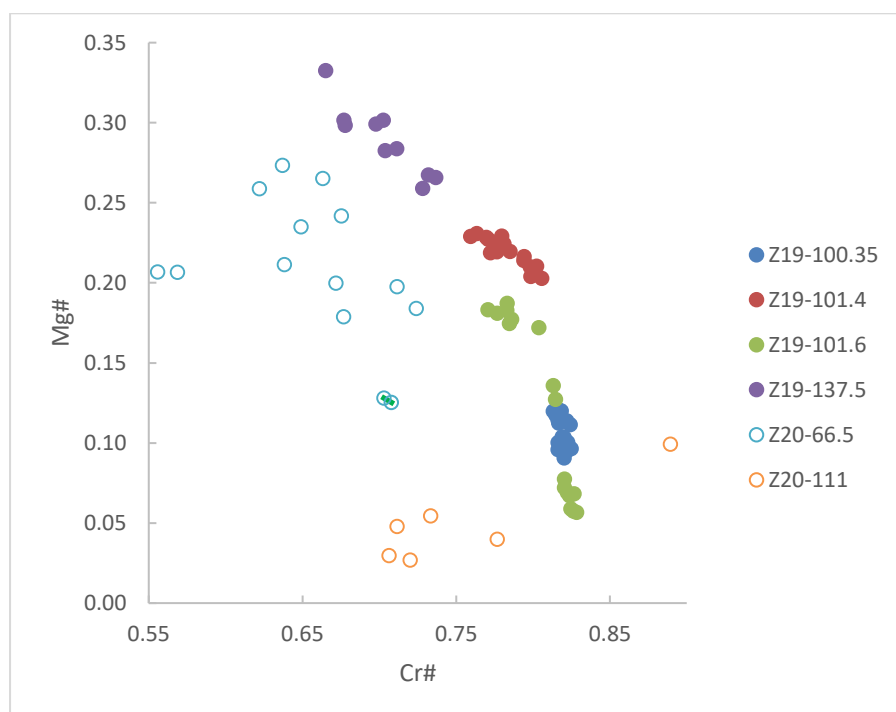
Figure 8-10: Cr# vs Mg# graphs for chromites hosted by magmatic lithologies from the southwestern portion of the Uitloop farm. Feldspathic pyroxenite (blue, marron, green and purple s) and feldspathic harzburgites (blue and orange), showing the proximity of chromite crystals to their original cumulus compositions.
