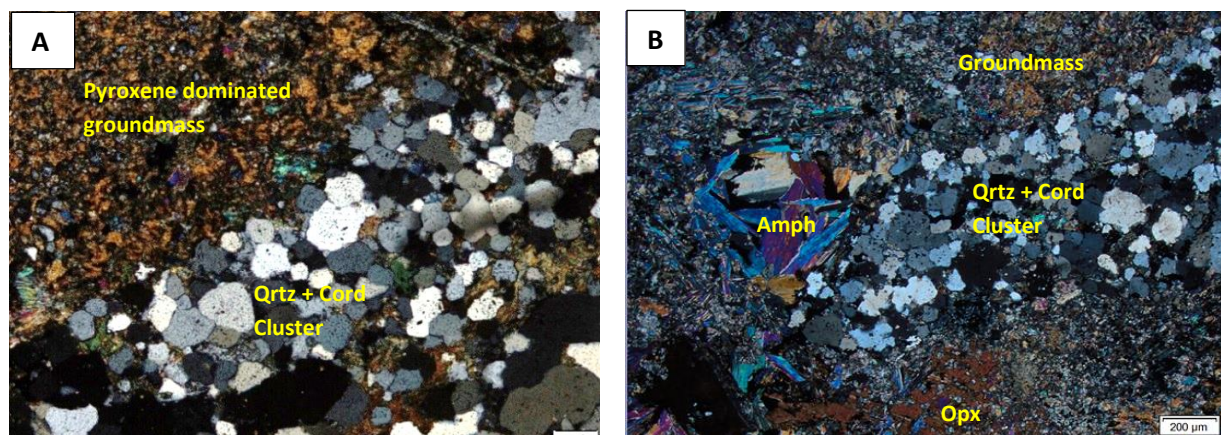
Figure 5-7: Photomicrographs (taken under XPL) of pyroxene hornfels from the footwall lithologies at the southwestern portion of the Uitloop farm. (A) Quartz and cordierite clusters as well as amphibole clusters set in a fine-grained pyroxene-rich groundmass in pyroxene hornfels, sample Z20-183.5. (B) Quartz and cordierite clusters in pyroxene hornfels, sample Z19-203.2.
