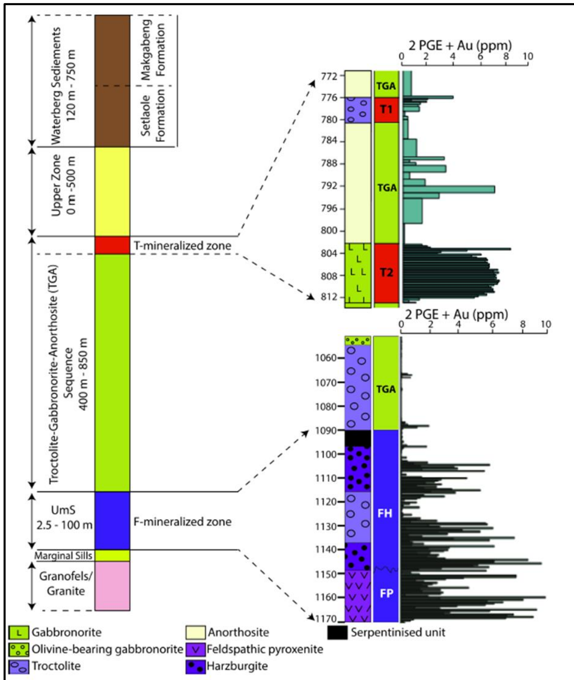
Figure 3-2: A simplified stratigraphy of the Waterberg project area showing the position of the mineralised intervals, F-zone and T-zone, PGE grades are also presented in the form of histograms (Kinnaird et al., 2017).
