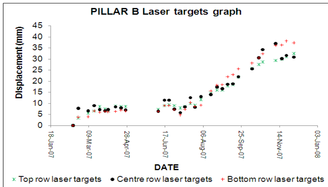
Figure 3.21 South Deep Mine Pillar B laser targets displacement results
