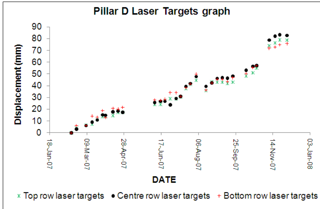
Figure 3.23 South Deep Mine Pillar D laser targets displacement results
