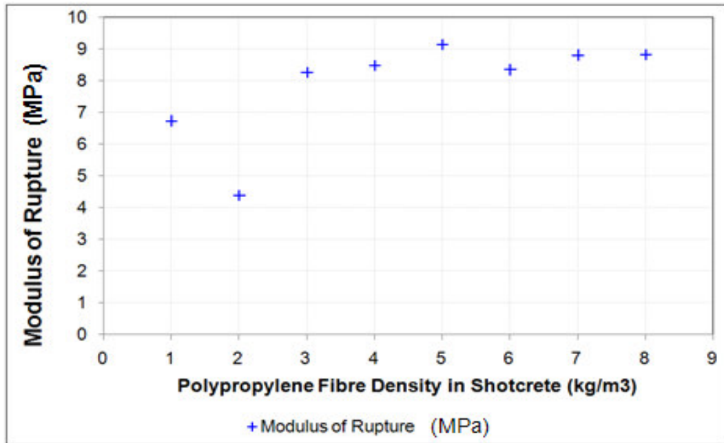
Figure 4.5 Modulus of rupture for the polypropylene fibre reinforced shotcrete ASTM beams
