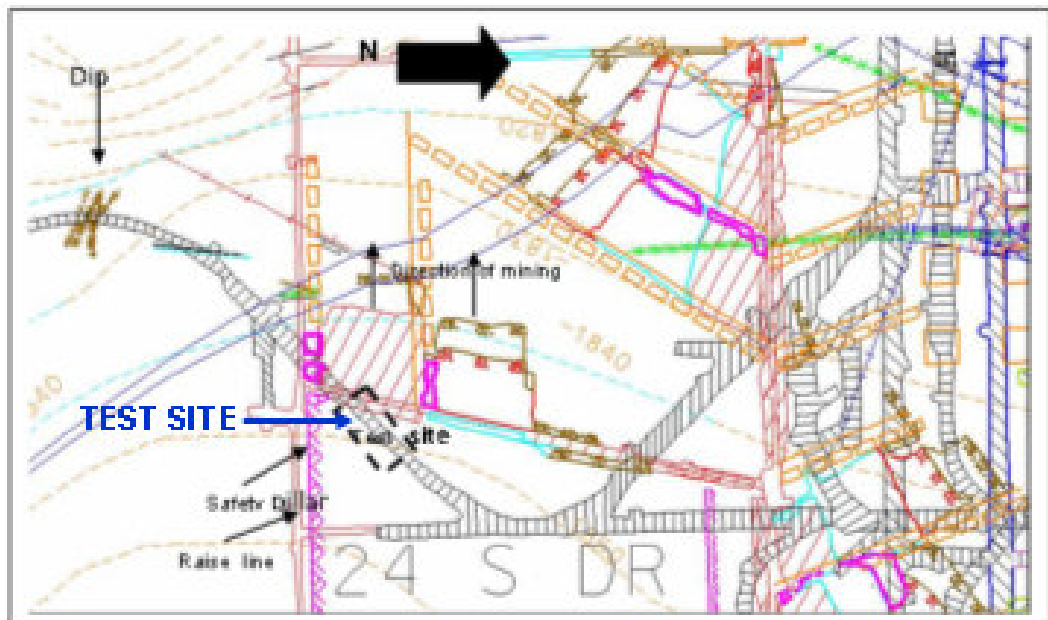
Figure 3.17 Impala Platinum Mine monitoring site plan (SRK SIMRAC Internal report, 2008)
