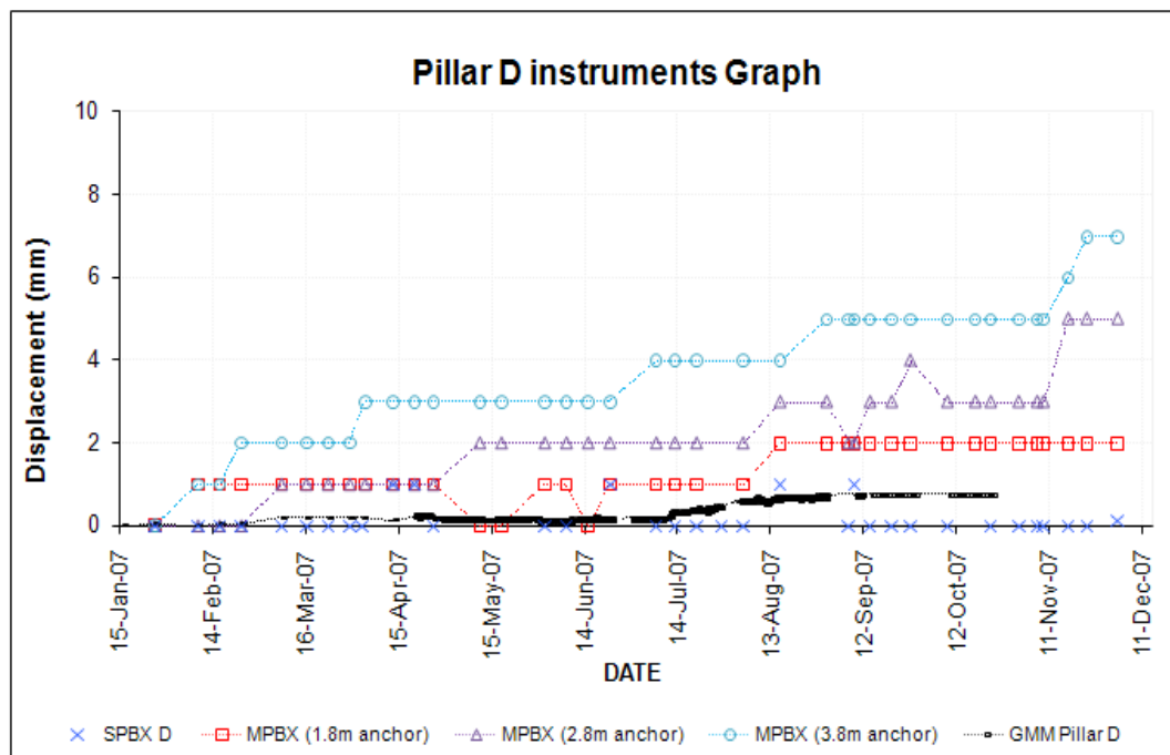
Figure 3.22 South Deep Mine Pillar D displacement results
