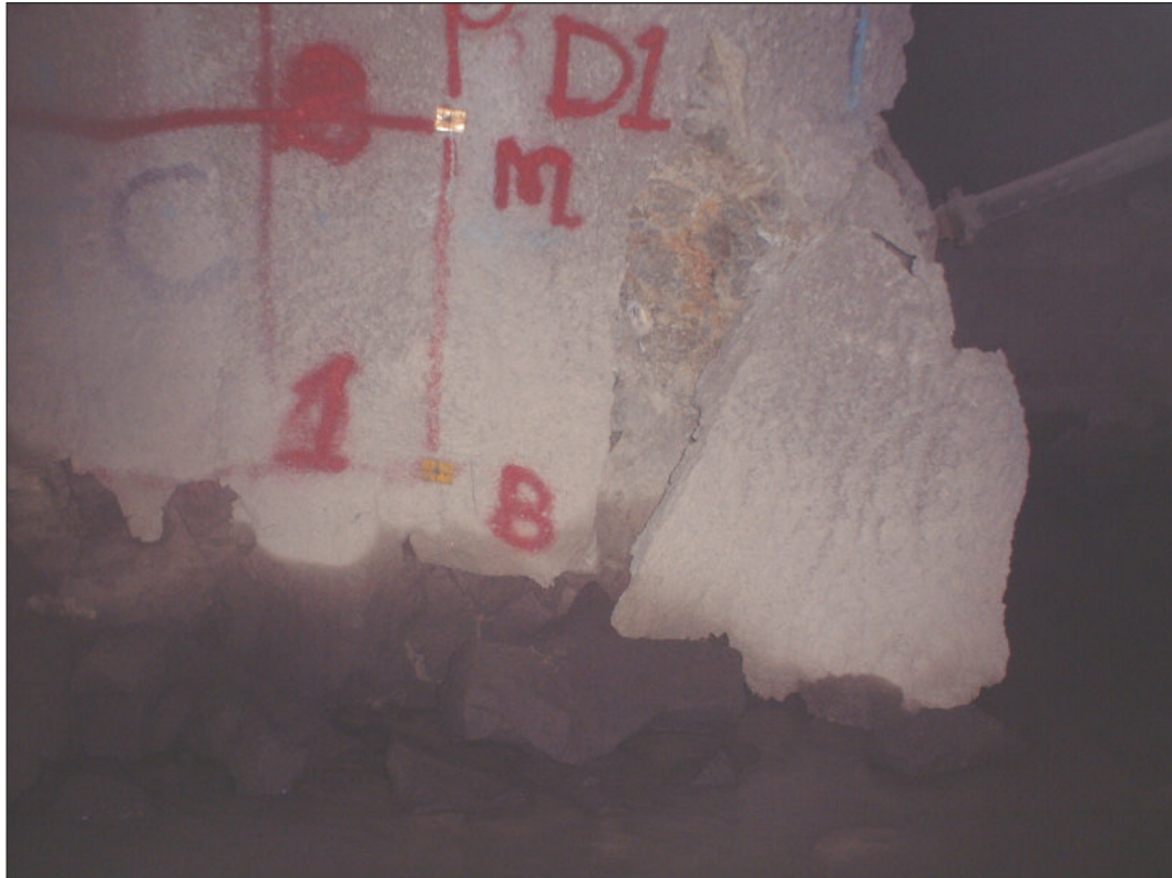
Figure 5.8 Damaged corner of one of the pillars that were monitored at South Deep Mine
