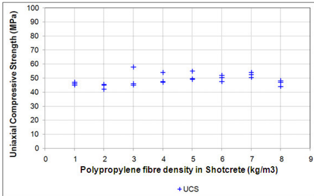
Figure 4.24 Uniaxial compressive strength test results for the polypropylene fibre reinforced shotcrete cores
