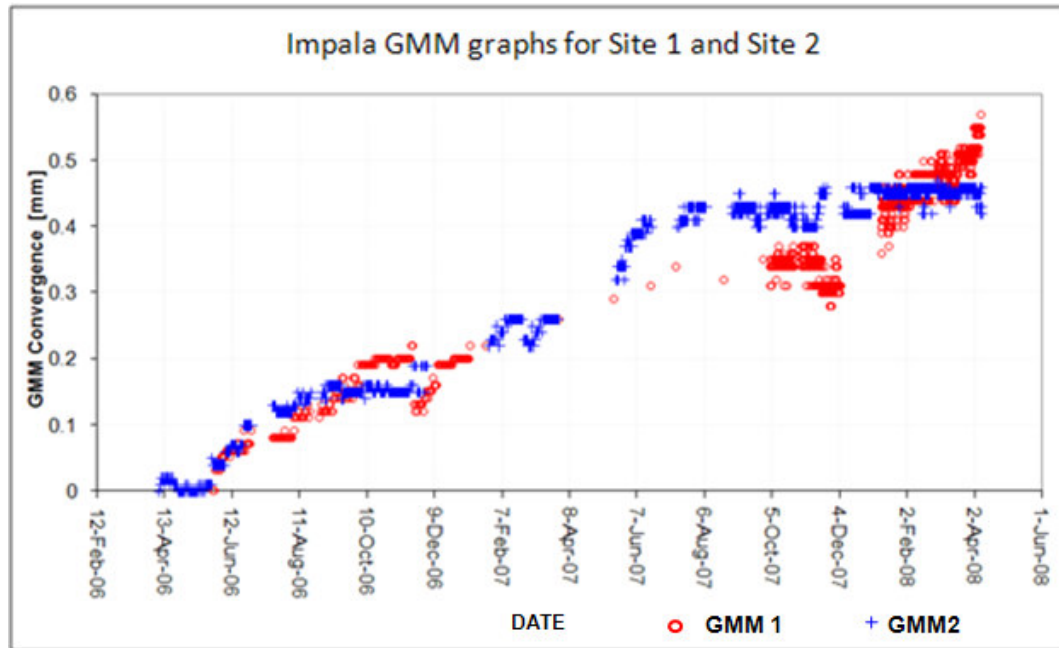
Figure 3.26 Impala Platinum Mine GMM displacement results
