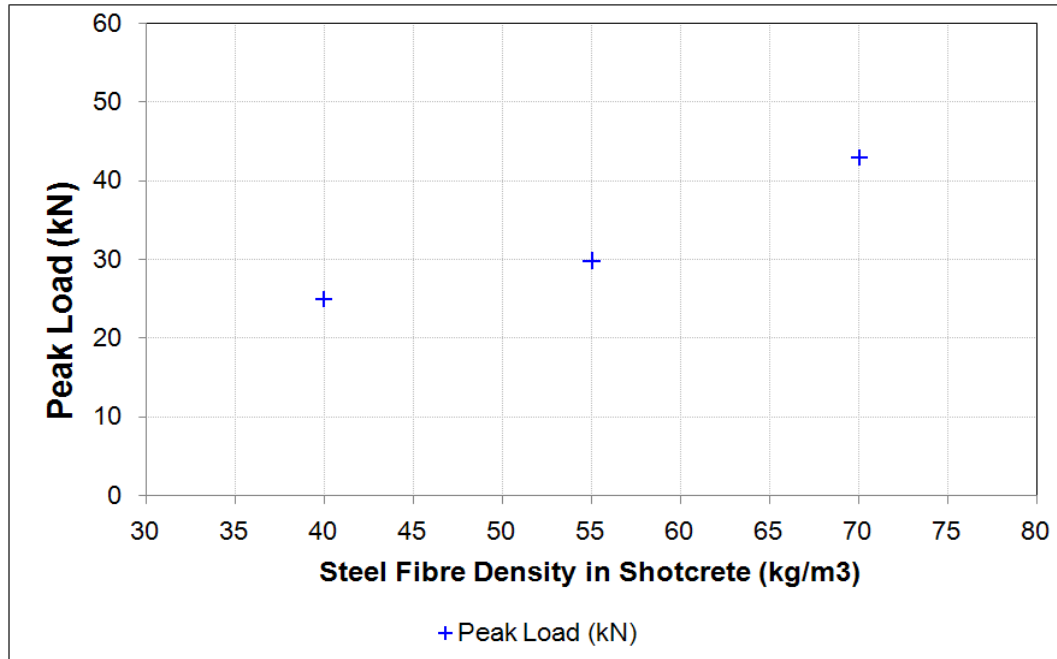
Figure 4.18 Peak loads for the steel fibre reinforced shotcrete round determinate panels
