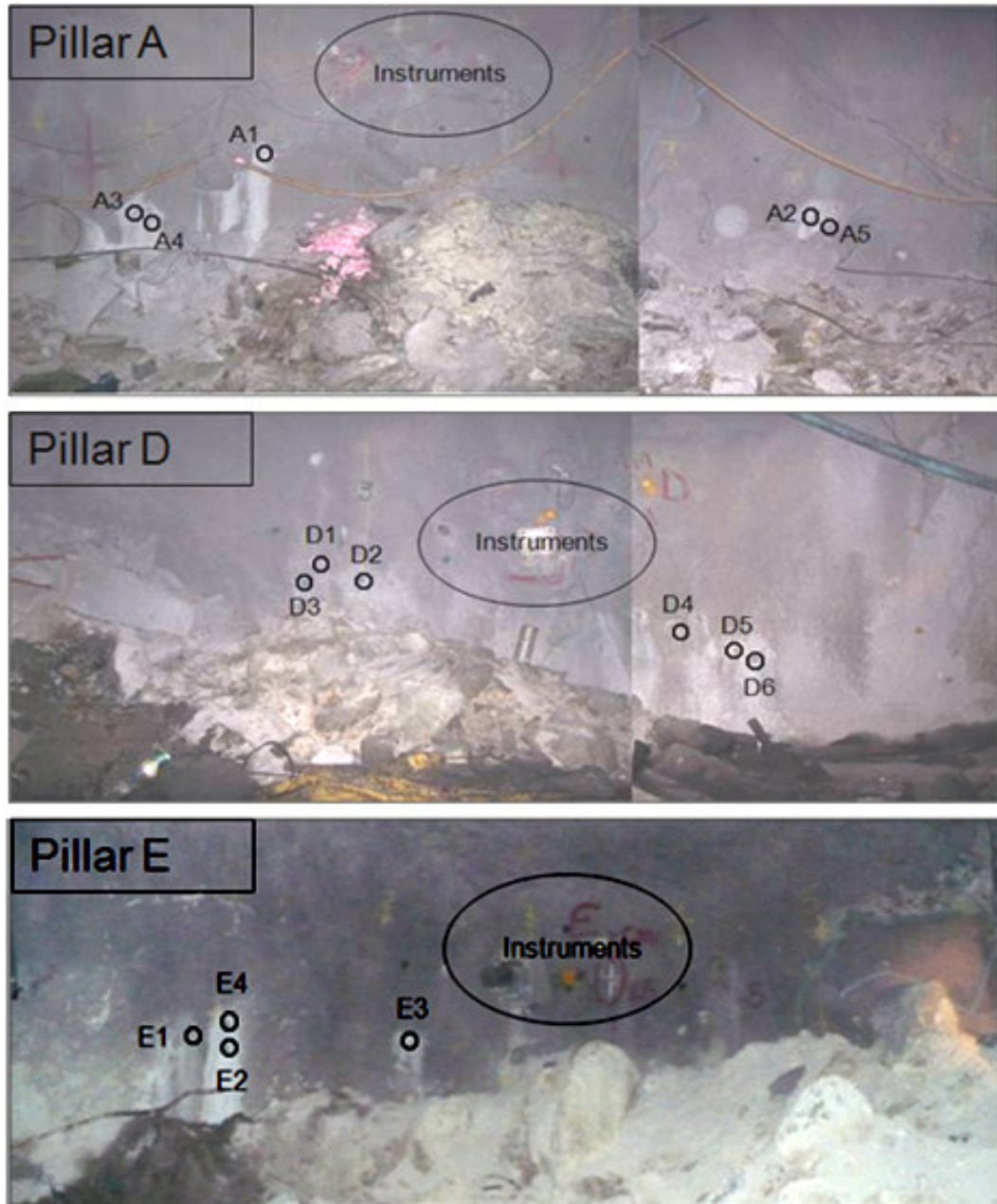
Figure 3.16 Photographs showing the location of drilled cores for UCS testing, bond strength testing and fibre density determination at South Deep Mine on pillars A, D and E
