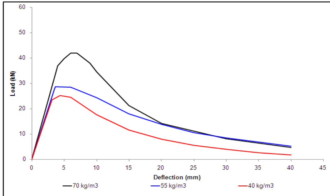
Figure 4.22 Load-deflection results for the steel fibre reinforced shotcrete round determinate shotcrete panels
