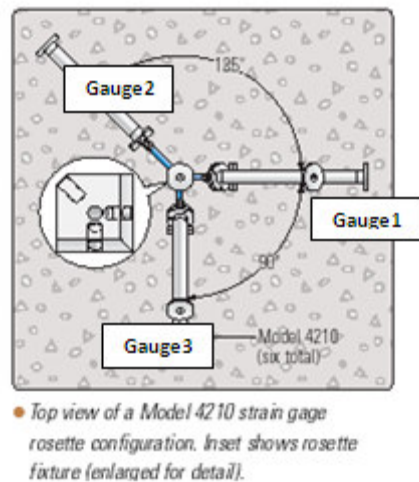
Figure 3.2 Strain gauge rosettes
