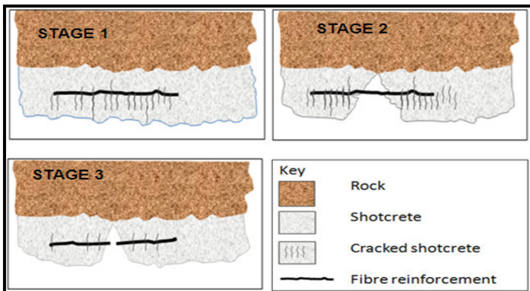
Figure 5.3a Diagram illustrating the tensile failure of fibres in fibre reinforced shotcrete
