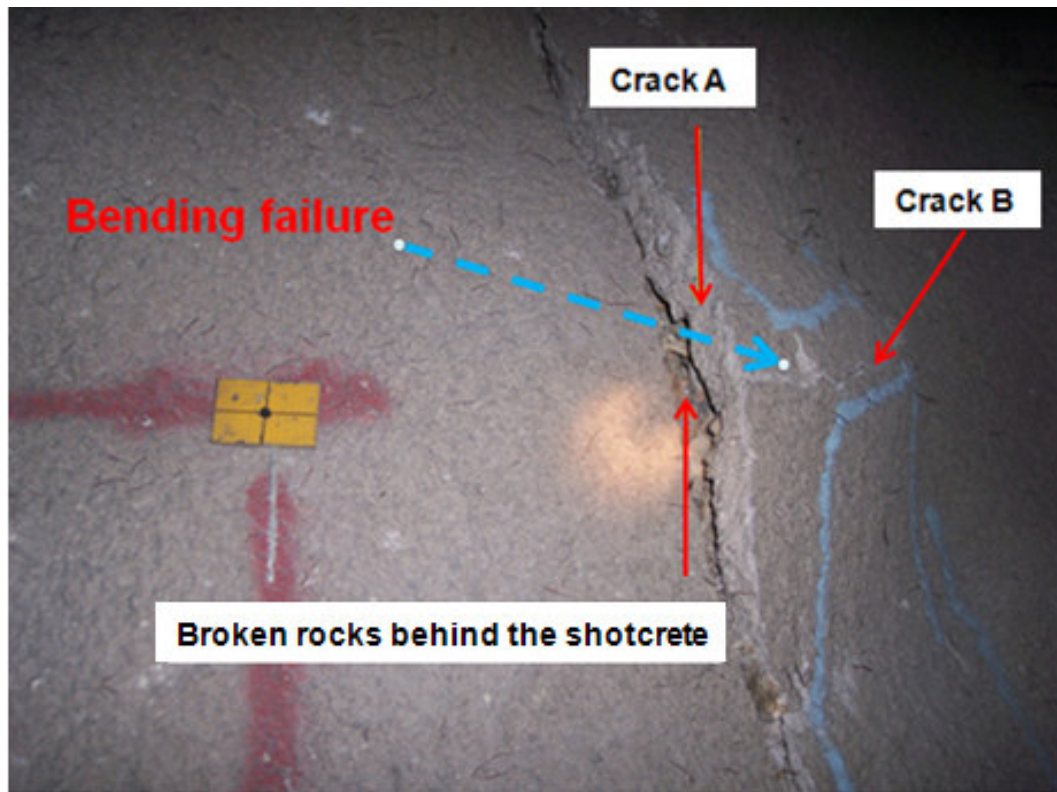
Figure 3.38a Photograph showing bending failure of shotcrete on Pillar B at South Deep Mine
