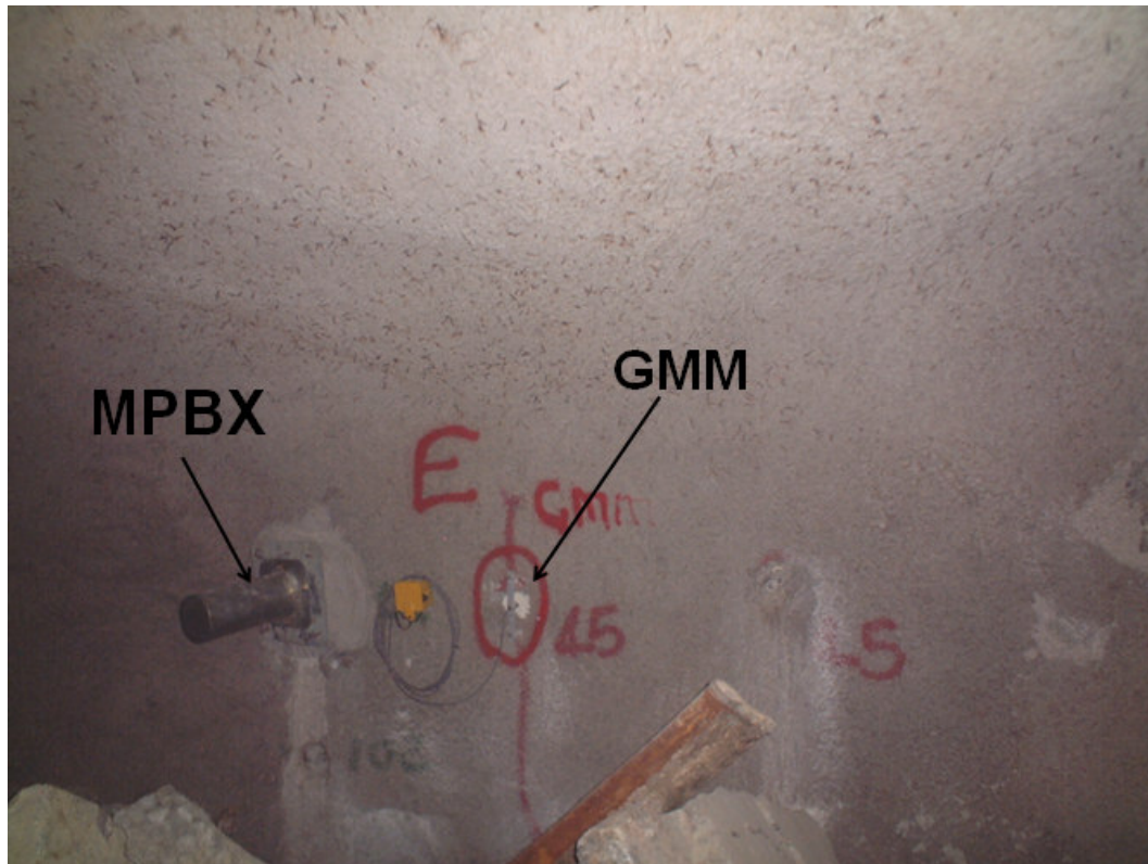
Figure 3.14 Photograph showing South Deep Mine Pillar E positioning of monitoring instruments
