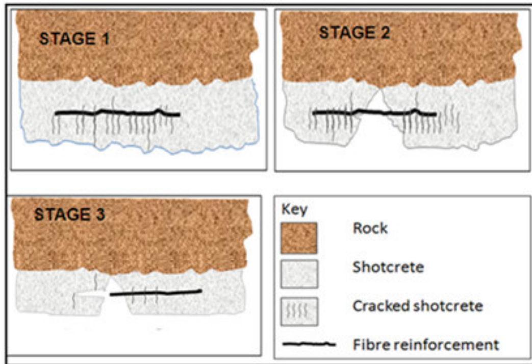
Figure 5.3b Diagram illustrating the pullout (failure) of fibres in fibre reinforced shotcrete
