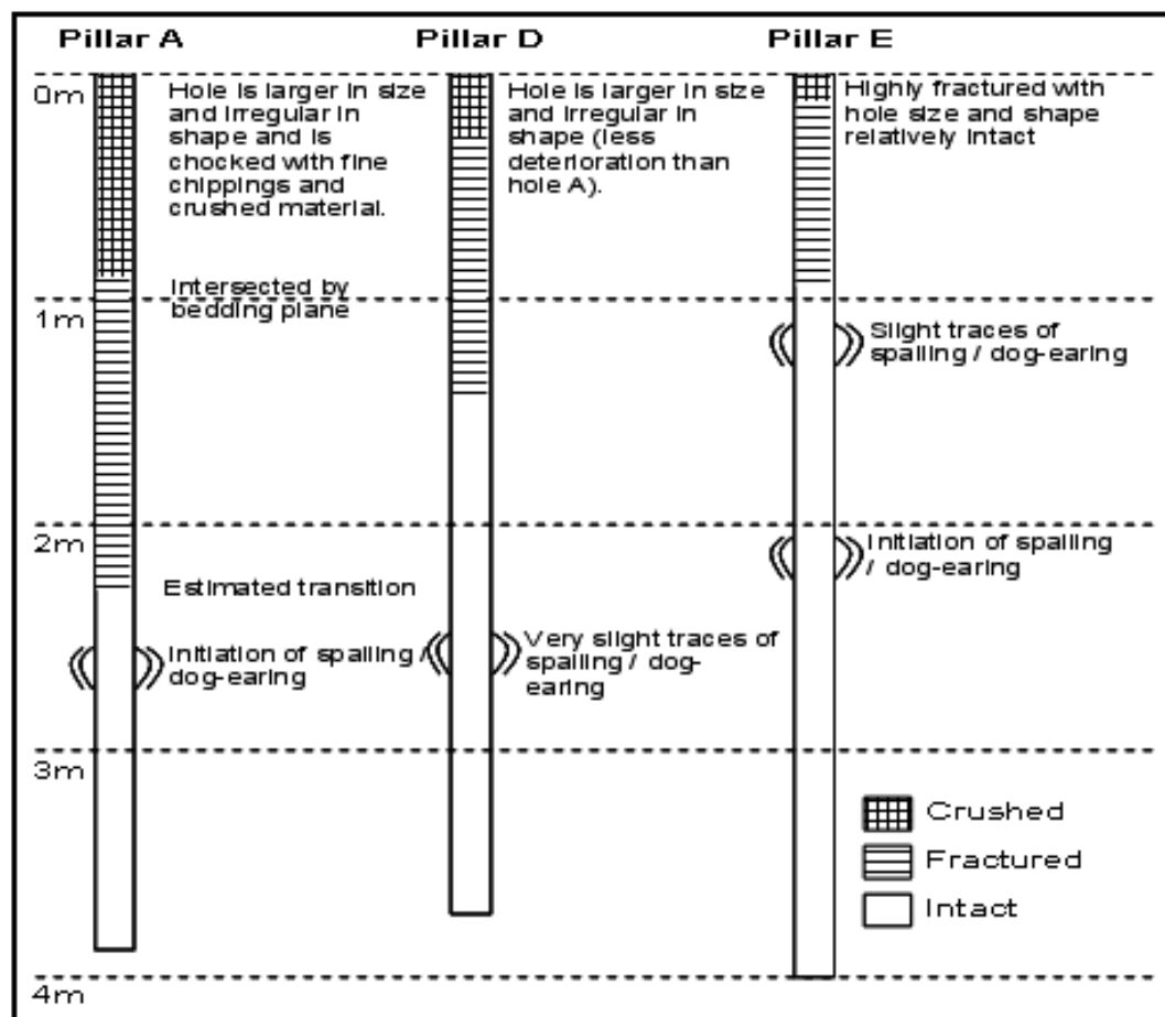
Figure 3.25 Fracture zones identified at South Deep Mine site from borehole inspection (SRK, SIMRAC Internal report, 2008).
