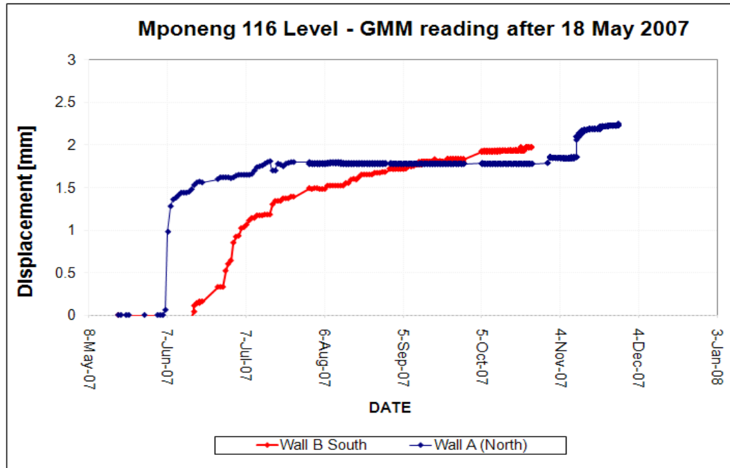
Figure 3.31 GMM displacement results for Mponeng Mine Level 116
