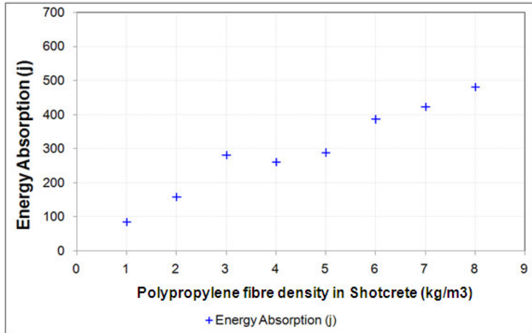
Figure 4.19 Energy absorption for the polypropylene fibre reinforced round determinate panels
