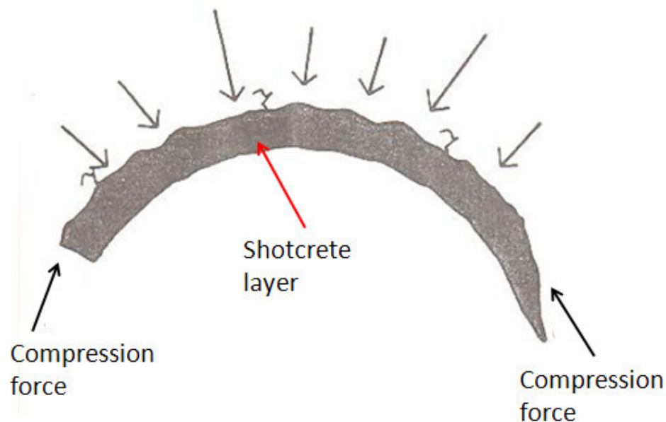
Figure 2.10 Shotcrete rock bearing capacity as an arch (After Stille and Franzen, 1990)
