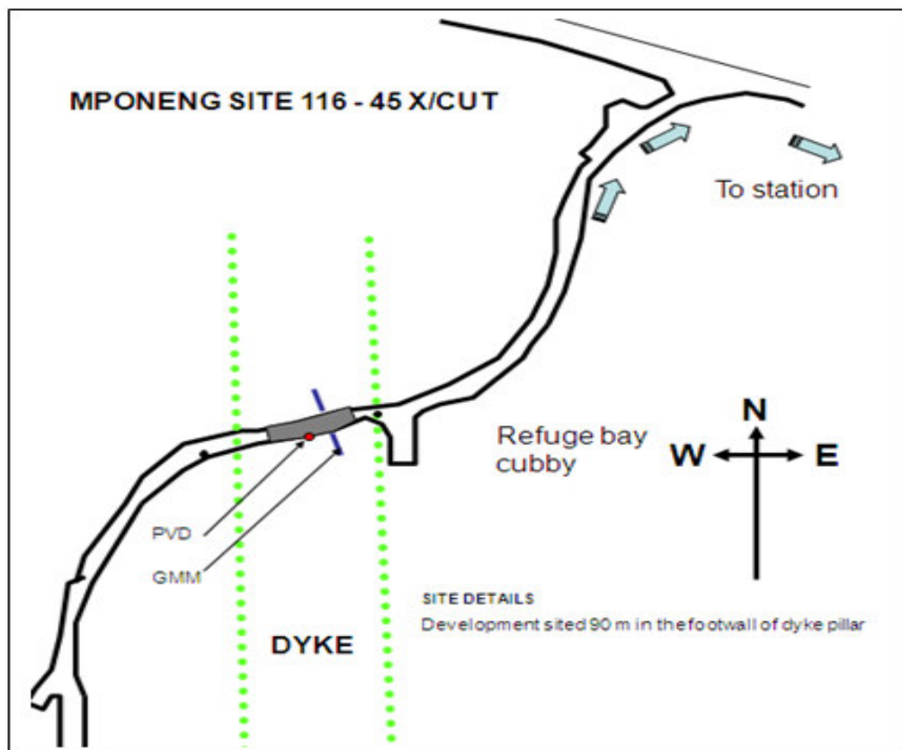
Figure 3.5 Mponeng Mine Level 116 site plan (SRK SIMRAC Internal report, 2008)
