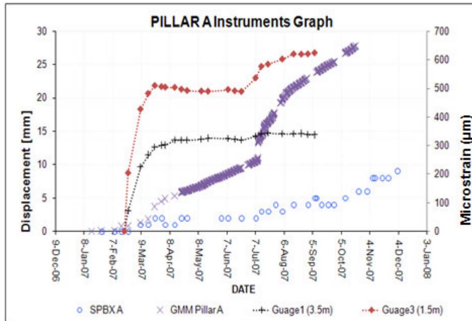
Figure 3.19 South Deep Mine Pillar A displacement and strain results
