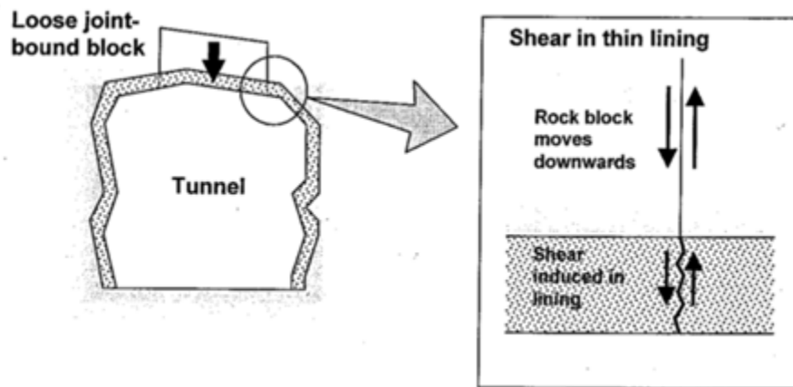
Figure 2.6 Shotcrete shear failure resulting from loose block movement (After Leach, 2002)
