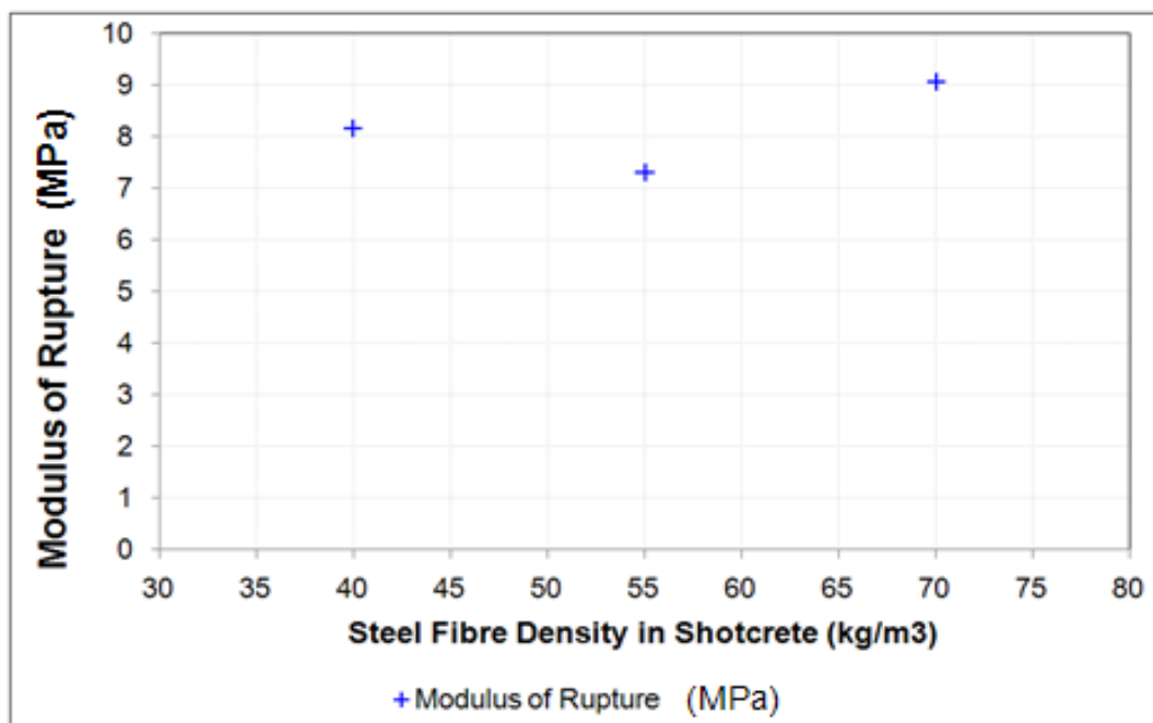
Figure 4.6 Modulus of rupture for the steel fibre reinforced ASTM shotcrete beams
