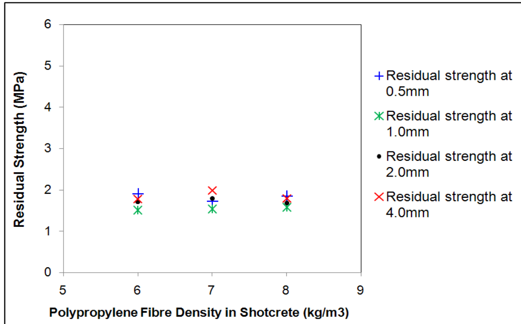
Figure 4.11 Residual strength for the polypropylene fibre reinforced shotcrete EFNARC beams
