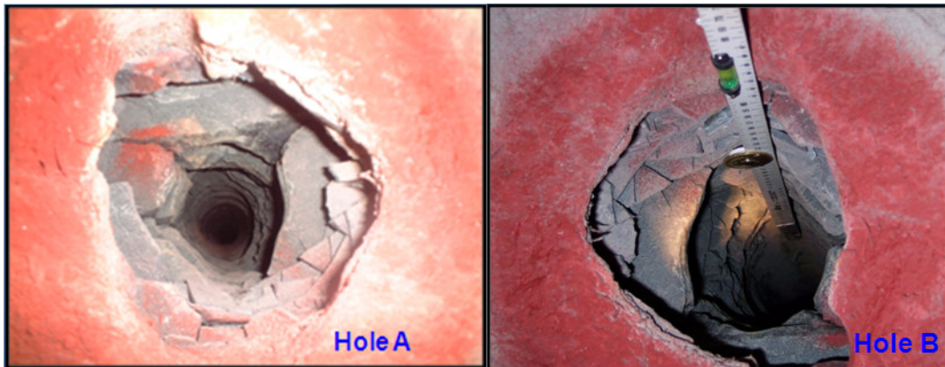
Figure 5.1a Borehole A and Borehole B in Mponeng Level 109 showing broken rock (about 0.5m) but interlocked in place by the shotcrete
