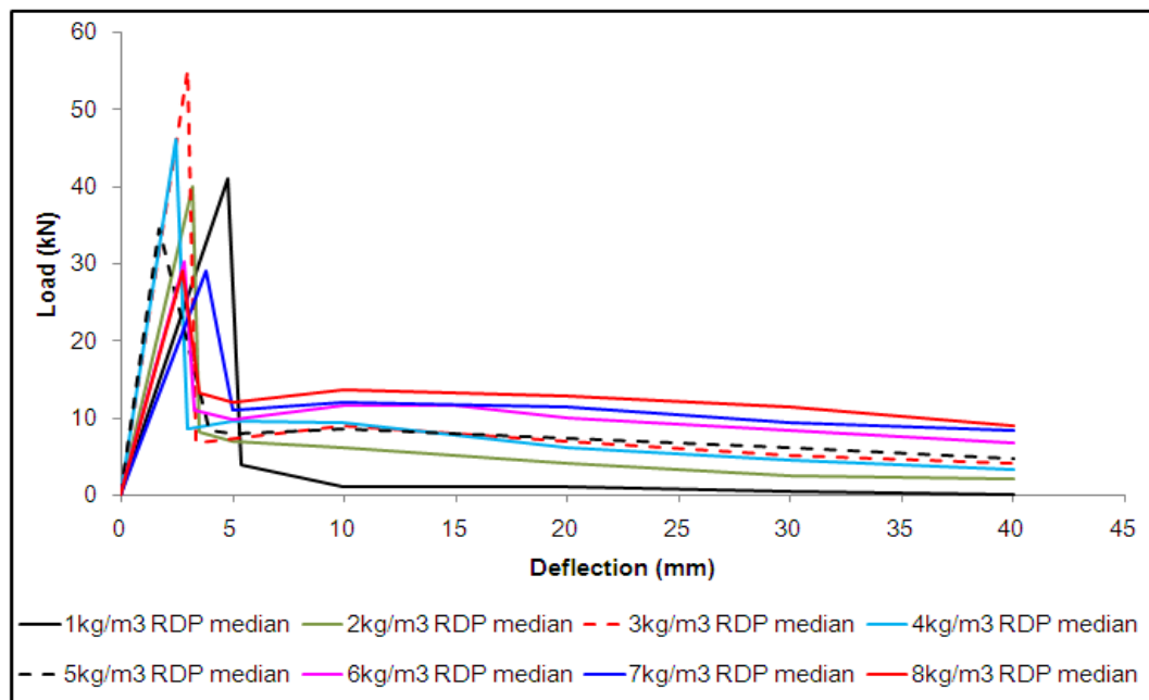
Figure 4.21 Load-deflection results for the polypropylene fibre reinforced shotcrete round determinate shotcrete panels
