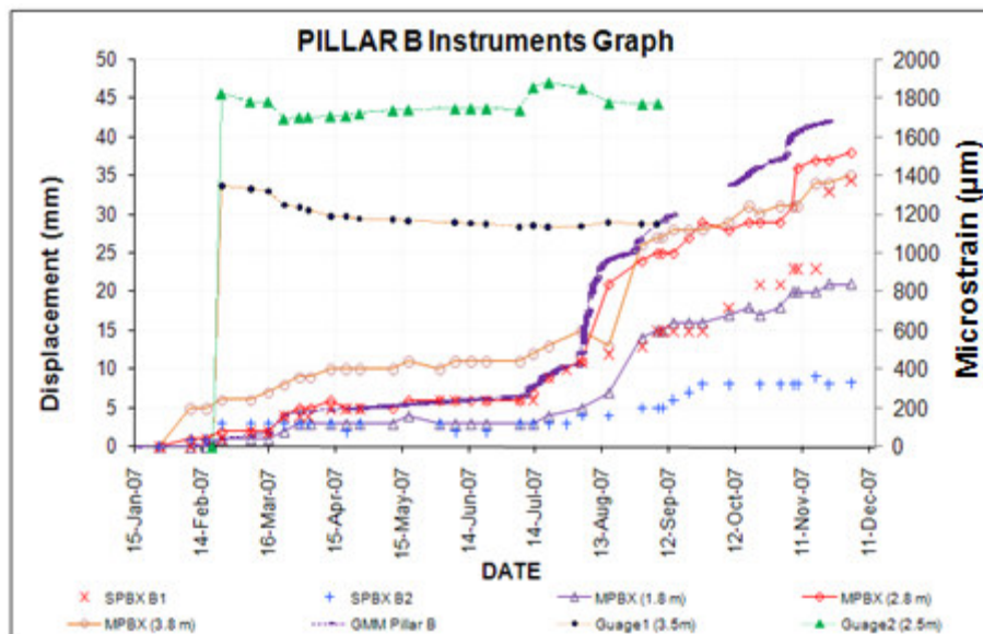
Figure 3.20 South Deep Mine Pillar B displacement results
