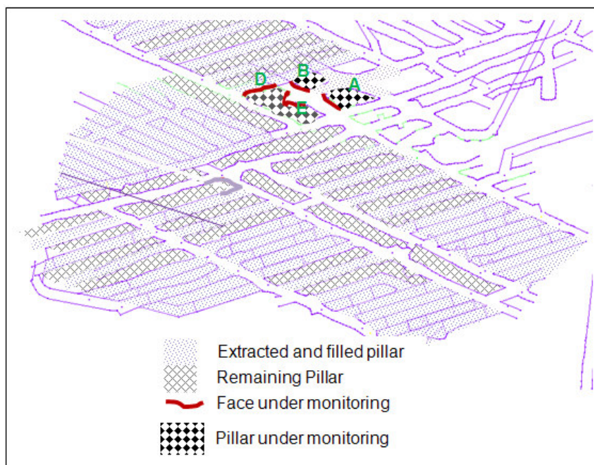
Figure 3.8 South Deep Mine plan showing location of test site (SRK SIMRAC Internal report, 2008)
