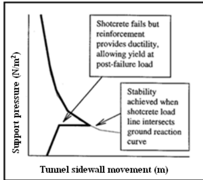
Figure 2.3c Shotcrete interaction with ground reaction curve: Stability with reinforced shotcrete (After Leach, 1998)
