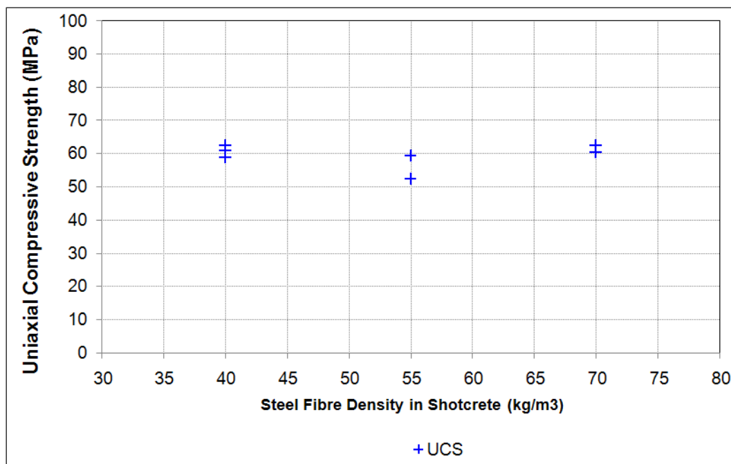
Figure 4.23 Uniaxial compressive strength test results for the steel fibre reinforced shotcrete cores
