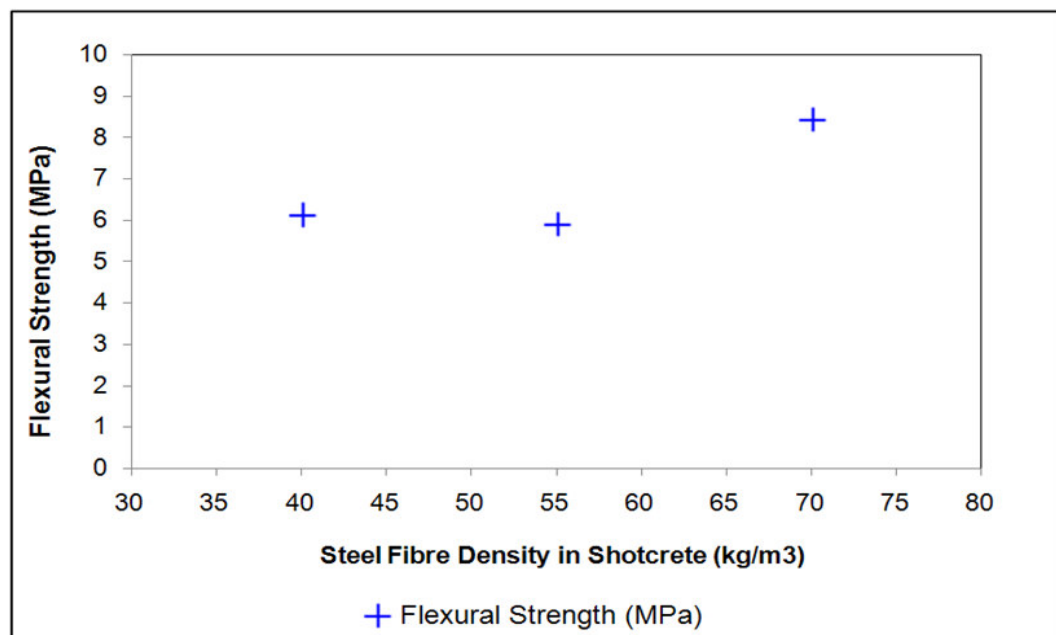
Figure 4.10 Flexural strength for the steel fibre reinforced shotcrete EFNARC beams
