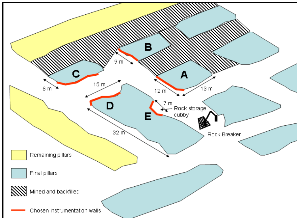
Figure 3.9 Test pillar detail at South Deep Mine Site (SRK SIMRAC Internal report, 2008)
