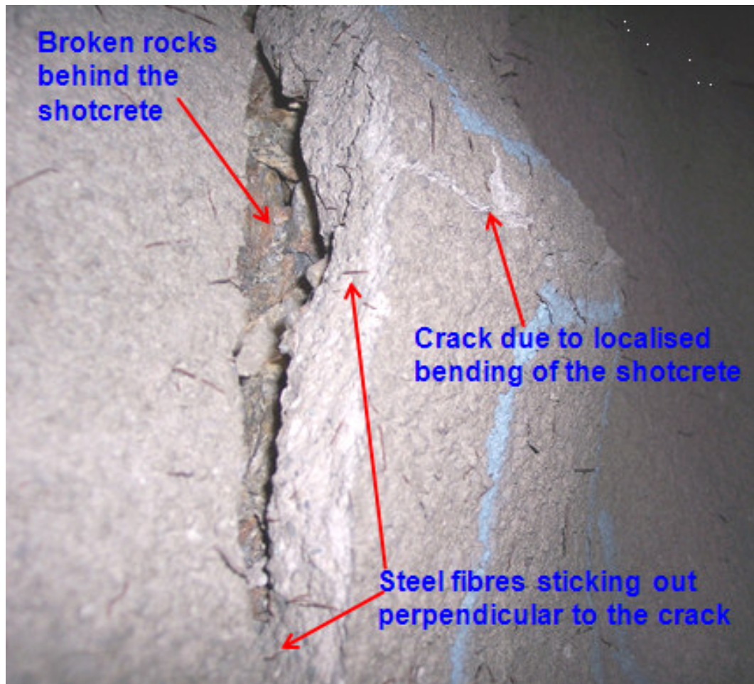
Figure 3.38b Photograph showing bending failure of shotcrete on Pillar B at South Deep Mine
