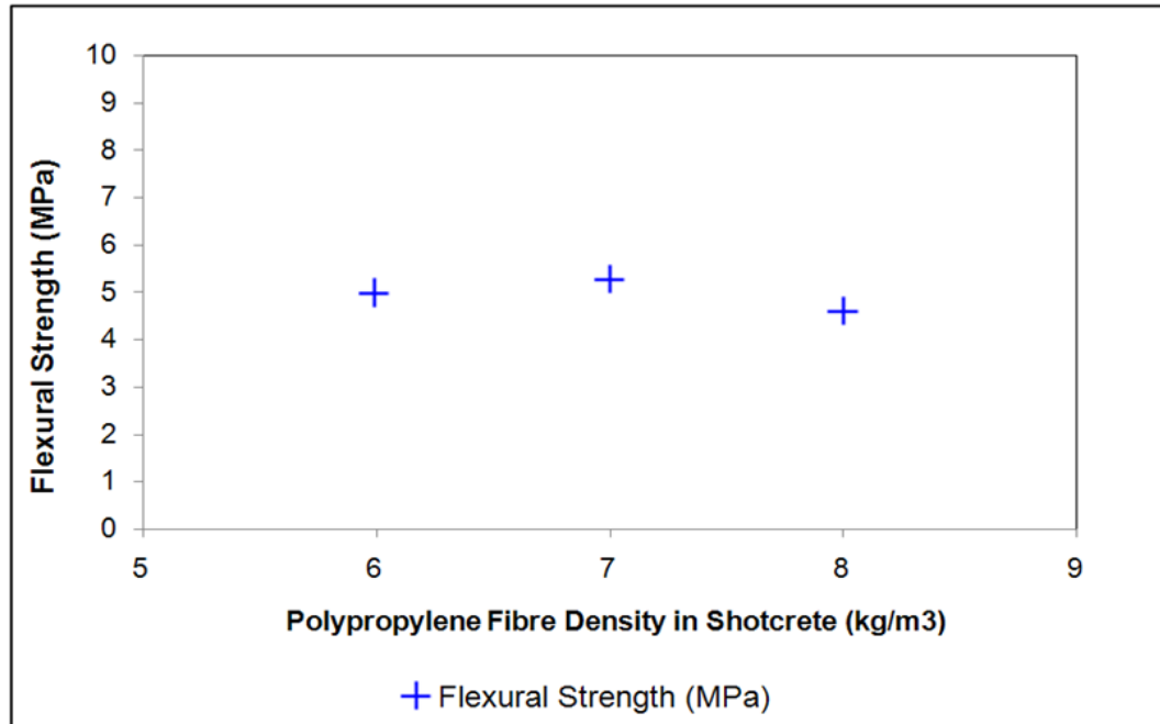
Figure 4.9 Flexural strength for the polypropylene fibre reinforced EFNARC beams
