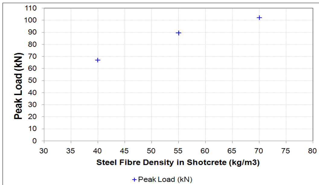
Figure 4.14 Peak loads for the steel fibre reinforced shotcrete EFNARC panels
