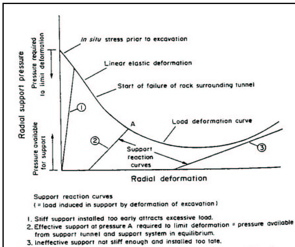
Figure 2.2 Simplified ground-support reaction curve (After Douglas and Arthur, 1983).
