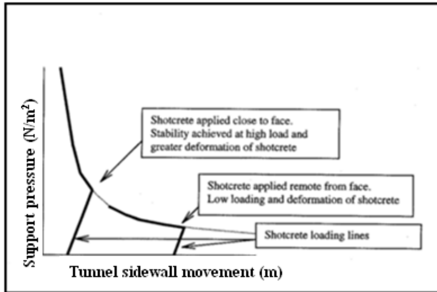
Figure 2.3a Shotcrete interaction with ground reaction curve: Difference between shotcrete applied close to the tunnel face and far from the tunnel face (After Leach, 1998)
