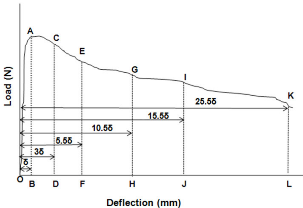
Figure 4.3 Determination of toughness indices (ASTM C1018, 1997)
