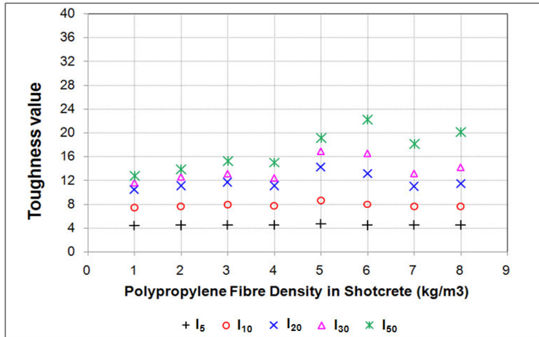
Figure 4.7 Toughness indices for the polypropylene fibre reinforced shotcrete ASTM beams
