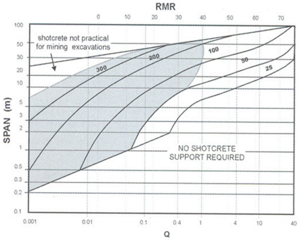
Figure 2.8 Simplified shotcrete design chart (Stacey, 2003, modified after Barton et al, 1974)
