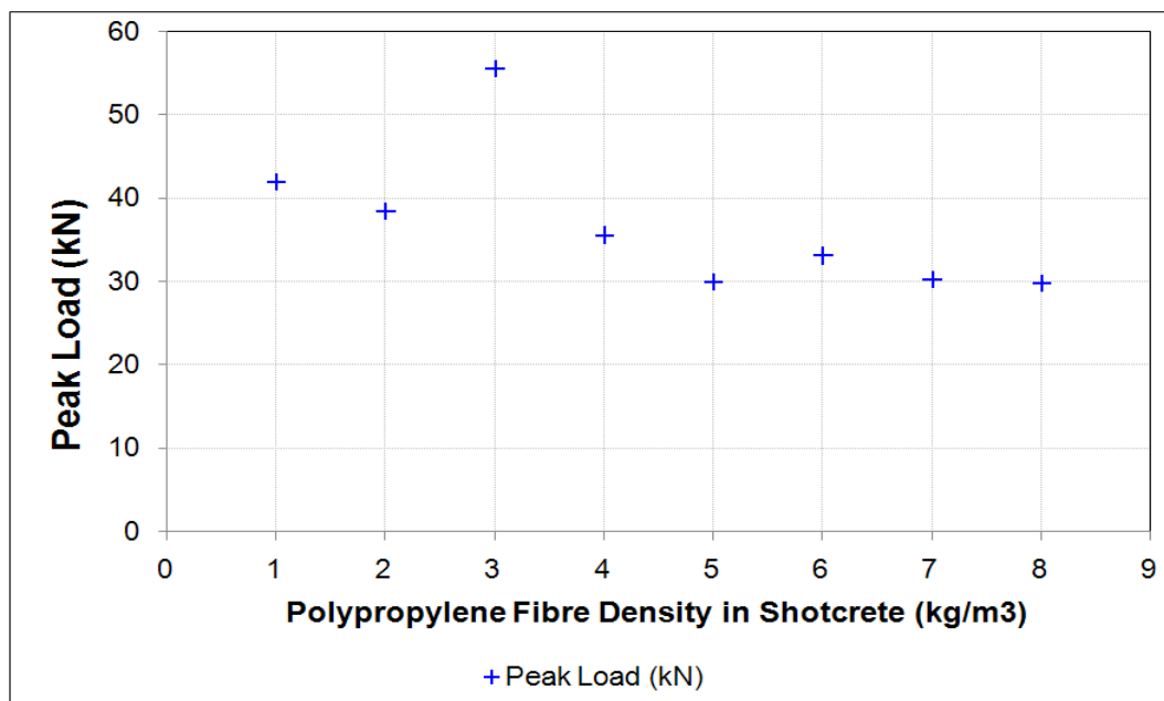
Figure 4.17 Peak loads for the polypropylene fibre reinforced shotcrete round determinate panels
