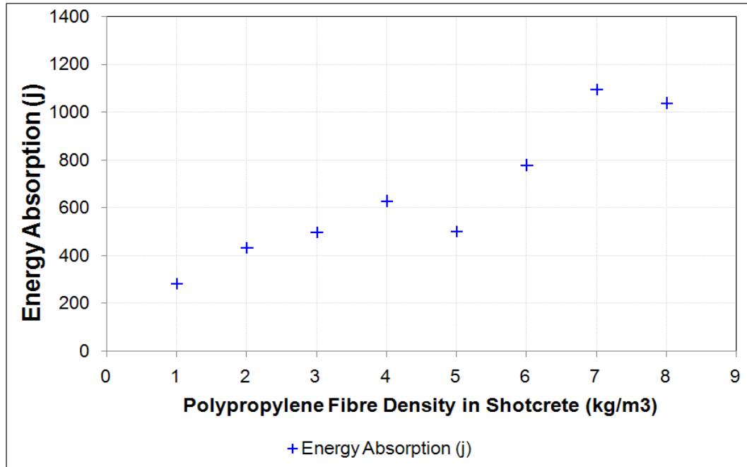
Figure 4.15 Energy absorption for the polypropylene fibre reinforced shotcrete EFNARC panels
