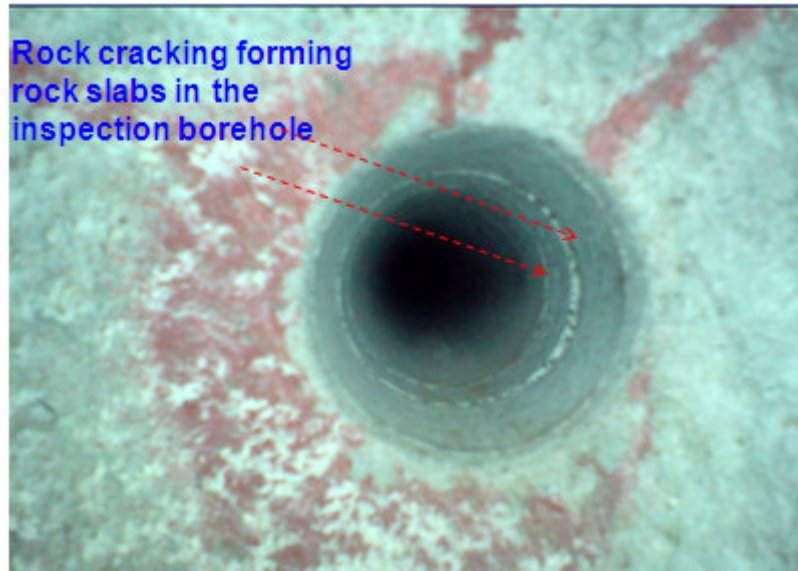
Figure 5.6 Cracks observed in a borehole showing a possibility of rock slabs forming in the tunnel walls due to mining induced stresses at Impala Platinum Mine
