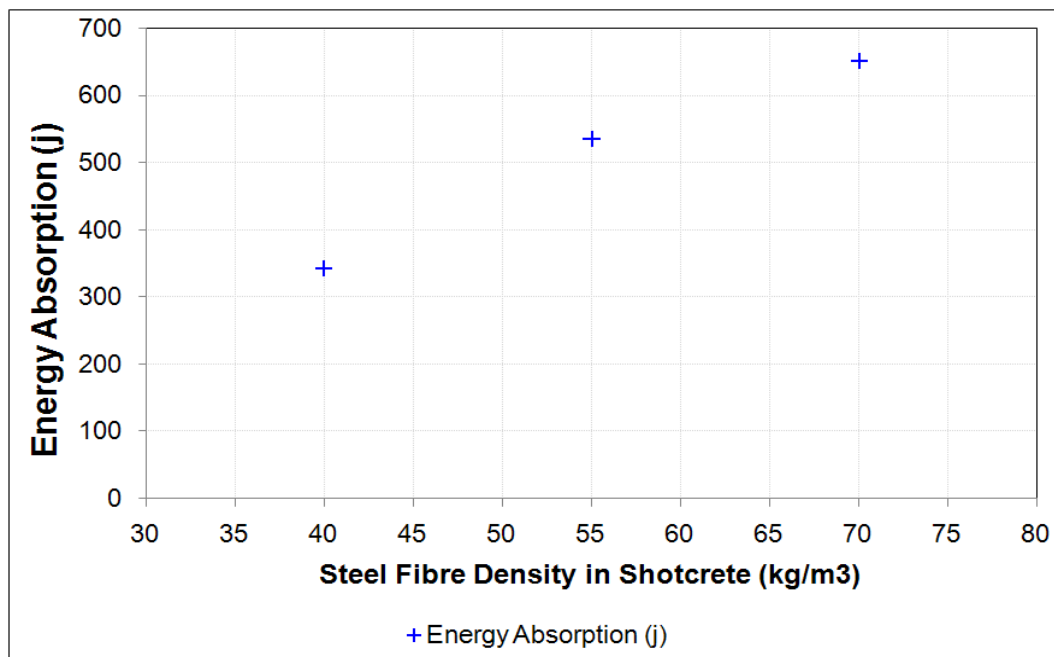
Figure 4.20 Energy absorption results for the steel fibre reinforced round determinate panels
