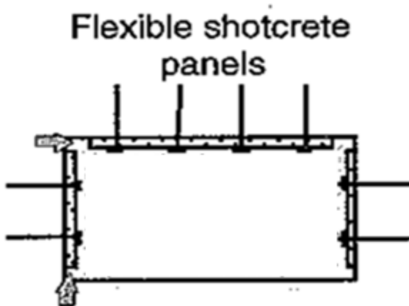
Figure 2.12 Shotcrete support as flexible retaining panels in a tunnel (After Kaiser and Tannant, 1997)
