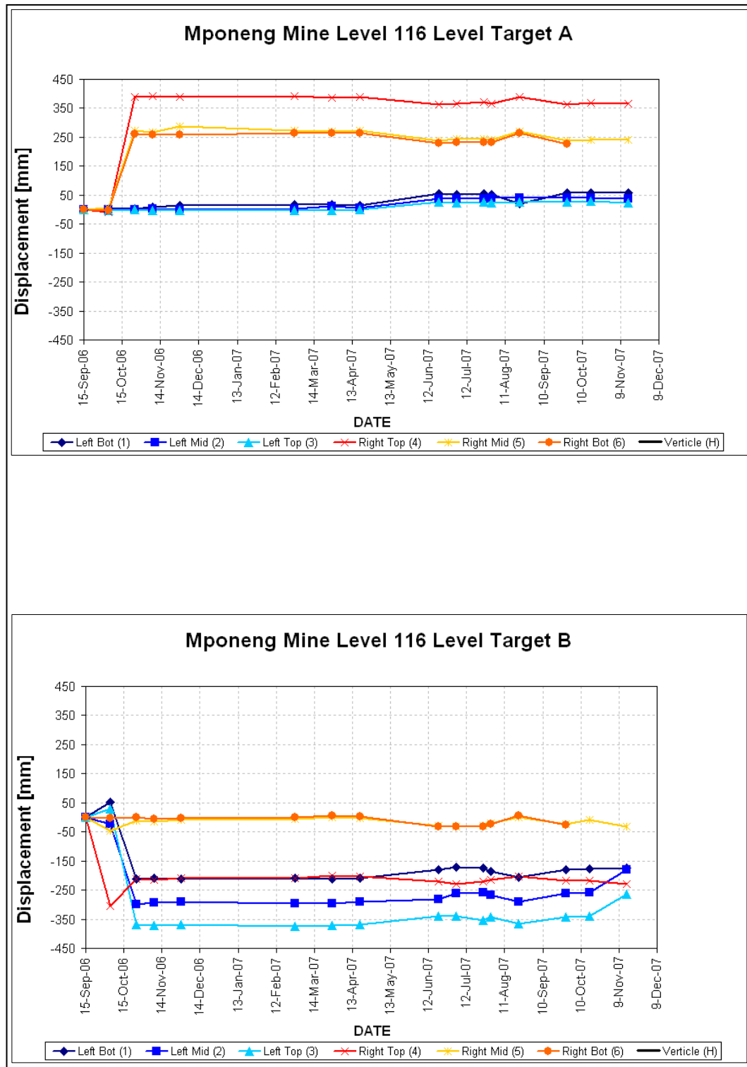
Figure 3.30 Laser targets displacement results for Mponeng Mine Level 116
