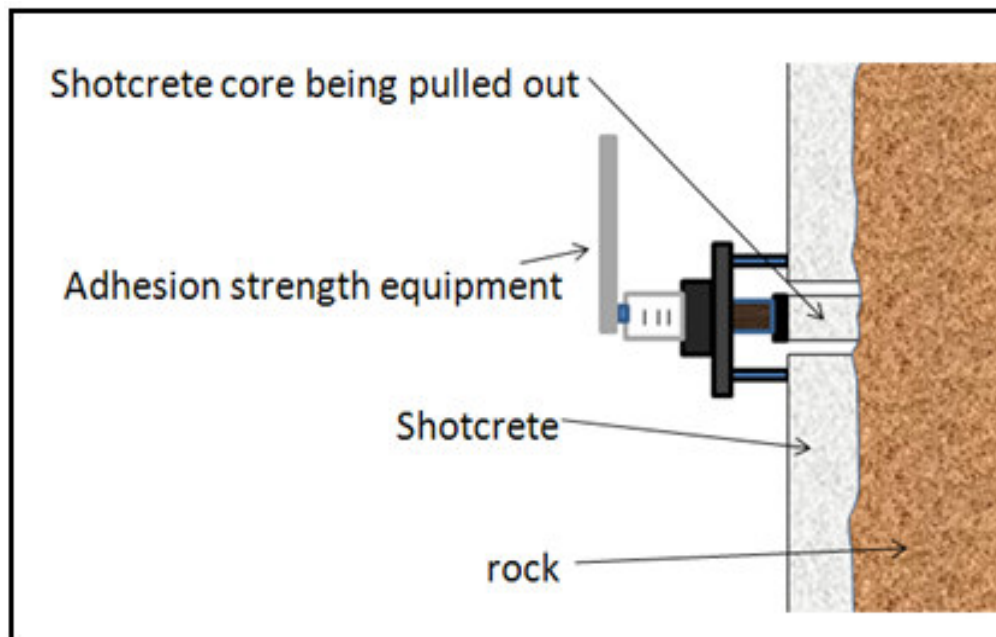
Figure 2.9 Adhesion testing equipment
