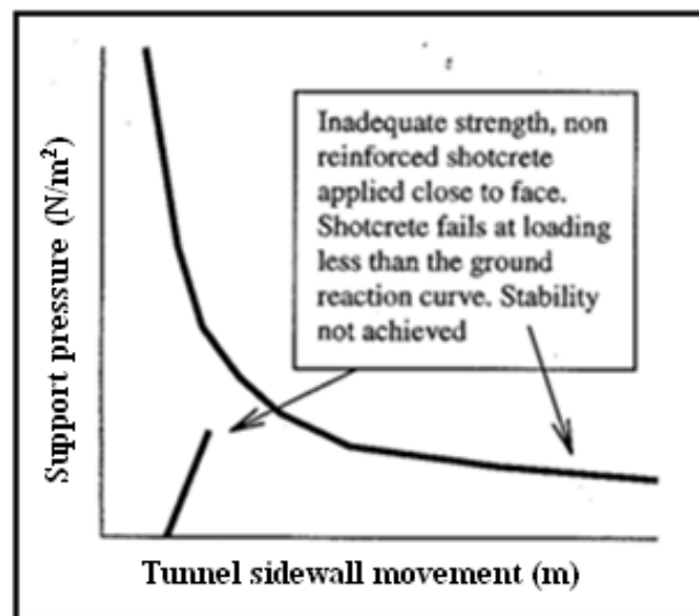
Figure 2.3b Shotcrete interaction with ground reaction curve illustrating the failure of plain shotcrete (After Leach, 1998)
