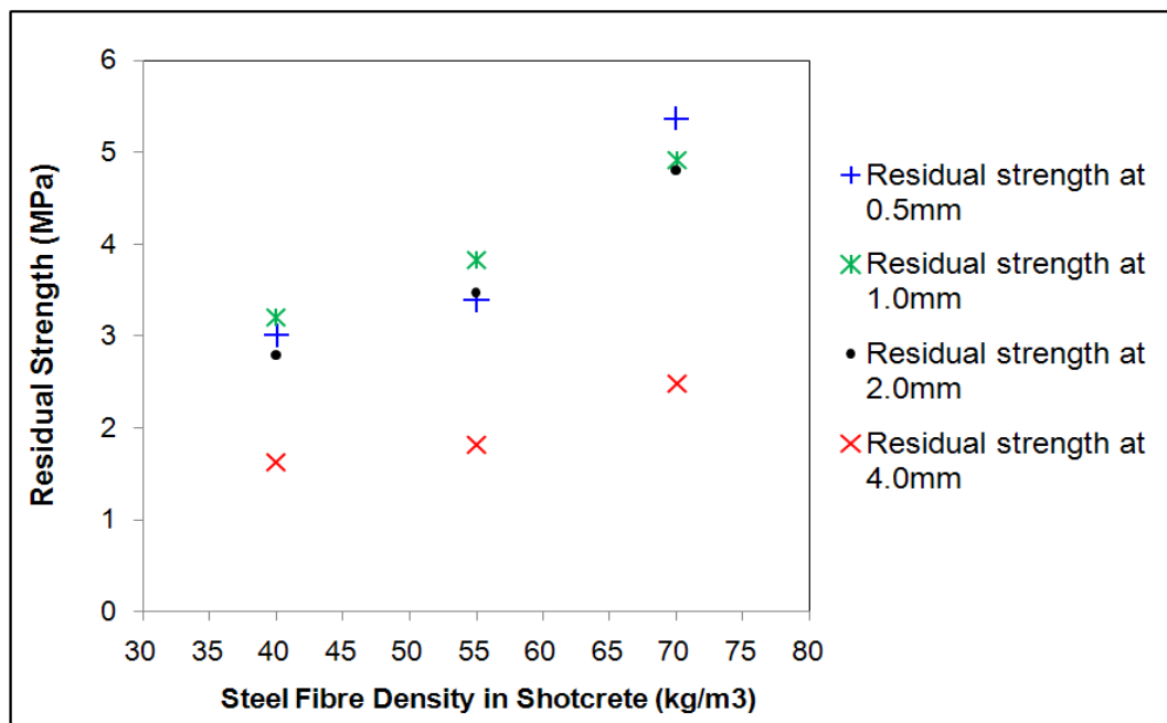
Figure 4.12 Residual strength for the steel fibre reinforced shotcrete EFNARC beams
