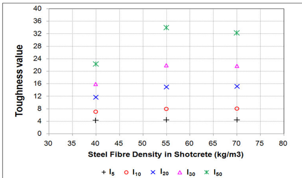
Figure 4.8 Toughness indices for the steel fibre reinforced shotcrete ASTM beams
