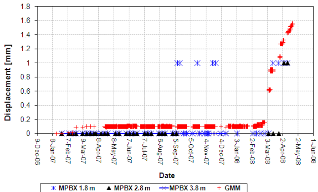
Figure 3.24 South Deep Mine MPBX and GMM monitoring results for Pillar E
