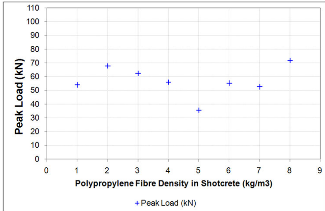
Figure 4.13 Peak loads for the polypropylene fibre reinforced shotcrete EFNARC panels
