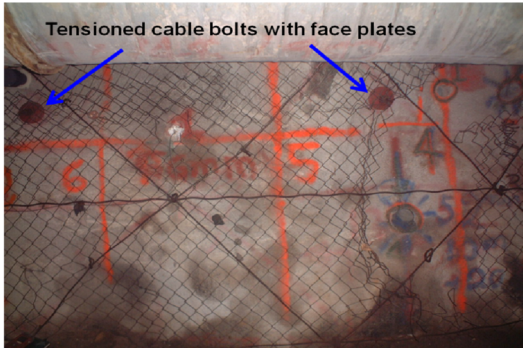
Figure 5.7 Tensioned cable bolting with face plates on the surface of shotcrete at Mponeng Mine Level 116
