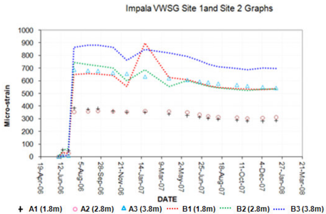
Figure 3.27 Impala Platinum Mine vibrating wire strain gauge results
