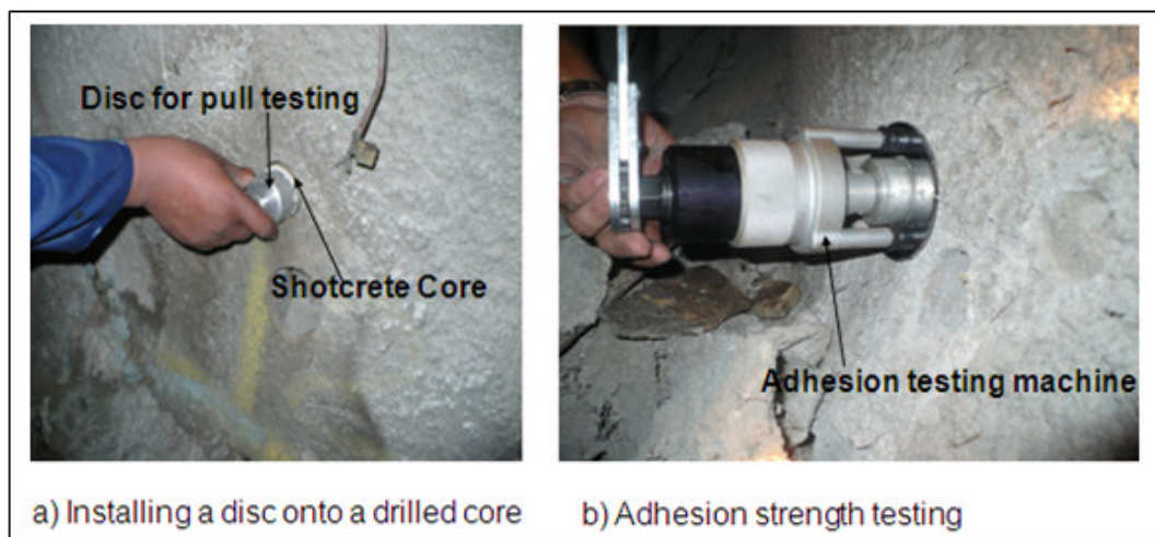
Figure 3.15 Photograph showing shotcrete-rock bond strength testing at South Deep Mine (Pillar A)
