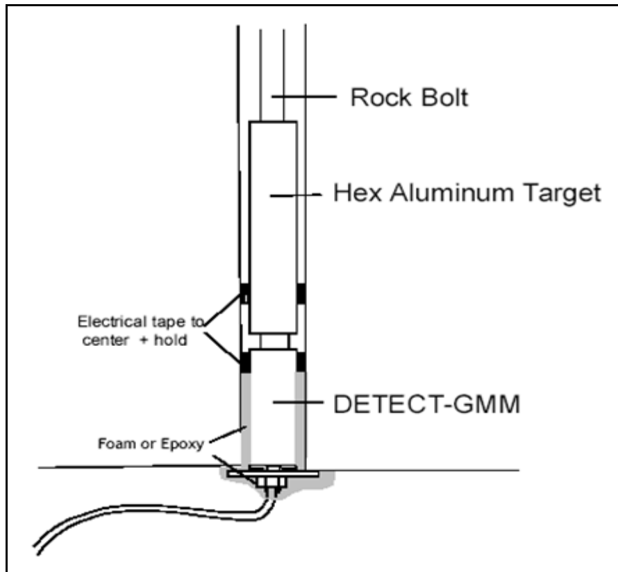
Figure 3.1 Ground motion monitor (GMM)
