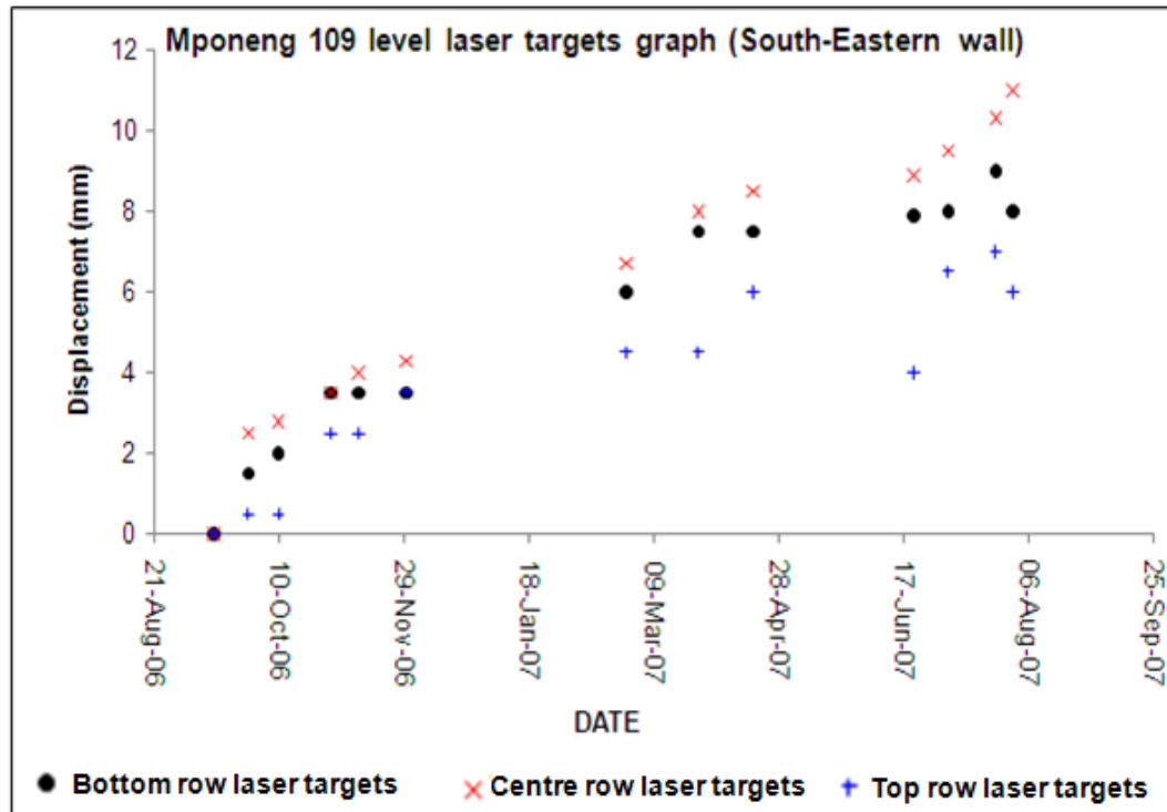
Figure 3.29 Mponeng Mine Level 109 South-East wall displacement results
