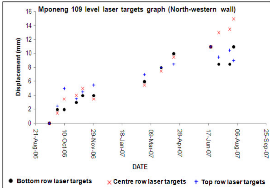
Figure 3.28 Mponeng Mine Level 109 North-West wall displacement results
