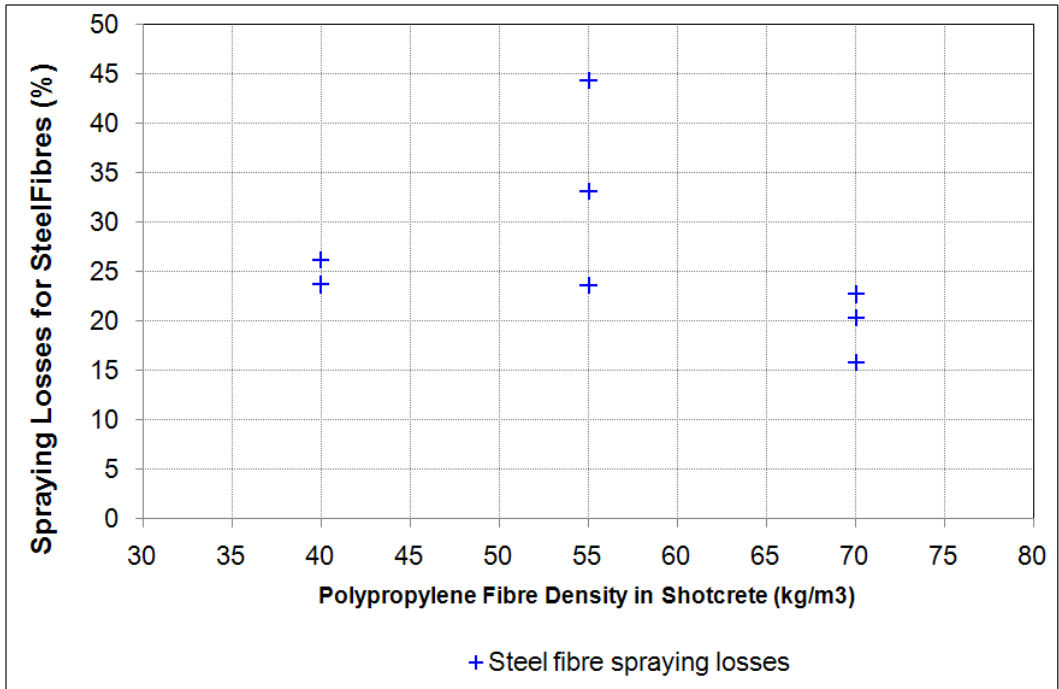
Figure 4.25 Steel fibre spraying rebound loss results for the steel fibre reinforced shotcrete specimens
