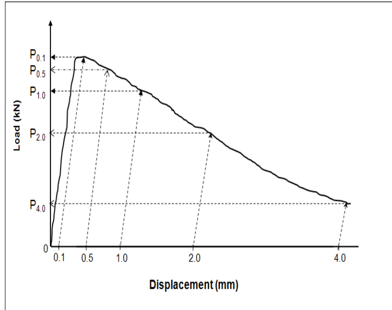
Figure 4.4 P values from the Load-Deflection graph for flexural and residual strengths (EFNARC, 1996)
