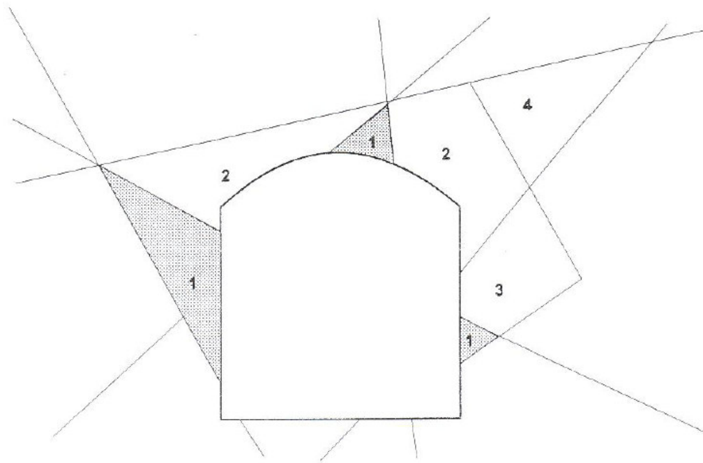
Figure 2.4 The key block theory diagram illustrating that when the shaded key blocks are stable, then stability around an excavation is maintained (After Barrett and McCreath, 1995)
