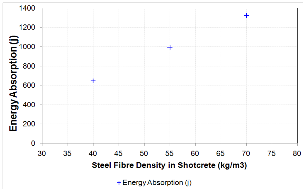
Figure 4.16 Energy absorption for the steel fibre reinforced shotcrete EFNARC panels
