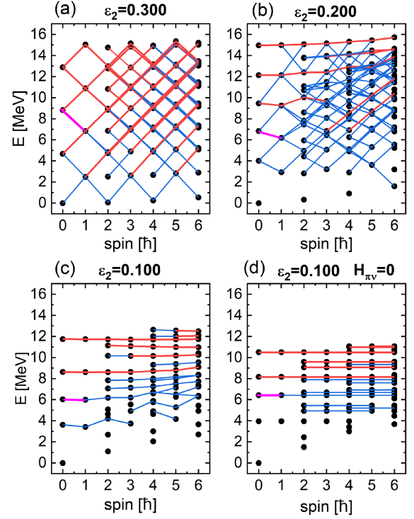
FIG. 2. The spectra and the M1 transitions calculated with the qp vacua. Panels (a)–(c) show results obtained with deformations \epsilon_2 = 0.3, 0.2 , and 0.1 , respectively, while panel (d) is the same as (c) except for a vanishing neutron-proton interaction. Dots in the plots represent the eigenstates and lines connecting them represent M1 transitions. For a given I state, we count both B(M1, I \rightarrow I - 1) and B(M1, I \rightarrow I + 1) . The red (thick) lines are for M1 transitions with B(M1) > 5\mu_N^2 and the blue (thin) lines are for those with 1\mu_N^2 < B(M1) < 5\mu_N^2 . Transitions with B(M1) < 1\mu_N^2 are not shown here. The magenta line highlights the M1 transition connecting the second 1^+ and third 0^+ states that will be analyzed later in Fig. 3.
