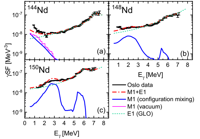
FIG. 1. Comparison of experimental \gamma SF data from the Oslo-method analysis (black solid line with error bars) [17], taken from the IAEA database [43], to the theoretical result (red dash dotted line) combined by the M1 \gamma SF (blue solid line) from the present calculation with full configuration mixing, and the E1 strength function (green dashed line) from the GLO or SLO fit to the giant or pygmy dipole resonances. Panel (a)–(c) gives the result for ^{144}\text{Nd} , ^{148}\text{Nd} and ^{150}\text{Nd} , respectively. The magenta steps for ^{148}\text{Nd} gives the M1 \gamma SF from the same calculation but with the qp vacuum configuration only.
