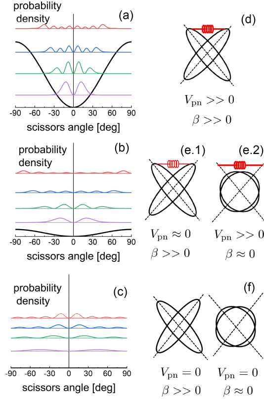
FIG. 4. Illustration of the scissors motion in strongly and weakly deformed nuclei, as well as in the limit case: A free scissors motion. (a) Schematic plot of the scissors potential (black line) as a function of the scissors angle, together with corresponding scissors angle distribution (colored lines), for well-deformed nuclei with a strong restoring force as illustrated in the cartoon representation in (d). (b) Similar to (a), but for well-deformed nuclei with a weak restoring force, as illustrated in the cartoon representation in (e.1), or for weakly deformed nuclei with a strong restoring force, as illustrated in (e.2). (c) Similar to (a), but for the limit case of free scissors motion, obtained with a vanishing neutron-proton interaction for well-deformed and near spherical nuclei, as illustrated in (f).
