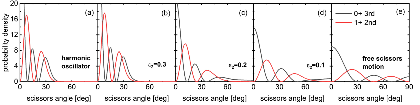
FIG. 3. Probability density distributions of the scissors angle for the third 0^+ state, 0_3^+ , and the second 1^+ state, 1_2^+ , in Fig. 2, connected by a strong M1 transition. Panel (a) gives the analytical result of the harmonic oscillator limit and panel (e) gives the analytical result of the free scissors motion. The numerical results from the angular-momentum-projected model with the qp vacuum configuration for deformations \epsilon_2 = 0.3, 0.2 , and 0.1 are shown in panels (b), (c), and (d), respectively.
