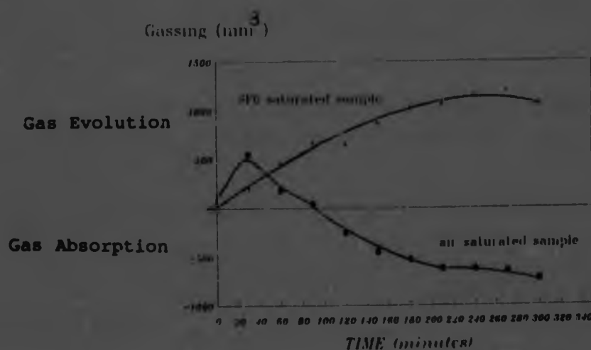
Figure - 2.2 Gassing of transformer oil Comparison of Air and \text{SF}_6
