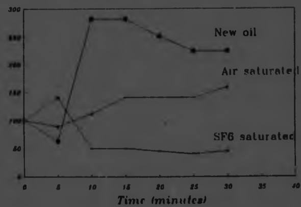
Figure 3.2 - Partial discharge magnitude - Transformer oil
