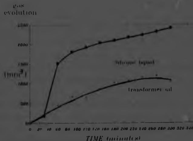
Figure 2.5 - gassing of \text{SF}_6 saturated liquids Comparison of transformer oil and silicone liquid
