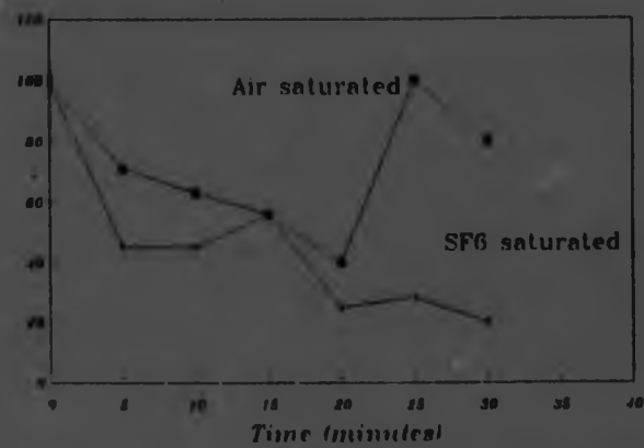
Figure 3.3 - Partial discharge magnitude - Silicone liquid
