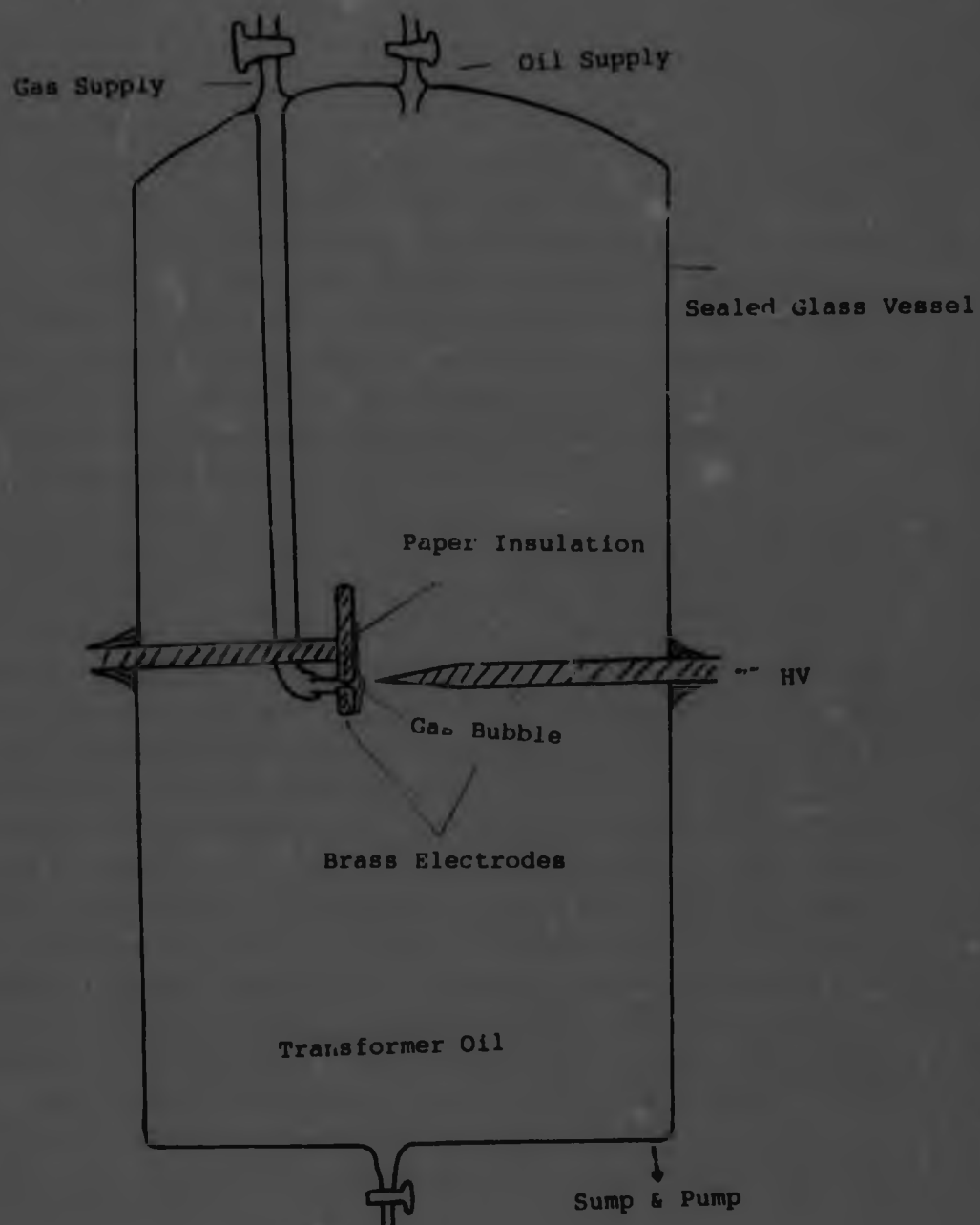
Figure 4.1 - Apparatus for Investigating Partial Discharge Activities
