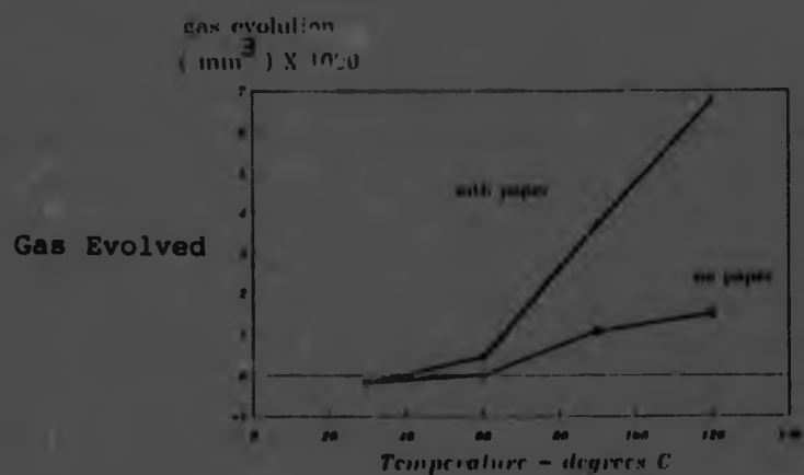
Figure 2.13 - Air Saturated Transformer Oil (with and without paper insulation)
