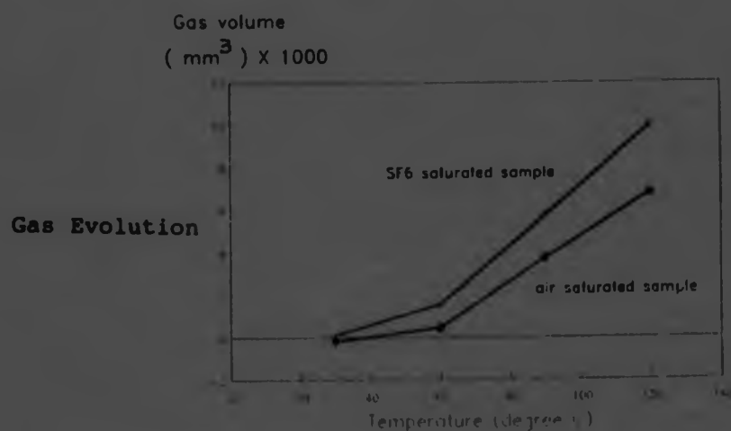
Figure 2.11 - Gassing of Transformer Oil and Paper (Air saturated & \text{SF}_6 saturated)
