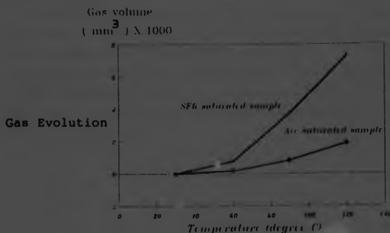
Figure 2.9 - Silicone liquid Air saturated & \text{SF}_6 saturated samples
