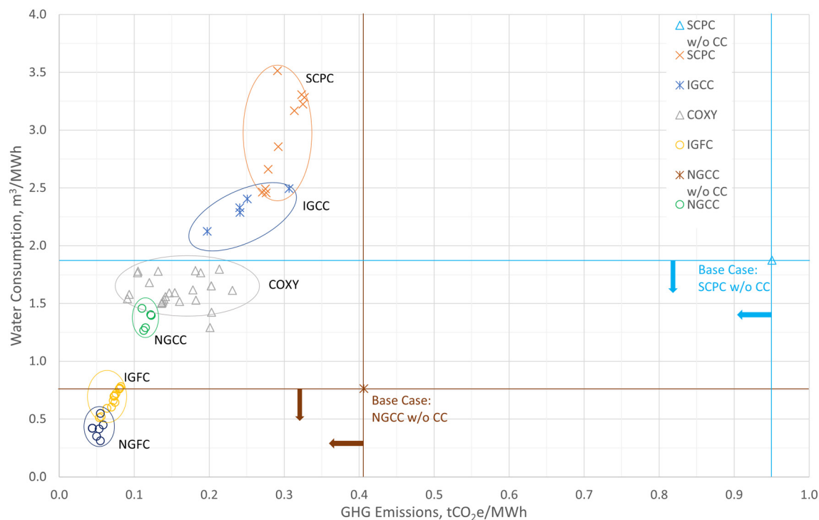
Fig. 9 Water consumption vs. GHG emissions of coal and natural gas fired carbon capture technologies.
