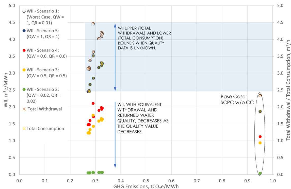
Fig. 10 WII and water usage vs. GHG emissions for a high WSI (0.999) and varying water qualities for SCPC technology cases.
