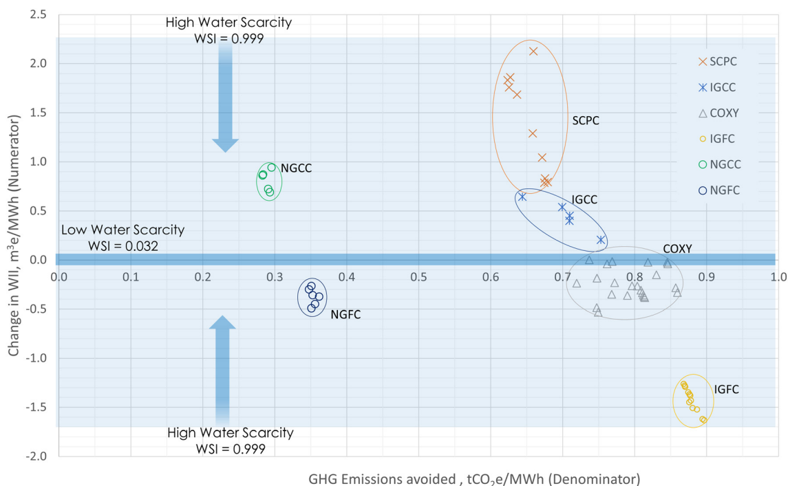
Fig. 12 Change in WII relative to carbon dioxide avoided using the worst-case scenario for water qualities and a high water scarcity index (WSI = 0.999). Blue shading reflects the impact of decreasing water scarcity; the data range moves in the direction of the arrows as the WSI decreases. See Fig. 13 for the magnified version of the darker blue shading at low water scarcity = 0.032.
