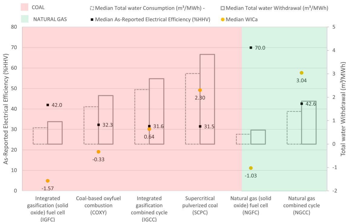
Fig. 14 Summary of the relationship between technology efficiencies, water usage and the WII.
