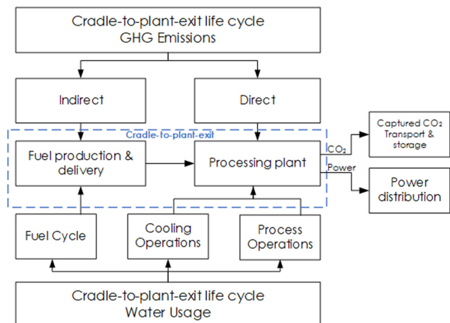
Fig. 6 Cradle-to-plant-exit life cycle water stages corresponding to GHG emissions.
