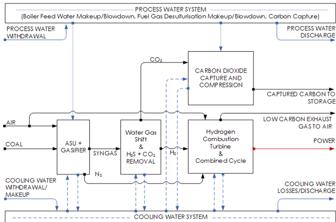
Fig. 3 Pre-combustion capture schematic for in coal-fired power generation plants (IGCC).
