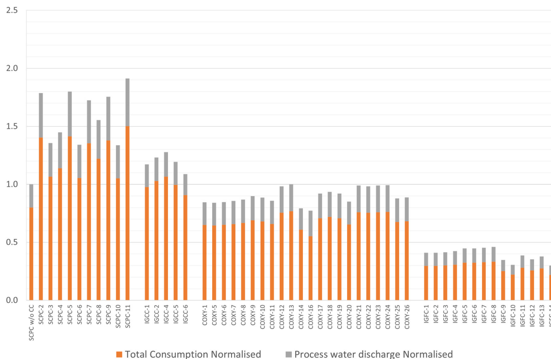
Fig. 7 Overall water usage data for carbon capture technologies in coal-fired plants.
