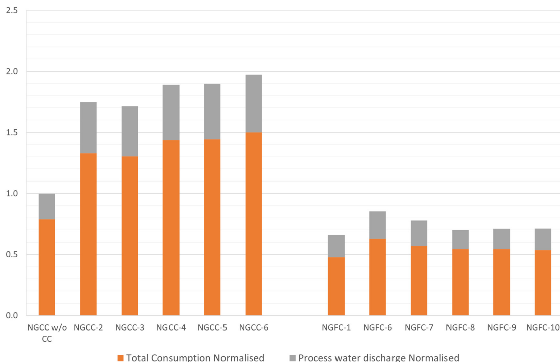
Fig. 8 Overall water usage data for carbon capture technologies in gas-fired plants.
