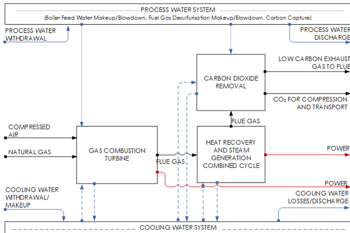
Fig. 2 Post-combustion capture schematic for natural-gas fired power generation plants.
