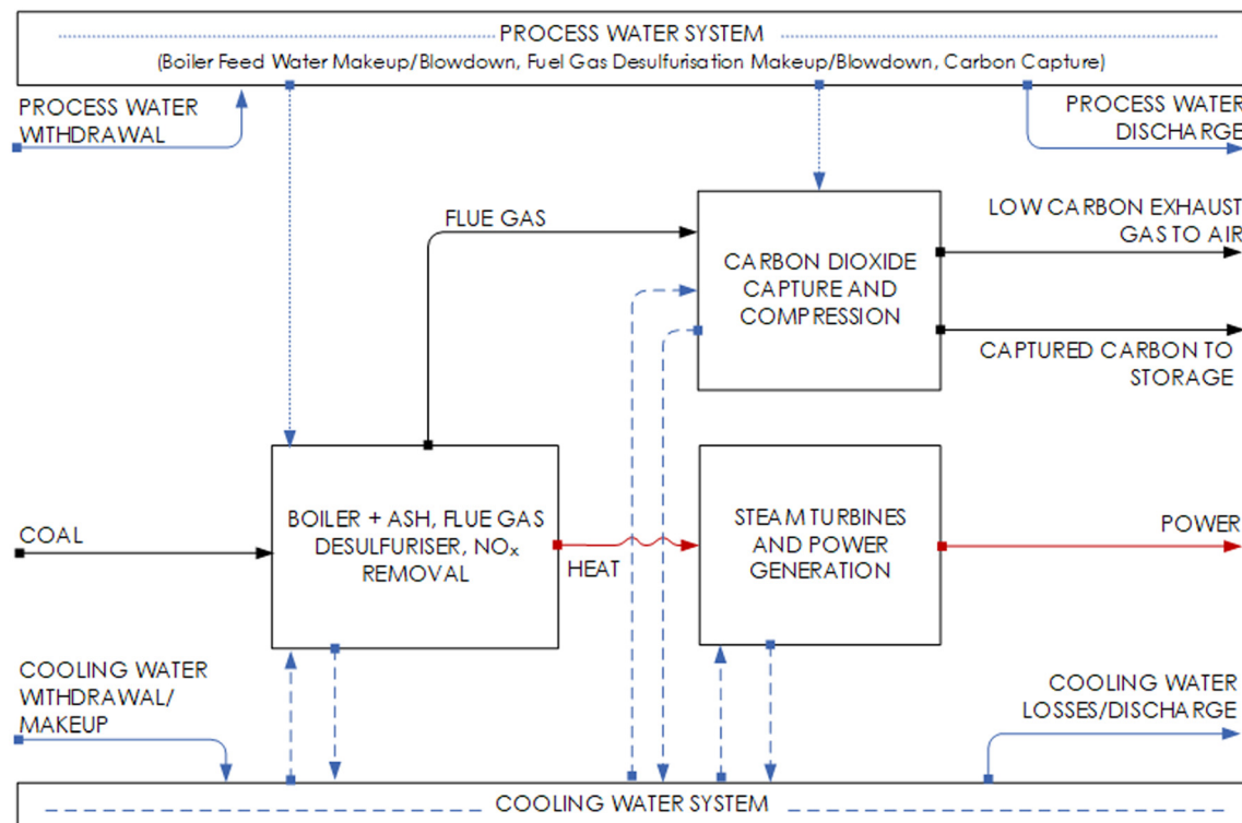
Fig. 1 Post-combustion capture schematic for coal-fired power generation plants.
