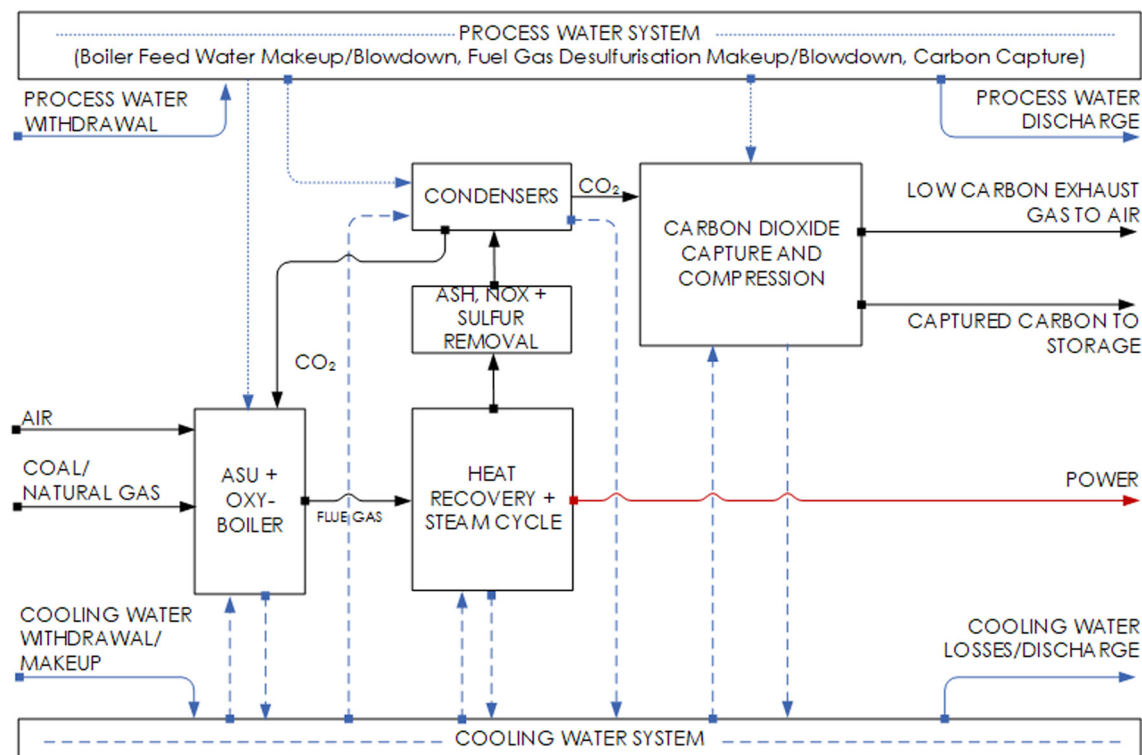
Fig. 4 Oxy-fuel combustion schematic for coal- or natural gas-fired power generation plants.
