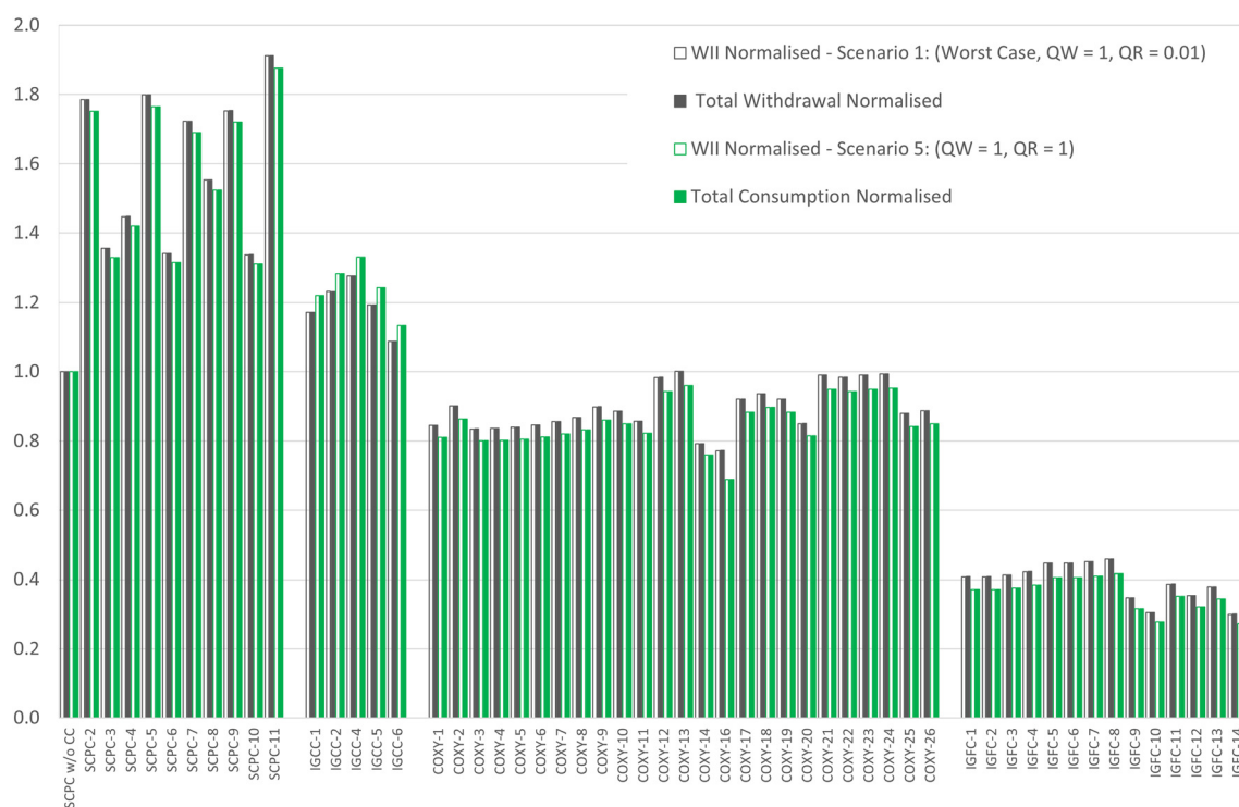
Fig. 11 Relationship between normalised WII and normalised withdrawal and consumption values for coal fired carbon capture technologies at a high WSI.
