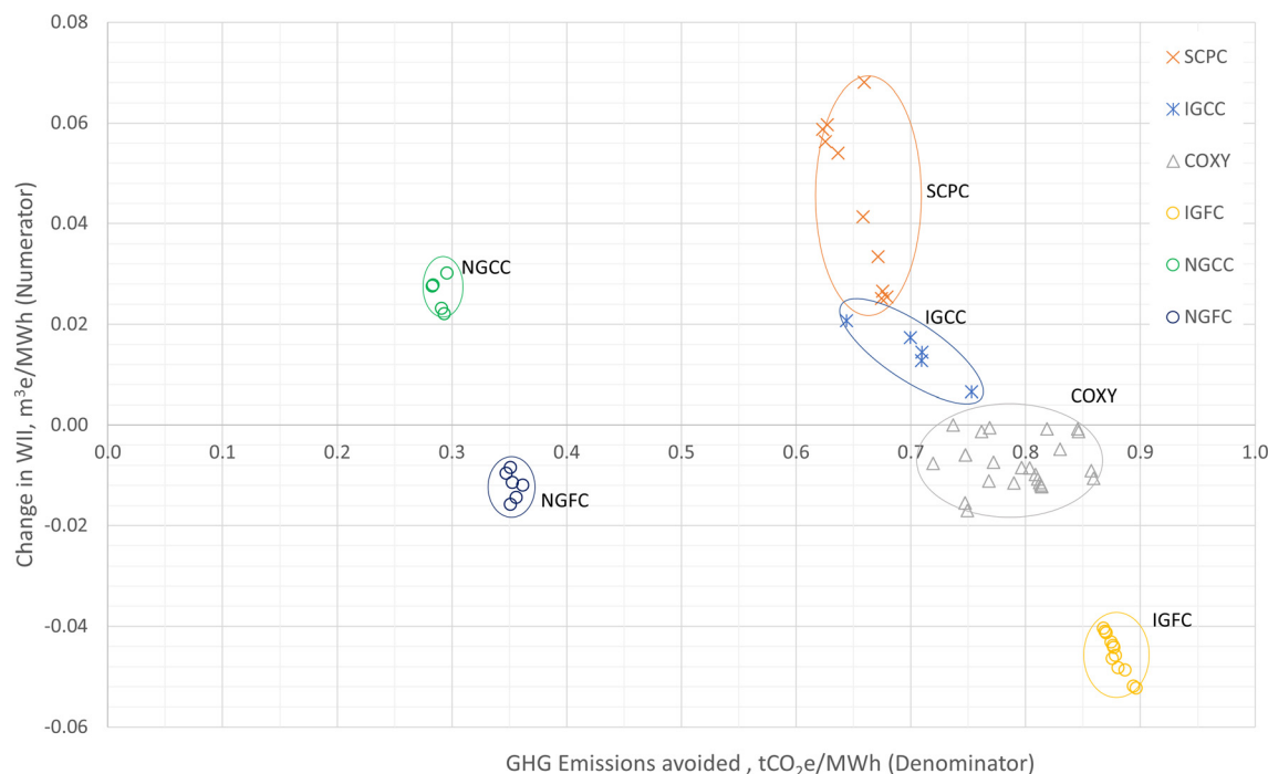
Fig. 13 Change in WII relative to carbon dioxide avoided using the worst-case scenario for water qualities and a low water scarcity index (WSI = 0.032). The expanded graph at high water scarcity (WSI = 0.999) is shown in Fig. 12.
