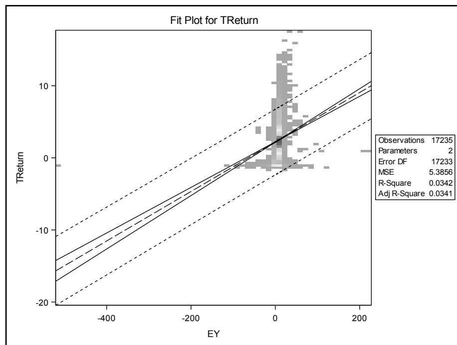
Plot 4 - Fit Plot of the Earnings Yield
