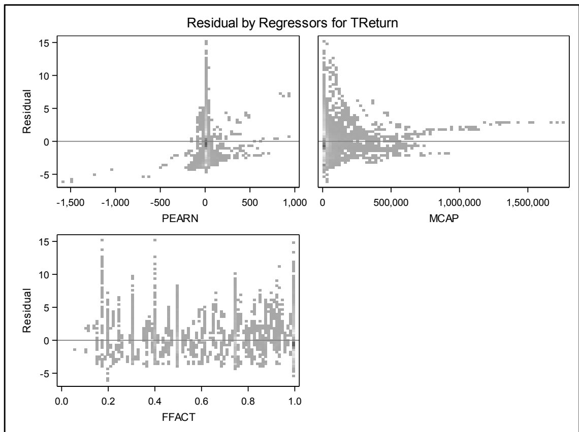
Figure 3: Residual by Regressors for TReturn – Hypothesis 3
