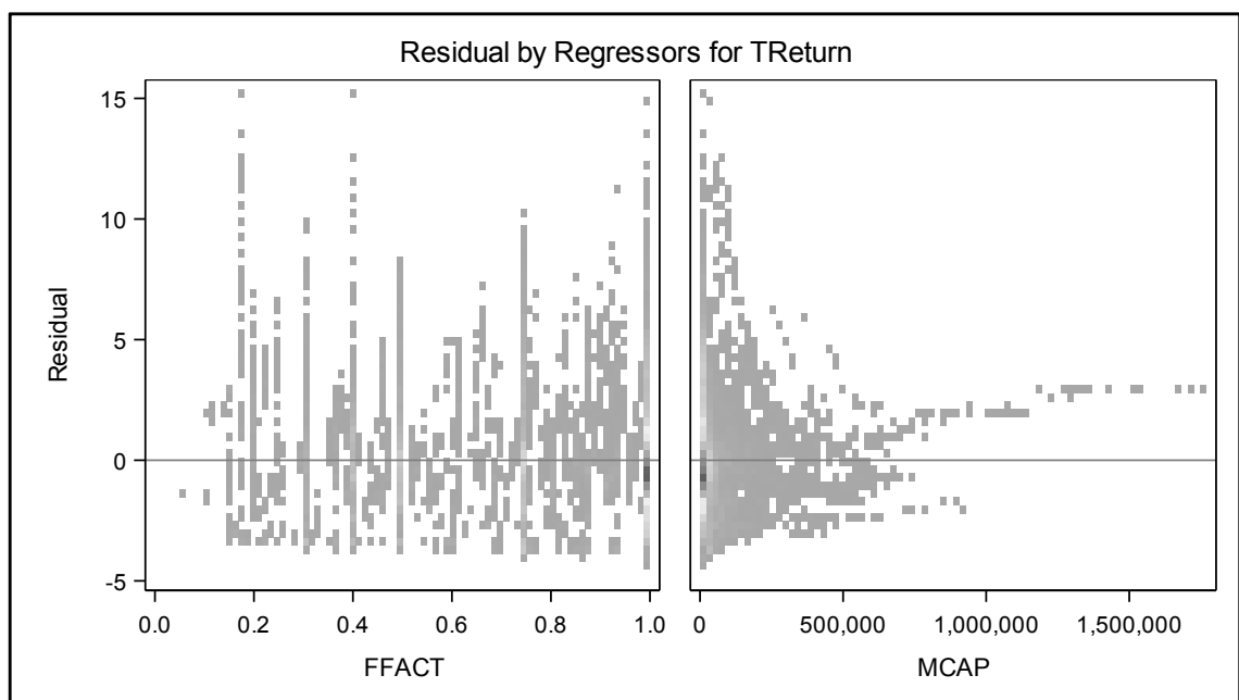
Figure 2: Residual by Regressors for TReturn - Hypothesis 2
