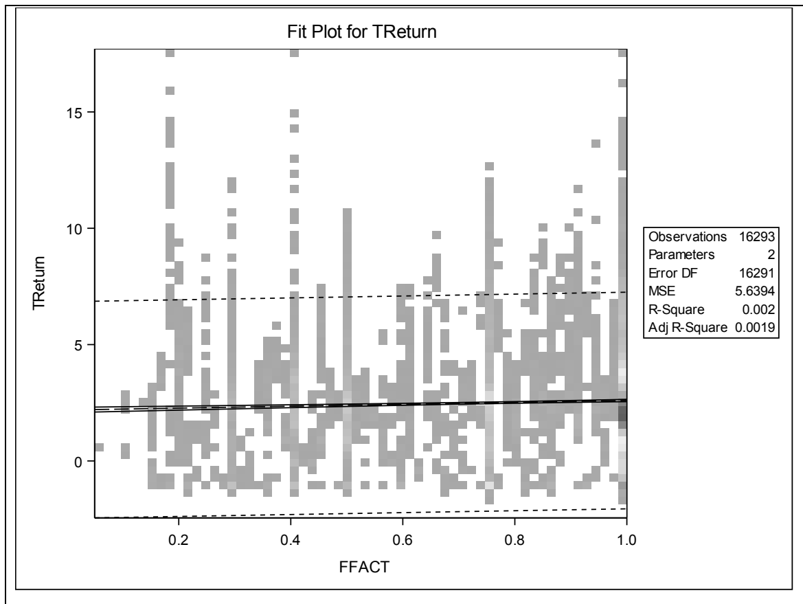
Figure 1: Fit Plot for TReturn – Hypothesis 1
