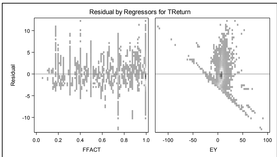
Figure 4: Residual by Regressors for TReturn – Hypothesis 4
