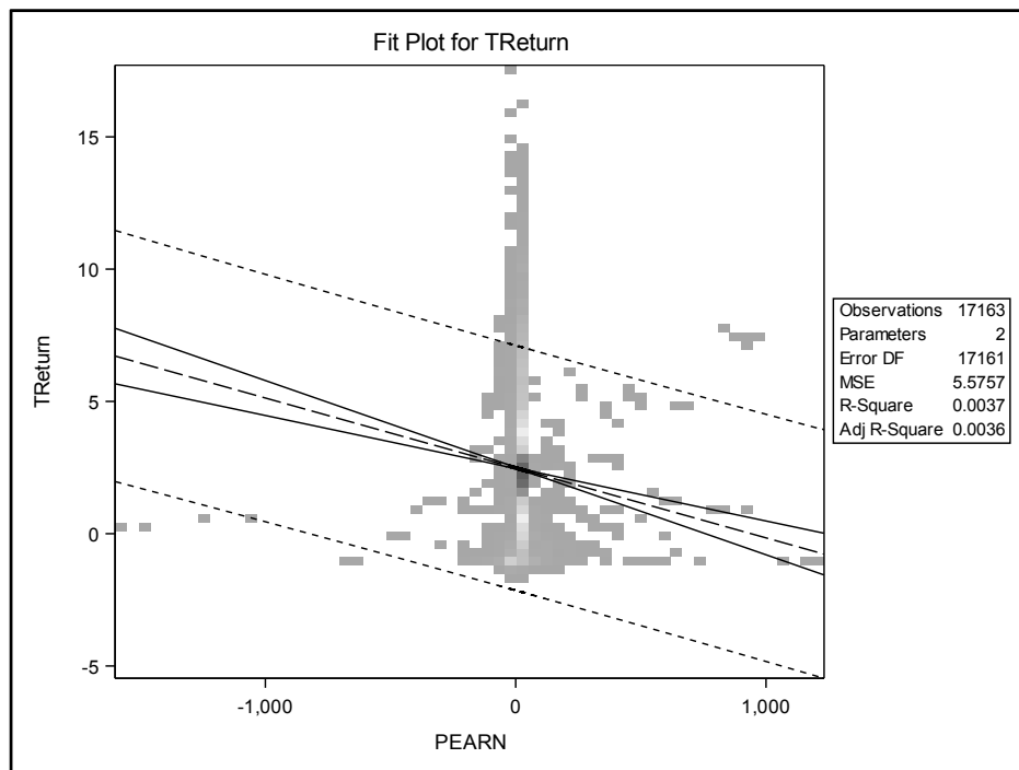
Plot 5 - Fit Plot of the Price Earnings Ratio
