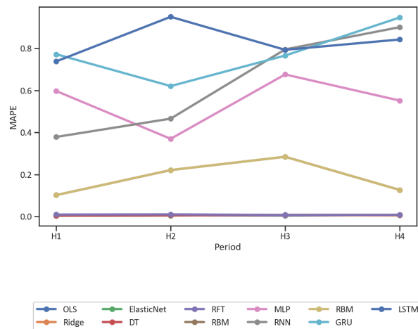
FIGURE 4.8: The top performance of each machine learning model over four periods
