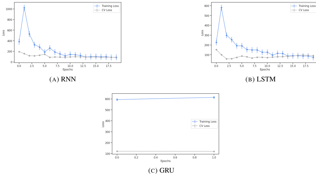
FIGURE 4.2: The loss function value across epochs of default neural networks when forecasting the reaction of stock market returns to changing economic activities in South Africa
