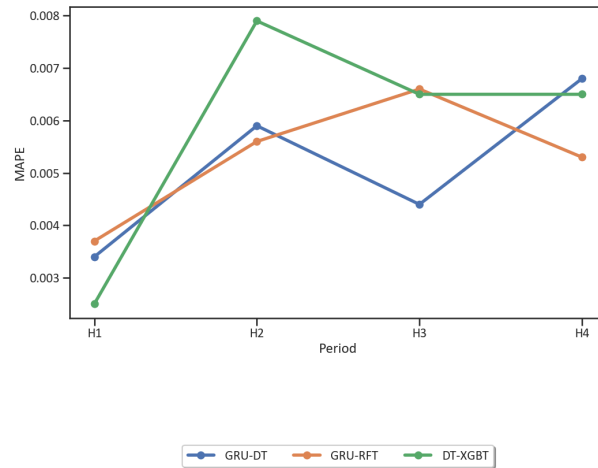
FIGURE 4.9: The top performance of each tree-based feature selection strategy
