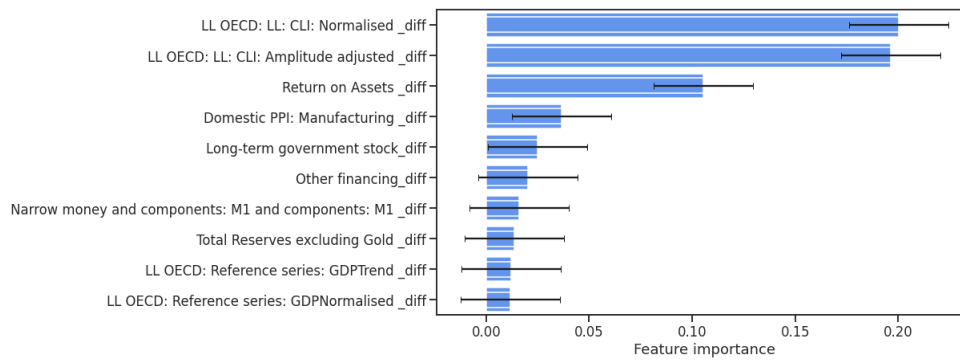
FIGURE 4.4: The top ten economic features in a feature subset selected by the random forest tree model, as measured by the gini impurity value
