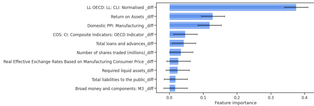
FIGURE 4.3: The top ten economic features in a feature subset selected by the decision tree model, as measured by the gini impurity value
