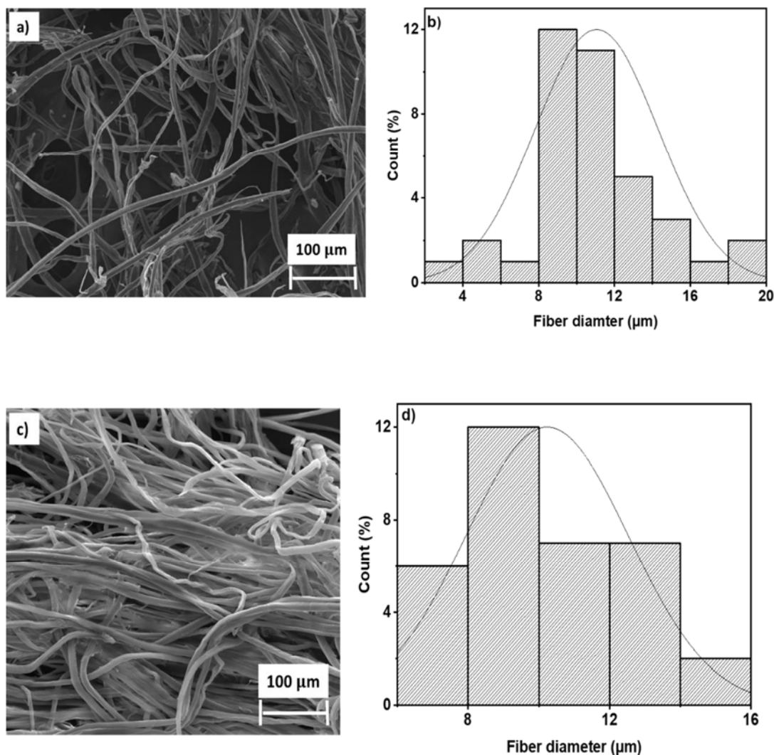
Figure 6.3: SEM images of a) bleached and c) cationised cellulose, and histograms of b) bleached and d) cationised cellulose.
