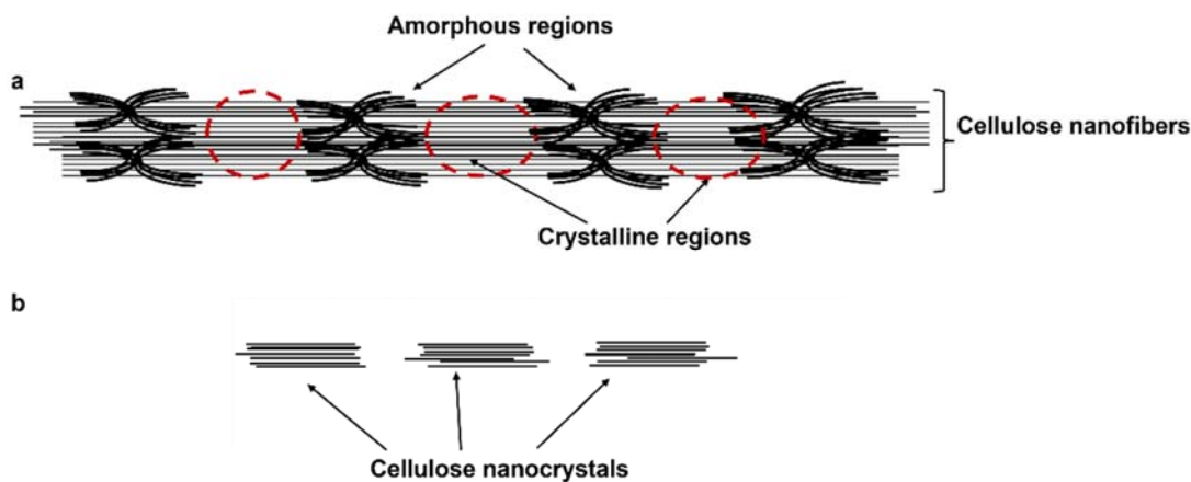
Figure 2.5: Cellulose acid hydrolysis mechanism.
