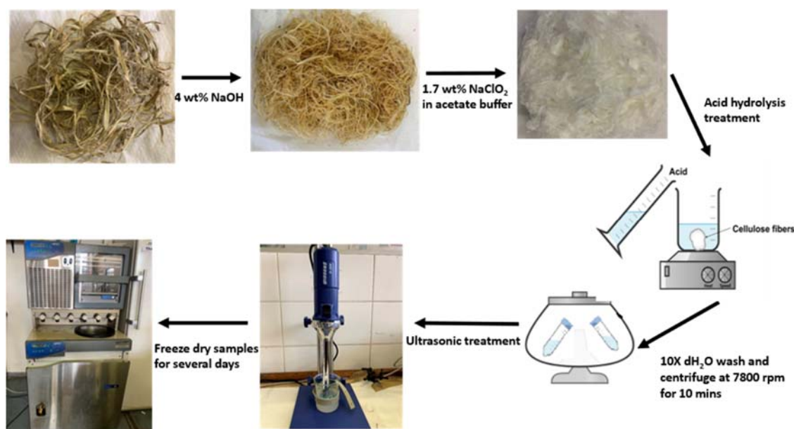
Figure 4.1: Schematic showing extraction and preparation of cellulose microfibrils from hemp bast fibres through acid hydrolysis process coupled with ultrasonic treatment.
