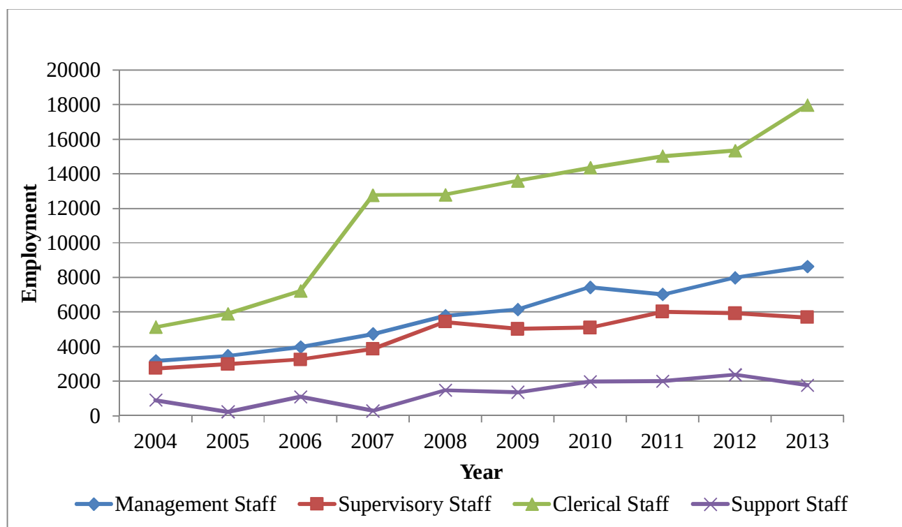
Fig 5.6: Employment in the Banking Sector
