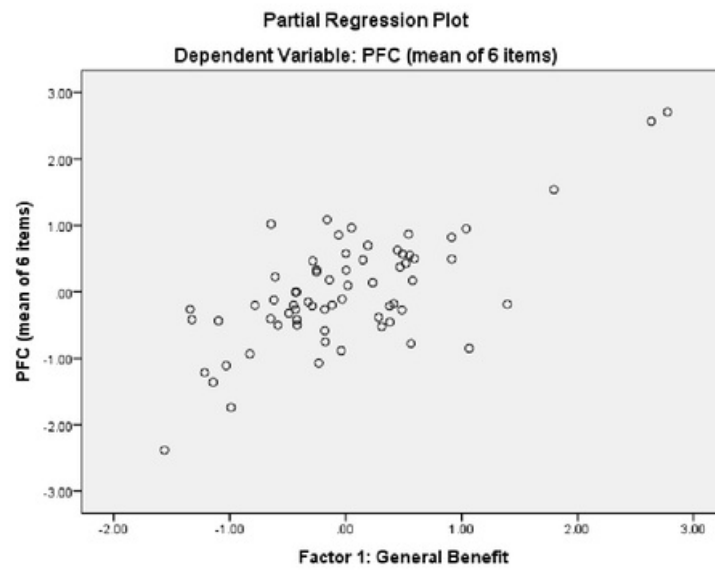
Figure 11: Partial regression plot: F1 General Benefit against PFC
