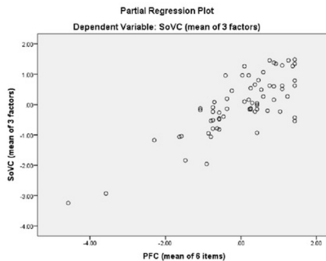
Figure 6: Partial regression plot: PFC and SoVC
