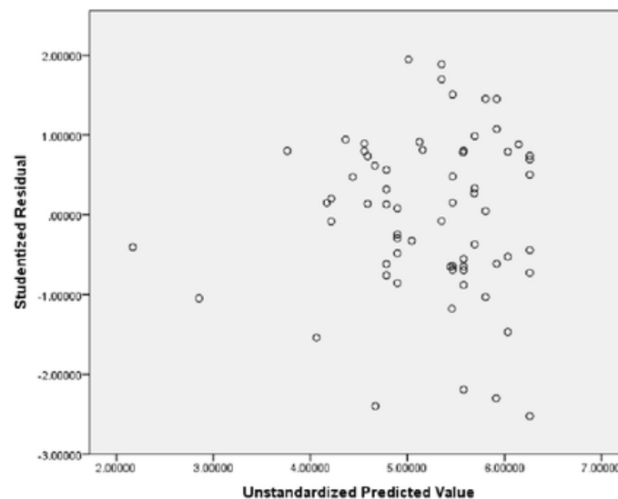
Figure 3: Studentised residuals against unstandardised predicted values (PFC = IV; SoVC = DP)
