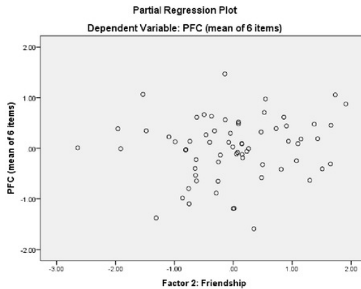
Figure 12: Partial regression plot: F2 Friendship against PFC
