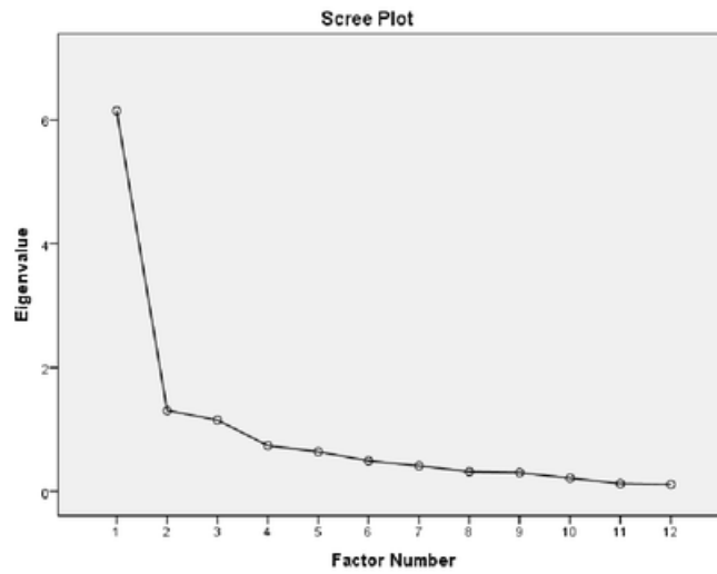
Figure 2: EFA scree plot
