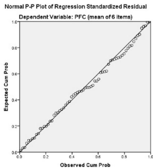
Figure 18: Multiple regression: Normal P-P plot (single IV)
