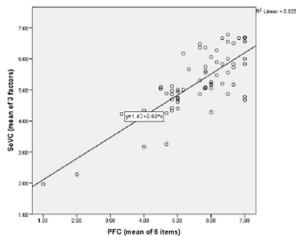
Figure 9: PFC and SoVC plot, with regression line
