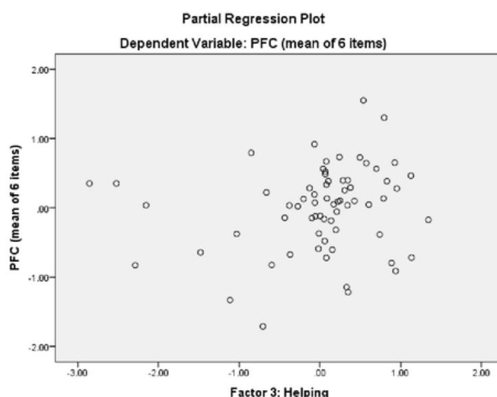
Figure 13: Partial regression plot: F3 Helping against PFC
