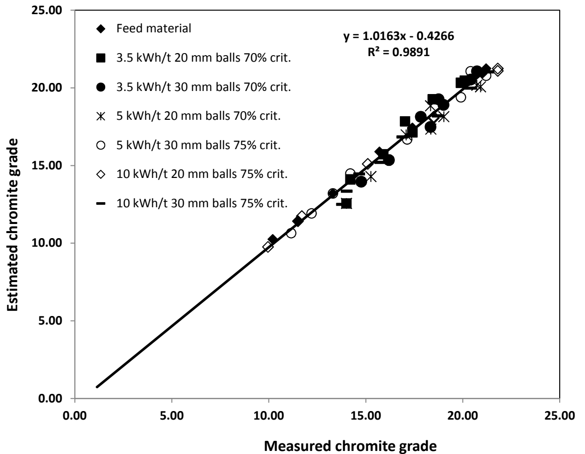
Figure 6.2 Measured chromite grade (abscissa) versus estimated chromite grade (ordinate)
