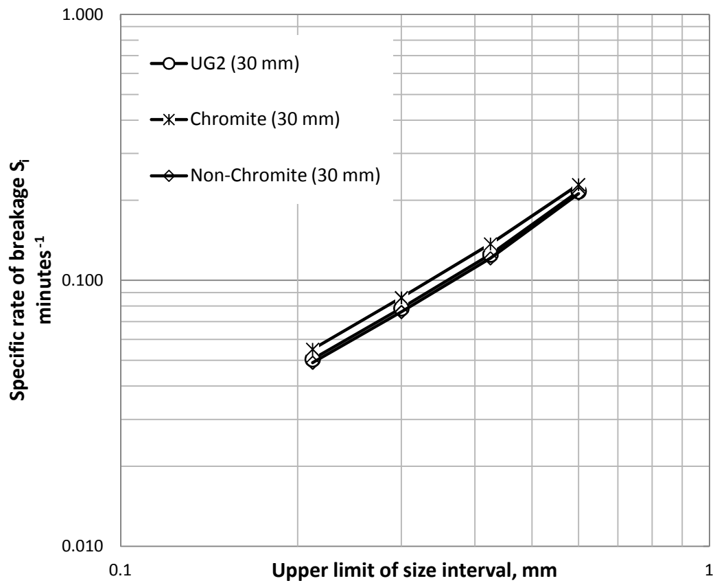
Figure 7.6 Specific rates of breakage of UG2 ore, Chromite Component and Non-Chromite Component as a function of particle size (Ball diameter = 30 mm)
