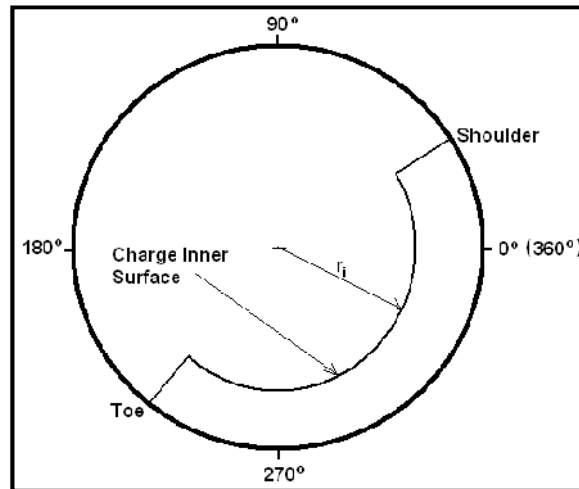
Figure 2.10 Active charge of the mill (after Morrell, 1993)
