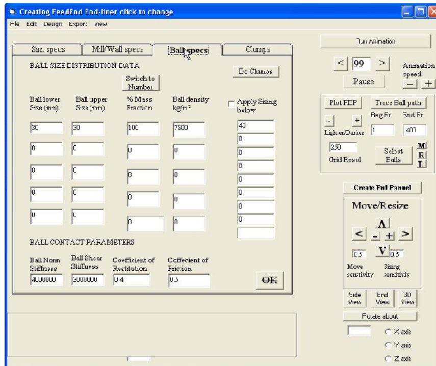
Figure A.1.2 DEM software presentation
