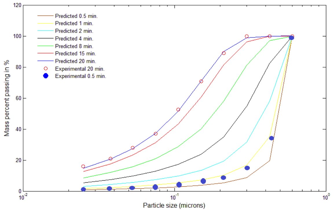
Figure 7.11b Measured and predicted particle size distributions corresponding to 20 mm balls and feed size: - 300 + 212 \mu\text{m}
