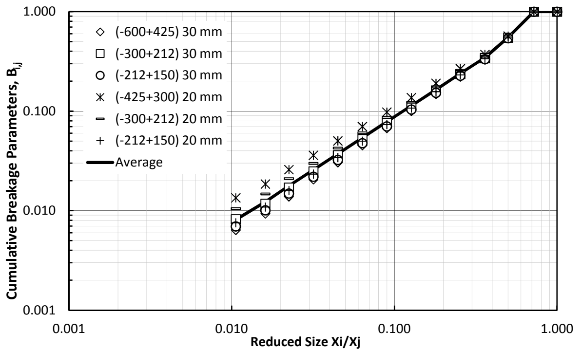
Figure 7.7 Breakage Function Distributions for various sizes of chromite component
