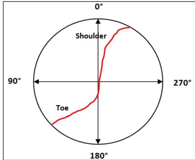
Figure 2.5 Load behaviour in a mill; definition of toe and shoulder position
