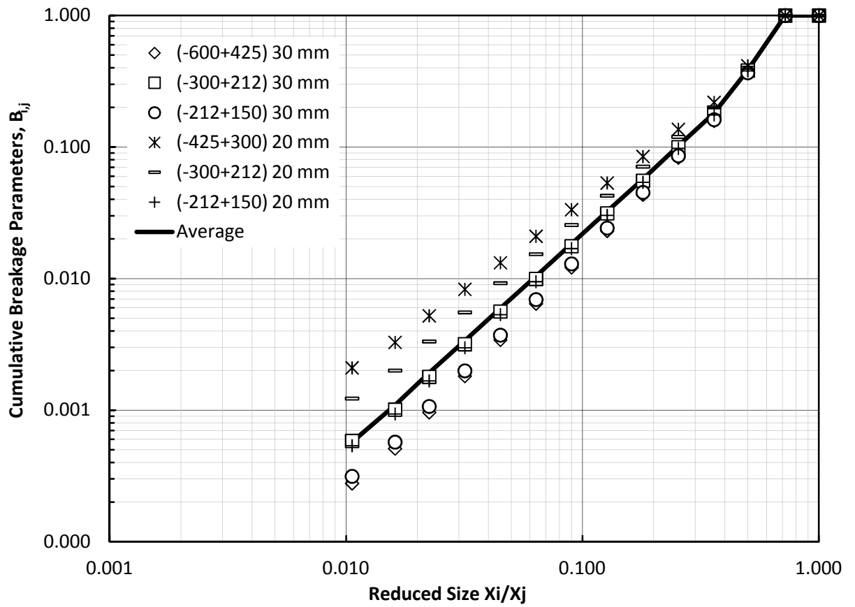
Figure 7.8 Breakage Function Distributions for various sizes of non-chromite component
