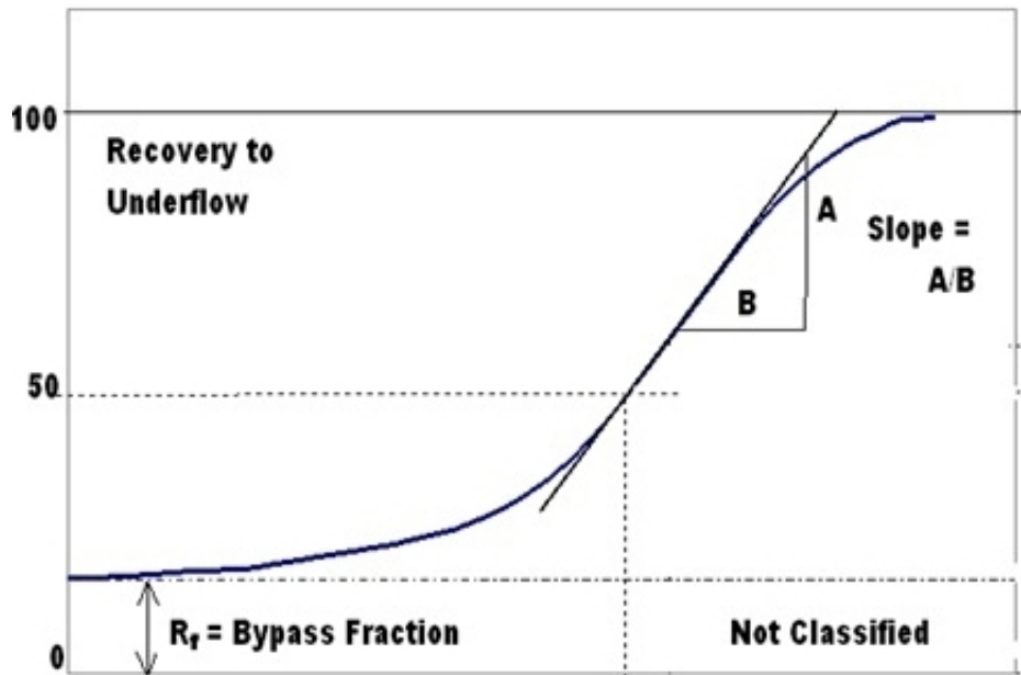
Figure 8.5 Cyclone partition curve (Plitt, 1976)
