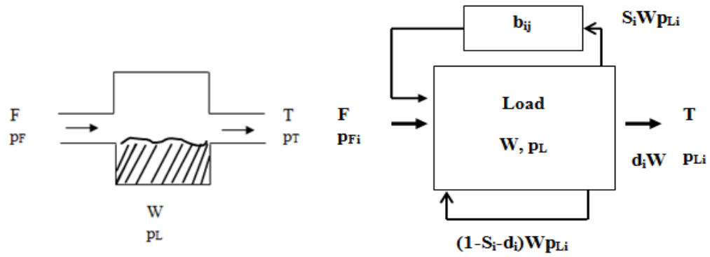
Figure 8.3 Continuous ball milling schematic
