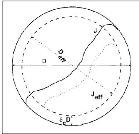
Figure 2.8 Modelling approaches of load behaviour by Moys (1990)
