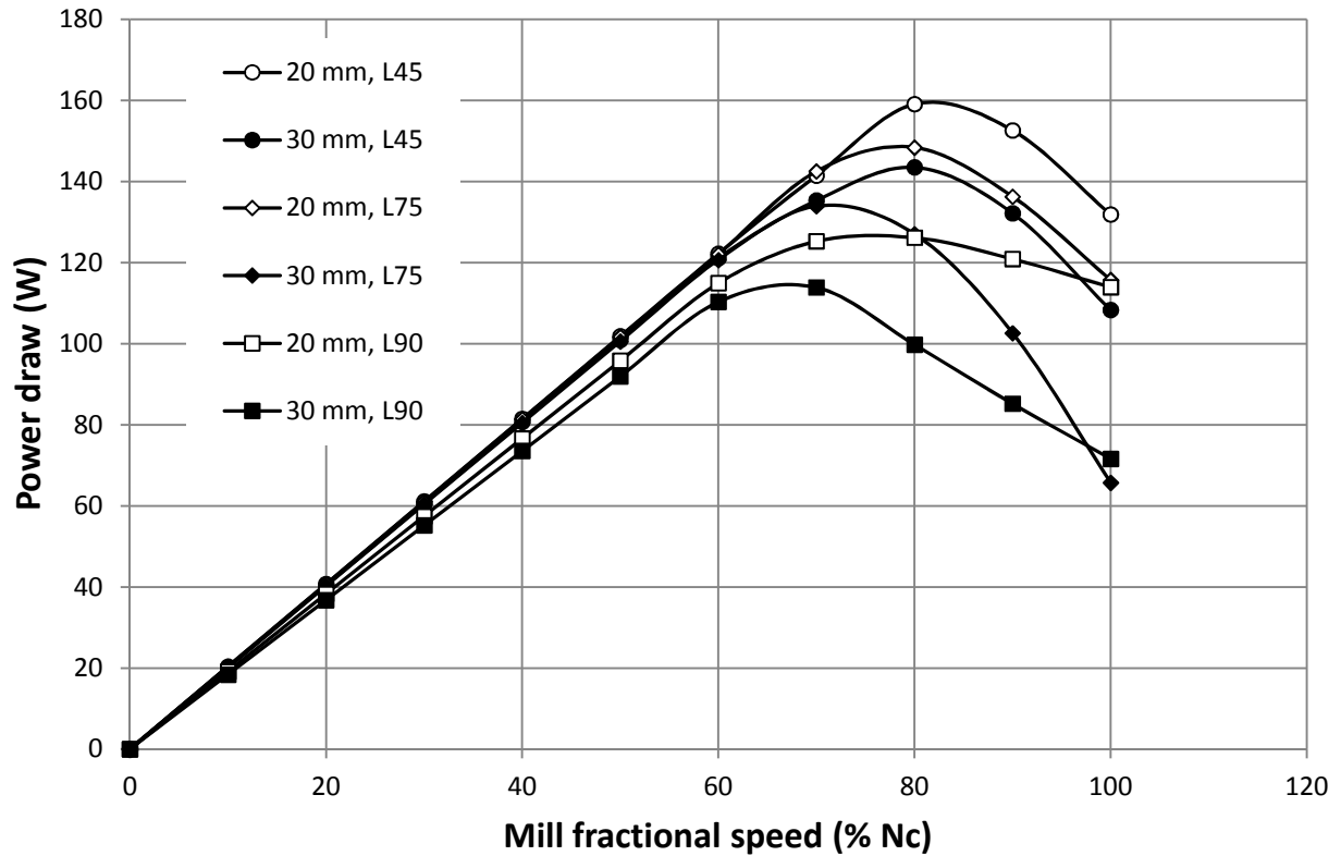
Figure 3.1 DEM simulations power draw prediction
