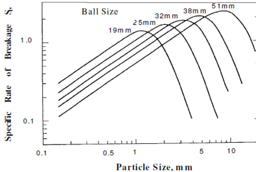
Figure 2.6 Effect of ball size on the rate of breakage of quartz particles in a laboratory ball mill (Austin et al. , 1984)
