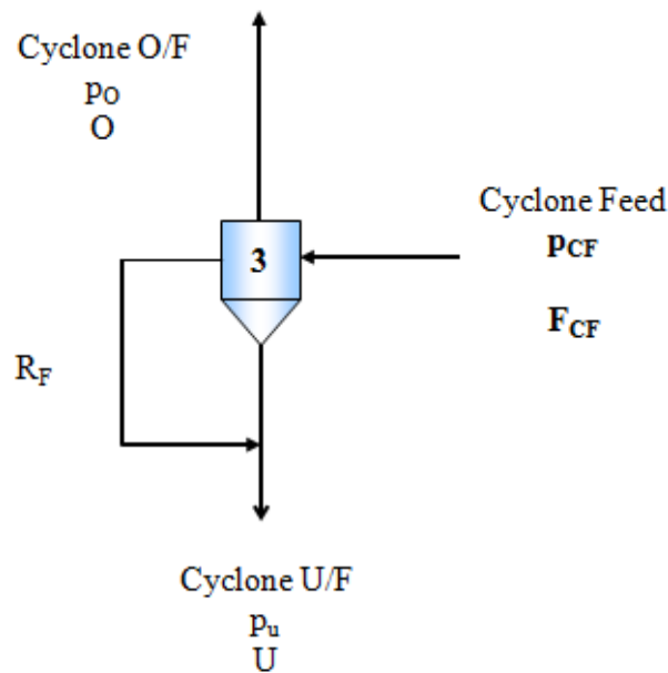
Figure 8.4 Cyclone mass balance
