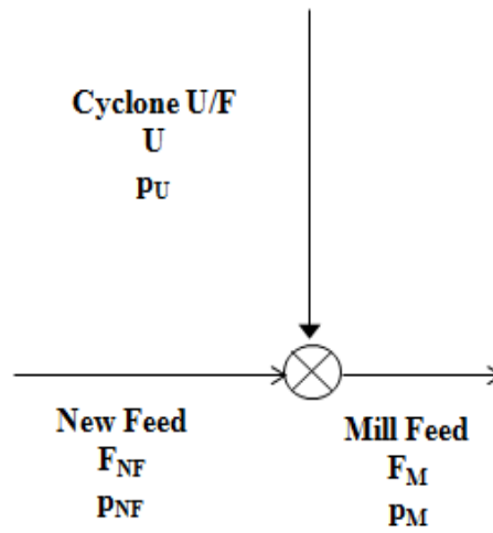
Figure 8.2 Mixing point mass balance
