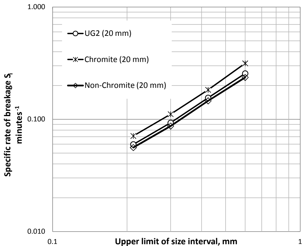
Figure 7.5 Specific rates of breakage of UG2 ore, Chromite Component and Non-Chromite Component as a function of particle size (Ball diameter = 20 mm)
