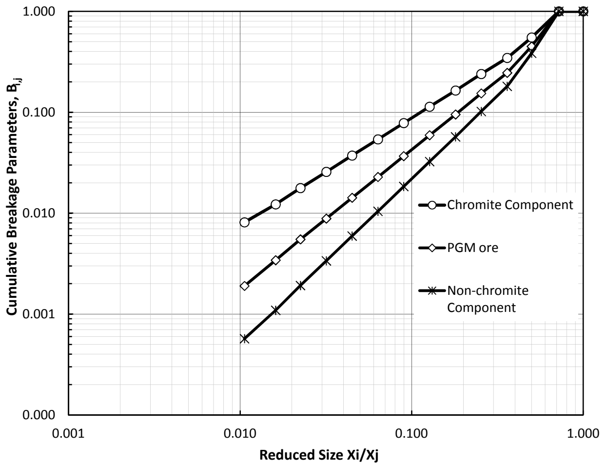
Figure 7.9 Comparison of the Cumulative breakage distribution functions (UG2 ore, Chromite Component and Non-Chromite Component)
