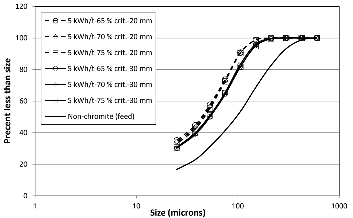
Figure 5.4 Effect of percent critical speed on the non-chromite particle size distributions (20 mm balls: dot lines and 30 mm balls: solid lines)
