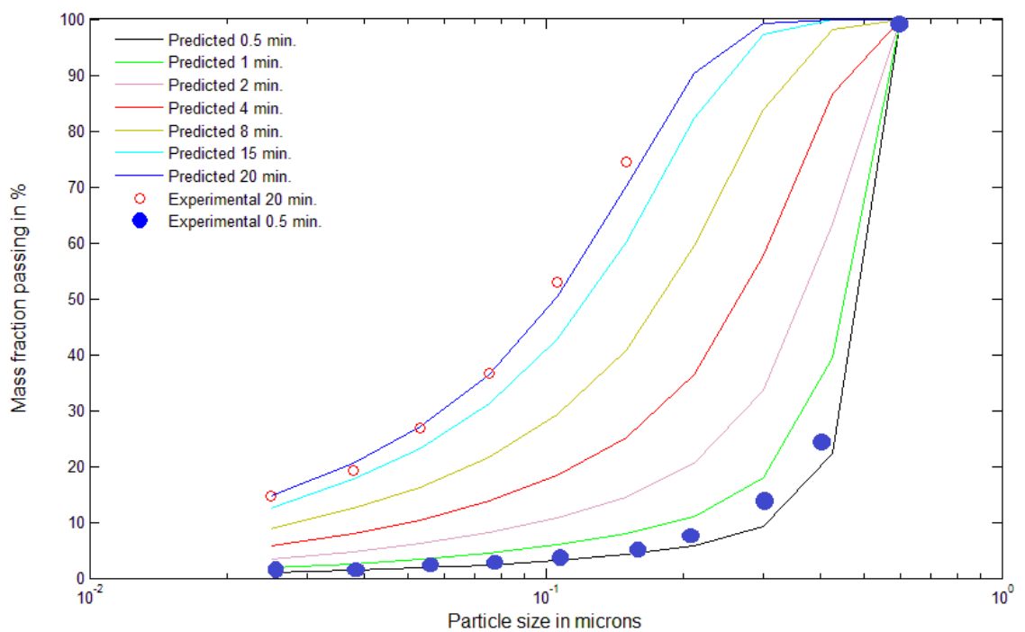
Figure 7.10d Measured and predicted particle size distributions corresponding to 30 mm balls and feed size: - 212 + 150 \mu\text{m}
