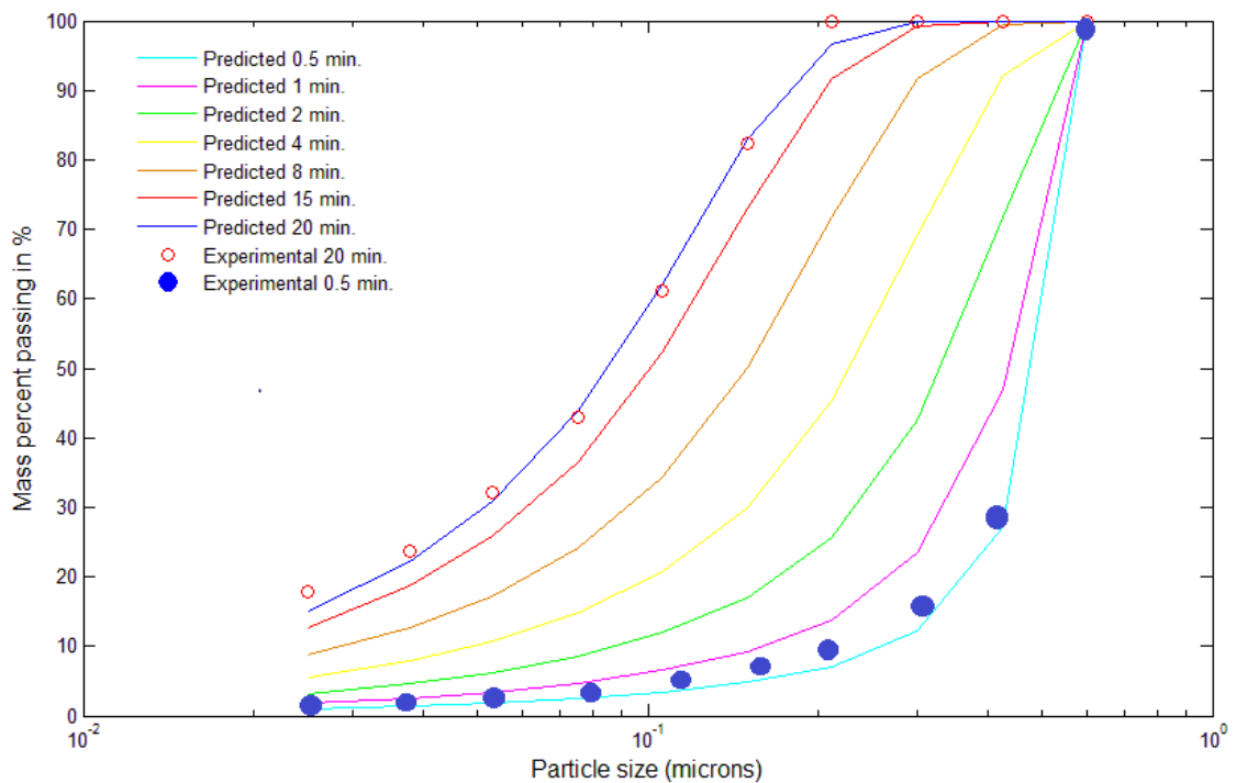
Figure 7.11a Measured and predicted particle size distributions corresponding to 20 mm balls and feed size: -212 + 150 \mu\text{m}
