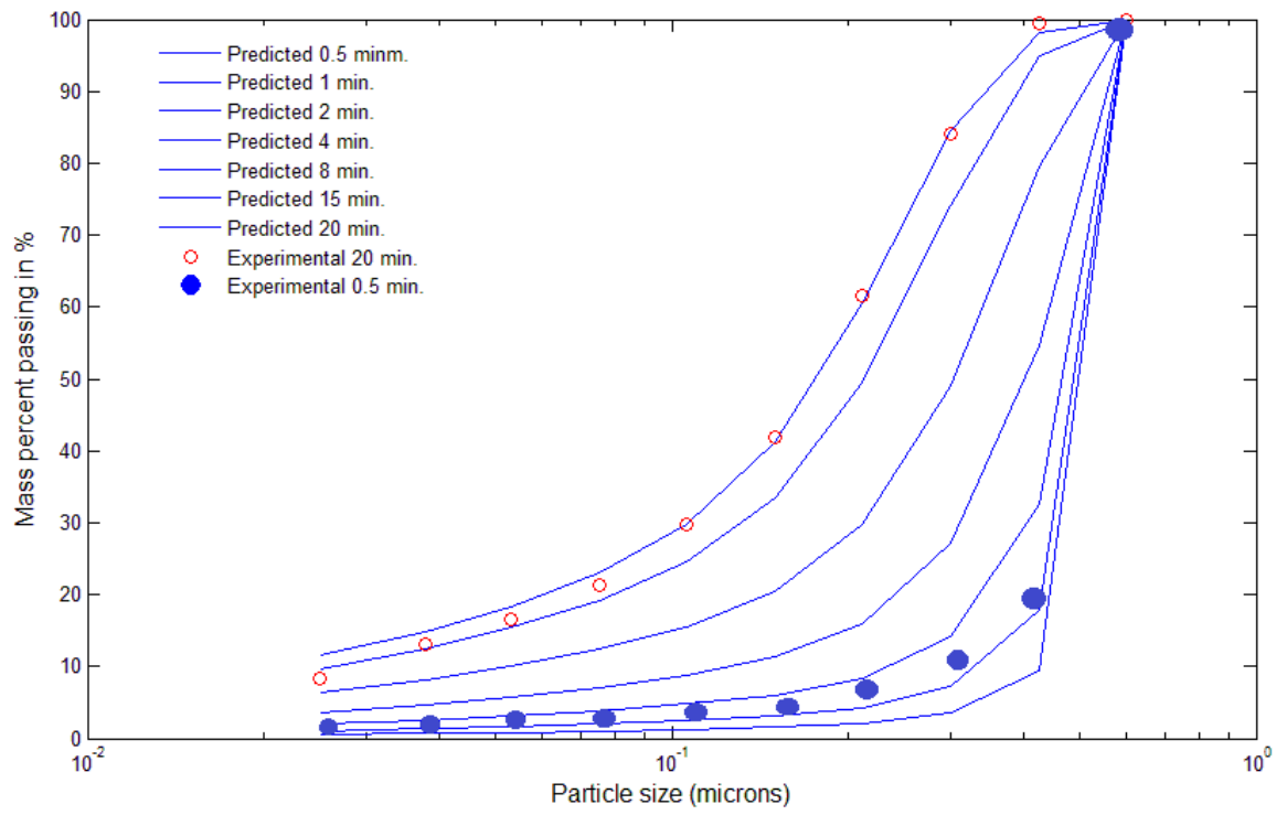
Figure 7.11f Measured and predicted particle size distributions corresponding to 30 mm balls and feed size: - 600 + 425 \mu\text{m}
