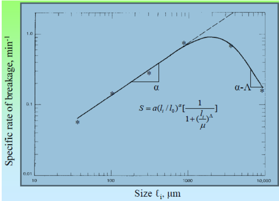
Figure 2.3 Variation of S with particle size and graphical procedure for the determination of the parameters (Austin et al., 1984)
