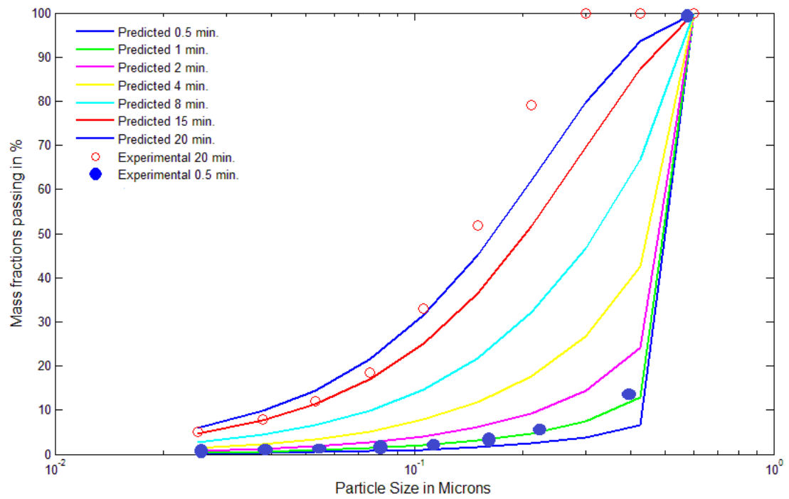
Figure 7.10e Measured and predicted particle size distributions corresponding to 30 mm balls and feed size: - 300 + 212 \mu\text{m}
