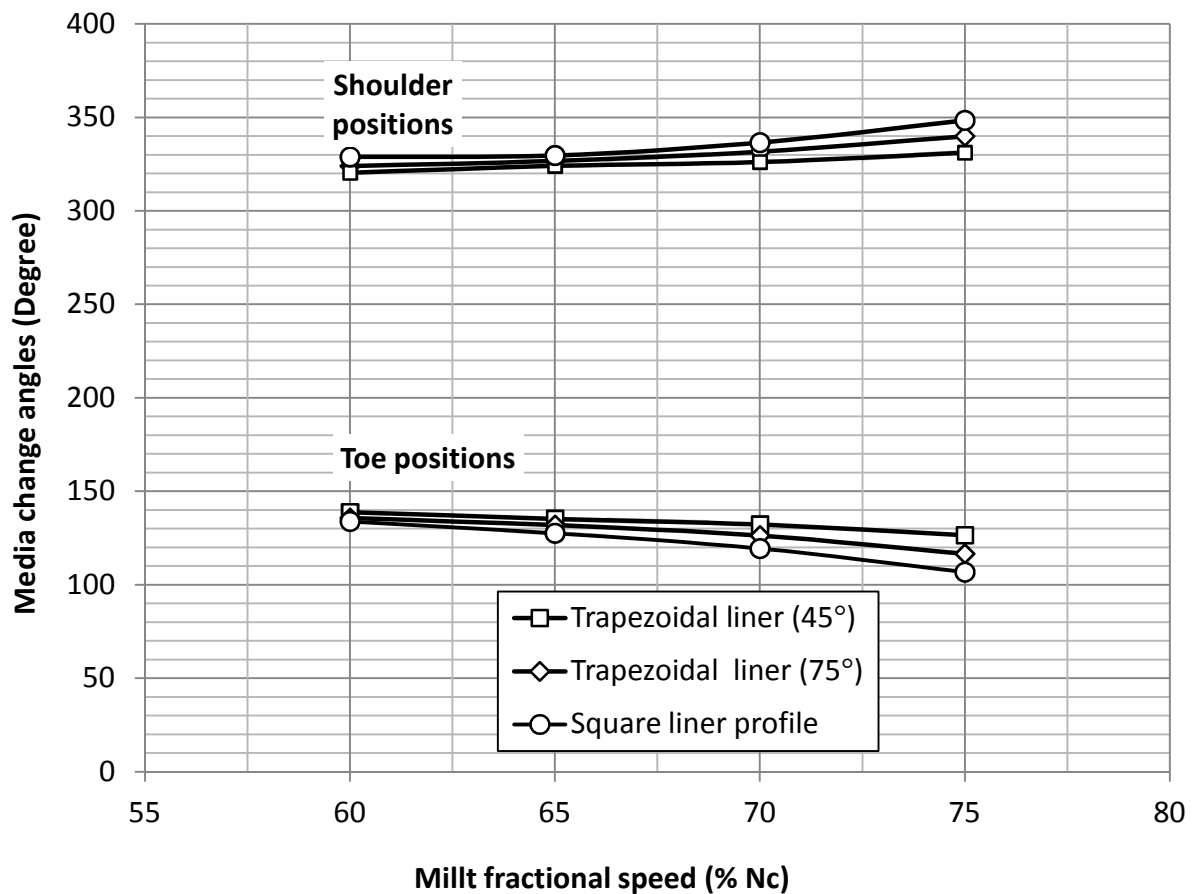
Figure 3.3 Variations of the toe and shoulder positions of the media charge with the percent fractional speed of the mill
