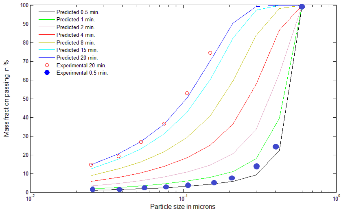
Figure 7.11d Measured and predicted particle size distributions corresponding to 30 mm balls and feed size: -212 + 150 μm
