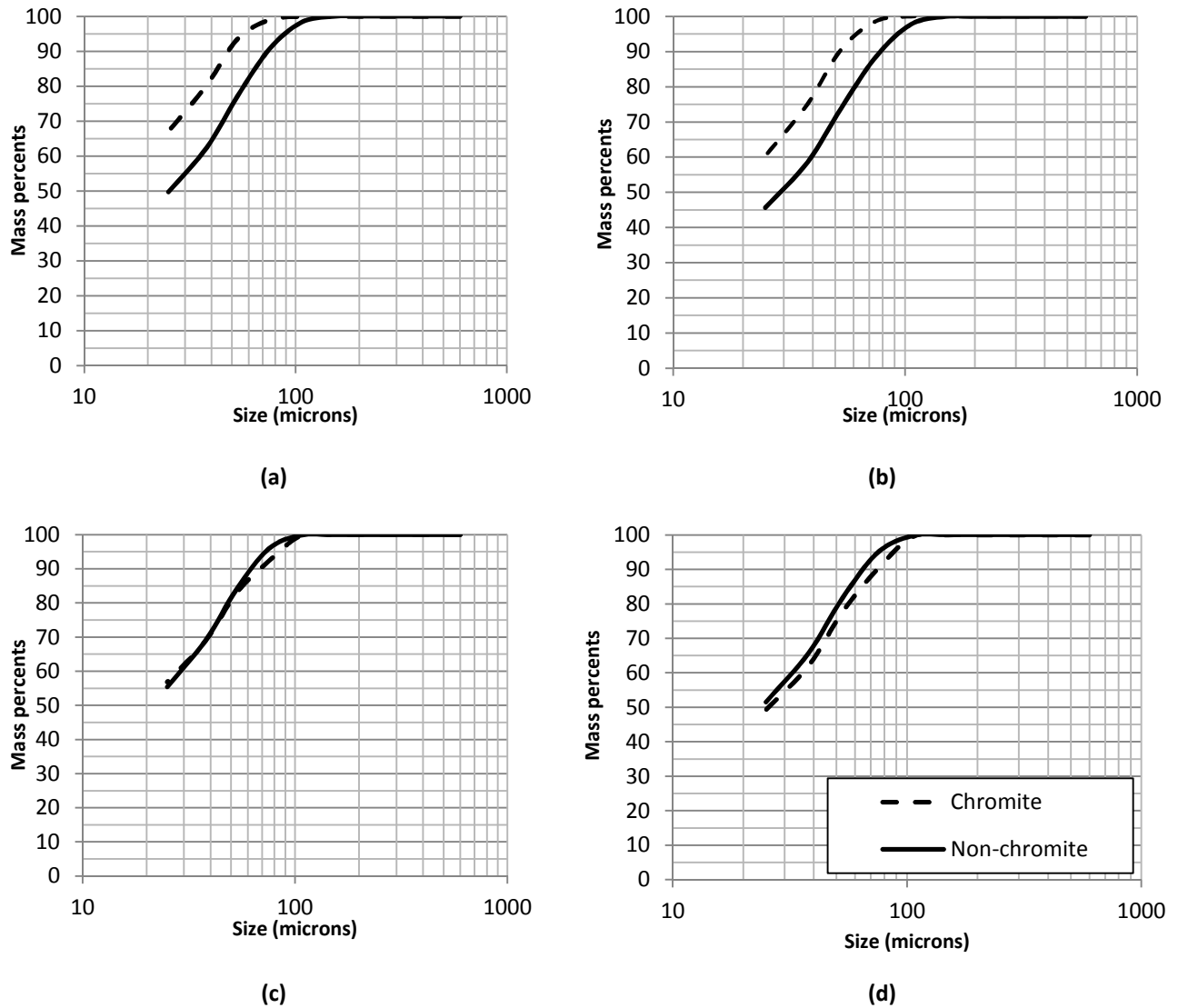
Figure 8.6 Showing chromite and non-chromite particle size distributions in the Cyclone overflow stream for different scenarios
