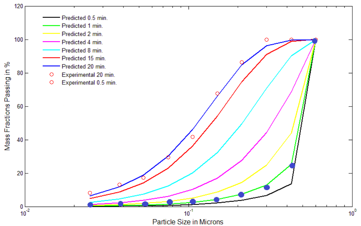
Figure 7.11c Measured and predicted particle size distributions corresponding to 20 mm balls and feed size: - 425 + 300 \mu\text{m}
