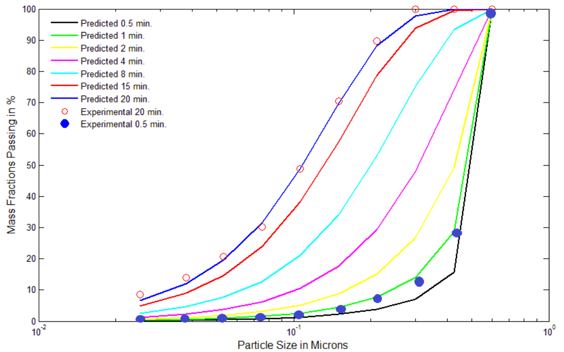
Figure 7.10b Measured and predicted particle size distributions corresponding to 20 mm balls and feed size: -300 + 212 \mu\text{m}
