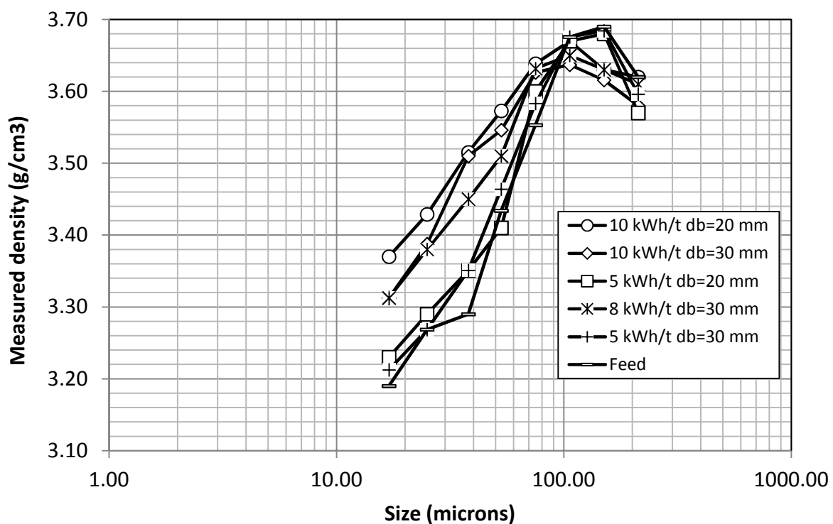
Figure 6.1 Measured density as a function of grain size
