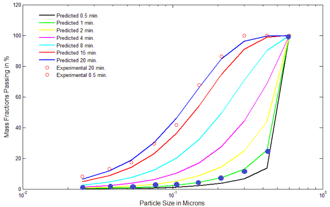
Figure 7.10c Measured and predicted particle size distributions corresponding to 20 mm balls and feed size: - 425 + 300 \mu\text{m}
