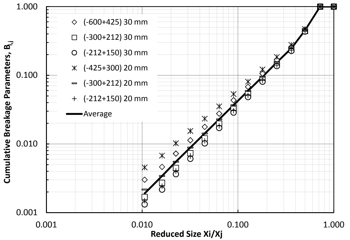
Figure 7.6 Breakage Function Distributions for various sizes of UG2 ore
