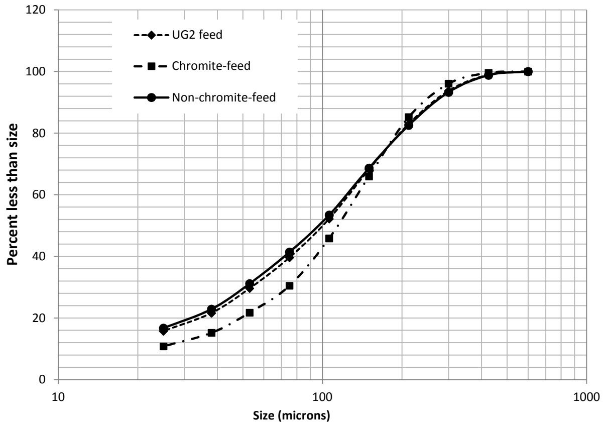
Figure 4.2 Particle Size Distribution of UG2 ore, chromite and non-chromite
