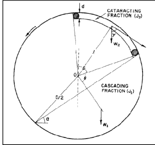
Figure 2.9 Modelling approaches of load behaviour by Fuerstenau et al. (1990)
