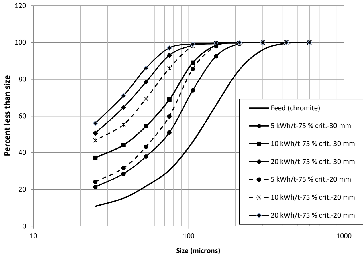
Figure 5.3 Effect of ball size and specific energy consumption on the chromite particle size distributions
