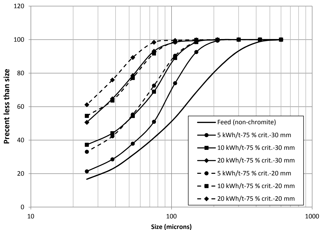
Figure 5.2 Effect of ball size and specific energy consumption on the non-chromite particle size distributions
