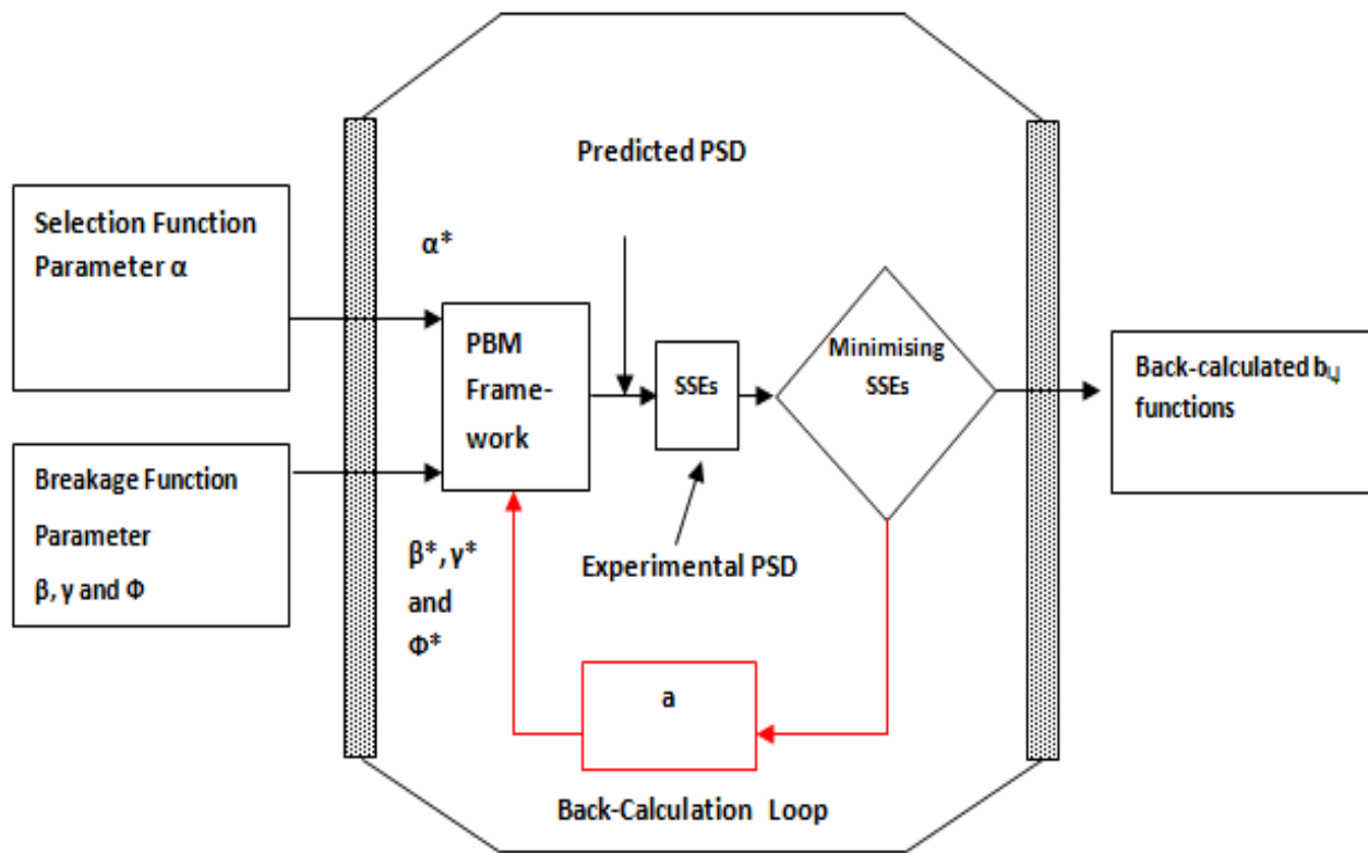
Figure 7.1 Schematic representation of the simulator used
