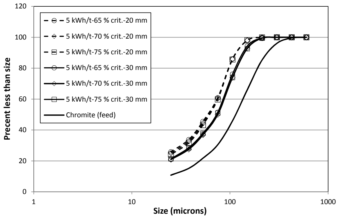
Figure 5.5 Effect of percent critical speed on the chromite particle size distributions (20 mm balls: dot lines and 30 mm balls: solid lines)
