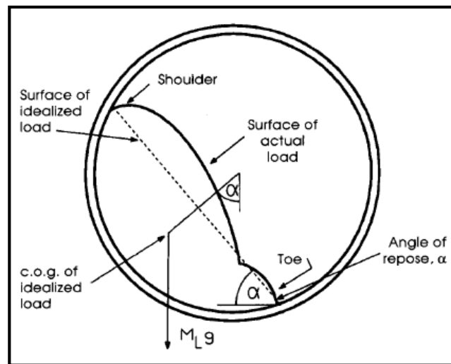
Figure 2.7 Rationale behind the torque-arm approach (Moys, 1993)
