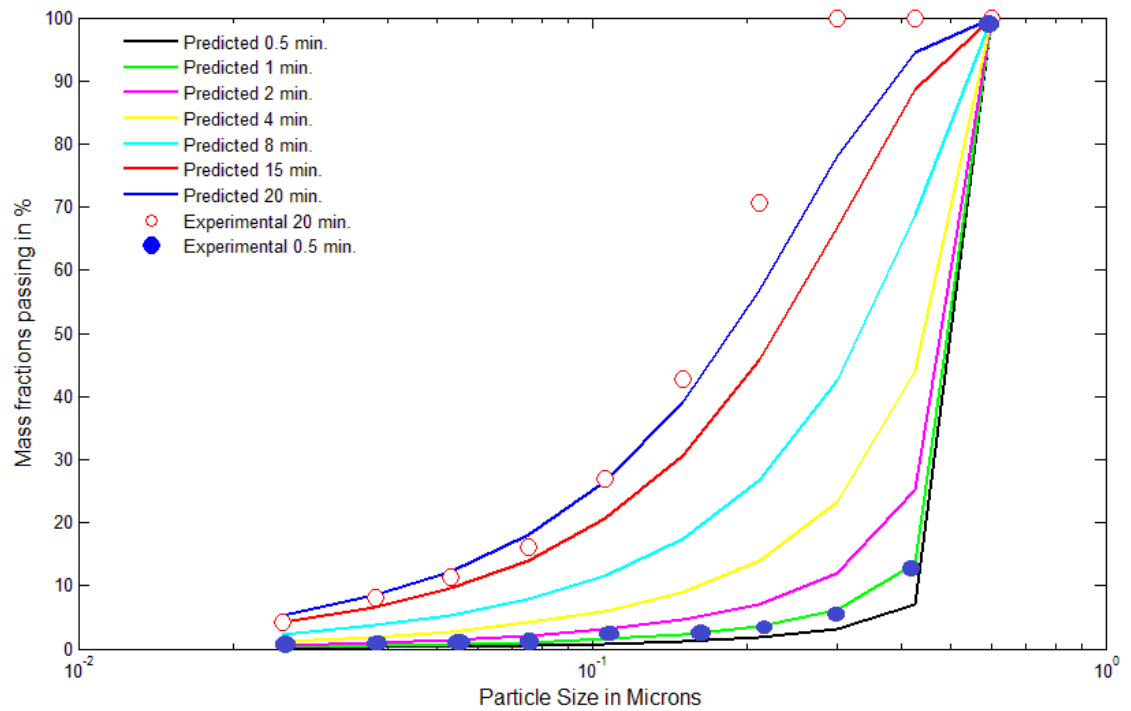
Figure 7.10f Measured and predicted particle size distributions corresponding to 30 mm balls and feed size: - 600 + 425 \mu\text{m}
