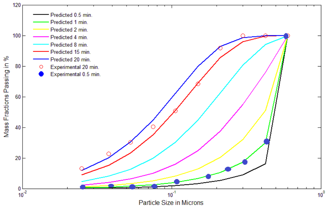
Figure 7.10a Measured and predicted particle size distributions corresponding to 20 mm balls and feed size: -212 + 150 \mu\text{m}
