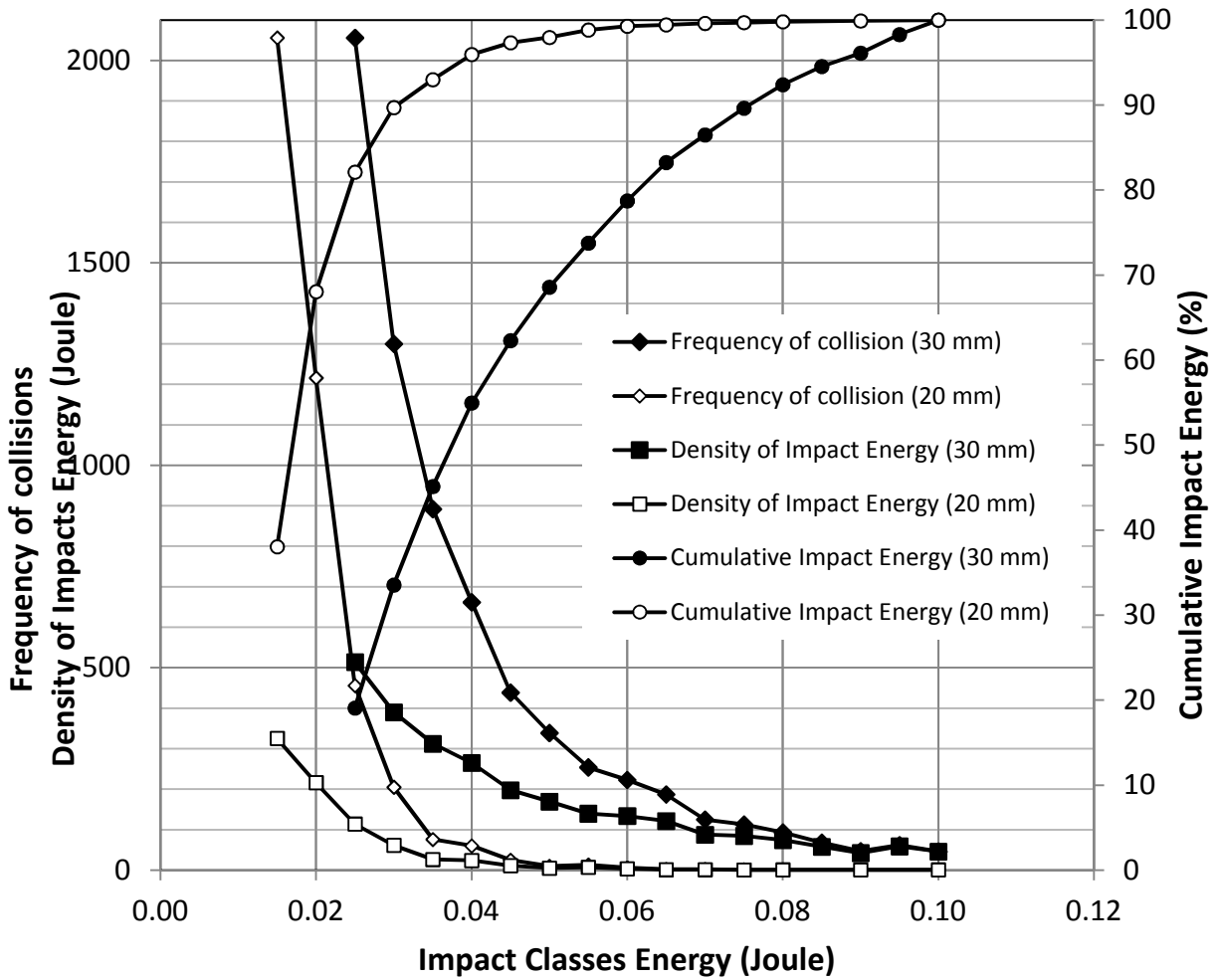
Figure 3.4 Impact energy spectra as a function of ball size
