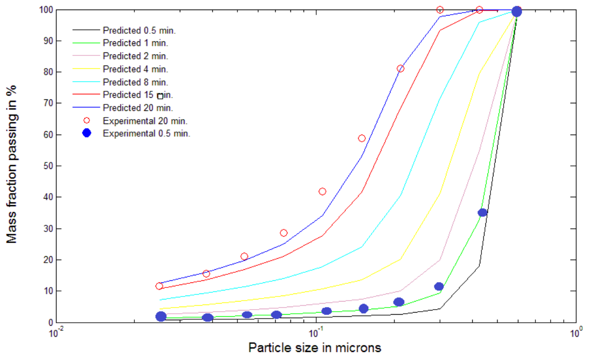
Figure 7.11e Measured and predicted particle size distributions corresponding to 30 mm balls and feed size: -300 + 212 μm
