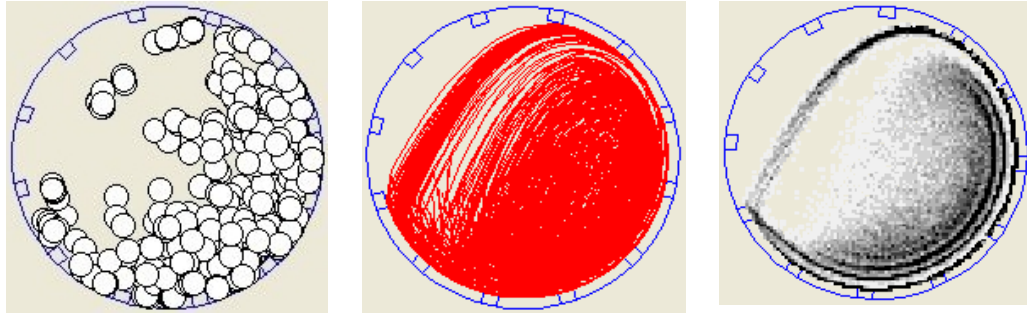
Figure A.1.4 DEM frames, particle paths for consecutive frames, position density plots (PDP) (ball diameter = 30mm)
