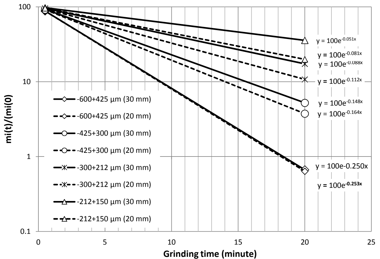
Figure 7.2 First-order plots for various feed sizes of UG2 ore ground in a laboratory-scale ball mill
