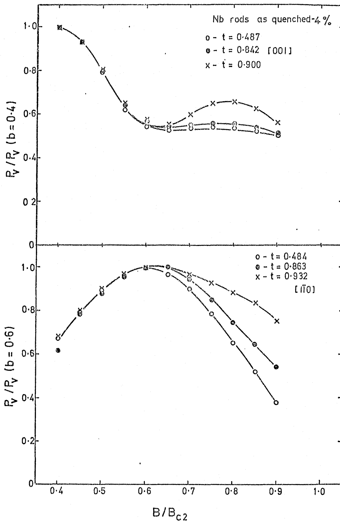
Figure 5.24a. The variation of the bulk pinning force density, normalized at b = 0.4 , with the reduced induction b for the [001] 4% deformed specimen, as-quenched and aged for 20 hours at 90K, showing class (i) behaviour and the anomaly at b = 0.8 .
