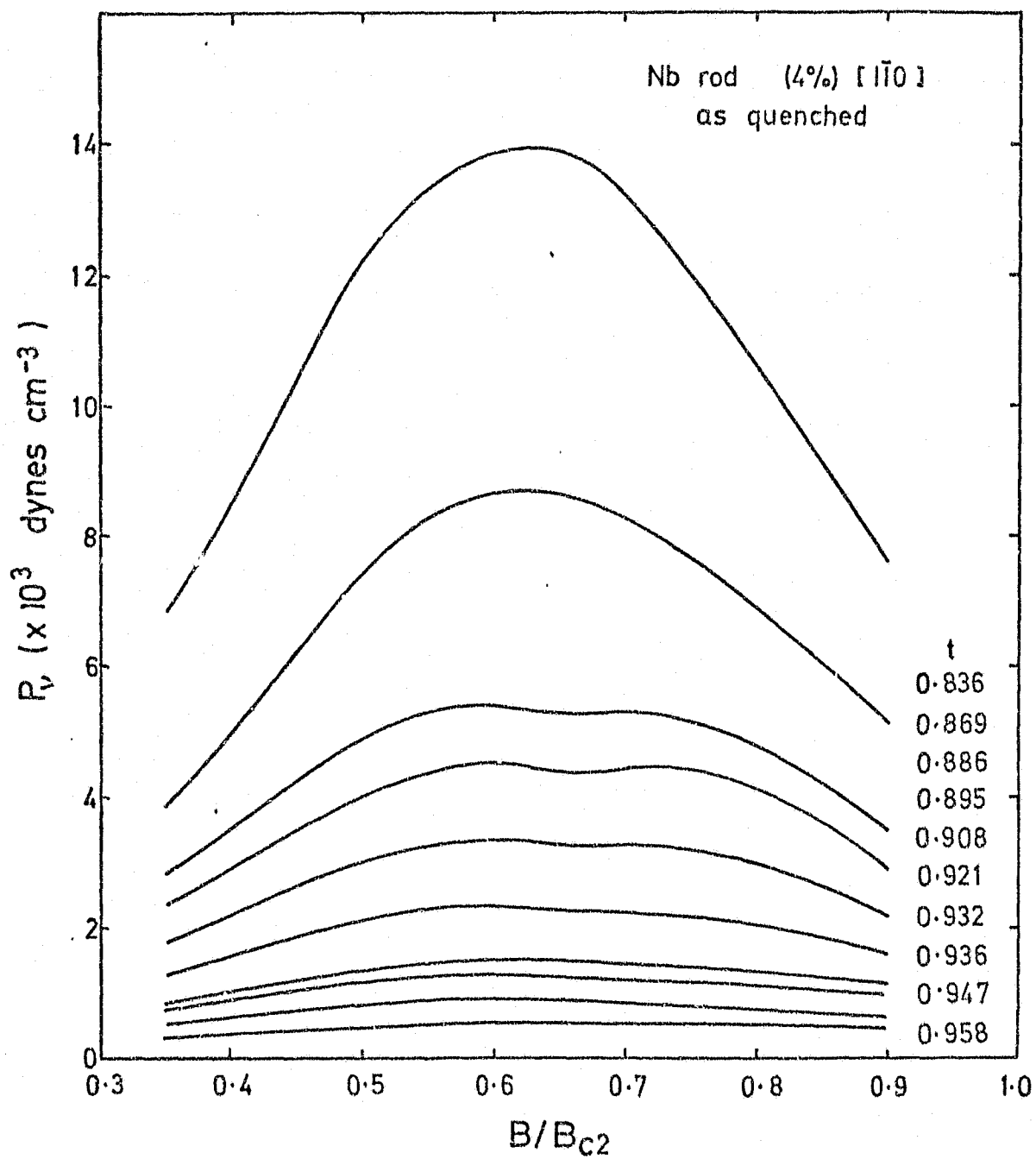
Figure 5.13b. The derived variation of the bulk pinning force density with reduced induction for the as-quenched [1\bar{1}0] 4% deformed rod specimen at various reduced temperatures.
