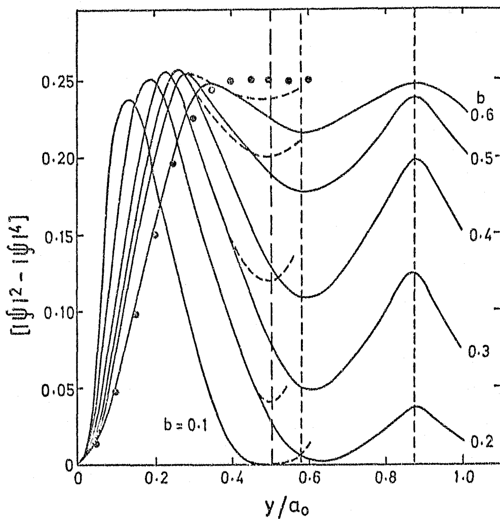
Figure 3.3. The variation of |\psi|^2 - |\psi|^4 versus the reduced distance along the y axis of figure 3.2 for various values of the reduced induction b=B/B_{c2} (full curves). The points have been obtained from equations 3.8 and 3.9 with b=0.6 . The dashed curves show the variation along the x axis.
