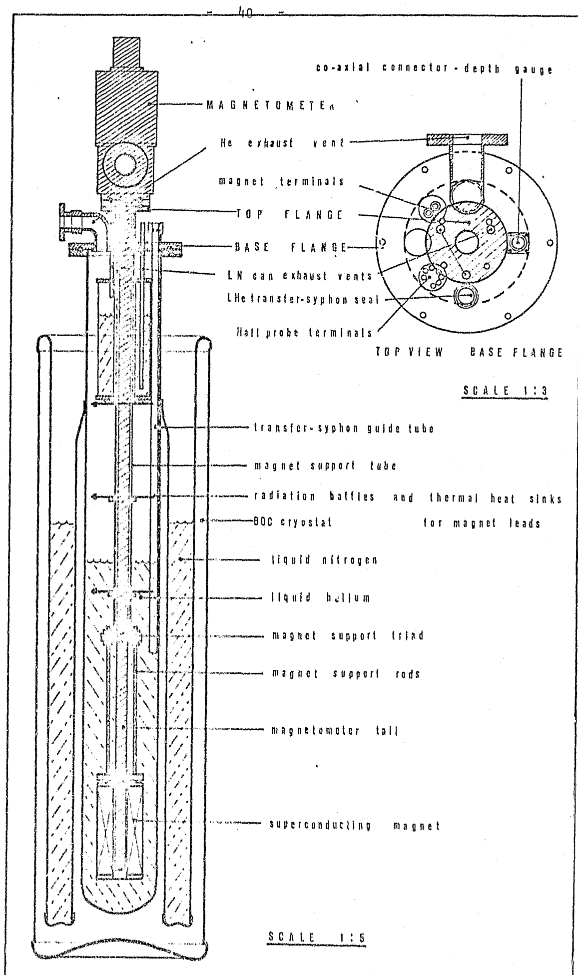
Figure 2.9. The magnetometer cryostat assembly showing the magnetometer, superconducting magnet and magnet support system.
