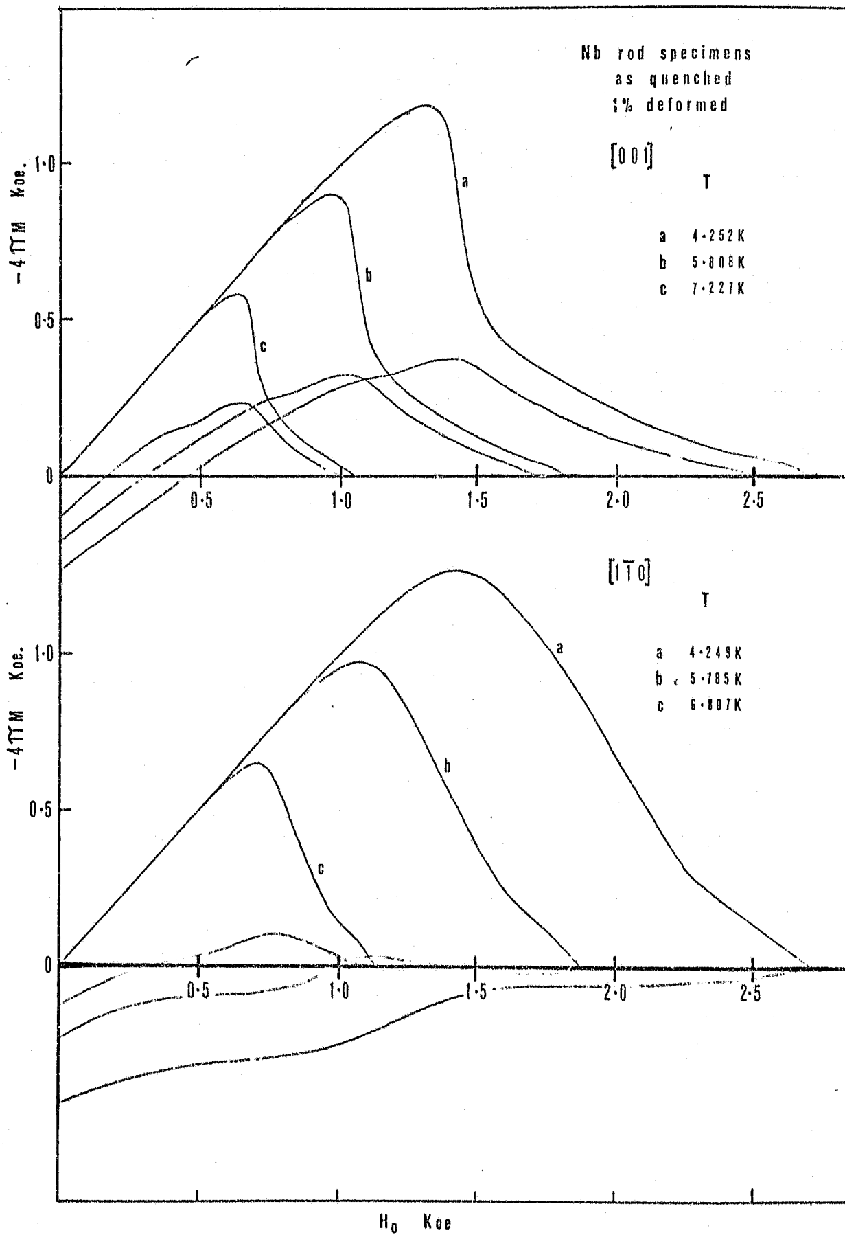
Figure 5.3b. Magnetization curves for the [1\bar{1}0] and [001] 1 per cent (nominal) deformed rod specimens.
