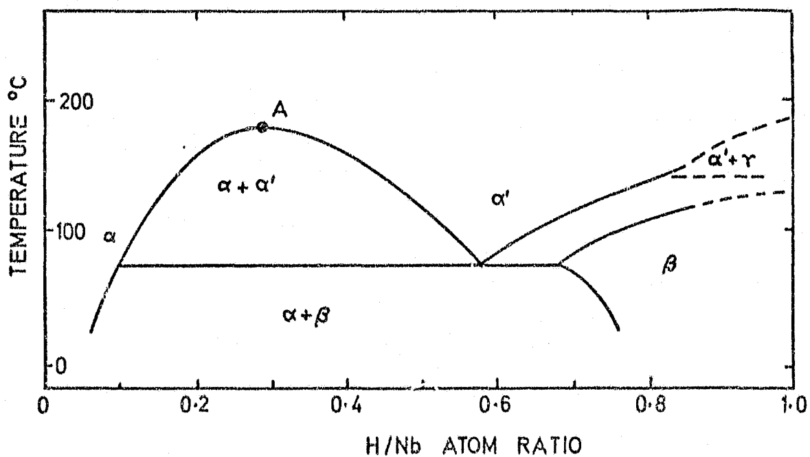
Figure 4.1a. Niobium-hydrogen phase diagram (from Walter and Chandler, 1965).
