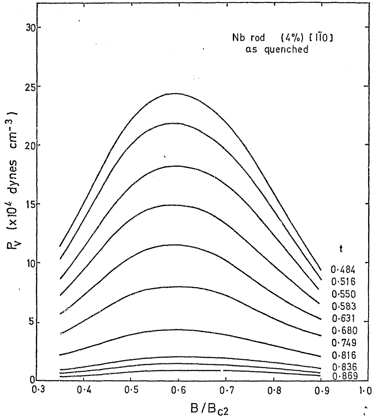
Figure 5.13a The derived variation of the bulk pinning force density with reduced induction for the as-quenched [110] 4% deformed rod specimen at various reduced temperatures.
