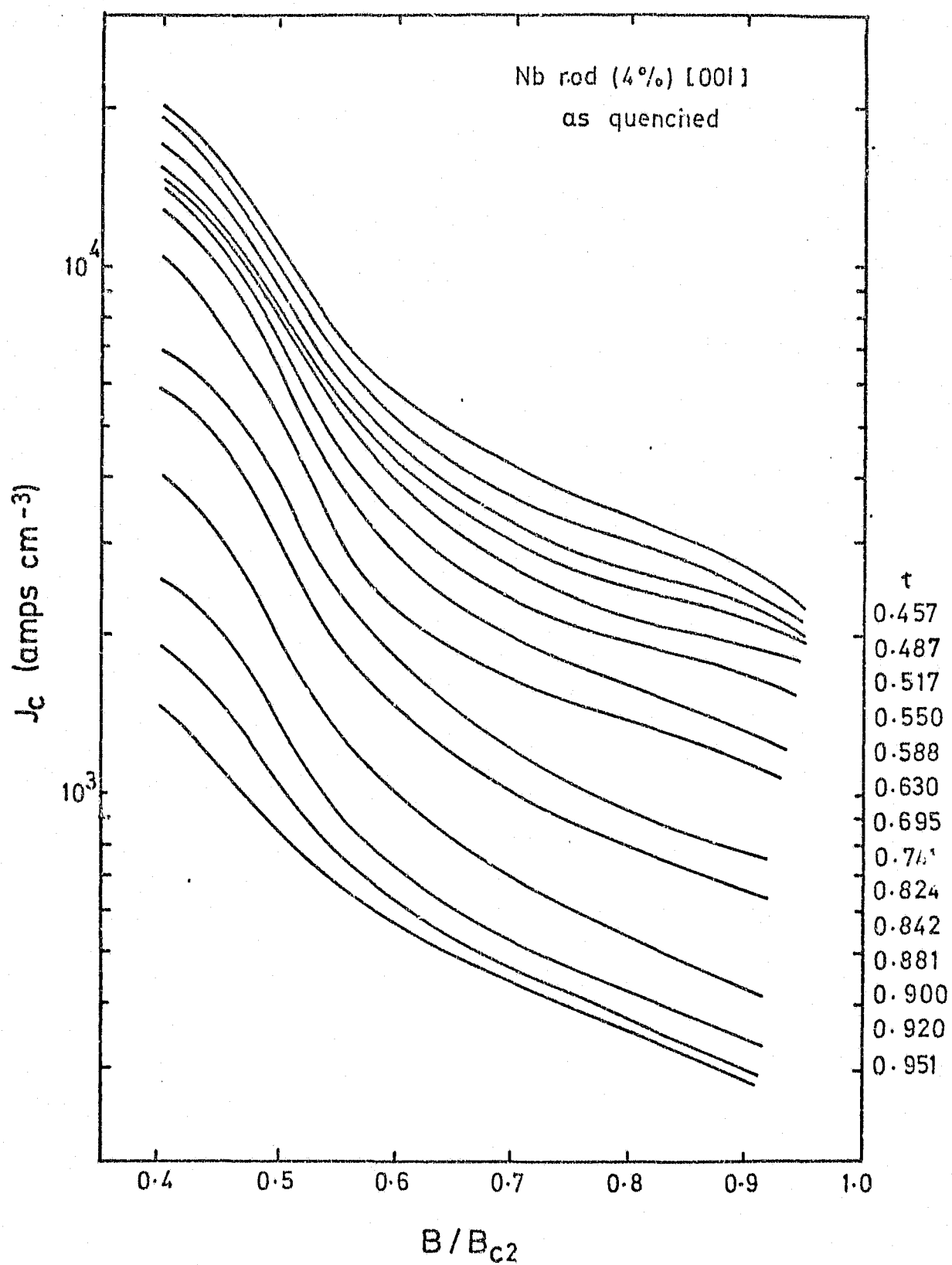
Figure 5.10. As for figure 5.7 for the as-quenched [001] 4% deformed rod specimen.
