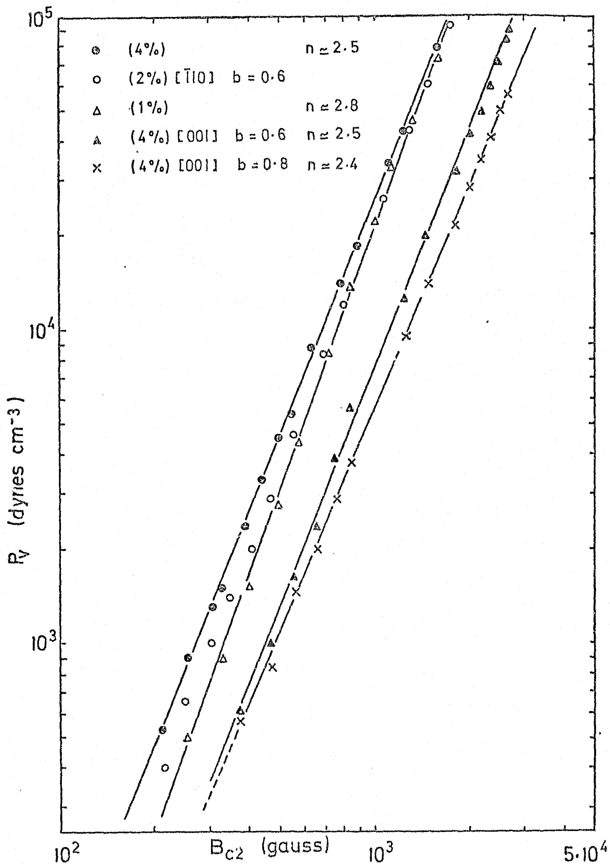
Figure 5.26. log-log plots of the bulk pinning force density at b \approx 0.6 versus the upper critical field (induction for various specimens and also at b \approx 0.8 for the [001] 4% deformed specimen. From these plots the temperature dependences of the bulk pinning force density have been obtained approximately in terms of an exponent n , i.e. P_v(t) \propto B_{c2}^n(t) , which is given in the figure for the various plots.
