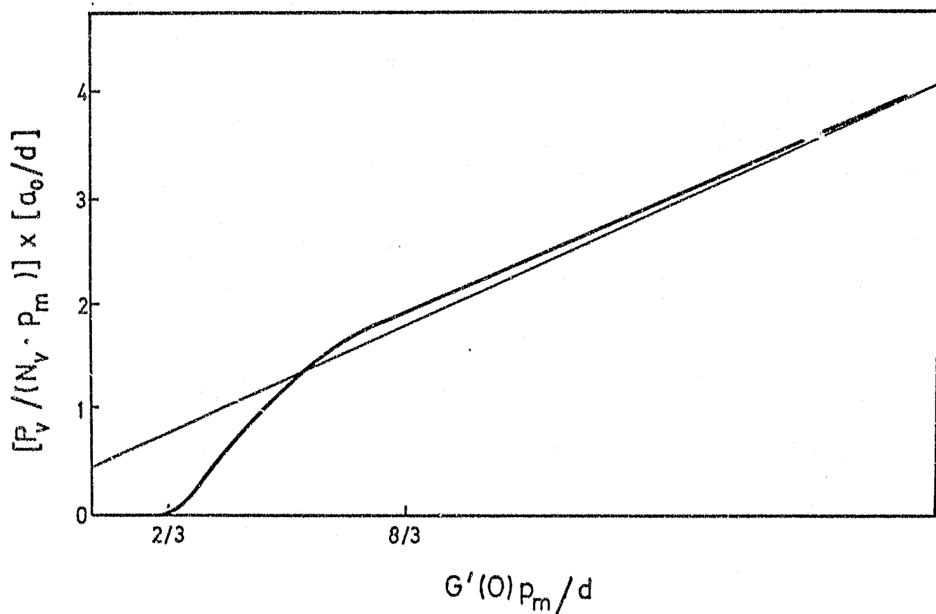
Figure 3.8. The variation in the reduced bulk pinning force density, due to an elementary pinning site, as a function of the reduced displacement of a fluxon. For small displacements, i.e. small p_m or d the pinning sites become ineffective and the bulk pinning force density falls to zero. (From Labusch, 1969b).
