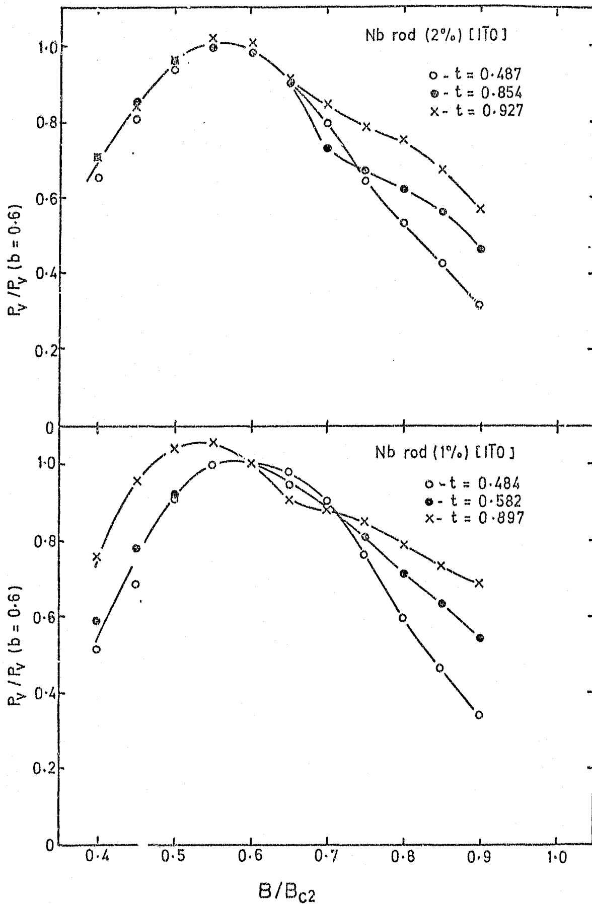
Figure 5.25a and 5.25b. As for figures 5.24b and for [1\bar{1}0] 2% and 1% deformed specimens respectively.
