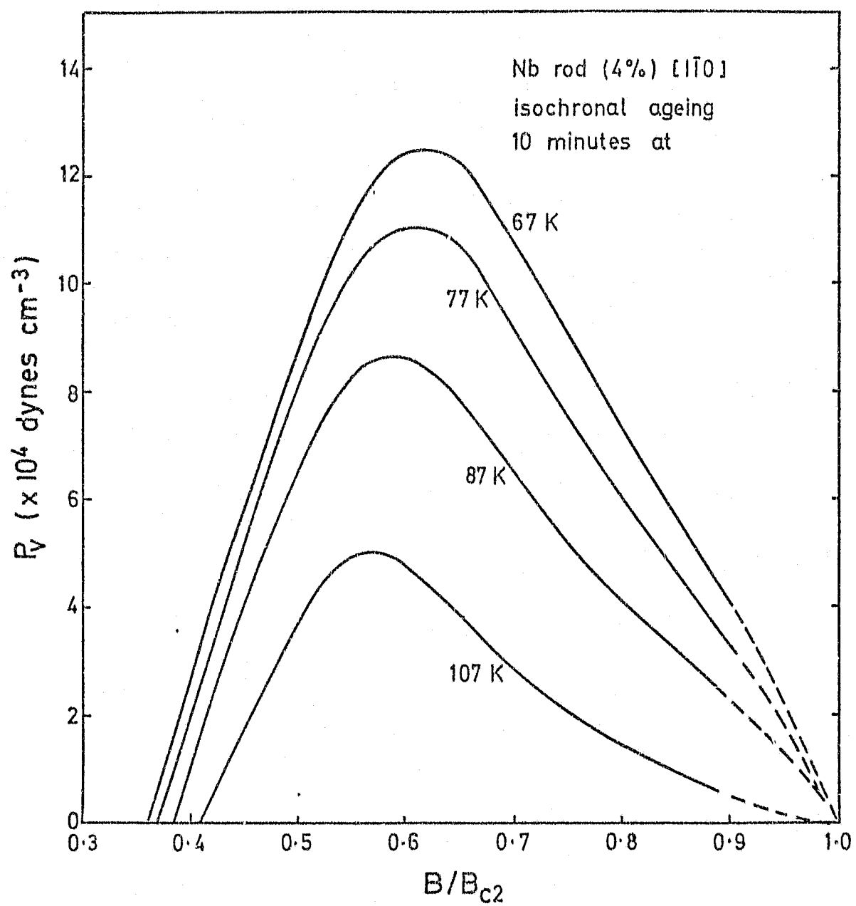
Figure 5.27. The variation of the bulk pinning force density at T = 4.05\text{K} with the reduced induction in class II (see text) after isochronal ageing at various ageing temperatures.
