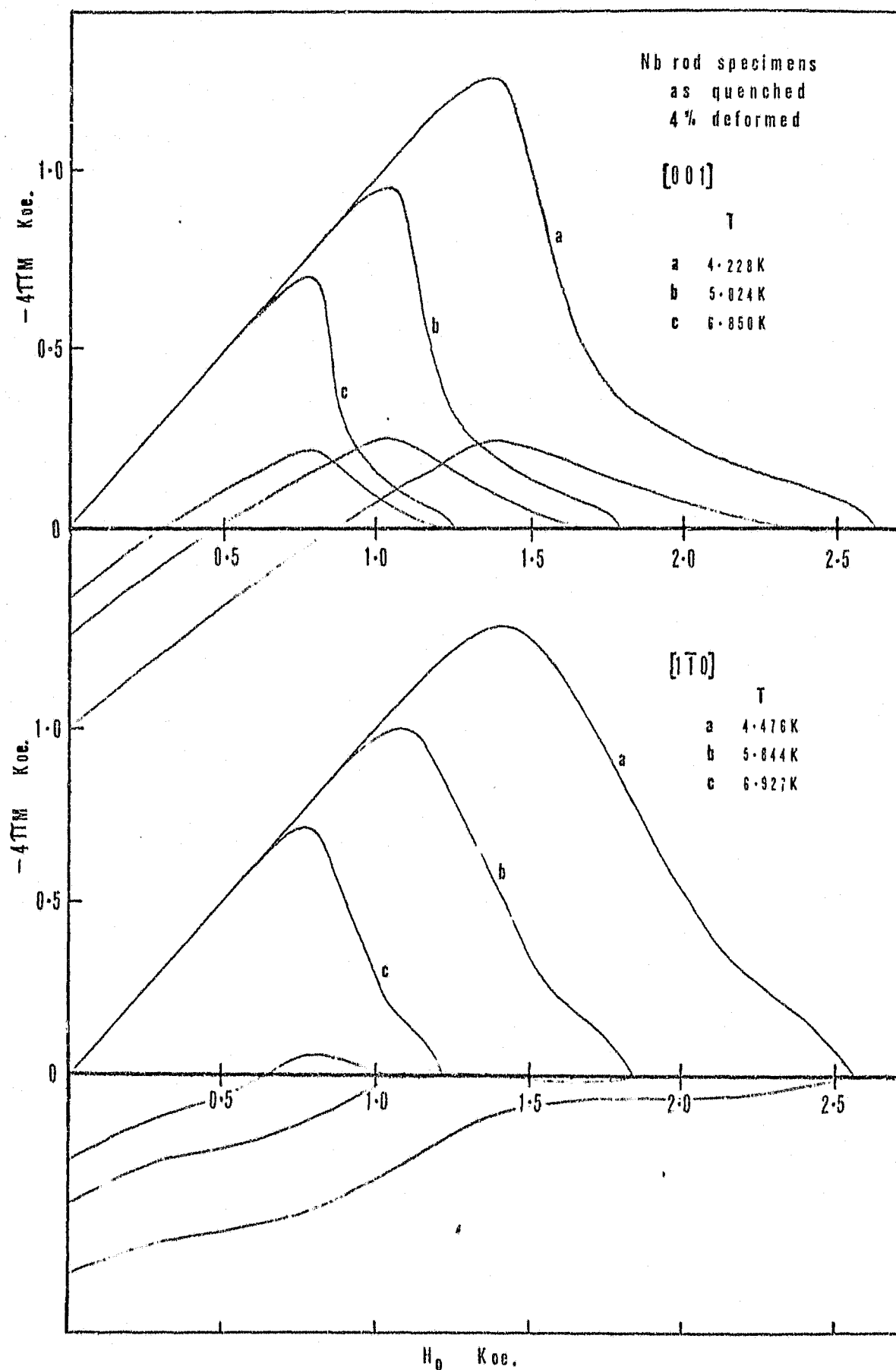
Figure 5.3d. Magnetization curves for the [1\bar{1}0] and [001] 4 per cent (nominal) deformed rod specimens.
