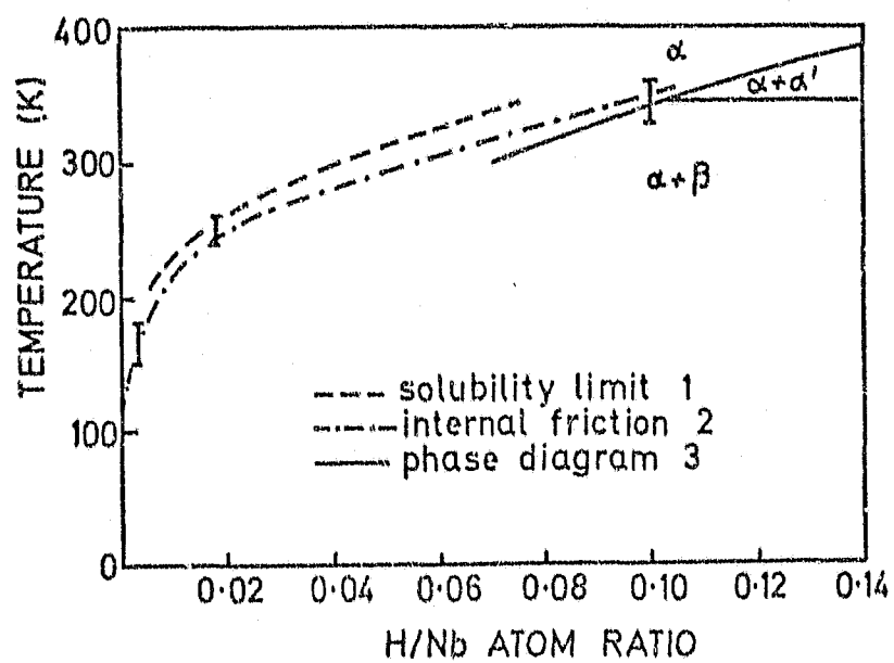
Figure 4.1b. The boundary between the \alpha and \alpha + \beta phases as obtained by various methods. (From Buck, Thompson and Wert, 1971.)
