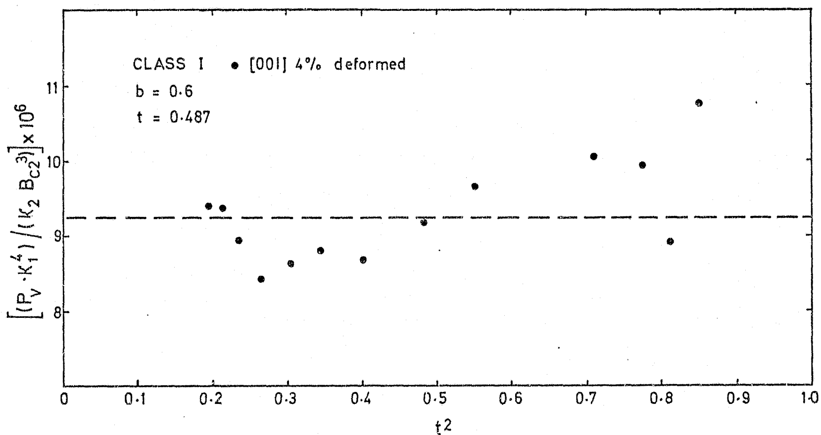
Figure 5.30. A plot of the temperature invariant component of the bulk pinning force density (in accordance with the model for class I), against t^2 showing a maximum relative deviation from theory of approximately 10% (except near t^2 = 1 ).
