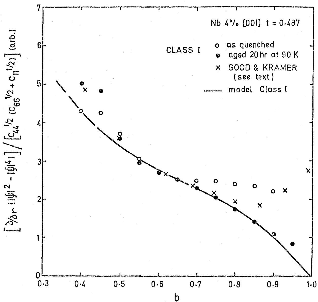
Figure 5.32. Comparison of the predicted b dependence of the bulk pinning force density, from the model for class I, with experiment on the as-quenched and aged [001] 4% deformed specimen (class (i)) and also with the experimental results of Good and Kramer at t \approx 0.48 .
