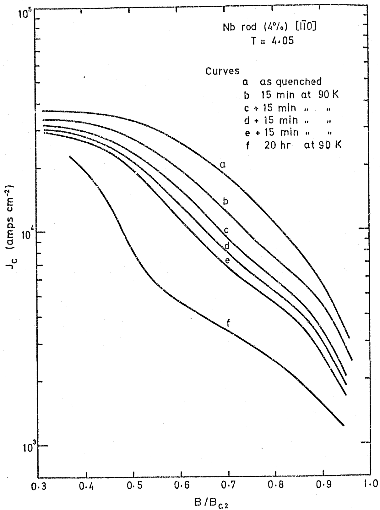
Figure 5.11. The variation at T = 4.05\text{K} of the critical current density with reduced induction for the [1\bar{1}0] , 4% deformed rod specimen after various isochronal ageing treatments.
