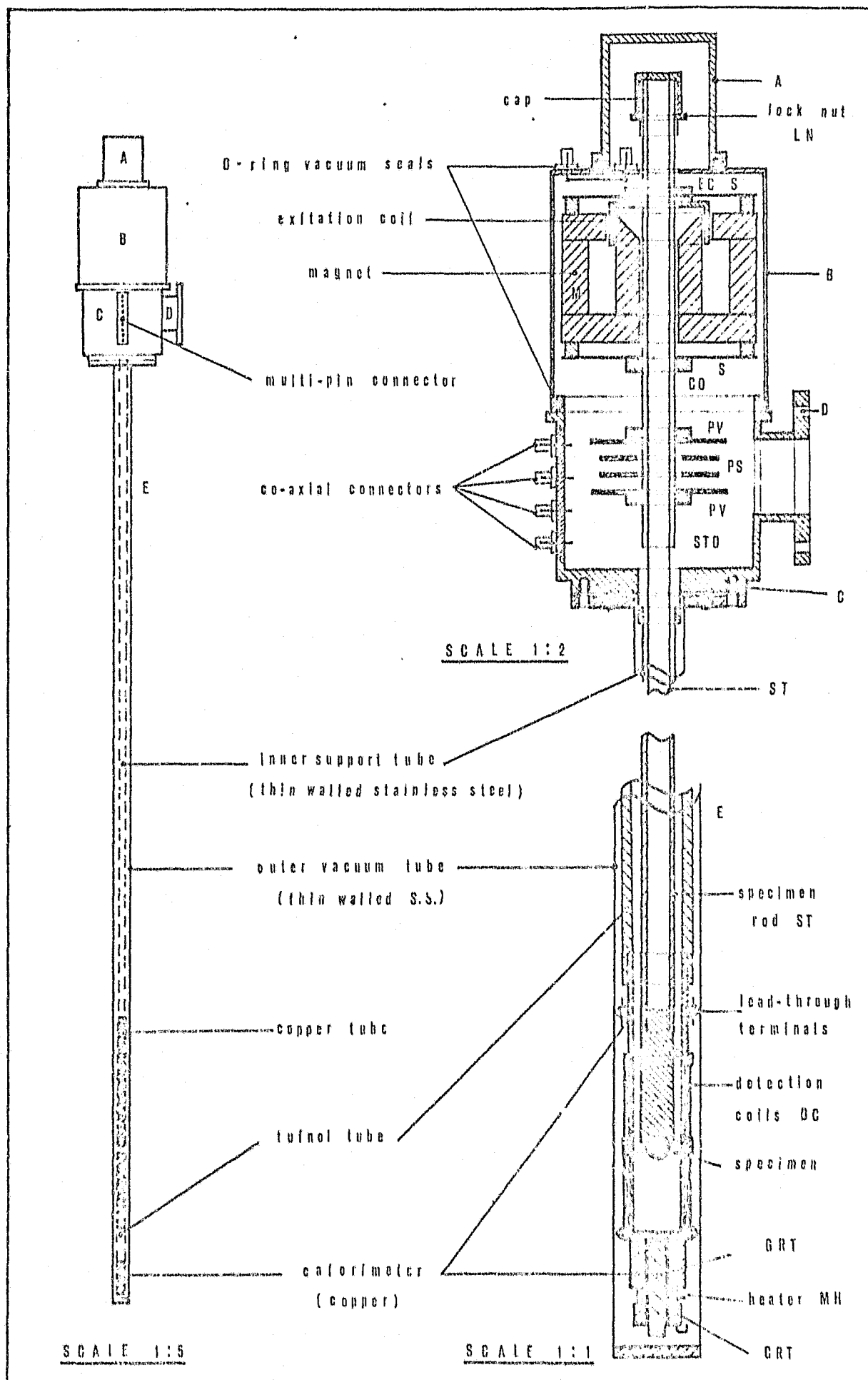
Figure 2.1. The magnetometer; showing the electro-mechanical transducer, reference capacitor, detection coils and the temperature controlled 'calorimeter'.
