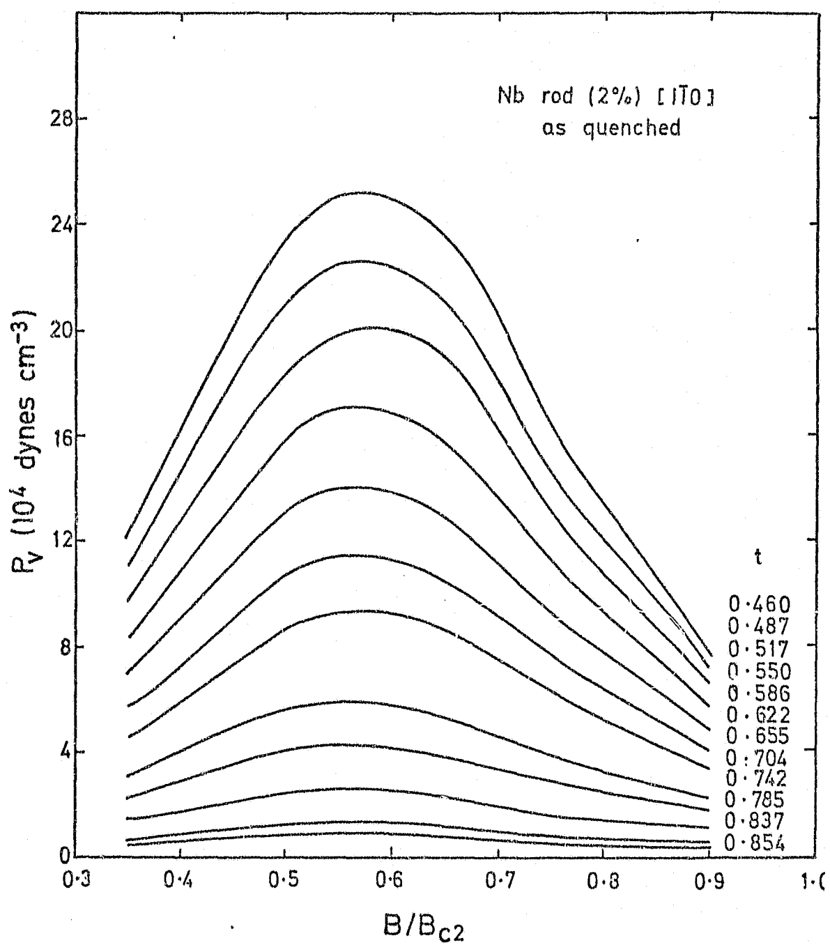
Figure 5.14a. As for figure 5.13 for the as-quenched [110] 2% deformed specimen.
