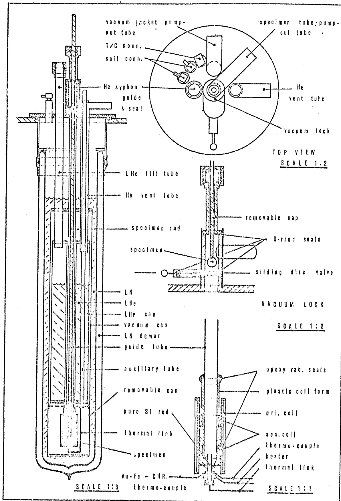
Figure 2.10. The variable temperature cryostat for resistivity measurements.
