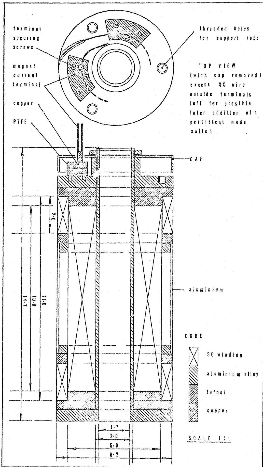
Figure 2.6. The superconducting solenoid magnet.
