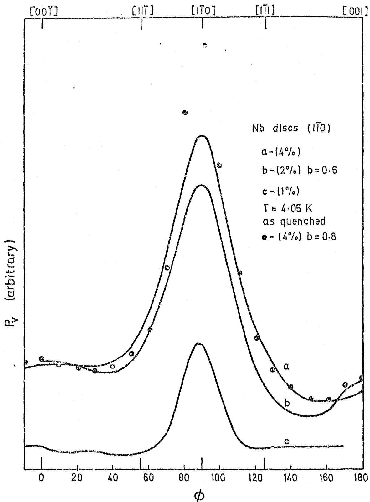
Figure 5.17. The anisotropy of the bulk pinning force density with the applied field in the (110) plane for the as-quenched deformed disc specimens at T = 4.05\text{K} and b = B/B_{c2} = 0.6 (solid curves) and b = 0.8 (points).
