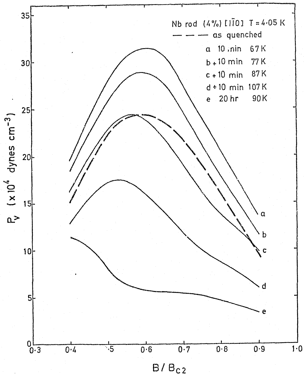
Figure 5.20. The variation in the bulk pinning force density with reduced induction, after 10 minute isochronal ageing procedures at various temperatures, for the [110] 4% deformed specimen. Included is the result for a 20 hour anneal at 90K.
