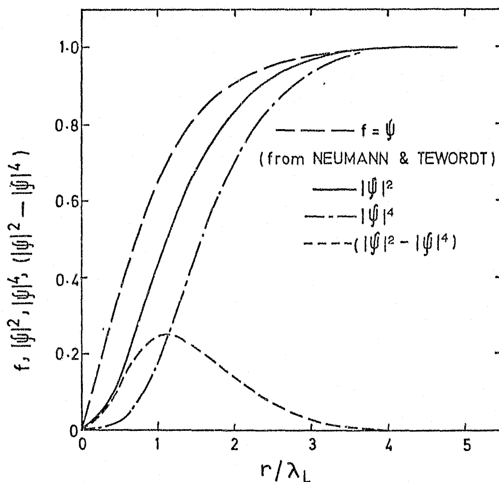
Figure 3.1. The variation of \psi , |\psi|^2 , |\psi|^4 and |\psi|^2 - |\psi|^4 (from Neumann and Tewordt, 1966) for an isolated fluxon as a function of the reduced distance r/\lambda_L from the fluxon axis. \lambda_L is the London penetration length.
