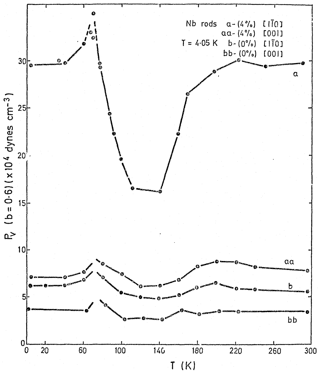
Figure 5.19. The variation of the bulk pinning force density, at b = 0.6 , with ageing temperature in the isochronal ageing experiments on the undeformed and 4% deformed [001] and [1\bar{1}0] rod specimens.
