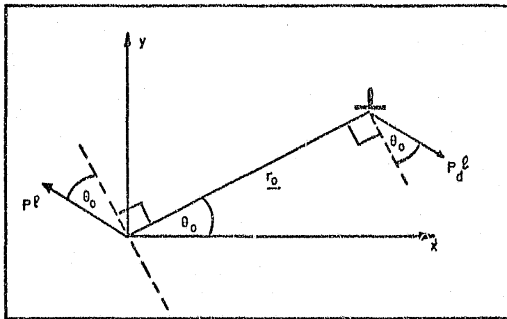
Figure 3.6. The forces due to the interaction between an edge dislocation at r_0 with a Burgers vector in the negative x direction and a fluxon collinear with the r=0 axis.
