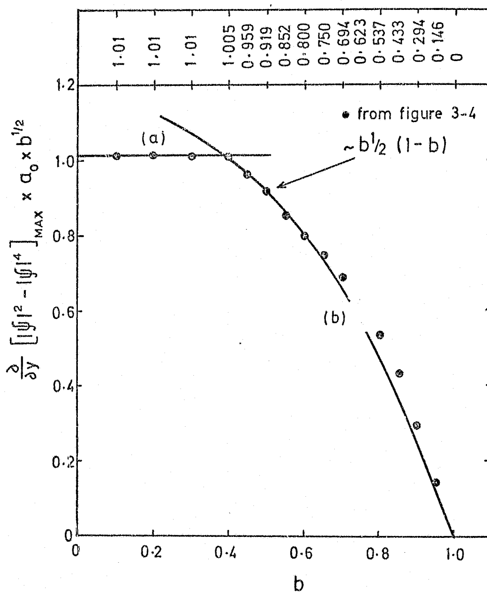
Figure 3.5. The variation in the maximum gradient in B_{c2}^{-1} [|\psi|^2 - |\psi|^4] along the y axis as a function of the reduced induction.
