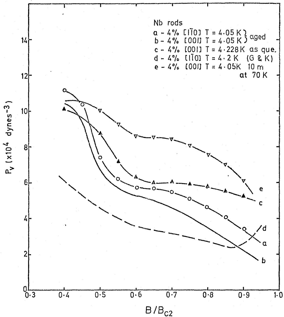
Figure 5.22. The variation of the bulk pinning force density with reduced induction in class (i) (see text).
