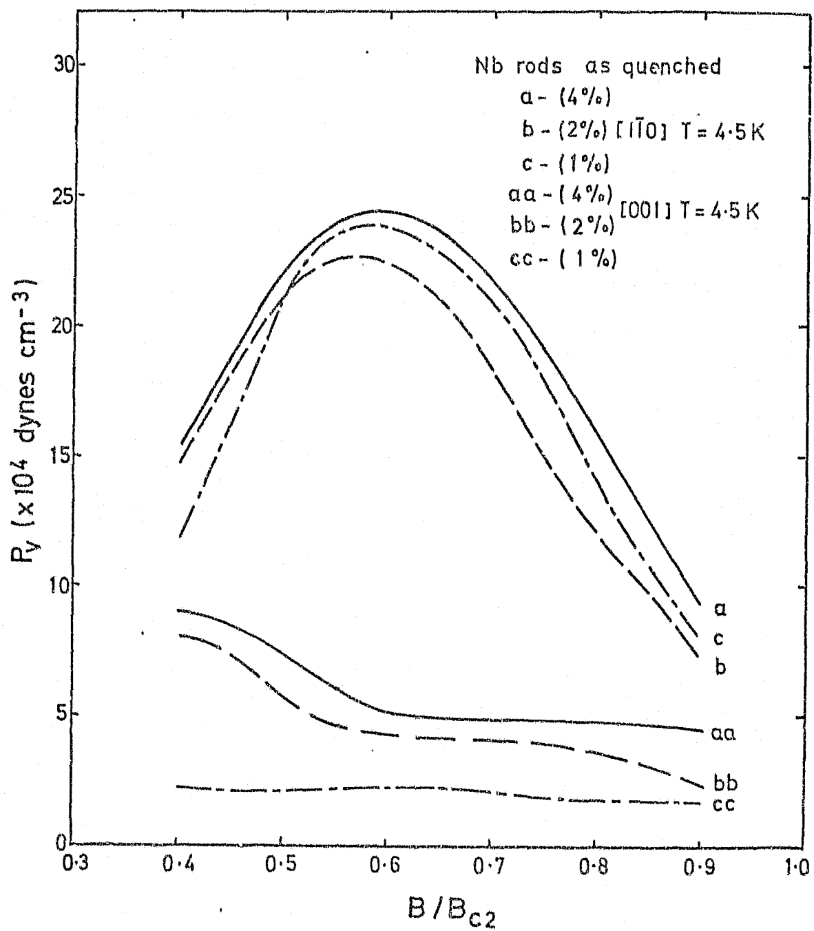
Figure 5.23. The variation of the bulk pinning force density with reduced induction for the deformed specimen at T = 4.5\text{ K} showing the difference in behaviour between the [1\bar{1}0] (class (ii)) and the [001] (class (i)) as-quenched specimens.
