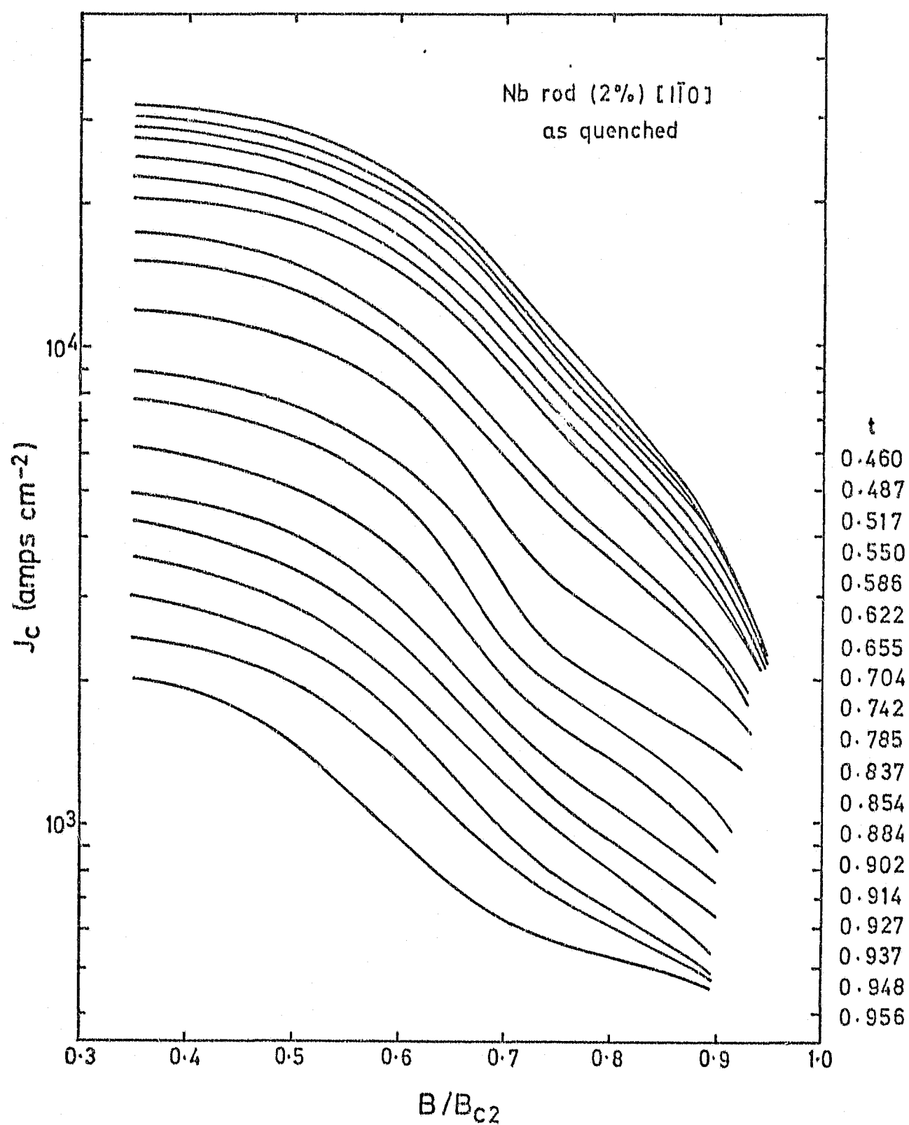
Figure 5.8. As for figure 5.7 for the as-quenched [1\bar{1}0] 2% deformed specimen.
