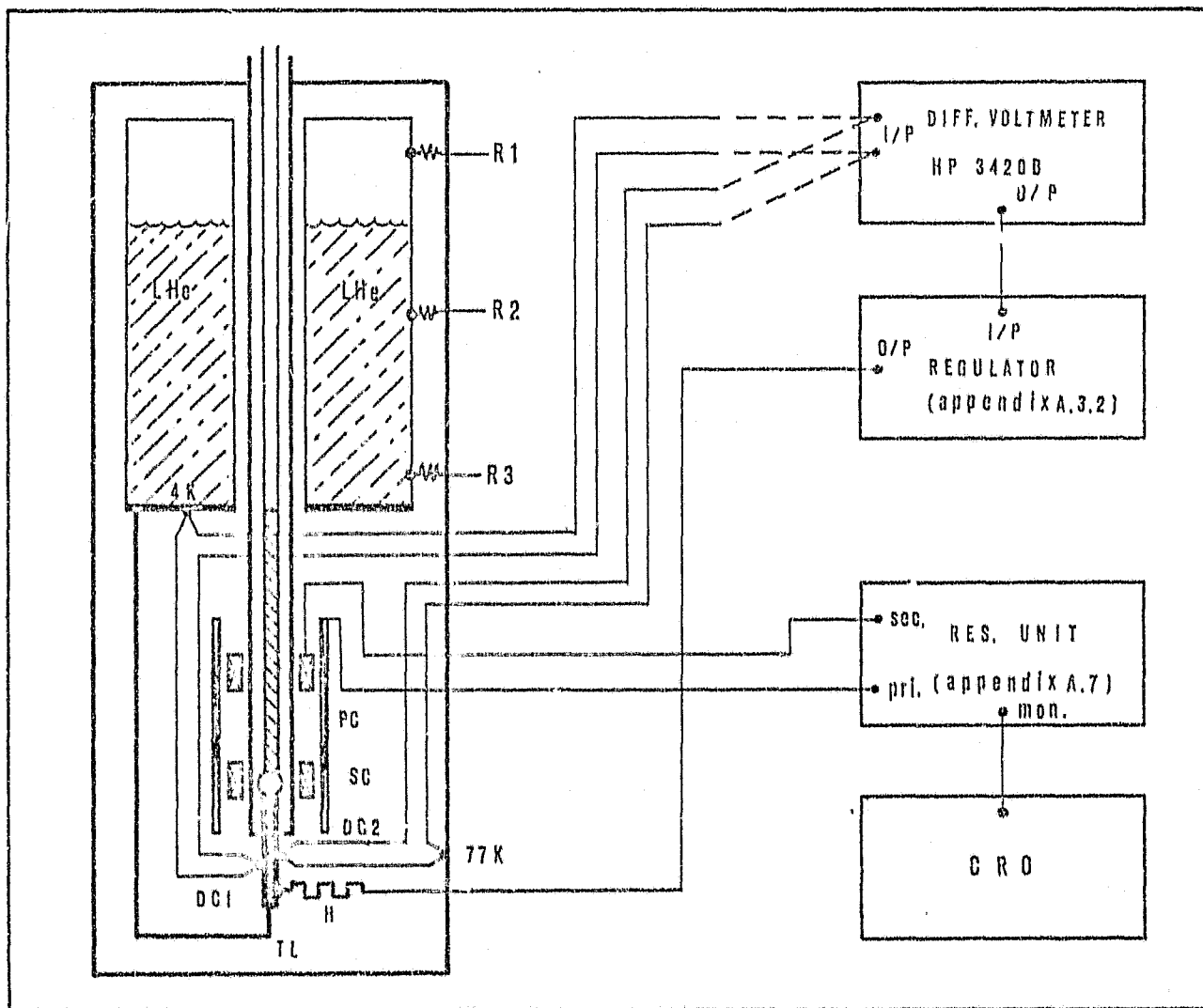
Figure 2.11. Schematic diagram of the system for resistivity measurement and temperature regulation in the variable temperature cryostat.
