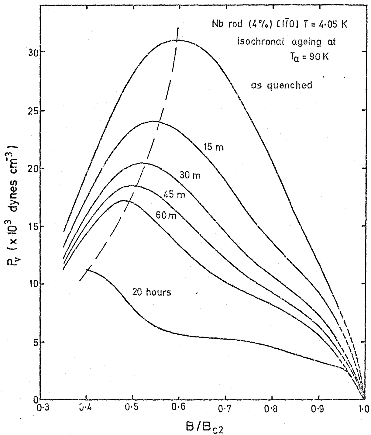
Figure 5.21. The variation in the bulk pinning force density with reduced induction, after successive 15-minute isochronal ageing procedures at 90K.
