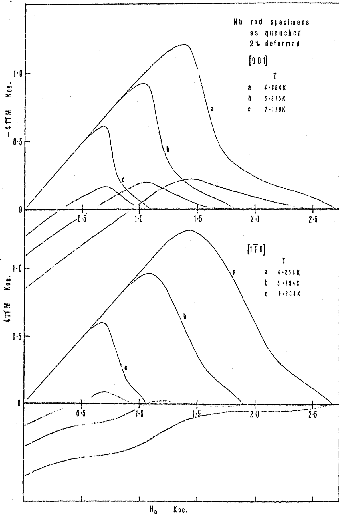
Figure 5.3c. Magnetization curves for the [1\bar{1}0] and [001] 2 per cent (nominal) deformed rod specimens.
