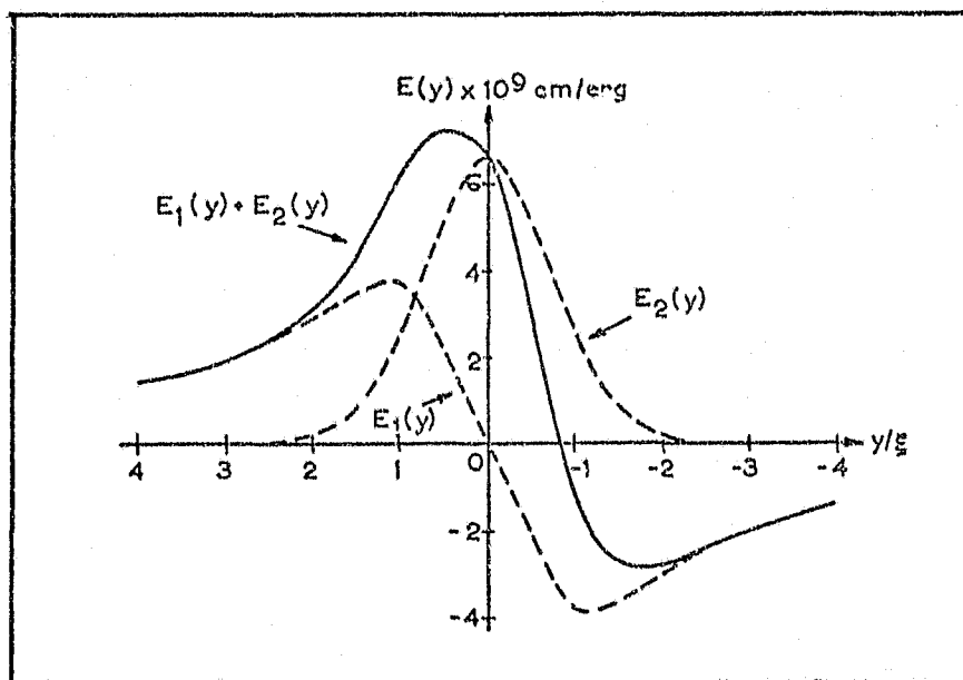
Figure 3.7. The interaction energy, at 4.2K in niobium, between a fluxon collinear with the z axis and a parallel edge dislocation as a function of its position on the y axis. The first order ( E_1 ), second order ( E_2 ) and combined ( E_1 + E_2 ) interaction energies are shown. (From Kramer and Bauer, 1967.)
