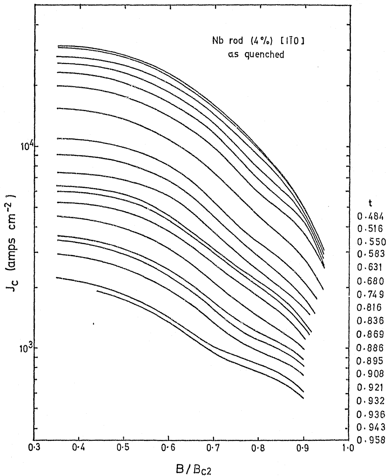
Figure 5.7. The variation, at various reduced temperatures, of the critical current density with reduced induction for the as-quenched [110] 4% deformed rod specimen.
