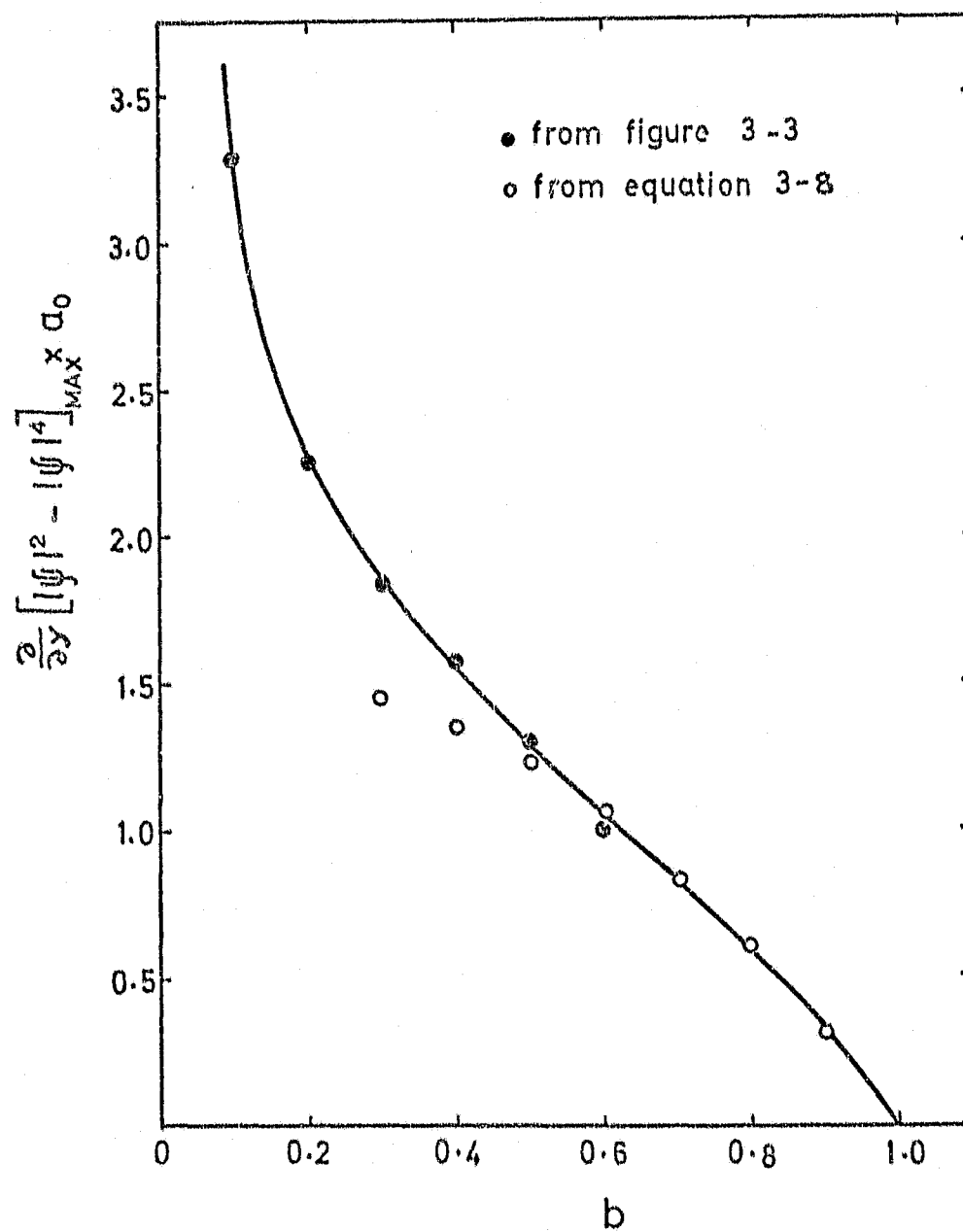
Figure 3.4. From the results of figure 3.3 and equations 3.8 and 3.9 the maximum gradient in [|\psi|^2 - |\psi|^4]_{MAX} \times a_0 along the y axis is shown (solid curve) as a function of the reduced induction.
