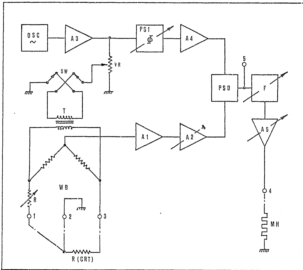
Figure 2.5. Schematic diagram of the electronic layout for the A.C. bridge temperature regulator.
