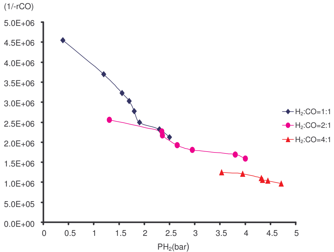
Figure 2.3A: A plot of ( 1/r_{CO} ) versus partial pressure of H_2 at 220 °C. Each curve corresponds to a different feed ratio of H_2/CO as indicated in the legend. The dimensions of the rate of CO consumption are \mu\text{moles CO/g}_{\text{cat}}\text{'s} .
