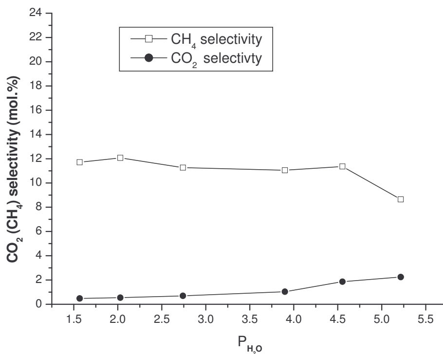
Figure 5. The effect of water addition on the \text{CH}_4 and \text{CO}_2 selectivity using \text{Co/Al}_2\text{O}_3 catalyst.
