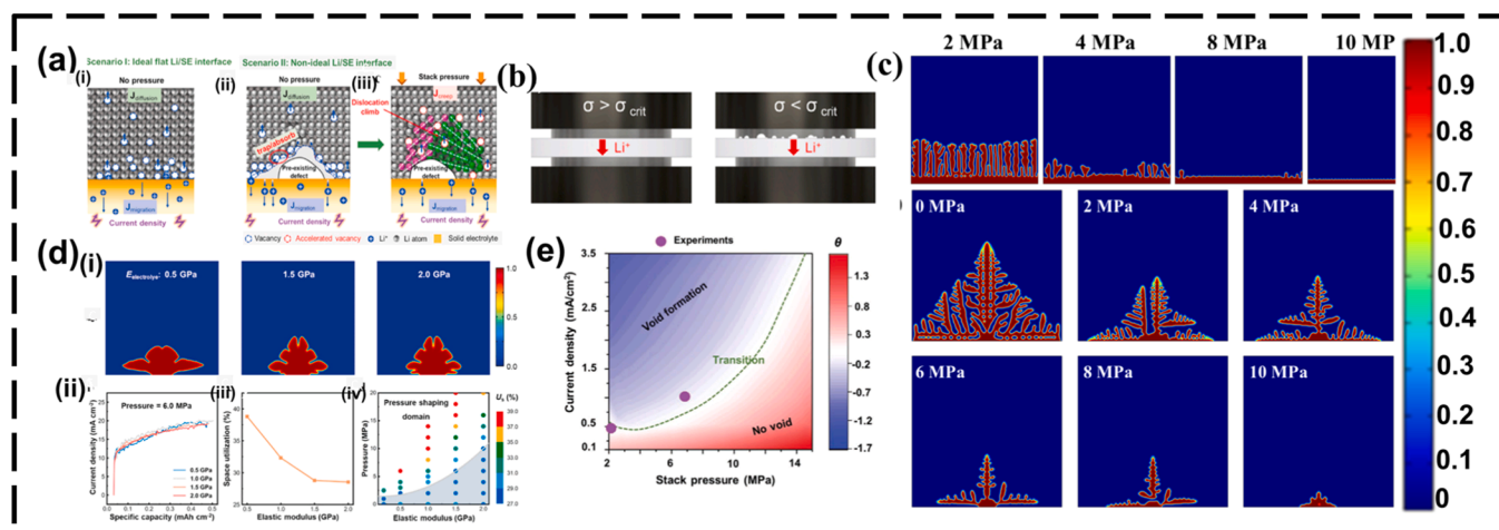
Fig. 13. (a) (i) shows the opposing effects on void formation caused by J_{migration} and J_{diffusion} at a non-ideal, flat Li-SE interface with pre-existing defects. (ii) When vacancies are absorbed or trapped at the surfaces of these defects, J_{migration} exceeds J_{diffusion} , making it insufficient to transfer interfacial vacancies into the bulk Li metal, leading to void formation. (iii) When sufficient stack pressure is applied, J_{creep} surpasses J_{migration} , facilitating the migration of vacancies from the interface into the bulk Li metal, thus preventing void formation (Adapted from Yan et al.) [222]. (b) The adequacy of the applied pressure for maintaining contact between Li and the electrolyte is demonstrated by the proposed microstructure of the Li-electrolyte interface, which depicts scenarios above and below the critical stack pressure (Adapted from Wang et al.) [229]. (c) Simulation results of single Li dendritic morphological growth as a function of external pressures (0 – 10 MPa) (Adapted from Gao et al.) [230]. (d) Lithium dendritic growth in electrolytes with elastic moduli ranging from 0.5 to 2.0 GPa is affected by external pressure. (i) shows the morphology of dendrites at a plating capacity of 0.40 mAh cm -2 , along with (ii) variations in current density during electroplating and (iii) the spatial utilization across different electrolytes. (iv) a phase diagram that links the electrolyte's elastic modulus at a plating capacity of 0.4 mAh cm -2 to the external pressure that is applied (Adapted from Shen et al.) [231]. (e) The graphic shows the relationship between stack pressure, current density, and void formation, with a green dotted line indicating the critical threshold for void generation. Experimental results are represented by purple circles (Adapted from Yan et al.) [222].
