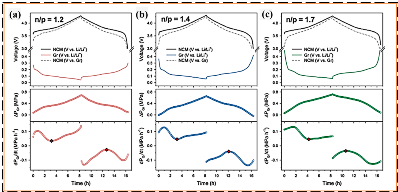
Fig. 11. Shows the results of Differential Electrochemical Pressiometry (DEP) for NCM/Gr all-solid-state three-electrode cells with three different n/p ratios at the 2nd cycle, 0.1C, and 30 °C. It includes charge-discharge voltage profiles for each electrode, corresponding pressure change curves ( \Delta P ), and DEP profiles ( dP/dt ) of Gr electrodes for NCM/Gr cells with n/p ratios of a) 1.2, b) 1.4, and c) 1.7. The red diamonds indicate the lowest and highest points of the DEP profiles throughout the charging and discharging processes (Adapted from Jun et al.) [212].
