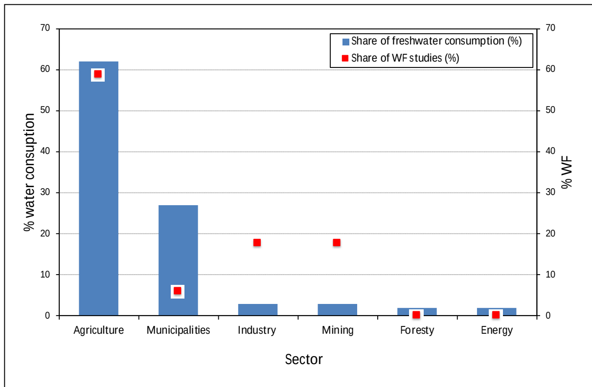
Figure 3: Relationship between the share of freshwater consumption (2019) (GreenCape 2019) and WF studies in South Africa
