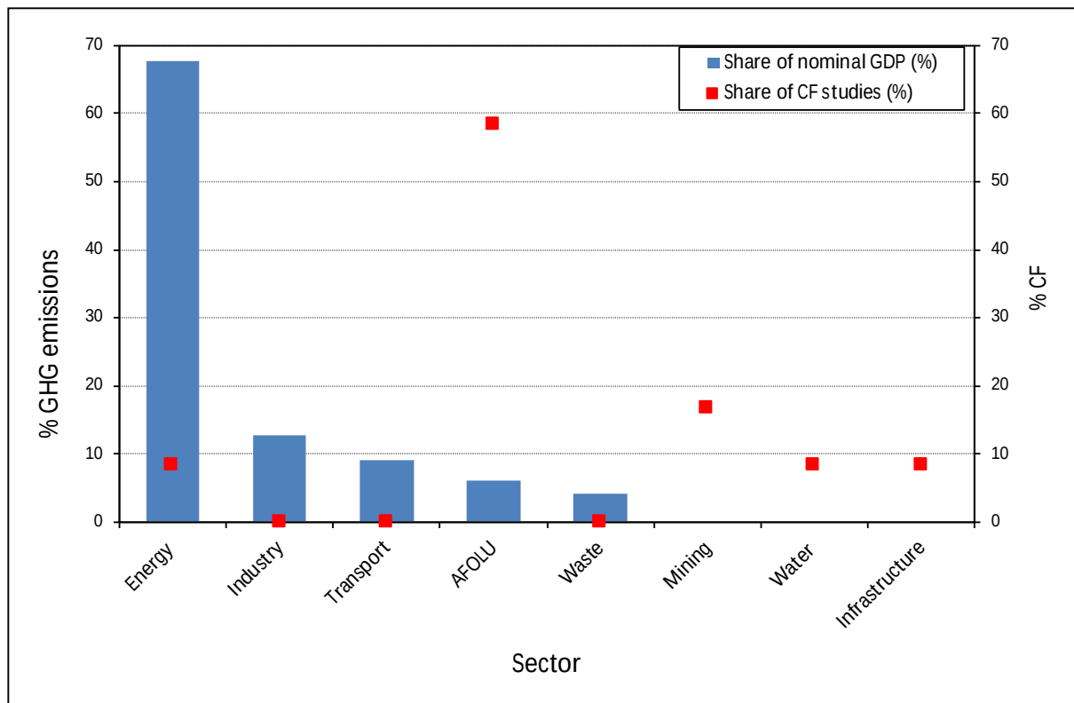
Figure 4: Relationship between the contribution to GHG emissions (2012) (Department of Environmental Affairs 2018) and CF studies in South Africa
