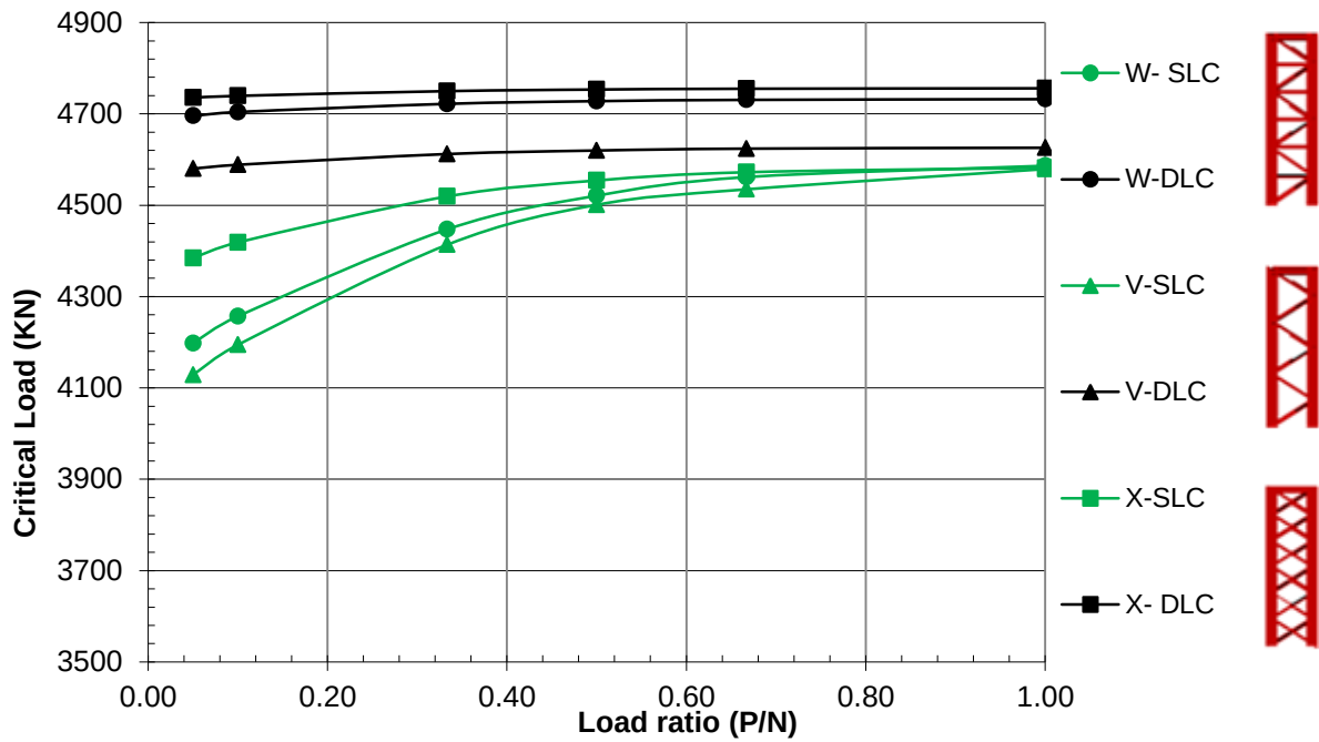
Figure 4:13 Critical load vs. load ratio for column widths of 0.5m
