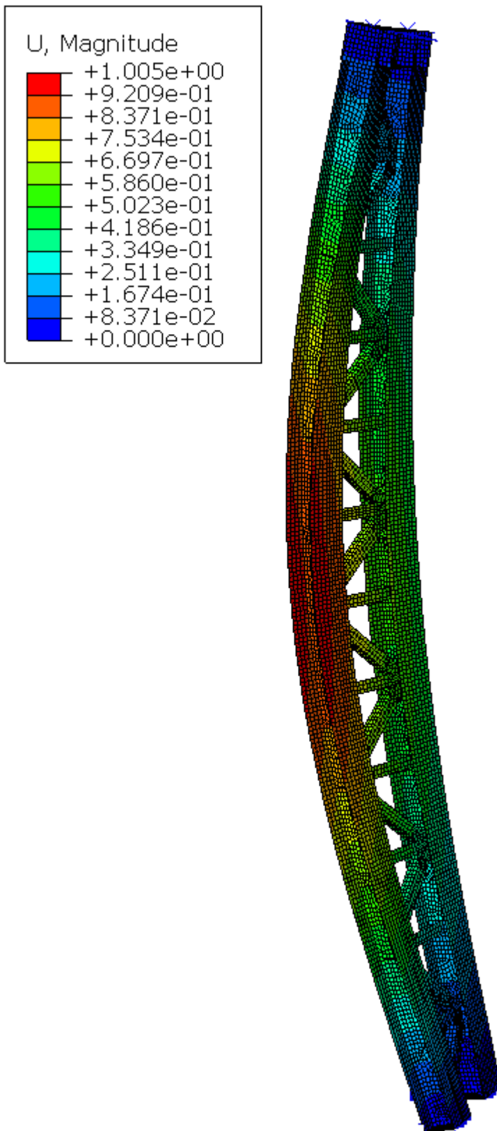
Figure 4:36 Buckled finite element model when the load ratio ( P/N ) < 1
