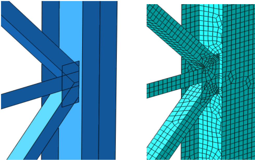
Figure 2:17 Connection detail of a gusset on single laced columns.
