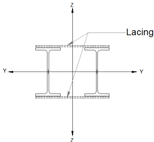
b) Plan view of a built-up column double laced (DLC) on both faces
