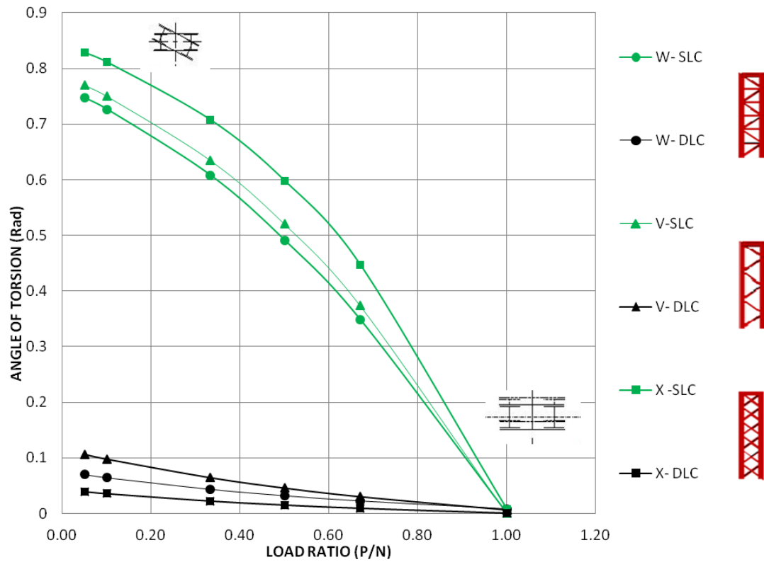
Figure 4:25 Torsion vs. load ratio for SLC and DLC at column widths of 0.75m
