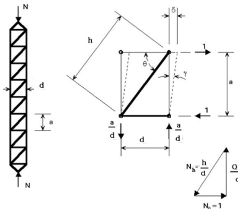
Figure 2:10 Effects of shear forces (Ahmed,2006)
