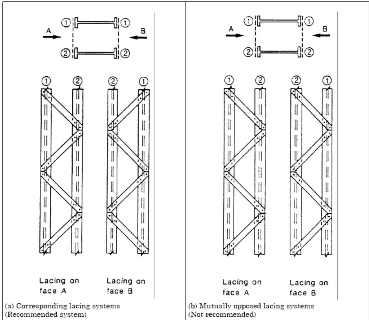
Figure 3:1 Lacing systems of on opposite sides of main components (EN 1993-1-1:2005:Table 6.9)
