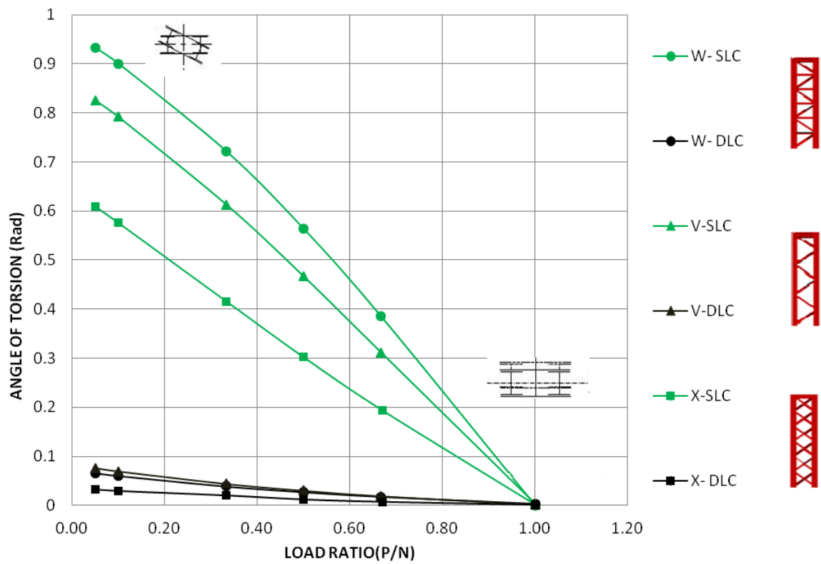
Figure 4:24 Torsion vs. load ratio for SLC and DLC at column widths of 0.5m
