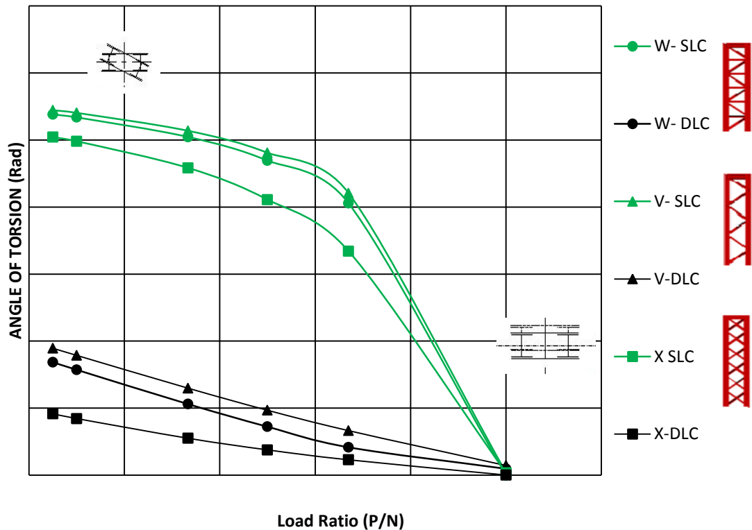
Figure 4:27 Torsion vs. load ratio for SLC and DLC at column widths of 1.5m
