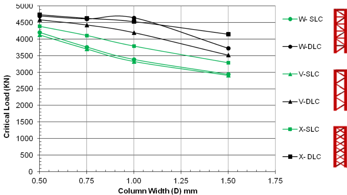
Figure 4:17 Critical load vs. column width for a fixed-free supports at a load ratio of 0.05
