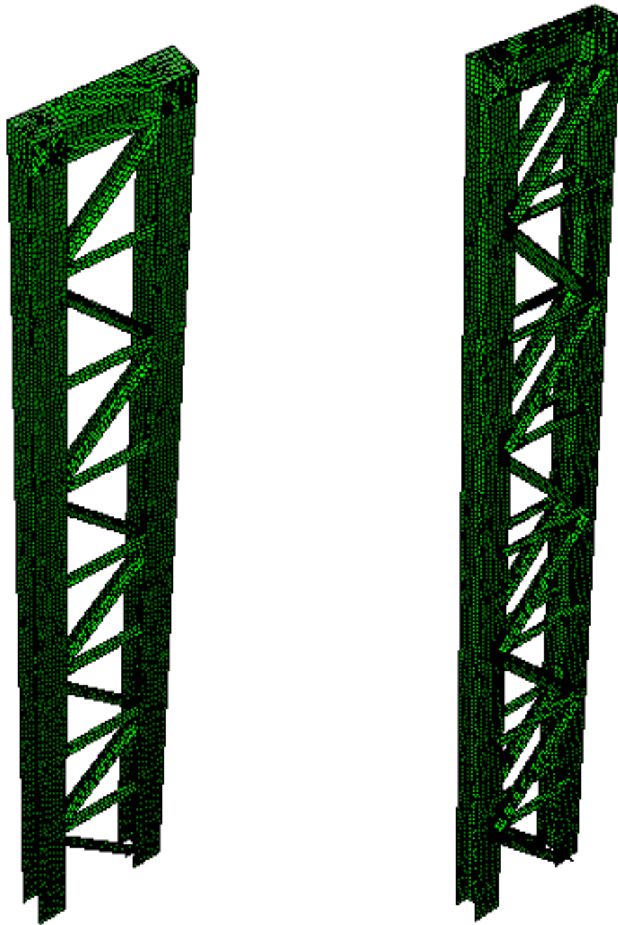
a) Single laced column; Elements: 14217 nodes: 45015 b) Double laced column; Elements: 17808; nodes: 56703
