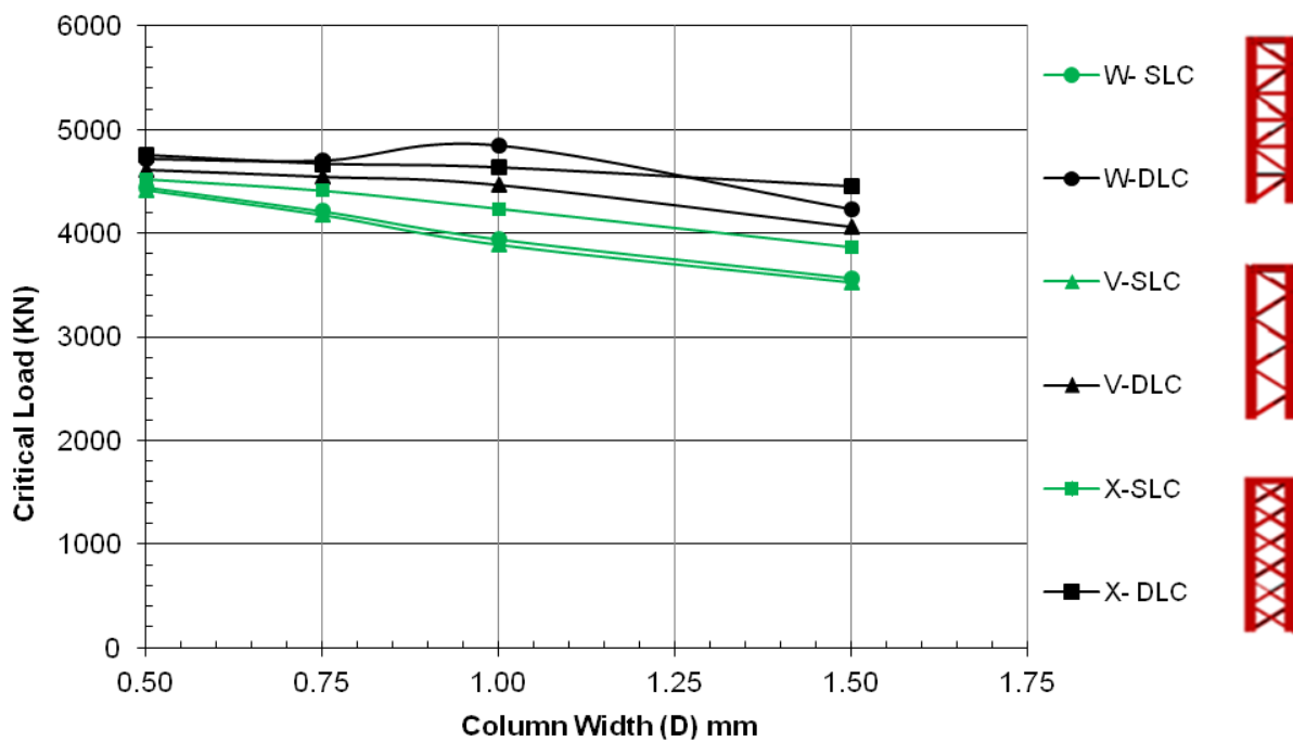
Figure 4:19 Critical load vs. column width for a fixed-free supports at a load ratio of 0.33
