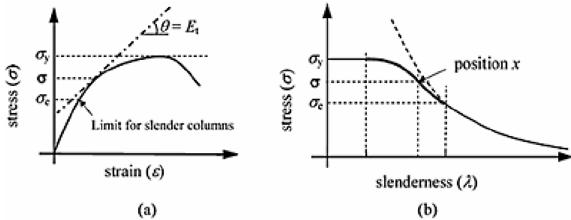
Figure 2.5 Stress / strain curve (McKenzie,2006)
