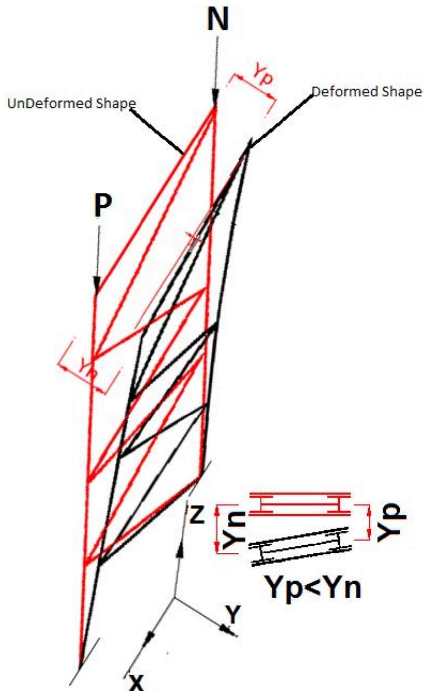
Figure 4:33 Sketch of mode buckled when the load ratio (P/N) > 1
