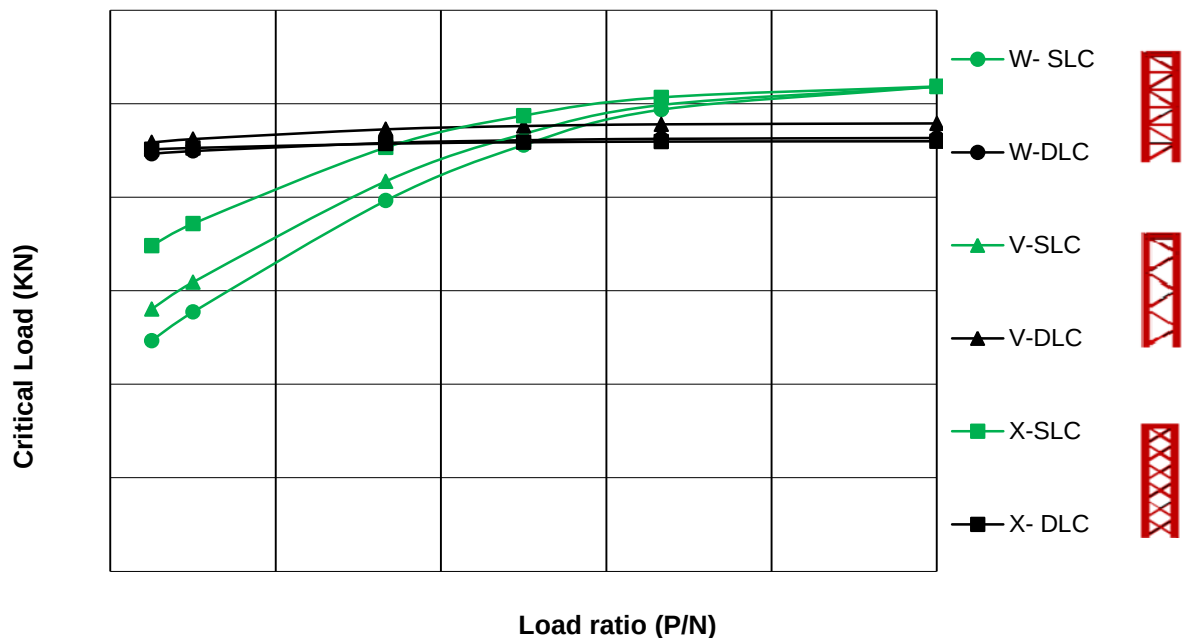
Figure 4:2 Critical load vs. load ratio of fixed-free columns of 0.5m width
