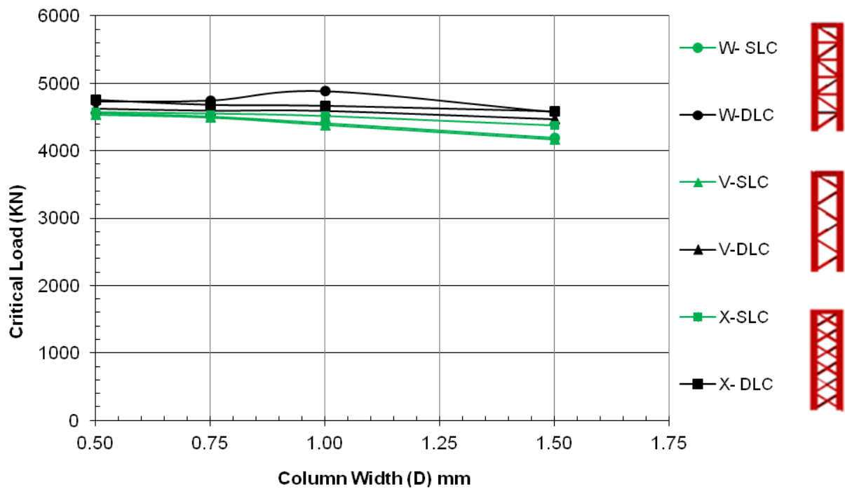
Figure 4:21 Critical load vs. column width for a fixed-free support at a load ratio of 0.67
