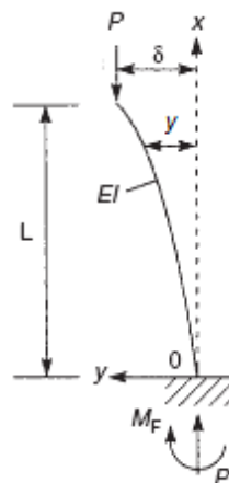
Figure 2:2 Fixed-free column support (Charles,2003)
