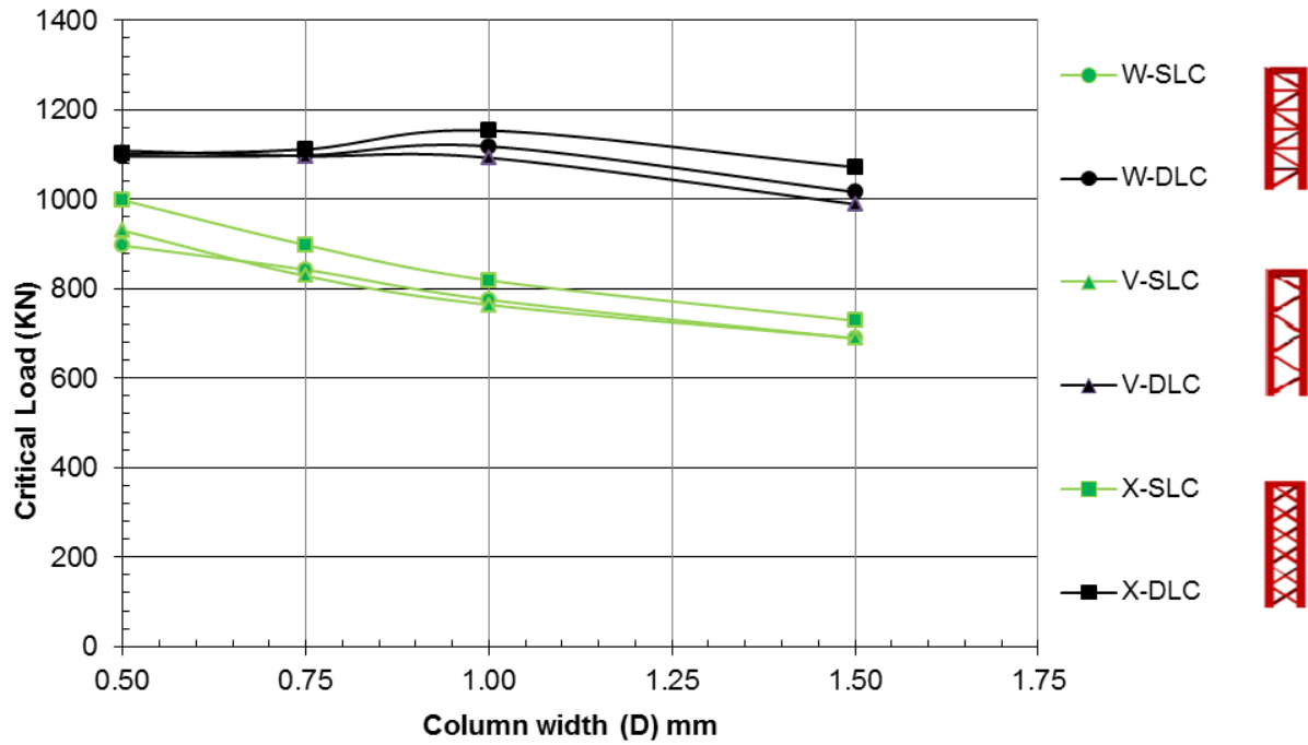
Figure 4:6 Critical load vs. column width for fixed-free columns at a load ratio of 0.05
