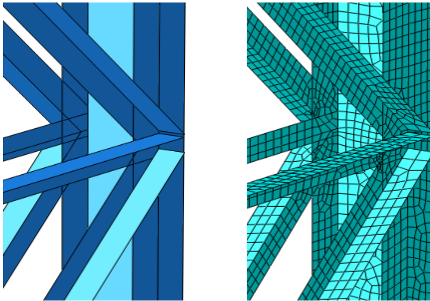
Figure 2:16 Connection detail of the lacing in the double laced columns
