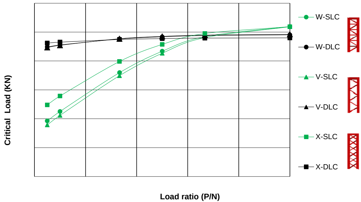
Figure 4:3 Critical load vs. load ratio of fixed-free columns of 0.75m width
