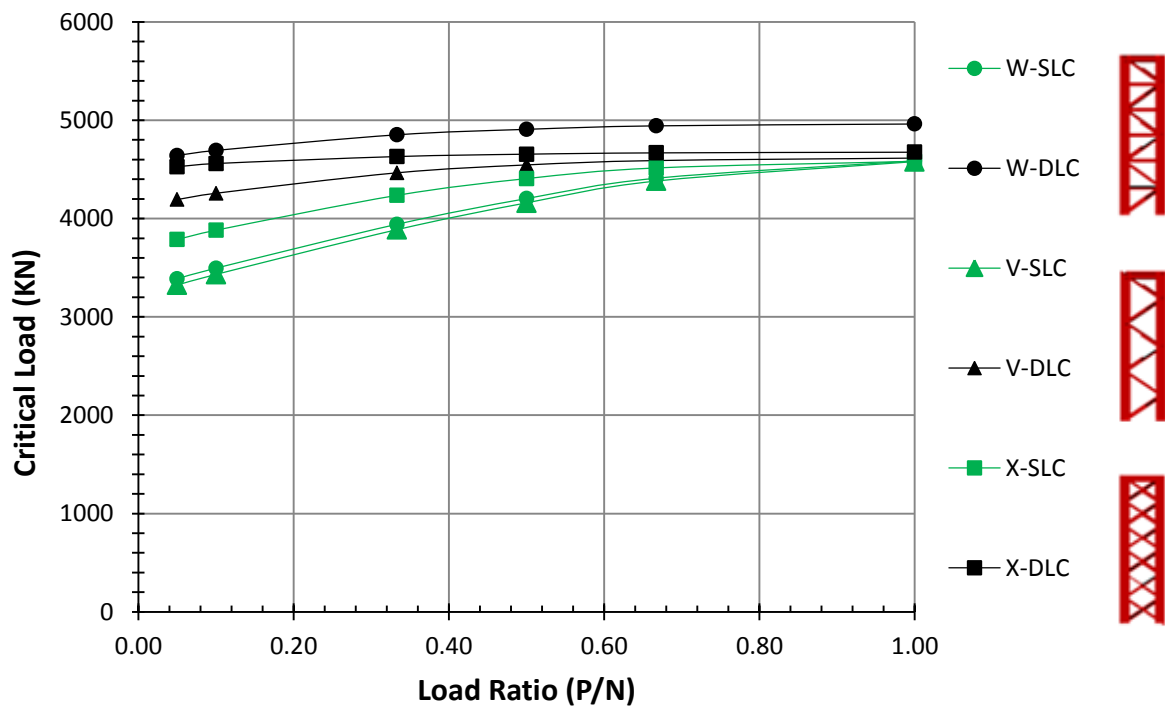
Figure 4:15 Critical load vs. load ratio for column widths of 1.0m
