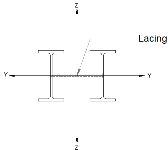
a) Plan view of a built-up column singly laced (SLC): Web-to-Web
