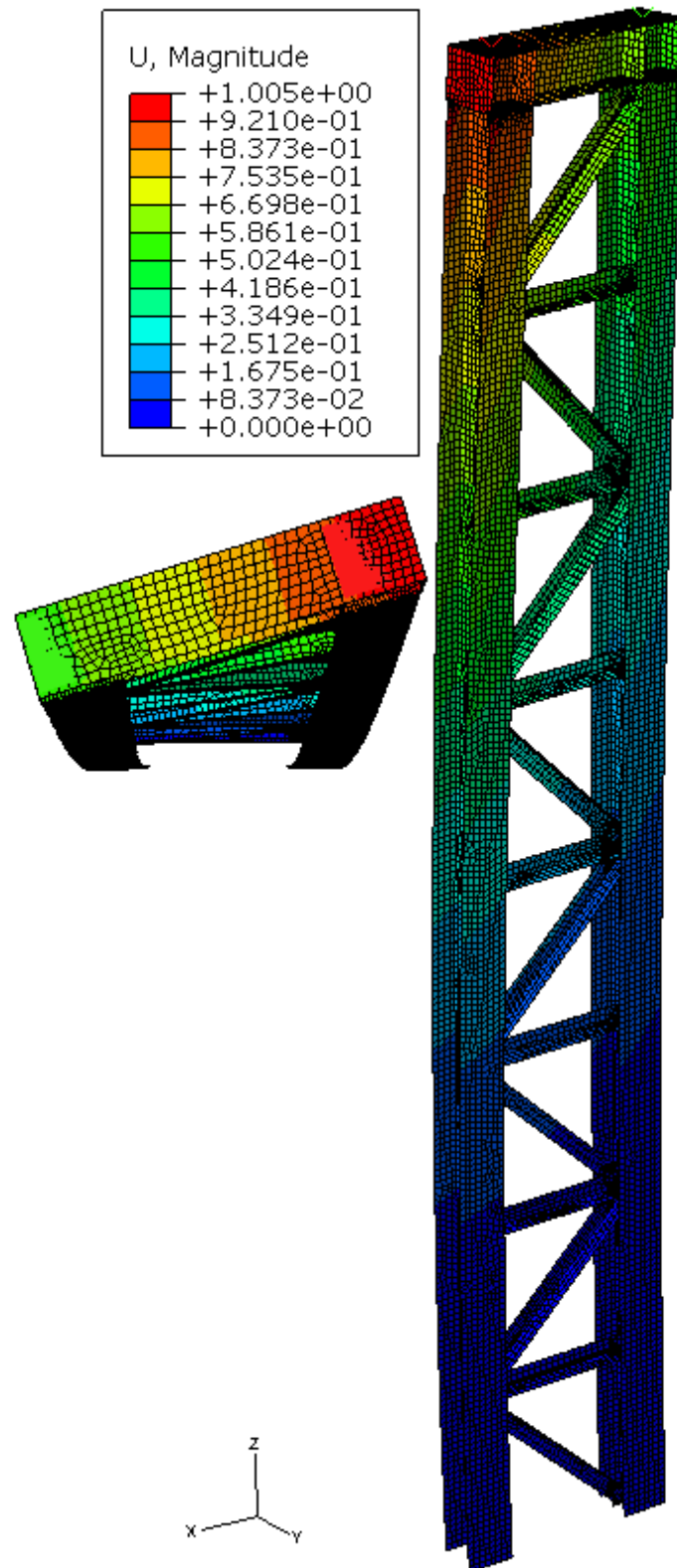
Figure 4:34 Finite element buckled mode shape when the load ratio ( P/N ) > 1
