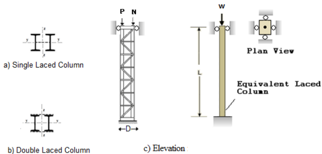
Figure 4:12 Pinned at bottom and roller support on top
