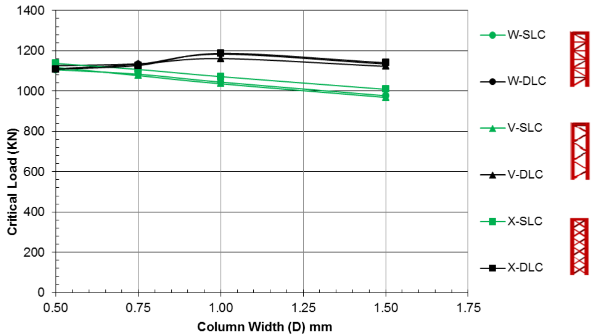
Figure 4:9 Critical load vs. column width for fixed-free columns at a load ratio of 0.5
