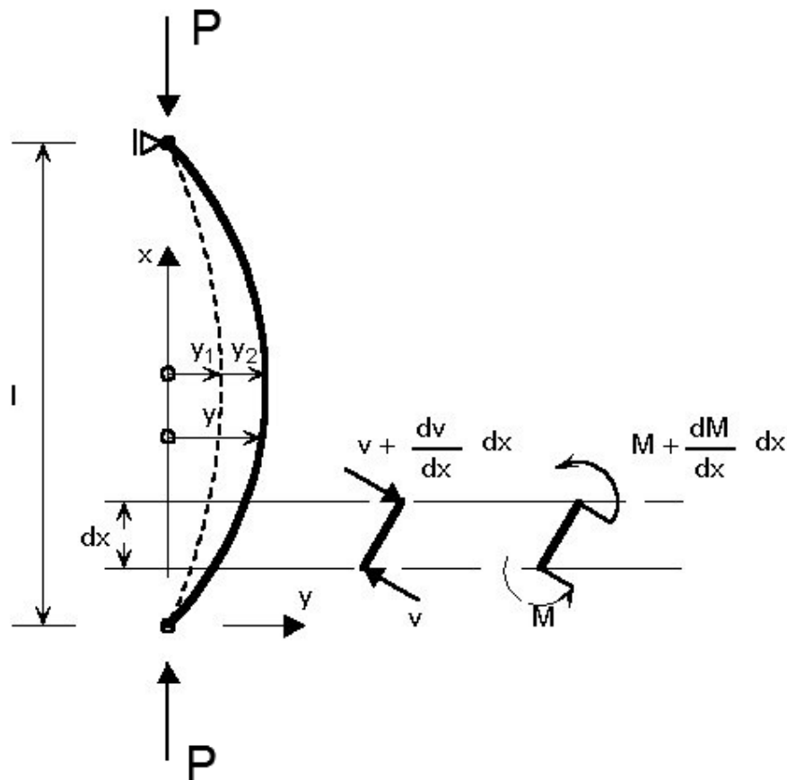
Figure 2:8 Effect of shear force (Ahmed,2006)
