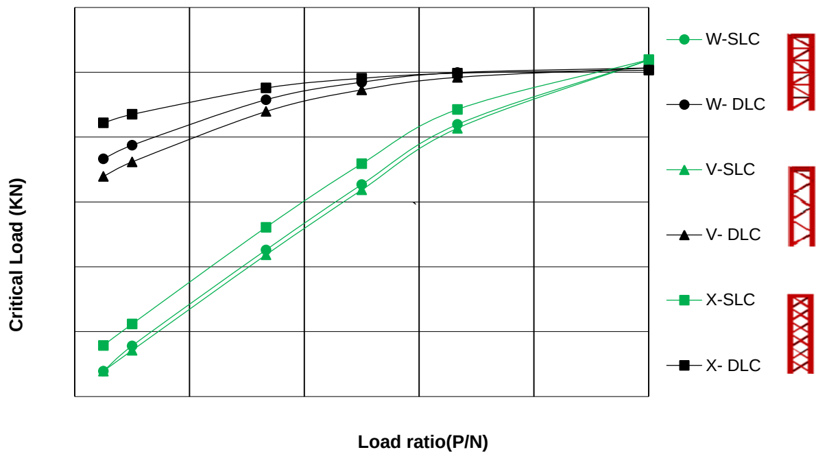
Figure 4:5 Critical load vs. load ratio of fixed-free columns of 1.5m width
