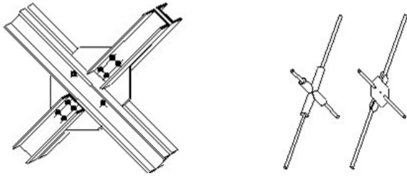
Figure 3:2 Recommend interruption detail of a Lacing systems(EN 1993-1-1:2005)
