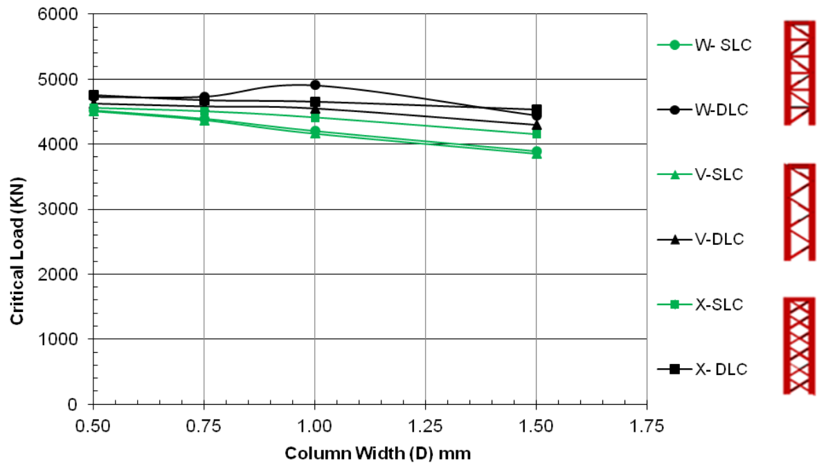
Figure 4:20 Critical load vs. column width for a fixed-free supports at a load ratio of 0.5
