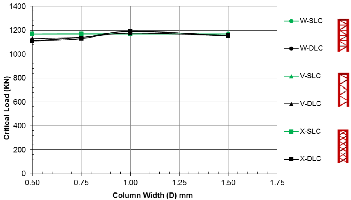
Figure 4:10 Critical load vs.column width for fixed-free columns at a load ratio of 0. 67
