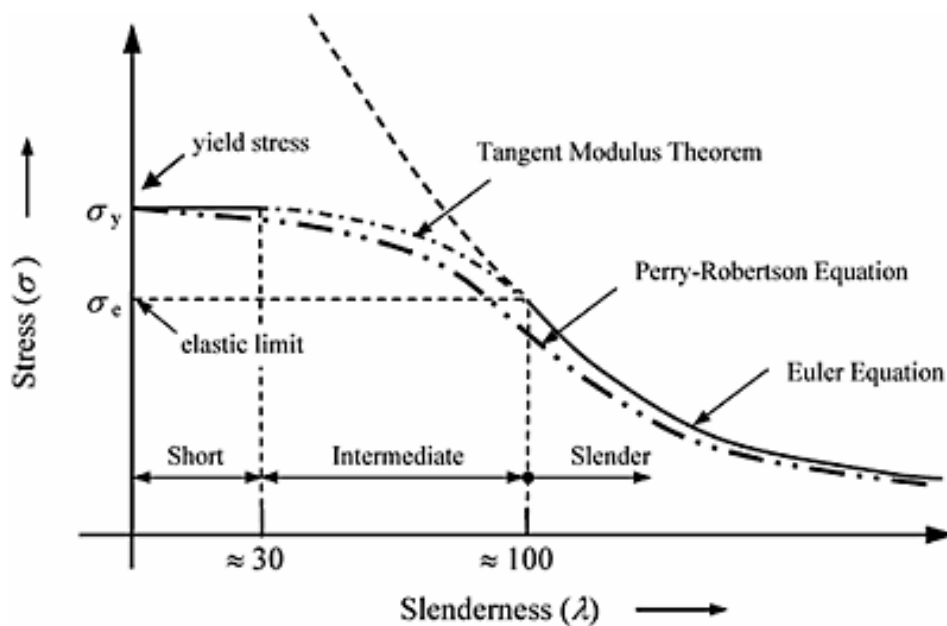
Figure 2:6 Typical stress/slenderness curve of columns (McKenzie,2006)
