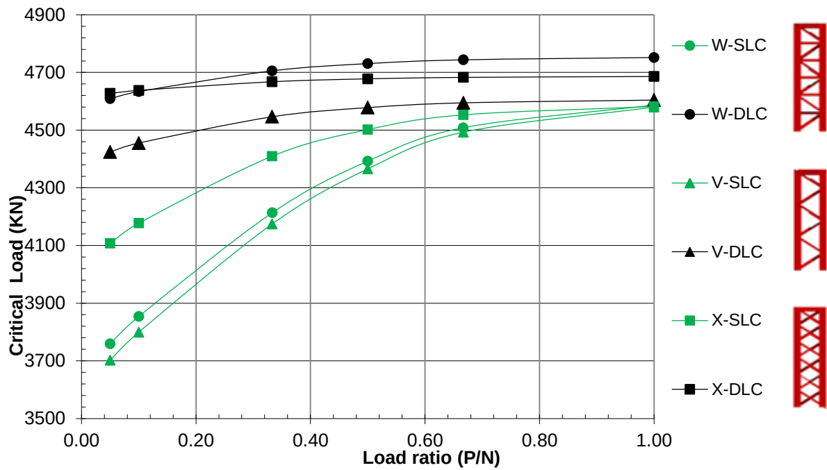
Figure 4:14 Critical load vs. load ratio for column widths of 0.75m
