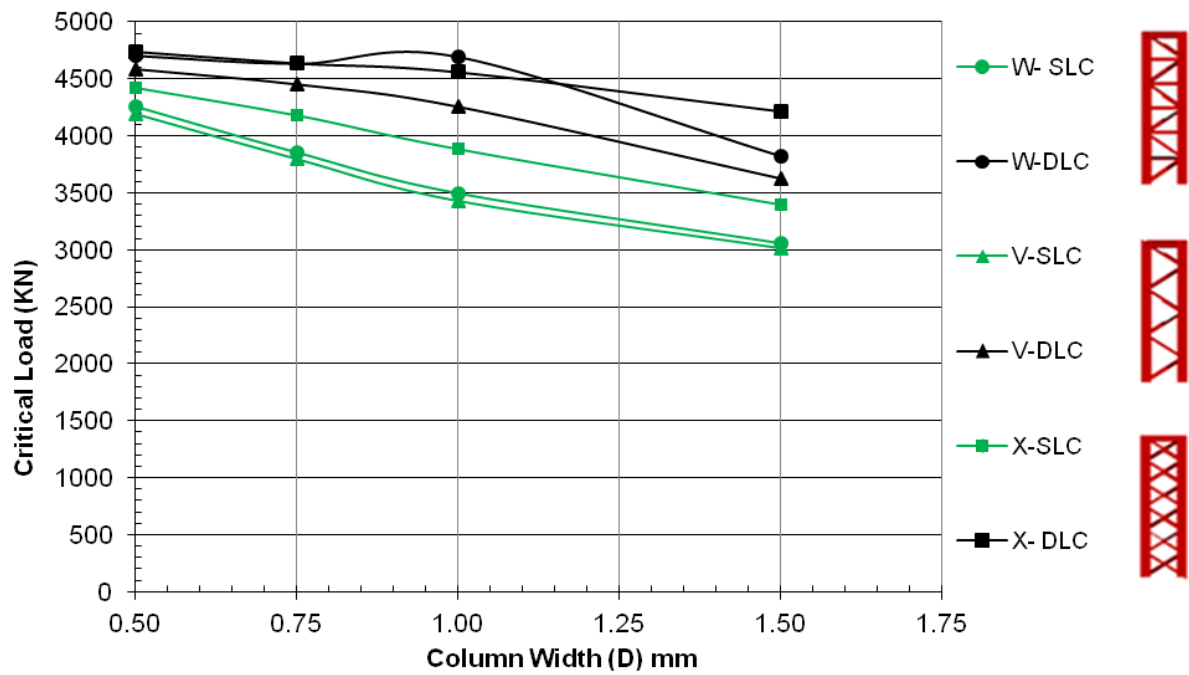
Figure 4:18 Critical load vs. column width for a fixed-free supports at a load ratio of 0.1
