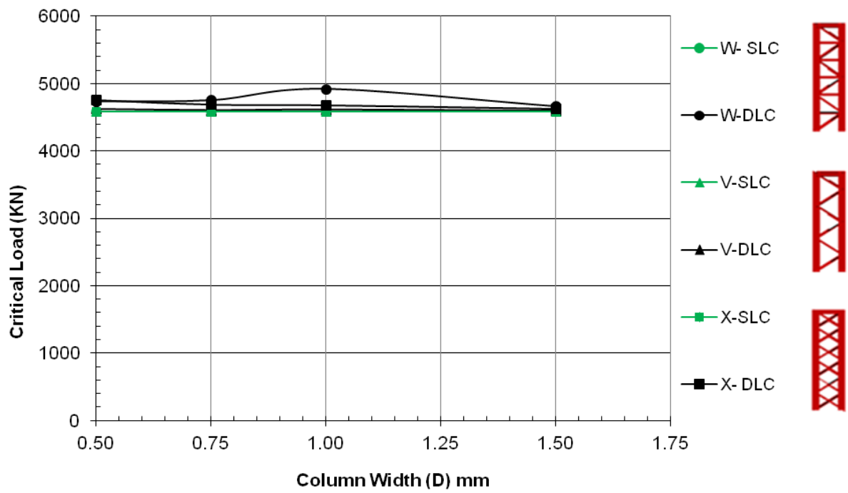
Figure 4:22 Critical load vs. column width for a fixed-free supports at a load ratio of 0.1
