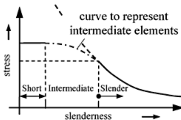
Figure 2:4 Stress/ slenderness for columns of all slenderness ratio (McKenzie,2006)
