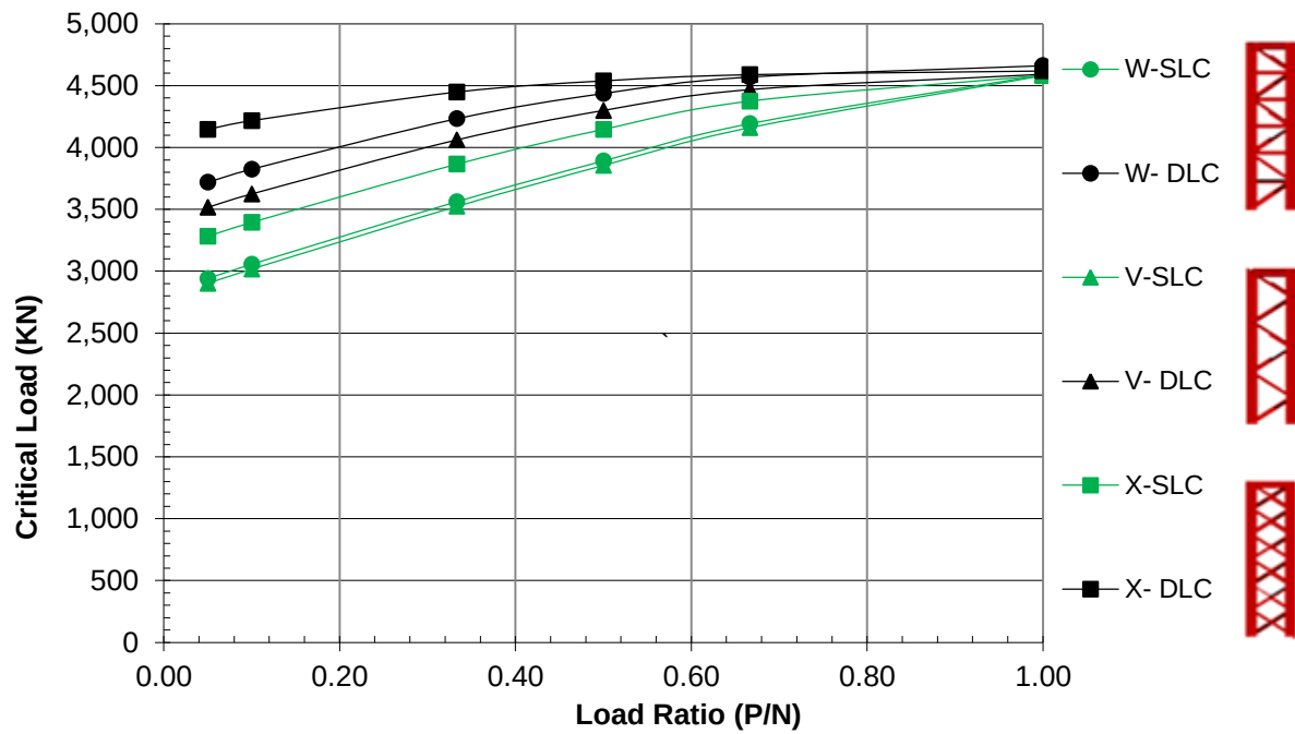
Figure 4:16 Critical load vs. load ratio for column widths of 1.5m
