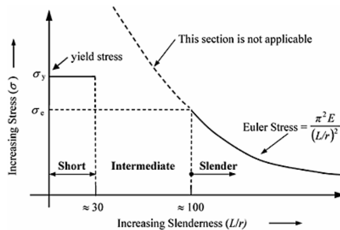
Figure 2:3 Stress vs slenderness for short and slender columns (McKenzie,2006)
