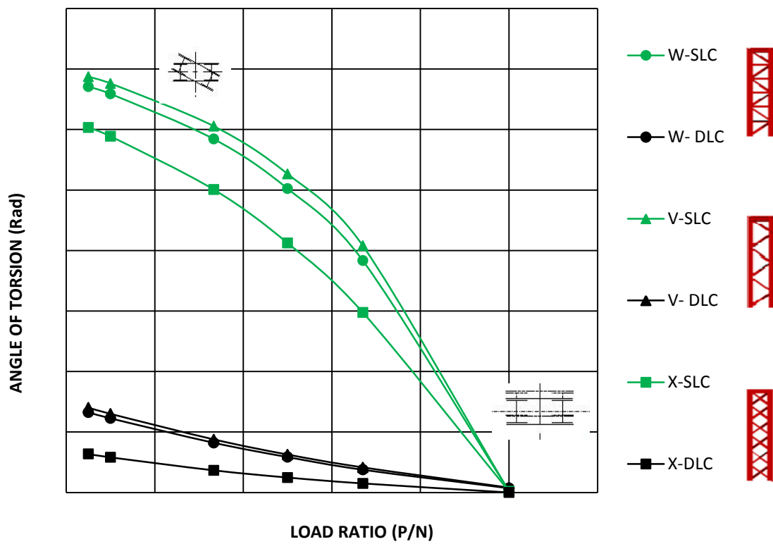
Figure 4:26 Torsion vs. load ratio for SLC and DLC at column widths of 1.0m.
