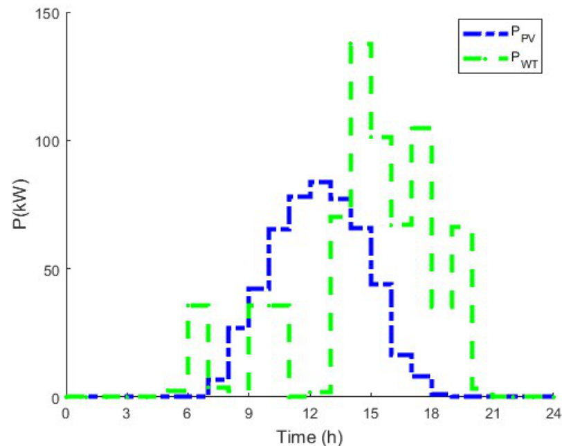
Figure 8. Wind and photovoltaic power generated by the hybrid systems.
