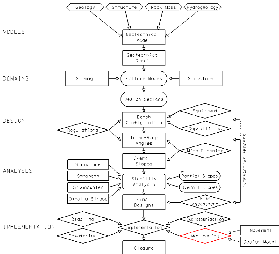
Figure 2 - The Slope Design Process Read and Stacey, 2009
