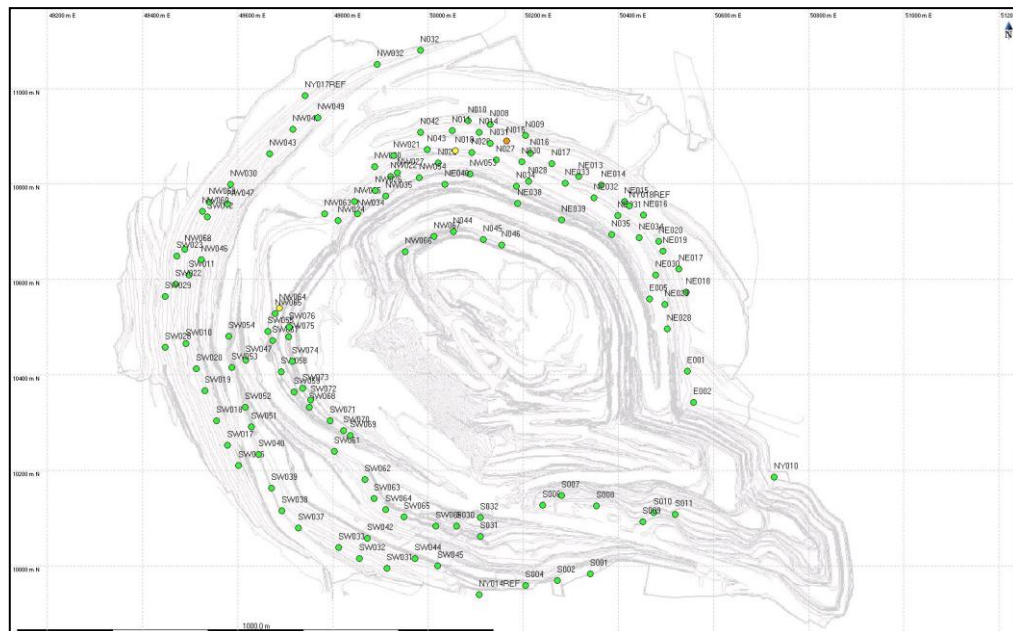
Figure 7 - Typical layout of an open pit operation with monitoring points (Thomas: 2010)
