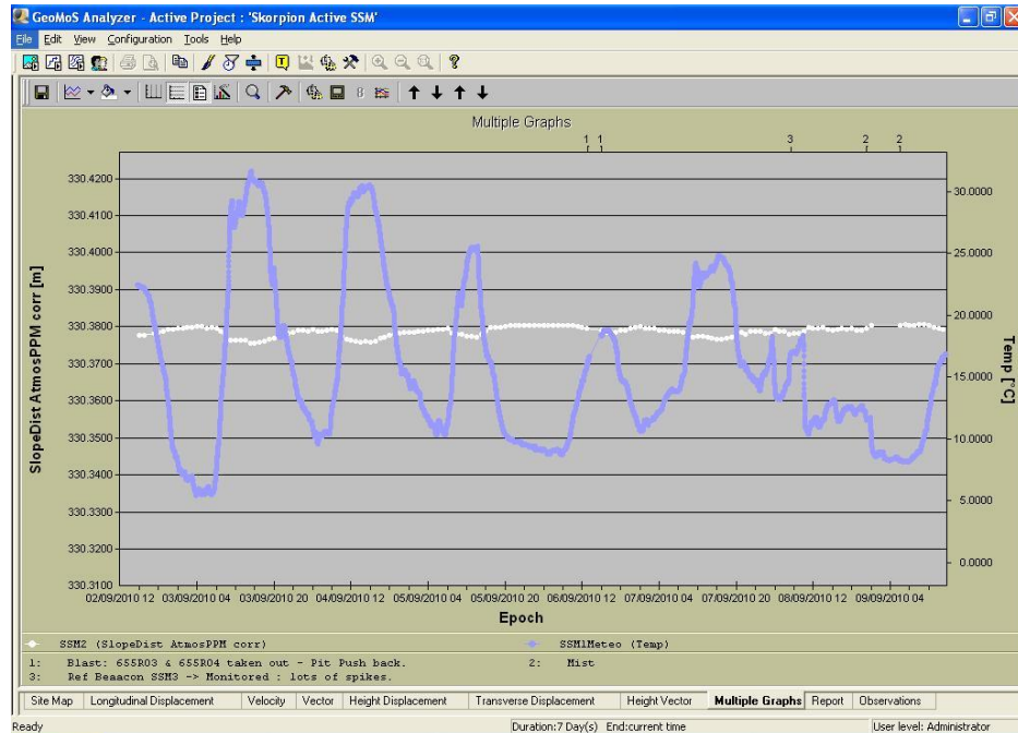
Figure 4 - The influence of temperature changes on measured slope distances (Thomas: 2010)
