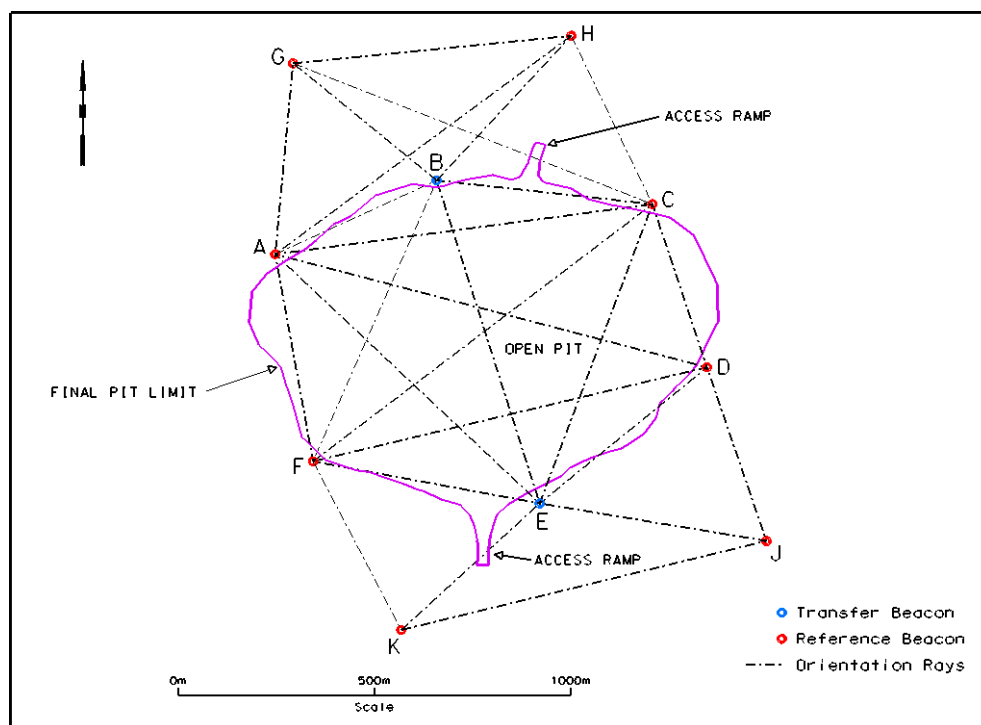
Figure 3 - Layout of an open pit with transfer and reference beacons showing orientation rays between beacons (Thomas: 2010)
