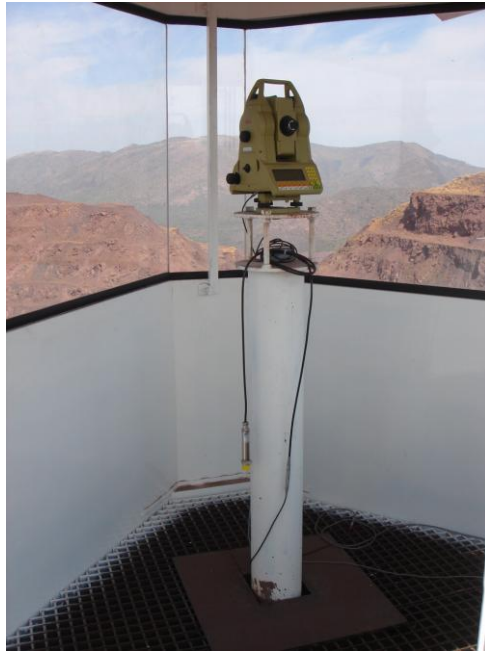
Plate 7 - Transfer beacon in protective enclosure; no insulation of the pillar beacon
