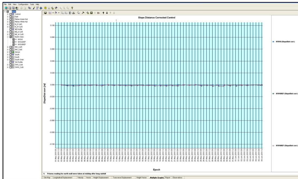
Figure 9 - GeoMoS graph showing variance of slope distances (corrected for ppm) between transfer and reference beacons (Thomas: 2010)
