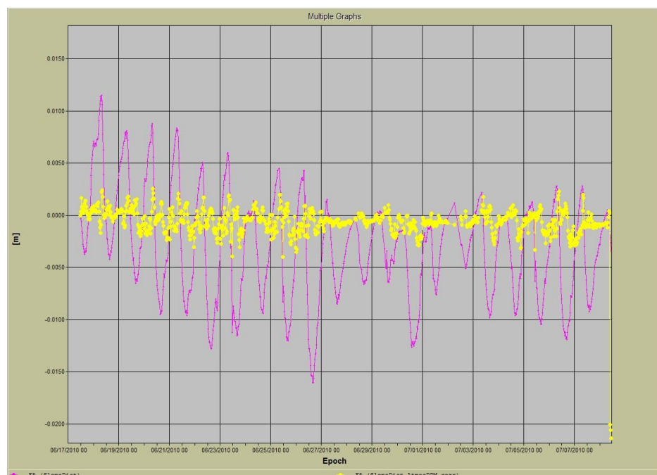
Figure 5 - The effect of ppm correction for temperature and pressure on measured slope distances – with ppm applied (yellow) and without ppm applied (purple) (Thomas: 2010)
