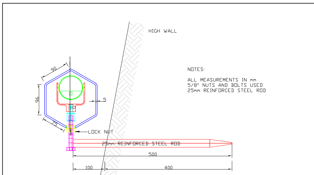
Figure 12 - Cross-section showing face prism configuration for attachment to highwall (Mogalakwena Platinum Mine, RSA).
