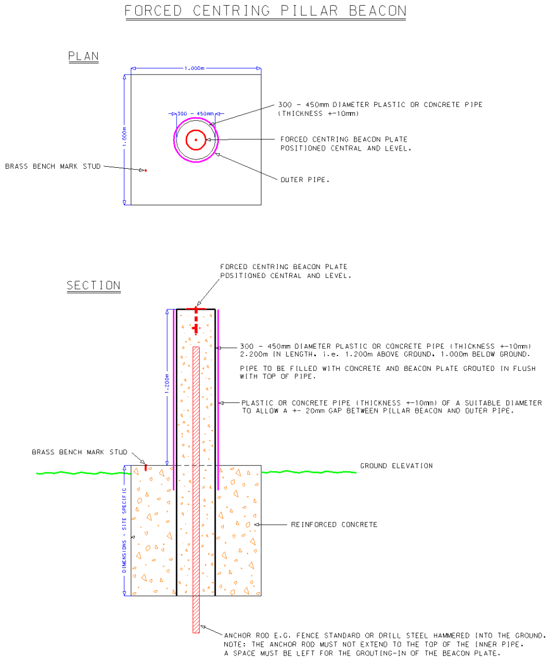
Figure 11 - Diagram showing a typical forced centring beacon design
