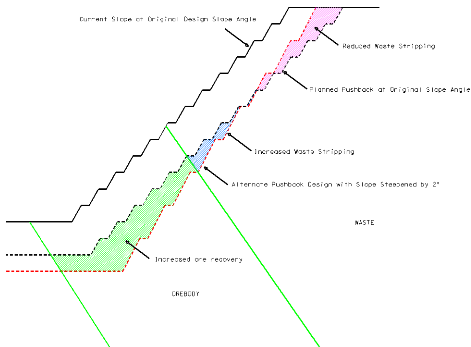
Figure 1 - The Potential Impacts of Slope Steepening Read and Stacey, 2009
