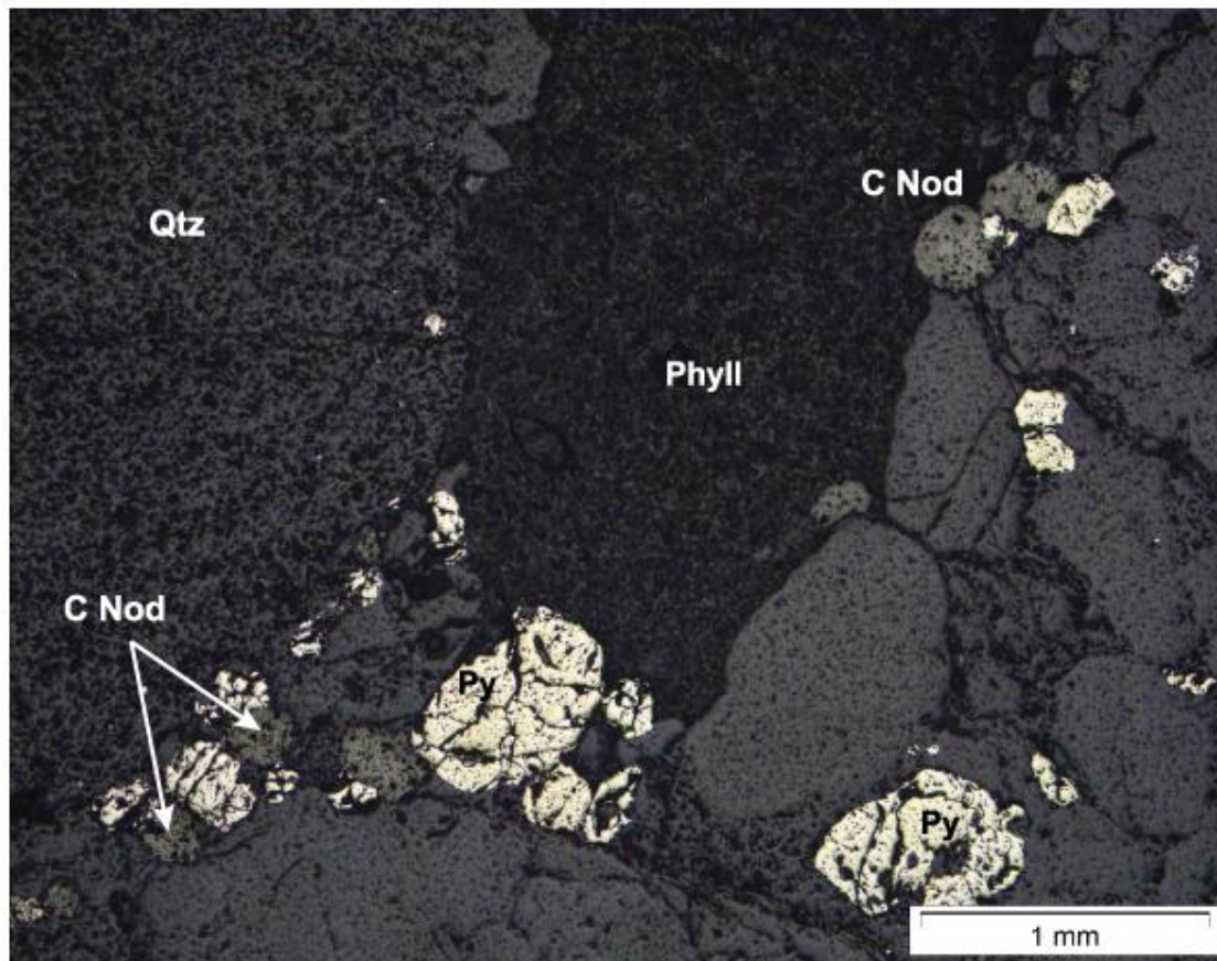
Figure 3.7 Reflected light image of rounded carbon nodules in CREEF07
