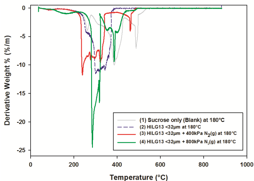
Figure 7.3 First derivative graphs of solvothermal products using HILG13 <32µm powders
