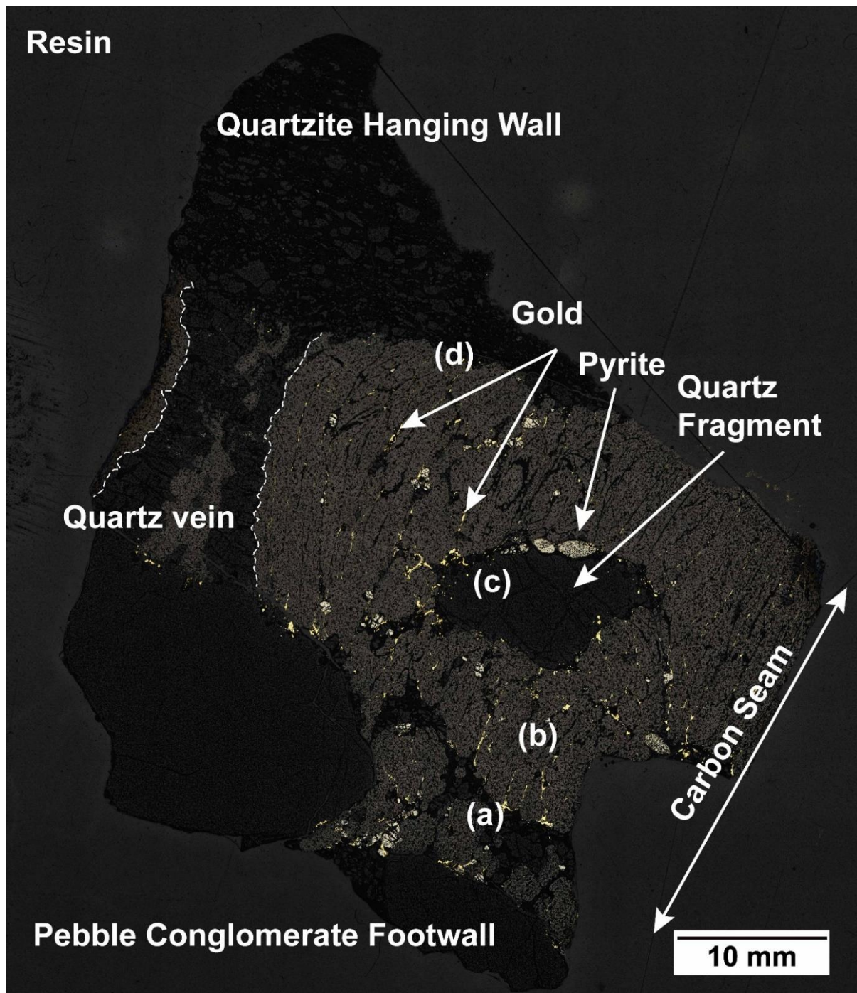
Figure 6.2. Stitched petrographic image of CLR ore block.
