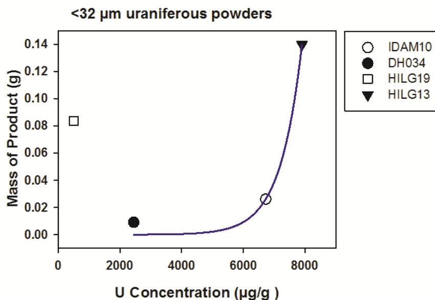
Figure 5.3 The mass of product formed vs Uranium concentration, for <32 \mu\text{m} uraniferous powders from CCVD reactions at 600°C; the line shows the exponential regression for the IDAM10, DH034 and HILG13 data. The HILG19 data is a statistical outlier. Each symbol represents the average of 3 experiments.
