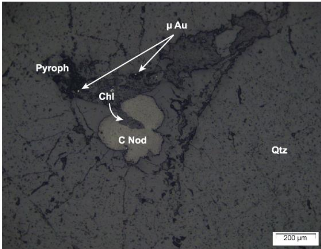
Figure 3.8 Reflected light image of an irregular carbon nodule in VCR1
