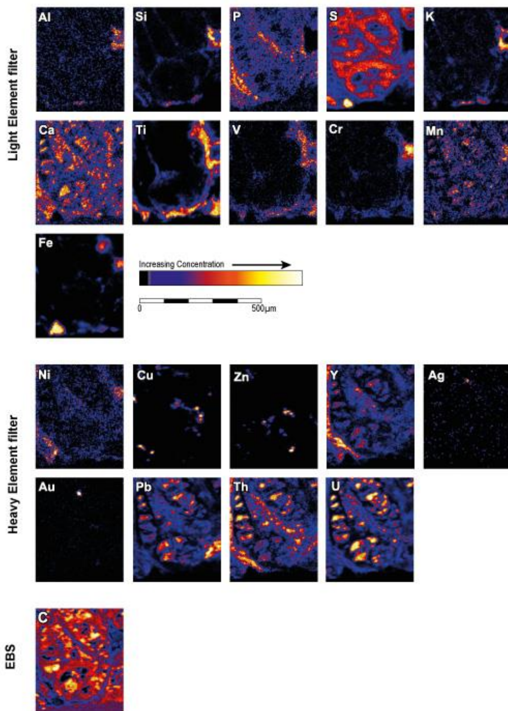
Figure 4.8 PIXE elemental micro-maps of MGS6513
