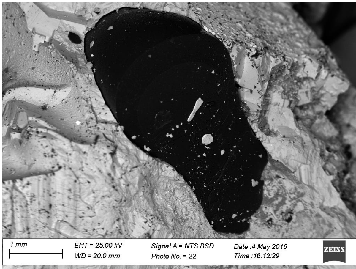
Figure 3.13 Electron Microscope Image of the Carbon Nodule in Recrystallised Pyrite
