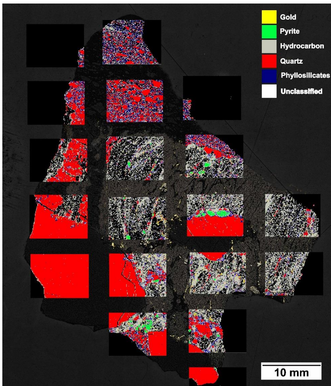
Figure 6.6 Mineral classification of CLR sample as shown by Auto-SEM-EDS
