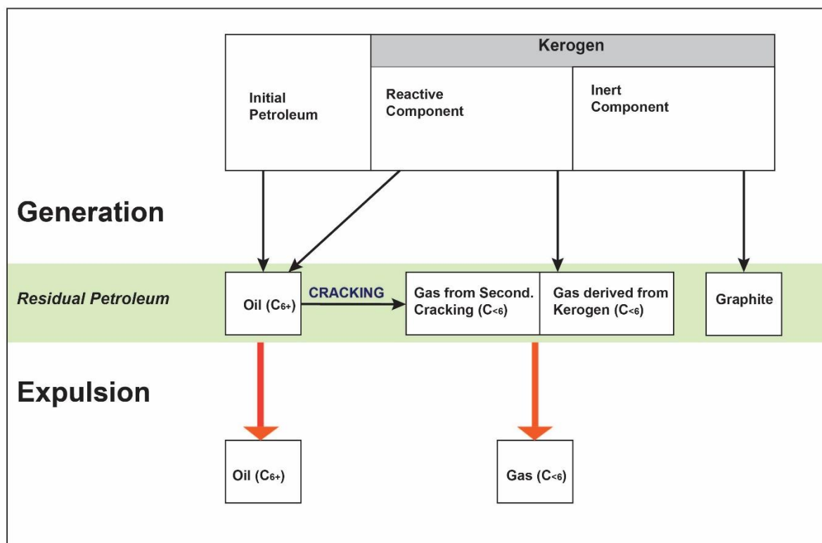
Figure 1.4 Schematic Diagram of Petroleum Generation
