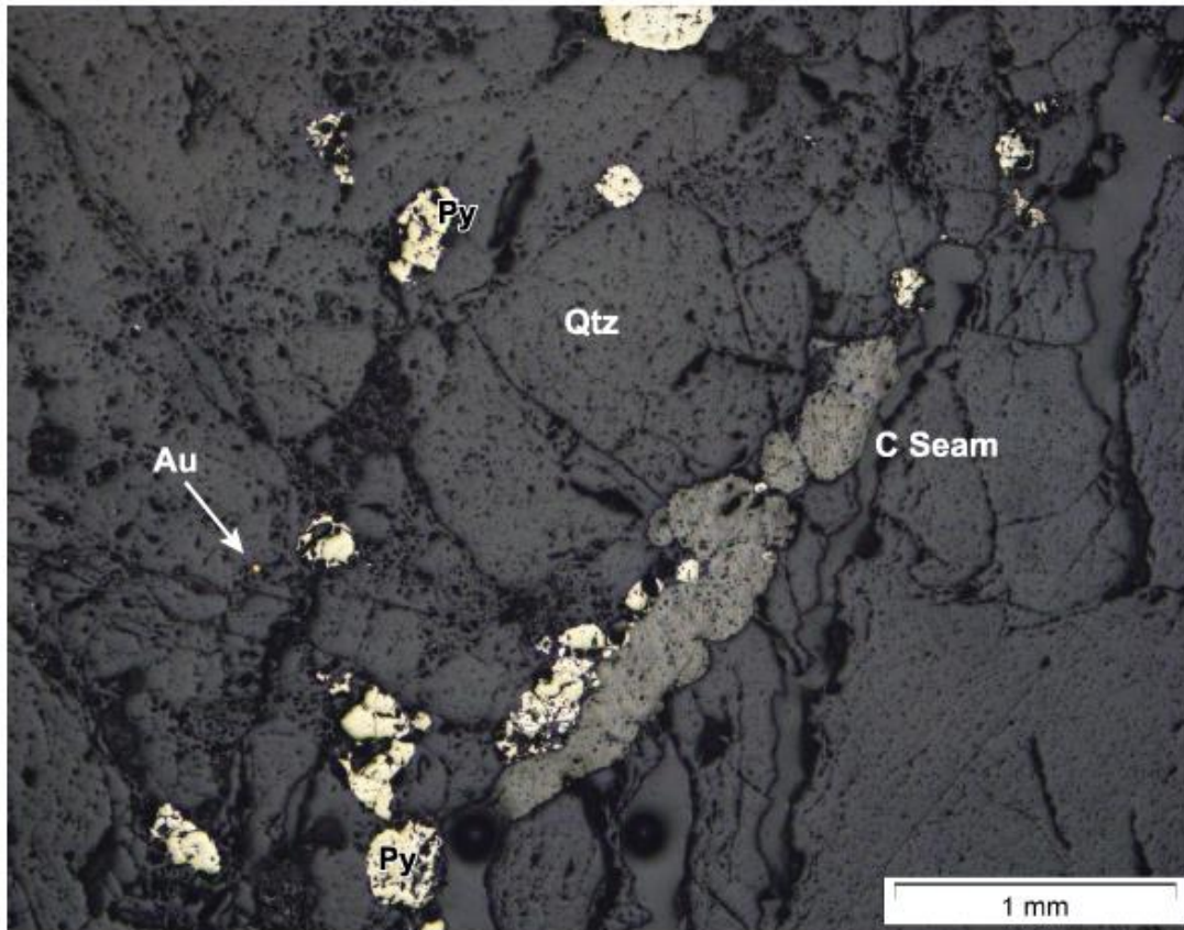
Figure 3.9 Reflected light image of a thin discontinuous carbon seam in CREEF07
