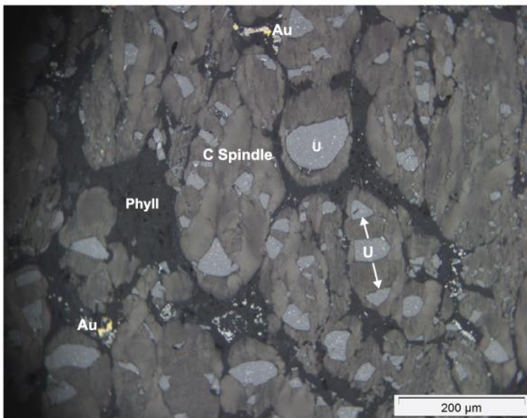
Figure 3.2 Reflected light image of carbon seam spindles containing “blown-up” uraninite in CREEF EM1
