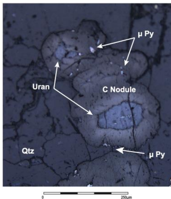
Figure 4.9 Reflected light image of carbon nodules encapsulating rounded uraninite in PSGM
