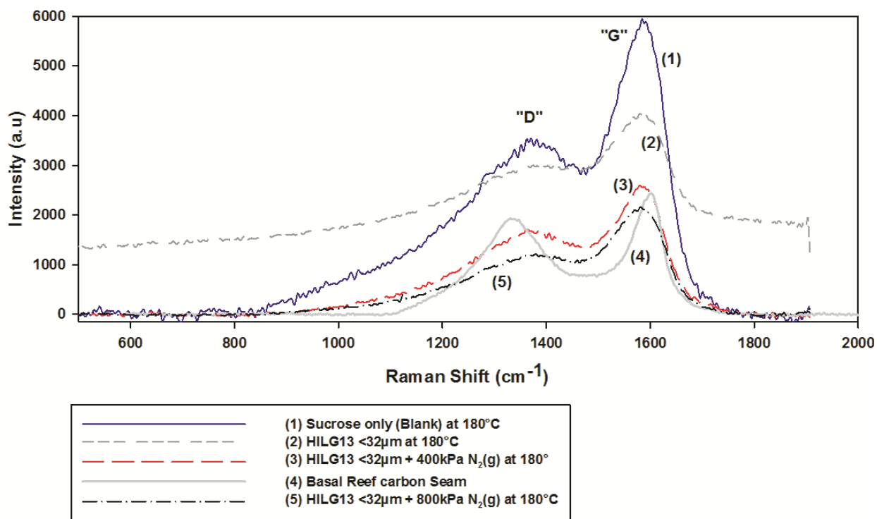
Figure 7.2 Raman spectra of the solvothermal products compared to Witwatersrand Carbon seam
