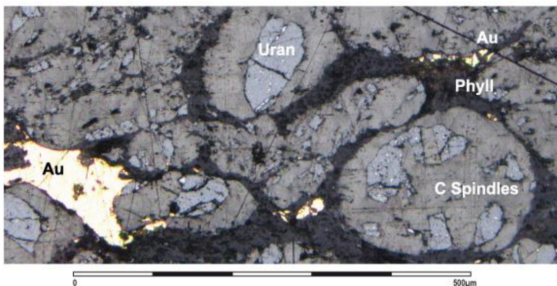
Figure 4.1 Reflected light image of carbon spindles and gold analysed in CREEF01
