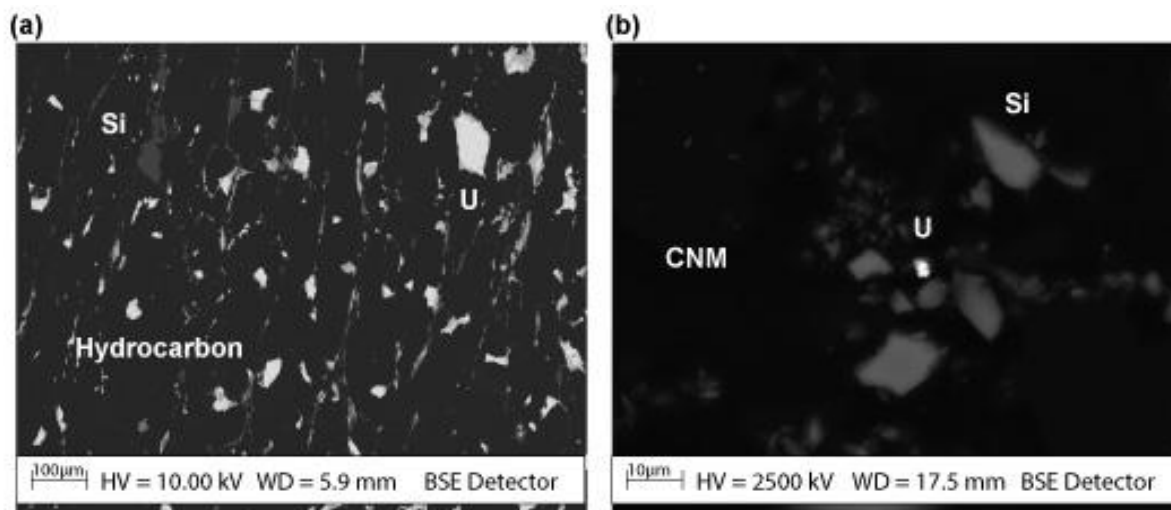
Figure 5.10 SEM Images of Beisa Reef compared to CCVD sample
