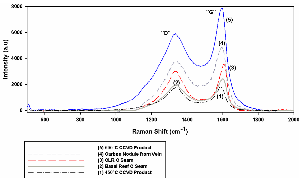
Figure 5.6 Raman spectra of the CCVD experimental products and Witwatersrand Carbon samples
