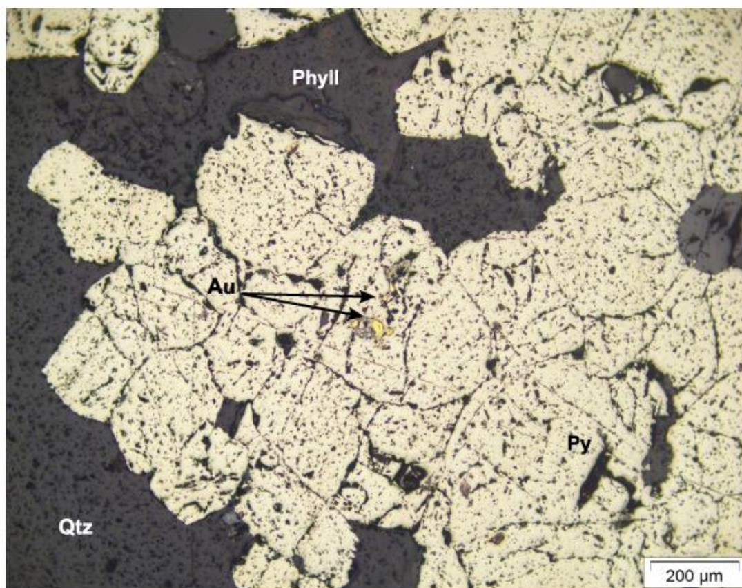
Figure 3.5 Reflected light image of gold within euhedral pyrite in MGS6514
