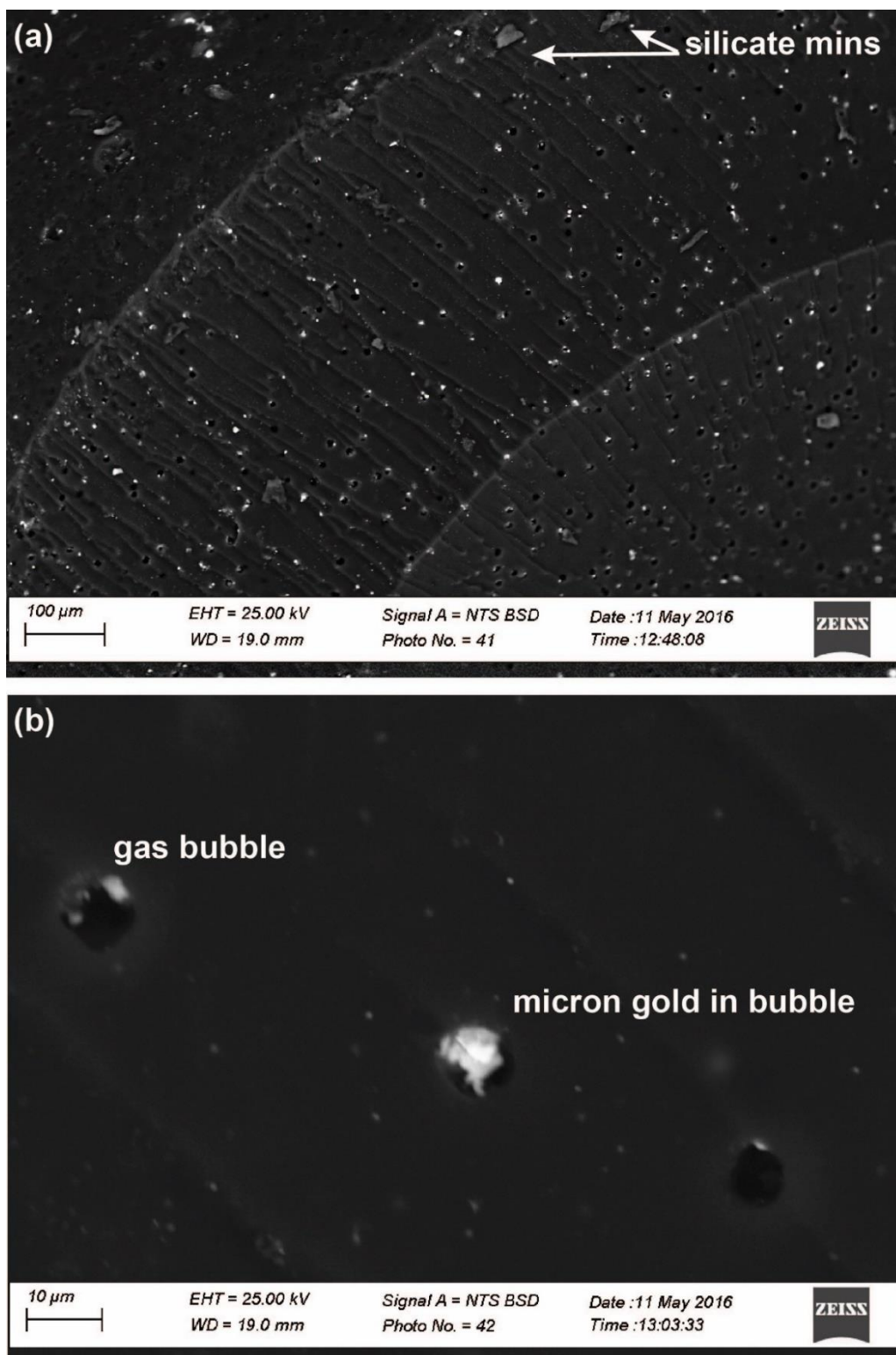
Figure 3.14 Electron Microscope Image showing the micron-scale inclusions of minerals
