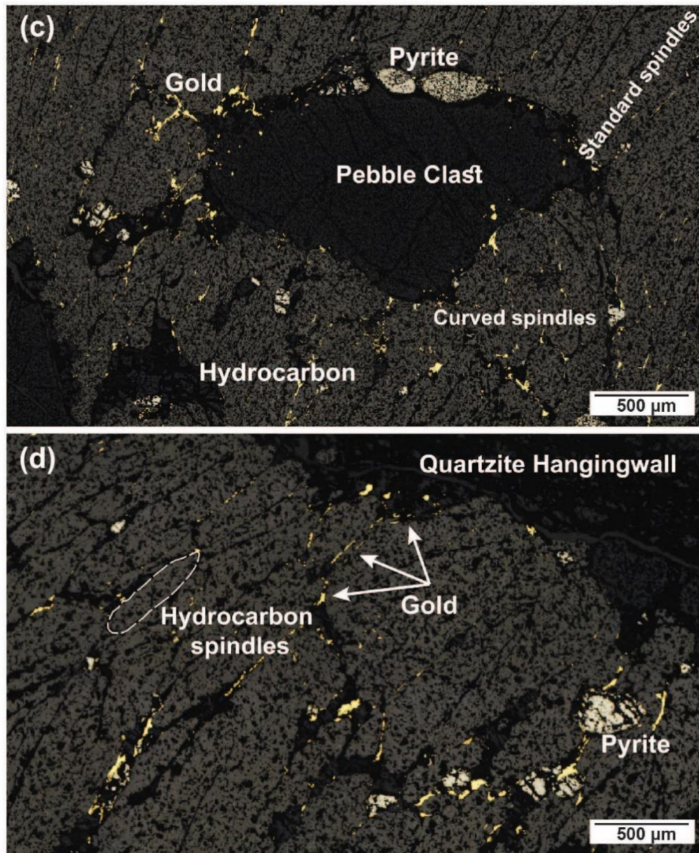
Figure 6.3 continued Enlarged reflected light images of CLR sample features
