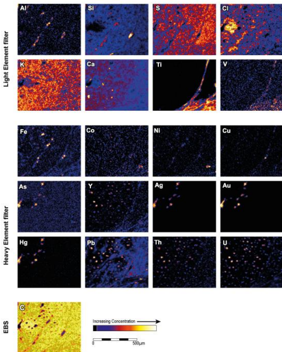
Figure 4.6 PIXE elemental micro-maps of LGM3
