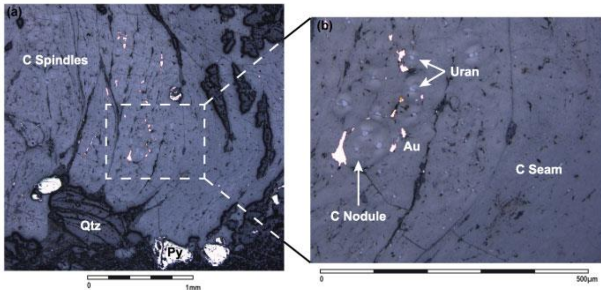
Figure 4.5 Reflected light image of elongated carbon spindles in LGM3
