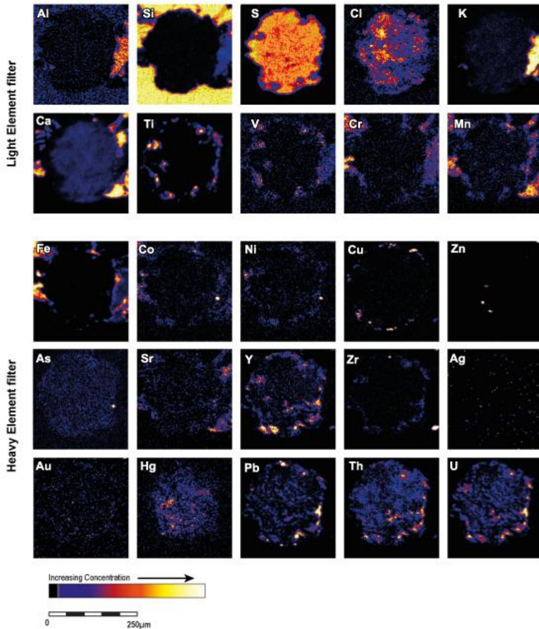
Figure 4.12 PIXE elemental micro-maps of a carbon nodule from the VCR
