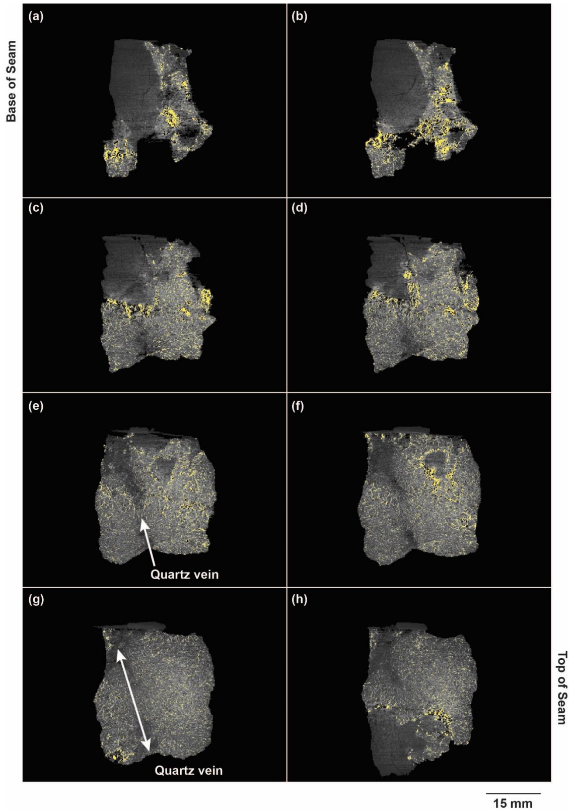
Figure 6.8. Tomography slices through CLR sample. The slices are taken from the base of the seam (a) moving up towards the quartzite hanging wall (h).
