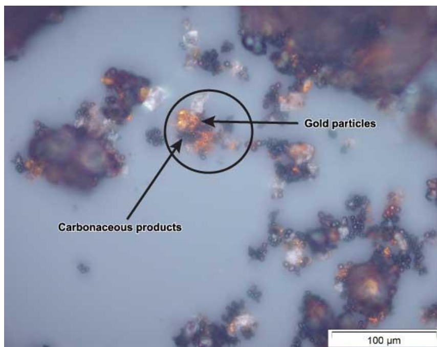
Figure 7.7 Optical microscope image of the solvothermal products formed from the gold in solution solvothermal experiment
