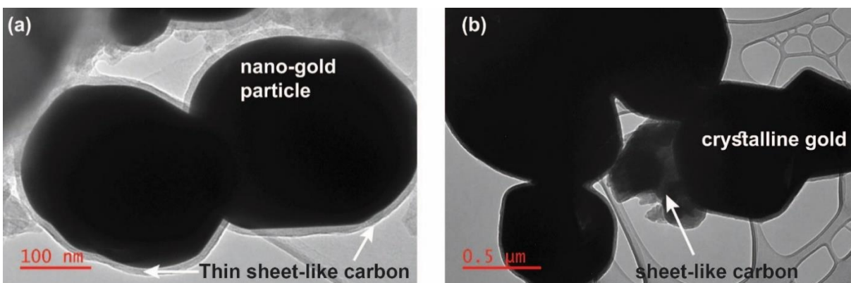
Figure 7.8 TEM images of gold products precipitated from a gold solution
