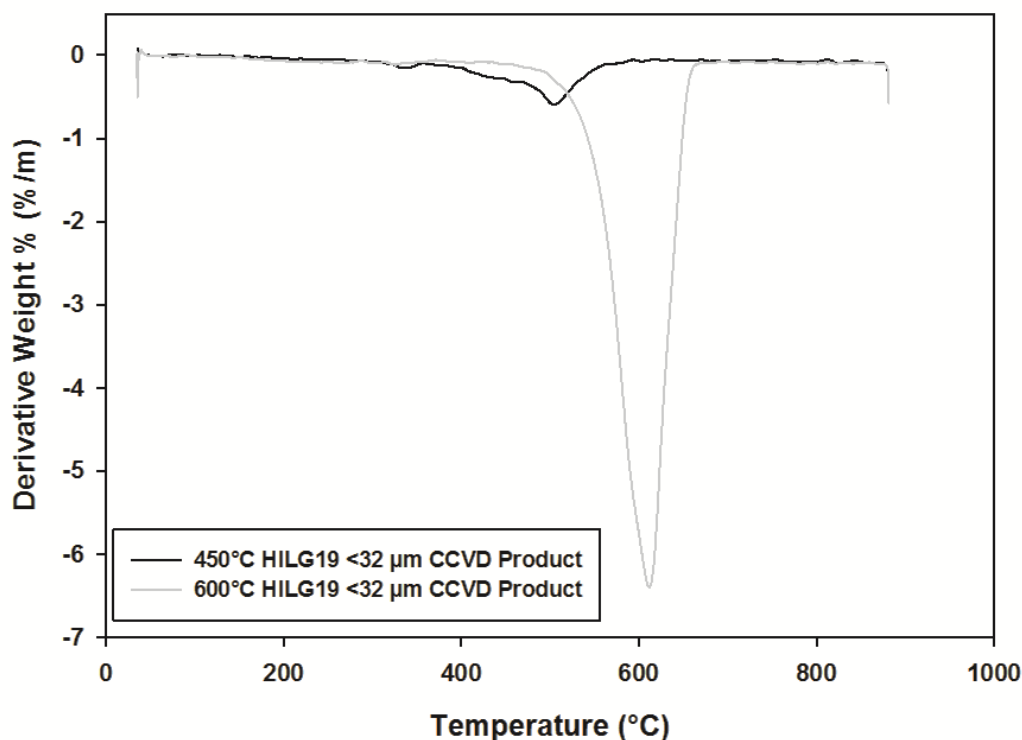
Figure 5.7 The first derivative curve of the TGA analysis of the CCVD products (for HILG19 powders <32 \mu\text{m} ) from 450°C and 600°C experiments
