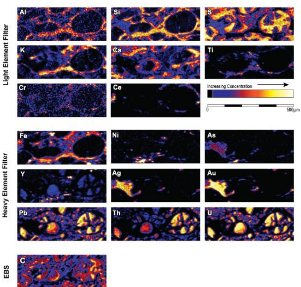
Figure 4.2 PIXE elemental micro-maps of CREEF01
