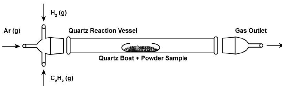
Figure 2.1 CCVD experimental set-up.
