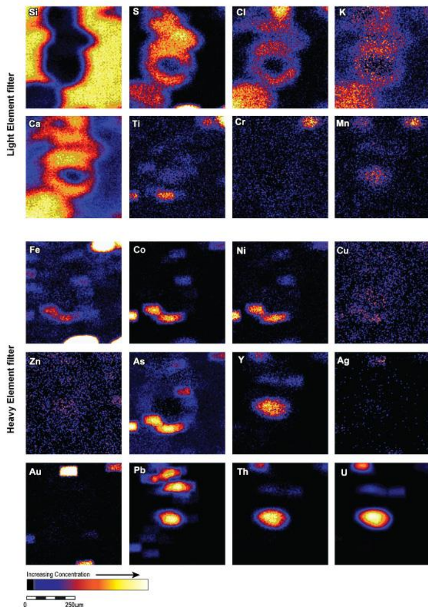
Figure 4.10 PIXE elemental micro-maps of PSGM
