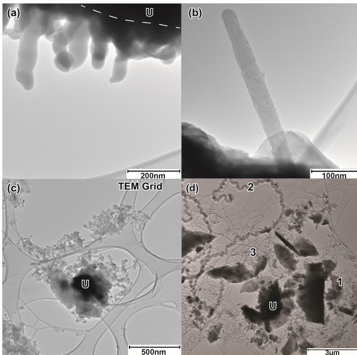
Figure 5.8 TEM micrographs of the CNSs that formed in the CCVD experiments
