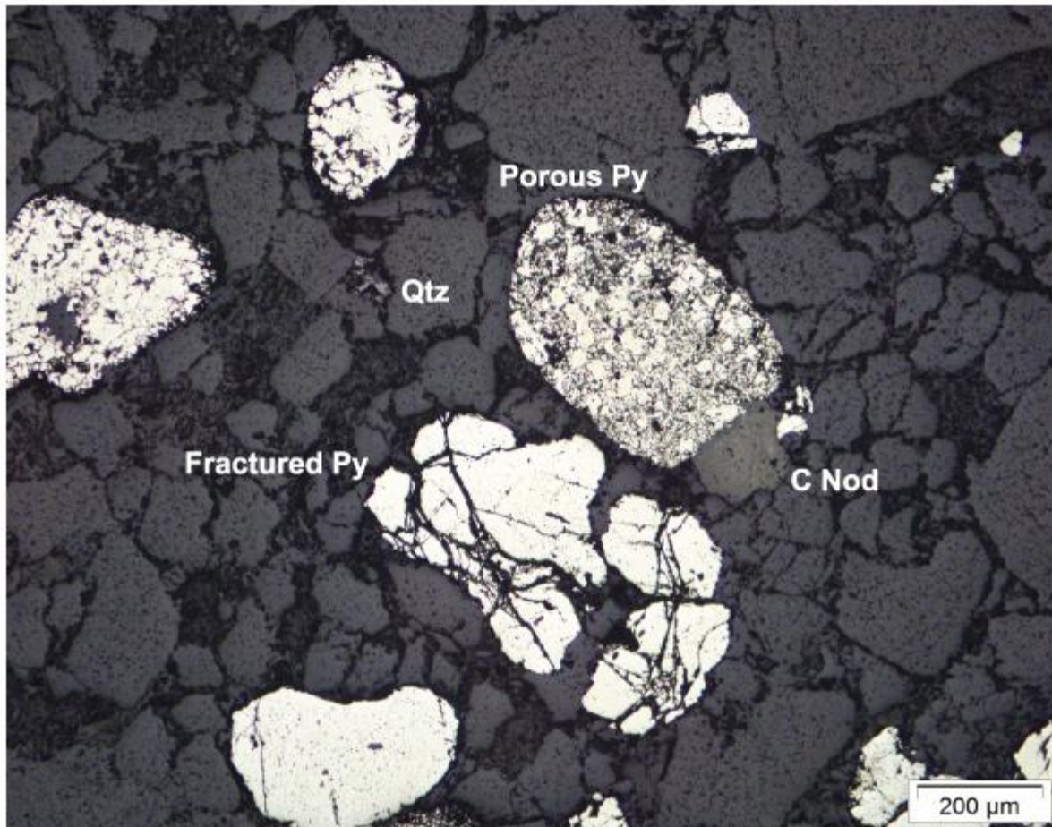
Figure 3.16 Reflected light image of typical rounded pyrite textures in LGM6
