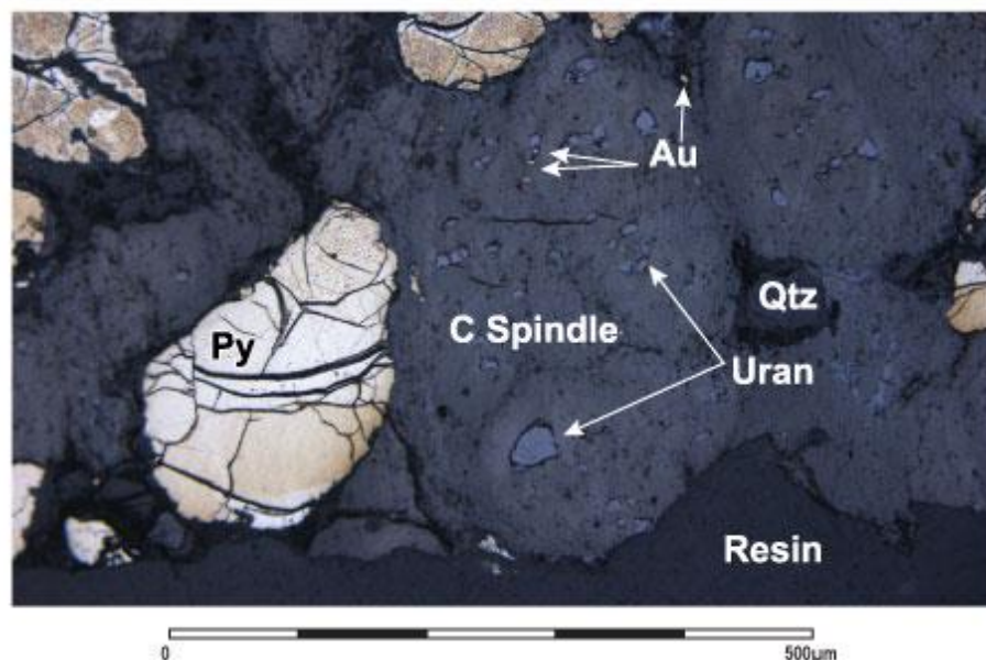
Figure 4.7 Reflected light image of rounded carbon spindles formed around pyrite in MGS6513
