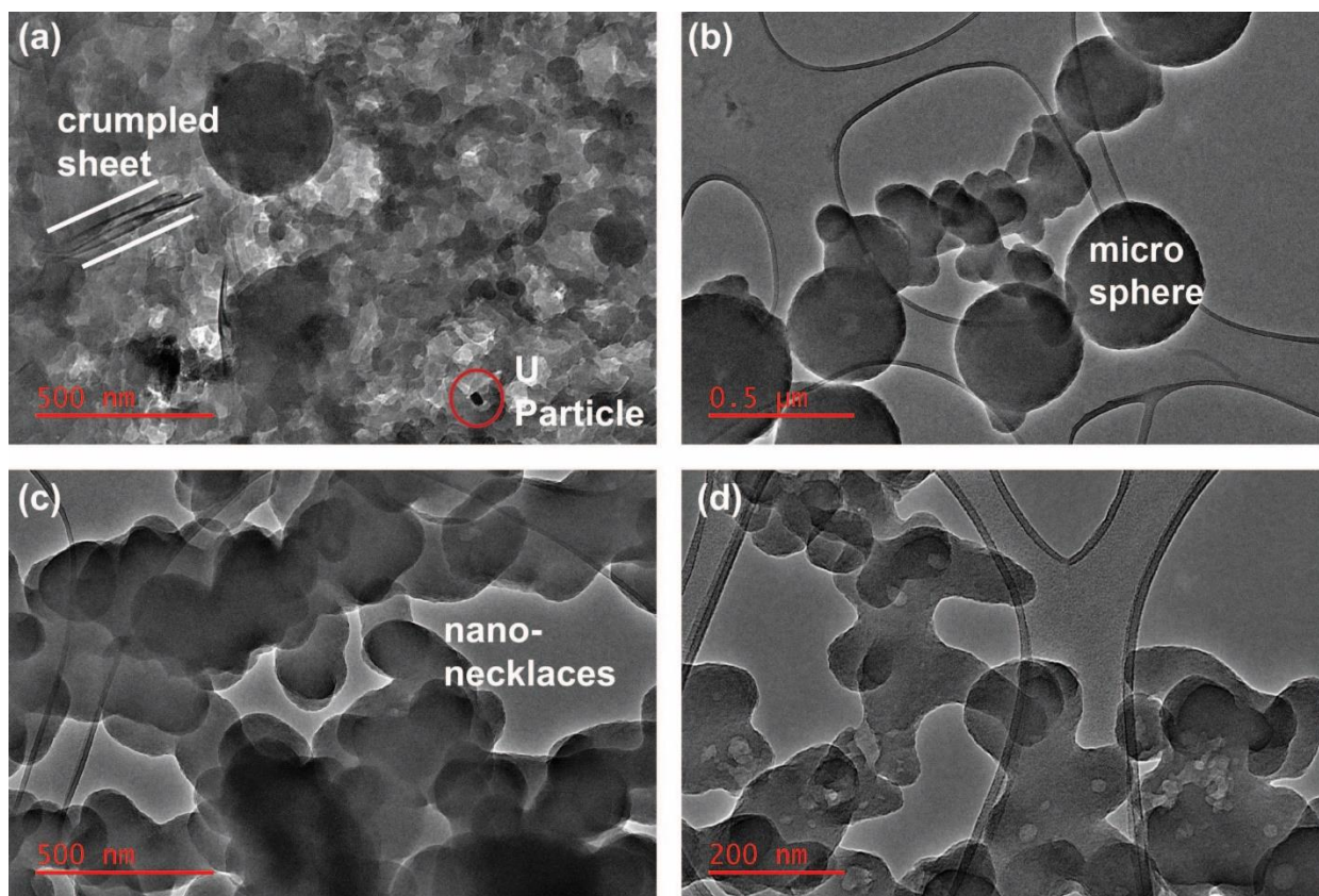
Figure 7.5 TEM of Solvothermal products formed on HILG13 32-75μm powders
