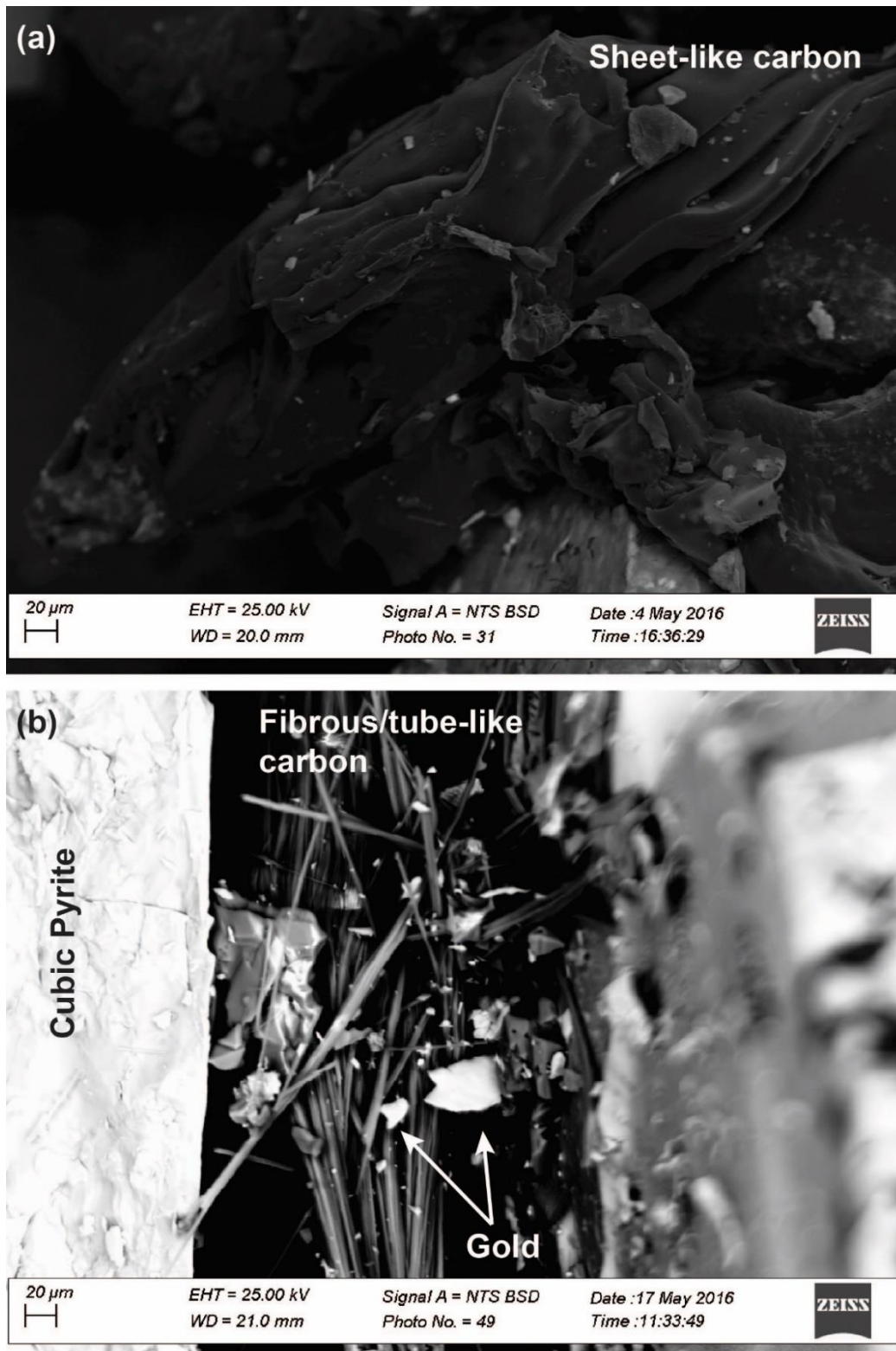
Figure 3.15 Electron Microscope Image showing the micron forms of carbonaceous materials
