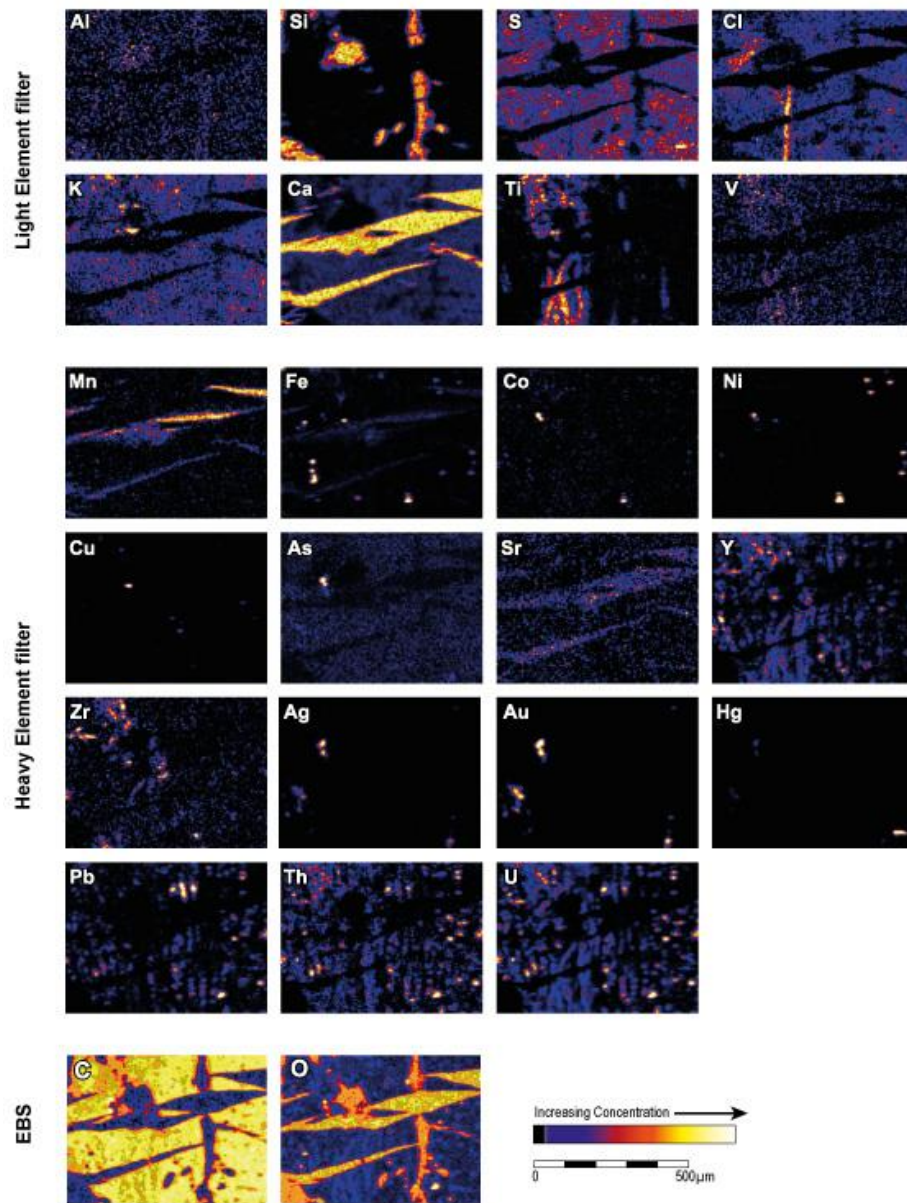
Figure 4.4 PIXE elemental micro-maps of DFN10
