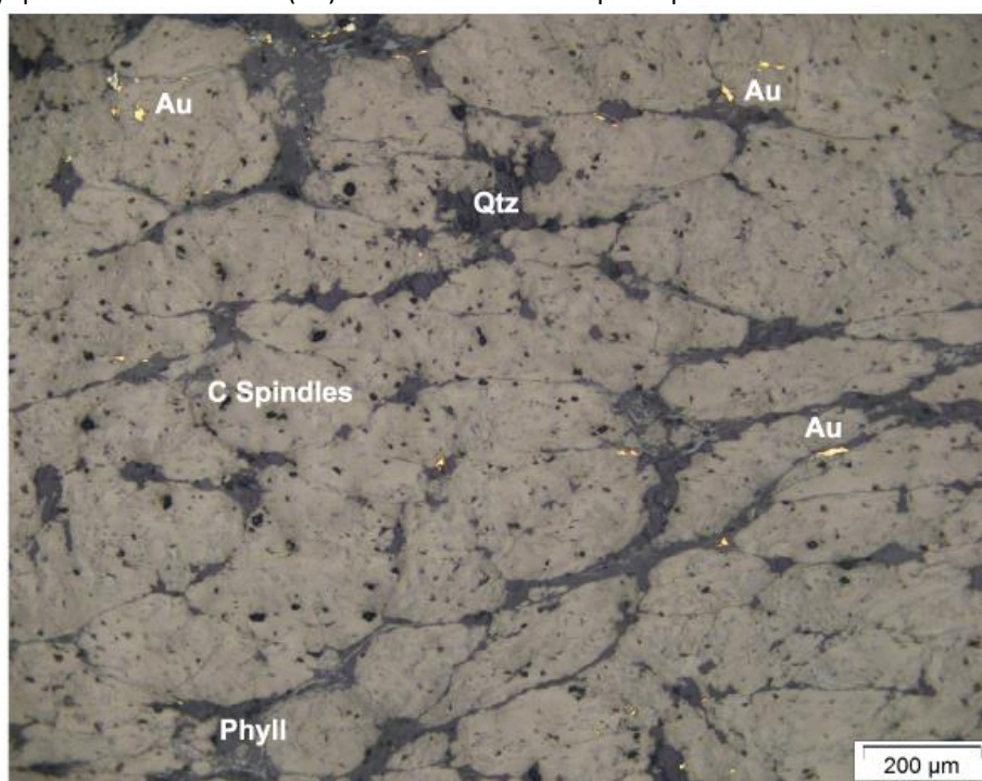
Figure 3.12 Reflected light image of carbon seam spindles with less U and no calcite veins in DFN10
