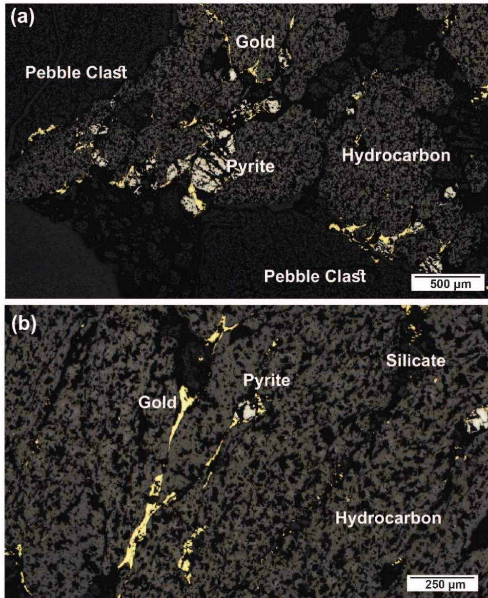
Figure 6.3 Enlarged reflected light images of CLR sample features
