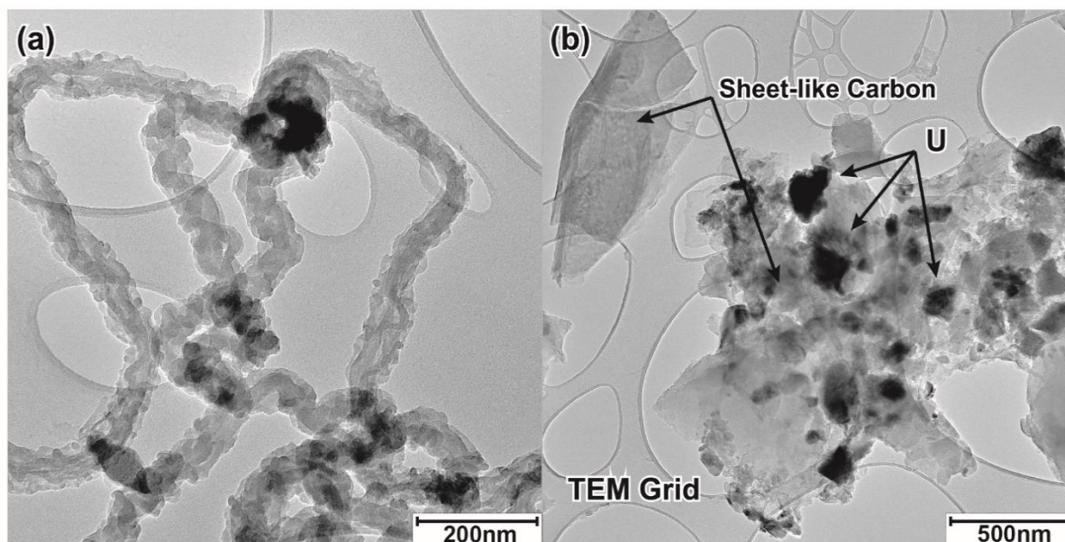
Figure 5.9 Additional TEM micrographs of the CNSs that formed in the CCVD experiments
