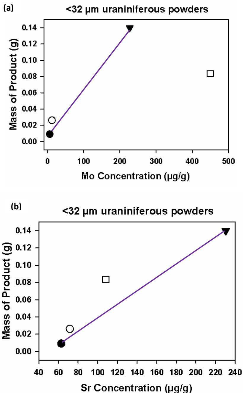
Figure 5.5 The mass of product formed during the CCVD reaction with <32 \mu\text{m} uraniferous powders at 600°C, versus the concentration of (a) Molybdenum and (b) Strontium. The fitted line demonstrates the observed trend if the HILG19 data, a statistical outlier is considered separately.
