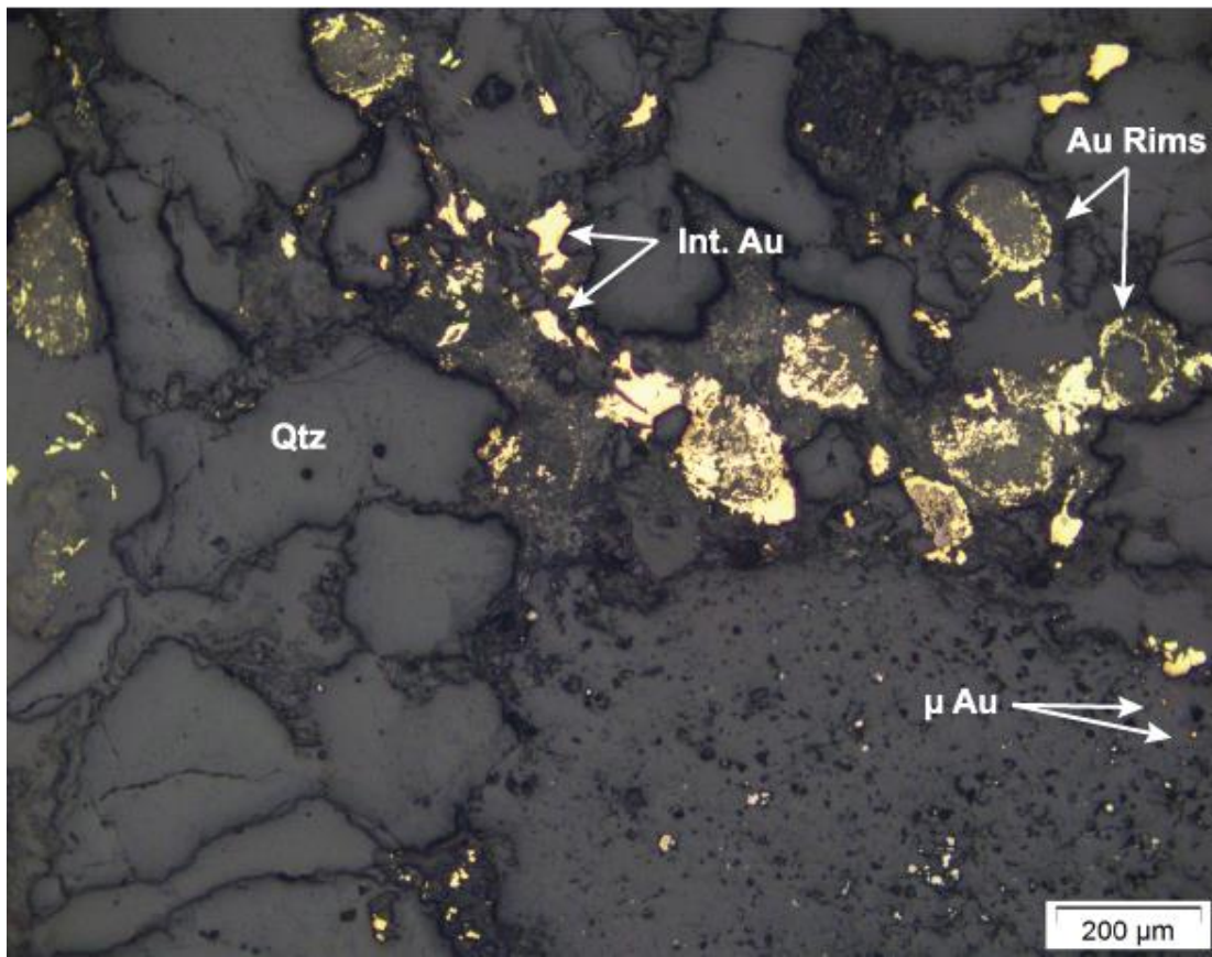
Figure 3.6 Reflected light image of various gold forms in MGS4071
