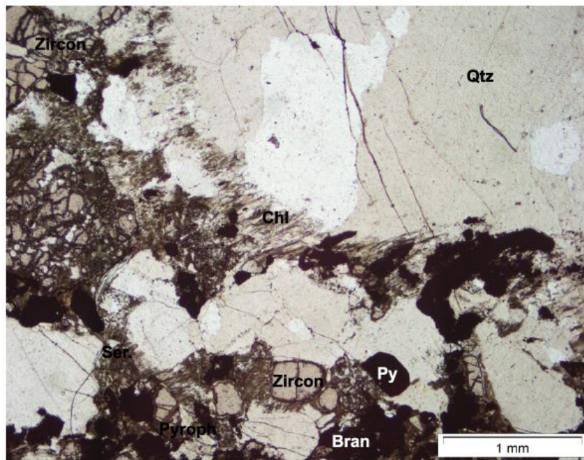
Figure 3.20 Transmitted light image of alteration minerals within matrix of BDN2
