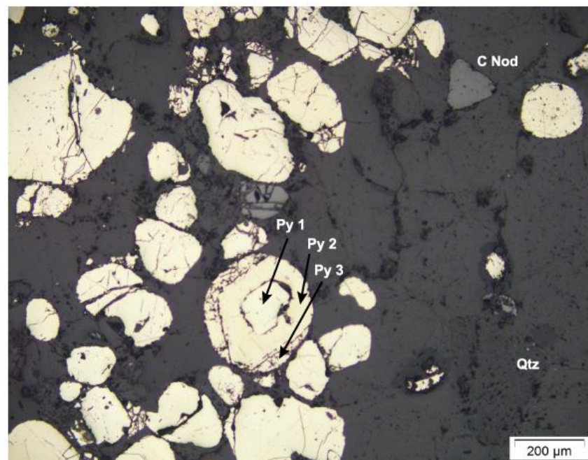
Figure 3.18 Reflected light image of multiple pyrite forms in a single grain in MGS6513
