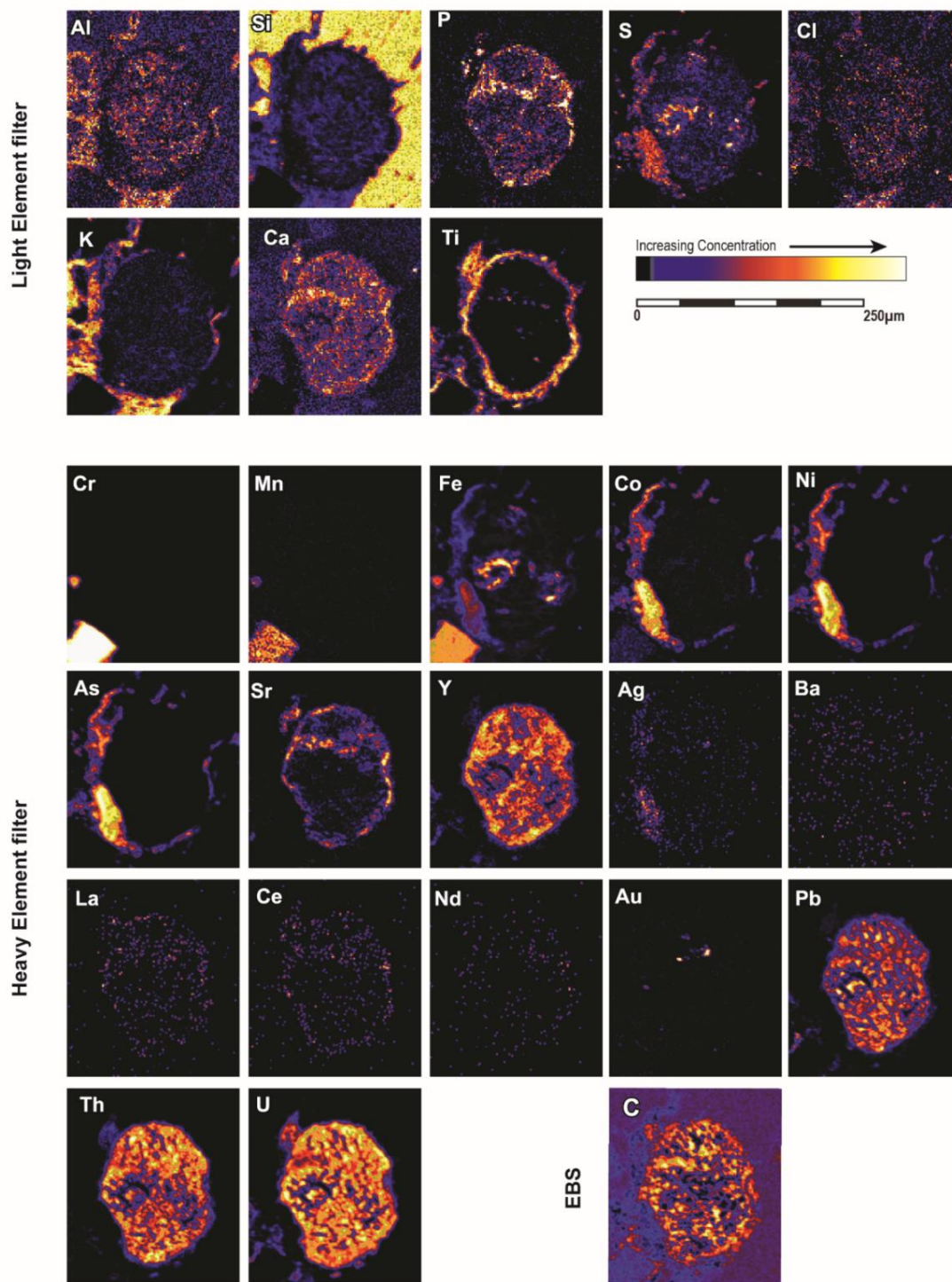
Figure 4.14 PIXE elemental micro-maps of “C” – Reef nodule
