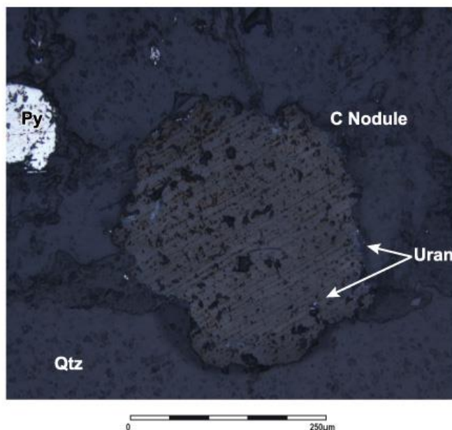
Figure 4.11 Reflected light image of carbon nodule in the VCR1
