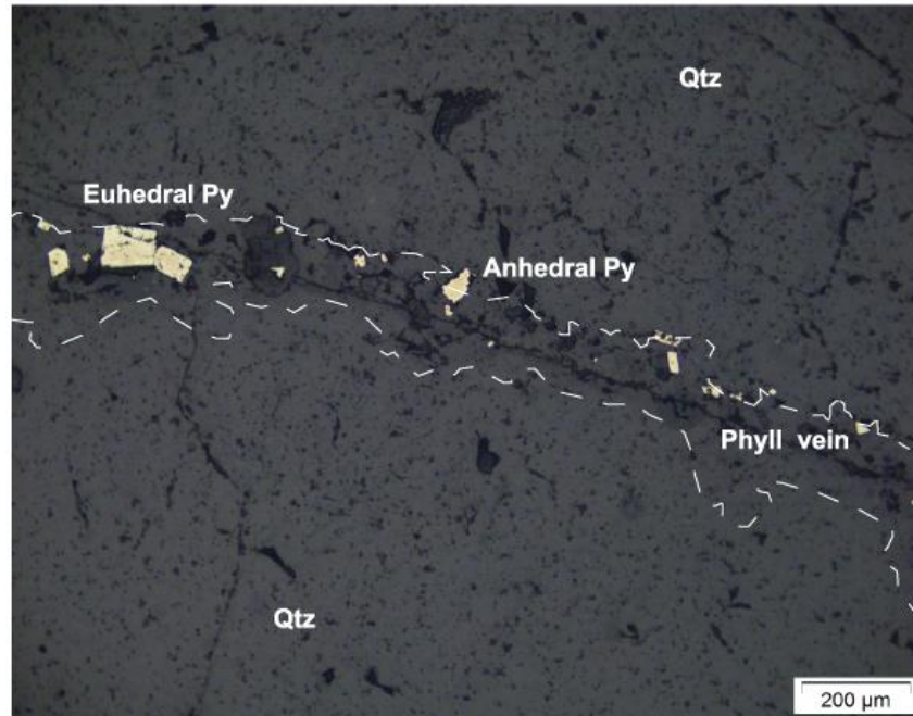
Figure 3.17 Reflected light image of euhedral pyrite within a phyllosilicate veinlet in LGM16
