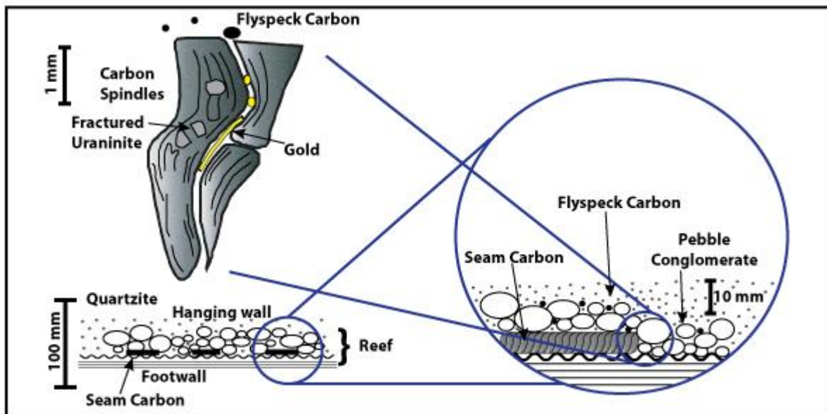
Figure 1.3 Schematic Diagram showing the form of Carbonaceous Matter
