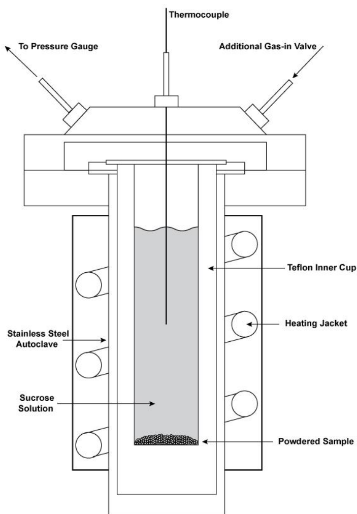
Figure 2.2 Schematic diagram of a solvothermal experimental set-up
