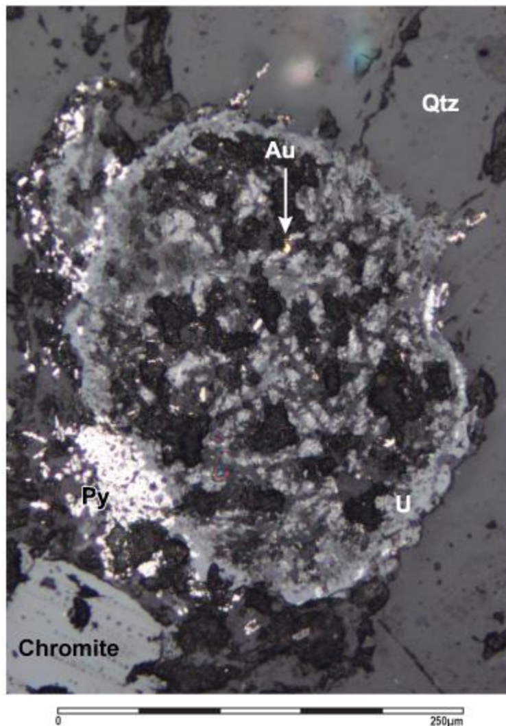
Figure 4.13 Reflected light image of a porous nodule from the "C" = Reef
