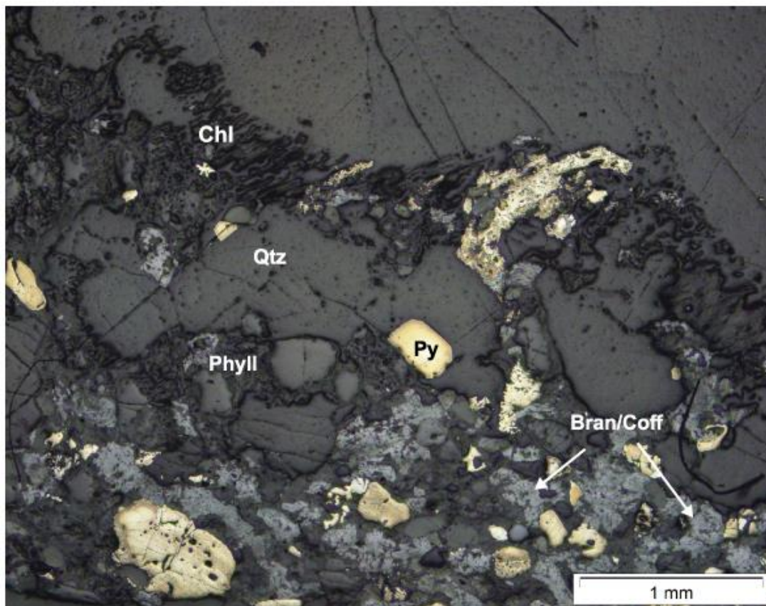
Figure 3.1 Reflected light image of secondary phases of brannerite and coffinite minerals in BDN2
