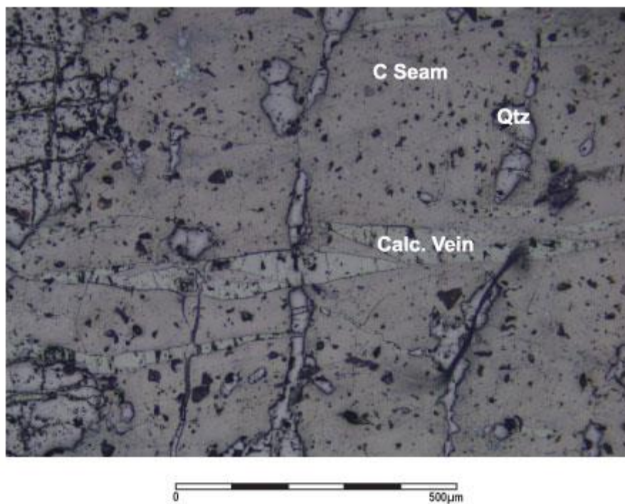
Figure 4.3 Reflected light image of carbon seam cut by calcite veinlets in DFN10
