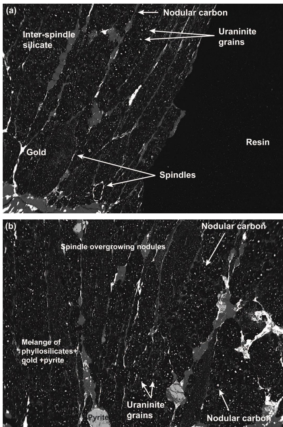
Figure 6.5 BSE image of seam portion of CLR sample
