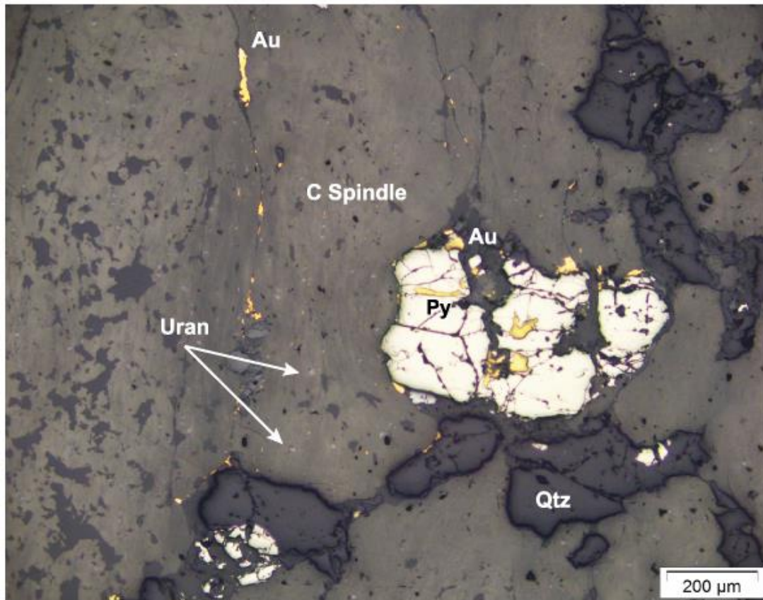
Figure 3.10 Reflected light image of carbon spindles with gold between the filaments in WD20
