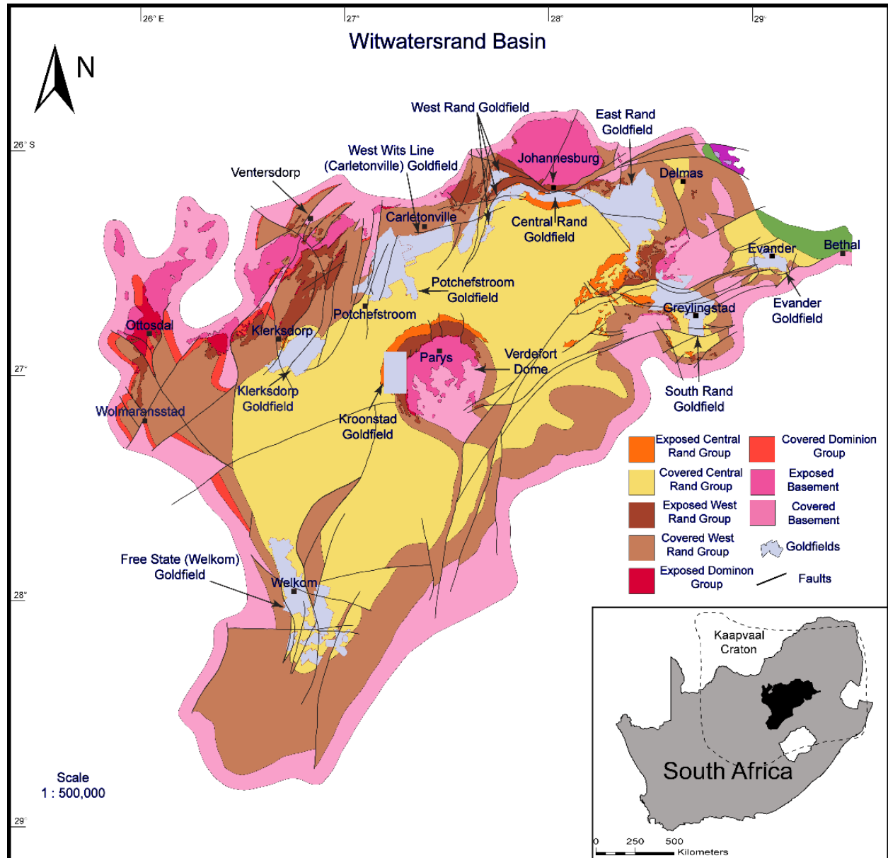
Figure 1.1 Geological Map of the Witwatersrand Basin in South Africa
