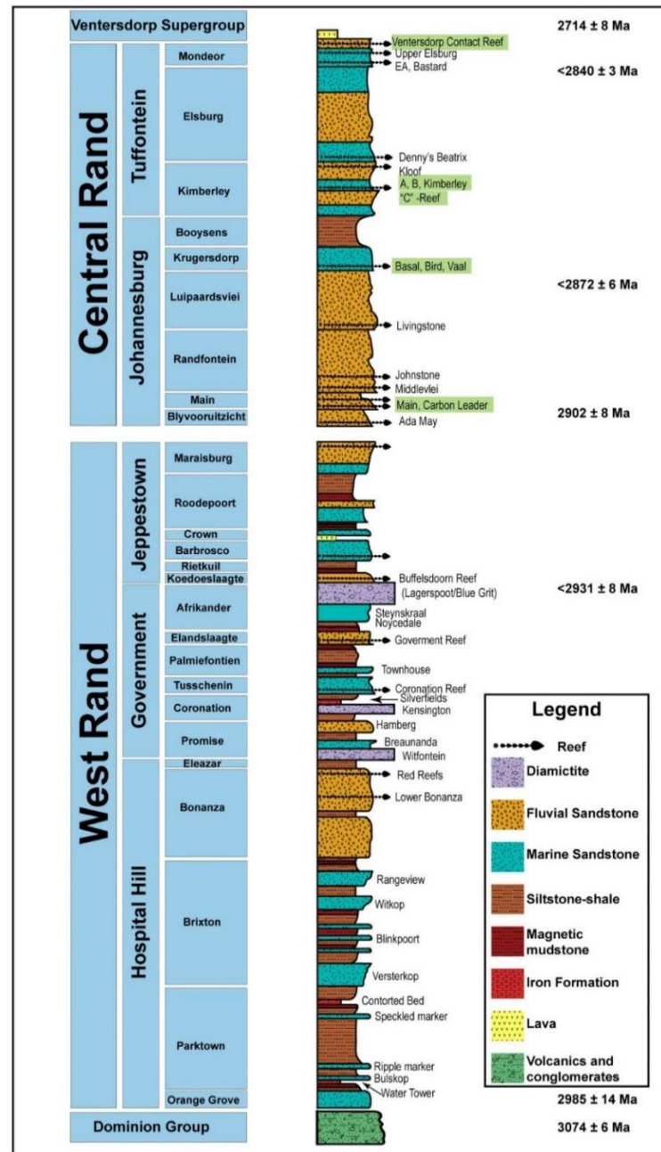
Figure 1.2 Stratigraphic Column of the Witwatersrand Basin
