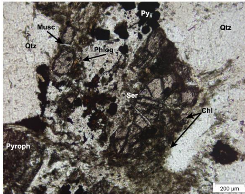
Figure 3.19 Transmitted, plane-polarised light image of alteration minerals in BDN2
