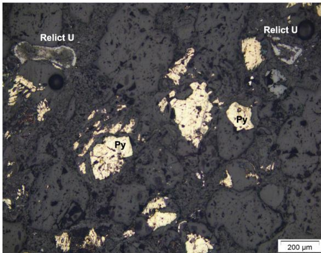
Figure 3.3 Reflected light image of relict uraninite grains in MGS4063
