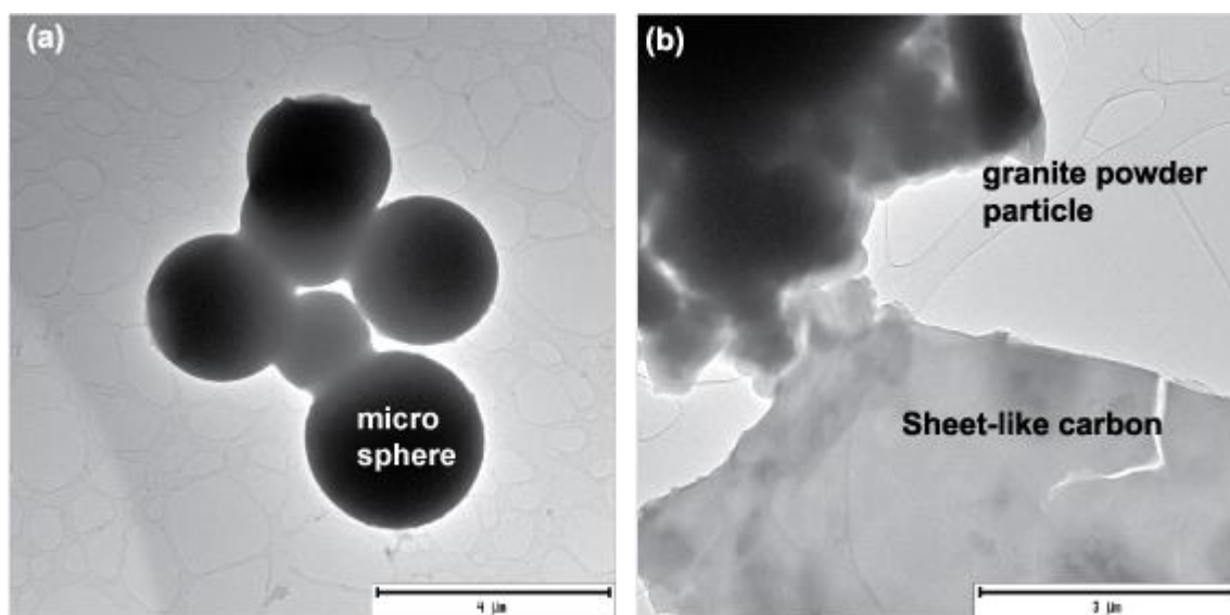
Figure 7.4 TEM images of solvothermal products
