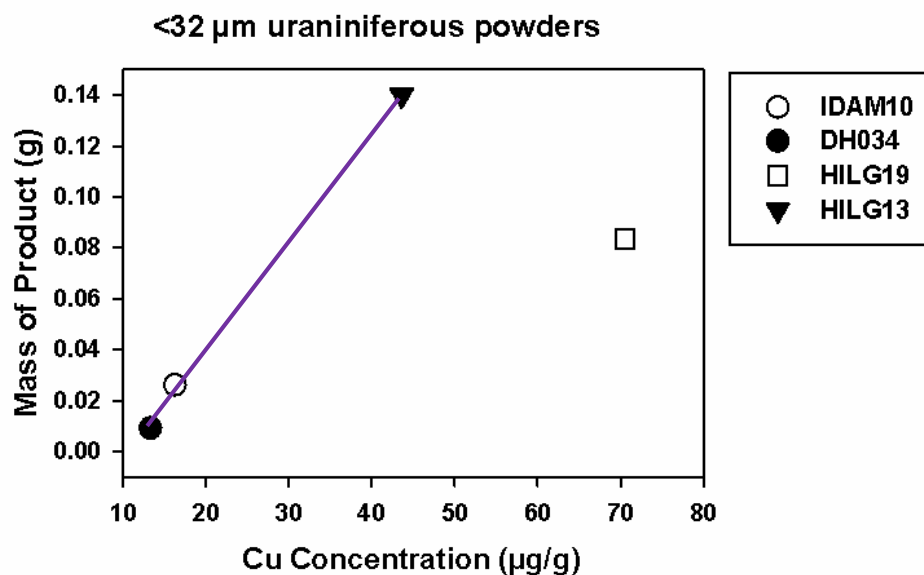
Figure 5.4 The mass of product formed during the CCVD reaction with <32 \mu\text{m} uraniferous powders at 600°C, versus the concentration of Copper. The fitted line demonstrates the observed trend if the HILG19 data, a statistical outlier is considered separately.
