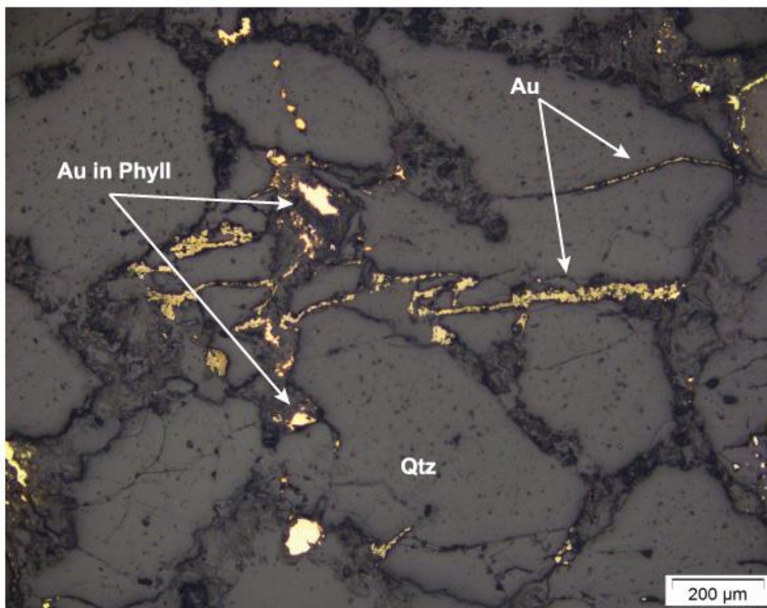
Figure 3.4 Reflected light image of gold in veinlets and phyllosilicate matrix minerals in MGS4071
