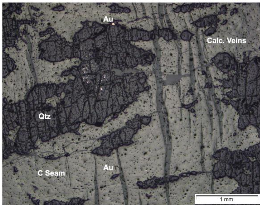
Figure 3.11 Reflected light image of a carbon seam cut by calcite veins in DFN10
