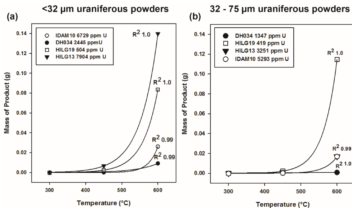
Figure 5.2 The mass of the black product formed during CCVD growth
