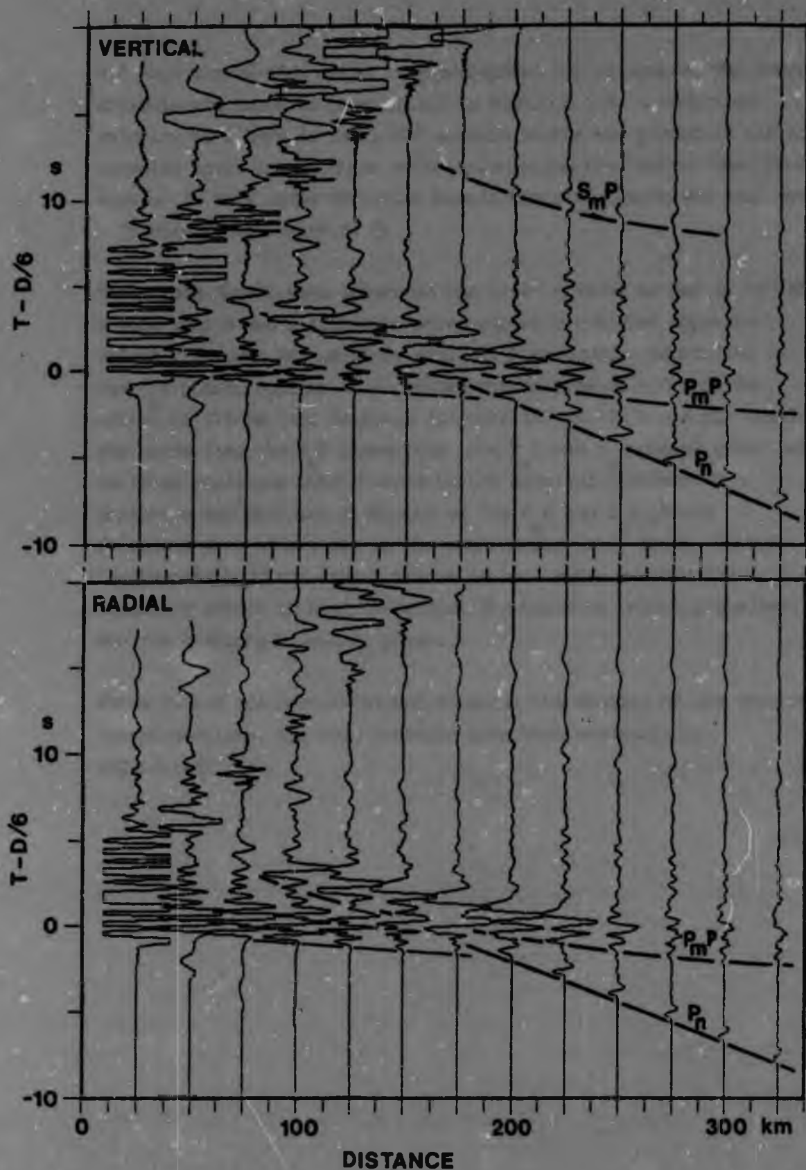
Figure 5.12B. Detail of the P-wave arrivals on the synthetic record section for a 1-D seismic velocity model of the Kaapvaal Craton computed using the reflectivity method.
