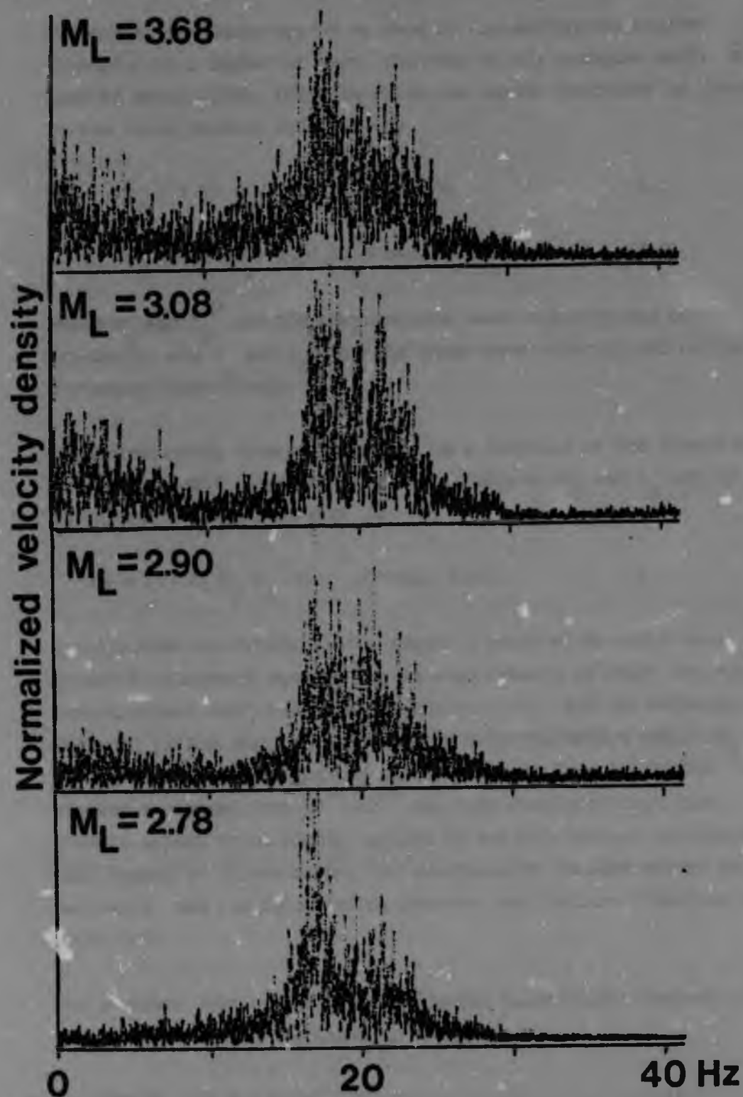
Figure 3.1. Normalized vertical component velocity density spectra of Klerksdorp goldfield tremors recorded at a station in the Vredefort Dome (about 65 km southeast of the source region).
