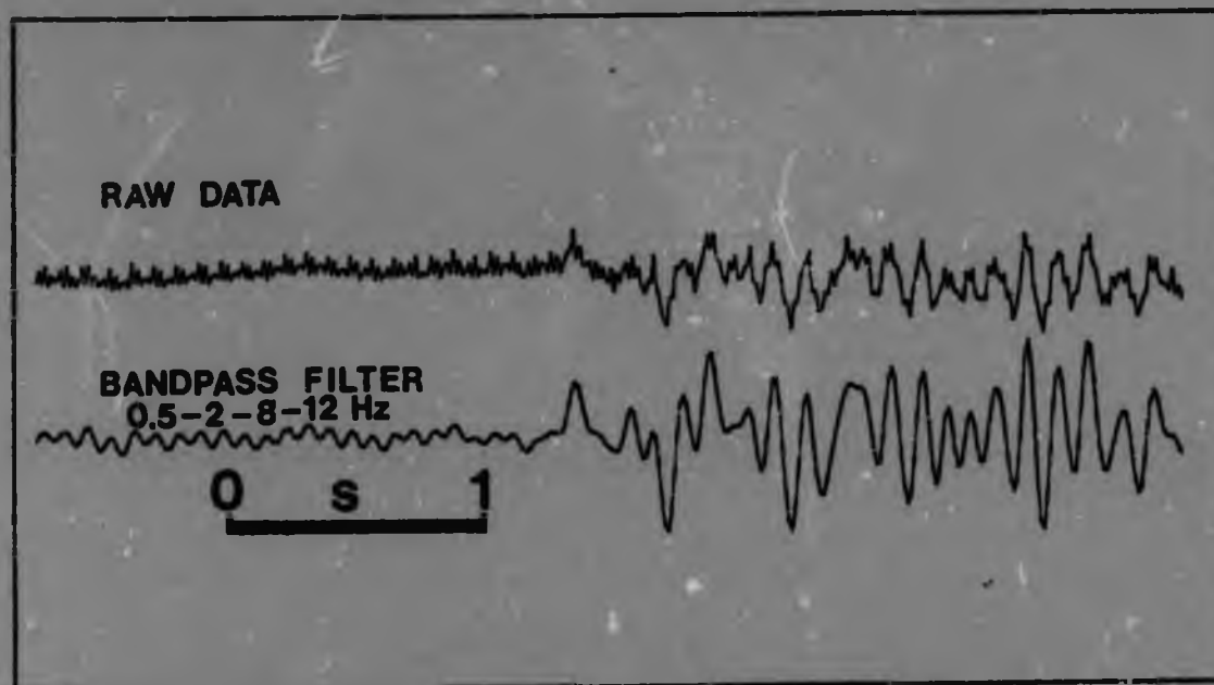
Figure 4.5. Filtration of a noisy seismogram. In this case the bandpass filter has removed high and low frequency noise, but not a noise component in the passband. The filtered trace is plotted with an expanded amplitude scale.
