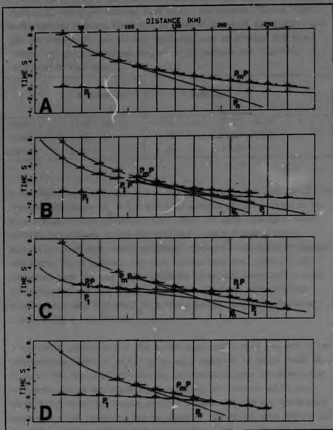
Figure 5.1 Synthetic record sections for simple 1-D models of the seismic velocity structure of the Kaapvaal Craton. (A) single-layer crust, (B) two-layer crust with layer 2 at 28 km, (C) two-layer crust with layer 2 at 14 km, (D) velocity gradient.
