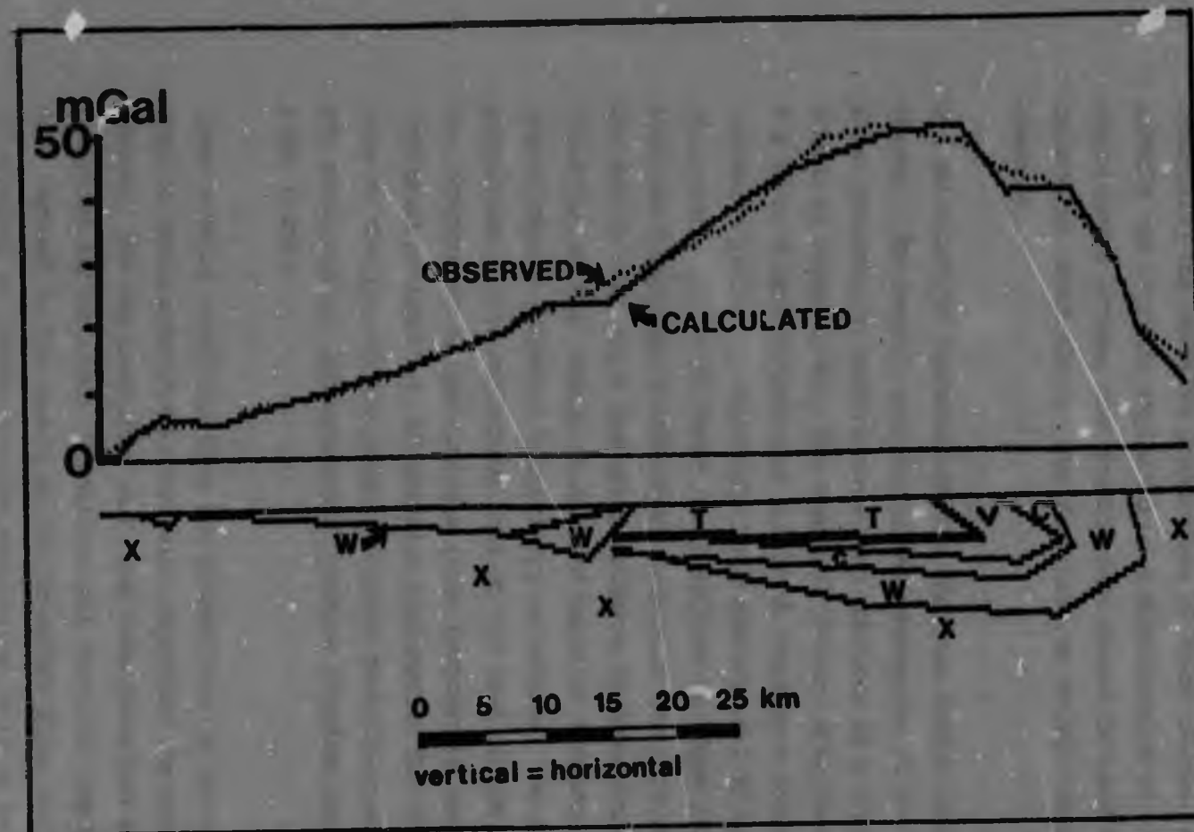
Figure 7.1. 2-D model of the Bouguer gravity anomaly along the trans-Witwatersrand Basin deep seismic reflection profile. The density of the formations with respect to a background of 2.67 \text{ g/cm}^3 is indicated. Geology: X - Basement Complex (0.0), W - Dominion and West Rand Groups (0.2), C - Central Rand Group (0.0), V - Venterdorp Supergroup (0.2), T - Transvaal Sequence (0.22).
