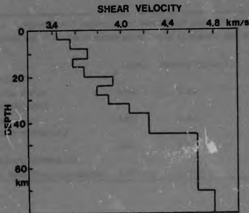
Figure 2.4. Shear wave velocity model for the Kariba-Pretoria path derived by Bloch et al. (1969).
