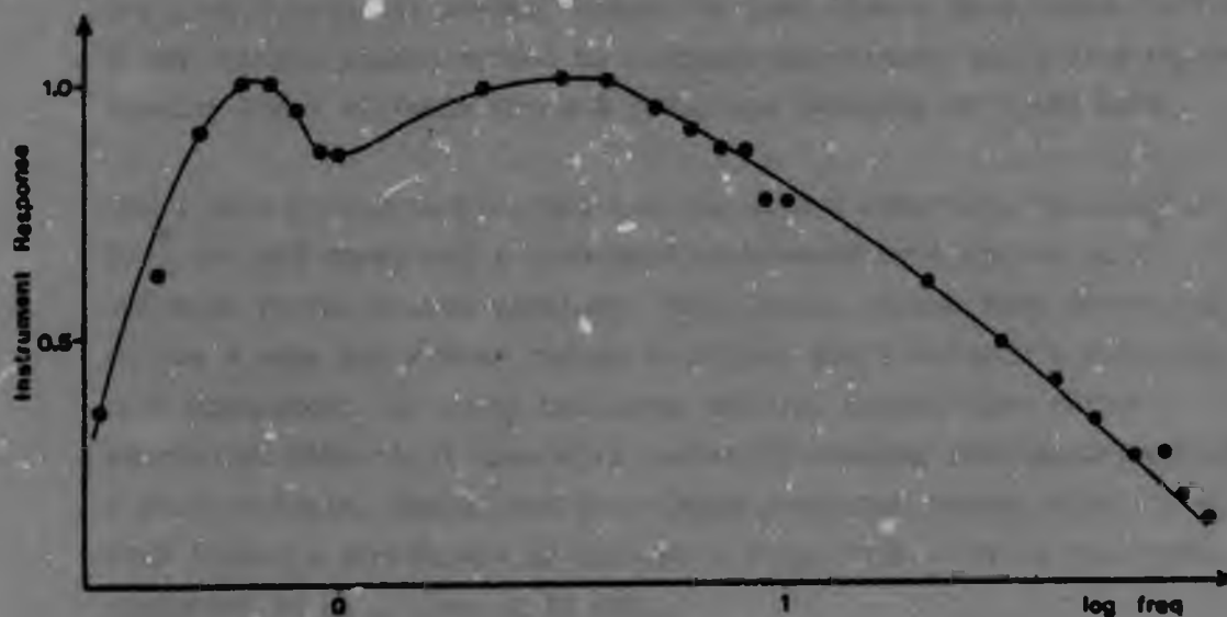
Figure 4.4. Measured velocity amplitude response of the recording system (from Peberdy, 1986).
