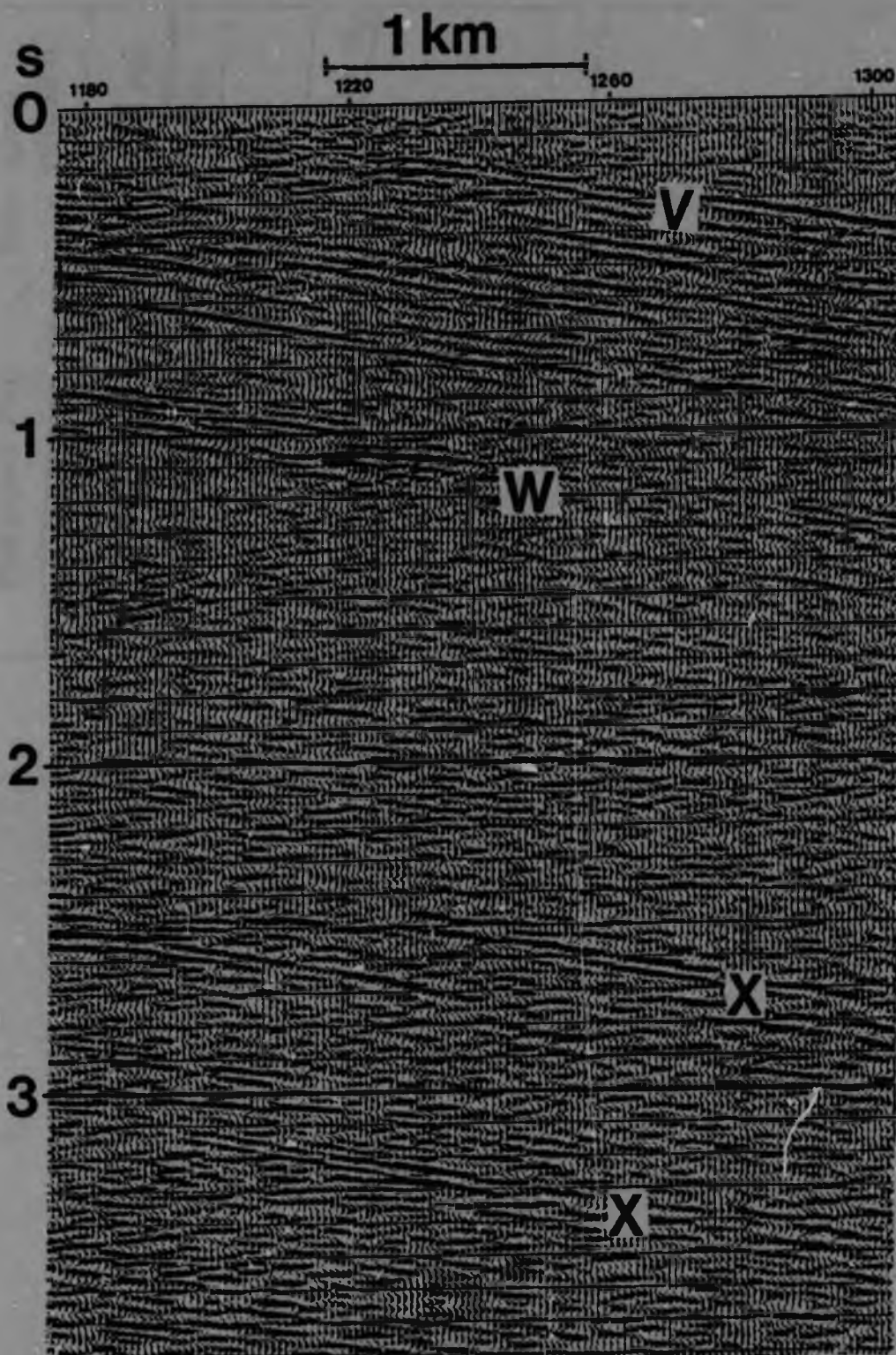
Figure 6.3B. Migrated panel (CDP 1180-1300) from the trans-Witwatersrand Basin deep seismic reflection profile. X - reflectors in the Basement Complex, W - base of Dominion and West Rand Groups, V - base of Ventersdorp Supergroup, M - base of Black Reef Formation and Malmani Subgroup, P - base of Pretoria Group.
