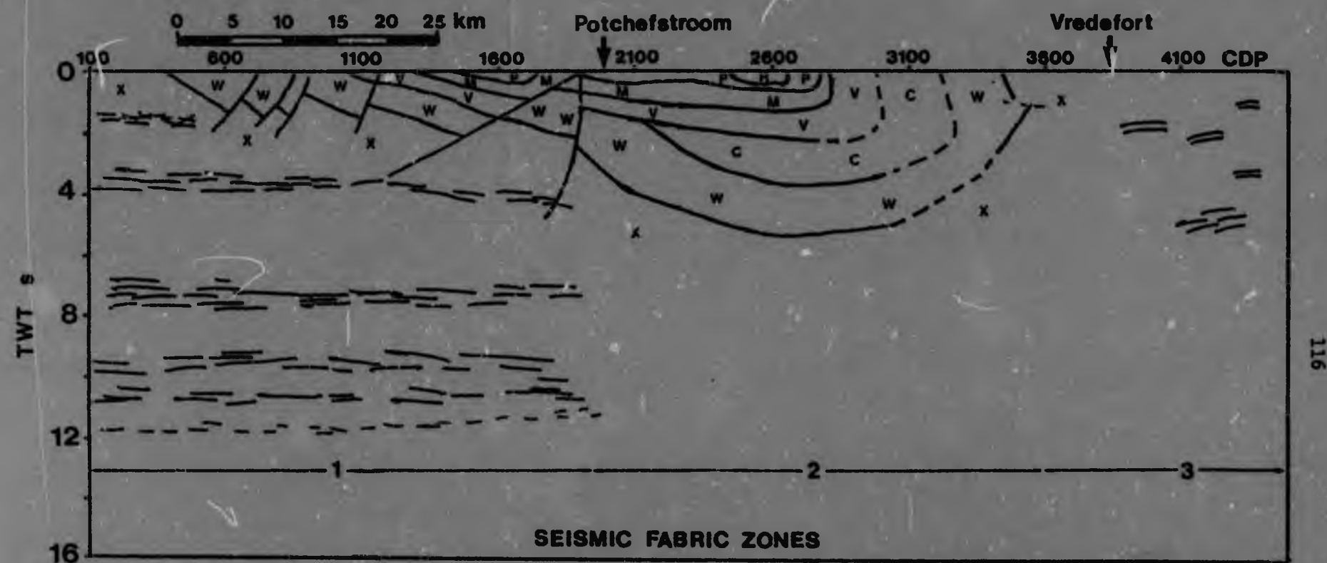
Figure 6.2. Interpretation of the trans-Witwatersrand Basin deep seismic reflection profile. Geology: X - Basement Complex, W - Dominion and West Rand Groups, C - Central Rand Group, V - Ventersdorp Supargroup, M - Black Reef Formation and Malmani Subgroup, P - Pretoria Group, R - Roodokraal Complex.
