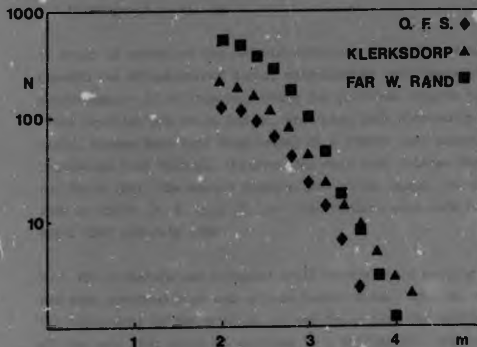
Figure 3.2. Magnitude-frequency distribution for mine tremors in Witwatersrand Basin gold fields for the period January 1985 to May 1988. N(m) —cumulative number of events of magnitude m per year. (Fernandez et al, 1988).
