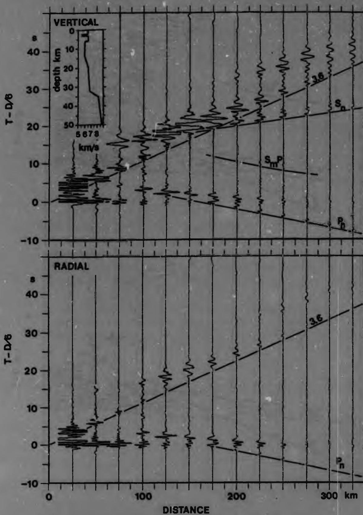
Figure 5.12A. Synthetic record section for a 1-D model of the Karpvaal Craton computed using the reflectivity method.
