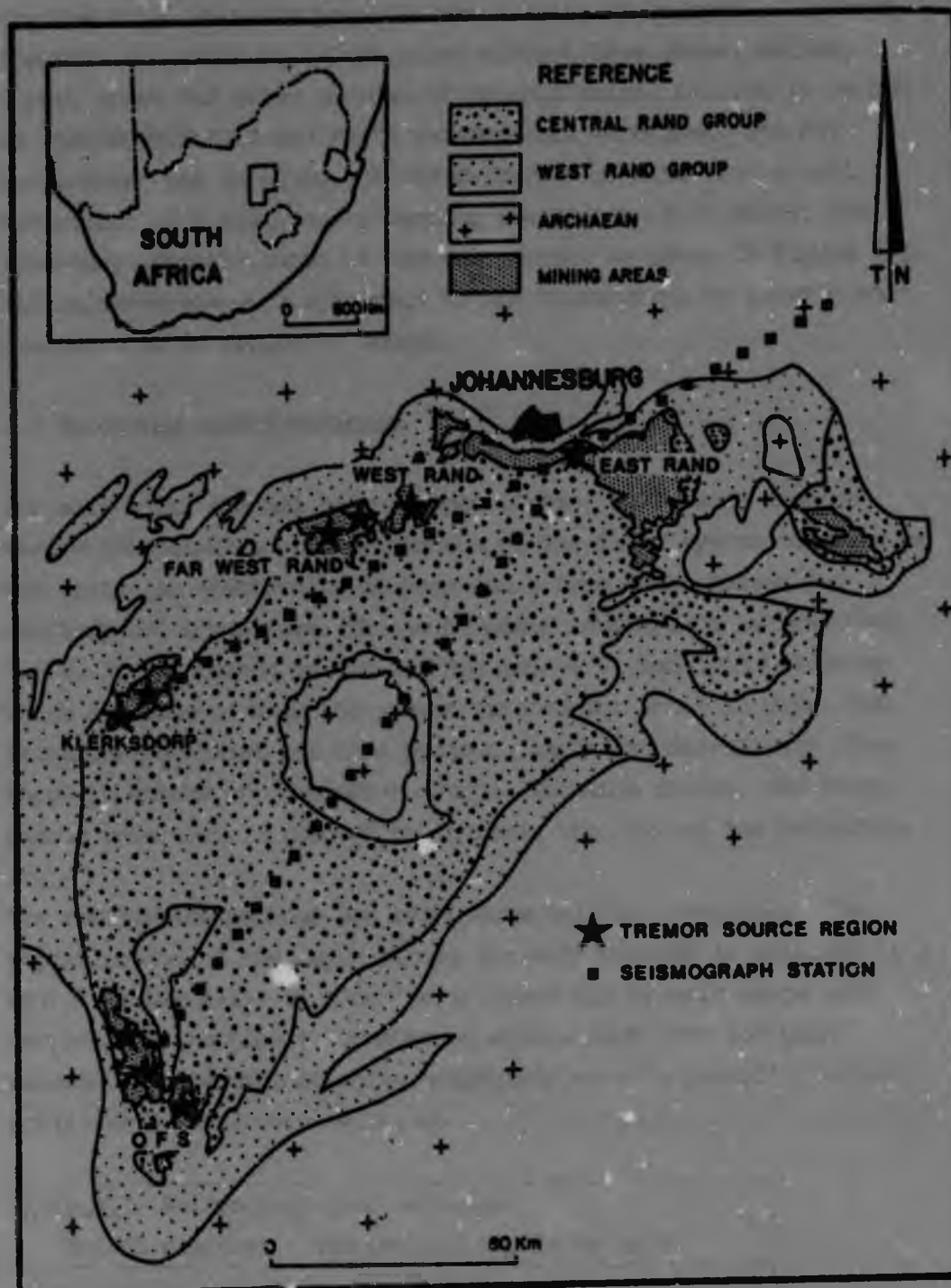
Figure 4.1. Seismograph locations on the Klerksdorp - East Rand - Witbank and East Rand - O F S profiles. Post Witwatersrand Supergroup rocks have been stripped (from Tweedie, 1986).
