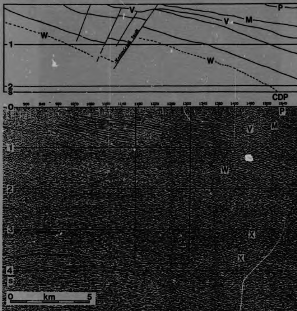
Figure 6.3A. Unmigrated panel (CDP 900-1540) from the trans-Witwatersrand Basin deep seismic reflection profile. An interpretation of the upper 2 s TWT is shown above. X - reflectors in the Basement Complex, W - base of Dominion and West Rand Groups, V - base of Ventersdorp Supergroup, M - base of Black Reef Formation and Malmani Subgroup, P - base of Pretoria Group. The box on the section shows the position of the panel shown in greater detail in Figure 6.3B.
