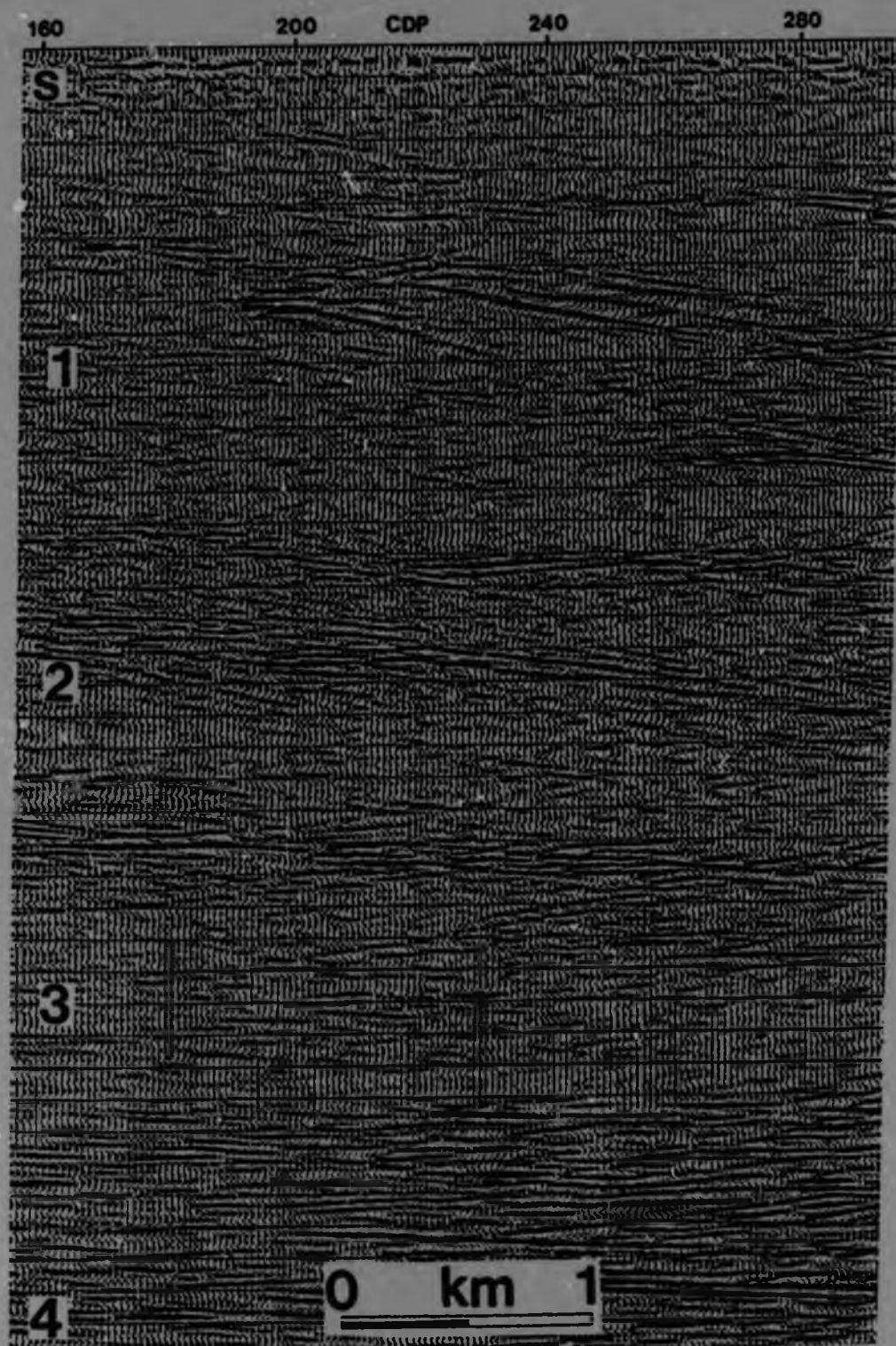
Figure 6.5A. Migrated panel (CDP 160-290) from the trans-Witwatersrand Basin deep seismic reflection profile. This panel shows the reflective character of the Ventersdorp Dome.
