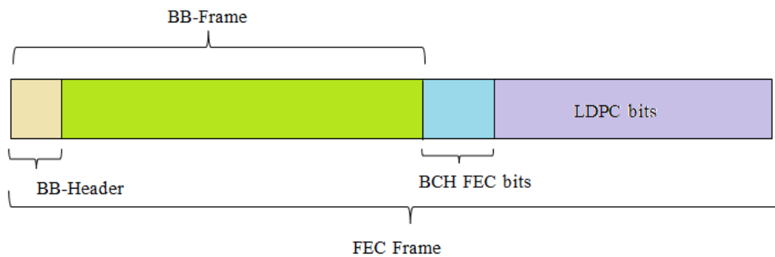
Figure 2.5 Baseband and FEC Frames Structure
