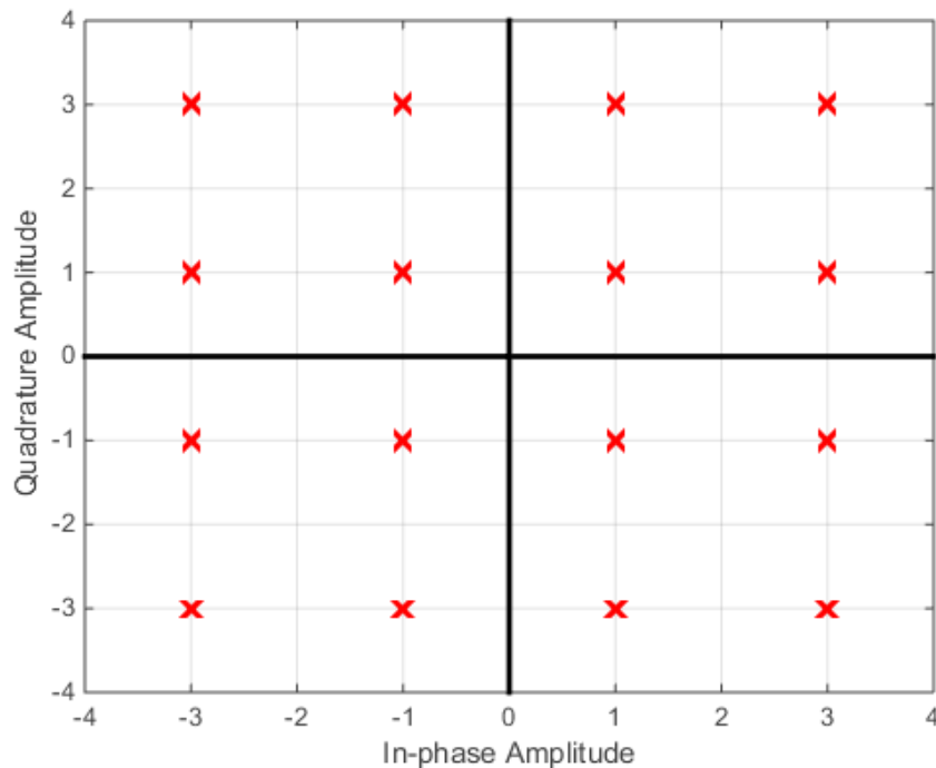
Figure 2.6 16 QAM Constellation
