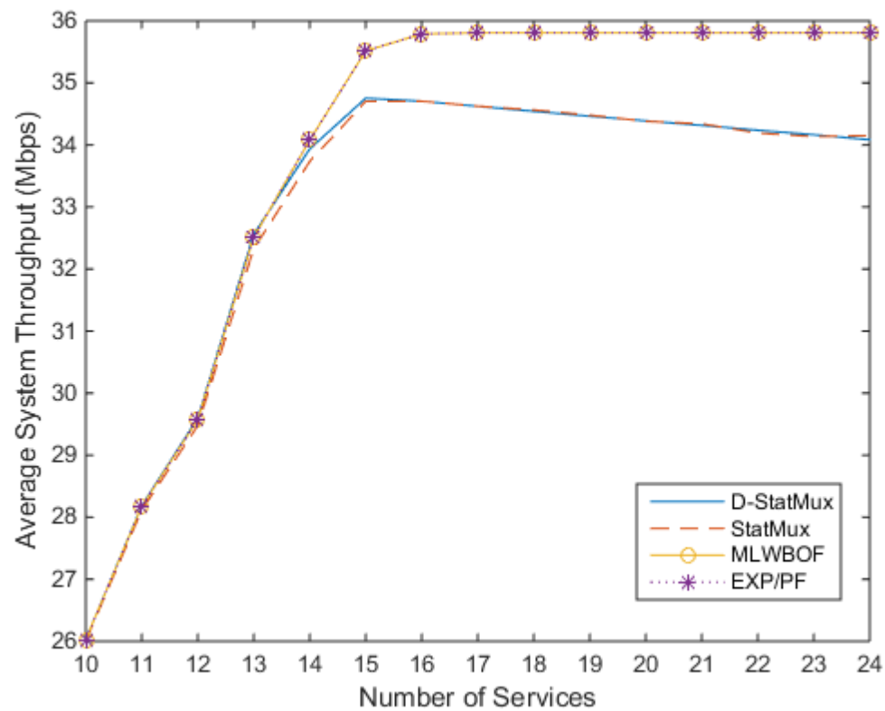
Figure 3.5 System Throughput with increasing number of services
