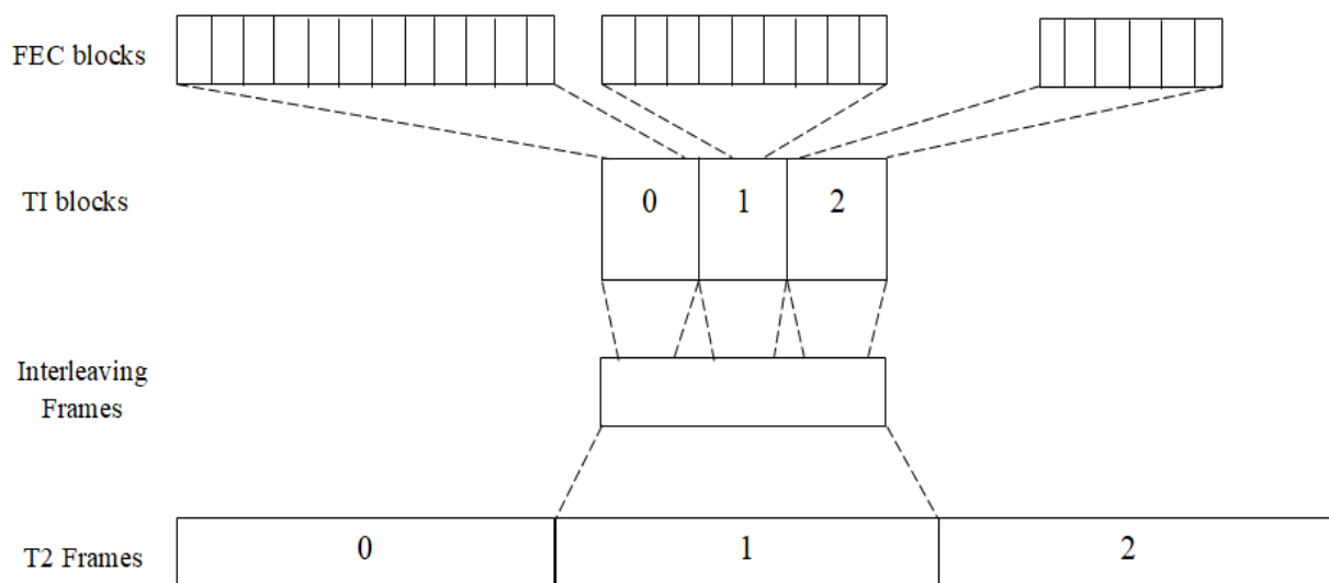
(c) Time Interleaving Option 3
