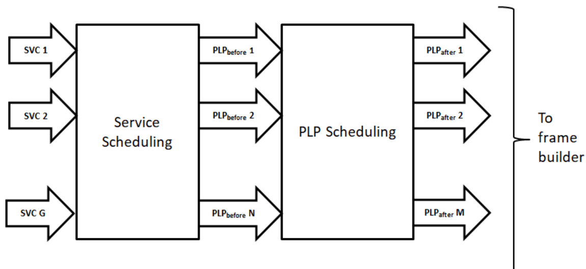
Figure 4.1 System Model for Joint Service and PLP Scheduling
