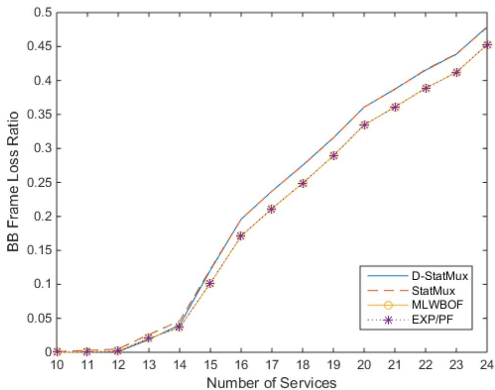
Figure 3.6 BB Frame loss with increasing number of services
