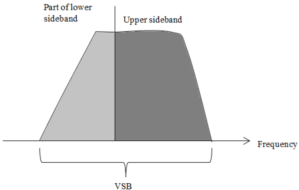
Figure 1.3 Illustration of VSB Modulation Scheme
