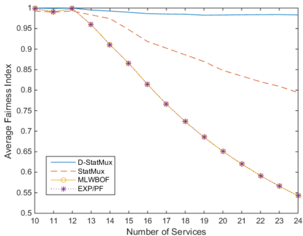
Figure 3.7 Fairness with increasing number of services
