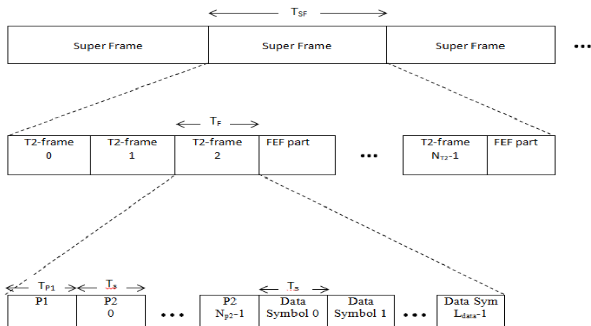
Figure 2.9 DVB-T2 Framing Structure
