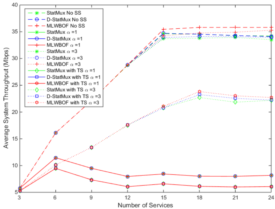
Figure 5.5 System Throughput with over-packing for Joint Service and PLP Scheduling with Time Slice Allocation
