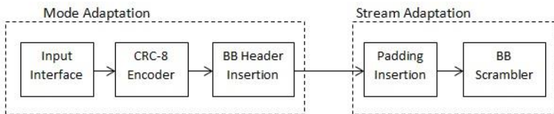
Figure 2.2 DVB-T2 Input Processing Module for Input Mode A
