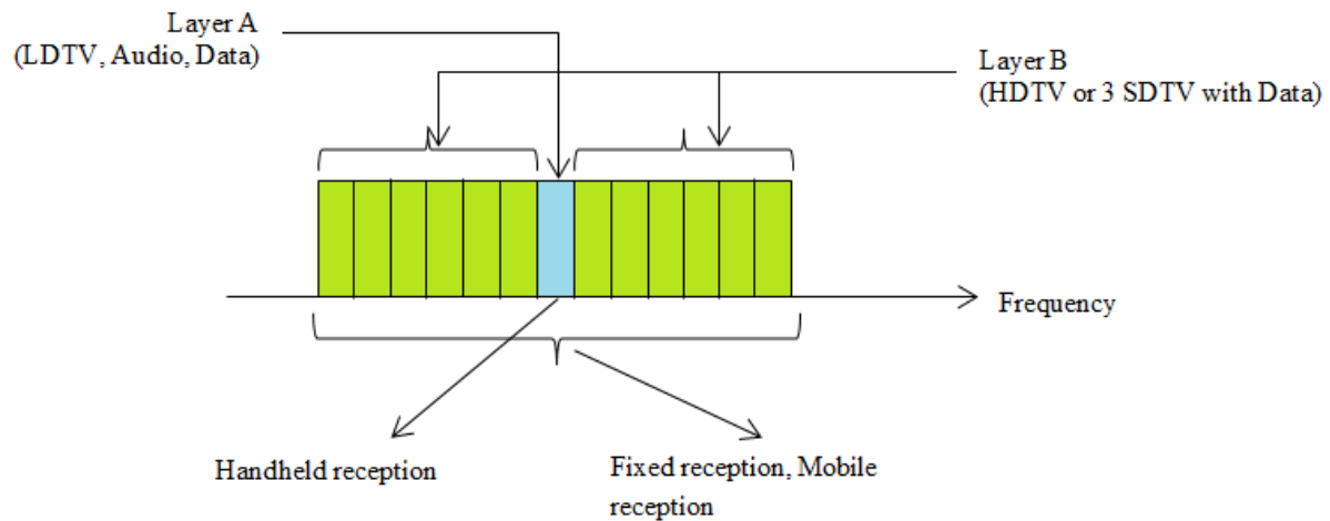
Figure 1.5 BST-OFDM Modulation Scheme
