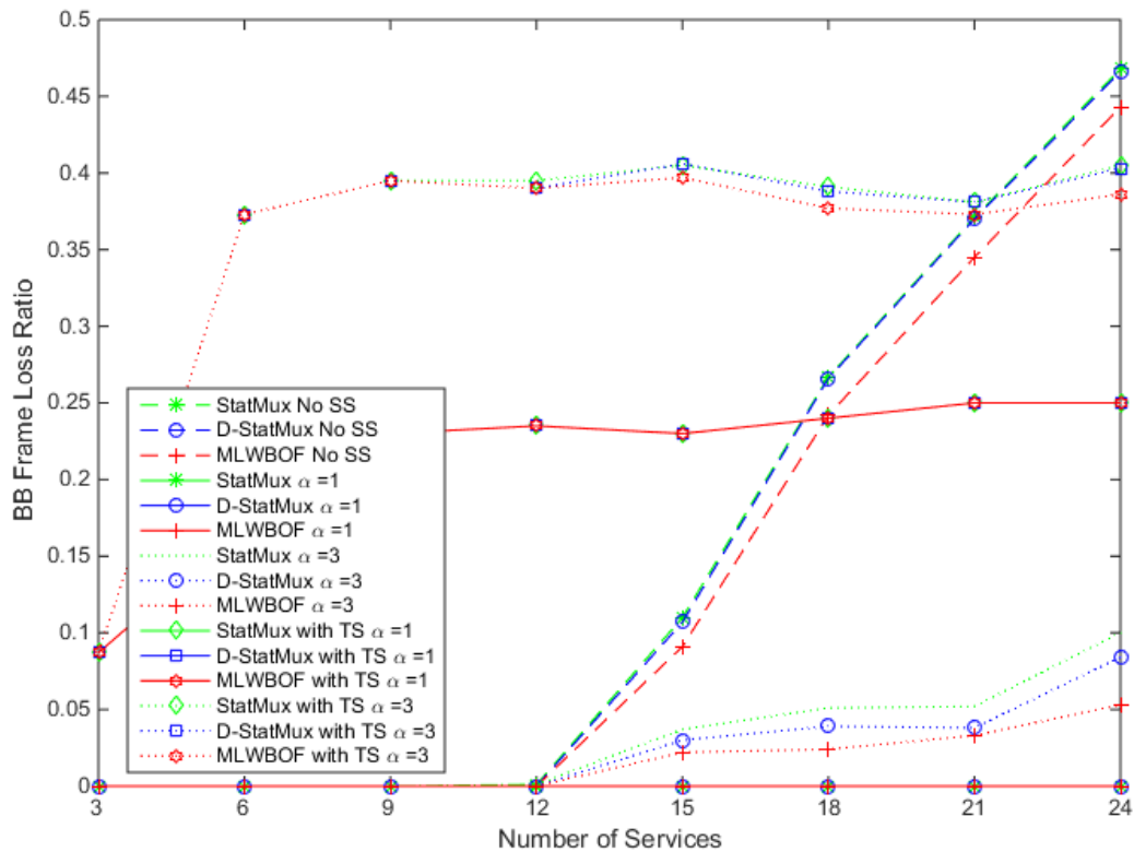
Figure 5.6 System BB Frame Loss due to Time Slice Allocation with over-packing for Joint Service and PLP Scheduling with Time Slice Allocation
