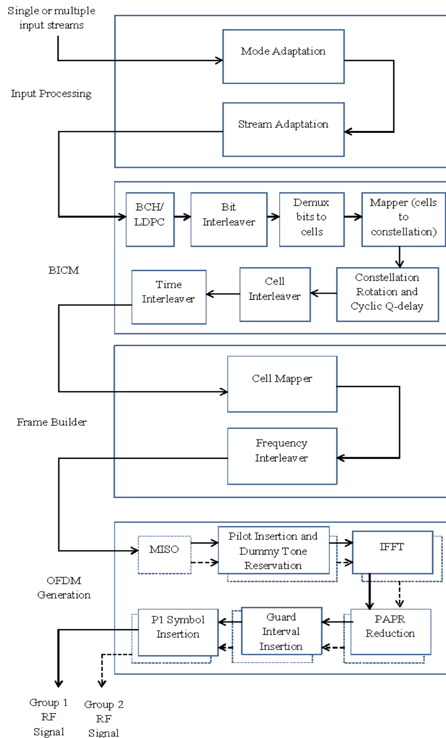
Figure 2.1 DVB-T2 system block Diagram
