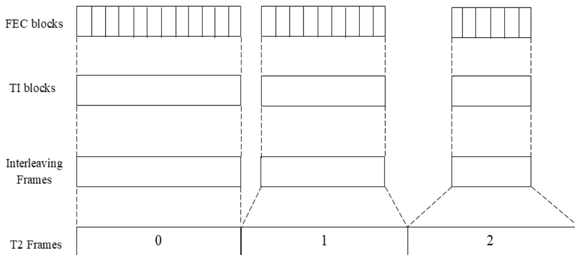
(a) Time Interleaving Option 1
