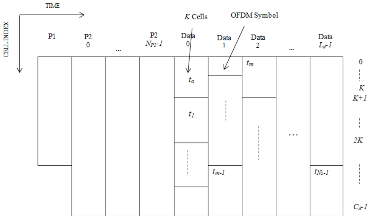
Figure 5.2 Slice Allocation Scheme's proposed data slices in a T2 Frame
