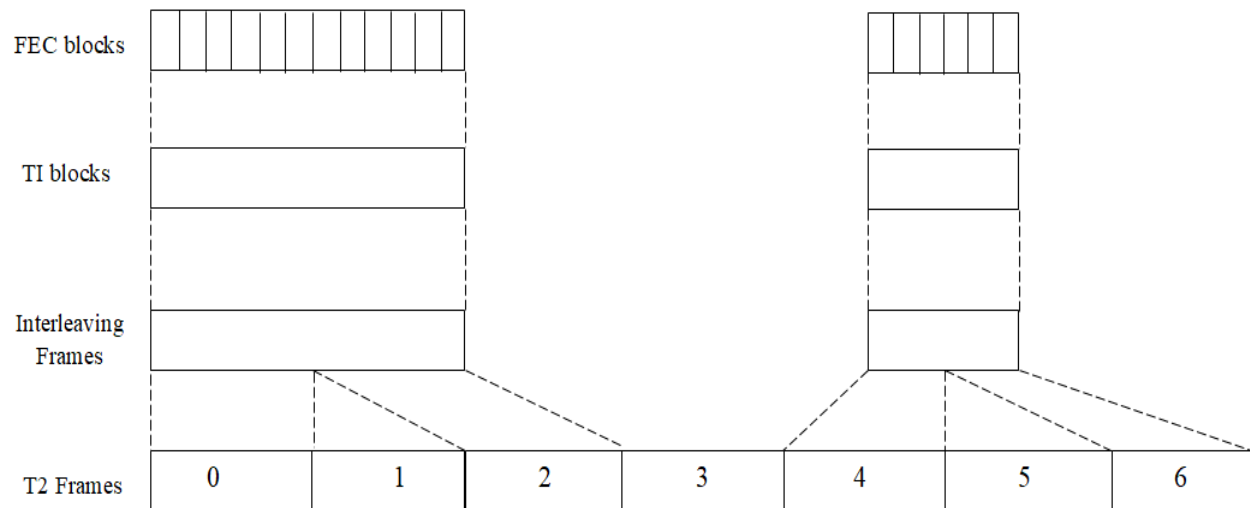
(b) Time Interleaving Option 2
