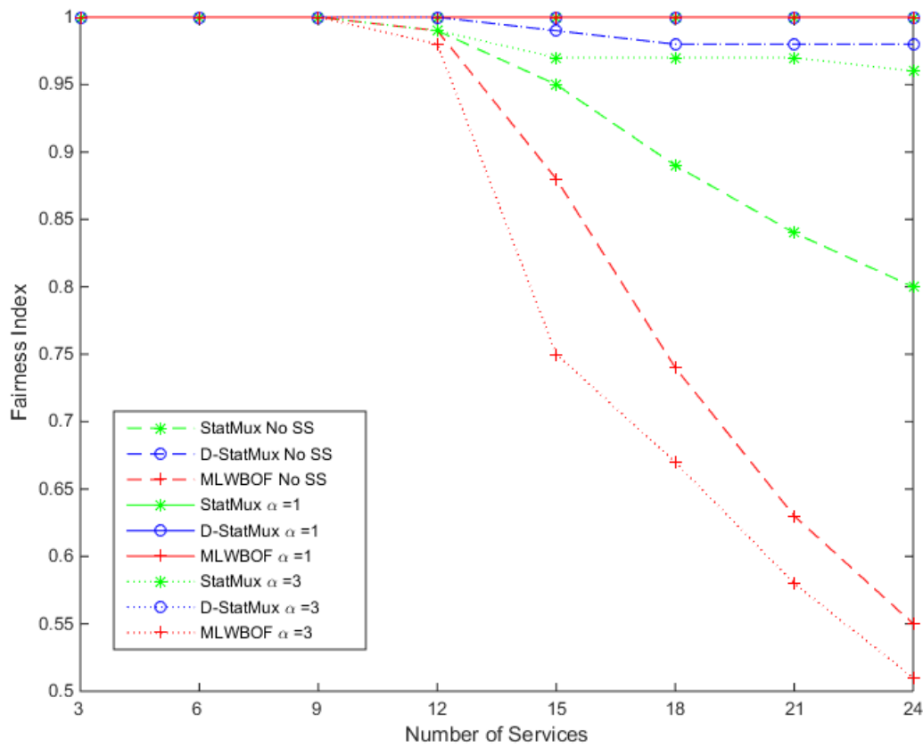
Figure 4.4 Fairness with increasing number of services
