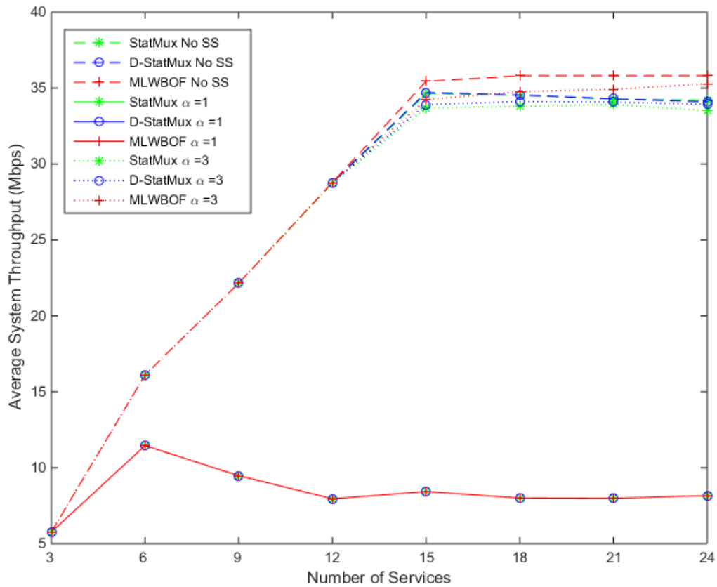
Figure 4.2 System Throughput with increasing number of services
