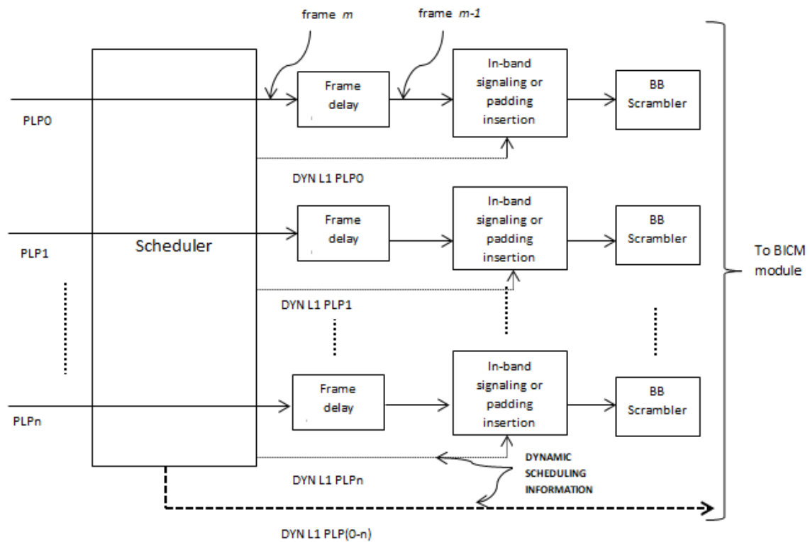
Figure 2.4 Stream Adaptation for Input Mode B
