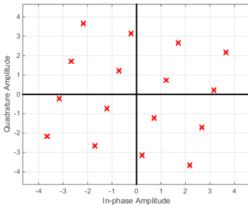
Figure 2.7 A Rotated 16 QAM Constellation
