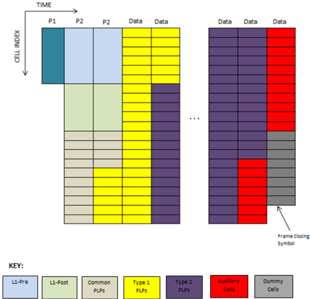
Figure 2.11 Cell Mapping in DVB-T2
