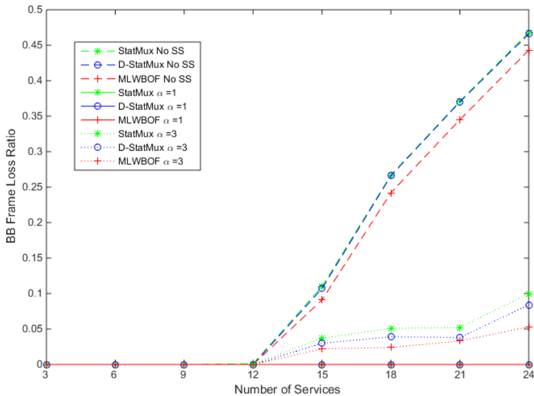
Figure 4.3 BB Frame loss with increasing number of services
