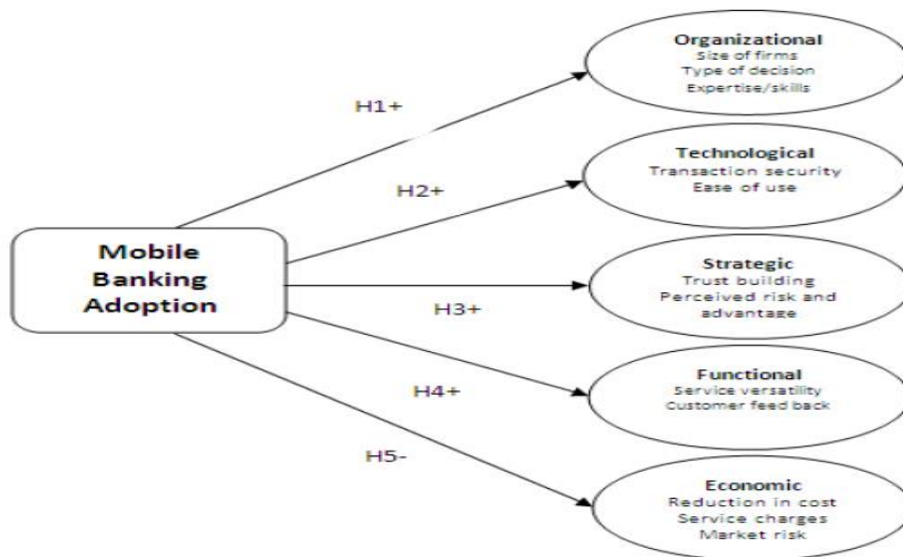
Figure 7: Saleem and Rashid conceptual model
