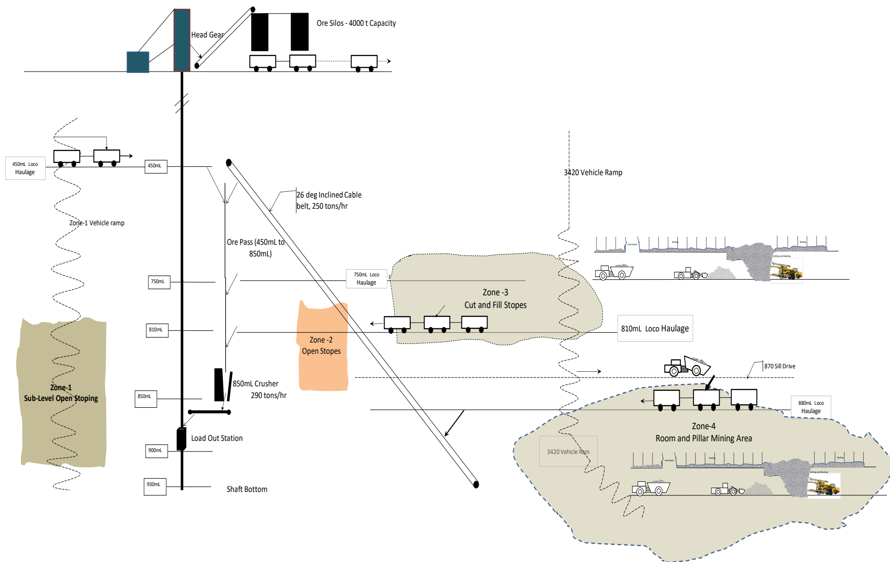
Figure 4.8 – Schematic of ShaftA3 at MineABC
