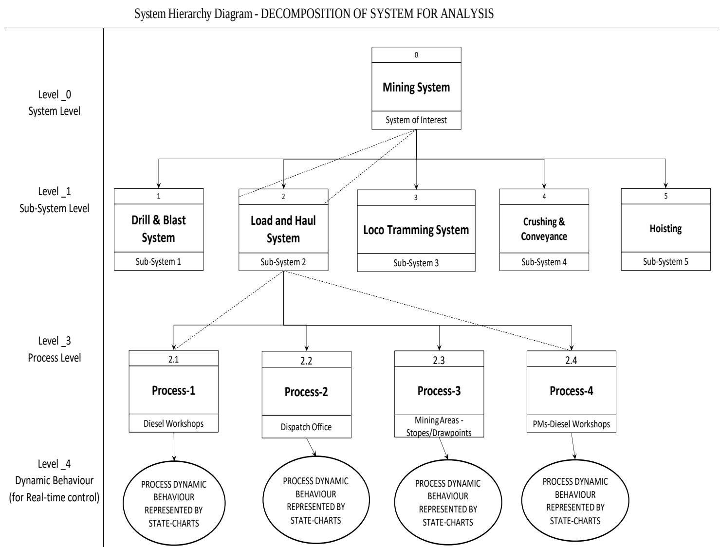
Figure 3.1 – LSE Technique for trackless mining production system analysis
