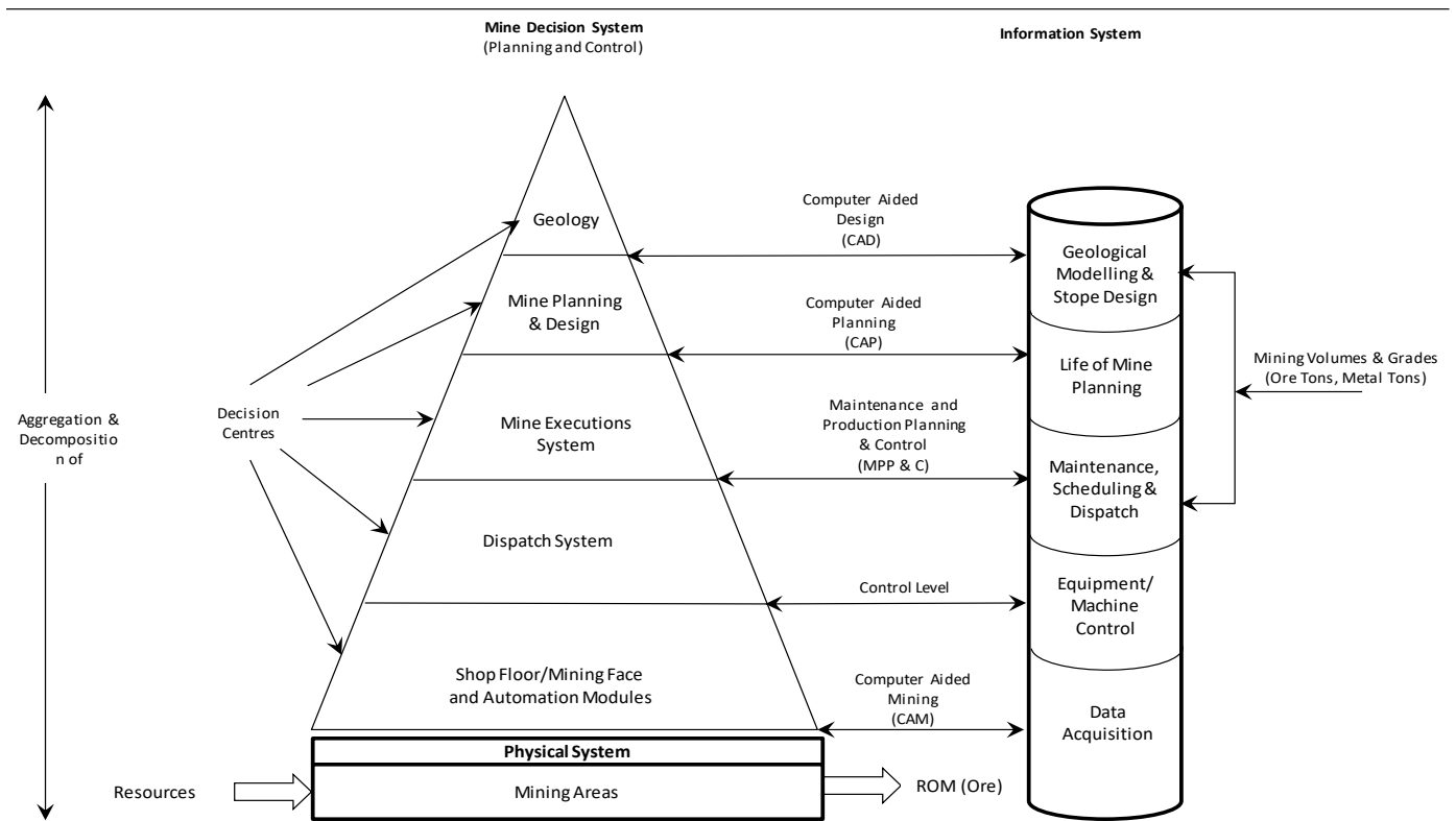
Figure 5.7 – Concept of a trackless mining planning and decision system (adapted from Rembold, et al (1993))
