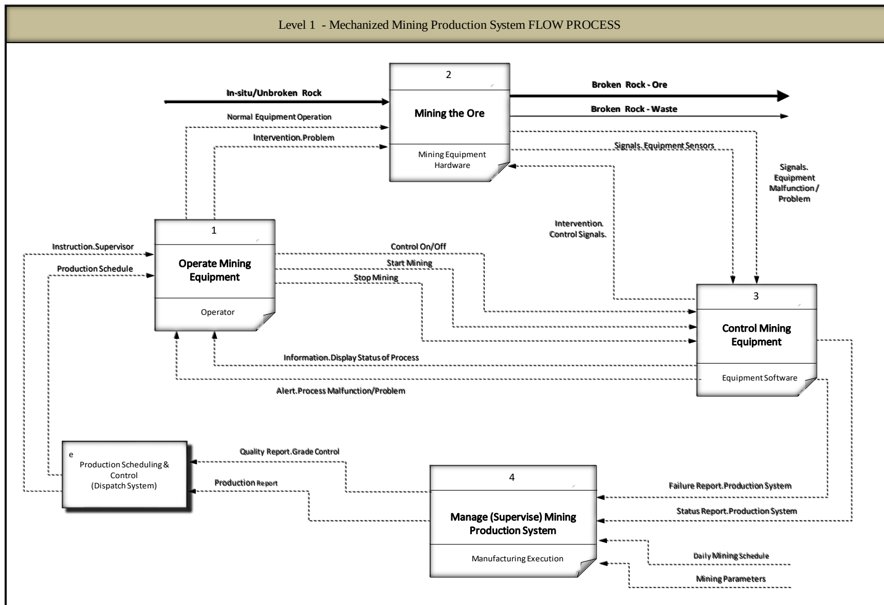
Figure 5.10 – Flow process for trackless production process
