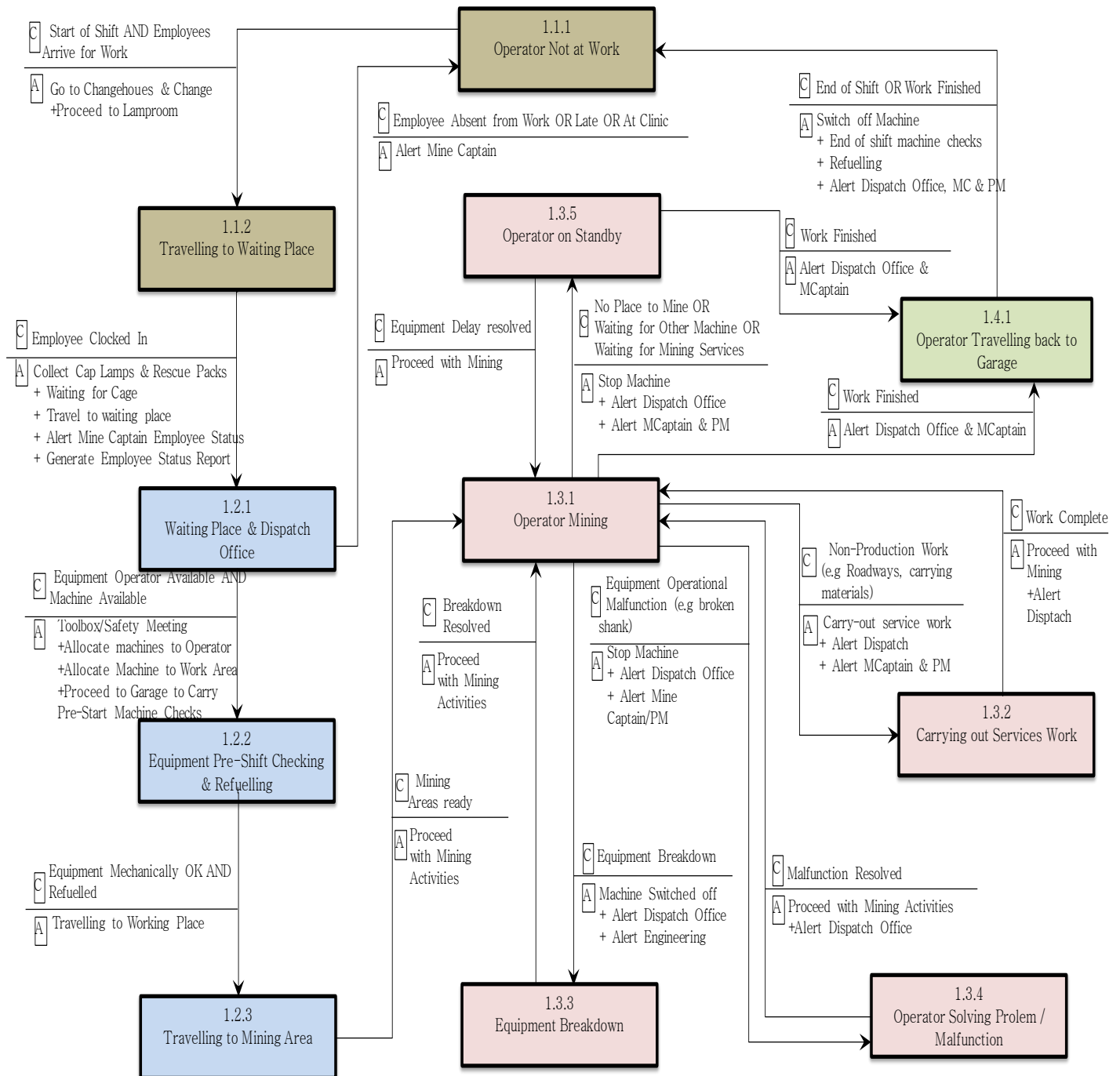
Figure 5.12 – State chart diagram for operating trackless mining equipment
