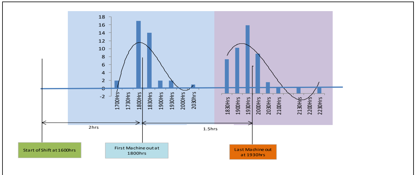
Figure 5.6 – Equipment dispatch time distributions at Shaft A2
