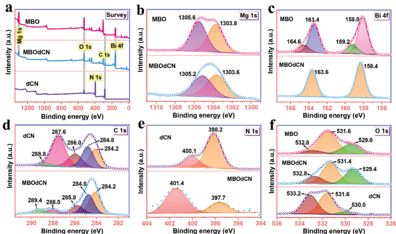
Figure 2. a) X-ray photoelectron spectroscopy (XPS) survey spectra, b) Mg 1s, c) Bi 4f, d) C 1s, e) N 1s, and f) O 1s high-resolution spectra of MBO, dCN, and MBODCN photocatalysts.
