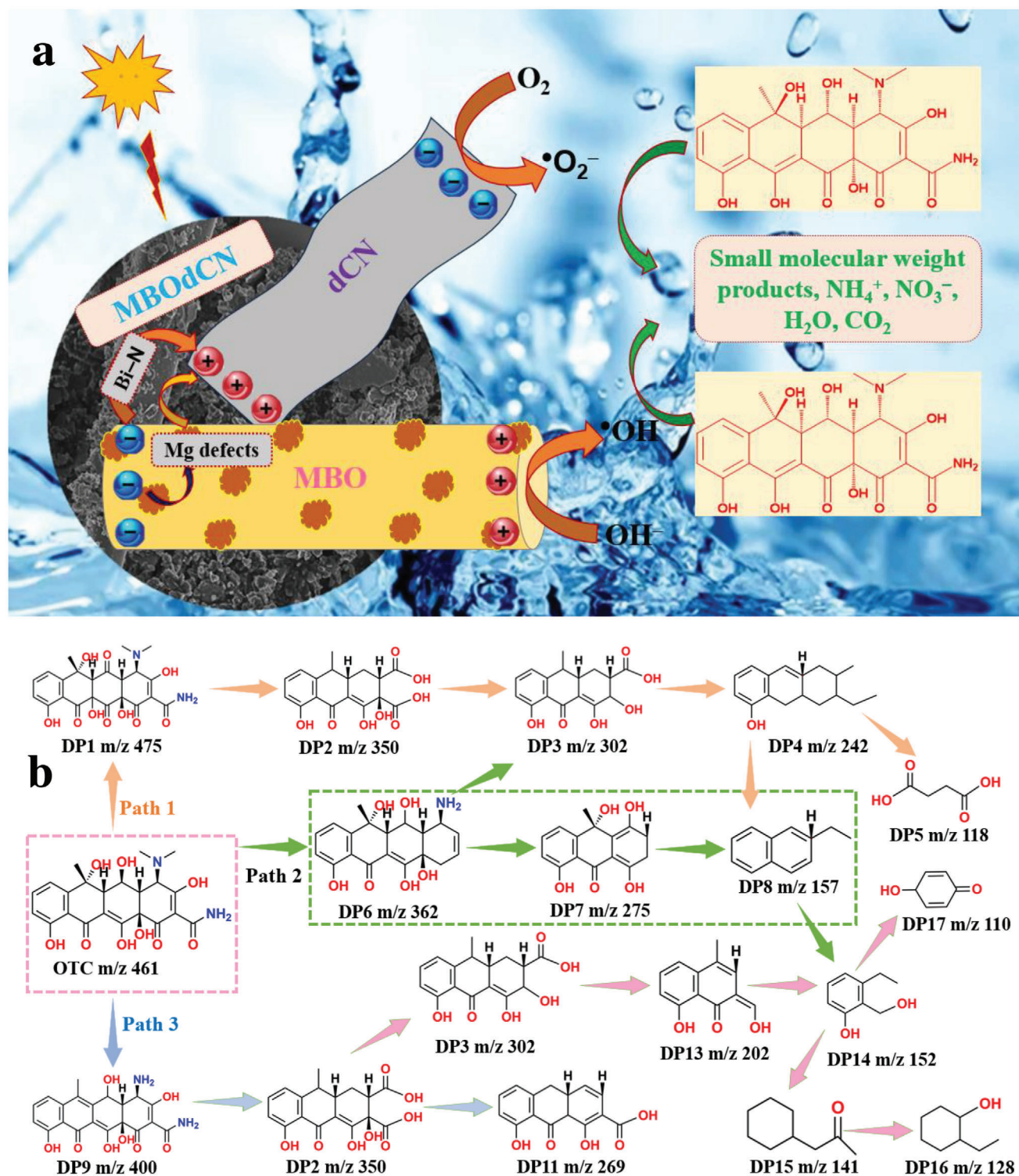
Figure 8. Schematic of the photocatalytic mechanism a) and degradation pathways b) of oxytetracycline (OTC) by MBODCN/vis system.
