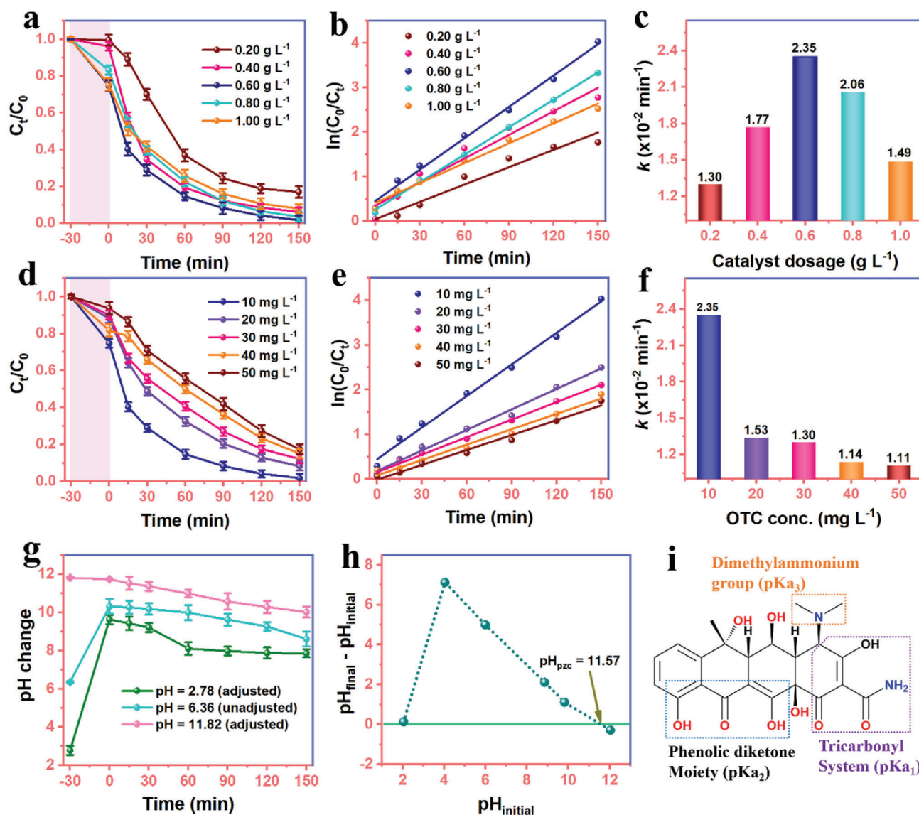
Figure 4. Effects of a–c) catalyst dosage and rate constants, d–f) initial concentration and rate constants of oxytetracycline (OTC), g) change in pH with increase in reaction time, h) pH_{\text{pzc}} of the MBODCN catalyst, and i) pK_{\text{as}} of the OTC structure.
