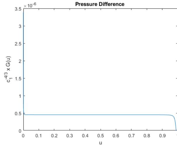
Figure 5.31: Graph of pressure difference P(0, u) = c_1^{-\frac{4}{3}} G_1(u) plotted against u for M_0 = 6 \times 10^3 for a silicic magma fracture. At the entry the pressure difference decrease rapidly from P(0, 0) = 15.355427 to P(0, u) = 0.5 \times 10^{-6}
