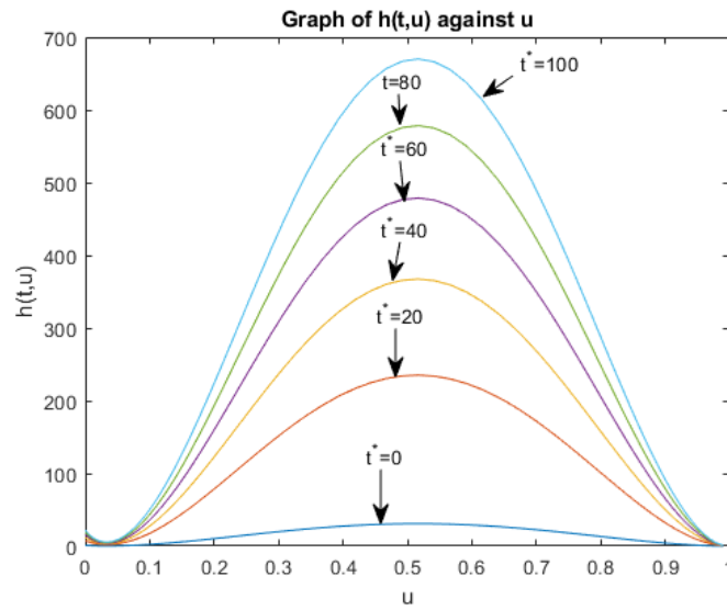
Figure 5.21: Graph of half-width h(t, u) plotted against u for M_0 = 1.05 \times 10^3 for a silicic magma fracture at a range of times from t^* = \frac{t}{c_1} = 0 to t^* = \frac{t}{c_1} = 100 .
