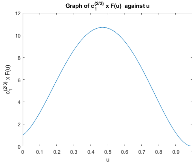
Figure 5.9: Graph of c_1^{\frac{2}{3}} F(u) plotted against u for M_0 = 2.6105 \times 10^2 for a silicic magma fracture.
