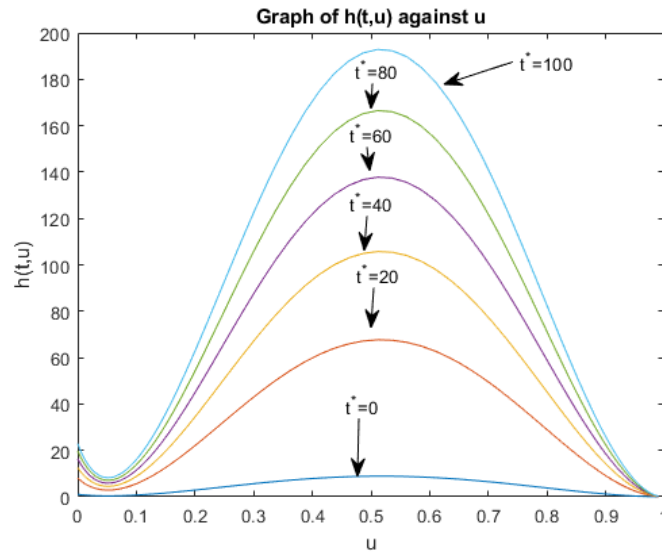
Figure 5.17: Graph of half-width h(t, u) plotted against u for M_0 = 2.618 \times 10^2 for a silicic magma fracture at a range of times from t^* = \frac{t}{c_1} = 0 to t^* = \frac{t}{c_1} = 100 .
