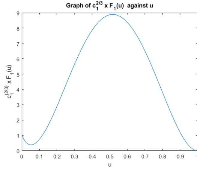
Figure 5.16: Graph of h(0, u) = c_1^{\frac{2}{3}} F_1(u) plotted against u for M_0 = 2.618 \times 10^2 for silicic magma fracture.
