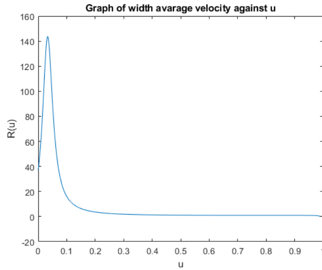
Figure 5.23: Graph of the ratio R(u) of the width average fluid velocity to the speed of propagation of the fracture \frac{dL}{dt} plotted against u for M_0 = 1.05 \times 10^3 for silicic magma fracture. At the entry R(0) = 37.0540 while the asymptotic results with Q_0 = 3.64557 \times 10^{-4} gives R(0) = c_1 Q_0 = 36.4557 .
