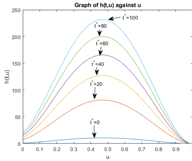
Figure 5.10: Graph of half-width h(t, u) plotted against u for M_0 = 2.6105 \times 10^2 for a silicic magma fracture at times and t^* = \frac{t}{c} = 0, 20, 40, 60, 80 and 100
