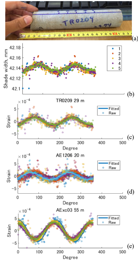
Fig. 5 Good examples [22]. The core sample TR0209 at 29 m: (a) a photo, (b): raw data, (c) strain and fitted sinusoidal curves. (d) and (e): the other good examples for comparison.
