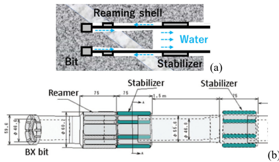
Fig. 4 The schematics representing the drilling with reverse circulation (a) and a recommended string sequence (b) [13]. Dashed arrows represent water that flows back inside the drilling rods to push out drilled cores. For the measurement, we select the core without cracks, veins as shown in (a), or lithological boundaries.
