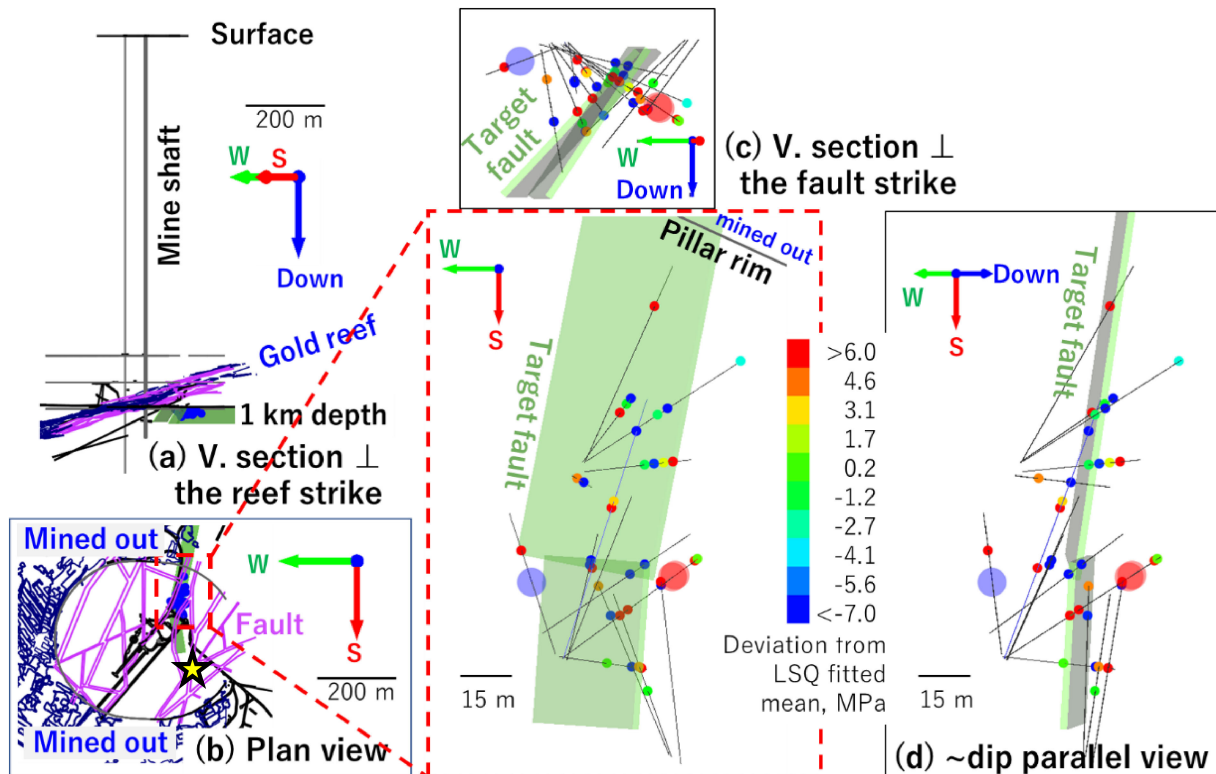
Fig. 3 The configuration of the boreholes (black thin lines in (b), (c) and (d)) and the locations (dots) where the core samples are selected for this DCDA. The mine's infrastructures and relevant information are also shown. See the details of the boreholes in Table 1. The locations highlighted with larger circles correspond to the data also highlighted in Figs. 8(a) and 9(a). The color for each dot represents the magnitude of deviation, MPa, with respect to the calculated value from the mean 3D differential stress field determined by the least-square-method (LSQ). A yellow star represents the location where an overcoring stress measurement was carried out (see Table 2 and Fig. 7 yellow symbols).
