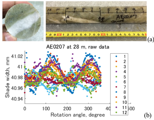
Fig. 6 A bad example [22]. The scale of the vertical axis is the same as Fig. 5(a).
