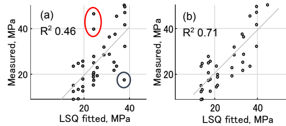
Fig. 8 A scatter plot of the measured versus the calculated stress. (a): all data with outliers; WO in Table 2 and Fig. 7. The locations for the data highlighted here are represented by larger circles in Fig. 3(c), (d). (b): without the data highlighted in (a); without outliers, WoO in Table 2 and Fig. 7.
