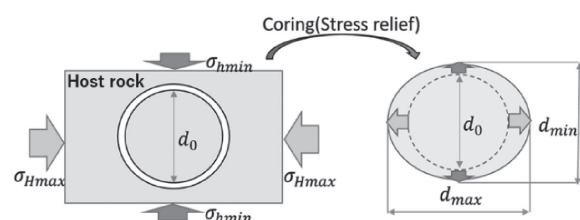
Fig. 1 The principle of elastic deformation during coring [1].
