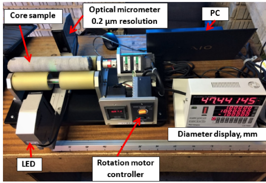
Fig. 2 The DCDA measurement system (Funato's 2017 model), compact enough for a single regular courier parcel or a piece of check-in luggage for an international flight.
