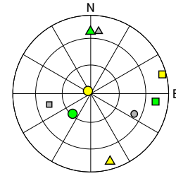
Fig. 7 A composite plot of the three results to compare the plunges and orientations of the measured principal stresses. Gray and green: pre-mining DCDA (WO and WoO, respectively; this study). Yellow: post-mining overcoring [14] at the location in Fig. 3(b). See measured values in Table 2. ○: \sigma_1 , △: \sigma_2 , □: \sigma_3 .
