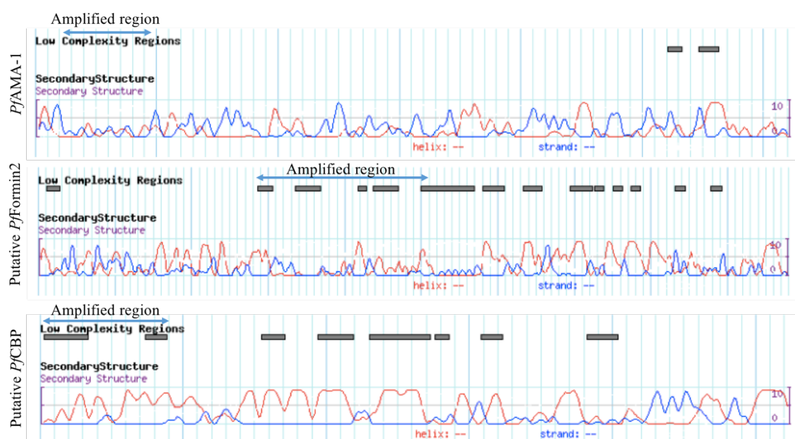
Figure 6.24. Secondary structure predictions of PfAMA-1 , putative PfFormin2 and putative PfCBP .
