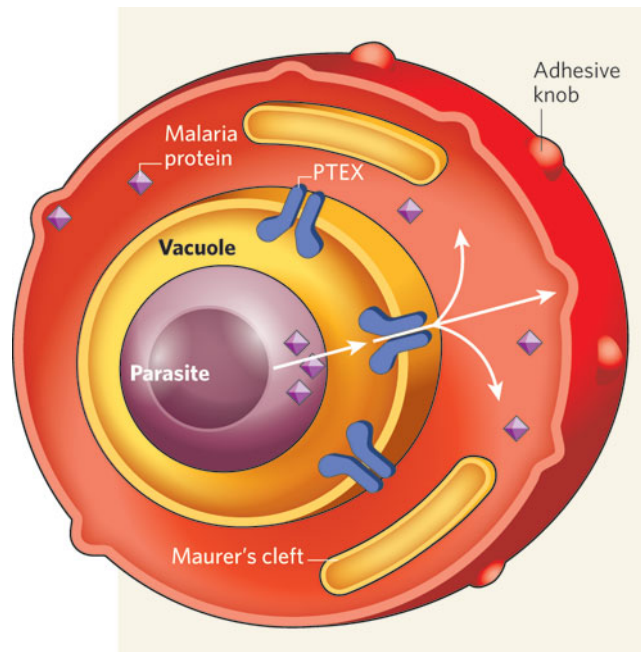
Figure 1.7. Protein export pathways across the parasite membrane.
