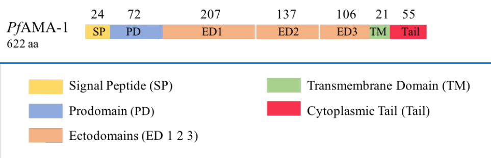
Figure 3.10. A schematic representing the domains of PfAMA -1, a P. falciparum microneme invasion protein.
