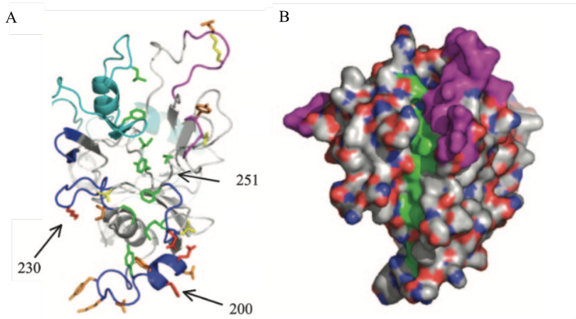
Figure 3.4. The conserved hydrophobic cleft found in the PfAMA-1 ectodomain.
