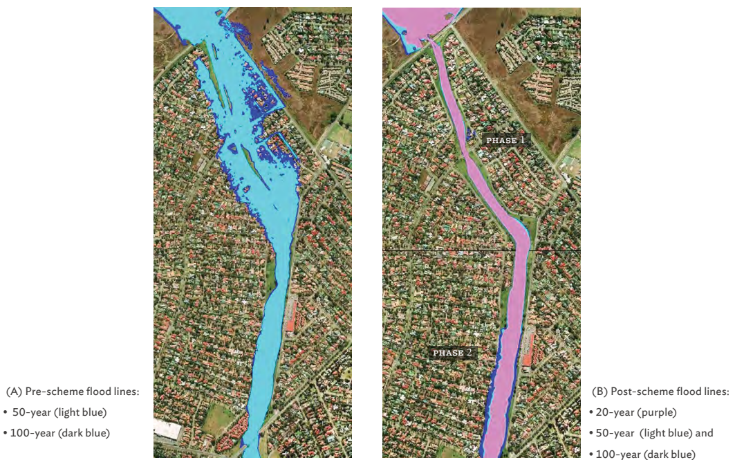
Figure 5.7: (A) Pre-development and (B) post-development 50- and 100-year flood lines. In the post-development figure, the 20-year flood line was included in the design drawings. (B) also indicates the location of the different phases of the project.
