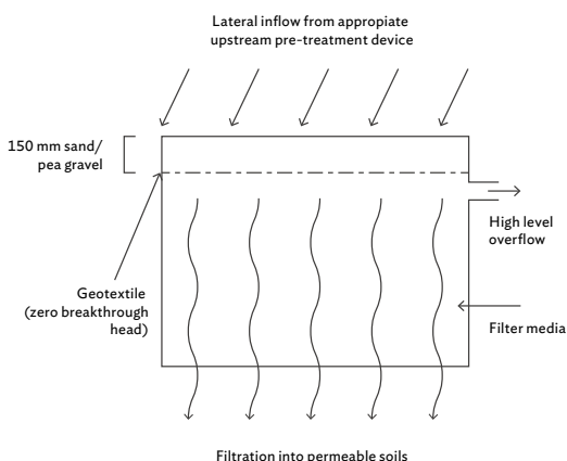
Figure 3.16: Soakaway
