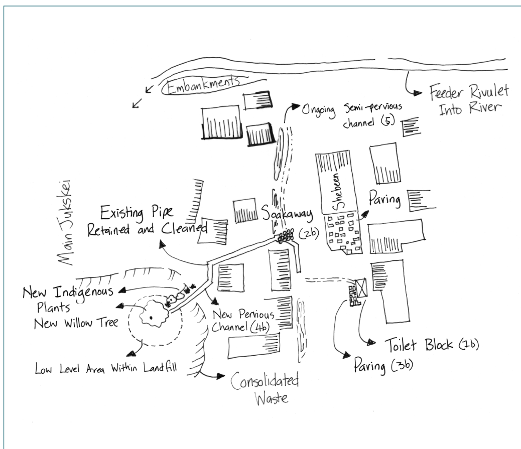
Figure 4.10: Schematic diagram of Site 1 after the interventions were introduced
