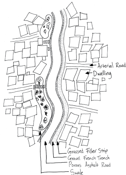
Figure 3.3: Plan view of swale along a road
