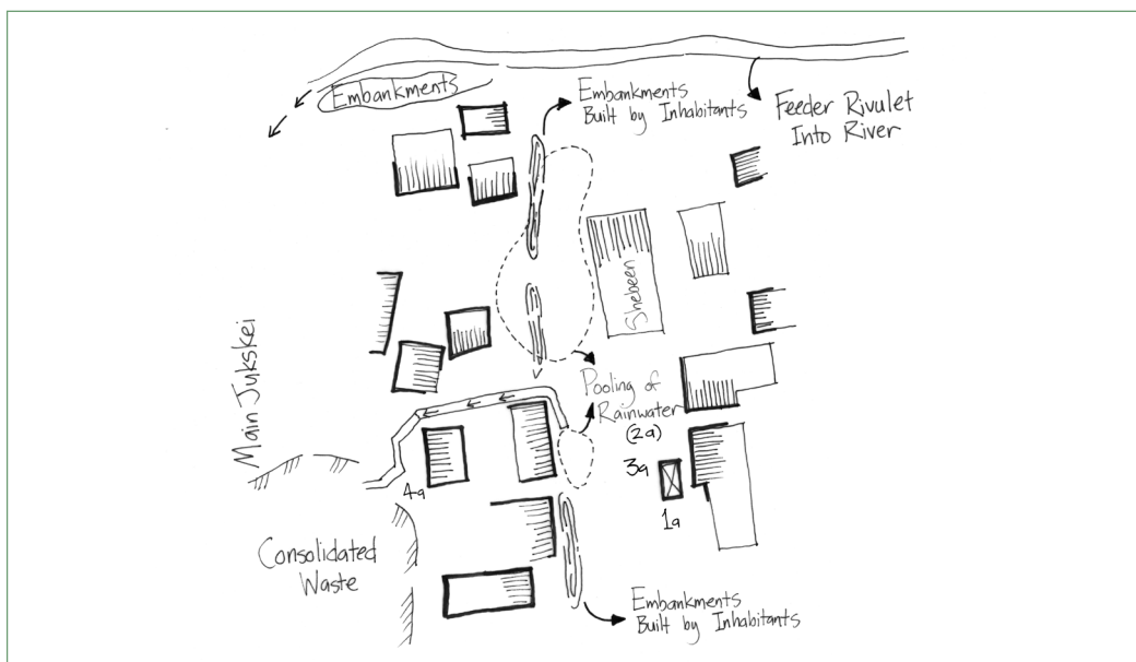
Figure 4.6: Schematic diagram of Site 1 before any interventions were introduced
