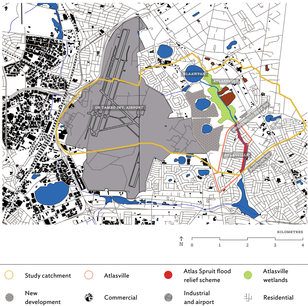
Figure 5.2: Atlas Spruit flood relief scheme and associated catchment, showing the main water bodies (in blue)
