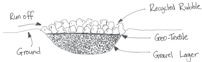
Figure 3.18: Cross-section of soakaway
