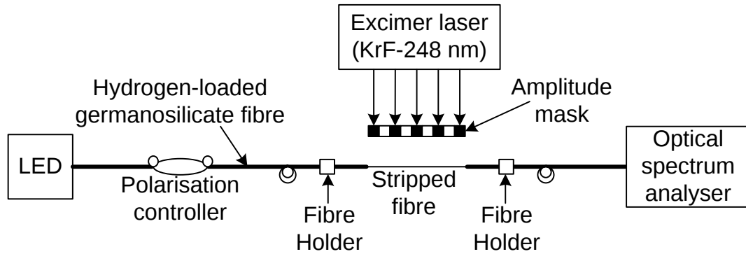
Figure 4.1: Setup to fabricate long-period gratings using an excimer laser[22]
