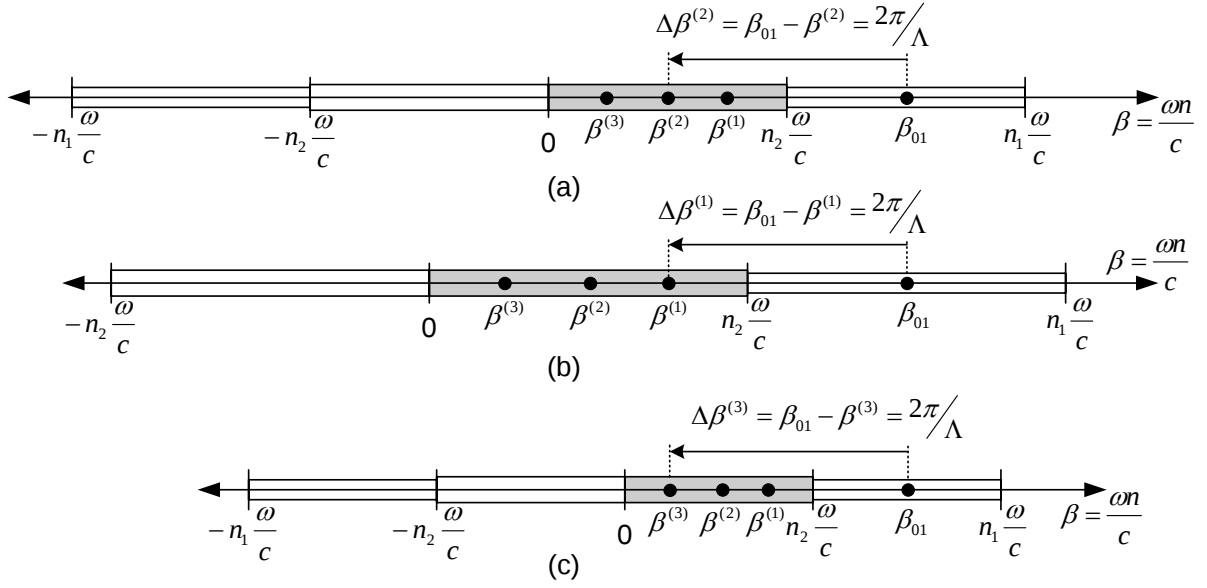
Figure 2.9: The coupling of LP_{01} guided mode to discrete, forward-propagating cladding modes. (a) The coupling to the LP^{(2)} cladding mode. (b) A stretched \omega -axis for coupling to the LP^{(1)} cladding mode. (c) A compressed \omega -axis for coupling to the LP^{(3)} cladding mode.
