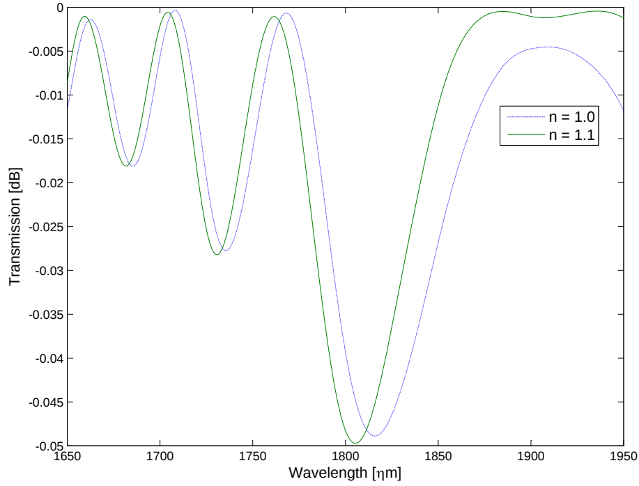
Figure 7.1: Transmission spectrum of a \Lambda = 320 \mu\text{m} grating between 1650 and 1950 nm. A wavelength shift of 11 nm from 1816 to 1805 nm can be observed in the 7 th order mode.
