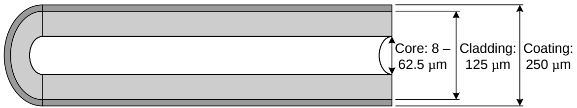
Figure 1.1: The three layer composition of an optical fibre together with typical dimensions
