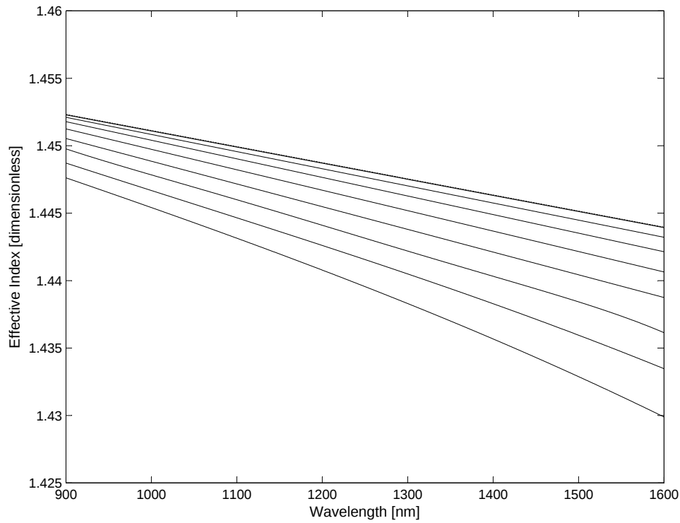
Figure 3.8: Spectral variation of the effective index n_{cl}^{(m)} of LP_{0,m} cladding modes ( m = 2 through 16 in steps of 2) in optical fibres with quenched silica and b = 62,5 \mu\text{m} . The ambient medium is assumed to be air and the dashed (topmost line) line represents the refractive index of the cladding. The bottom line represents the m = 16 cladding mode.
