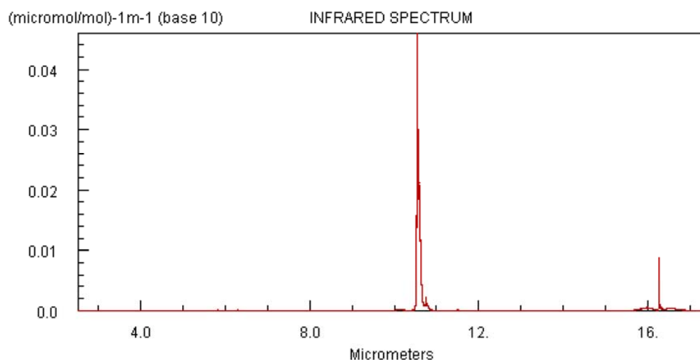
Figure 1.5: The absorption spectrum of SF 6 between 3 and 17 \mu\text{m} [14]
