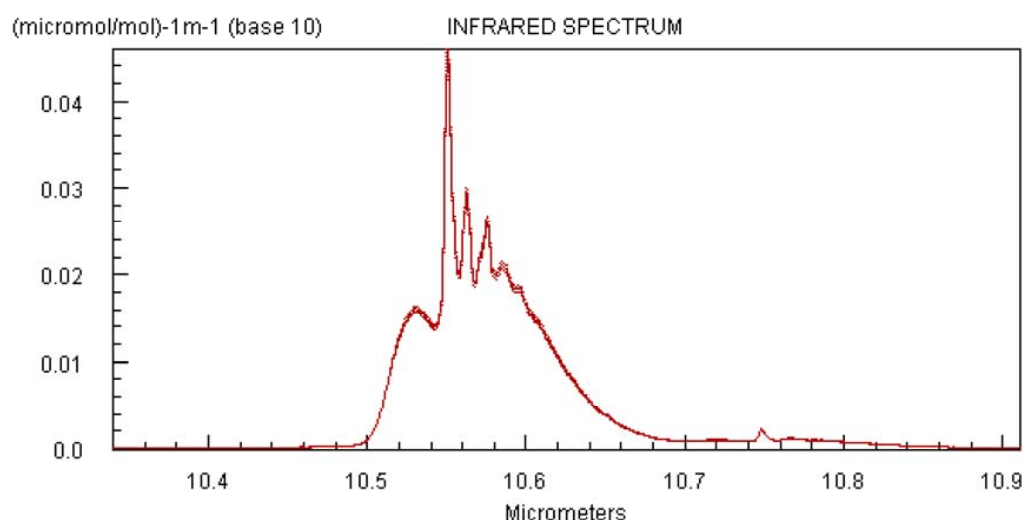
Figure 1.6: The absorption spectrum of SF 6 between 10,4 and 10,9 \mu\text{m} [14]
