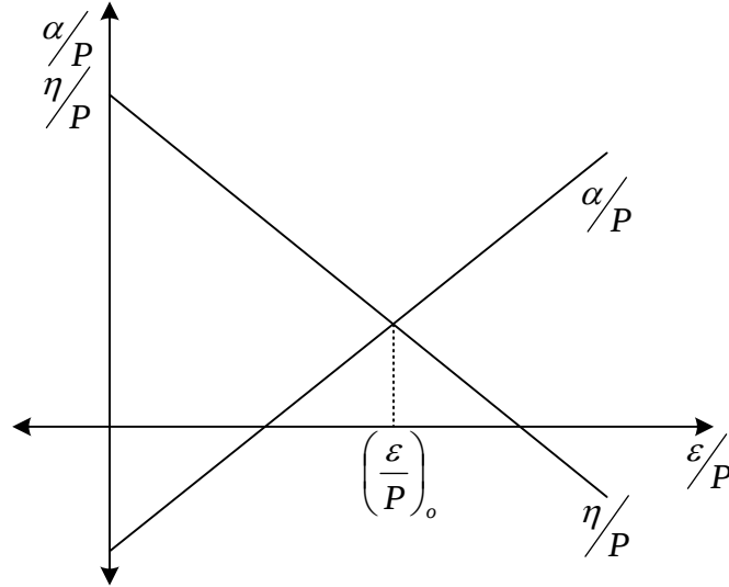
Figure A.2: A rough graph of \frac{\alpha}{p} versus \frac{E}{p} and \frac{\eta}{p} versus \frac{E}{p} for \text{SF}_6 .
