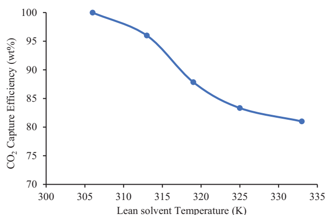
Figure 5. Effect of lean solvent temperature on CO 2 absorption efficiency. Reaction conditions: CPZ = 5wt% CMDEA = 30 wt%, P = 101.325 \text{ kN/m}^2 .
