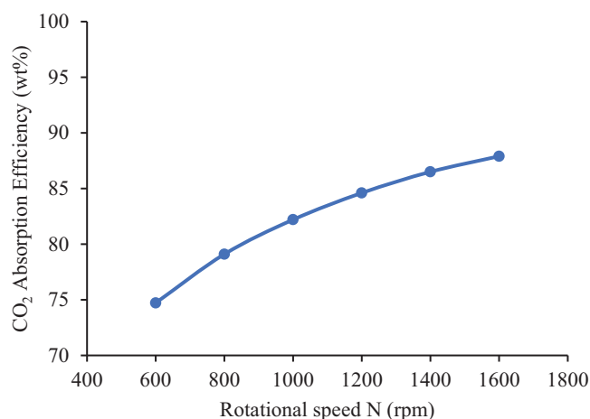
Figure 4. Rotational speed against CO 2 absorption efficiency. Reaction conditions: CPZ = 5wt% CMDEA = 30 wt%, P = 101.325 \text{ kN/m}^2 , T = 313 \text{ K} .
