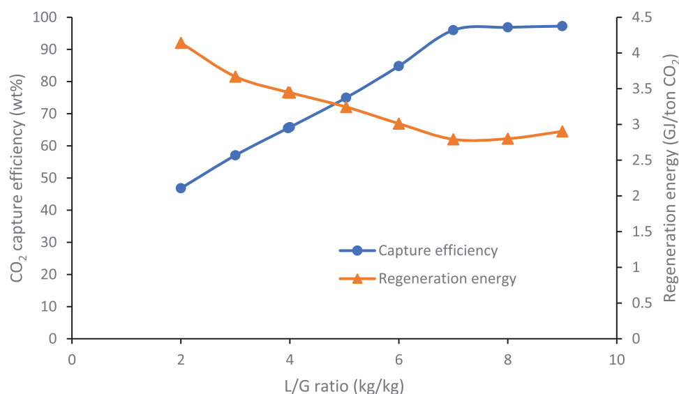
Figure 8. Effect of liquid-to-gas ratio on reboiler duty reaction conditions: CPZ = 5wt% CMDEA = 25 wt%, P = 101.325 \text{ kN/m}^2 , T = 313 \text{ K} .
