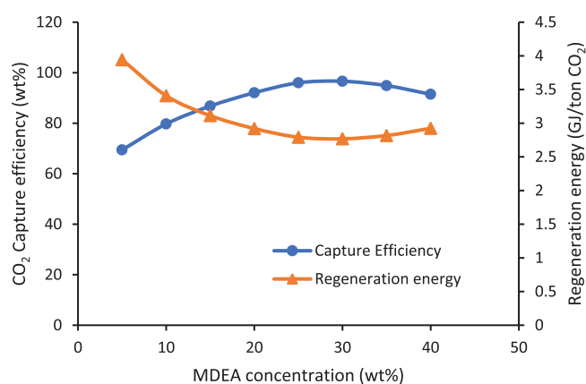
Figure 7. Effect of MDEA concentration on CO 2 absorption efficiency. Reaction conditions: CPZ = 5 wt%, CMDEA = 5–40 wt%, P = 101.325 \text{ kN/m}^2 , T = 313 \text{ K} .
