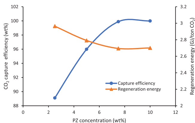
Figure 6. Effect of PZ concentration on CO 2 absorption efficiency. Reaction conditions: CPZ = 2.5–10 wt%, CMDEA = 25 wt%, P = 101.325 \text{ kN/m}^2 , T = 313 \text{ K} .
