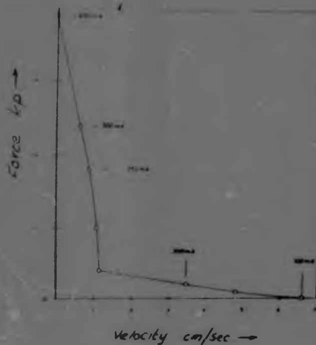
Fig.4.5. Force-Velocity at maximum activation of prosthesis motor system. (After Hirsch, Kaiser and Petersen (7).)
