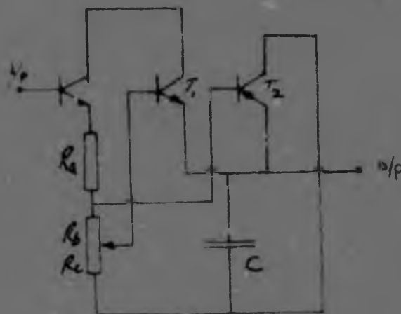
BACKLASH GENERATOR.
