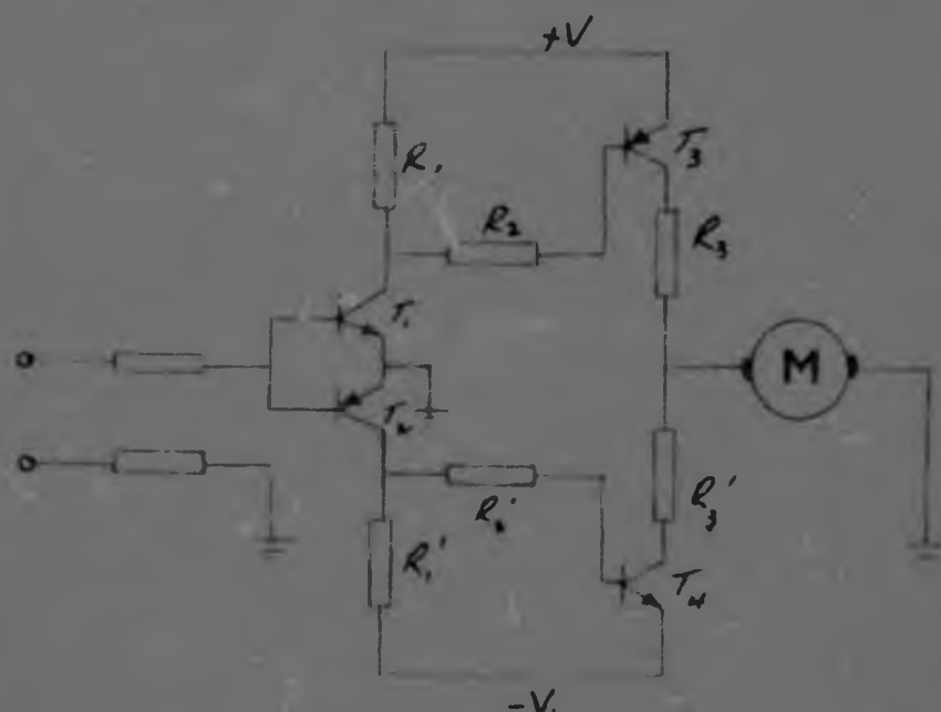
Fig.5.9. Motor Control Circuitry.
