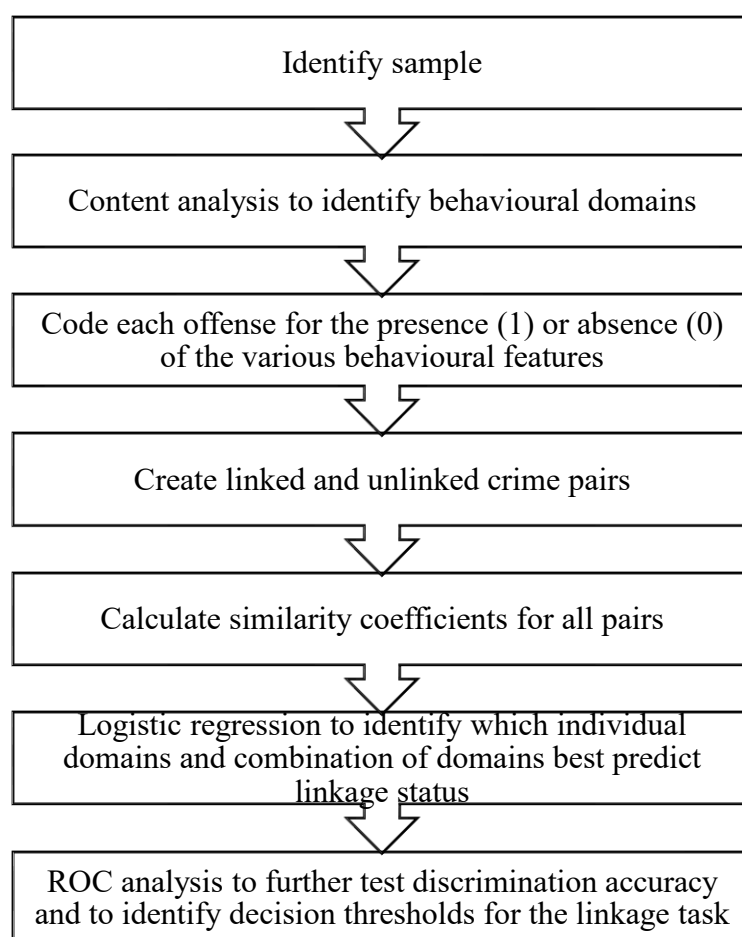
Figure 3.1 Adaption of “the Bennell approach to behavioural consistency, distinctiveness, and discrimination accuracy” (Tonkin, 2015, p.114 ).
