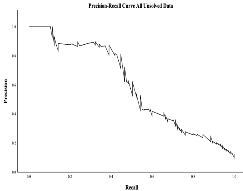
Figure 4.7 ROC and PRC for all unsolved data AUC .88 ( p < .001 , SE = .02 , 95% CI = .84 - .91).
