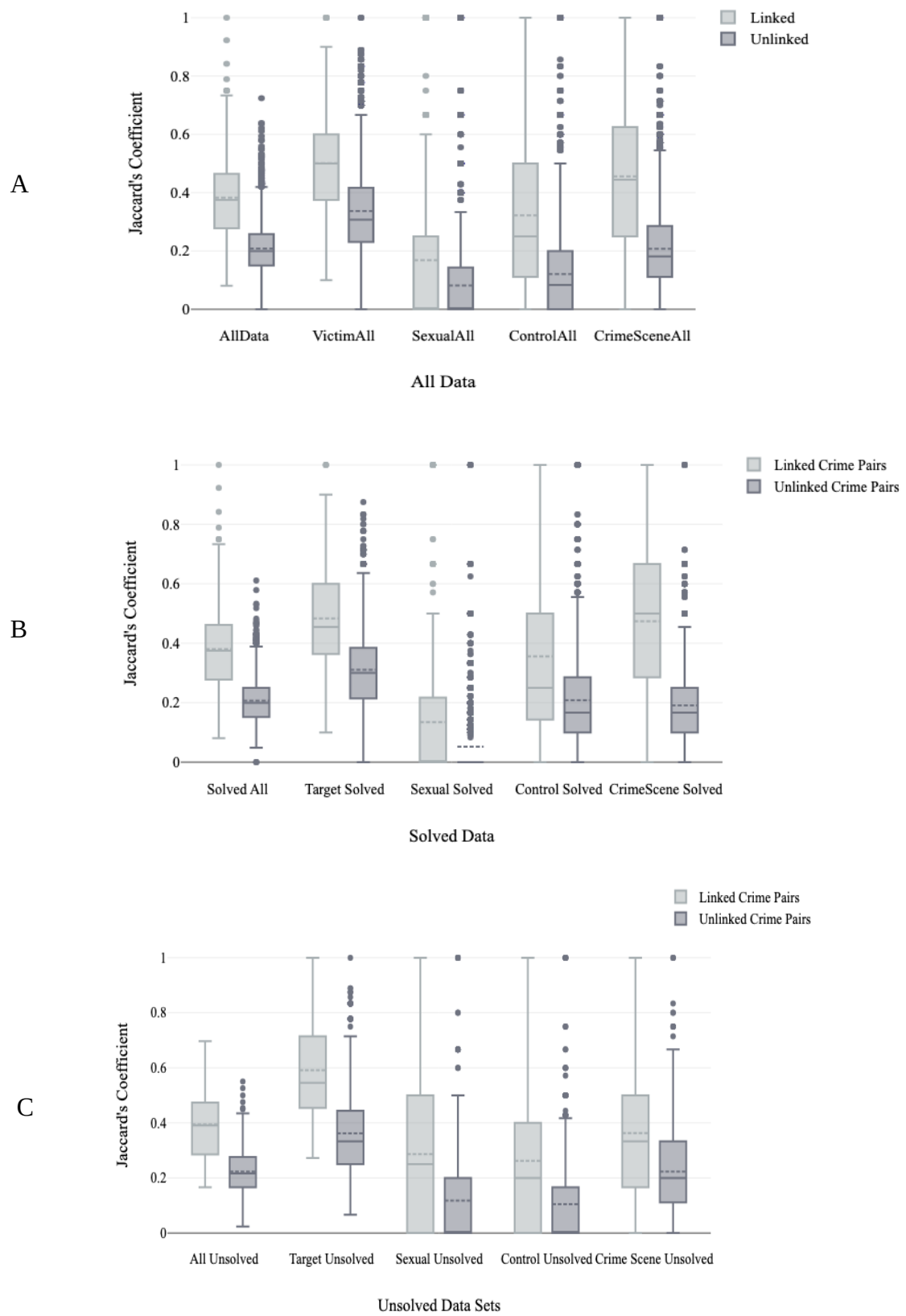
Figure 4.4 Boxplots of linked and unlinked crime pairs Jaccard's coefficients per A) all data (solved and unsolved); B) all solved data; C) all unsolved datasets.
