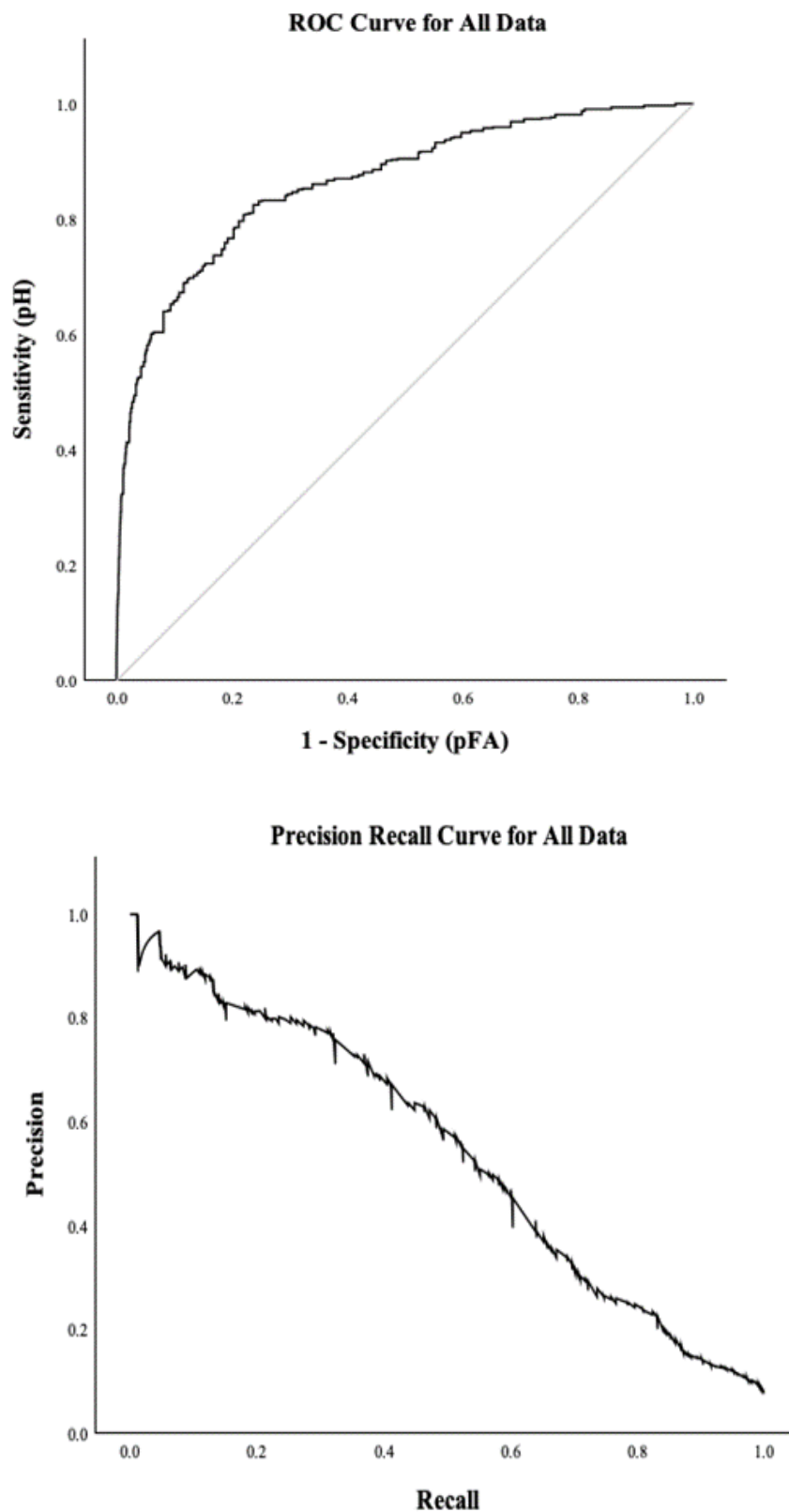
Figure 4.5 ROC and PRC for all data: AUC .87 ( p < .001 , SE = 0.1, 95% CI = .85 - .88).
