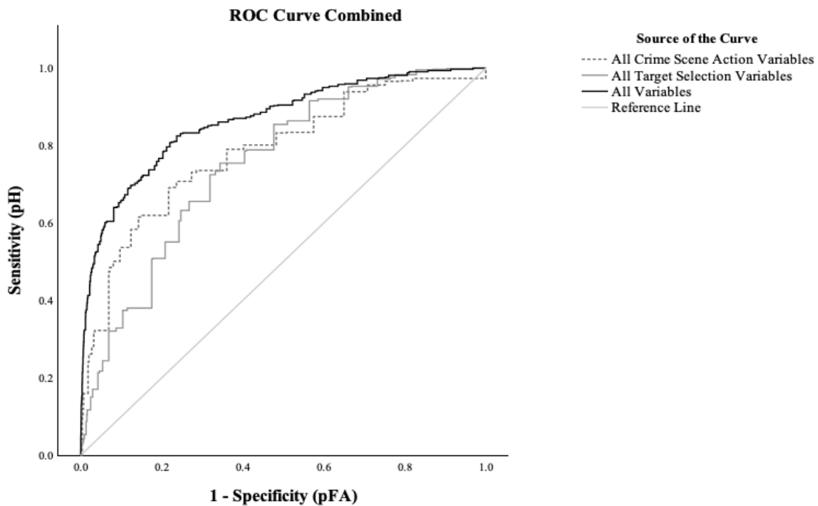
Figure 4.8 Comparison of Full ROC curves between All Data, All target selection variables, and all crime scene characteristics.
