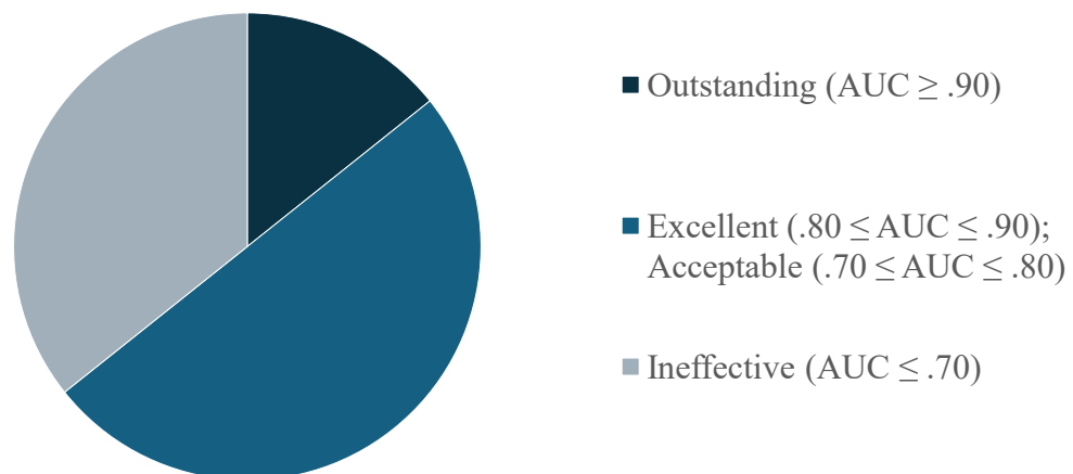
Figure 2.1 Accuracy of crime linkage studies examined by Bennell et al. (2014) according to AUC value Interpretation.
