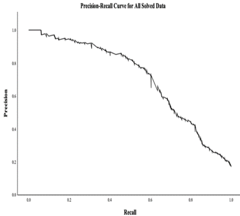
Figure 4.6 ROC and PRC for all solved data AUC .86 ( p < .001 , SE = .01, 95% CI = .85 - .88).
