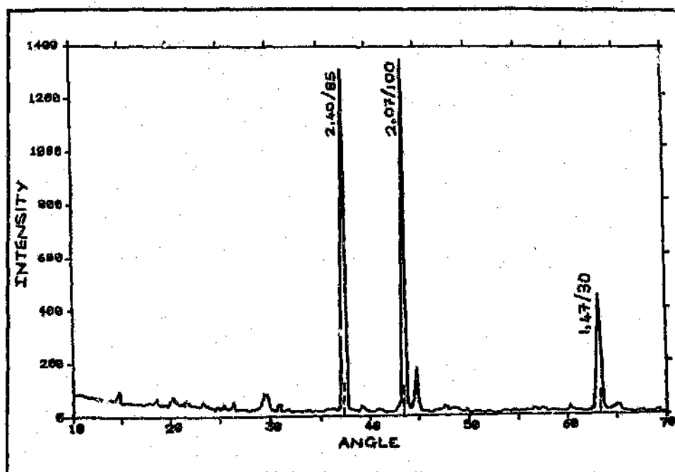
Figure.4.15. Typical diffractogram of VC coated sample.
