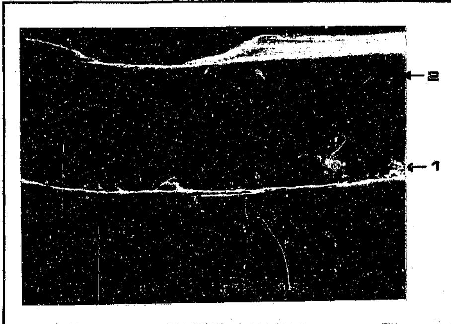
Figure.4.53. Close-up view of spalled area displaying apparent brittle fracture surface.
