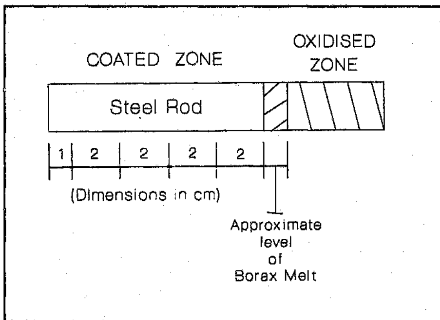
Figure.3.3. Method of sectioning of coated EN8 steel rods.
