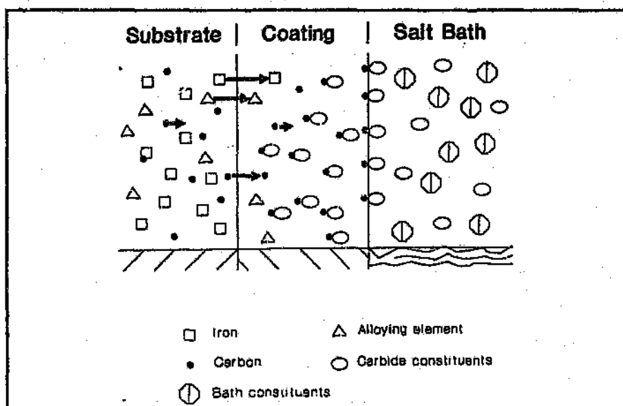
Figure.2.5.4. Growth model of carbide layer on steel surface (25).
