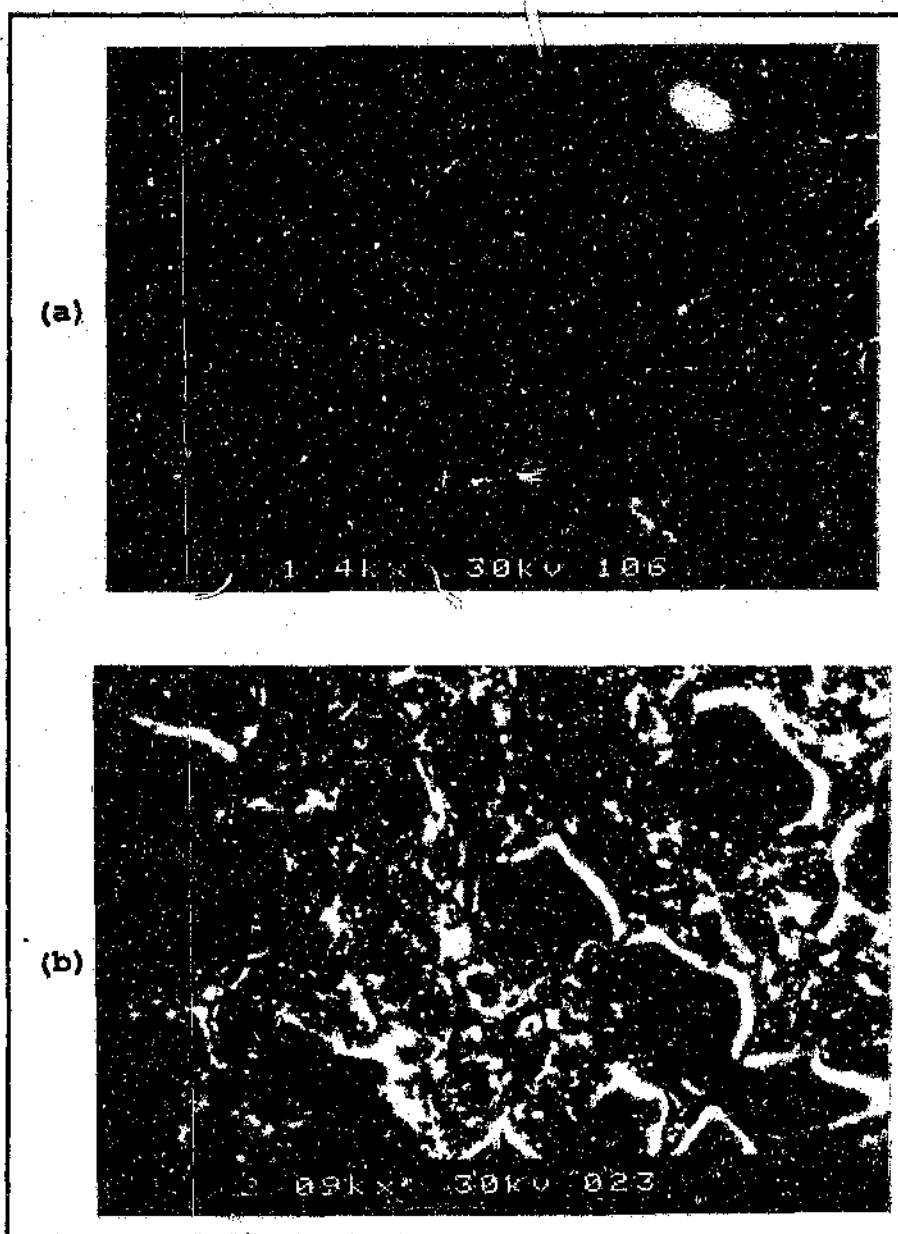
Figure.A.3.3. Microstructure of (a) as-received (b) hardened and tempered samples. Etched nital.
