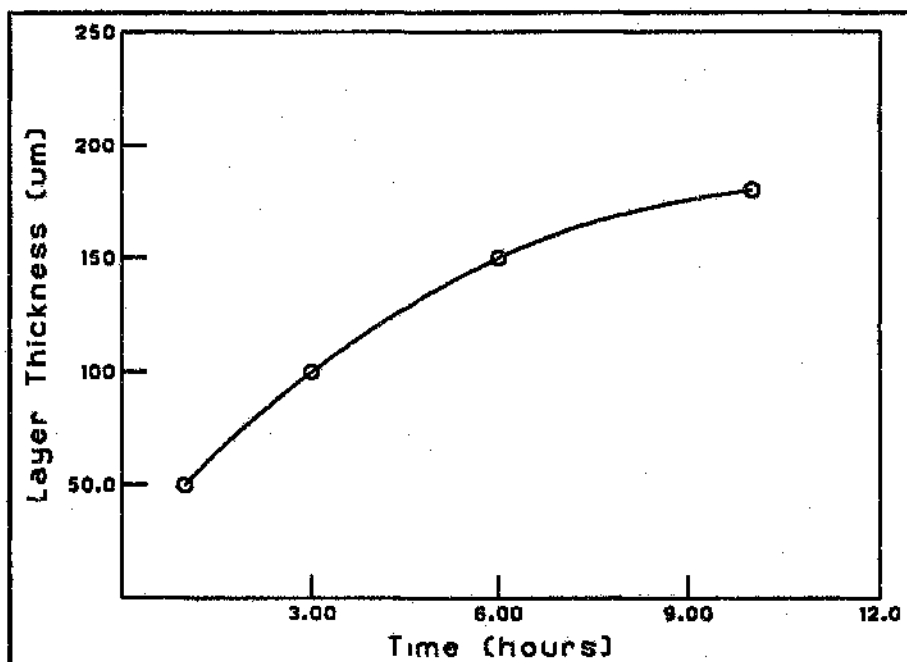
Figure.2.2.2. Variation of boride layer thickness with time (9) .
