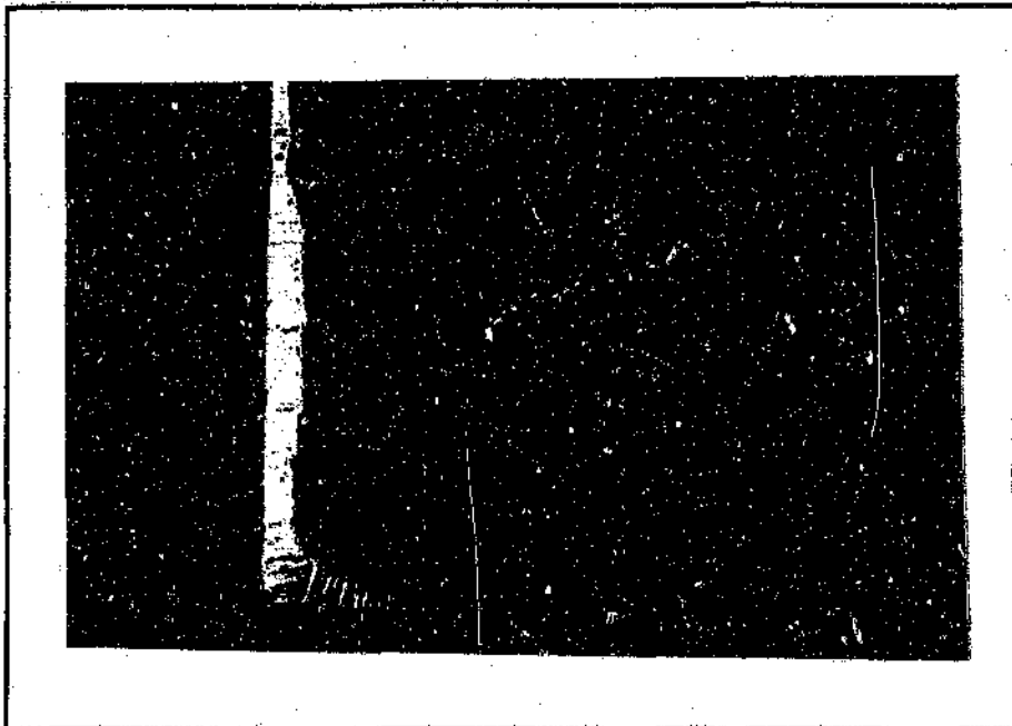
Figure.4.54. Appearance of quench cracked specimen[8X].
