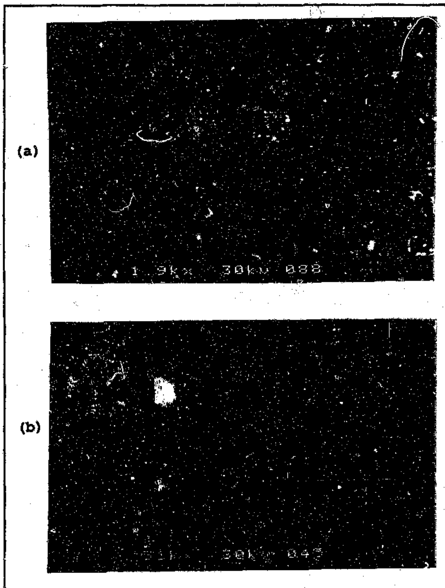
Figure.A.3.1. Microstructure of (a) as-received (b) hardened and tempered samples. Etched nital.
