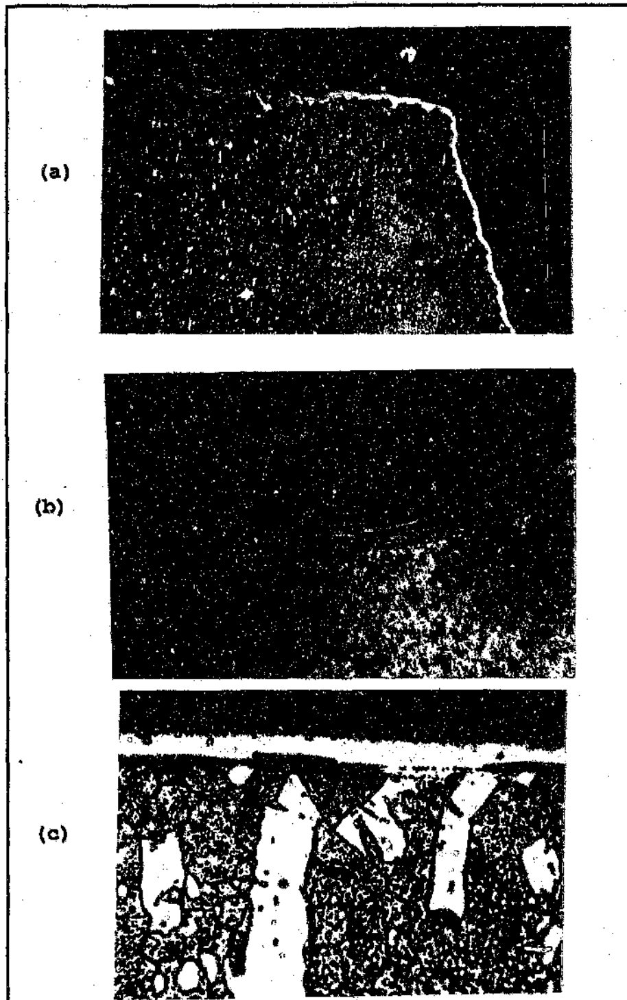
Figure.4.42. Appearance of VC coating (a)round corner[200X] (b)inside a hole[200X] (c)on D2 toolsteel[1000X]. Etched nital.
