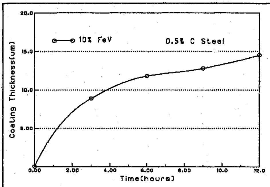
Figure.4.1. Growth of VC layer on 0.5% C steel treated in a 10% FeV bath for 3, 6, 9, and 12 hours at 950°C.
