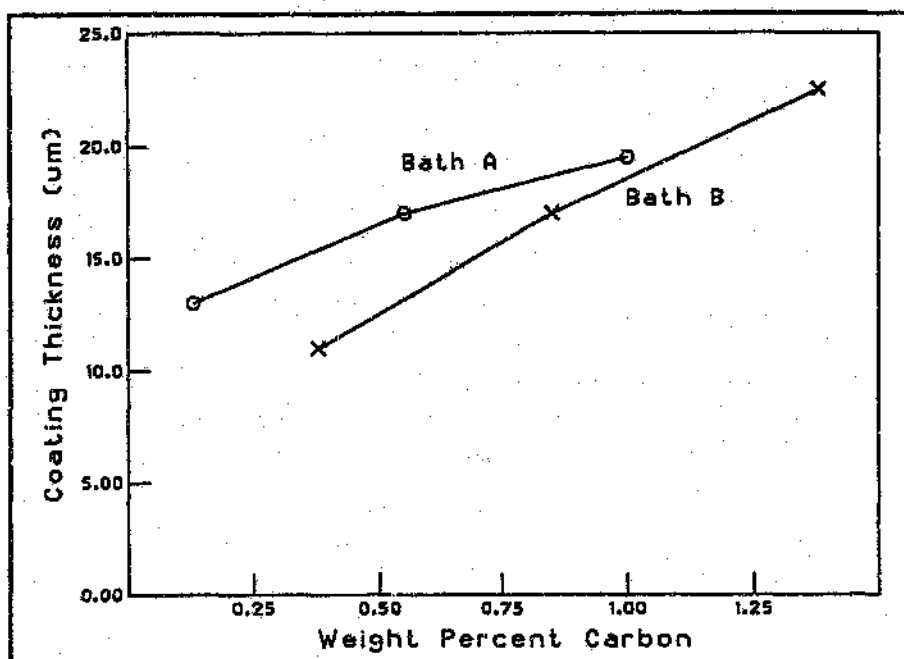
Figure.2.5.7. Effect of carbon content on layer formation rate(4 hours treatment at 1000°C) (26).
