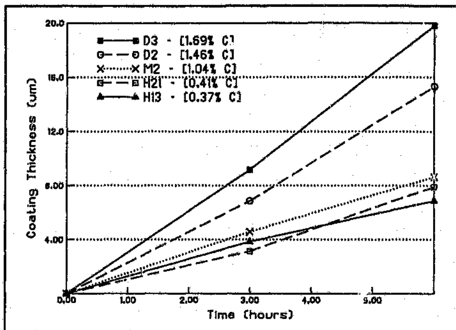
Figure.4.38. Coating thickness produced on tool steels treated for 3h and 6h at 950°C.
