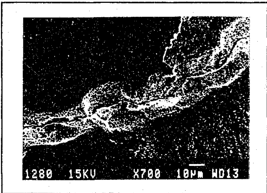
Figure.4.55. Extension of quench crack through carbide layer.
