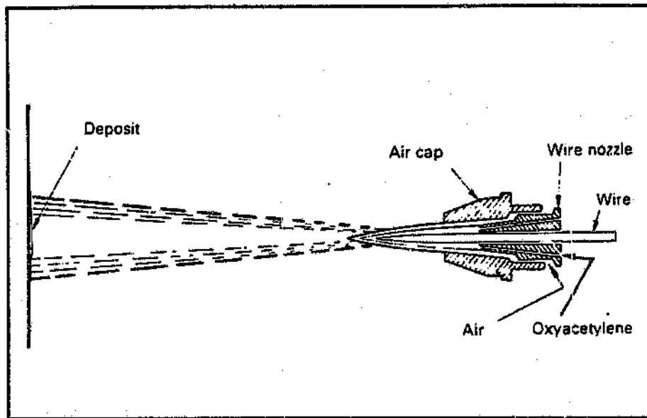
Figure.2.2.4. Oxyfuel gas wire spraying (4) .
