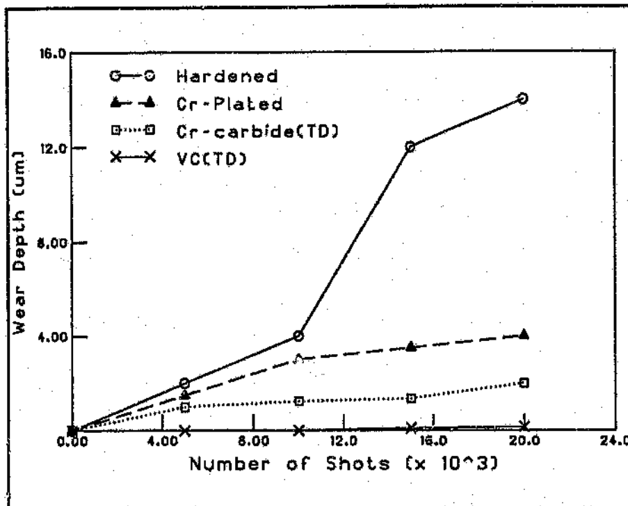
Figure.2.5.12. The effect of carbide species on wear depth in compression tests (32) .
