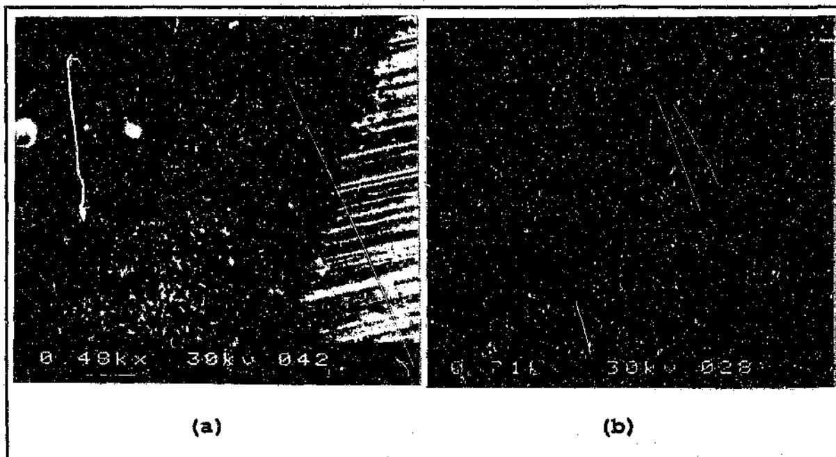
Figure.4.35. Nature of (a) lacquer/sample interface and (b) general surface corrosion of coated steel sample after potentiodynamic test.
