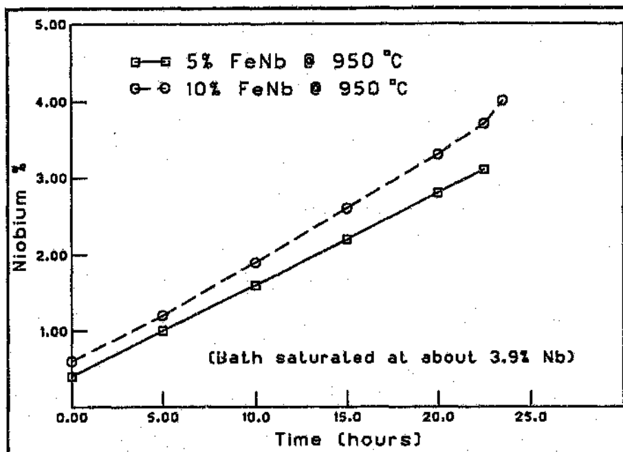
Figure.2.5.5. The time taken to establish saturation in borax/ferro-niobium baths (26) .
