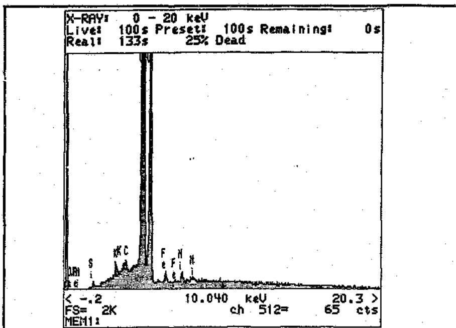
Figure.4.58. Typical EDS spectrum of "stained" area.
