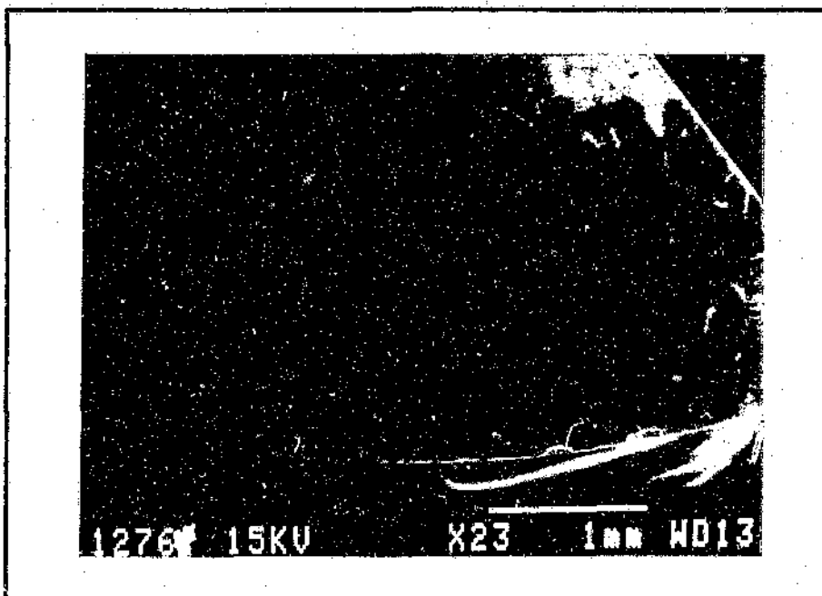
Figure.4.56. "Stained" area of coated sample.
