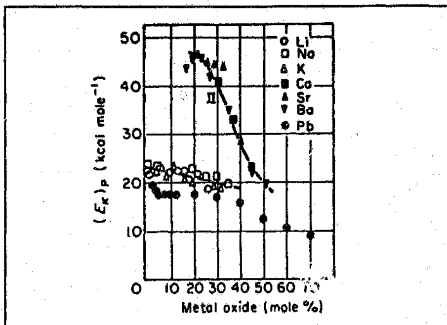
Figura.2.4.5. Activation energies for electrical conduction of some binary borates (17) .
