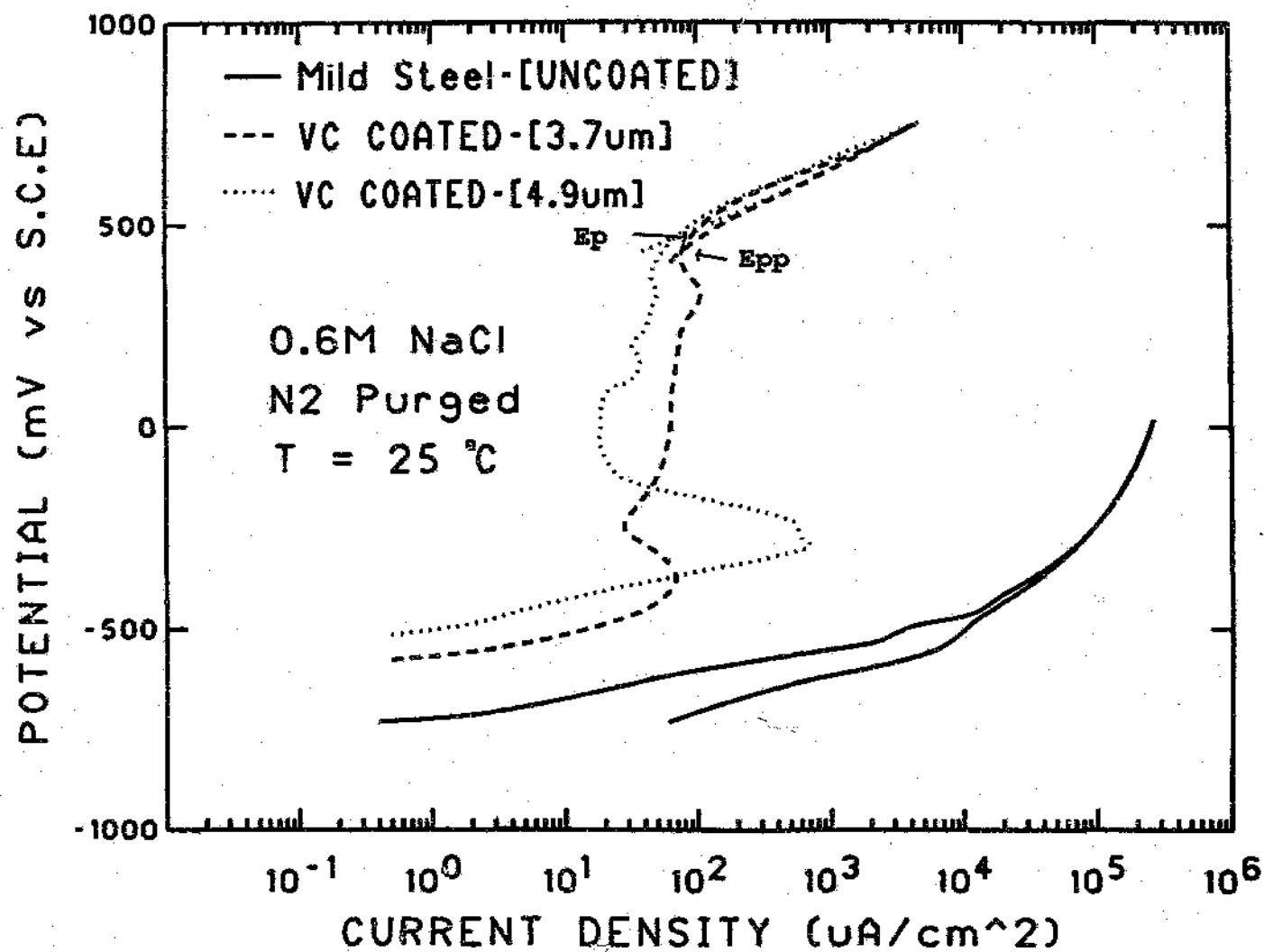
Figure.4.32. Typical cyclic polarization curves for mild steel samples.
