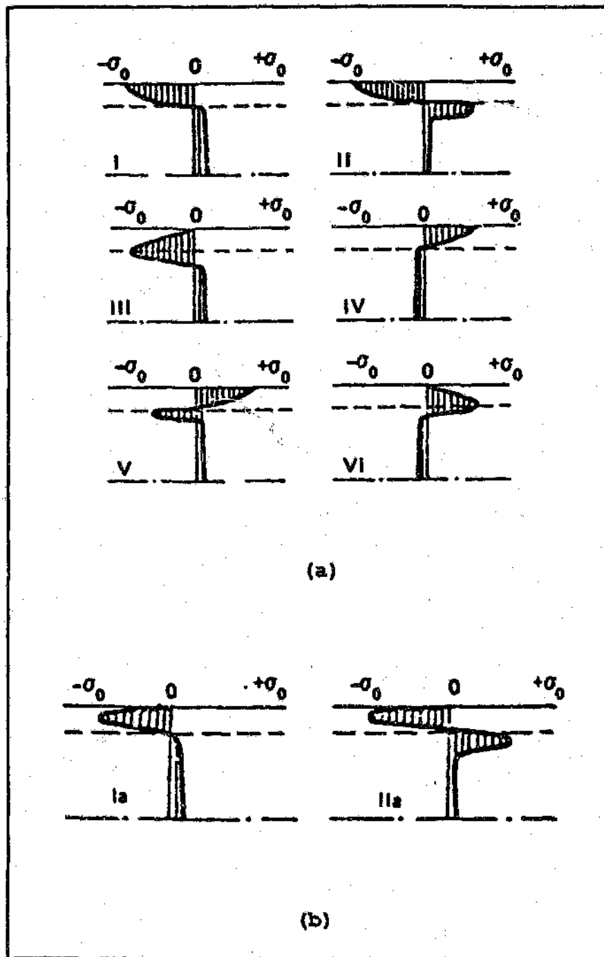
Figure.2.3.1. Basic(a) and Auxiliary(b) diagrams of the distribution of axial residual stresses (9) .
