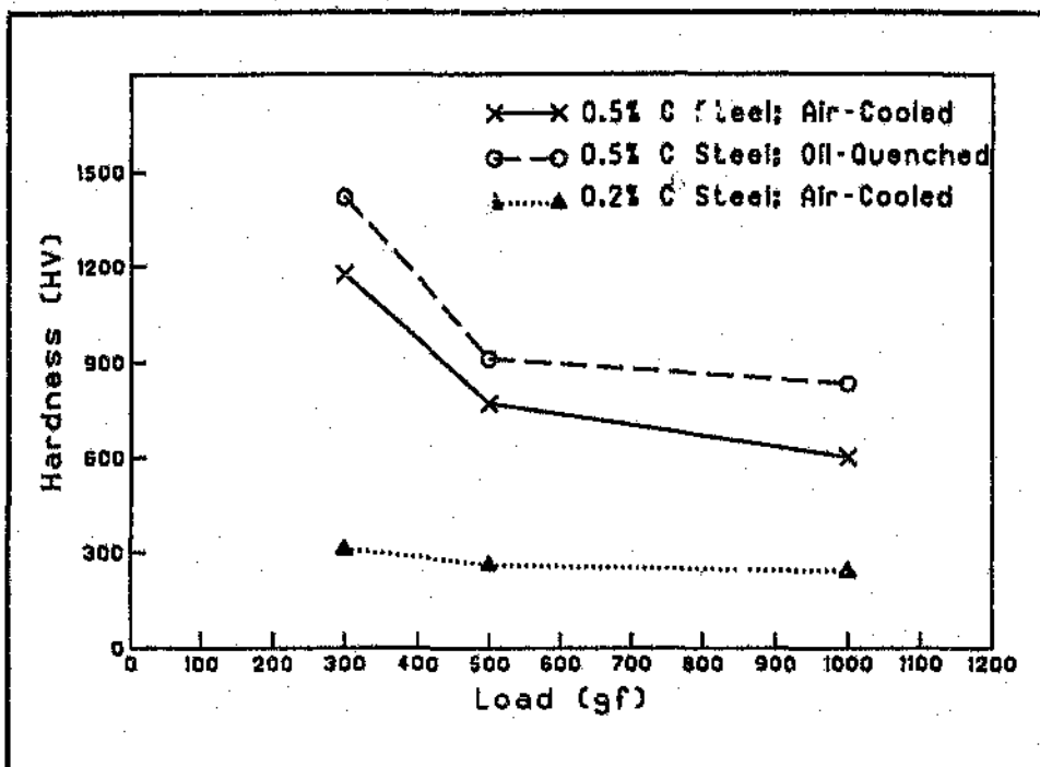
Figure.4.13. Variation in "composite" hardness with load of VC coated 0.5% C steel and 0.2% C steel.
