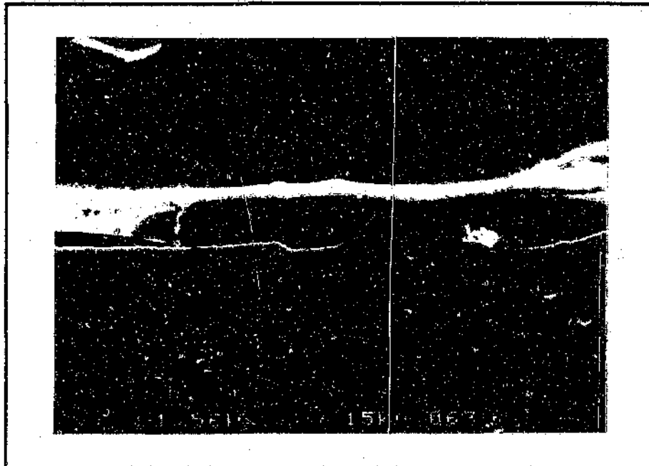
Figure.4.51. Cross-sectional view of spalling carbide layer typifying varying extent to which spalling occurred.
