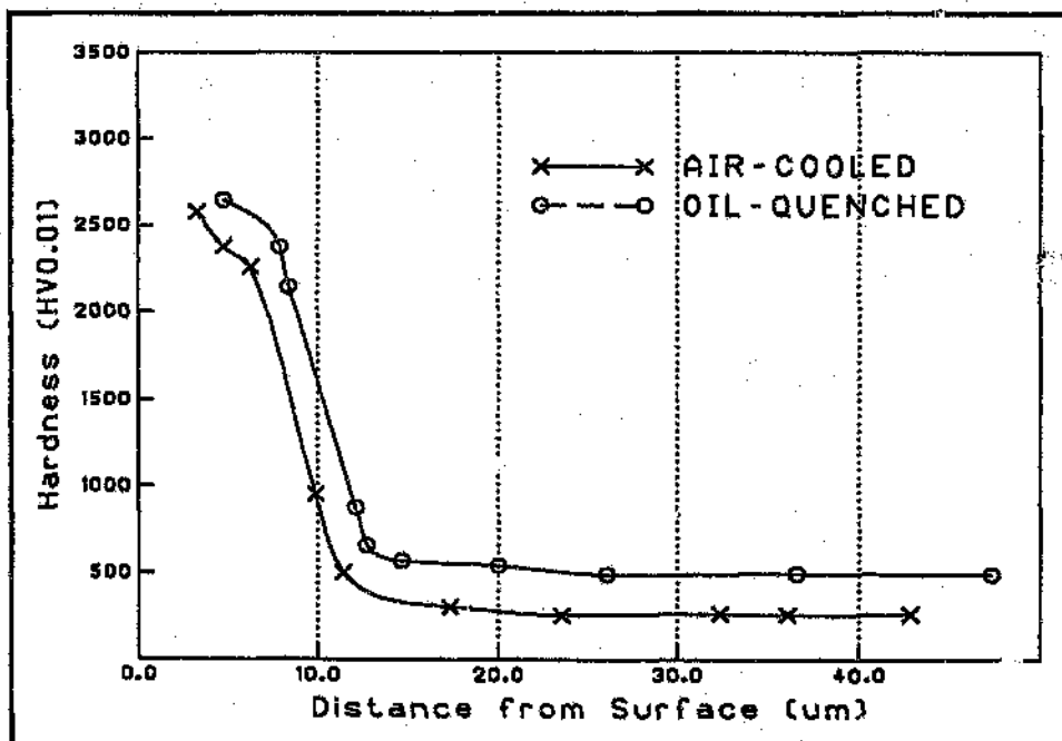
Figure.4.12. Hardness profiles on VC coated 0.5% carbon steel samples (Load = 10gf).
