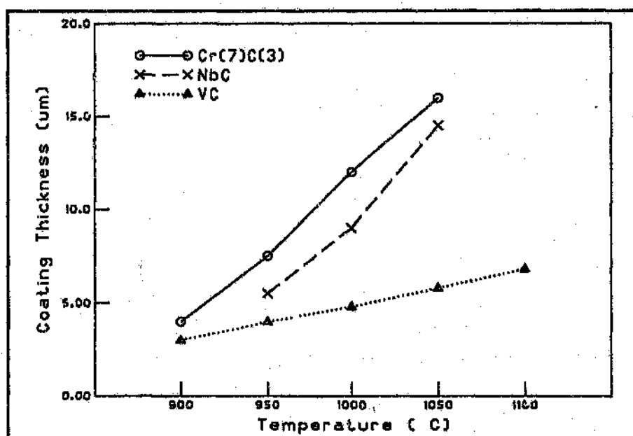
Figure.2.5.8. Effect of carbide type on layer formation rate(4 hours treatment at 1000°C) (26).
