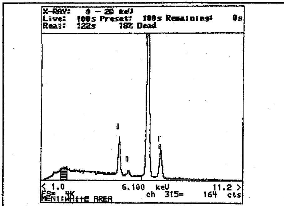
Figure.4.47. Typical EDS spectrum of light area using spot analyses.
