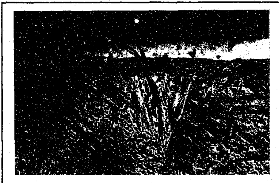
Figure.4.9. Microstructure of hardened 0.5% C steel after coating at 950°C. Etched nital, 1000X.
