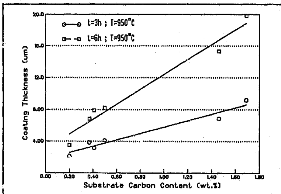
Figure.4.39. Variation in coating thickness with substrate carbon content for 3h and 6h treatment times at 950°C.
