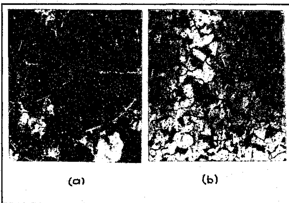
Figure.4.6. Microstructure of (a) 0.5% C (400X) and (b) 0.2% C (400X) steel towards the core of treated samples, nital etch.
