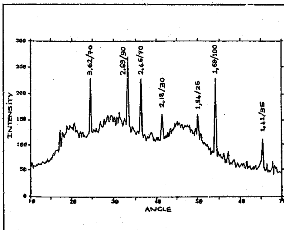
Figure.4.29. Typical diffractogram of bath sample.
