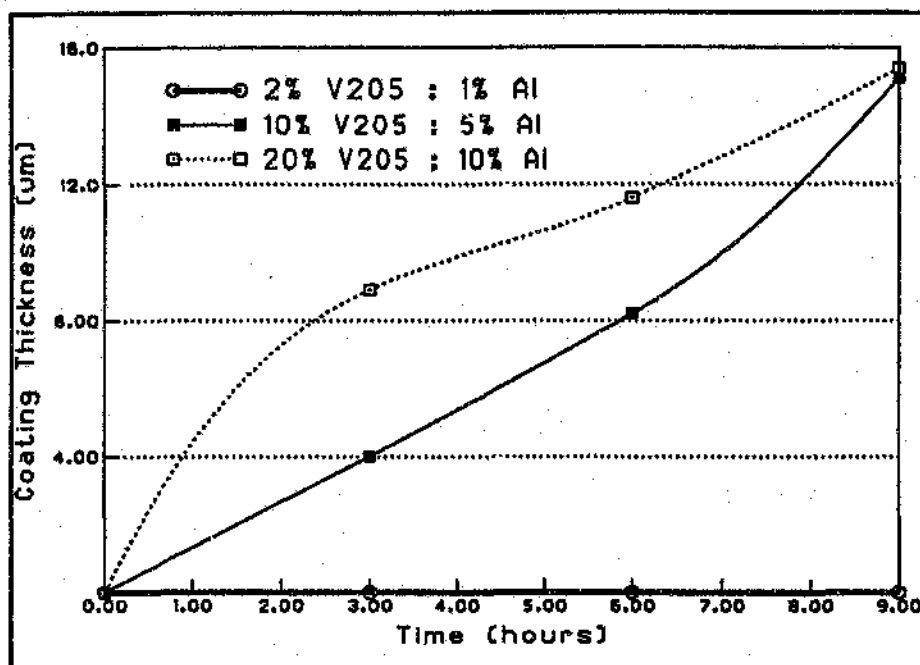
Figure.4.20. Change in bath activity with bath composition at 950°C ( V_2O_5:Al = 2:1 ).
