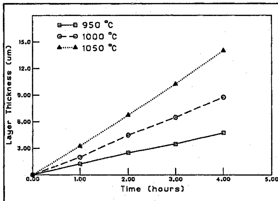
Figure.2.5.6. Effect of treating temperature and time on thickness of NbC layer (30) .
