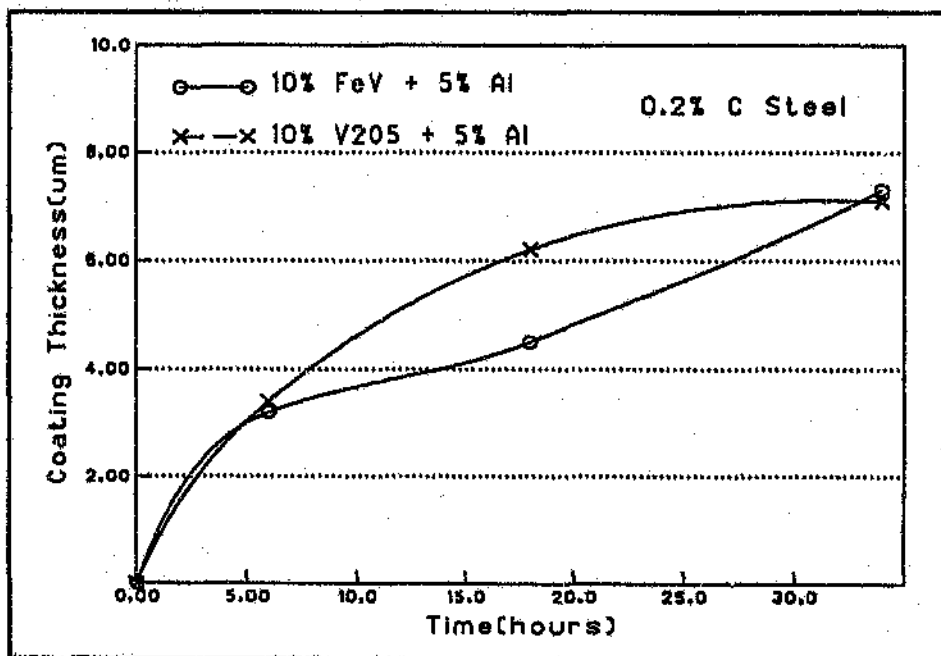
Figure.4.2. Comparison of the activities of baths containing FeV and V 2 O 5 .
