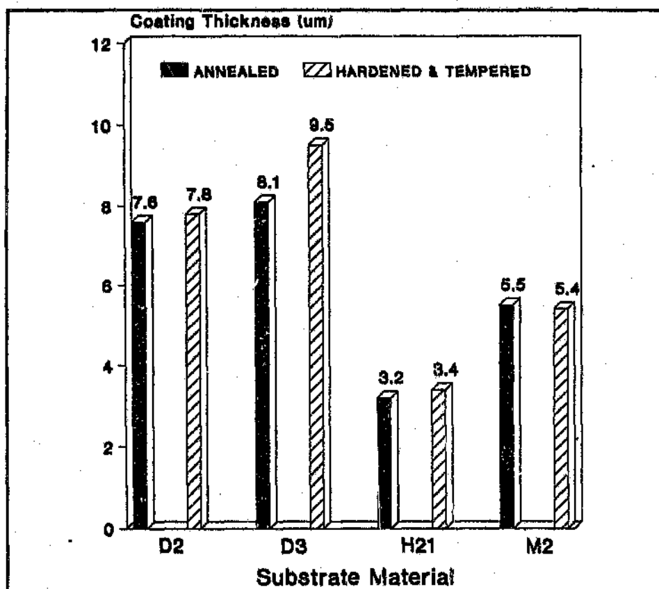
Figure.4.40. Comparison of average coating thicknesses produced on annealed and heat treated substrate treated for 3h at 950°C.
