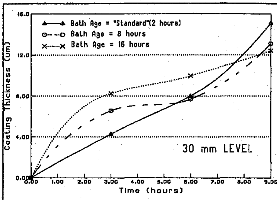
Figure.4.25. Comparison of coating thicknesses produced on 0.5% C steels treated in three 10% V_2O_5 and 5% Al baths aged for 2h, 8h, and 16h respectively.
