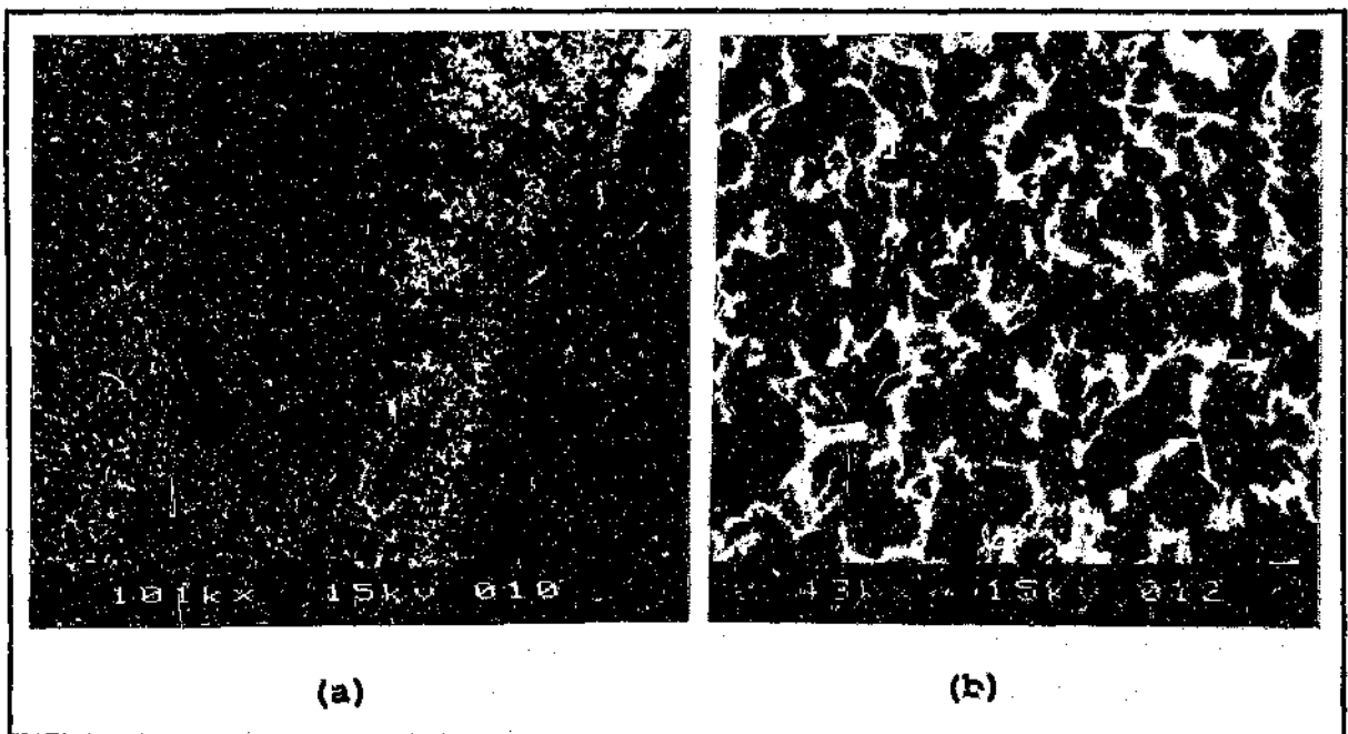
Figure.4.37. Extensive corrosion of uncoated steel substrate: (a) Lacquer/sample interface (b) General surface corrosion.
