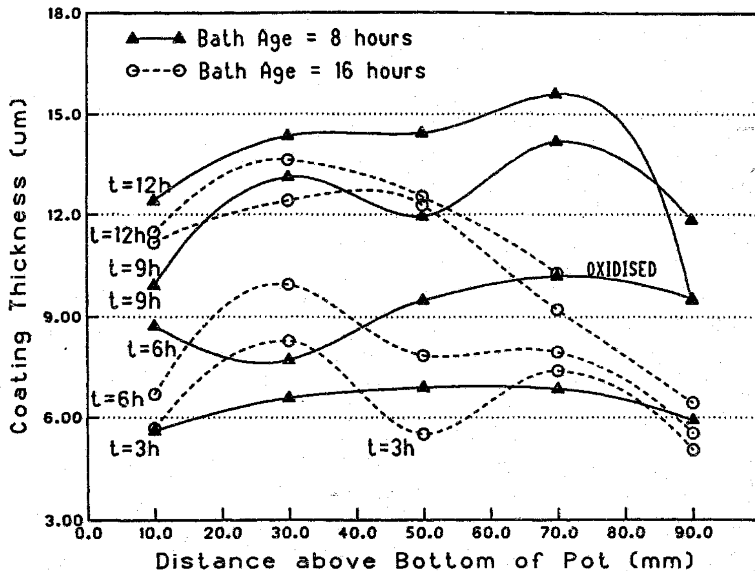
Figure 4.23. Variation in coating thickness with distance above the bottom of the bath for rods treated in baths aged for 8h and 16h.
