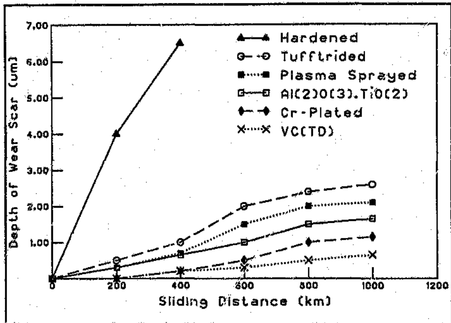
Figure.2.5.10. Comparison of wear resistance of VC coatings in sliding wear test against textile fiber (27) .
