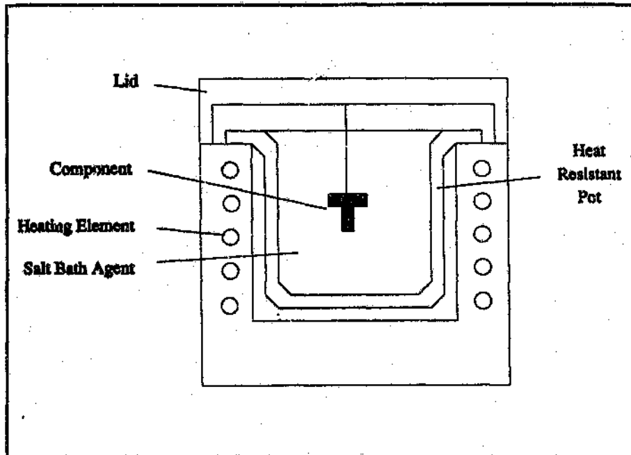
Figure.2.5.1. Salt bath furnace for carbide coating (27) .
