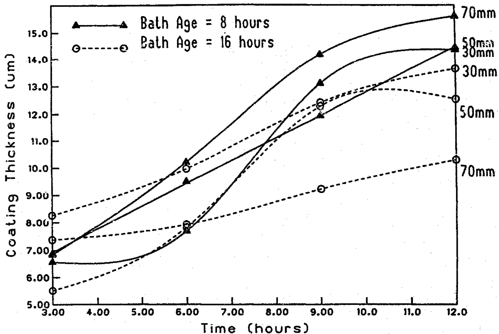
Figure.4.24. Comparison of coating thicknesses at distances of 30mm, 50mm, and 70mm above the bath bottom on rods treated in baths aged 8 and 16 hours.
