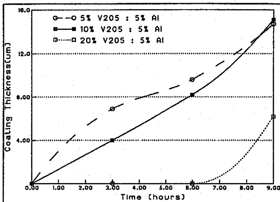
Figure.4.18. Effect of %V 2 O 5 on the thickness of coatings produced at 950°C and 3, 6, or 9h of treatment.
