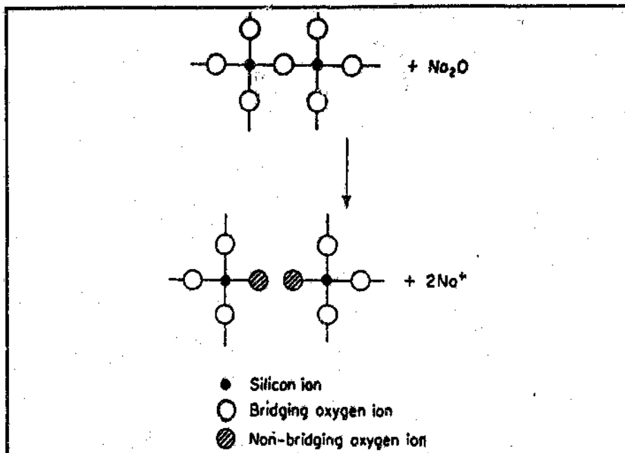
Figure.2.4.2. Reaction between sodium oxide and silica tetrahedra (17) .
