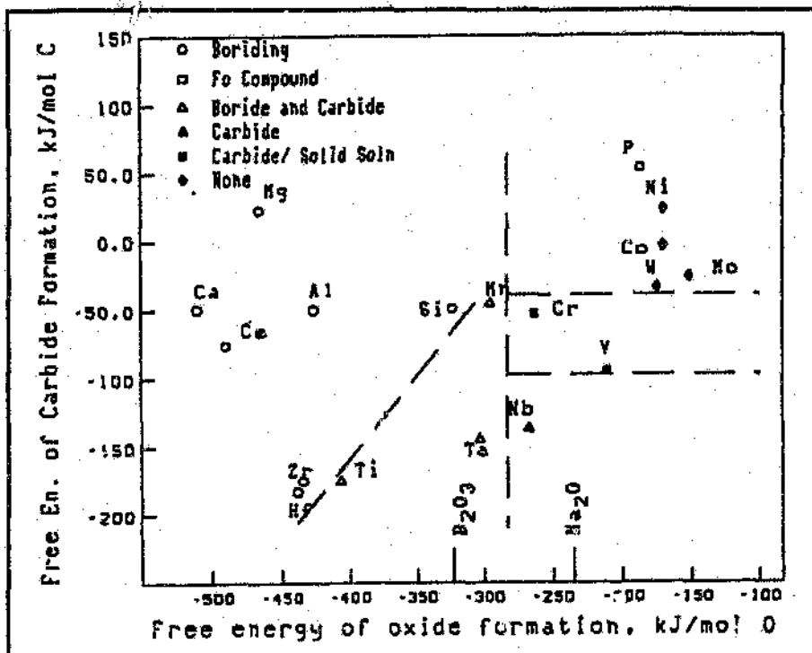
Figure.2.5.3. Relationship between free energy of formation of oxides of elements contained in the bath and kinds of layers formed(1000°C) (25).
