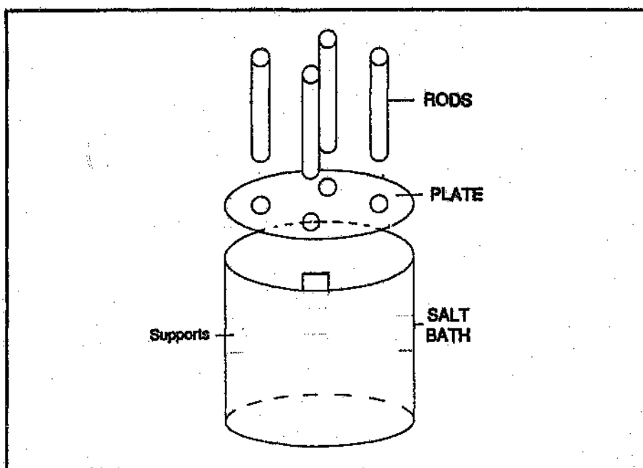
Figure.3.2. Method of immersion of sample rods.
