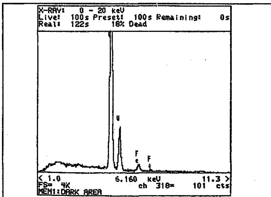
Figure.4.48. Typical EDS spectrum of darker area using spot analyses.
