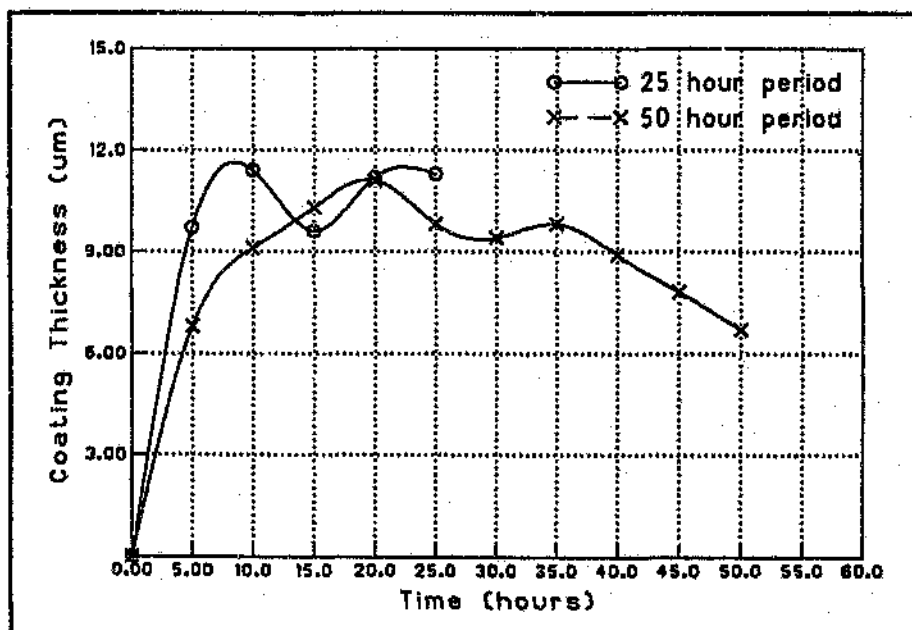
Figure.4.22. Change in bath activity over 25h and 50h periods at 950°C. Samples treated in 5h intervals.
