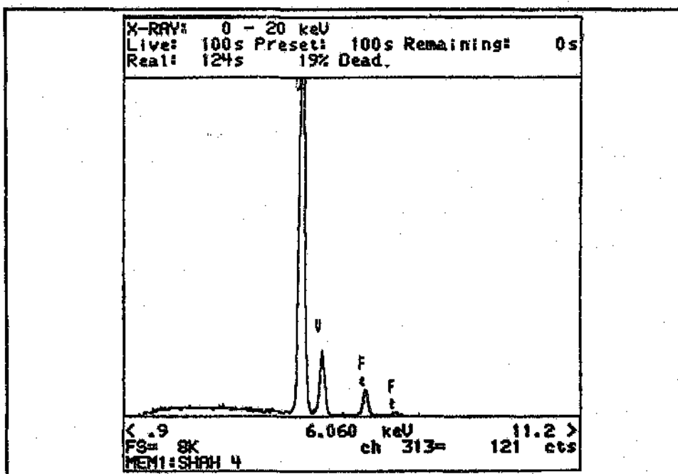
Figure.4.14. Typical EDS spectrum of VC Coating.
