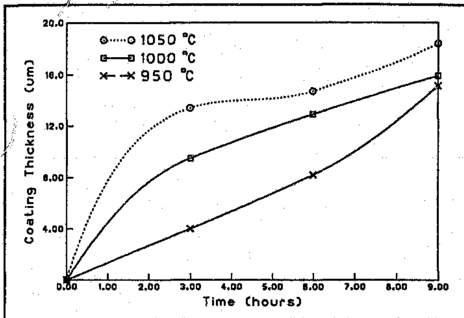
Figure.4.16. Effect of temperature on coating thickness produced in a bath of 10% V_2O_5 plus 5% Al.
