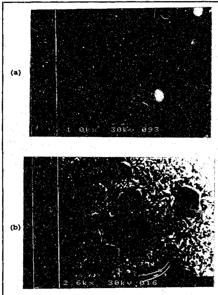
Figure.A.3.2. Microstructure of (a) as-received (b) hardened and tempered samples. Etched nital.
