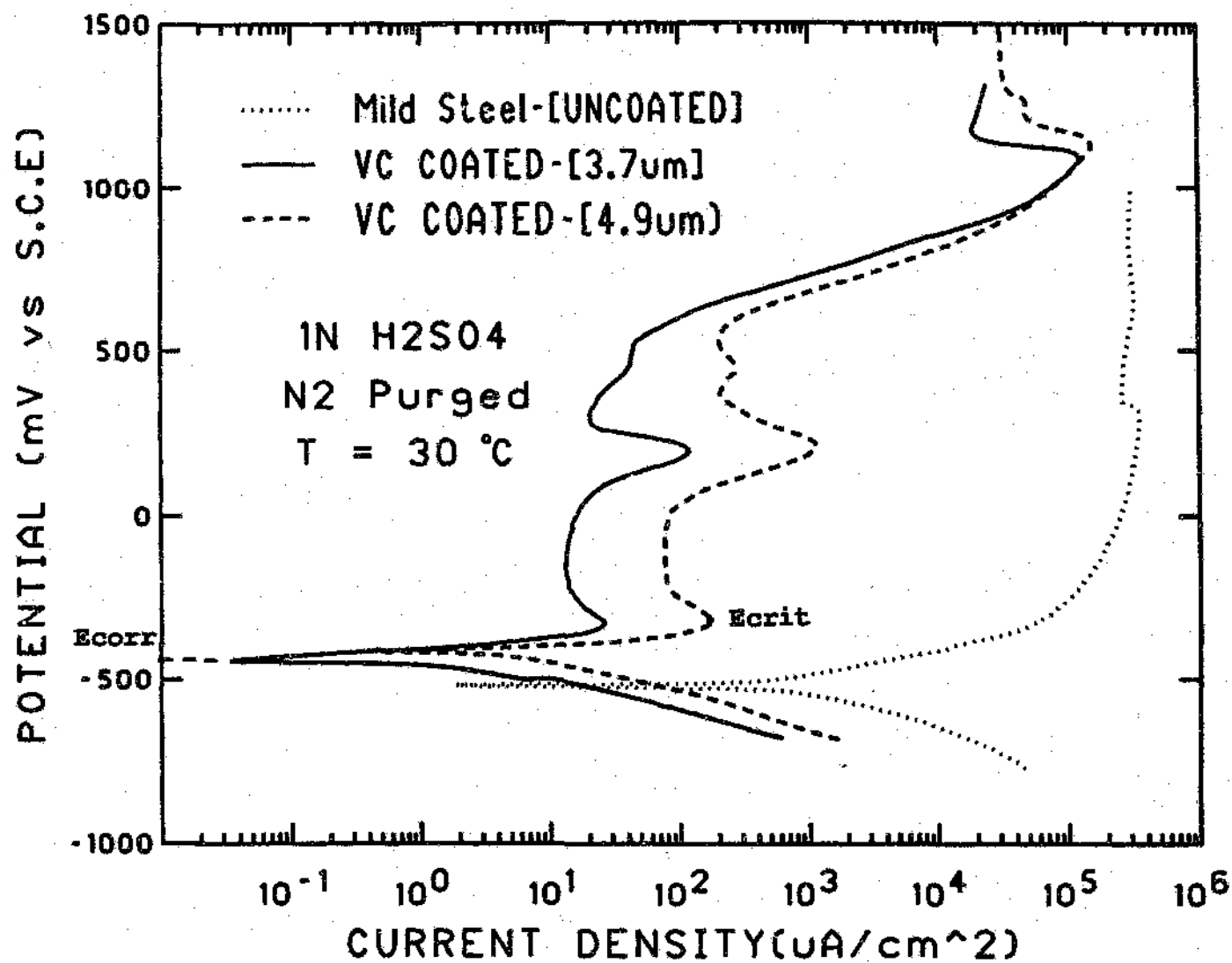
Figure.4.30. Typical potentiodynamic curves for mild steel samples.
