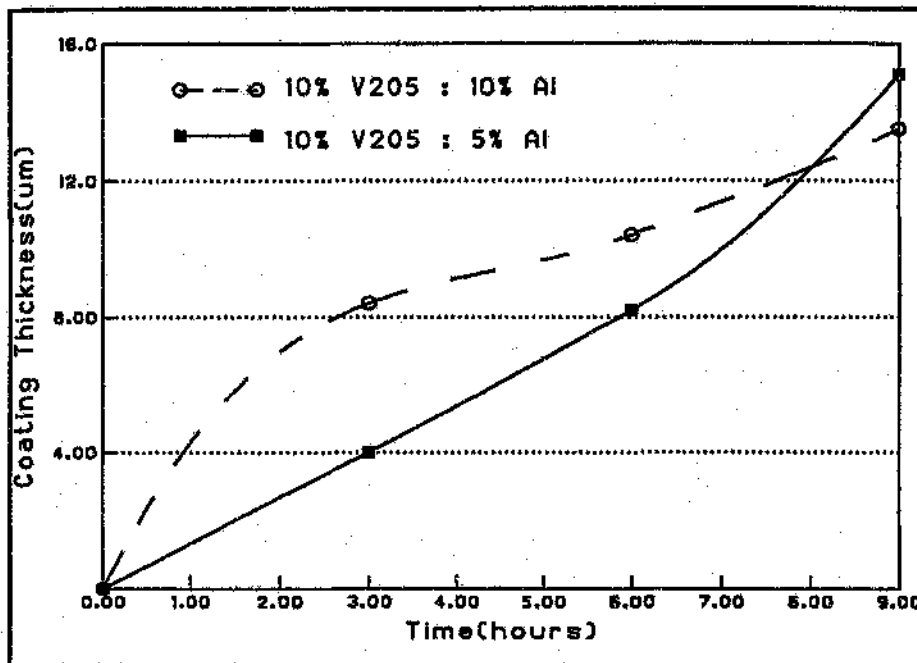
Figure.4.19. Effect of %Al on bath activity at 950°C for 3, 6, 9h of treatment.
