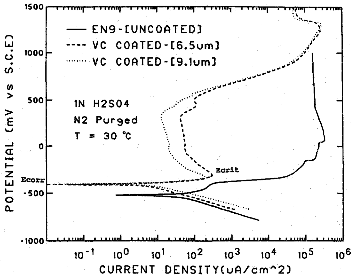
Figure.4.31. Typical potentiodynamic curves for EN9 steel samples.
