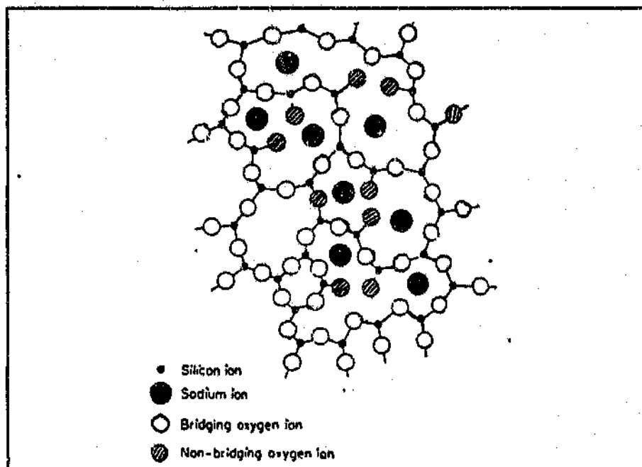
Figure.2.4.3. 2-Dimensional representation of the structure of soda-silica glass (17) .
