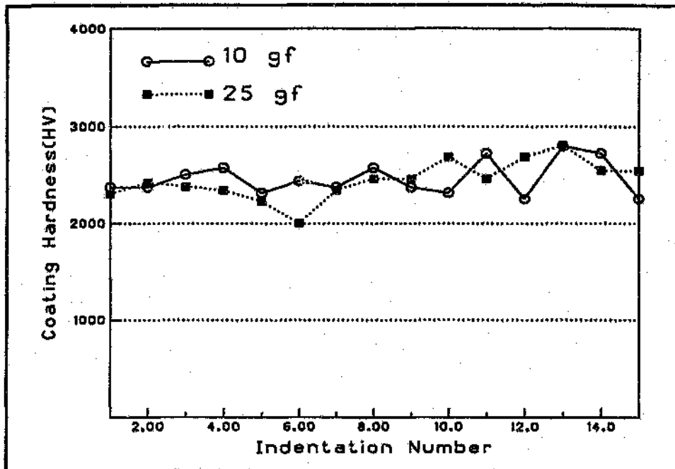
Figure.4.11. Variation in hardness with load. Average coating thickness = 11.3 \mu\text{m} .
