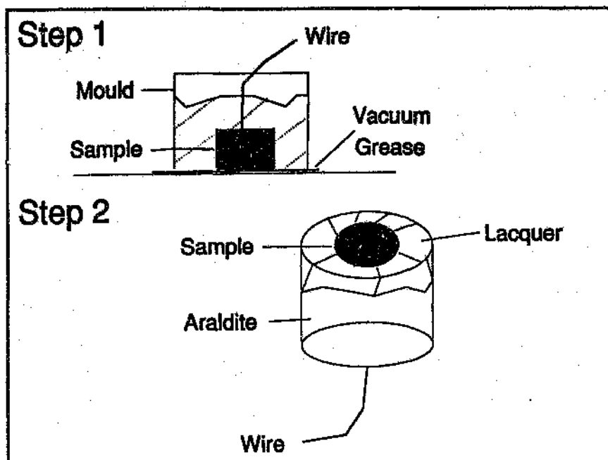
Figure.3.4. Method of mounting of corrosion samples.
