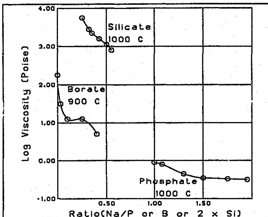
Figure.2.4.4. The effect of sodium oxide addition on the viscosities of its mixtures with P_2O_5 , B_2O_3 , and SiO_2 (21) .
