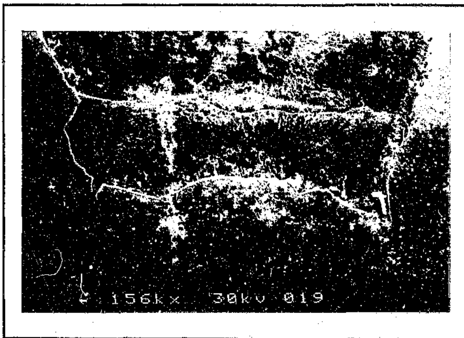
Figure.4.50. Spalling of carbide layer.
