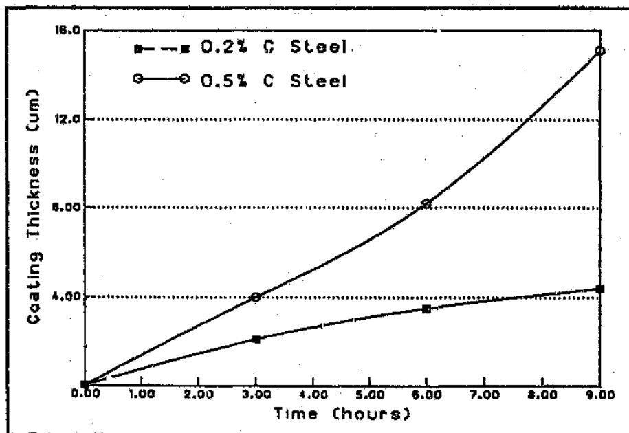
Figure.4.17. Comparison of carbide layer growth on 0.2% and 0.5% C steels treated at 950°C for 3, 6, and 9h.
