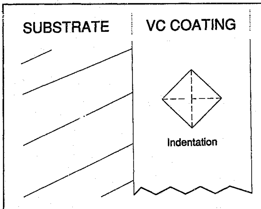
Figure.3.1. Position of hardness indentations in coated specimens.
