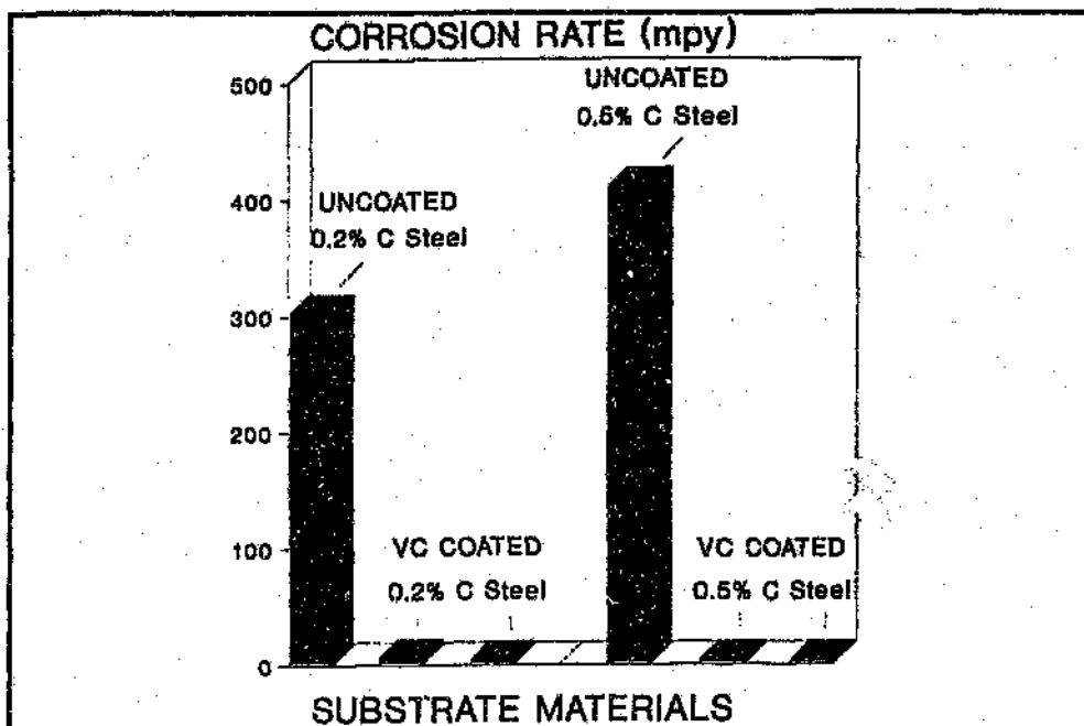
Figure.4.34. Comparison of corrosion rates of coated and uncoated substrate.
