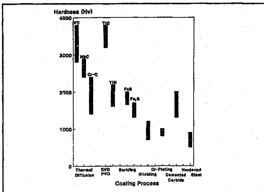
Figure.2.5.9. Variation in hardness with carbide species (32) .
