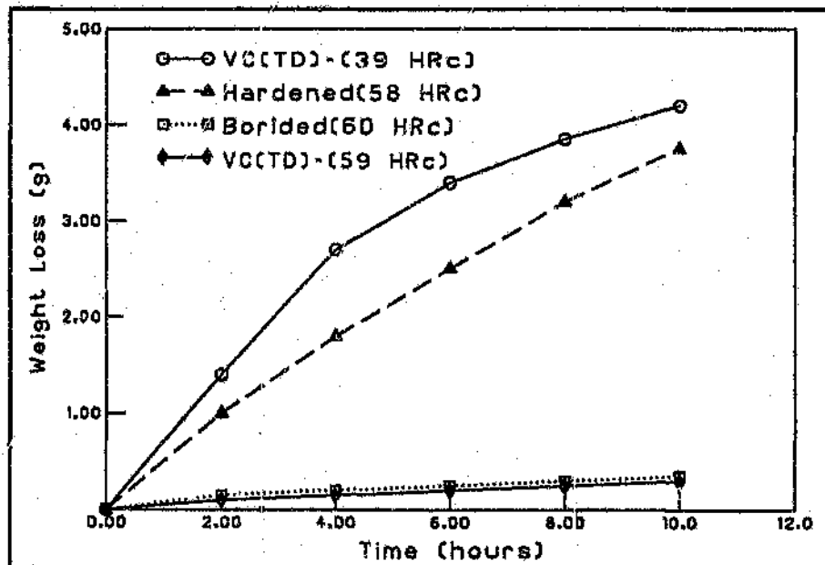
Figure.2.5.11. The effect of substrate hardness on wear loss in sand crushing tests (32) .
