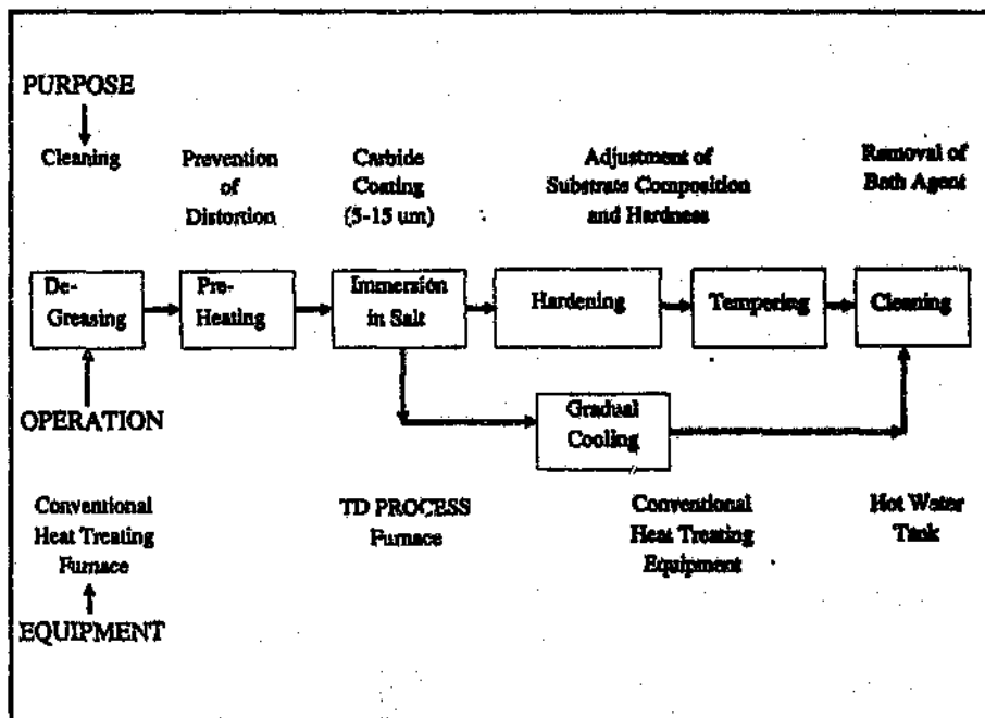
Figure.2.5.2. Outline of the TD Process (27) .
