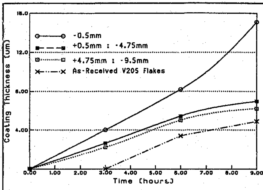
Figure.4.21. Effect of particle size on bath activity at 950°C for 3, 6, and 9h of treatment.
