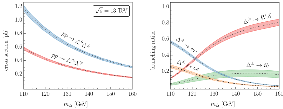
Fig. 2. (color online) Left: Production cross-section for pp \rightarrow \Delta^0 \Delta^+ and pp \rightarrow \Delta^+ \Delta^+ as a function of the triplet mass including the NNLL and NLO QCD correction factor and uncertainties of Refs. [63, 64]. Right: Dominant branching ratios of the charged component \Delta^+ as a function of its mass. The errors are estimated from the decays for a SM Higgs with a higher (hypothetical) mass from h \rightarrow t\bar{t}^*, ZZ^* and h \rightarrow c\bar{c} [65]. While these uncertainties are sizable, we checked that their impact on the final significance is very small ( \approx 0.1\sigma ).
