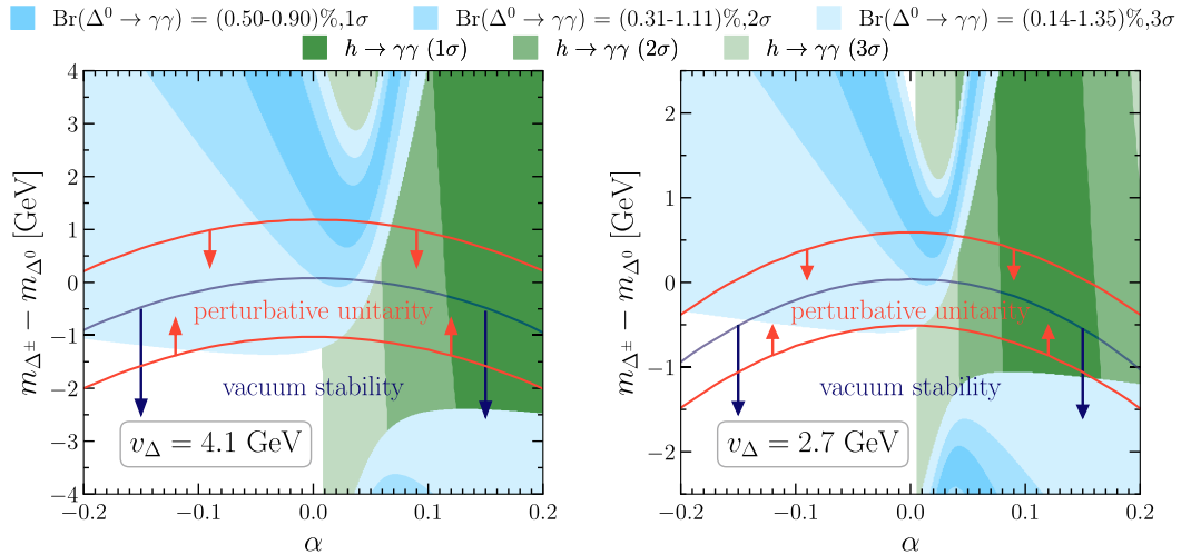
Fig. 6. (color online) Preferred regions in the \alpha vs m_{\Delta^\pm} - m_{\Delta^0} plane for m_{\Delta^0} = 152 GeV and two values of v_\Delta : 4.1 GeV (left) and 2.7 GeV (right), corresponding to the central value obtained from the global electroweak fit with and without including the CDF-II measurement. The band between the two orange lines satisfies perturbative unitarity and the one below the blue line leads to a stable vacuum at the electroweak scale. The green regions are allowed by the SM Higgs signal strength to photons ( h \rightarrow \gamma\gamma ) [73, 74] at the 1\sigma (1.02–1.15), 2\sigma (0.96–1.22), and 3\sigma (0.90–1.29) levels. The 1\sigma , 2\sigma , and 3\sigma regions for \text{Br}(\Delta^0 \rightarrow \gamma\gamma) are shown in violet. Note that both \text{Br}(\Delta^0 \rightarrow \gamma\gamma) and \text{Br}(h \rightarrow \gamma\gamma) are sensitive to mass splitting since this determines the tri-linear Higgs coupling entering the processes via the \Delta^\pm loop.
