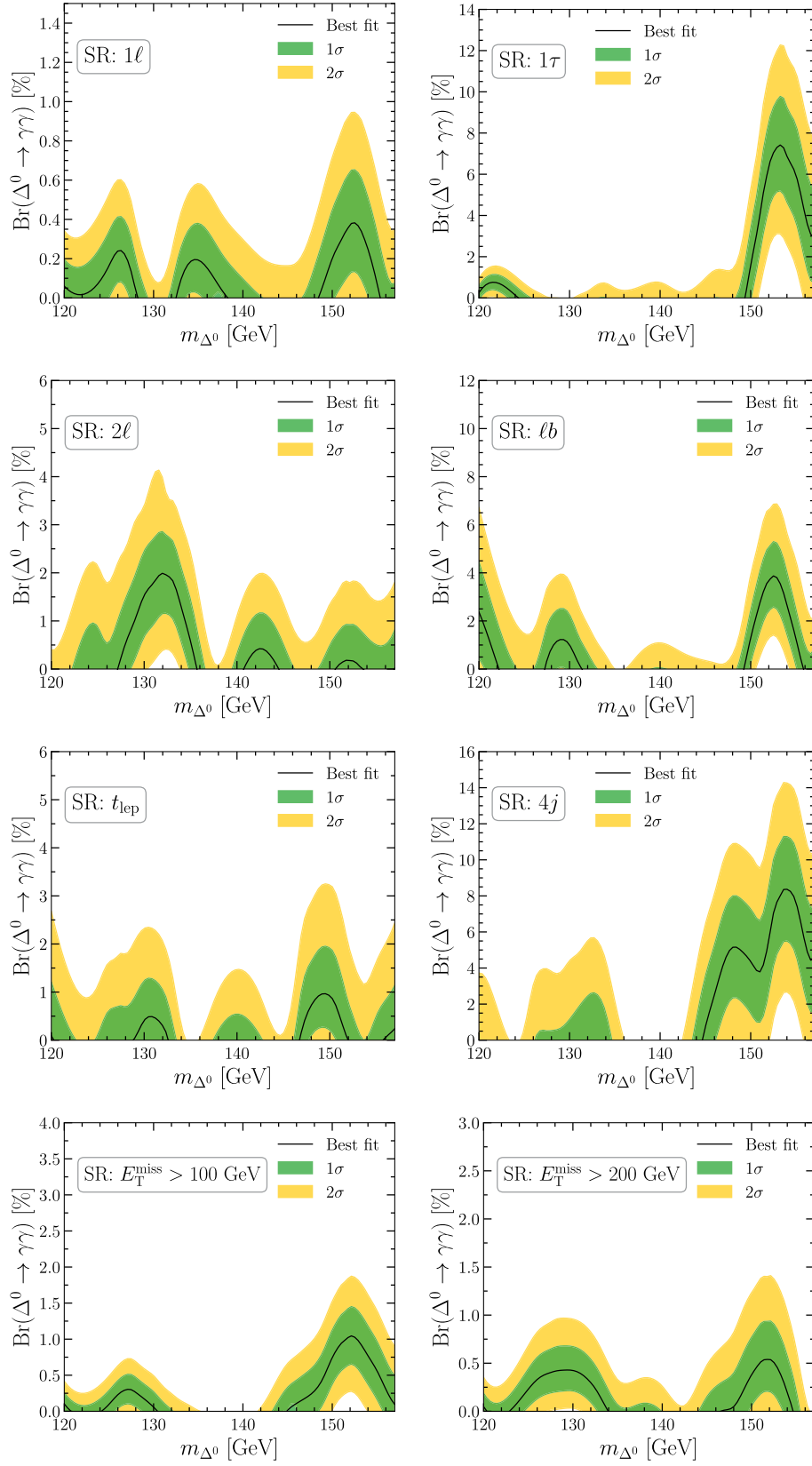
Fig. 4. (color online) Preferred range for the branching ratio of \Delta^0 \rightarrow \gamma\gamma for the eight signal regions sensitive to the our model's signal. Note that four of the signal regions show significant excesses at \approx 152 GeV while the other channels will be included as constraints in the combined fit.
