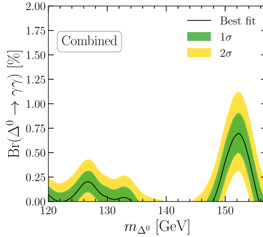
Fig. 5. (color online) Statistical combination of the eight relevant channels including their correlations within the \Delta SM, resulting in a significance of \approx 4\sigma at m_\Delta \approx 152 GeV. Note that this significance includes the slight tensions between the different signal regions shown in Fig. 4.
