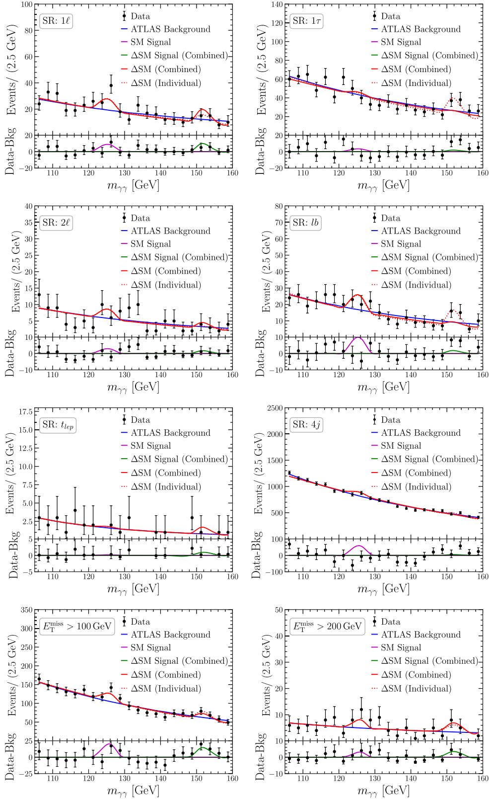
Fig. 3. (color online) Di-photon invariant mass distributions for the eight relevant signal regions. The data (black) is shown together with the continuum background (blue) from the ATLAS analyses and the total \Delta SM events (red). The latter is comprised of the refitted background (not shown for brevity), the predicted SM Higgs signals at 125 GeV (magenta) and 152 GeV (green). The solid (dotted) lines correspond to combined (individual) best-fit signals.
