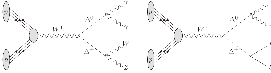
Fig. 1. Feynman diagrams showing the Drell-Yan production and decays of the triplet Higgses: pp \rightarrow W^* \rightarrow (\Delta^\pm \rightarrow tb, WZ)(\Delta^0 \rightarrow \gamma\gamma) , which we search for using the side-bands of the SM Higgs analyses of ATLAS [59, 60].
