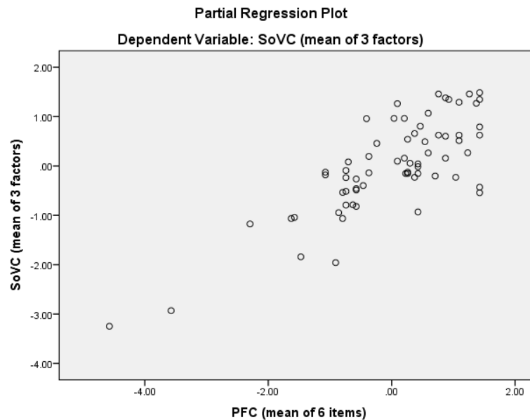
Figure 16: Partial regression plot: SoVC (Mean of 3 Factors) and PFC
