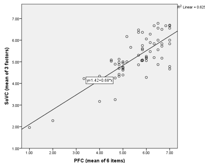
Figure 9: PFC and SoVC plot, with regression line
