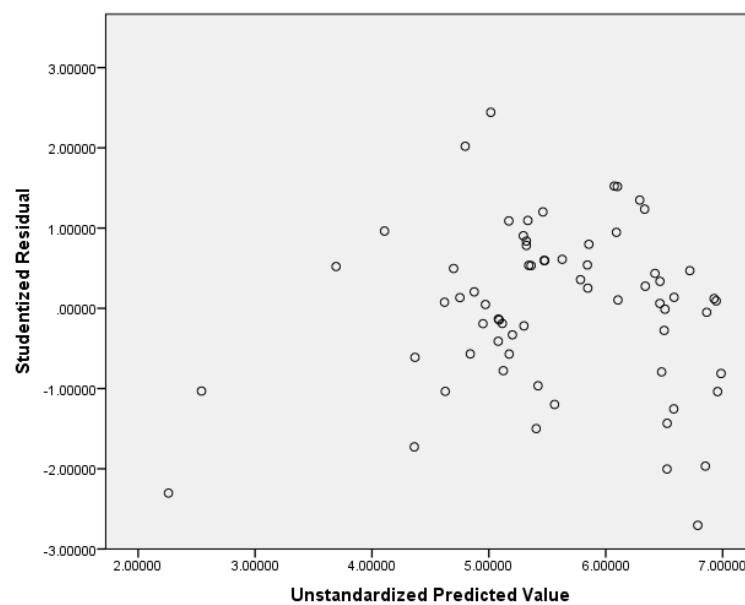
Figure 10: Studentised residuals against unstandardised predicted values (SoVC factors = IVs; PFC = DV)
