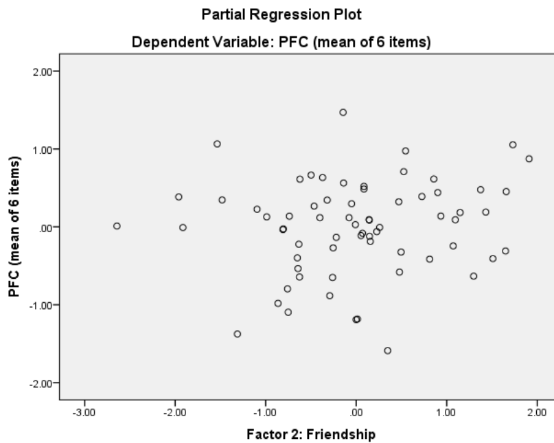
Figure 12: Partial regression plot: F2 Friendship against PFC
