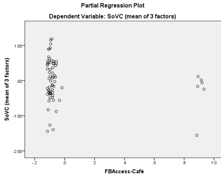
Figure 5: Partial regression plot: FB Access at Café and SoVC
