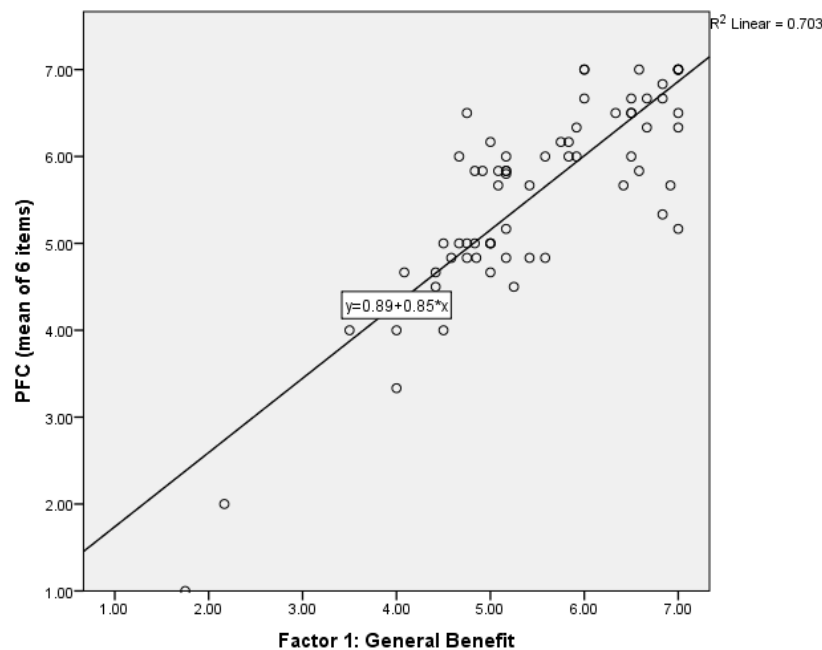
Figure 15: F1 General Benefit plotted against PFC
