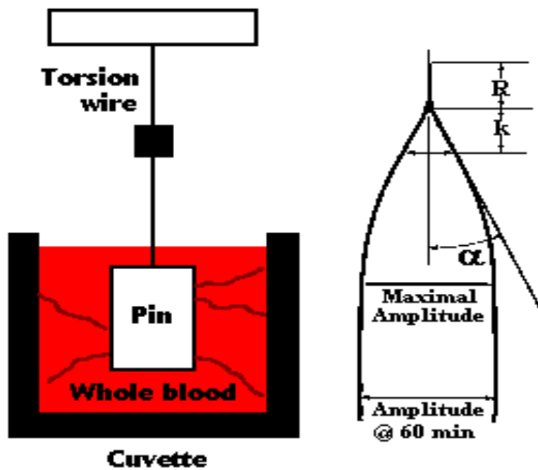
Figure 2.4: The “cup and pin” of the TEG®
