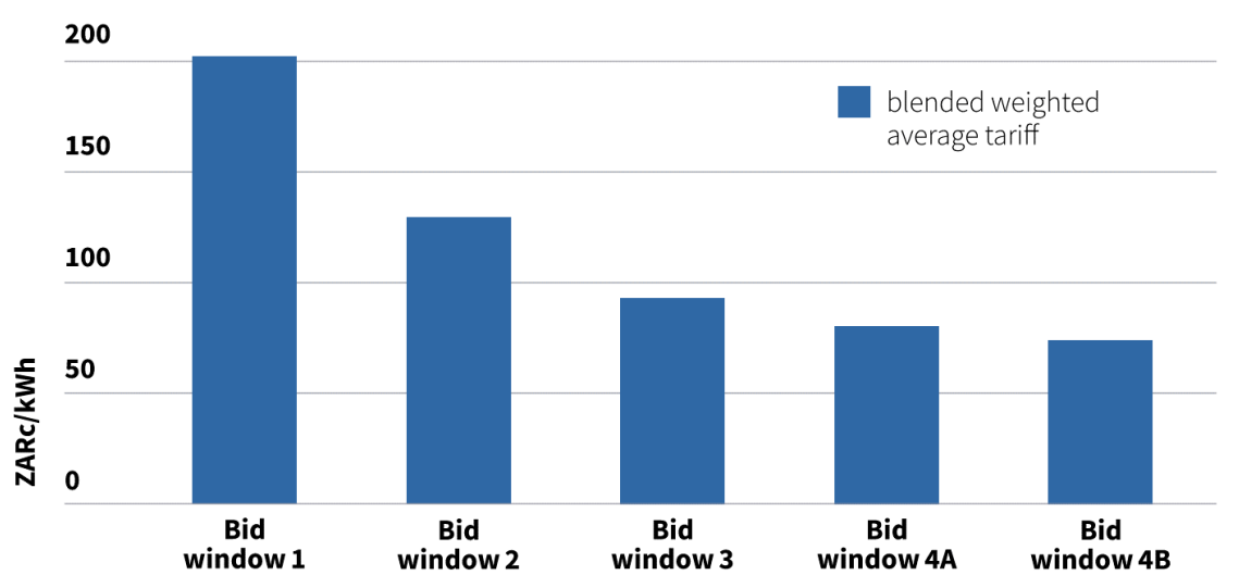
Figure 4 - Renewable energy costs in ZAR c/kWh across the first five rounds of the REIPPPP (Climate Bonds Initiative, 2021)
