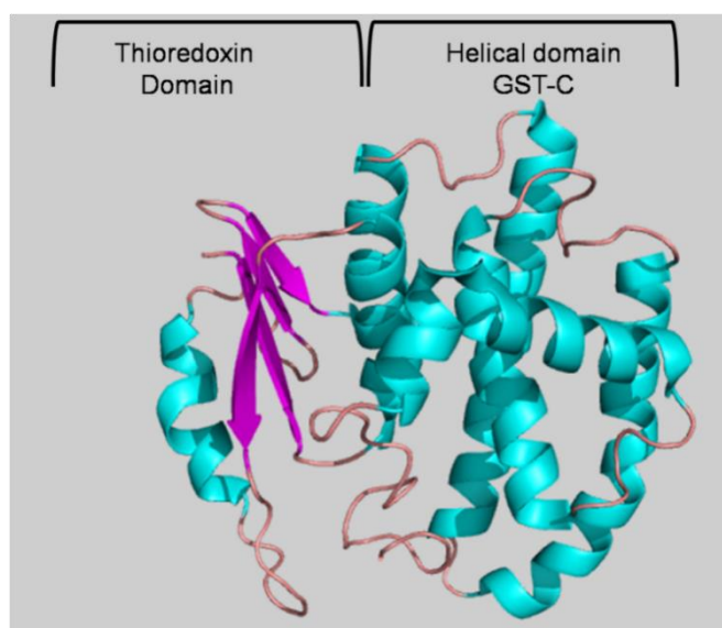
Figure 1.1: The GST-fold. A Ribbon diagram representation of hGSTM2-2 which is characterised by the GST fold. The N-terminal thioredoxin fold and C-terminal alpha helices are annotated on the image. The image was generated using PyMOL (DeLano, 2002) PDB ID: 1XW5.
