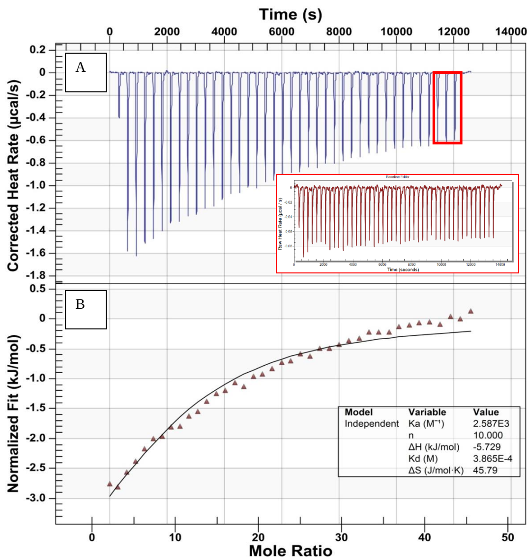
Figure 3.18: Representative calorimetric titration profile of the binding of the anionic dye ANS to EcSspA protein. The experiment was performed at 20 °C. The conditions were 0.05 mM protein and 10 mM ANS in 20 mM potassium phosphate buffer containing 1 mM EDTA at pH 6.5 (A) Exothermic heat effects associated with the injection of ANS into the ITC sample cell containing EcSspA protein. The insert panel shows the heats of dilution of ANS into buffer and is boxed in red to show corresponding heats on (A). (B) Binding isotherm corrected for heats of dilution corresponding to data in (A). The solid line through the data represents the line of best fit obtained using single independent binding site model.
