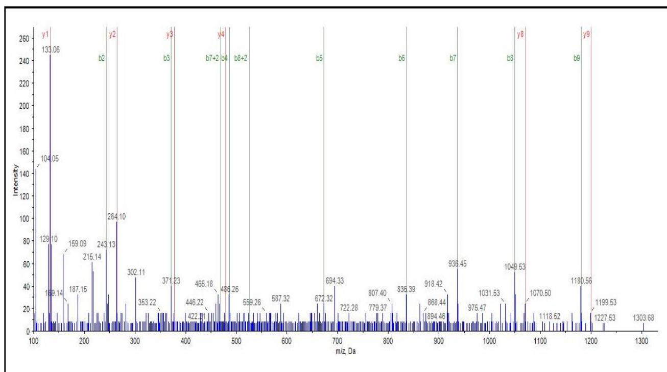
Figure 3.7: LC-MS/MS spectrum for a selected peptide match (IEKDWTLMN) derived from in-gel trypsin digest represented by a series of b and y ions. Following in gel protein digestion, peptides are separated by liquid chromatography then fragmented by Collision Induced Dissociation (CID) resulting in the above MS/MS spectrum that consists of a series of b and y ions. Fragment peaks that are generated from the amino terminus are labelled as b ions whereas peaks from the carboxyl terminus are labelled as y ions. Peptides are sequenced from both the amino and carboxyl terminus. The spectrum is analysed by ProteinPilot software against a protein sequence database for protein identification. m/z on the x axis represents the mass to charge ratio and Da is Daltons.
