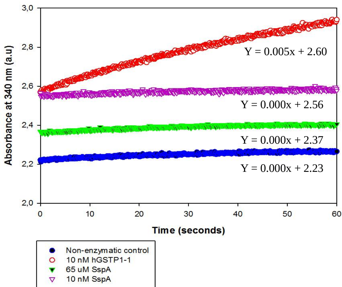
Figure 3.14: Progress curves of the CDNB/GSH catalysis. The progress curves show the enzymatic reaction carried out using hGSTP1-1 and EcSspA in 50 mM potassium phosphate, 1 mM EDTA and 0.02 % sodium azide at pH 6.5. The curve for the non-enzymatic control is included in the curves. The curves for proteins were not corrected for the non-enzymatic control. The final concentration of hGSTP1-1 used was 10 nM to obtain the linear progress curve. The final concentrations of EcSspA used were 65 \mu M protein and 10 nM diluted SspA. No enzymatic response was observed in the presence of EcSspA irrespective of the protein concentration.
