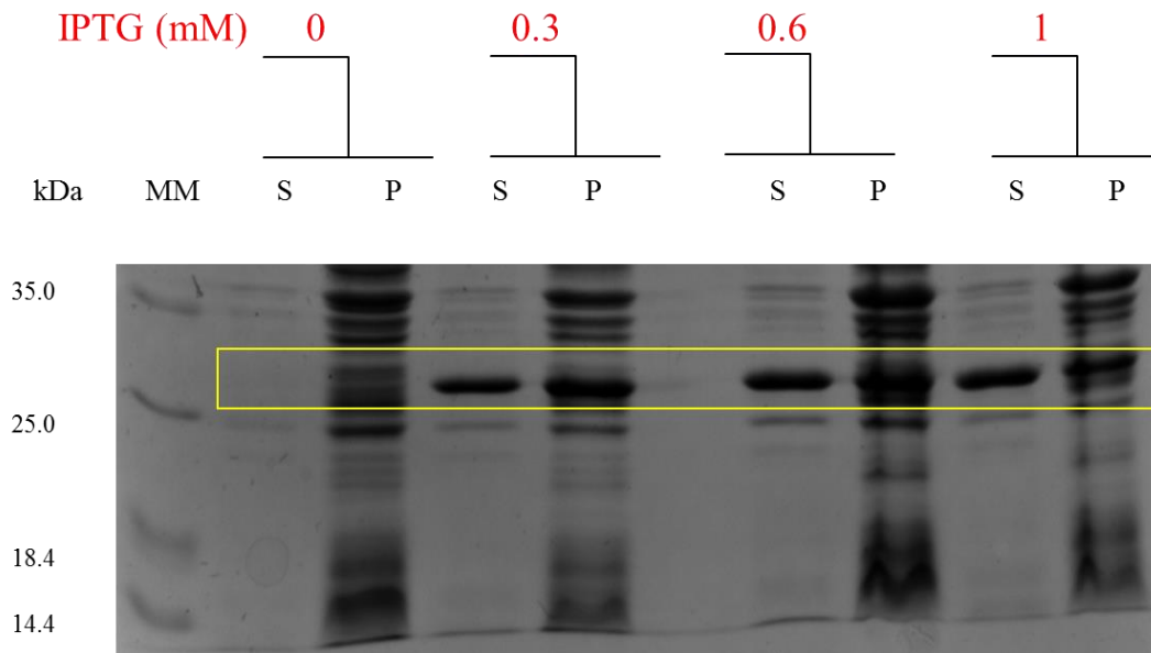
Figure 3.3: Expression trials of SspA in Escherichia coli BL21 (DE3) pLysS cells in 2x YT media at 30 °C. Expression of SspA was induced at OD_{600} = 0.6 with various concentrations of IPTG for 4 hours (A) and 6 hours (B). The protein was expressed in both the soluble supernatant (S) and the insoluble pellet (P). The protein band which corresponds to the estimated size of SspA is boxed in yellow.
