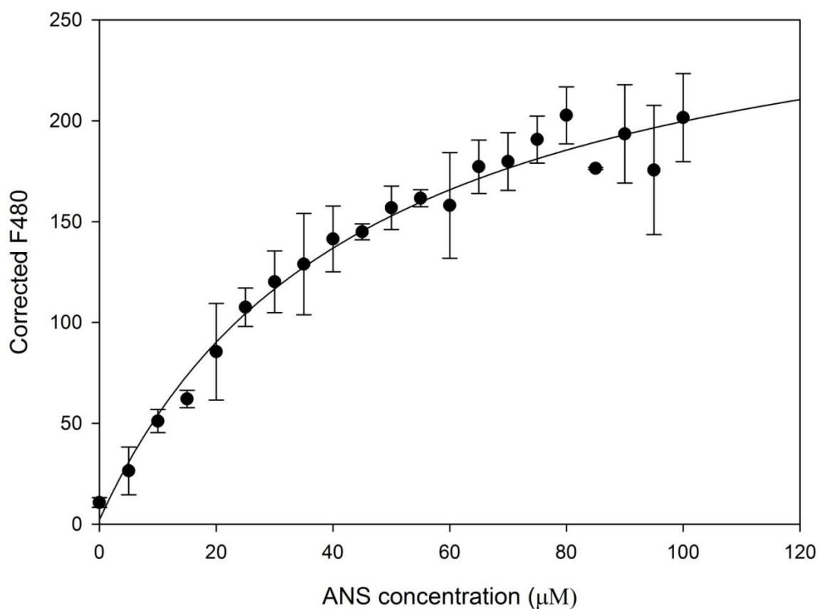
Figure 3.17: An isotherm showing the binding of ANS to EcSspA obtained using fluorescence spectroscopy at pH 6.5 at 20 °C. The extent of binding, as measured by the fluorescence intensity of bound ANS at 480 nm is plotted against increasing concentration of ANS. The dimeric protein concentration was 2 μM and the buffer solution was 20 mM potassium phosphate containing 1 mM EDTA. The solid line gives the best fit to the data for a non-cooperative model and yields a K_d value of 50 μM at an R^2 = 0.96 and was plotted using Sigma Plot software.
