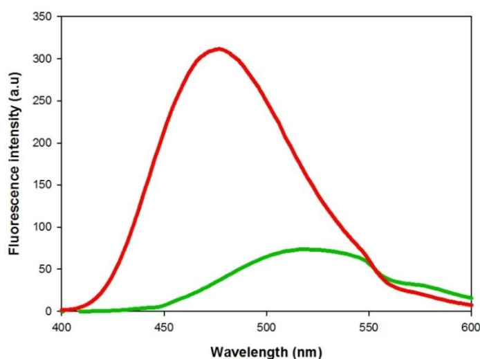
Figure 3.16: Fluorescence emission spectra of ANS bound to EcSspA. Fluorescence emission spectrum of free ANS at pH 6.5 (green) and ANS bound to EcSspA (red). The fluorescence spectrum of ANS bound to EcSspA was corrected for free ANS. The experimental data were obtained by incubating 2 \mu M SspA in 20 mM potassium phosphate pH 6.5 with ANS at a final concentration of 100 \mu M. ANS was selectively excited at 390 nm and emission spectrum determined from 400 to 600 nm. The maximum emission wavelength for free ANS and ANS bound to SspA were 520 nm and 480 nm, respectively.
