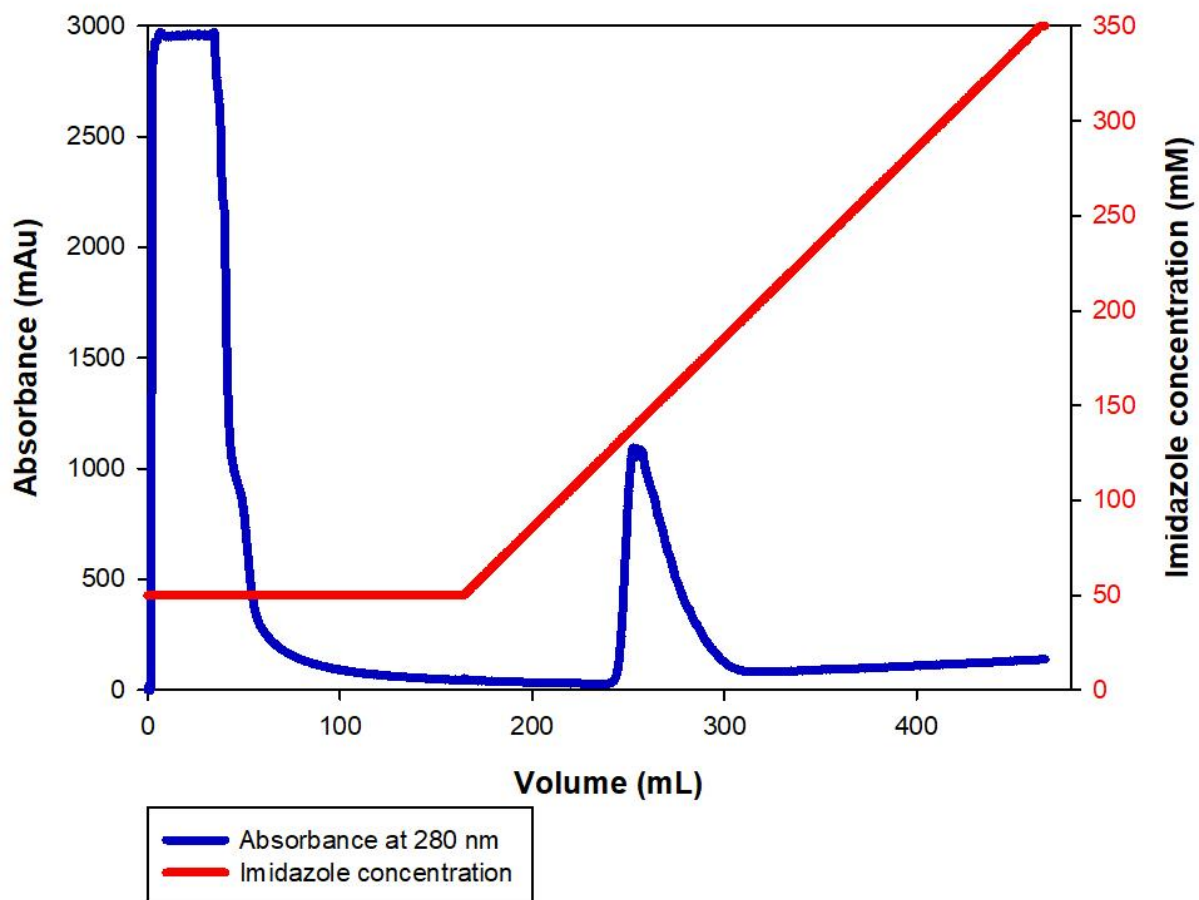
Figure 3.4: IMAC Elution profile for EcSspA purification. The elution profile of EcSspA using IMAC on the AKTA purification system. The blue profile monitors protein absorbance from supernatant loading to protein elution. The red profile monitors imidazole concentration. The protein started eluting from the column at 120 mM imidazole concentration. The insert SDS-PAGE shows the SspA purification stages. MM- molecular mass marker; L- cell lysate; S- supernatant; FT- flow through and the pure SspA protein.
