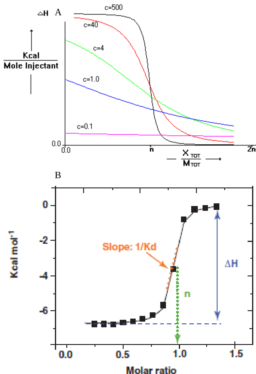
Figure 4.3: Simulated binding isotherms for various c -value parameters and extraction of the binding parameters. (A) The different coloured binding isotherms show that a higher c -value will result in a titration curve that is too steep to resolve K accurately (while N and \Delta H are well resolved). Lower c -values results in shallow titration curves from which all three parameters are poorly resolved. The image was adapted from Wiseman et al. (1989). (B) A titration profile showing raw thermodynamic data extracted from a typical ITC experiment. The data is plotted based on a suitable binding model. The change in enthalpy \Delta H , stoichiometry N , and the association constant K_a can be directly determined from the plot. The change in enthalpy is determined from the pre and post transition regions of the curve. The stoichiometry of binding is determined from the inflection point of the curve. The slope at the transition region is used to determine the association constant. This image was adapted from Nunez et al. (2002).
