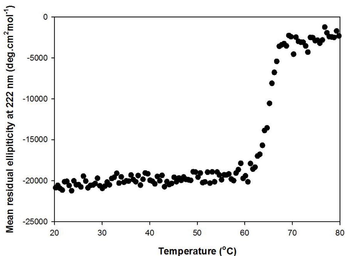
Figure 3.13: Melting curve of EcSspA using circular dichroism as a probe. Thermal unfolding of EcSspA at pH 8 was monitored using circular dichroism mean residual ellipticity at 222 nm ( MRE_{222\text{ nm}} ) as probe. The T_m for the unfolding of the secondary structure of the protein at pH 8 is 60°C. Insoluble precipitates were observed after the protein was exposed to temperatures above 60°C.
