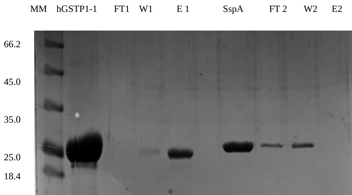
Figure 3.15: An SDS-PAGE showing the binding capability of pure EcSspA and hGSTP1-1 on a GSH-agarose column. FT= flow through W= wash solution E= Efluent. It can be seen from the gel that hGSTP1-1 binds to the column as none of the protein comes out during the flow through and wash step the protein comes out in the eluent when eluted using a 10 mM glutathione elution buffer. With EcSspA no binding of the protein to the resin was observed as most of the protein was observed in the flow through and wash step solution and nothing comes out during elution thus suggesting that EcSspA does not bind GSH.
