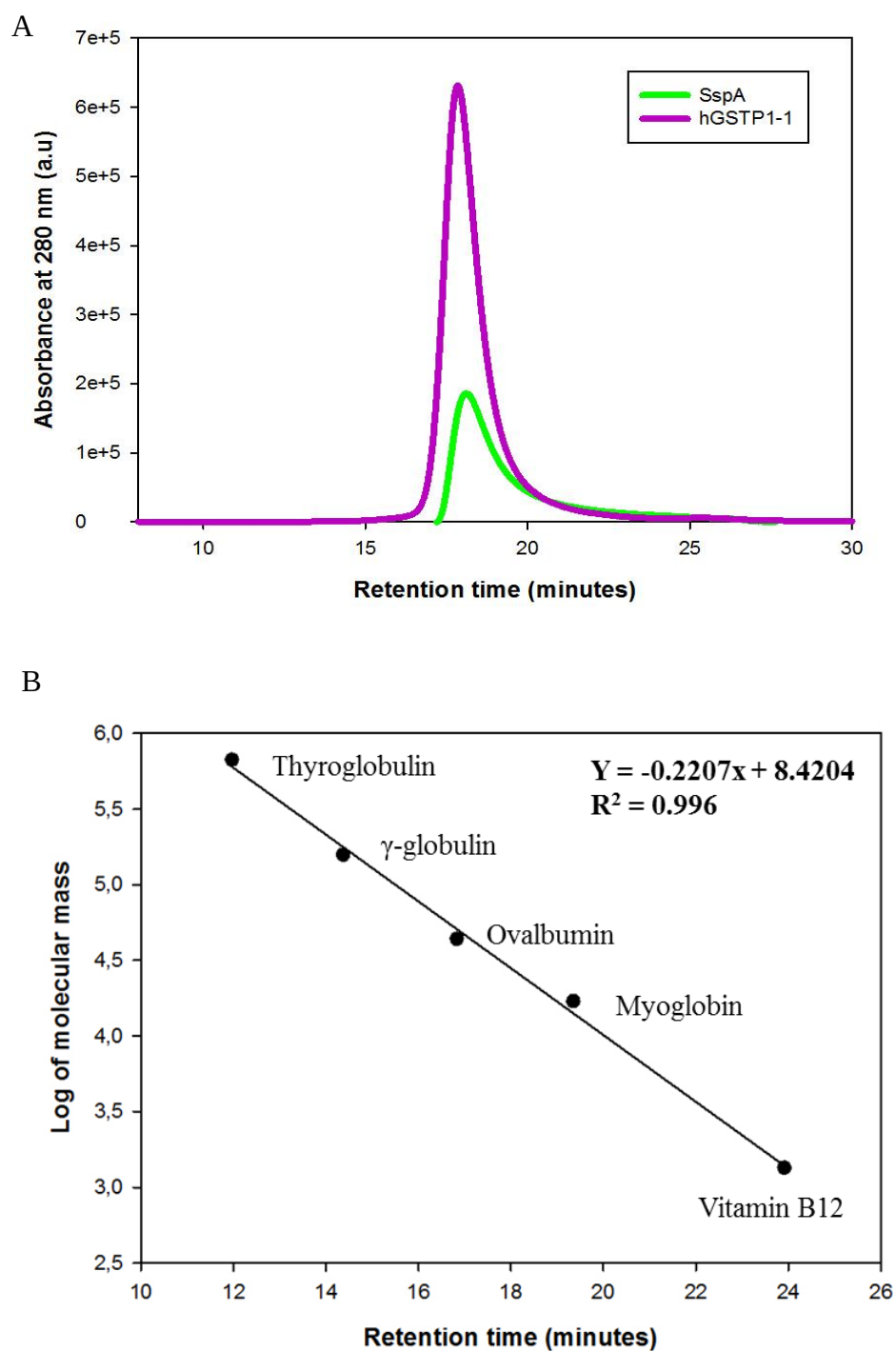
Figure 3.12: SE-HPLC elution profiles of EcSspA and hGSTP1-1. (A) The elution profiles of the proteins were recorded using absorbance at 280 nm on a Shimadzu HPLC system. The proteins were eluted in a 20 mM sodium phosphate; 500 mM NaCl at pH 7. The retention times for SspA and hGSTP1-1 were 17.46 and 17.91 minutes, respectively at a flow rate of 0.25 ml/min. (B) Calibration curve of gel filtration standards: thyroglobulin (670 kDa), γ-globulin (154 kDa), ovalbumin (44 kDa), myoglobin (17 kDa) and vitamin B 12 (1.35 kDa). The correlation coefficient is 0.996.
