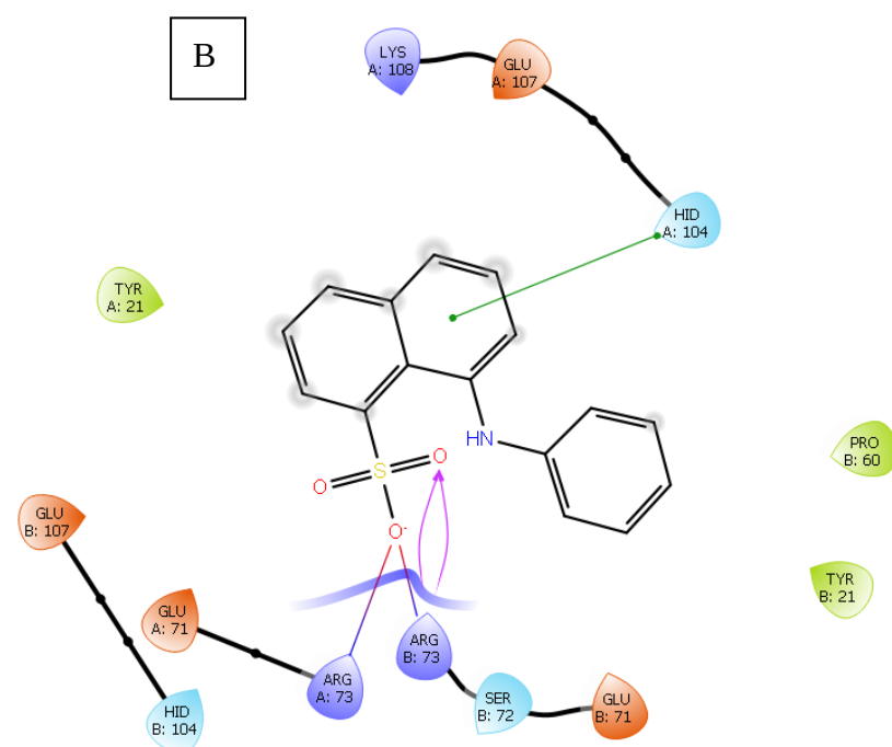
Figure 3.20: Simulated binding of ANS to EcSspA homology model. (A) Green ball and stick representation of ANS bound at the dimer interface simulated using glide docking. EcSspA binding site is represented by the molecular surface and residues found within the binding site are labelled. EcSspA-ANS interactions are shown by; pink broken lines (salt bridge), yellow broken line (H-bonds), and blue (aromatic H-bonds). (B) A 2D ligand interaction diagram with nearby residues at the binding site (dimer interface).
