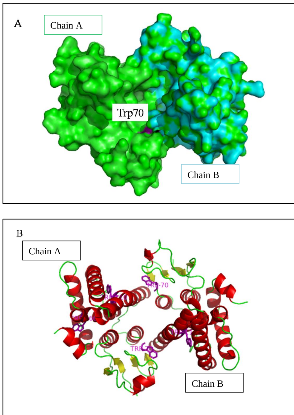
Figure 4.1: Tryptophan residue distribution in dimeric EcSspA. (A) Molecular surface of EcSspA showing the distribution of a single tryptophan residue at the surface. Of the three residues found in each subunit only a patch representing Trp70 appears on the surface of the protein. All the other residues are masked in the interior. (B) The distribution of tryptophan residues on the secondary structures of EcSspA. Red ( \alpha -helices), yellow ( \beta -structures) and yellow (loops). The tryptophan residues are mainly located on \alpha -helices. The residues are coloured purple. The images were generated using PyMOL and are in the same orientation (DeLano, 2002).
