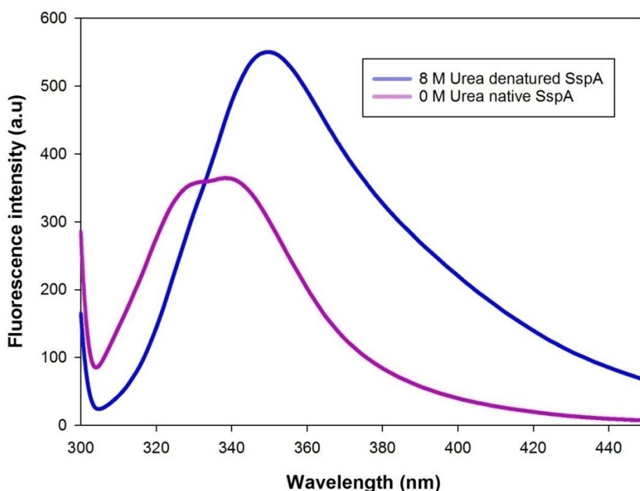
Figure 3.11: Intrinsic fluorescence emission spectrum of EcSspA. Fluorescence spectra of 0.5 \mu M EcSspA in 5 mM potassium phosphate at pH 7.4 in the native form (pink) and urea induced unfolding of EcSspA (blue) recorded at 20 °C. The spectra were corrected for a buffer blank. The natively folded EcSspA emits energy at a wavelength of 341 nm after excitation at 295 nm. The denatured EcSspA has an increased quantum yield and shows maximum emission wavelength of 350 nm.
