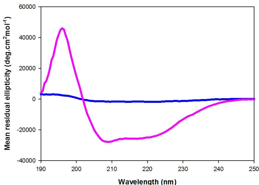
Figure 3.10: Far-UV circular dichroism spectrum of EcSspA. Circular dichroism spectrum of 2 \mu M SspA (pink) in milliQ water (blue). The spectrum shows a minimum at 208 nm and 222 nm which is characteristic of a predominantly \alpha -helical protein. The spectrum was recorded at 20 °C.
