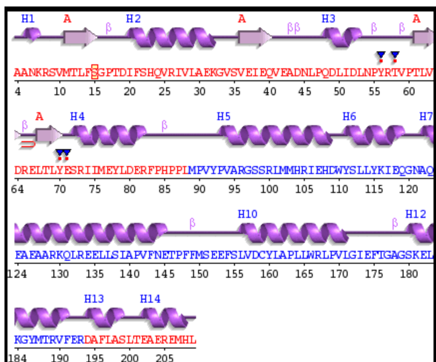
Figure 1.2: YpSspA sequence and secondary structure topology. The YpSspA sequence illustrating the proteins primary and secondary structural elements. Helices are labelled with a blue H and \beta -strands are labelled as \beta in purple. The image was adapted from PDBsum database (Laskowski et al. , 1997).
