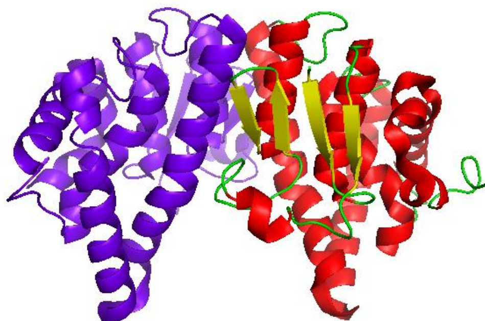
Figure 1.3: The ribbon diagram representation of dimeric YpSspA. The structure is coloured in order to show the two subunits that make up the homodimer. The subunit on the right is coloured according to the secondary structure; \beta -strands (yellow) and \alpha -helices (red). Image was generated with PyMOL (DeLano, 2002) Protein Data Bank (PDB) code: 1YY7 (Hansen et al. , 2005a).
