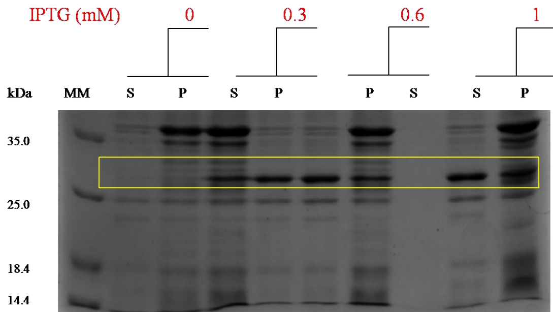
Figure 3.2: Expression trials of EcSspA in Escherichia coli BL21 (DE3) pLysS cells in 2x YT medium at 37 °C. Expression of SspA was induced at O. D 600 = 0.6 with various concentrations of IPTG for 4 hours (A) and 6 hours (B). The protein was expressed in both the soluble supernatant (S) and the insoluble pellet (P). The protein band which corresponds to the estimated size of SspA is boxed in yellow.
