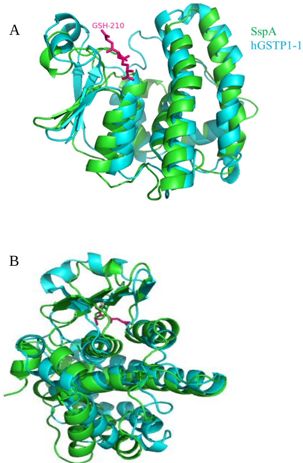
Figure 4.2: Structural comparison of EcSspA and hGSTP1-1. (A) Superimposition of an EcSspA subunit onto that of hGSTP1-1 bound to a GSH molecule (PDB ID: 6GSS). (B) Superimposition of the same molecules in a different orientation. The subunits superimpose with a rmsd of 4.71 Å for 161 corresponding Ca atoms. The proteins are illustrated as ribbon diagrams (helices as spirals, \beta -strands as arrows and loops as pipes). The pink molecule is GSH. The images were generated using PyMOL (DeLano, 2002).
