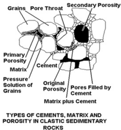
Figure 25 Illustration of porosity in clastic rocks (Steve Cannon Geosciences Ltd)
