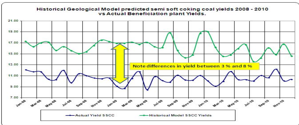
Figure 73 Historical geological model planned SSCC yields and actual beneficiation plant SSCC yields.
