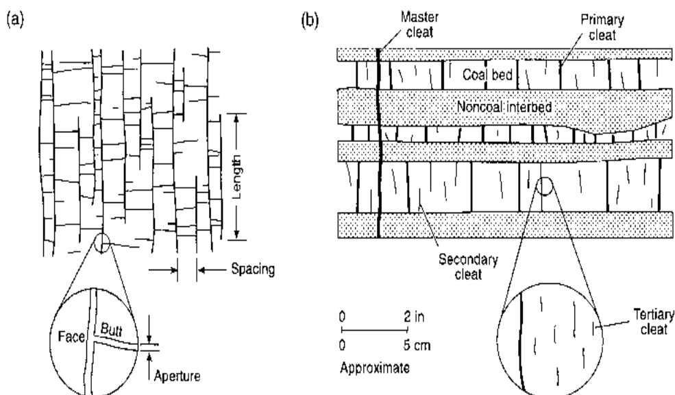
Figure 29 A Schematic depicting cleat formations in coal. ( Laubach et al, 1998).
