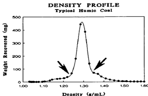
Figure 14 Typical Vitrinite peak. (Crelling, 1994)
