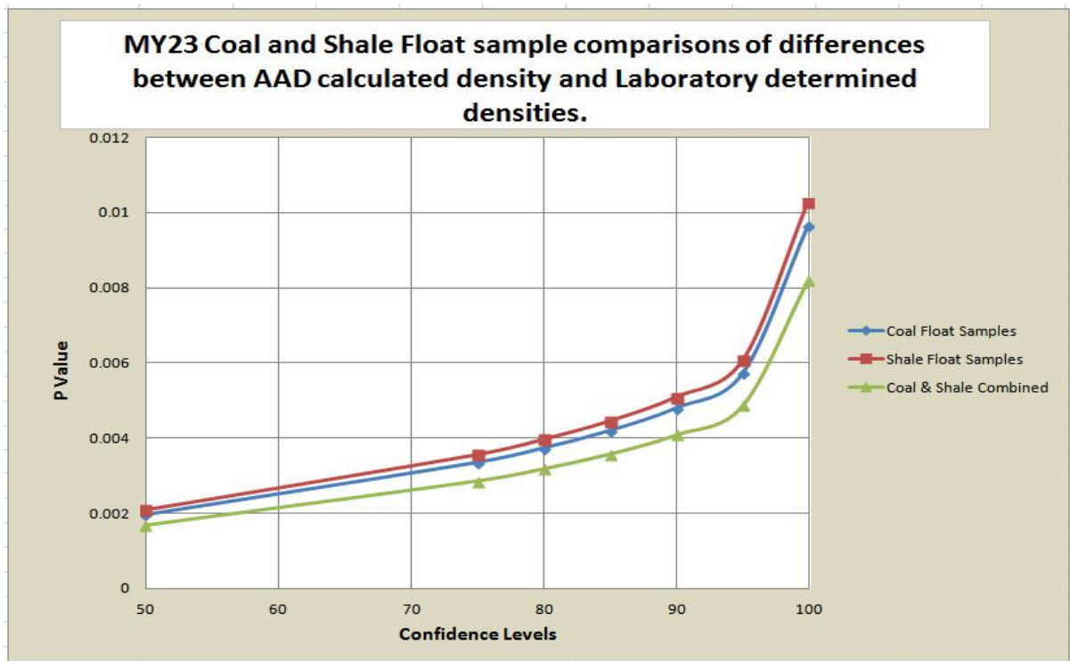
Figure 46 Plot of P values obtained at statistical confidence levels ranging from 50% to 99.9%
