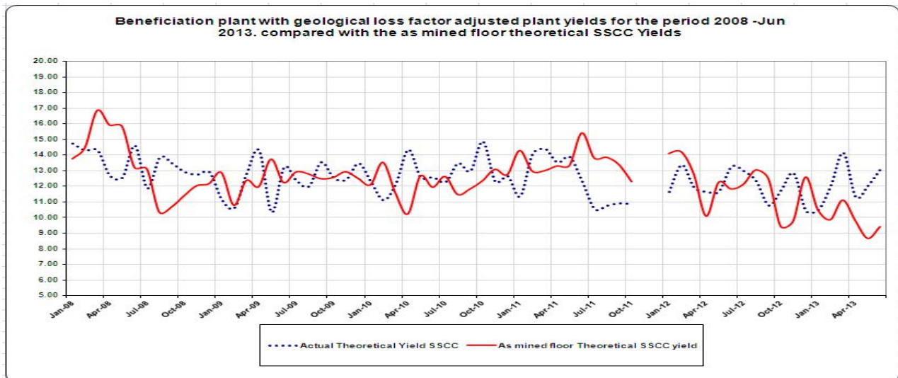
Figure 79 The 17.82% loss factor adjusted plant yields compared with as mined floor AAD theoretical yields.
