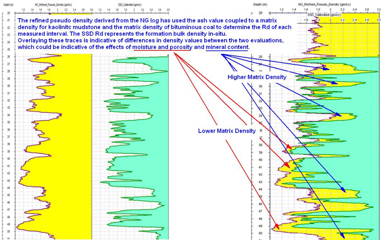
Figure 88 Overlay comparison of NG pseudo density on SSD apparent bulk density. The NG trace, far left, apparent bulk density next and the last column representing the overlay of the apparent density on the inferred matrix density.
