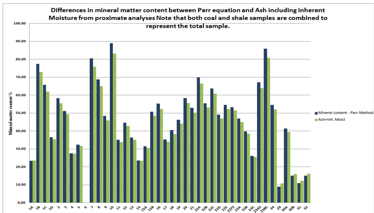
Figure 59 Mineral matter determined by Parr method compared with mineral matter from inherent moisture corrected residual ash.
