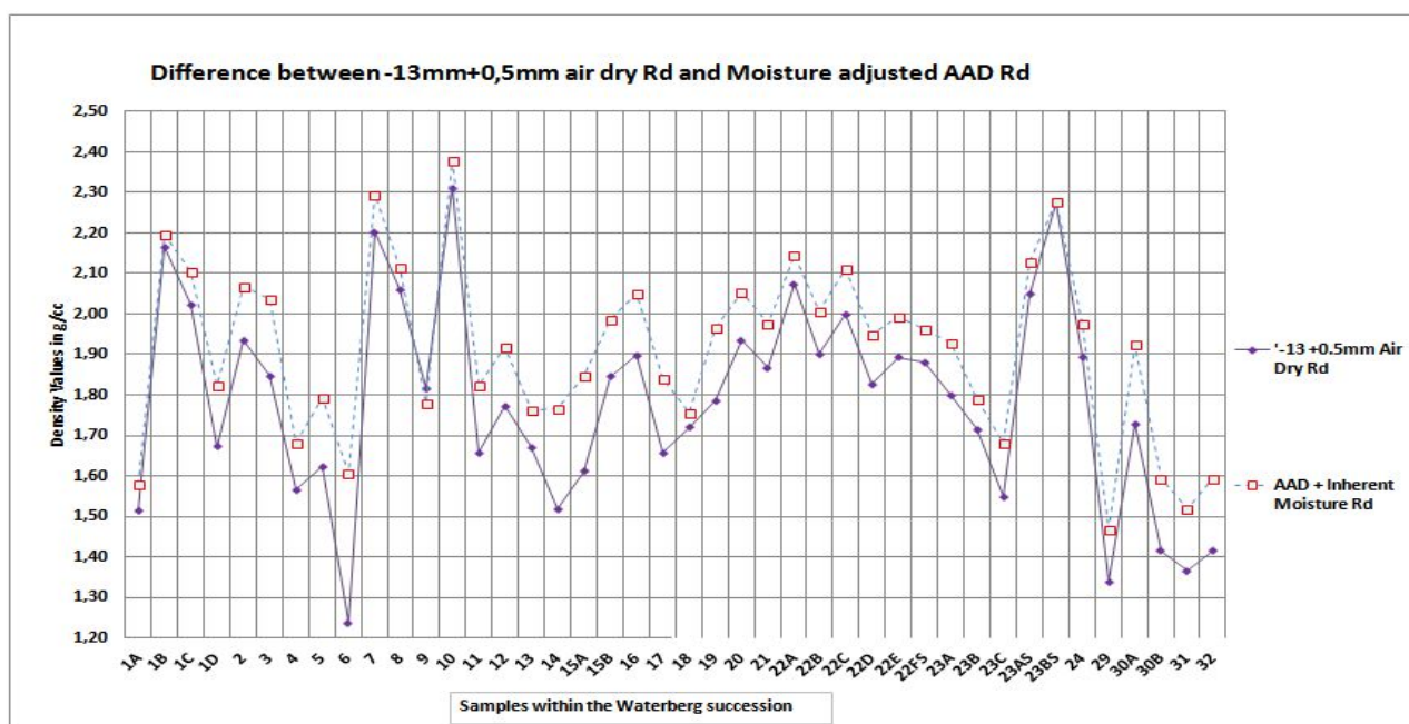
Figure 56 A sequential plot of the moisture corrected AAD density for the absolute density of the solid matrix and the air dried density determined from the -13mm + 0.5mm material.
