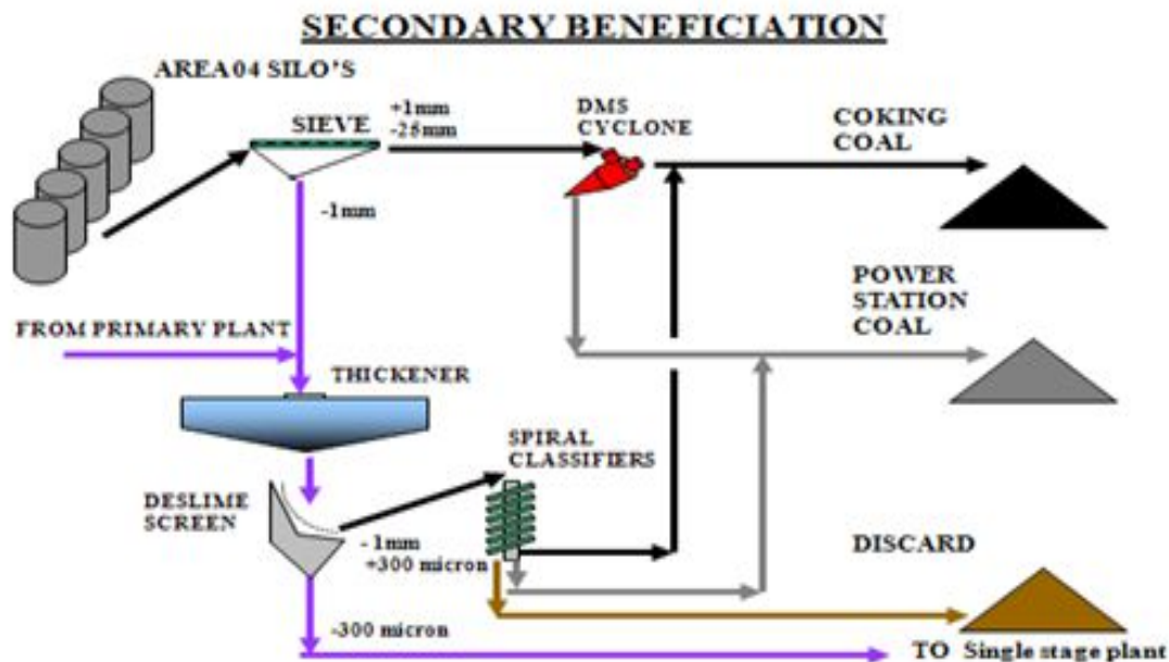
Figure 66 Schematic of double stage beneficiation process.
