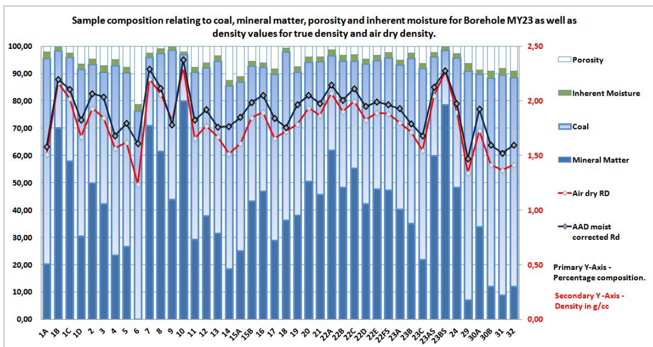
Figure 57 sequential plots of the individual sample's composition with regard to coal, indestructible mineral matter (represented by residual ash), porosity and inherent moisture within the Waterberg Coalfield succession as well as the selected densities for total true density and air dry density.
