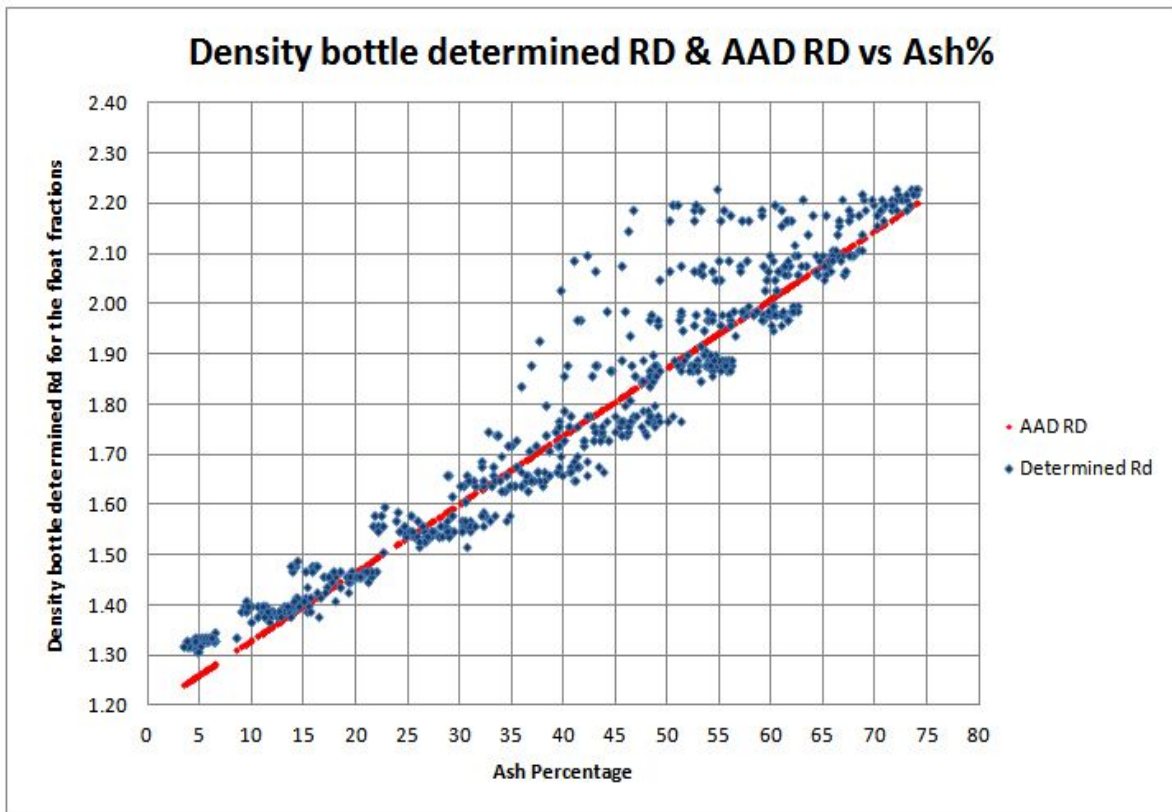
Figure 44 Plot of re-determined relative densities using the Australian Standard method, "AS1038.21 Item 4 combined with the AAD relative densities against the ash percentages from proximate analyses of the individual float fractions.
