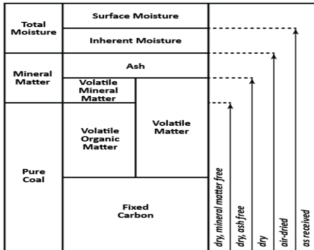
Figure 24 Relationship between the various constituents of coal and reporting bases (Ward, 1984)
