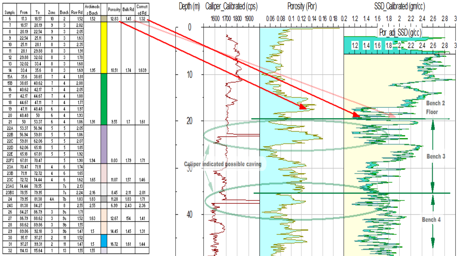
Figure 92 is the expanded section of GK86, showing on the left a table of information relative to sample depths, zone classification, representative bench, the raw RD per sample, composited RD per bench, inferred porosity SSD log bulk density and the corrected RD based on the inferred porosity. The log traces shown are caliper, inferred porosity and a combination of the inferred matrix density the porosity corrected density overlain. Cross-overs where the corrected density is lower than the bulk density are shaded in blue.
