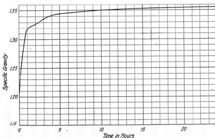
Figure 19 Graphical representation of increase in specific gravity over 24 hours time that coal sample is submerged in water at room temperature. (Nebal, 1916)
