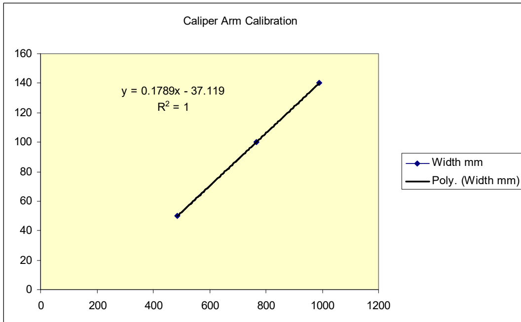
Figure 37 Caliper arm calibration data and curve with coefficients.
