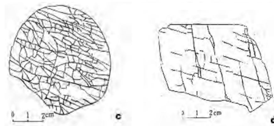
Figure 34 Sketch c reflective of a high density cleat system in various directions and sketch d, low density parallel cleats. (Fan, 1997)
