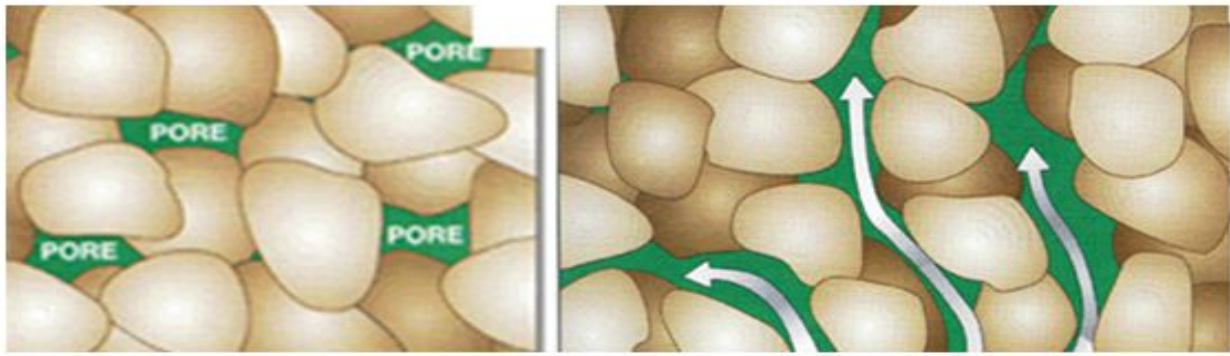
Figure 22 Illustrated basic concepts and density variations as a result of rock porosity.(MPG, Petroleum Inc.)
