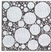
Poorly Sorted Low Porosity
