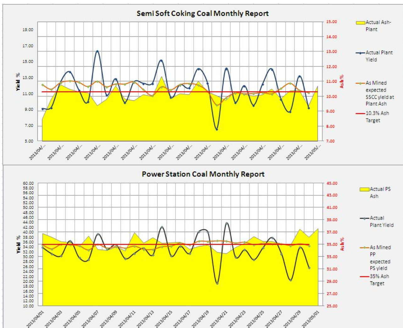
Figure 84 Combined plots of monthly SSCC and PS coal production compared with plant ash content.
