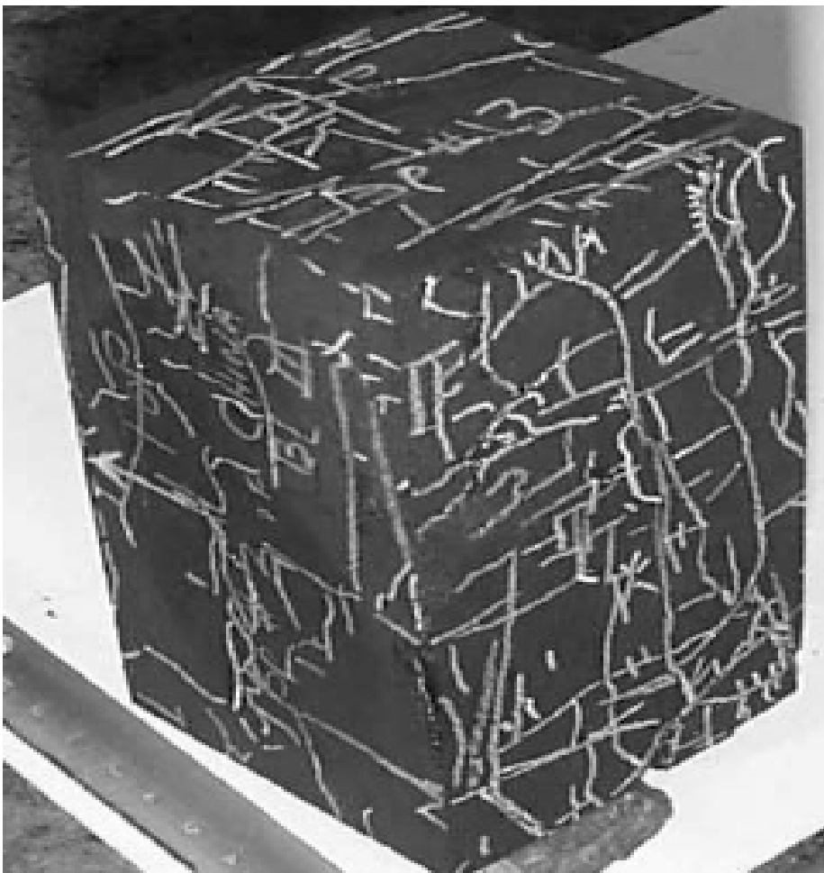
Figure 35 Photograph of a 40mm coal cube displaying the major cleats in filled with silicone to contrast against the coal background and also to strengthen and retain the coal sample intact. (Massorotto, 2003)
