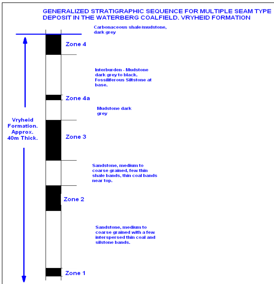
Figure 5 Cyclic Sedimentary Subdivision of Coal sequence for the Vryheid Formation
