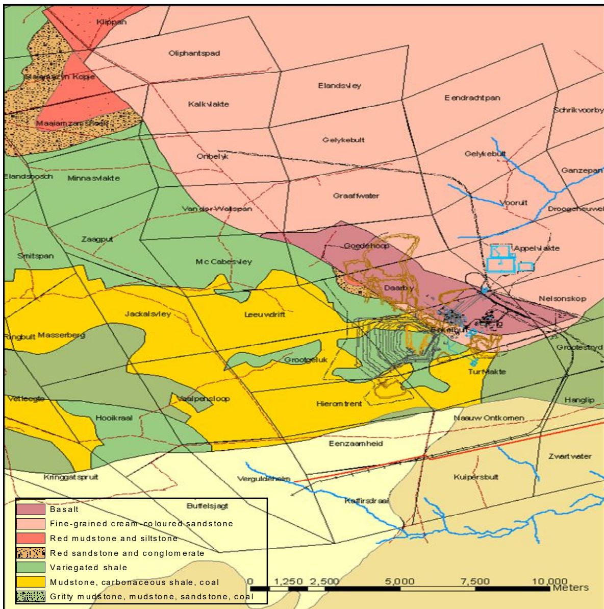
Figure 3 Regional Geological Map with Grootegeluk locale overlain.
