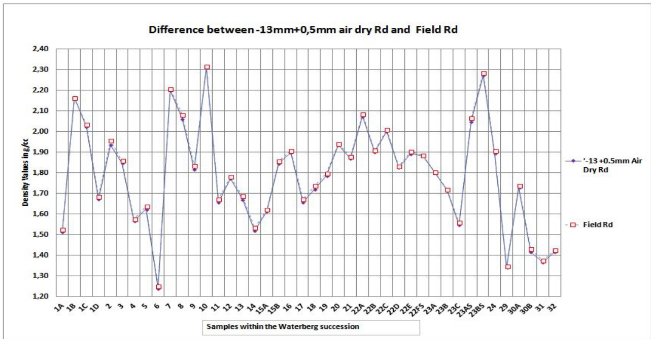
Figure 55 A sequential plot of the -13mm +0.5mm air dry determined density against the field determined density. Note that the values plotted correlate perfectly therefore the plots overlap.
