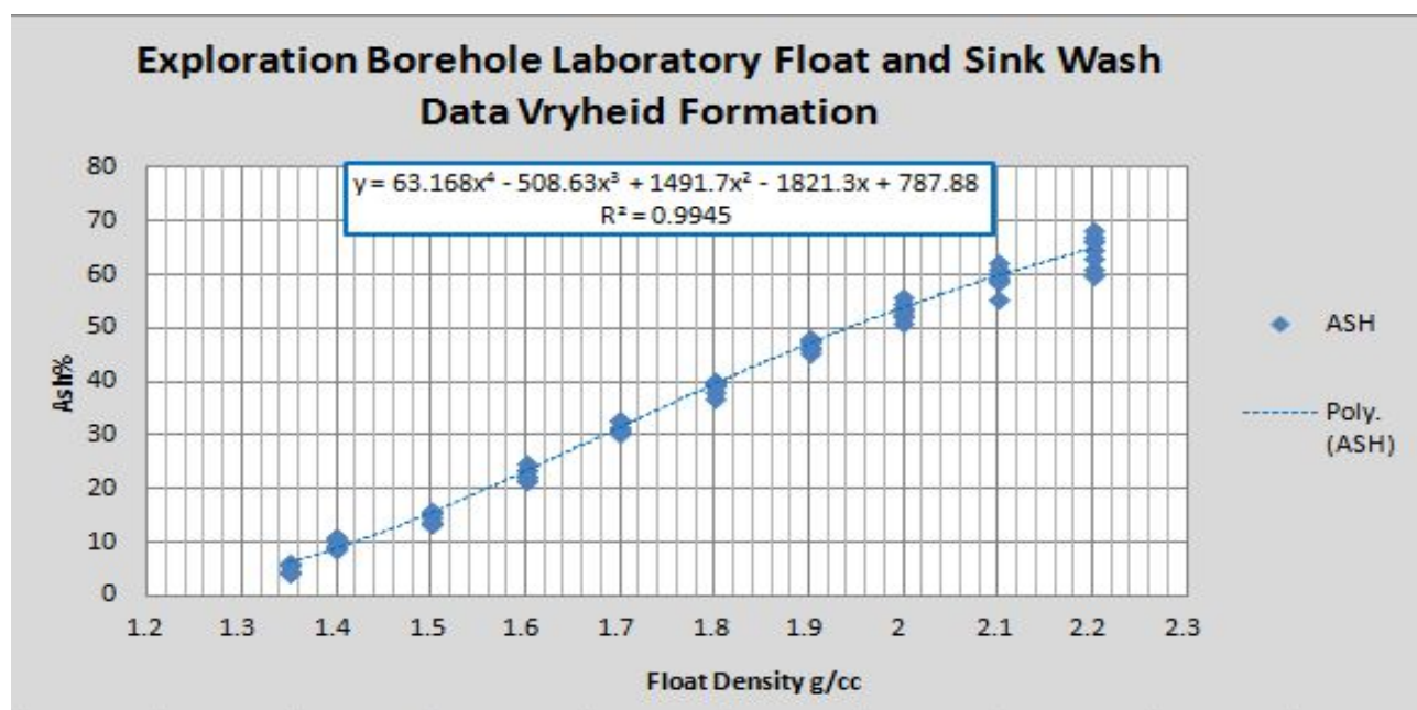
Figure 42 Vryheid Formation coal sample wash data as primarily obtained at fixed density cut points.
