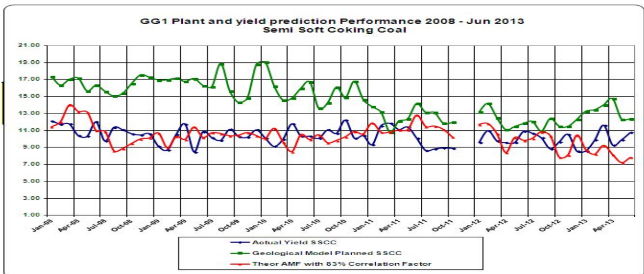
Figure 75 Geological model planned yields against actual plant production and the as mined ash adjusted density yields with an 83% correlation factor applied.
