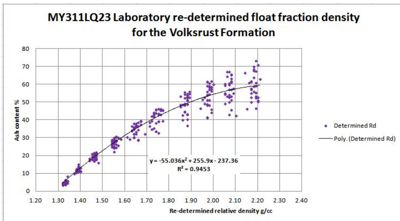
Figure 41 Re-determined relative density values for the respective float fractions of the same borehole in the Volksrust Formation.
