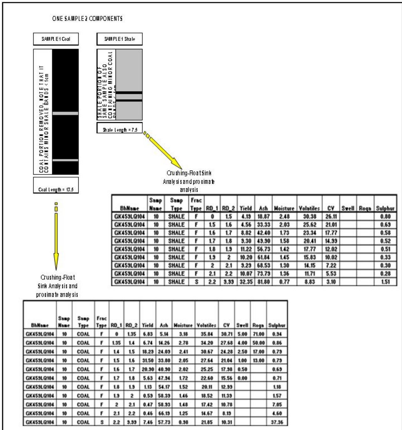
Figure 12 Grootegeluk wash table configuration.
