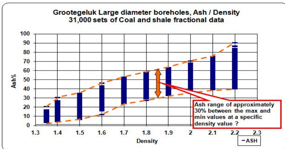
Figure 1 Illustration of the range of ash determinations around a specific density fraction
