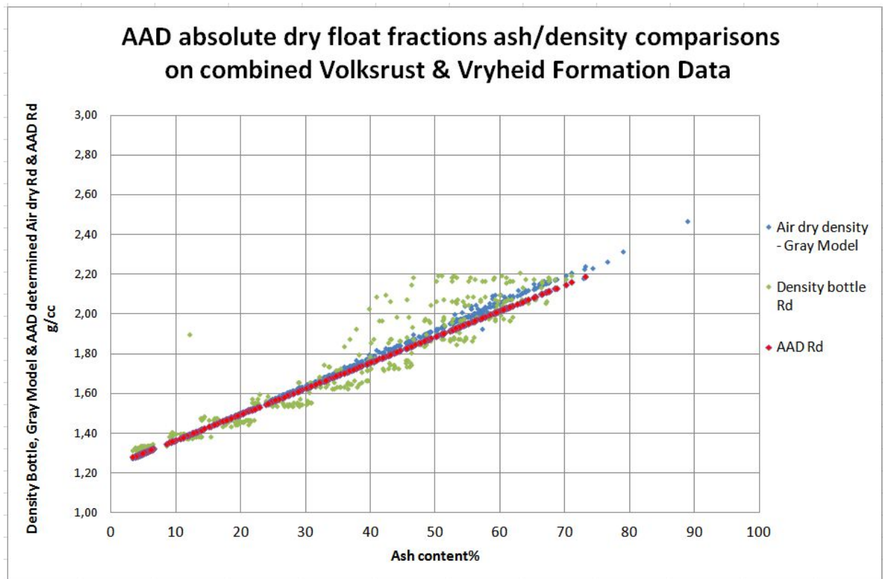
Figure 51 Plot of absolute dry density obtained from AAD against the Gray model and density bottle determined densities.
