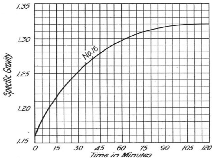
Figure 20 Graph of coal samples showing the change in specific gravity of coal samples immersed in water at room temperature. . (Nebal, 1916)
