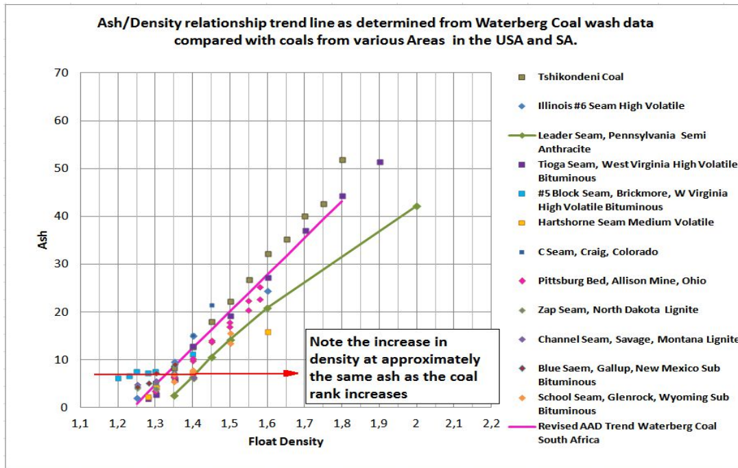
Figure 6 Comparison of Northern hemisphere coals, their rank and South African coals
