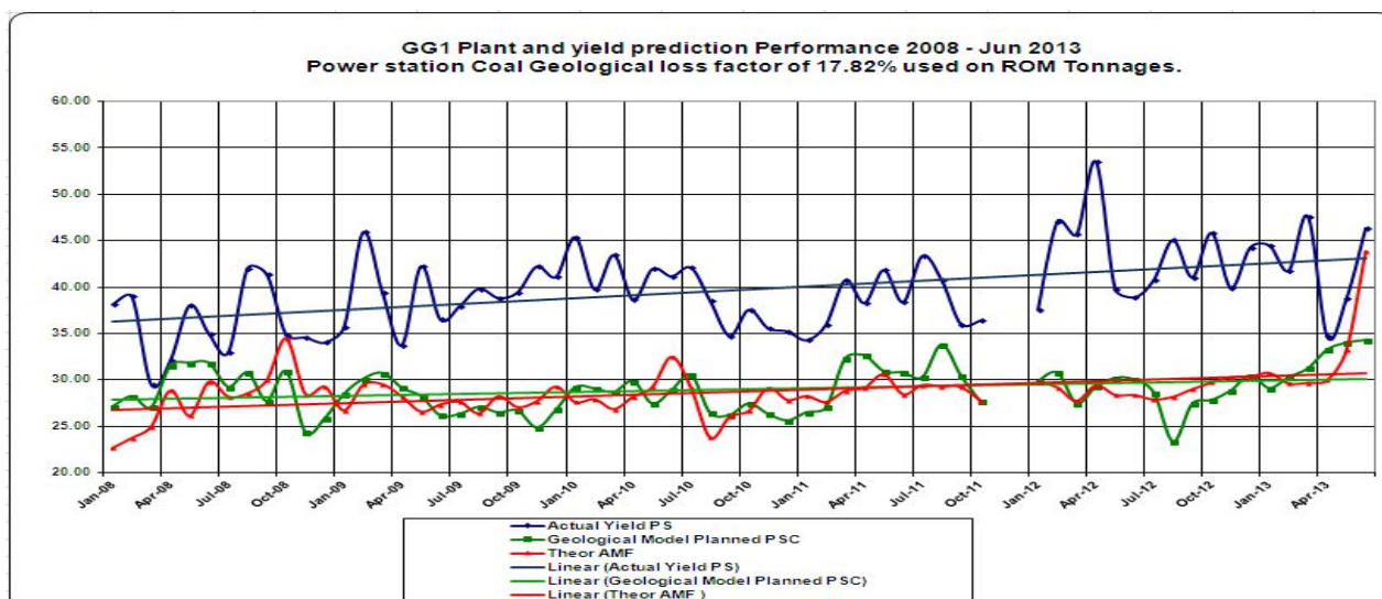
Figure 80 Theoretical, as mined and actual power station coal yield based on adjusted ROM tonnages.
