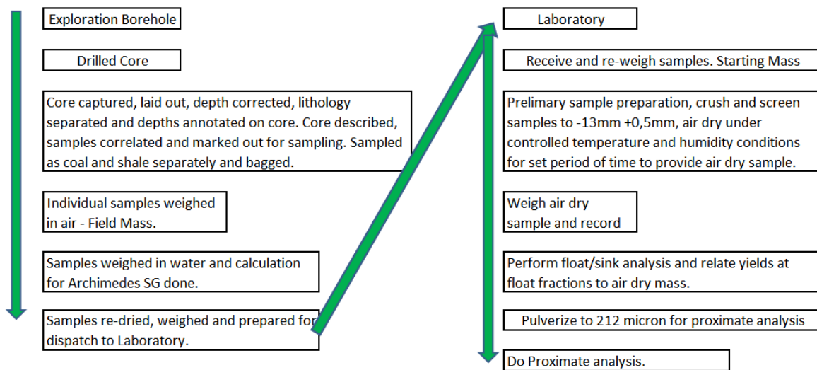
Figure 13 Flowchart of processes and data available from an exploration borehole through the laboratory and back to the original site.
