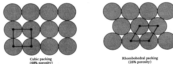
Cubic packing 47% porosity (left) Rhombic packing 26% porosity (right)
