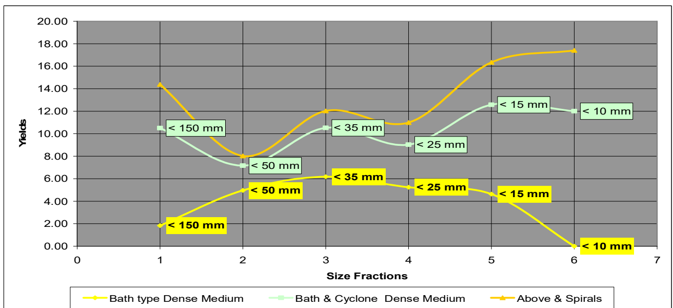
Figure 67 Schematic reflecting the results of the six subdivided samples at their various top sizes and the beneficiation mediums used for separation.
