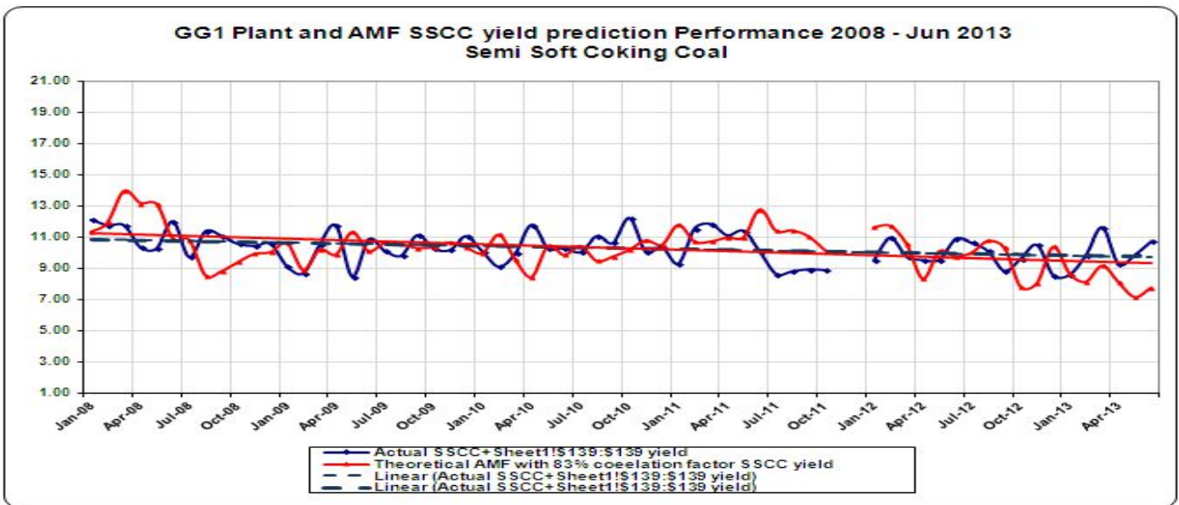
Figure 72 Plot of actual SSCC yield against as mined AAD yield over the entire monitoring period. If however the entire monitoring period (2008 – 2013) is taken into consideration the correlation between the actual beneficiation plant semi soft coking coal yields and the as mined values with an 83% correlation factor adjustment applied to the semi soft coking coal yields, is 98% , an excellent correlation.
