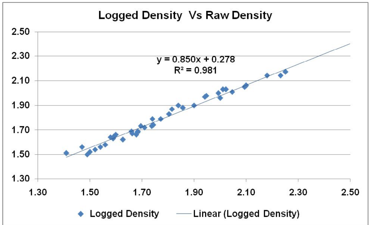
Figure 38 Reverse compatibility density values from geophysical logs compared with laboratory raw density
