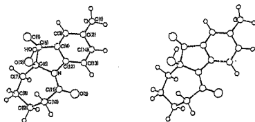
Fig.4. Molecular Structure of OR43.
