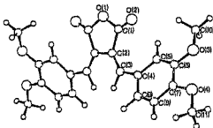
Figure A. Atomic numbering scheme.
