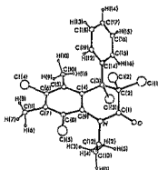
Fig.10. The crystal structure of OR12.
