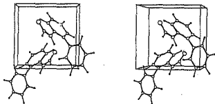
Fig.24. Packing diagram for OR15.
