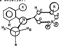
Fig.25. Lowest energy conformation for 57a in solution.
