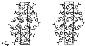
Fig.7. Stereoscopic packing diagram of OR03 showing the hydrogen bonds between the oxygen atoms. Hydrogen atoms have been omitted for clarity.
