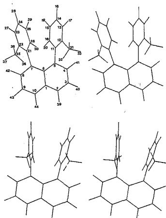
Fig.33. Stereoscopic drawings of the cis and trans forms of 1,8-di-tolynaphthalene as obtained by molecular mechanics.
