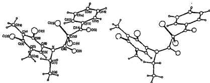
Fig.27. Molecular structure of OR22.
