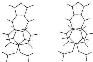
Fig.57. Calculated structure of rotamer (180,180).
