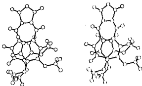
Fig.46. Calculated structure for compound 133.
