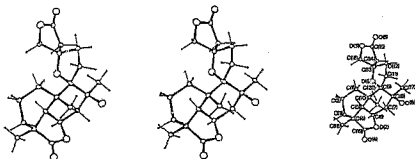
Fig.16. Molecular structure of OR42.
