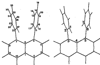
Fig.20. Stereoscopic drawing of the minimum energy arrangement of 1,8-ditolynaphthalene obtained by molecular mechanics.
