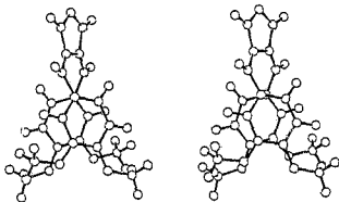
Fig.48. Calculated structure of compound 132.
