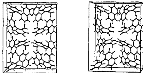
Fig.35. Packing diagram for OR44.
