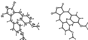
Fig.51. Molecular Structure of OR38.
