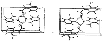
Fig.21. Packing diagram for OR10.
