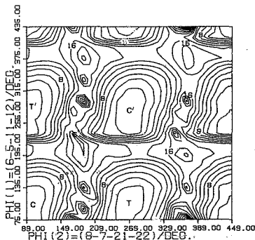
Fig.31. Two dimensional contour map of the conformational energy of 1,8-di(meta-methylphenyl)naphthalene as a function of the rotation of the two phenyl rings. Contour intervals are 2 kcal/mol.
