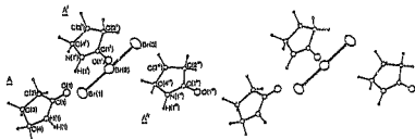
Fig.12. The asymmetric unit of OR05.
