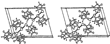
Stereoscopic view of the tribromide ion-containing channel in the [011] direction Fig. 13 of the SDI-9311, containing channel in the [011] direction of the unit cell.
