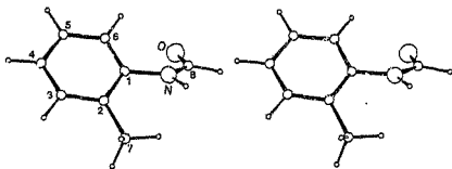
Fig.20. Molecular structure and numbering scheme of OR10.
