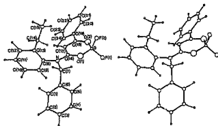
Fig.28. Molecular structure of OR01.
