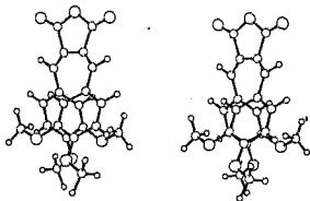
Fig.40. Molecular structure of OR02.
