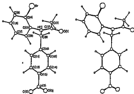
Fig.26. Molecular structure of OR04.
