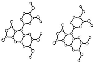
Fig.42. Molecular structure of OR08.
