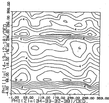
Fig.54. Steric energy surface for E,E-bis(p-methoxy)fulgide. Contour interval is 1 kcal/mol.
