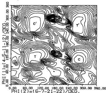
Fig.32. Conformational energy of 1,8-di-tolyl-naphthalene as a function of two phenyl ring rotations. Contours are drawn at 2 kcal/mol.
