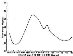
Fig.45. Steric energy of 133 as a function of one aryl ring rotation.
