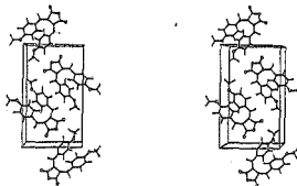
Fig.53. Packing diagram for OR38.
