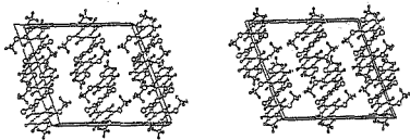
Fig.49. Packing diagram for OR02.
