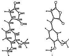
Fig.38. Molecular structure of OR34.
