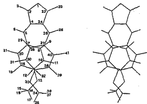
Fig.55. Calculated structure of rotamer (0,0).
