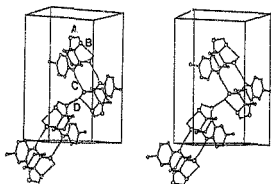
Fig.3. Packing diagram for OR24.
