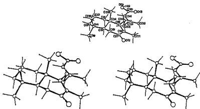
Fig.17. Molecular structure of OR26.
