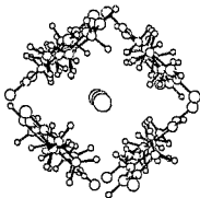
Fig.14. Cross-section of a channel in the lattice of OR05.
