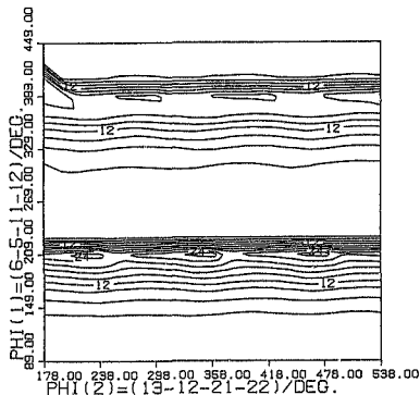
Fig.36. Conformational energy map for 1-tolynaphthalene as calculated by molecular mechanics.
