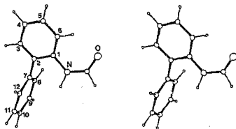
Fig.23. Molecular structure of OR15 showing the numbering scheme used.
