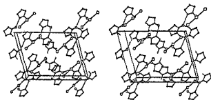
Fig.15. Stereoscopic packing diagram of OR05 showing the four different hydrogen bonding interactions. C-H bonds have been omitted for clarity.
