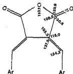
Fig.44. Some bond angles for OR02.
