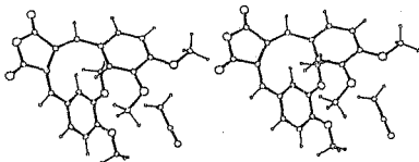
Fig.43. Molecular structure of OR41.
