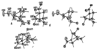
Fig. 6. The asymmetric unit of OR03. Thermal ellipsoids are at 50% probability.
