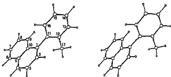
Fig.34. The molecular structure of OR44.
