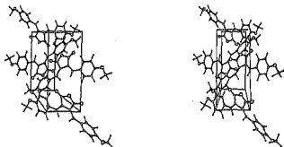
Fig.52. Packing diagram for OR37.
