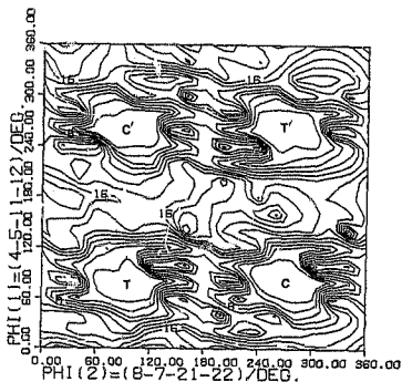
Fig. 29. Two dimensional contour map of the conformational energy of 1,8-diphenylnaphthalene as a function of the rotation of the two phenyl rings. Contour intervals are 2 kcal/mol.
