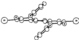
Fig.37. View of 130 along the twofold symmetry axes.
