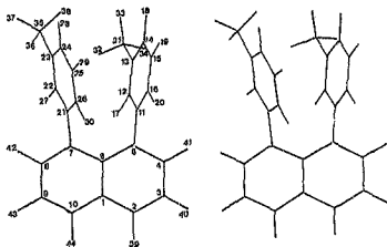
Fig. 30. Stereoscopic drawing of the minimum energy arrangement of 1,8-di(meta-methylphenyl)naphthalene obtained by molecular mechanics.
