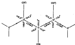
Fig. 8. Schematic diagram showing the hydrogen bonds in OR03.
