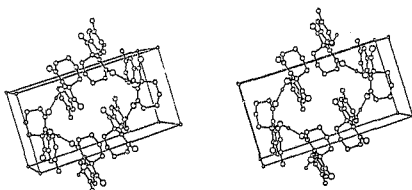
Fig.5. Packing diagram of OR43. All hydrogen atoms (except hydroxyl proton) have been omitted for clarity).
