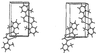
Fig.19. Packing diagram for OR09.
