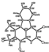
Fig.9. The crystal structure of OR07.
