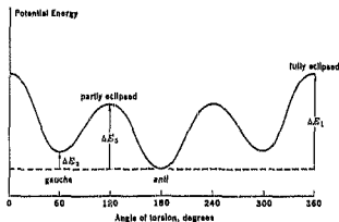
Fig.1. Potential energy curve for 1,2-dichloroethane.
