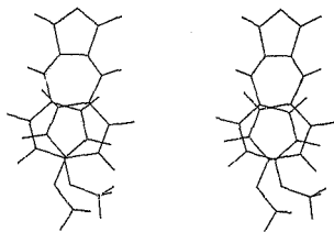
Fig.56. Calculated structure of rotamer (180,0).
