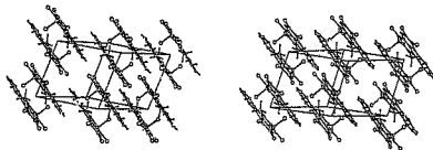
Fig.11. Packing diagram for OR07.
