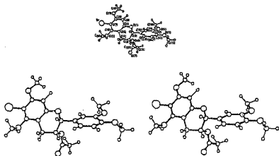
Fig.39. Molecular structure of OR11.
