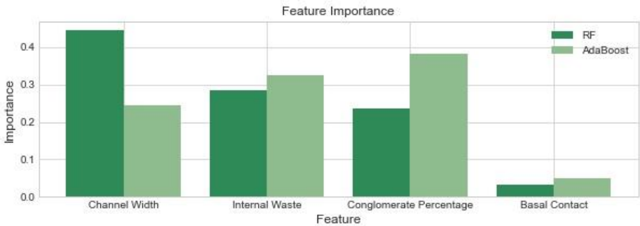
Figure 4.13: Graphical illustrations of the RF and AdaBoost algorithms' feature importance statistics for the full subset.
