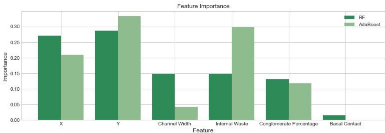
Figure 4.14: Graphical illustrations of the RF and AdaBoost algorithms' feature importance statistics for the full subset (including spatial features).
