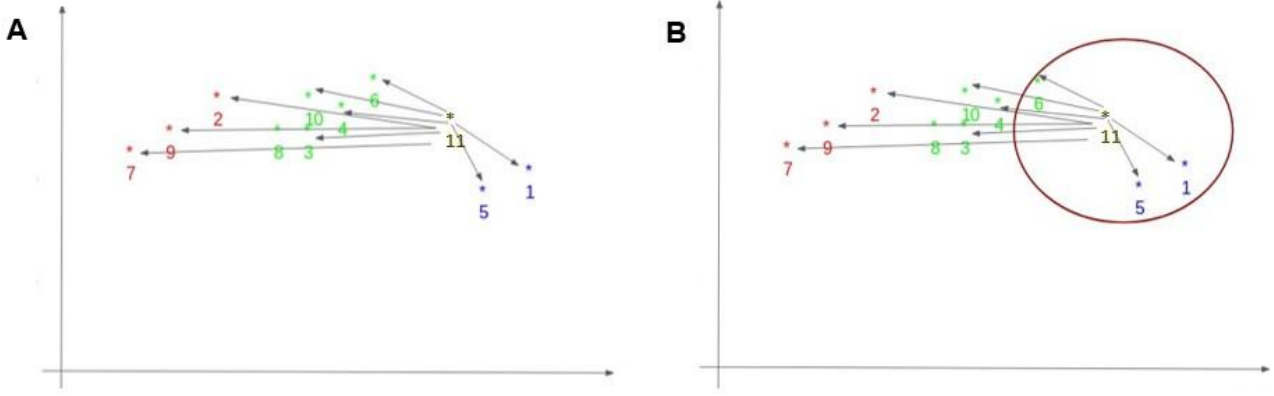
Figure 3.3: Simplified sketch illustrating the KNN algorithm's process. The training data's values are represented by red, green and blue, while black represents a value from the testing set. The coordinates are arbitrary feature dimensions. In subfigure A, the distance between the training and testing datapoints is computed. In subfigure B, we assume that k = 3 , for example; in this case, 5, 1 and 6 will be selected as our point's nearest neighbours based on their proximity (adapted from Kramer, 2013).
