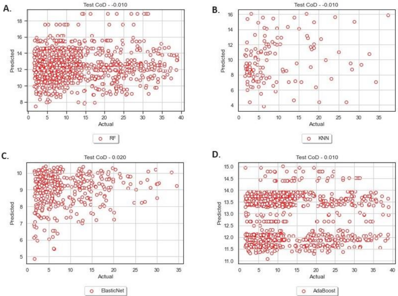
Figure 4.23: Graphical illustrations of the 'bad' dataset's second round of testing, visualising each algorithm's CoD scores.
