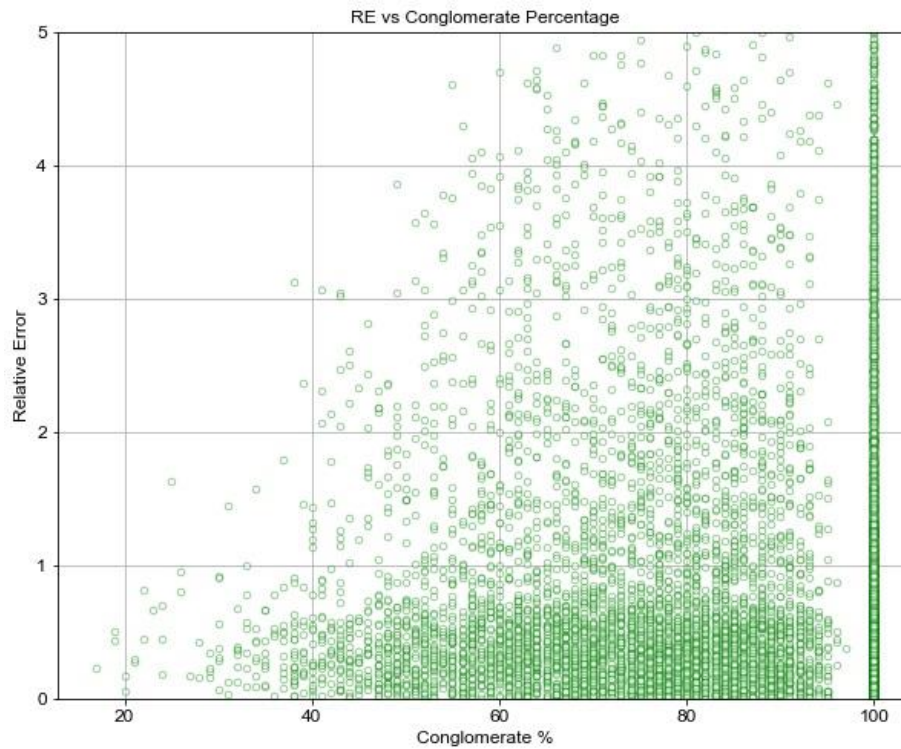
Figure 4.27: Scatter plot investigating the relationship between the RE and the Conglomerate Percentage.
