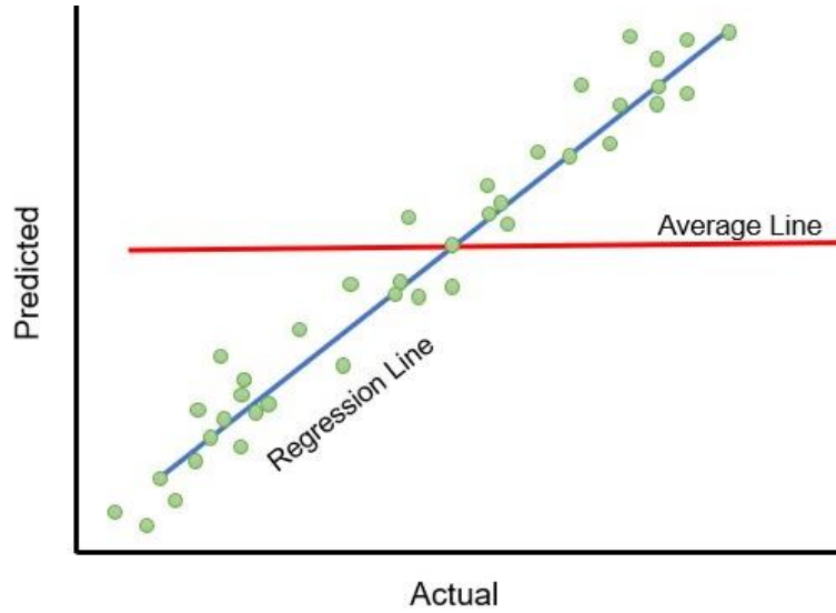
Figure 2.11: Graphical explanation of the CoD metric (adapted from Alencar et al., 2017 and Botchkarev, 2018).
