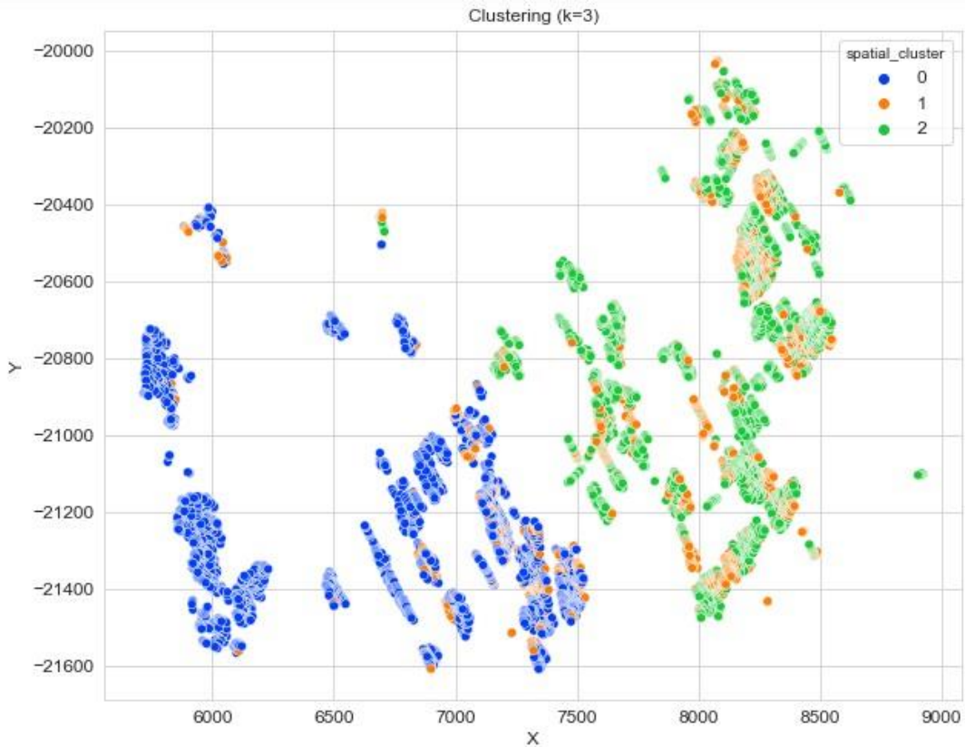
Figure 4.12: Spatial map visualising the full subset's clustered datapoints when spatial features are incorporated.
