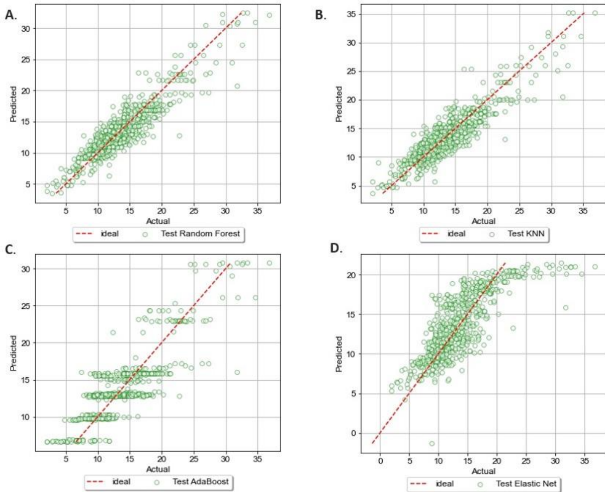
Figure 4.16: Graphical illustrations of the good subset's first round of testing for each of the four algorithms.
