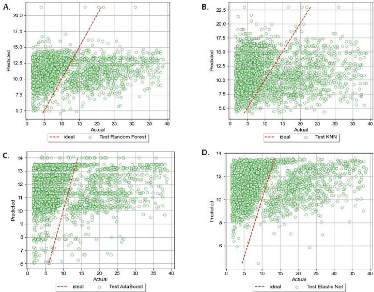
Figure 4.21: Graphical illustrations of the bad dataset's first round of testing for each of the four algorithms.
