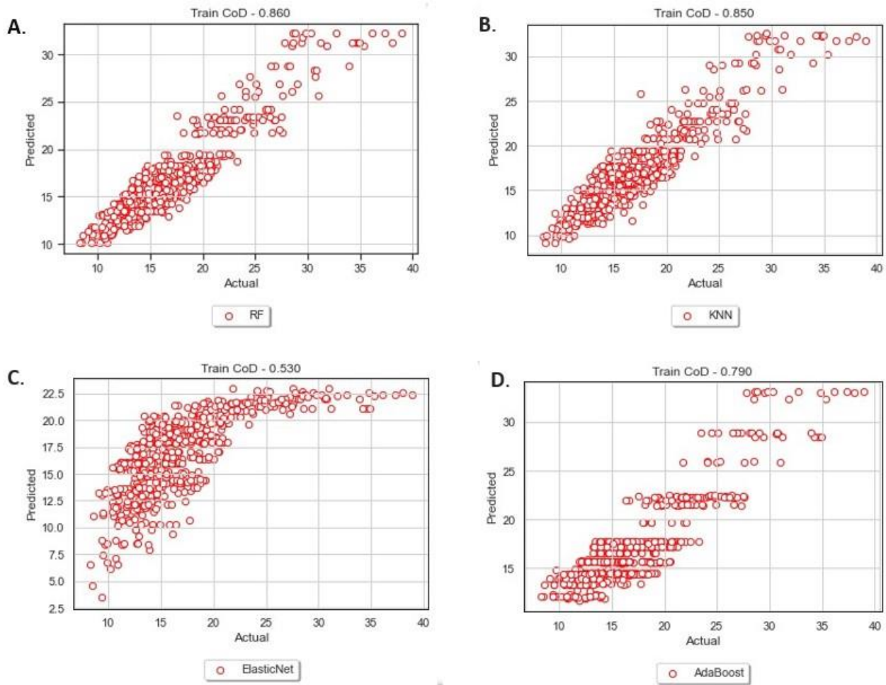
Figure B3: Graphical illustrations of the 'good' dataset's second round of training, visualising each algorithm's CoD scores.
