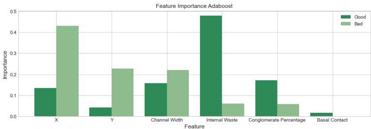
Figure 4.33: Graphical illustration of the AdaBoost's feature importance statistics for the 'good' and 'bad' datasets when spatial features are incorporated.
