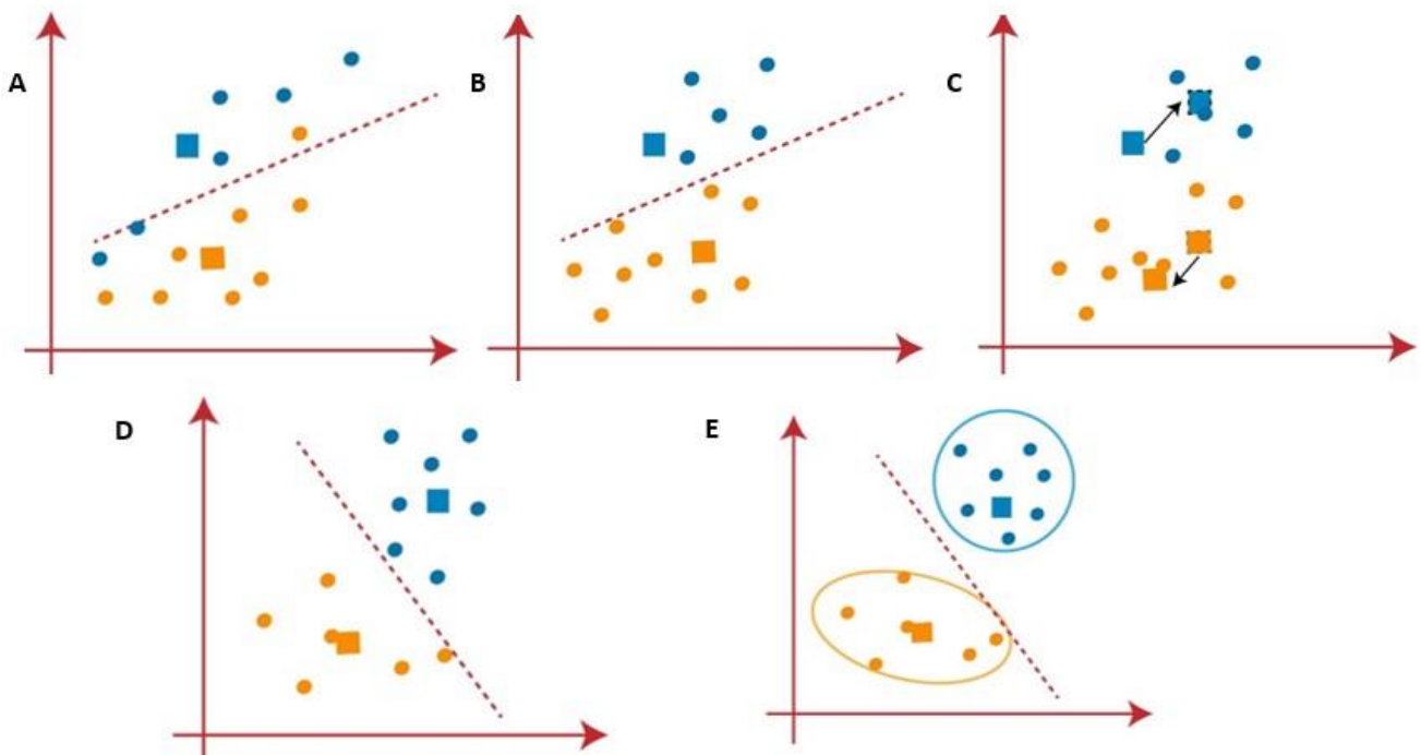
Figure 3.5: Graphical representation of the K-Means algorithm's clustering process. A K of 2 is assigned, and the clustered datapoints are represented in blue and orange. The median line (dashed) is generated by computing the median between the two centroids (adapted from Tan et al., 2021).
