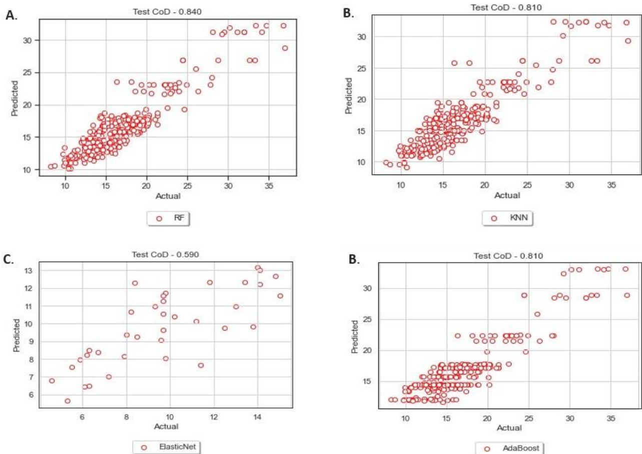
Figure 4.18: Graphical illustrations of the 'good' dataset's second round of testing, visualising each algorithm's CoD scores.
