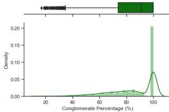
Figure 4.6: Boxplot and histogram illustrating the distribution of the Percentage Conglomerate data.
