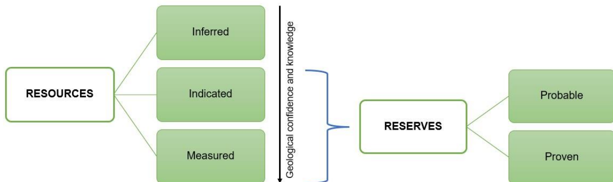
Figure 2.3: Generalised relationship between mineral resources and reserves (adapted from Dumakor-Dupey and Arya, 2021).
