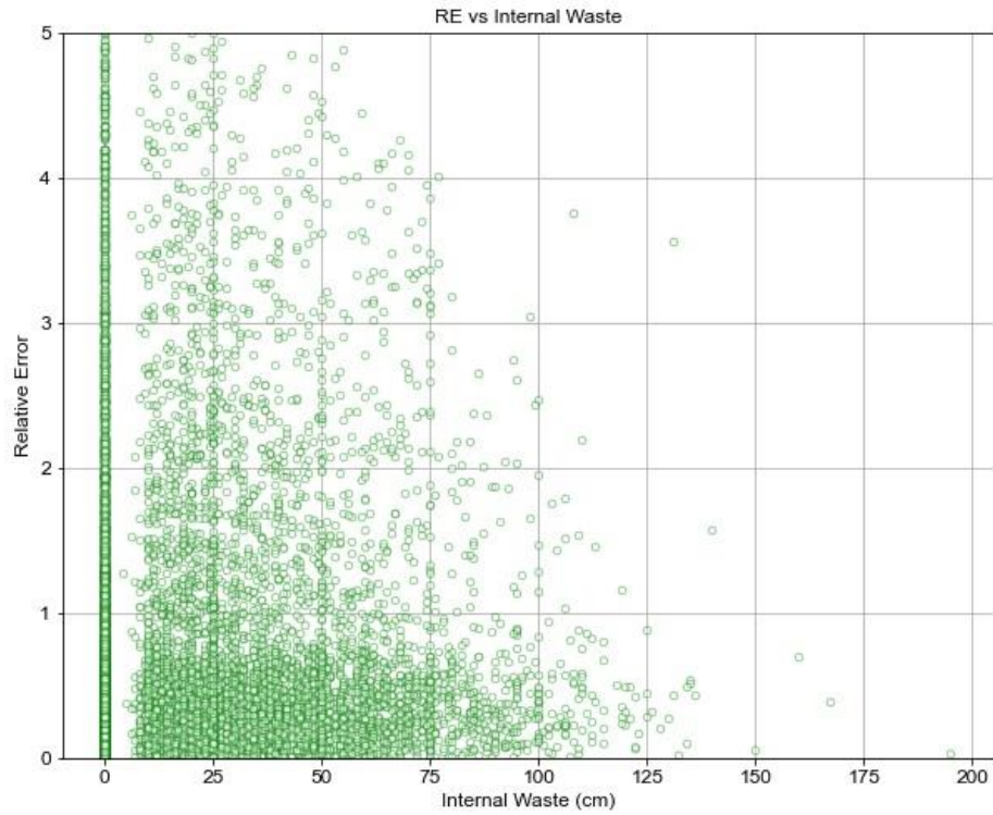
Figure 4.28: Scatter plot investigating the relationship between the RE and the Internal Waste.
