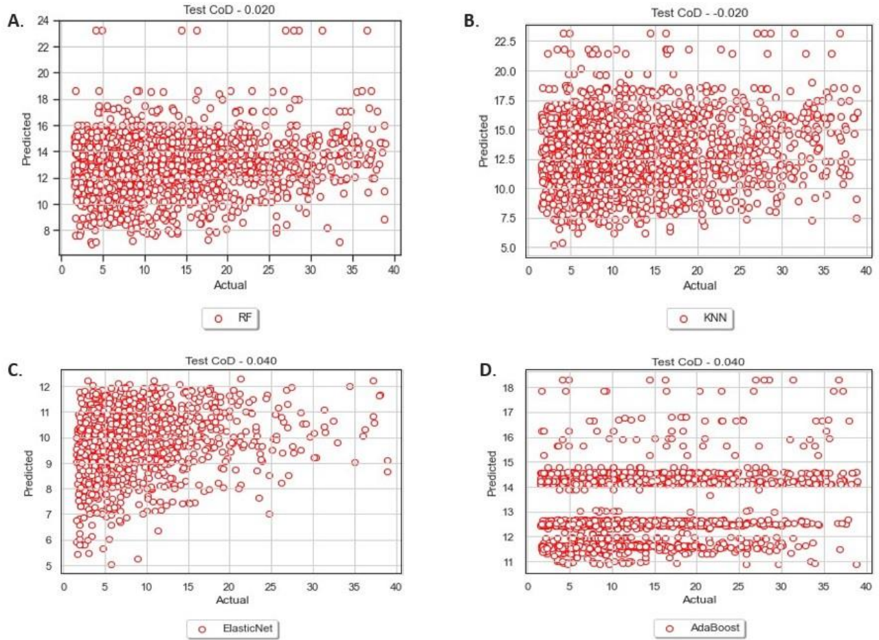
Figure 4.11: Graphical illustrations of the full subset's second round of testing, visualising each algorithm's CoD scores.
