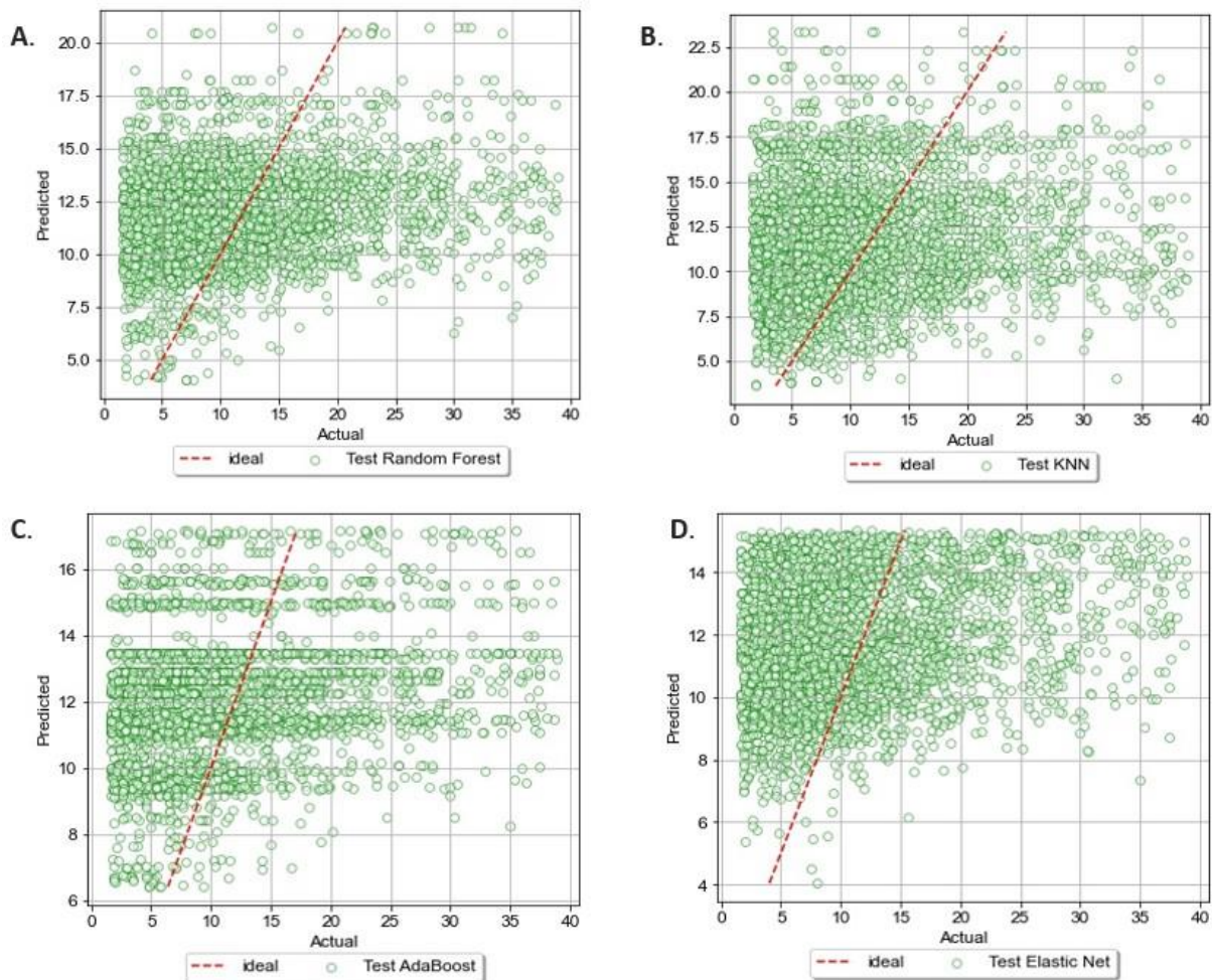
Figure 4.9: Graphical illustrations of the full subset's first round of testing for each of the four algorithms.
