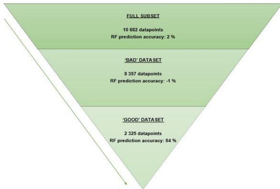
Figure 5.1: Figure illustrating the sample distribution between the full, 'bad' and 'good' datasets. The RF prediction score for each set is included.
