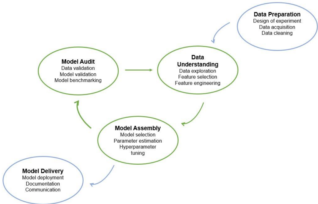
Figure 2.10: Flow chart illustrating an iterative variant of the CRISP-DM tool-agnostic predictive modelling procedure. The process is initiated by data preparation and followed by data understanding, model assembly and model audit. These three phases can be iterated. Then finally, the model delivery step concludes the process (adapted from Wickham and Grolemund, 2017 and Hall et al., 2019).
