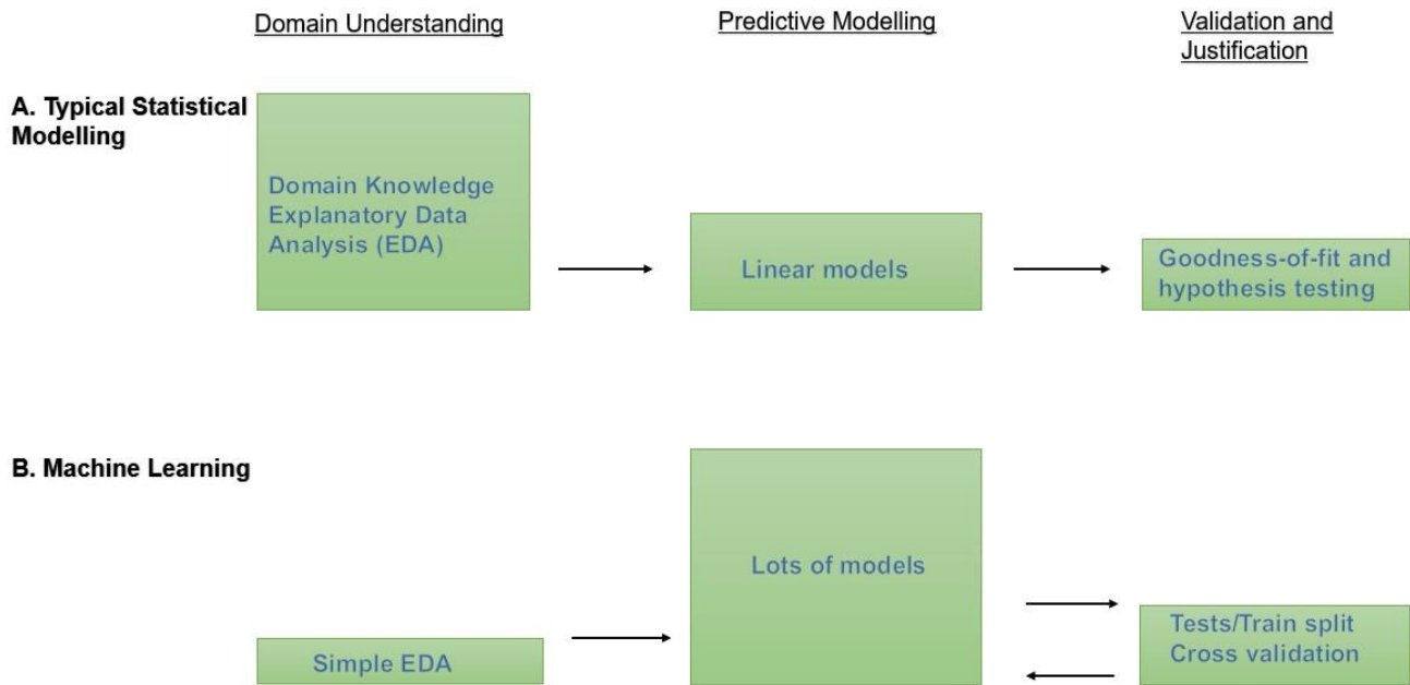
Figure 2.9: A simplified overview of the different predictive modelling processes in typical statistical modelling compared to machine learning. In typical modelling (A), much weight is placed on domain understanding, while in machine learning (B), much focus is placed on the predictive modelling process (adapted from Inglis et al., 2021).
