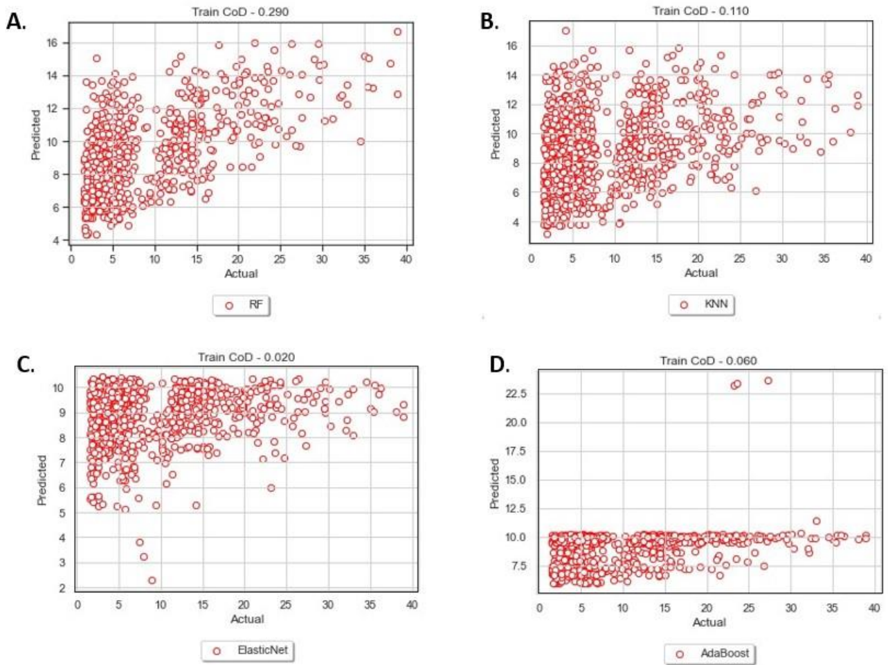
Figure B2: Graphical illustrations of the 'bad' dataset's second round of training, visualising each algorithm's CoD scores.
