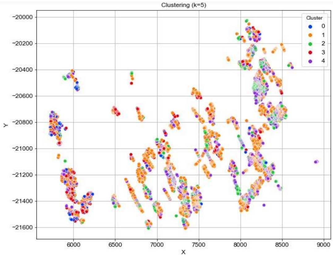
Figure 4.22: Spatial map visualising the 'bad' dataset's clustered datapoints when K = 5.
