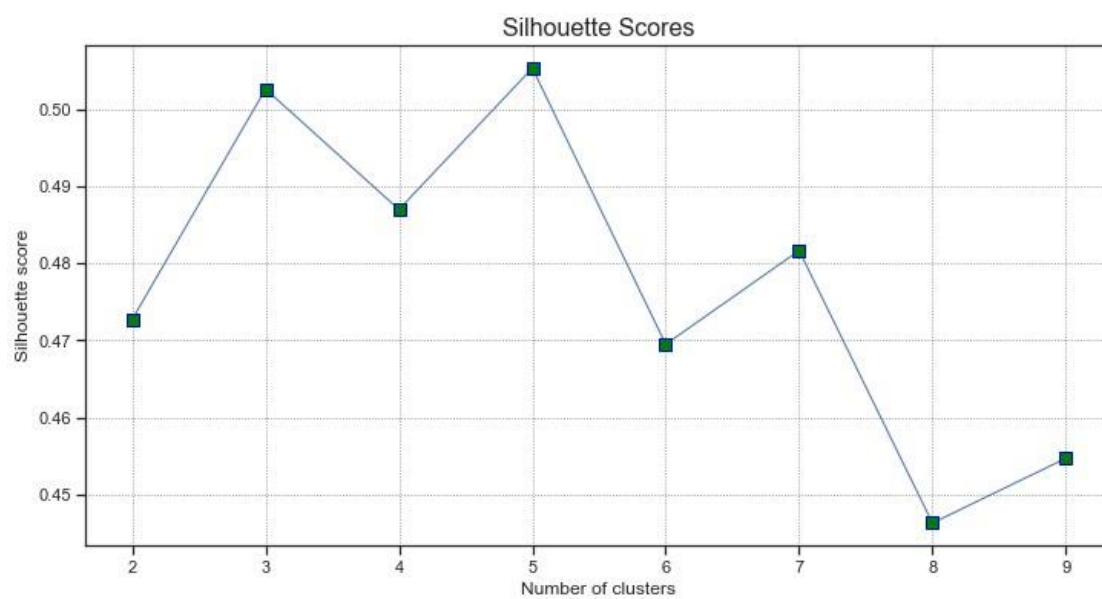
Figure A3: Graph visualising the 'good' dataset's silhouette scores.
