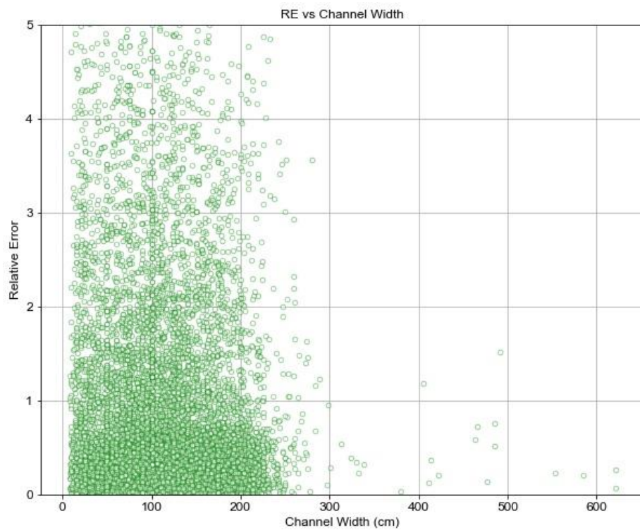
Figure 4.29: Scatter plot investigating the relationship between the RE and the Channel Width.
