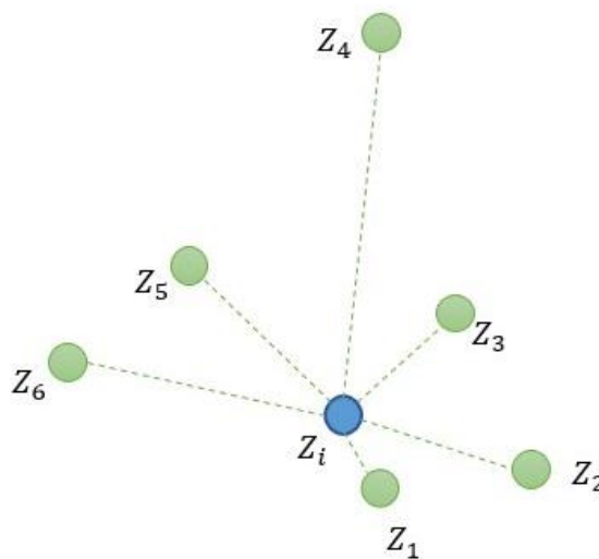
Figure 2.4: Generalised illustration of the IDW technique, where Z_i is the known point and the unknown points are in green. Z_1 would be assigned the highest weight (adapted from Coleman, 2021).
