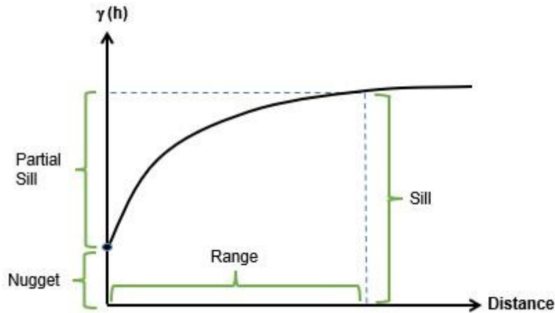
Figure 2.5: Simplified illustration of the semi-variogram (adapted from Rossi and Deutsch, 2014 and Coleman, 2021).
