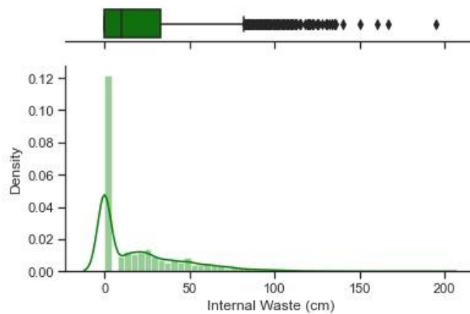
Figure 4.5: Boxplot and histogram illustrating the distribution of the Internal Waste data.
