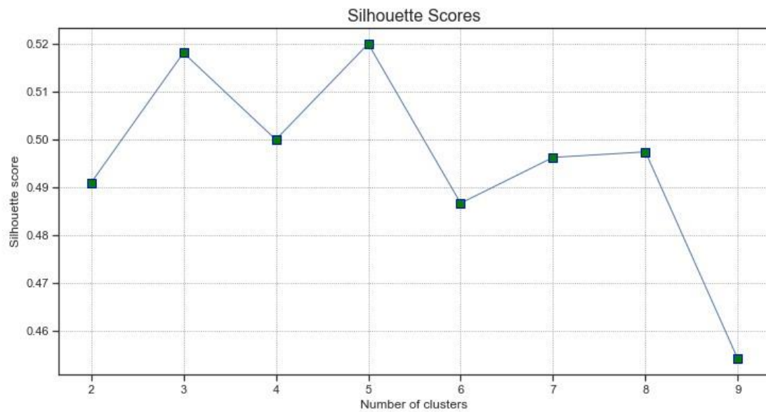
Figure A2: Graph visualising the 'bad' dataset's silhouette scores.
