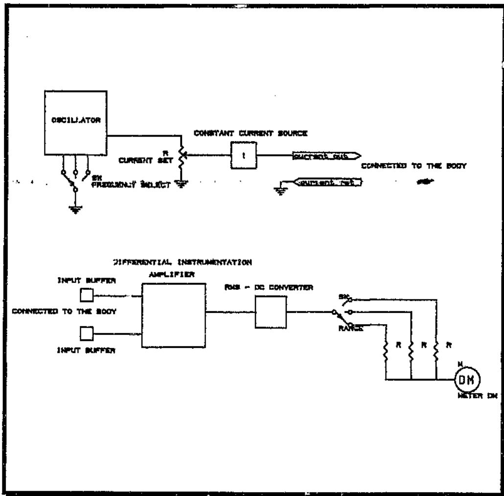
Figure 4.1: Block circuit diagram of impedance instrument
