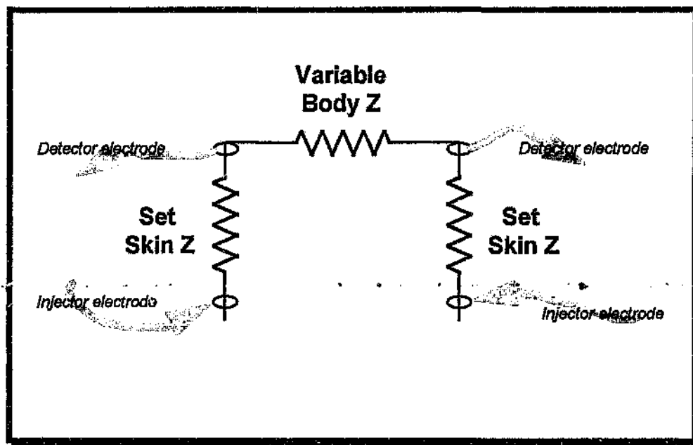
Figure 4.2: Graphic depiction of phantom impedance model of the body
