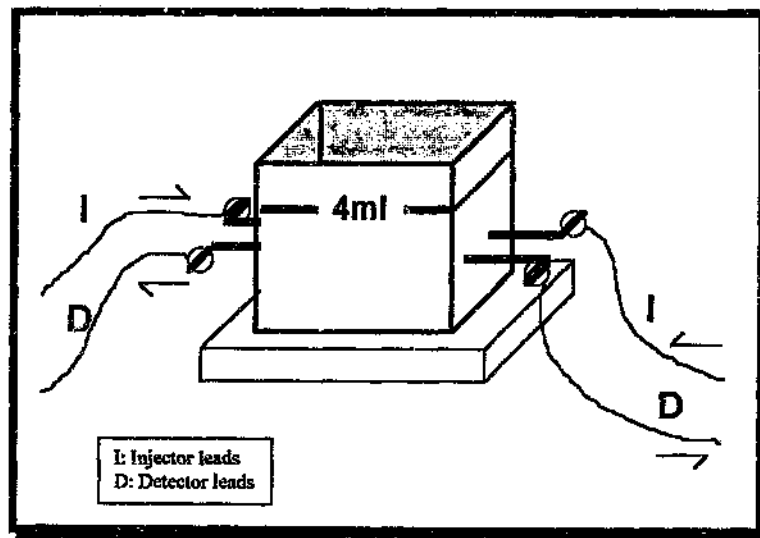
Figure 2.2: Blood impedance chamber
