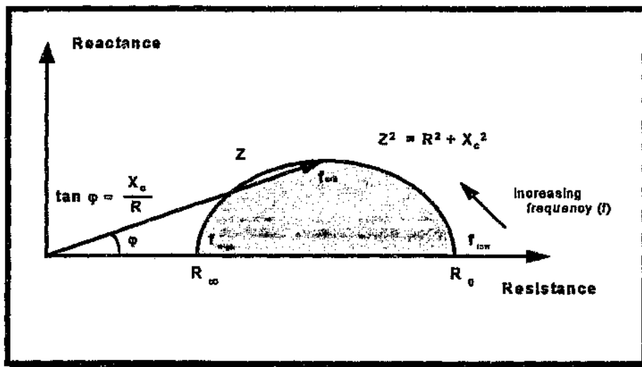
Figure 1.5: The relationships of impedance ( Z ), resistance ( R ), reactance ( X_c ) and current frequency ( f ).
