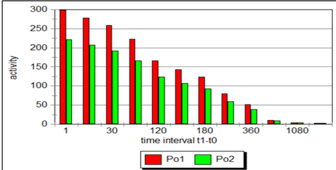
Figure 4-9: Scenario 3 - Expected activities for Po 1 and Po 2 (Initial Po = 0.3 Bq)
