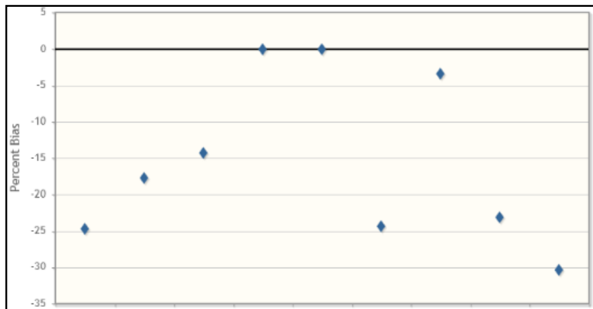
Figure 4-30: MAPEP Percentage bias for 234 U in water (S26-34 from left to right)
