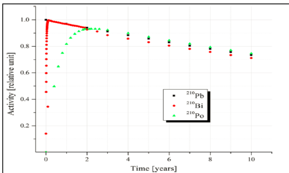
Figure 2-24: Changes of relative activities for ^{210}\text{Pb} , ^{210}\text{Bi} and ^{210}\text{Po} in time in an isolated system (Seslak et al. , 2016)
