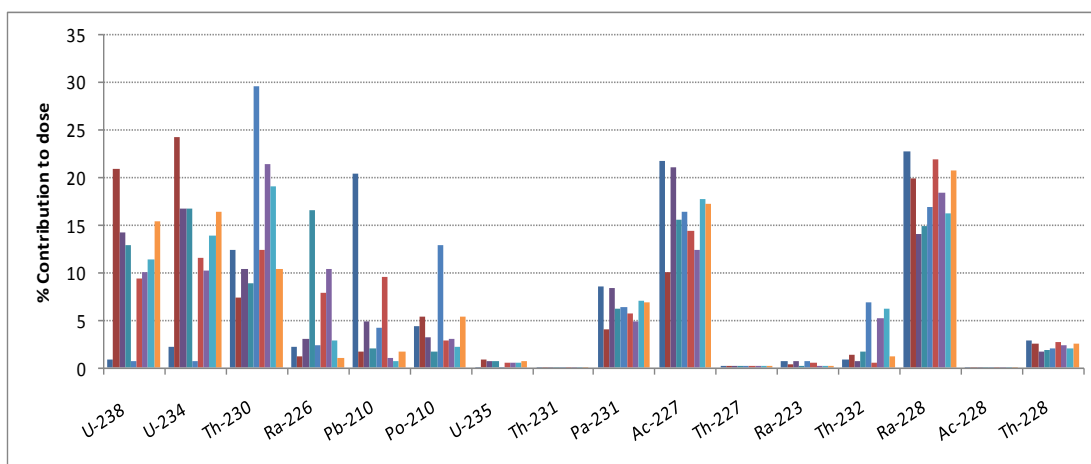
Figure 5-17: DWS region C - Relative contribution of individual nuclides to dose
