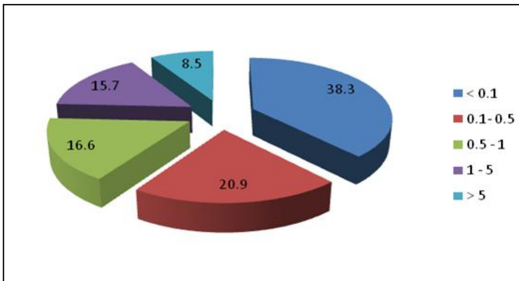
Figure 5-21: Gross alpha screening results of water samples from NORM industries analysed in 2014 (Bq.L -1 )
