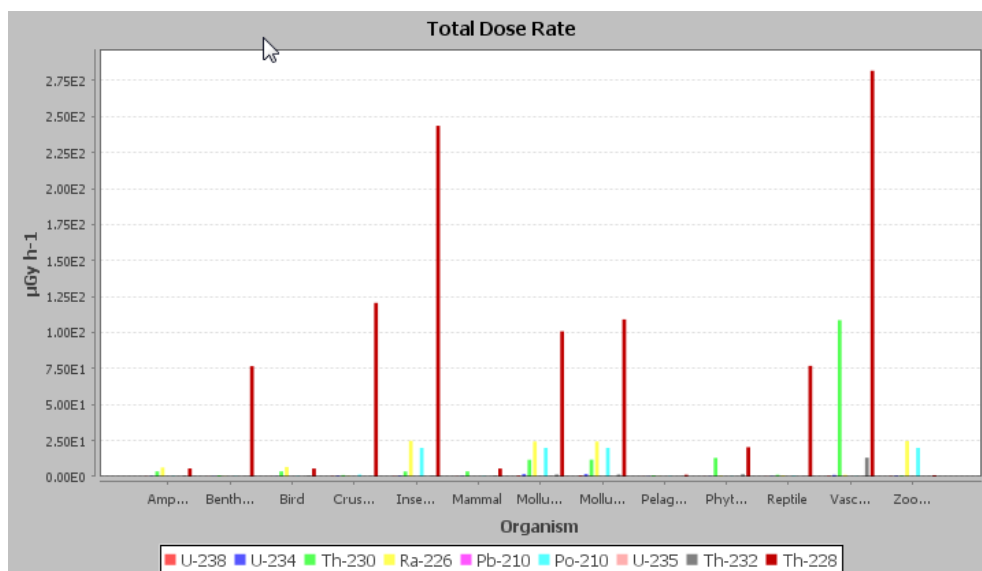
Figure 5-34: Dose rates ( \mu\text{Gy.h}^{-1} ) to aquatic reference organisms for phosphate industry site.
