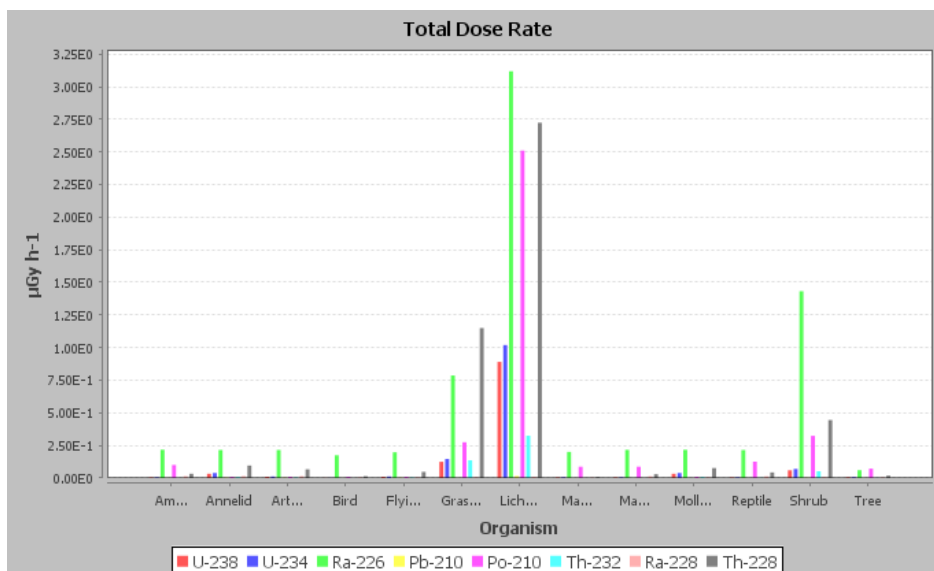
Figure 5-32: Dose rates ( \mu\text{Gy.h}^{-1} ) to terrestrial reference organisms for mineral sands site.
