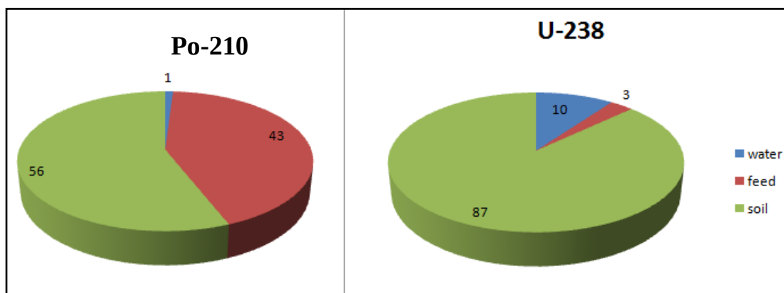
Figure 5-30: Cattle Ingestion percentages from soil, grass and water
