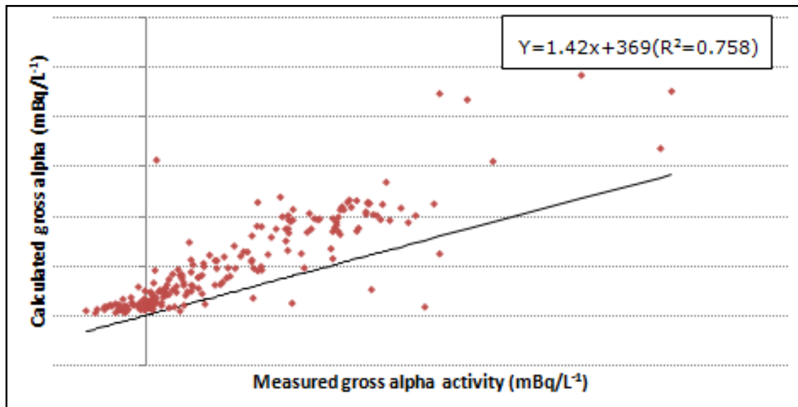
Figure 5-15: DWS region C - Comparison of calculated gross activity with measured gross activity
