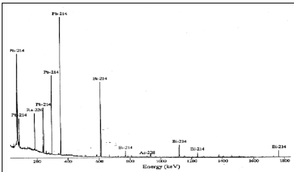
Figure 4-5: A typical gamma spectrum of natural radioactivity
