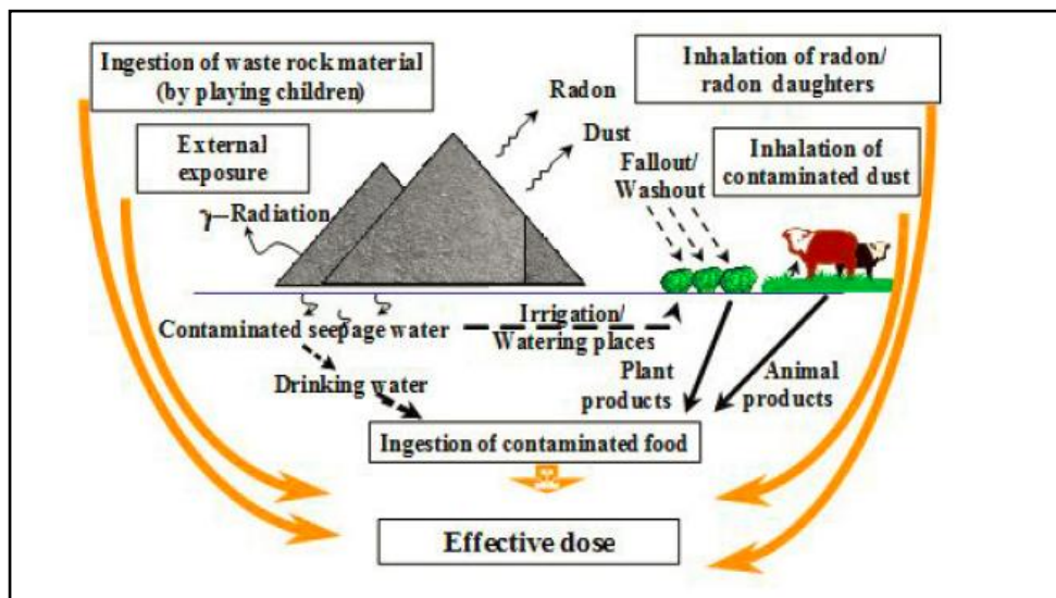
Figure 2-20: Exposure pathways at a tailings storage facility
