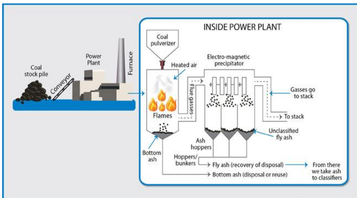
Figure 2-16: Schematic of a Pulverized fuel power station (WCA, 2013)
