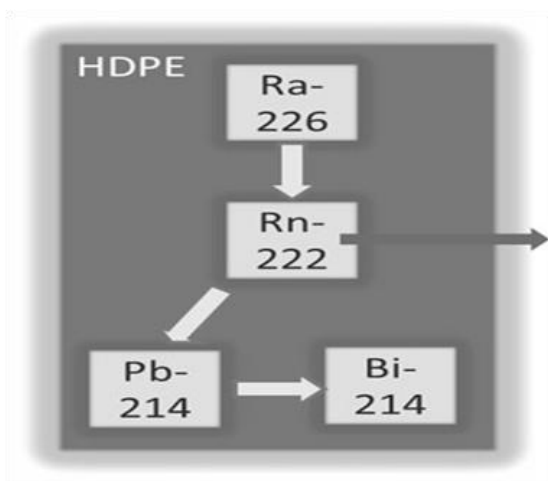
Figure 4-3: Measurement of ^{226}\text{Ra} via radon progeny (dark arrow represents leakage)
