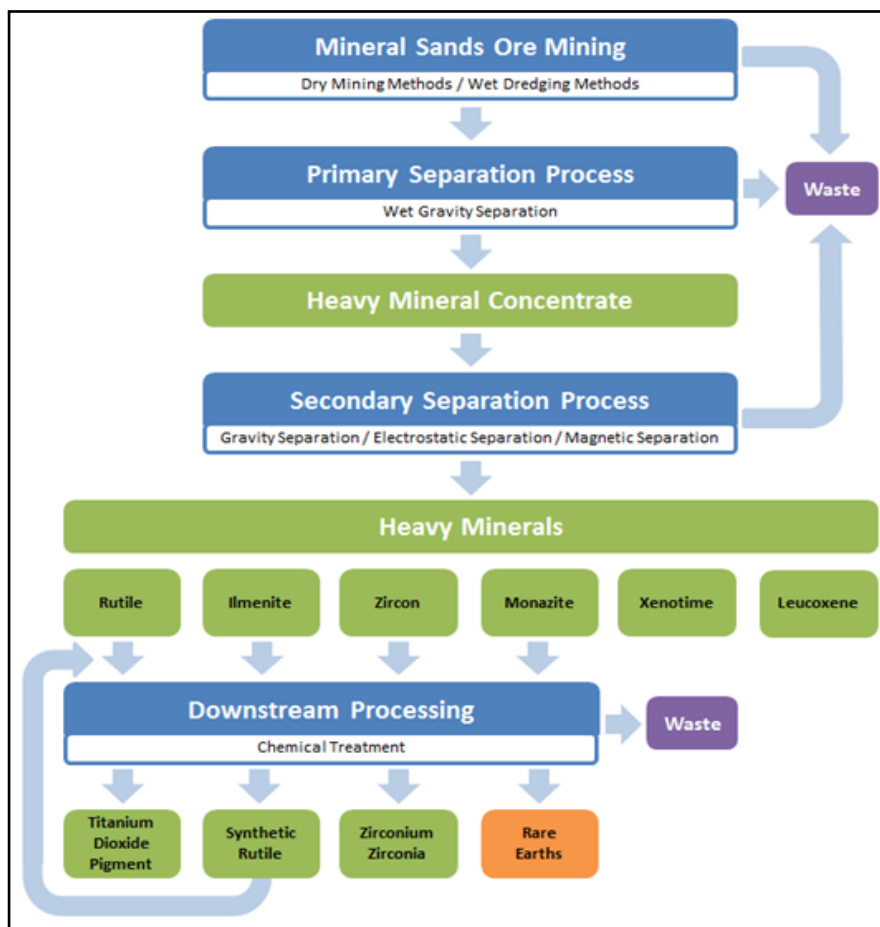
Figure 2-12: Mineral sands separation process (Collett et al. , 2014)
