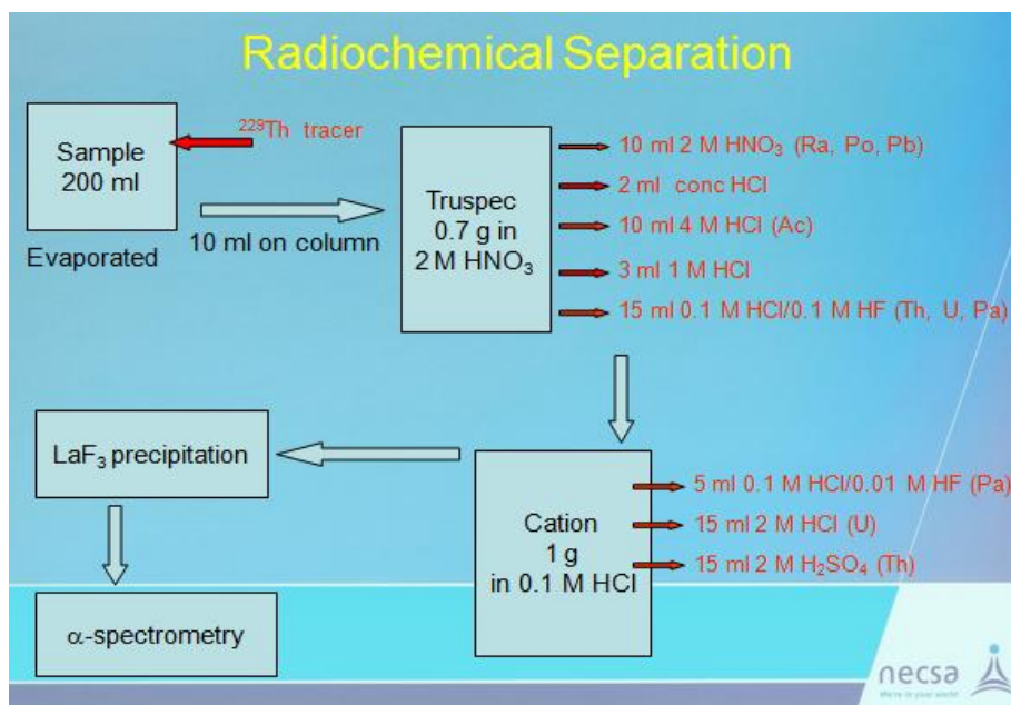
Figure 4-19: Schematic presentation of method for Th determination using TRU resin
