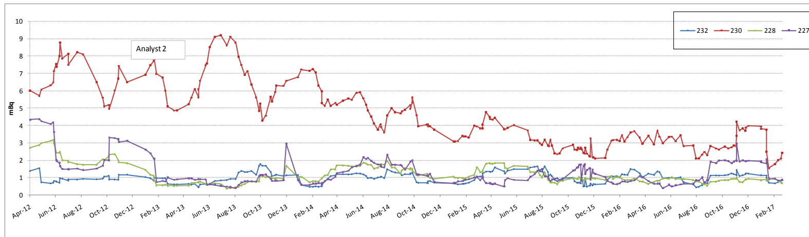
Figure 4-32: Moving average of Th blank from 2012-2017 (mBq)
