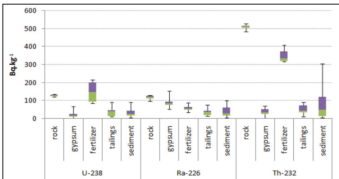
Figure 5-44: Minimum, median, 75% percentile and maximum concentrations for solids from the phosphate industry (Bq.kg -1 )
