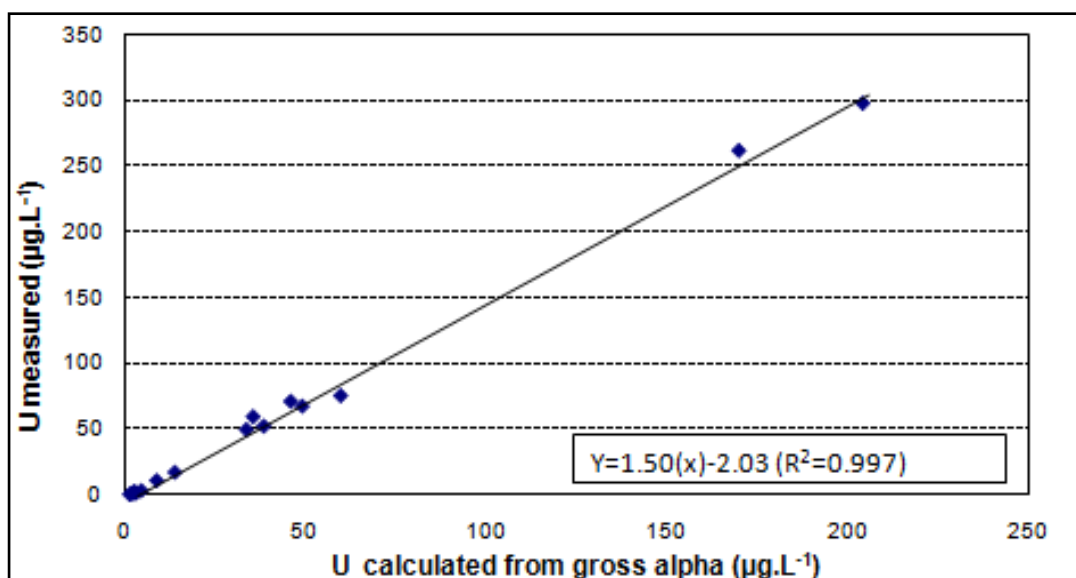
Figure 5-11: DWS Surface water - Comparison of measured (KPA) to expected uranium concentrations (from gross alpha)
