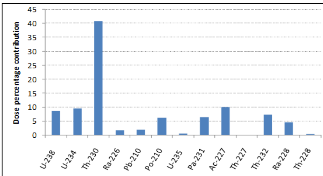
Figure 5-28: Dose overestimation due to high limit of detection for ^{238}\text{U} ( =^{230}\text{Th} )
