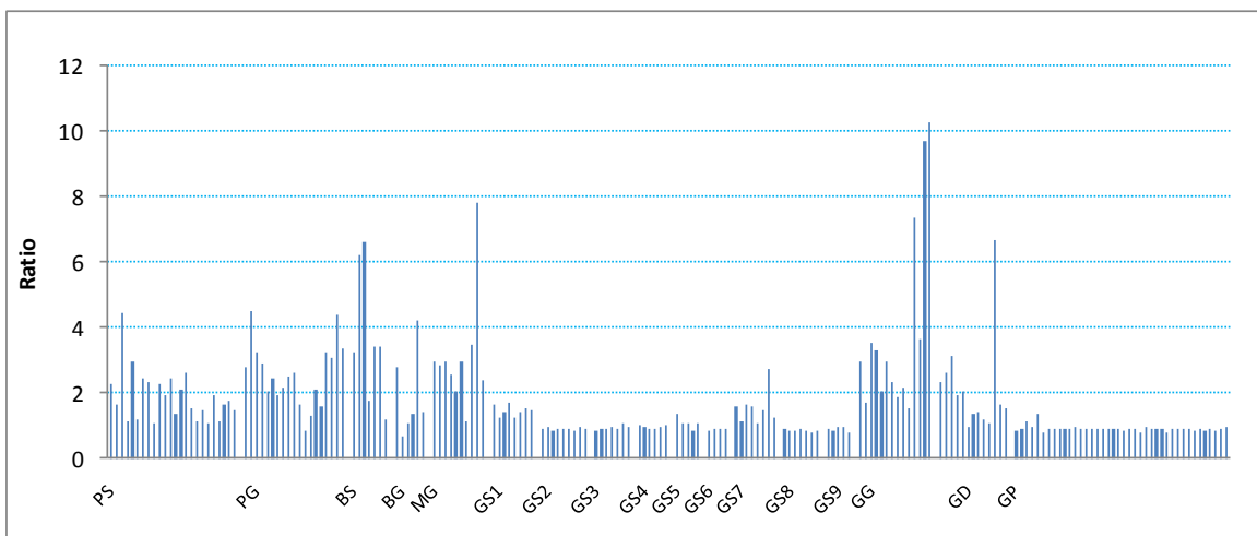
Figure 5-22: ^{234}\text{U}/^{238}\text{U} ratios observed in water samples from NORM industries
