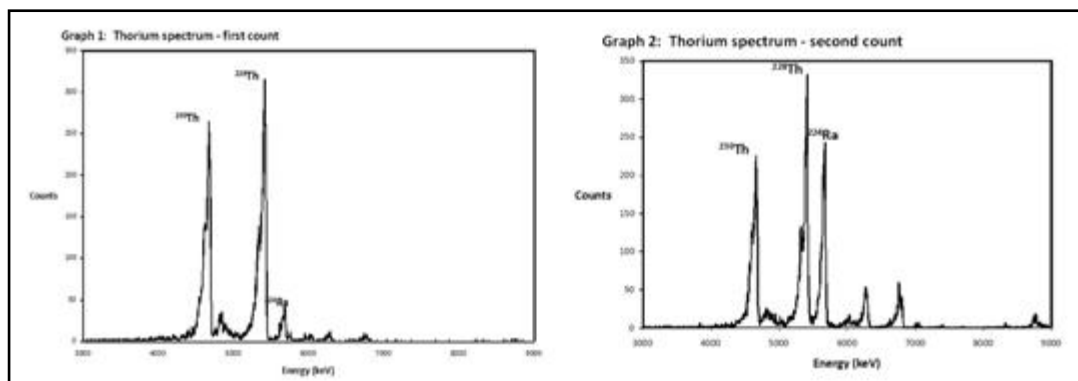
Figure 4-24: Alpha spectrum of thorium in ammonium -diuranate
