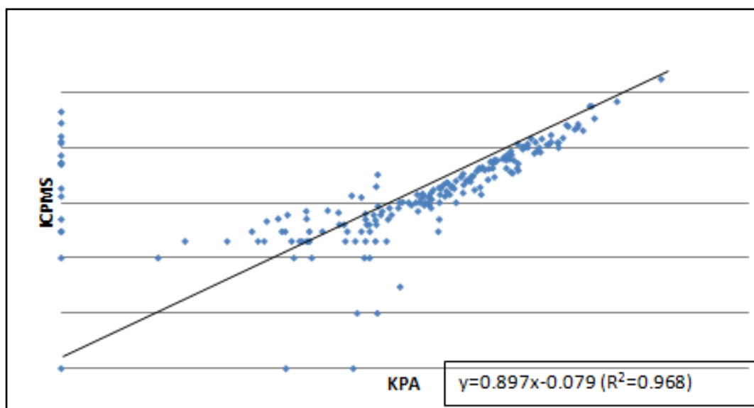
Figure 5-12: Comparison of KPA and ICPMS values for U measured in DWS groundwater samples
