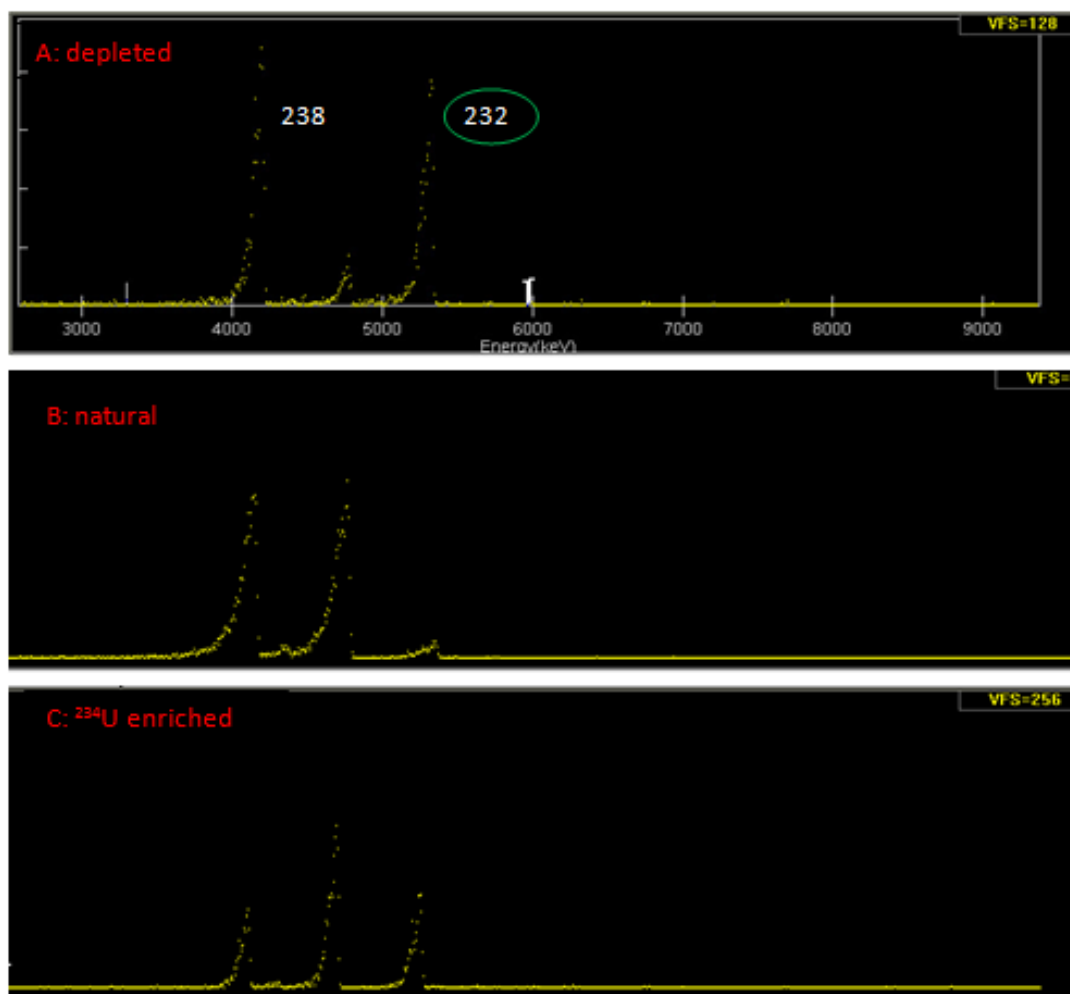
Figure 4-17: Typical energy spectra for uranium analysis showing the peaks for ^{238}\text{U} , ^{235}\text{U} , ^{234}\text{U} and ^{232}\text{U}
