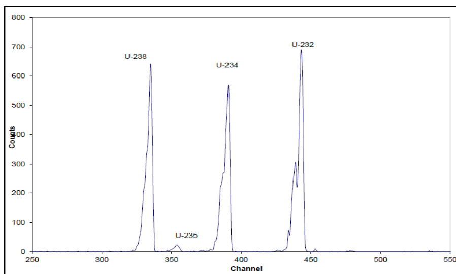
Figure 2-25: Typical alpha spectrum for natural uranium
