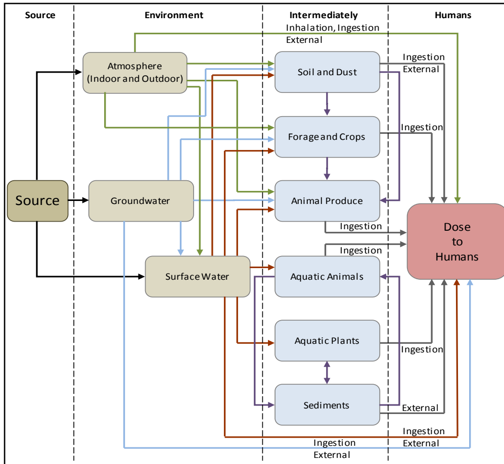
Figure 2-5: Source-pathway-receptor approach for dose assessment (IAEA, 2003a).
