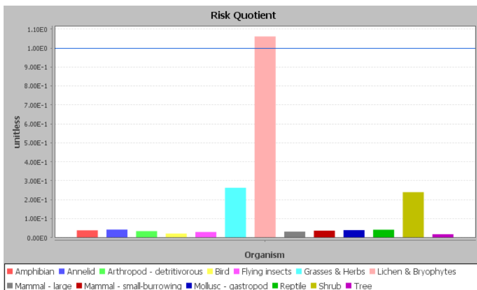
Figure 5-31: Risk Quotient for Tier 2 screening Terrestrial environment (Mineral sands site)
