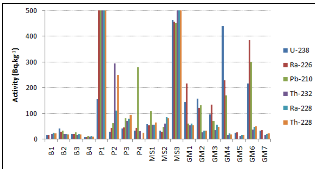
Figure 5-39: Average activity concentrations in sediment samples from areas affected by NORM industries
