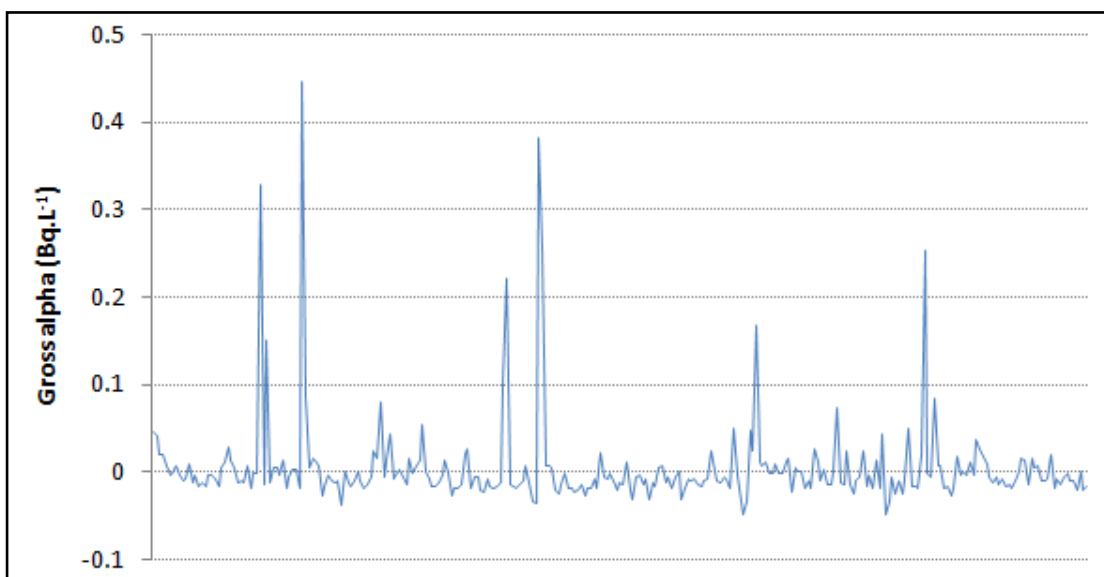
Figure 5-2: Gross alpha activity of bottled water (Bq.L -1 )
