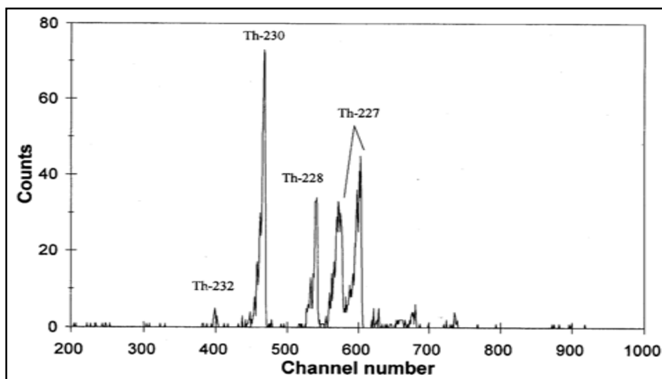
Figure 2-1: Typical alpha-particle spectrum of thorium analysis by radiochemical separation showing high ^{230}\text{Th} concentration.
