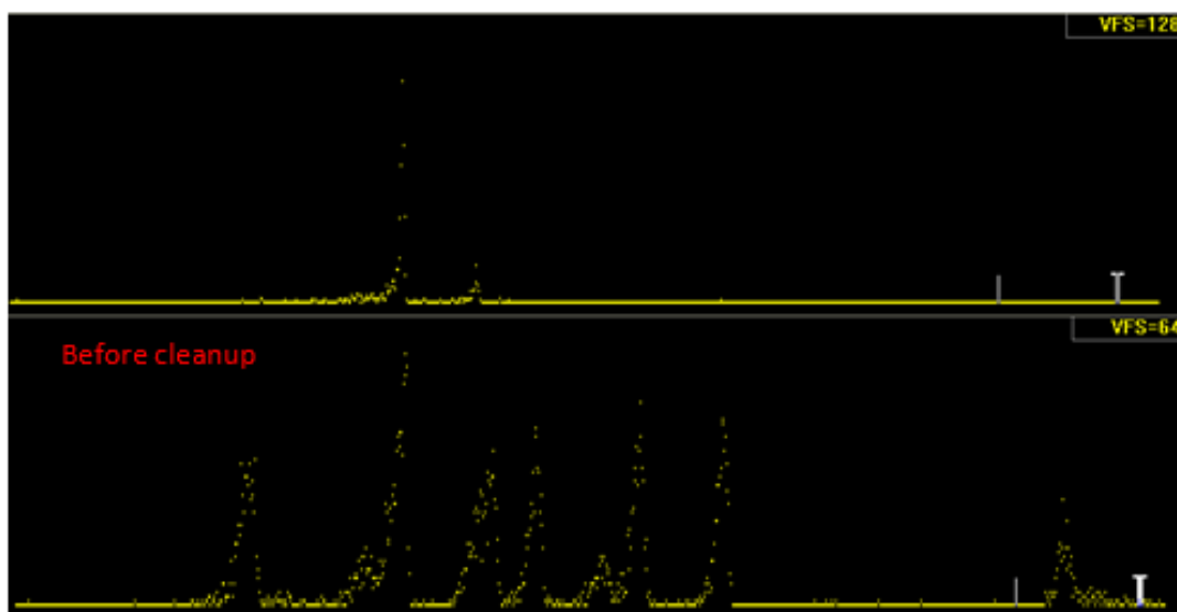
Figure 4-12: Spectrum of ^{210}\text{Po} showing interference of high Th concentration removed by TRU resin
