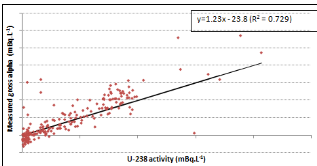
Figure 5-14: DWS region C - Correlation between gross alpha activity and ^{238}\text{U} activity Dose and Radiological Quality
