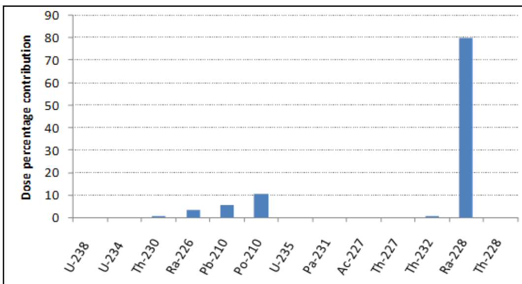
Figure 5-27: Showing large contribution of ^{228}\text{Ra} to dose for some vegetable samples
