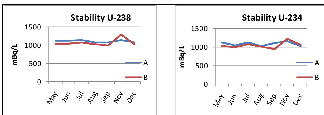
Figure 4-26: Uranium activity concentrations for stability sample fractions A and B
