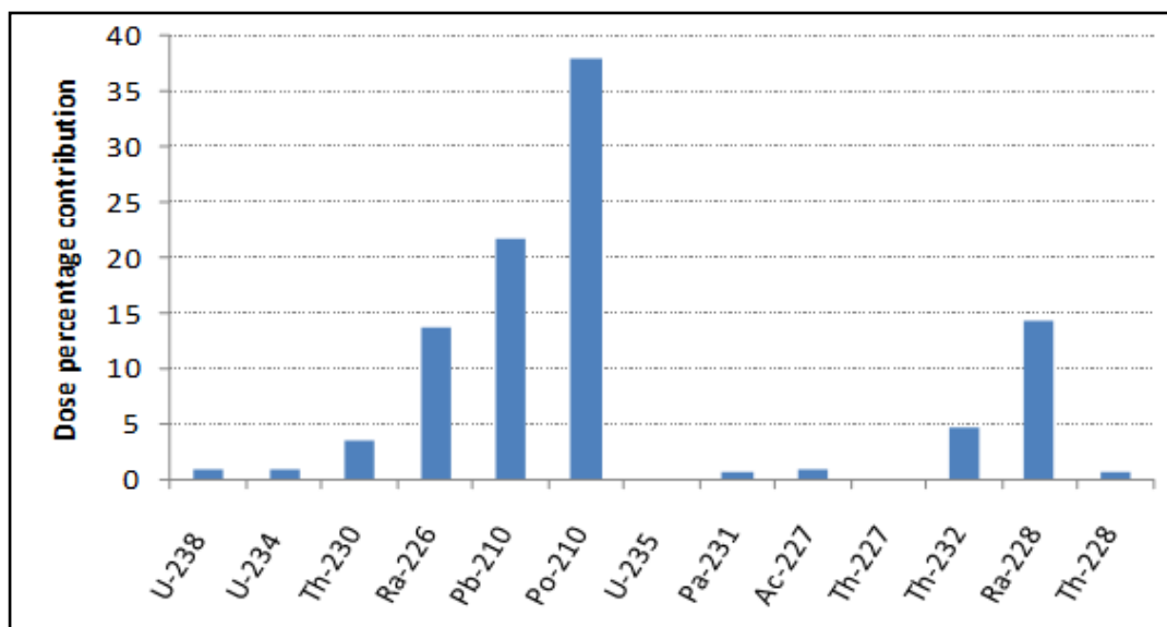
Figure 5-26: Typical dose contribution for most vegetable samples
