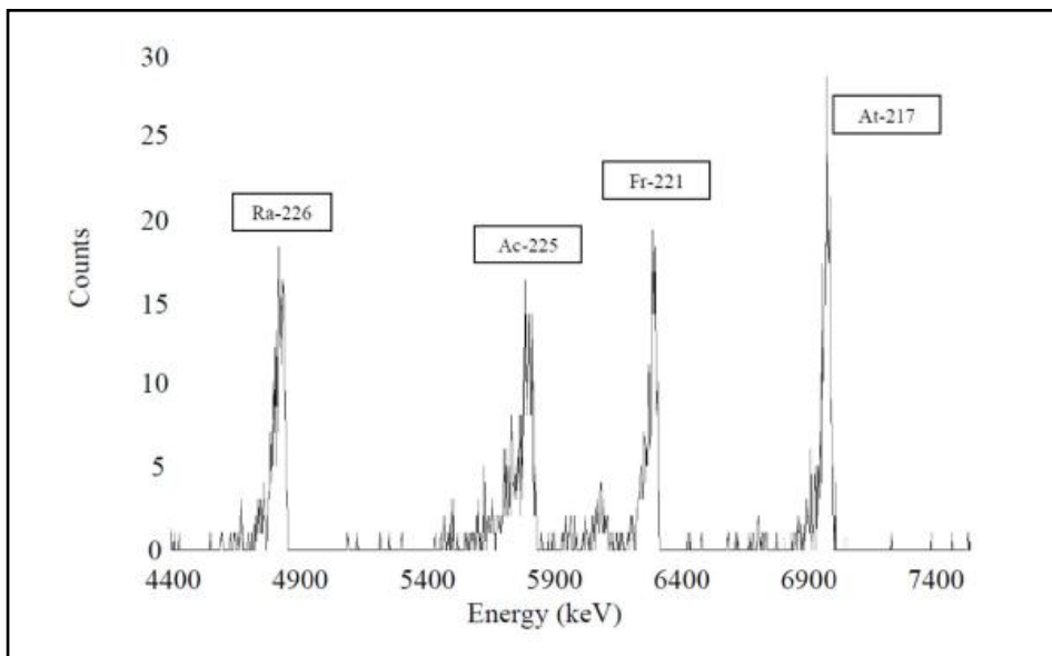
Figure 2-27: Spectrum of ^{226}\text{Ra} with ^{225}\text{Ra} as tracer
