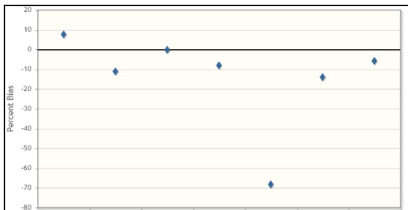
Figure 4-29: MAPEP Percentage bias for U in water by KPA (S27-34 from left to right, S30 not reported)
