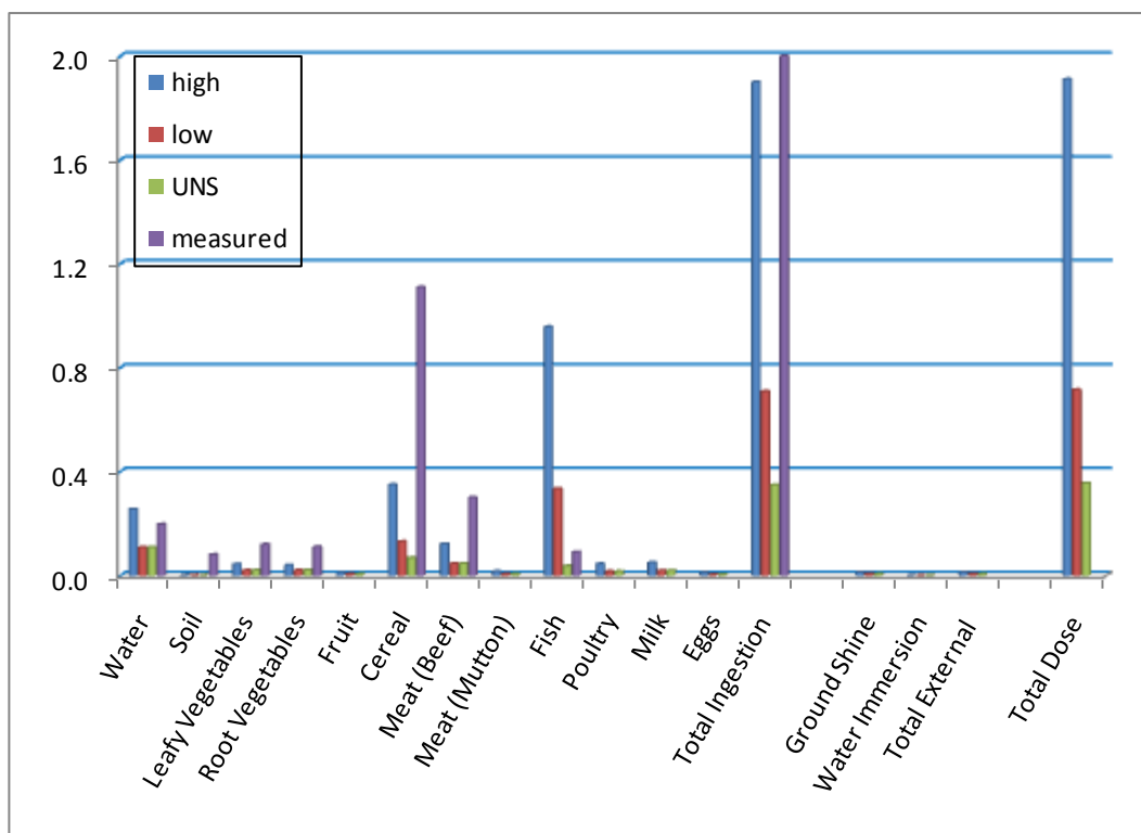
Figure 5-46: Effective dose for the Hypothetical Farmer Exposure Condition (modelled)
