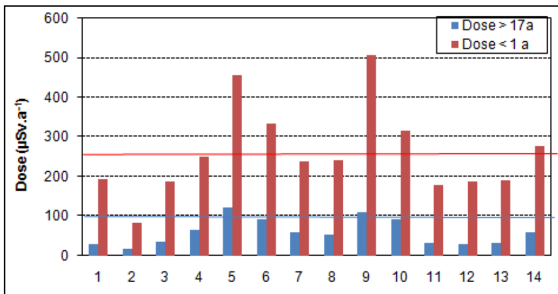
Figure 5-16: DWS region C - Average annual effective dose per sampling point (μSv.a -1 )
