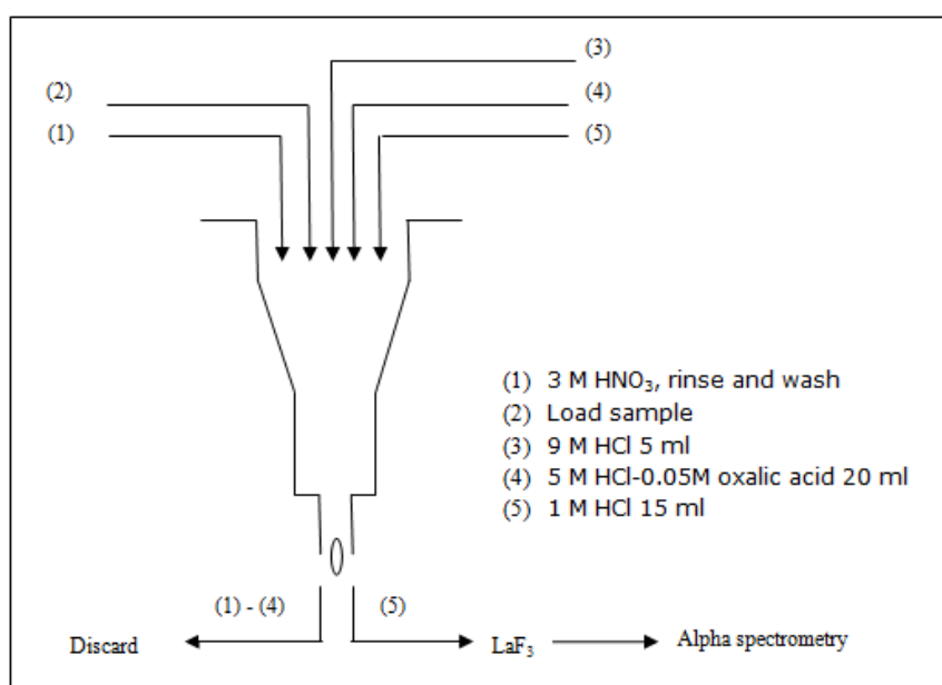
Figure 4-14: Analysis sequence for separation of U on UTEVA resin
