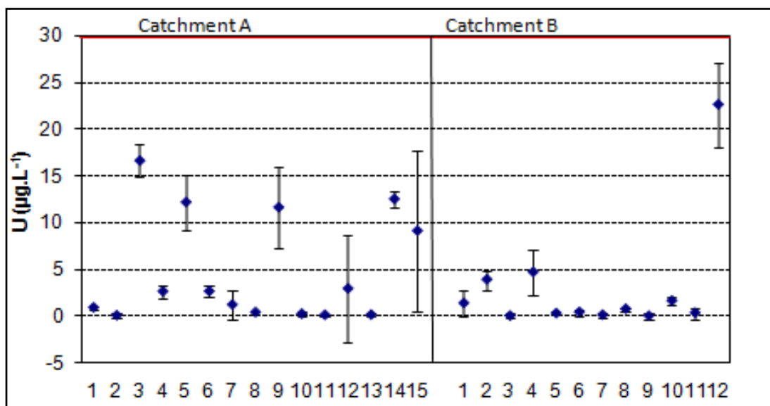
Figure 5-6: Uranium concentration ( \mu\text{g.L}^{-1} ) in DWS groundwater samples
