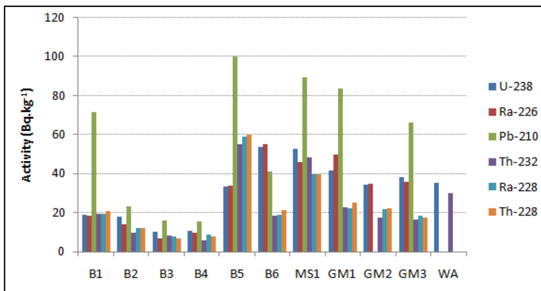
Figure 5-38: Average activity concentrations in soil samples from areas affected by NORM industries (B-Baseline; MS-Mineral Sands; GM-Gold Mine; WA-World Average)
