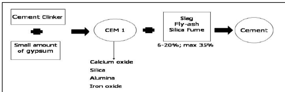
Figure 2-14: Production of cement
