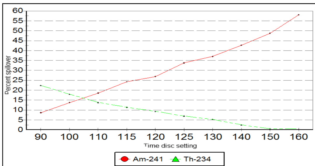
Figure 4-21: Time discriminator setting chart: Percentage spill versus pulse discriminator setting
