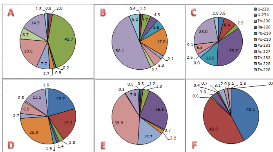
Figure 5-25: Contribution of individual nuclides to ingestion dose for water from different sources
