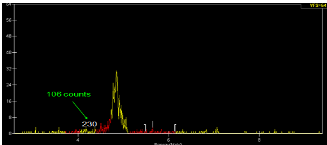
Figure 4-25: Spectrum showing high counts in ROI for ^{230}\text{Th} due to overlap from ^{229}\text{Th} peak
