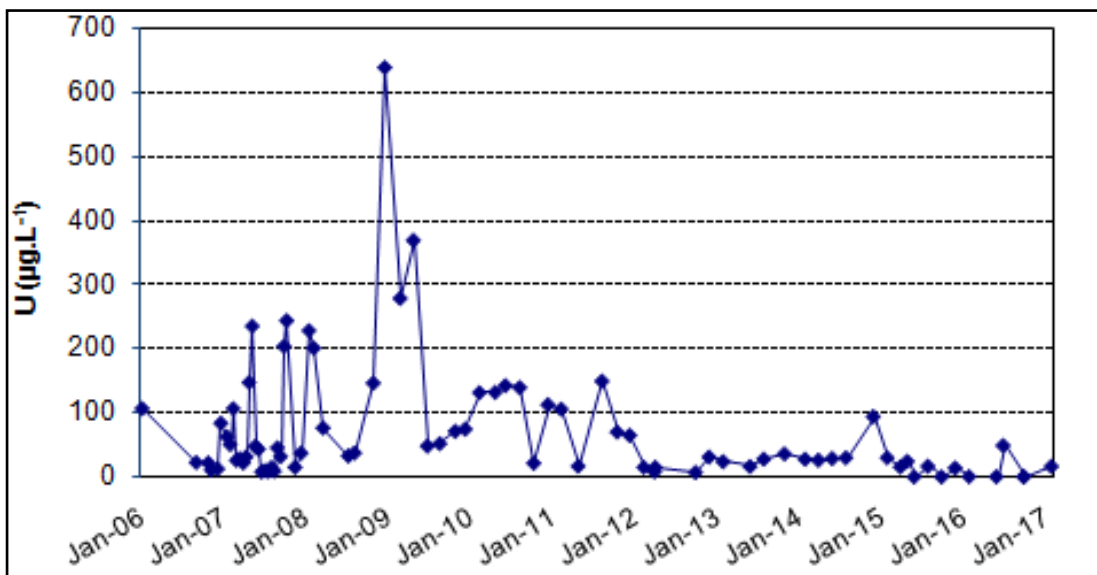
Figure 5-10: Variation in U concentration at sampling point 4 of DWS surface water
