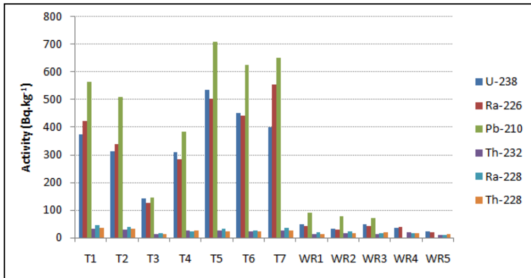
Figure 5-40: Average activity concentrations in tailings and waste rock samples from a gold mine
