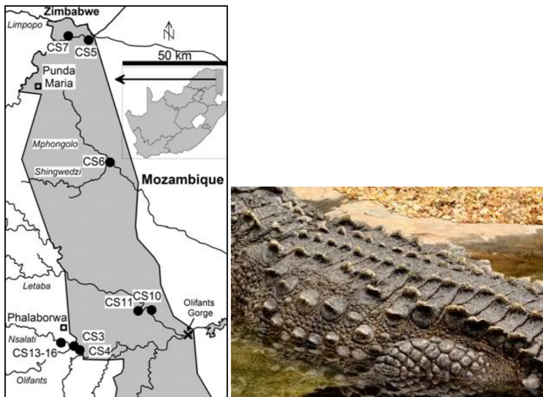
Figure 5-36: Sampling points Crocodile
