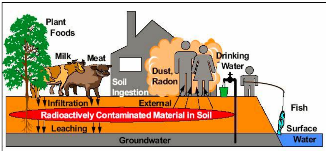
Figure 2-6: Pathways to consider for dose assessment (USDOE, 2002)
