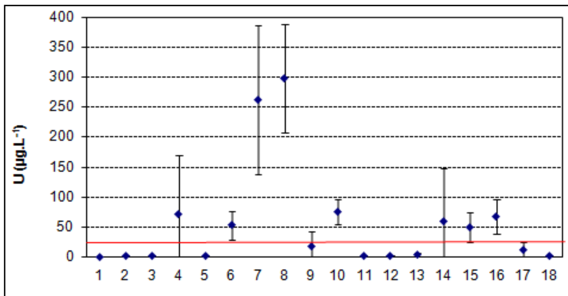
Figure 5-8: Uranium concentration in DWS surface water samples (µg.L -1 )
