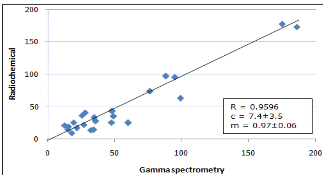
Figure 5-42: Correlation plot for ^{228}\text{Th} in cement samples (Activity concentration in \text{Bq.kg}^{-1} )
