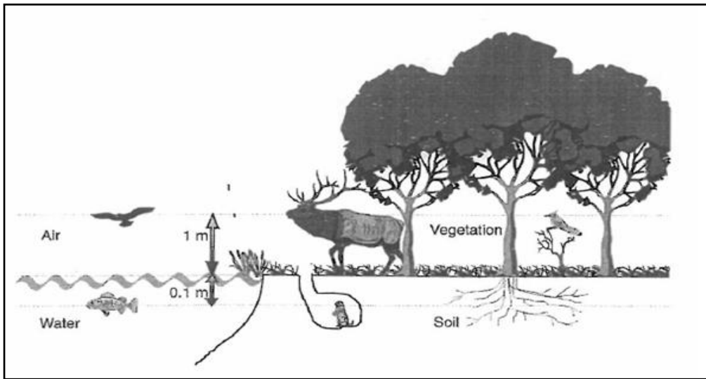
Figure 2-7: Exposure pathways for plants and animals
