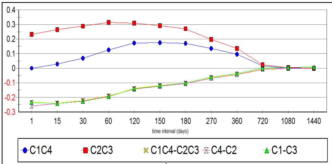
Figure 4-10: Decay and ingrowth of Po as function of t_1-t_0 ( t_2-t_1=60 d, \text{Pb}=\text{Po}=0.3 Bq)
