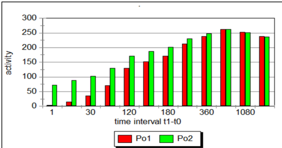
Figure 4-8: Scenario 2 - Expected activities for \text{Po}_1 and \text{Po}_2 (Initial \text{Pb} = 0.3\text{Bq} )
