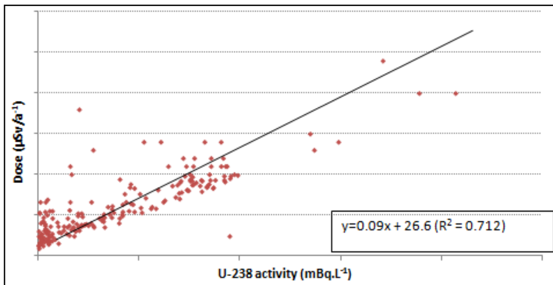
Figure 5-18: DWS region C - Correlation between dose and ^{238}\text{U} activity concentration
