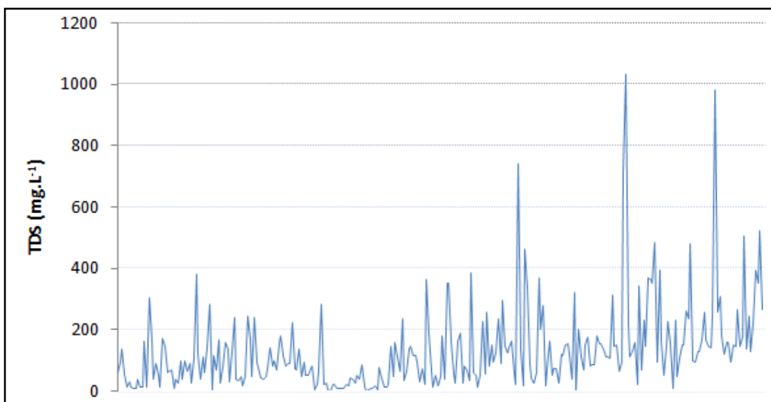
Figure 5-1: Total Dissolved Solids (TDS) for bottled water (mg.L -1 )
