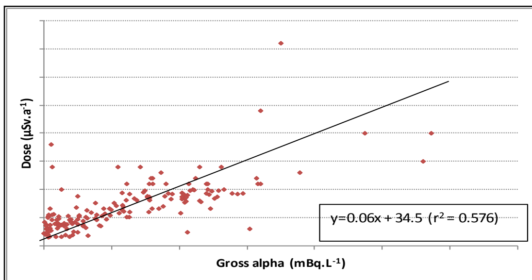
Figure 5-19: DWS region C - Correlation between annual radiation dose and gross alpha activity
