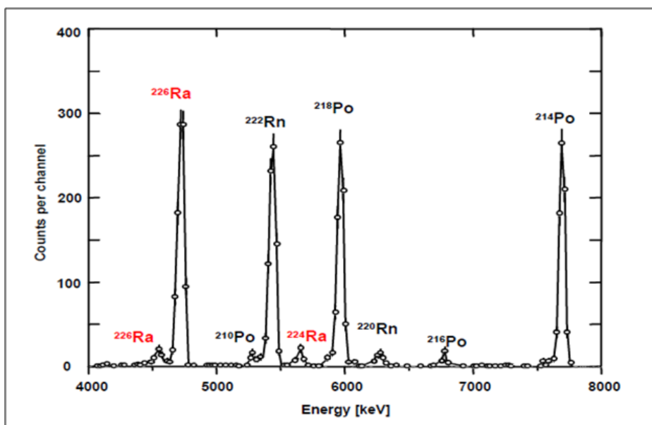
Figure 2-26: Alpha spectrum of ^{226}\text{Ra} and progeny
