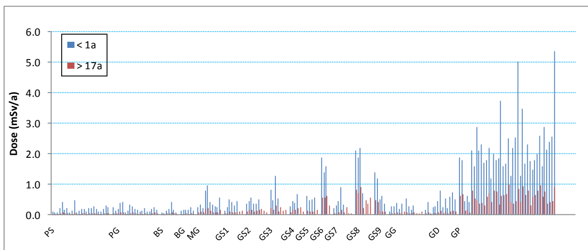
Figure 5-24: Annual ingestion dose for adult and infant age groups for all water sources from NORM industries
