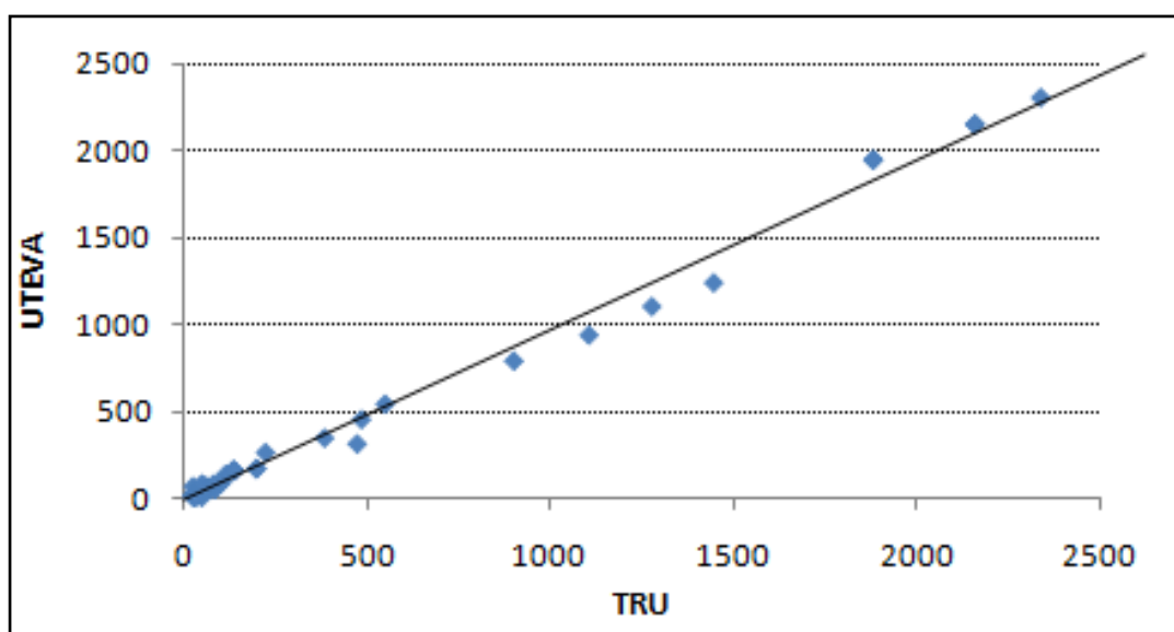
Figure 4-18: Comparison of ^{238}\text{U} results for water samples from the mining industry obtained with two different resins [y = 0.98x - 3.38 (R^2 = 0.992)]
