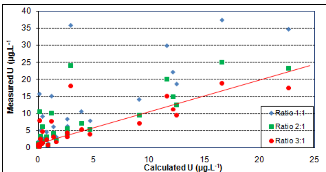
Figure 5-7: DWS Groundwater: Comparison of measured (KPA) to expected uranium concentrations (from gross alpha)
