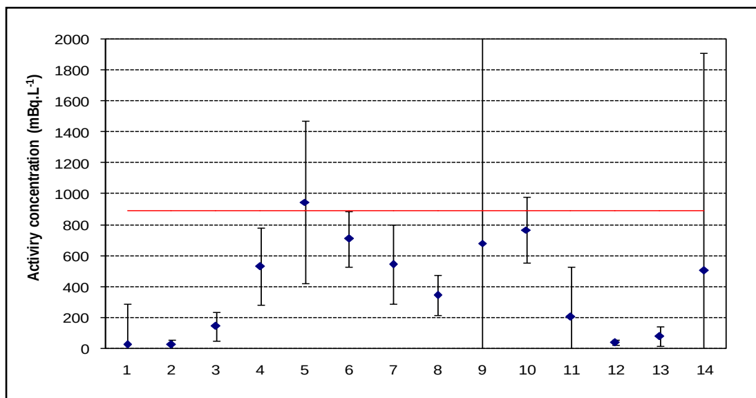
Figure 5-13: DWS region C - Uranium-238 activity concentration in water samples (mBq.L -1 )
