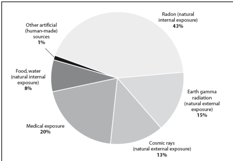
Figure 1-1: Sources of radiation contributing to public exposure (UNSCEAR, 2000)
