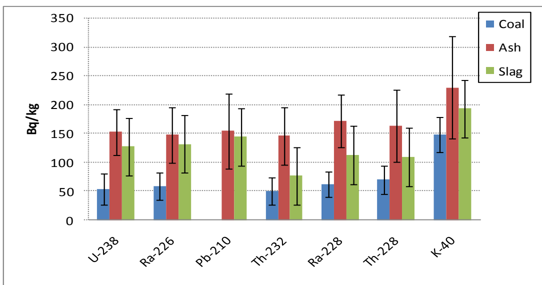
Figure 5-43: Activity concentrations in coal, ash and slag
