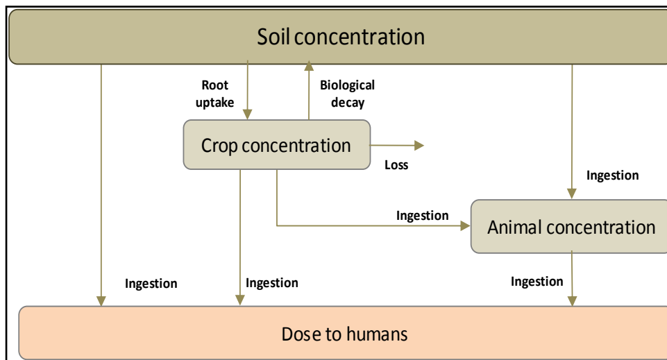
Figure 2-11: Pathways for soil
