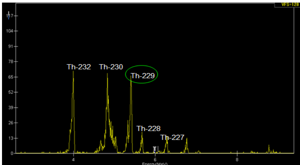
Figure 4-20: Typical energy spectrum for thorium analysis showing the peaks for ^{232}\text{Th} , ^{230}\text{Th} , ^{229}\text{Th} , ^{228}\text{Th} and ^{227}\text{Th}
