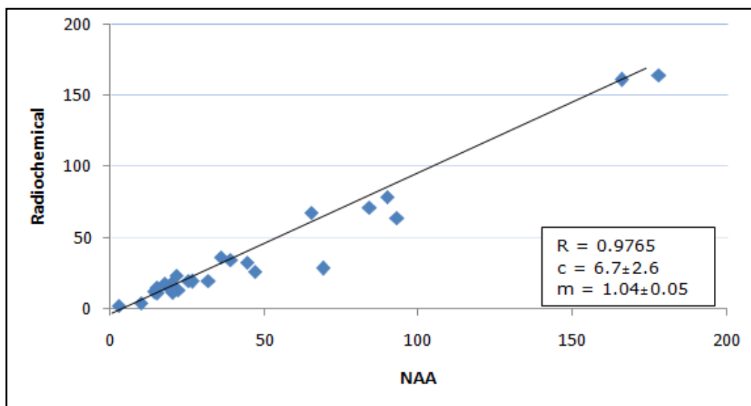
Figure 5-41: Correlation plot for ^{232}\text{Th} in cement samples (Activity concentration in \text{Bq.kg}^{-1} )
