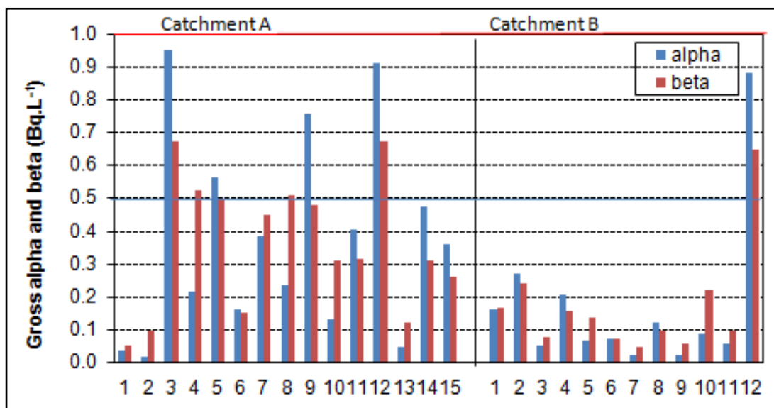
Figure 5-5: GA and GB in DWS groundwater samples (Bq.L -1 )
