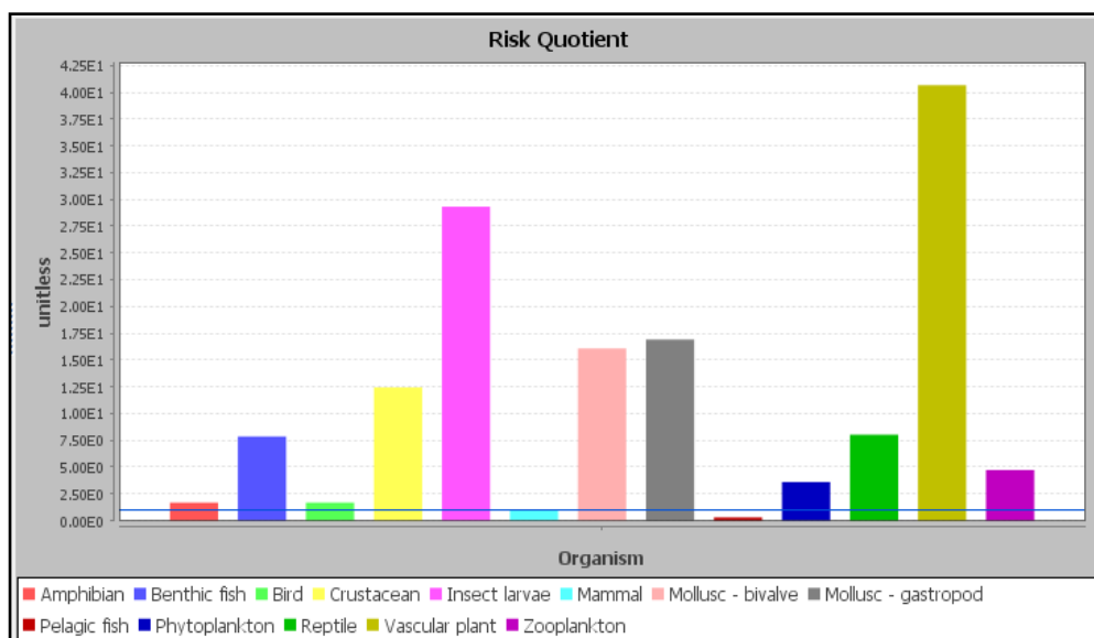
Figure 5-33: Risk Quotient for Tier 2 screening Aquatic environment (Phosphate industry)
