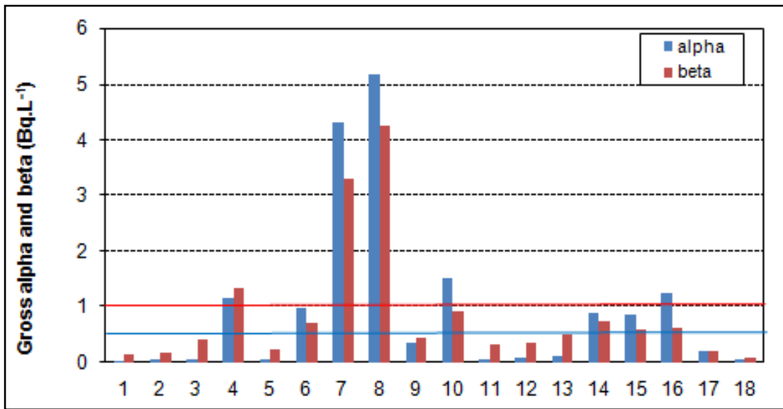
Figure 5-9: GA and GB activity in DWS surface water (Bq.L -1 )
