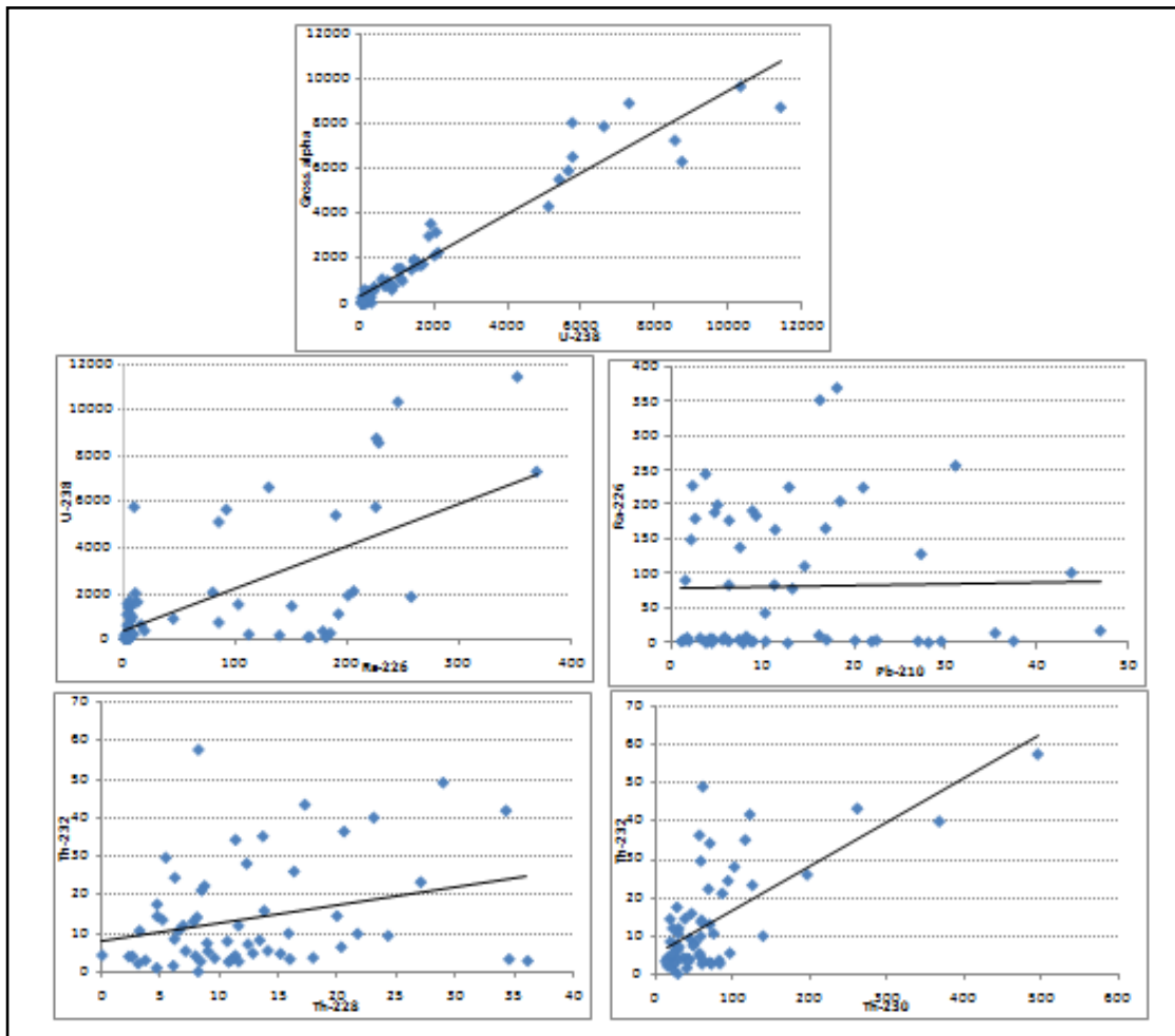
Figure 5-23: Correlation plots for surface mine water
