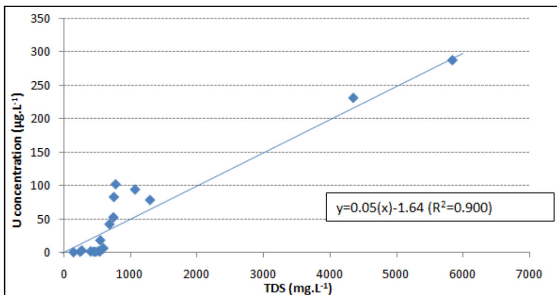
Figure 5-4: Correlation between TDS and uranium concentration for DWS surface water samples
