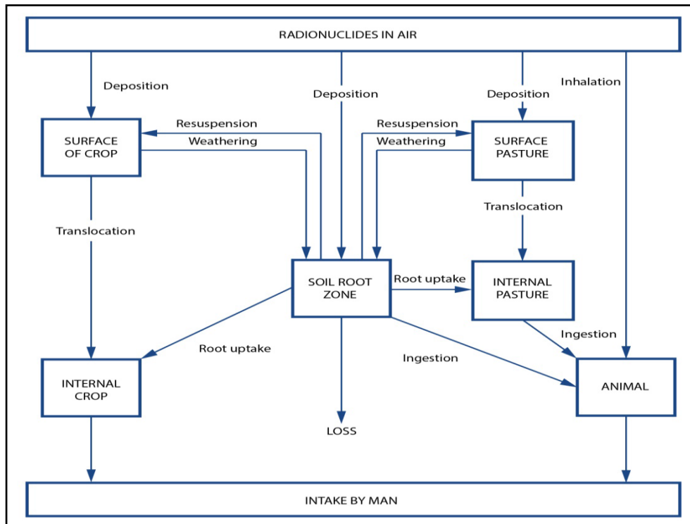
Figure 2-9: Processes for transfer of radionuclides in a terrestrial ecosystem (UNSCEAR, 2016)
