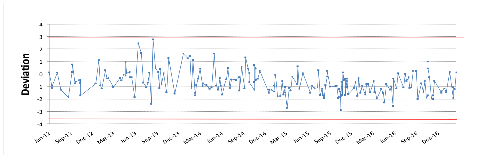
Figure 4-34: Quality control chart ^{232}\text{Th} control sample 2012-2016
