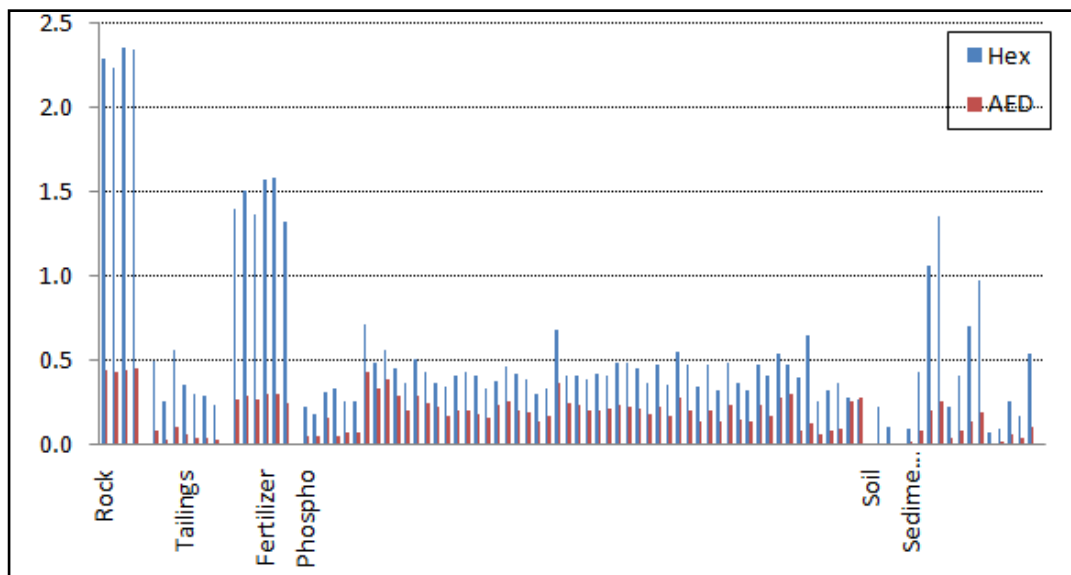
Figure 5-45: External radiation index and Annual Effective Dose (AED) of solids from the phosphate industry
