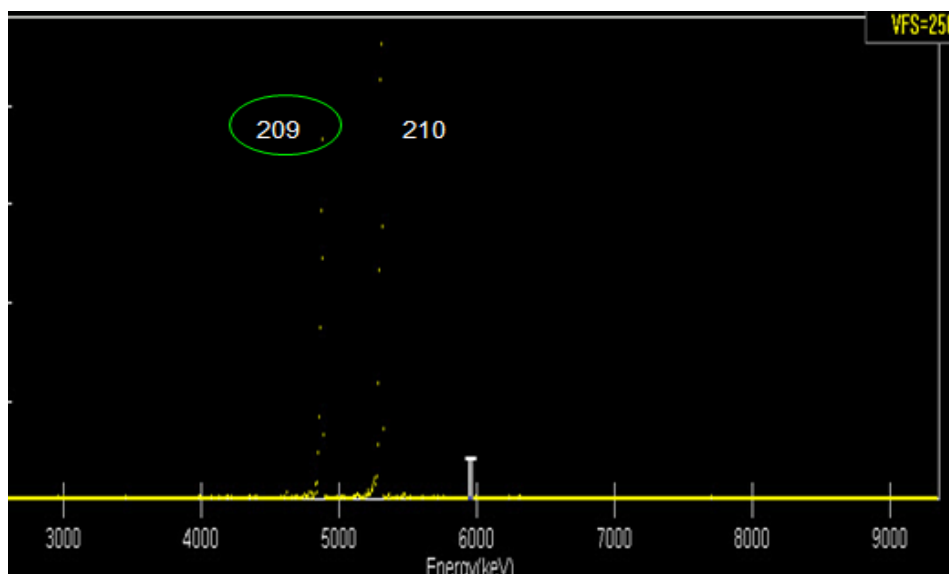
Figure 4-7: Typical energy spectrum for polonium analysis showing the peaks for ^{209}\text{Po} and ^{210}\text{Po}
