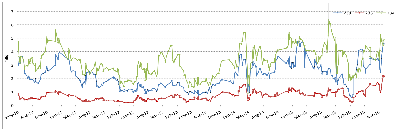
Figure 4-31: Moving average of U blank from 2010-2016 (mBq)
