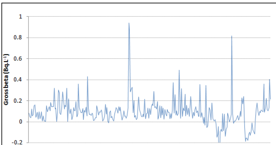
Figure 5-3: Gross beta activity of bottled water (Bq.L -1 )
