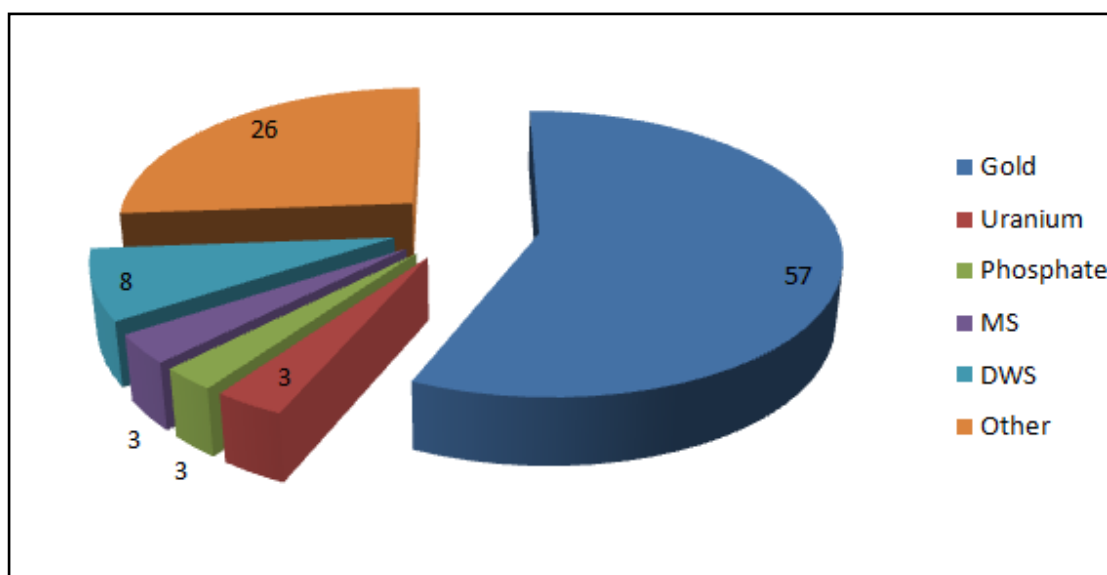
Figure 5-20: Water from NORM industries analysed in 2014 (% of total samples)
