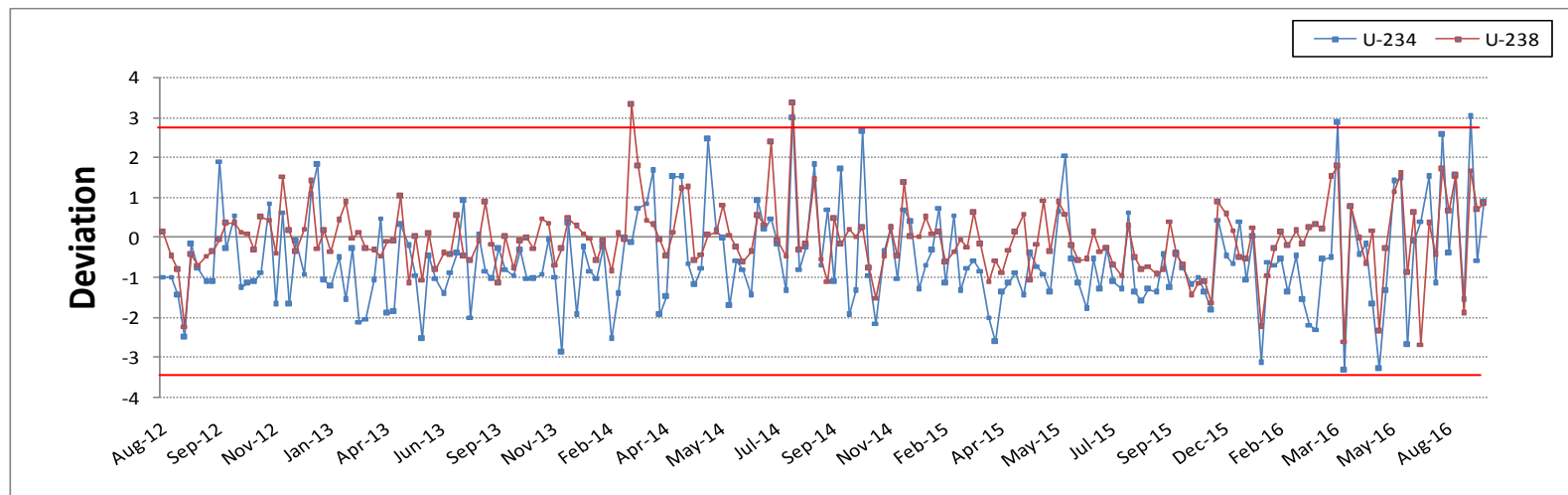
Figure 4-33: Quality control chart ^{238}\text{U} and ^{234}\text{U} control sample 2012-2016
