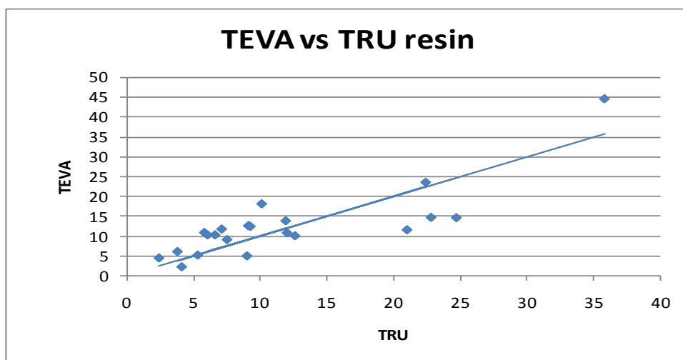
Figure 4-23: Comparison of ^{232}\text{Th} results in mine water samples separated on TRU and TEVA resin (solid line represents 1:1 correlation between results obtained with the two different resins)
