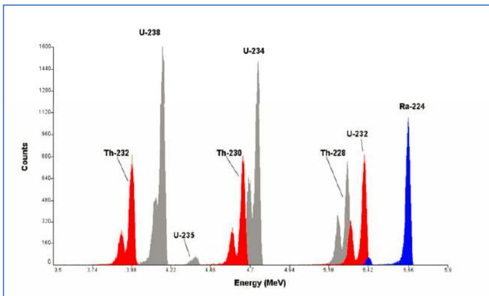
Figure 2-23: Overlap of interfering peaks of U and Th Isotopes
