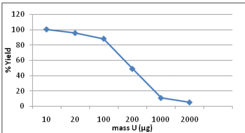
Figure 4-16: Influence of mass of U on \text{LaF}_3 precipitation recovery
