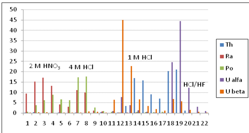
Figure 4-22: Elution curves showing behaviour for the nuclides of interest on TRU resin (1-5:2 M \text{HNO}_3 ; 6-9:4 M \text{HCl} ; 10-17:1 M \text{HCl} ; 18-20:0.1 M \text{HCl} /0.1 M \text{HF} )
