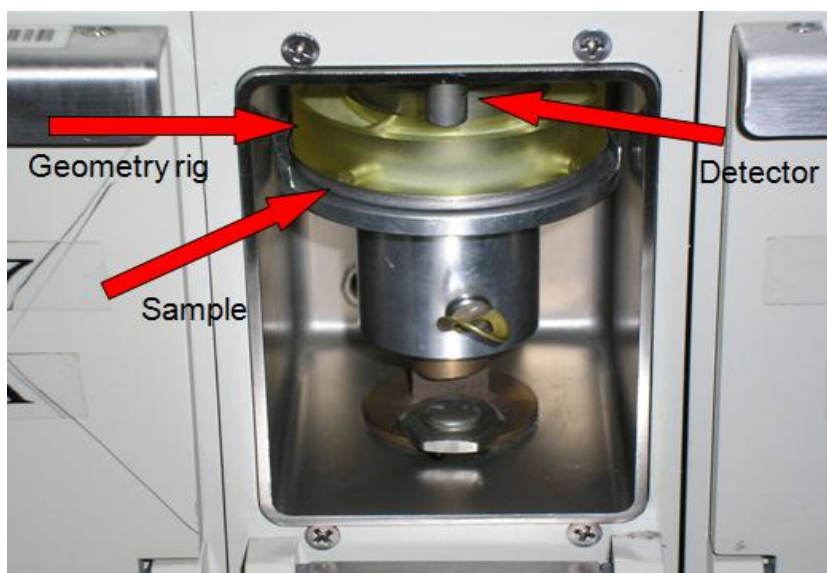
Figure 4-6: Inside of the alpha spectrometer detector chamber
