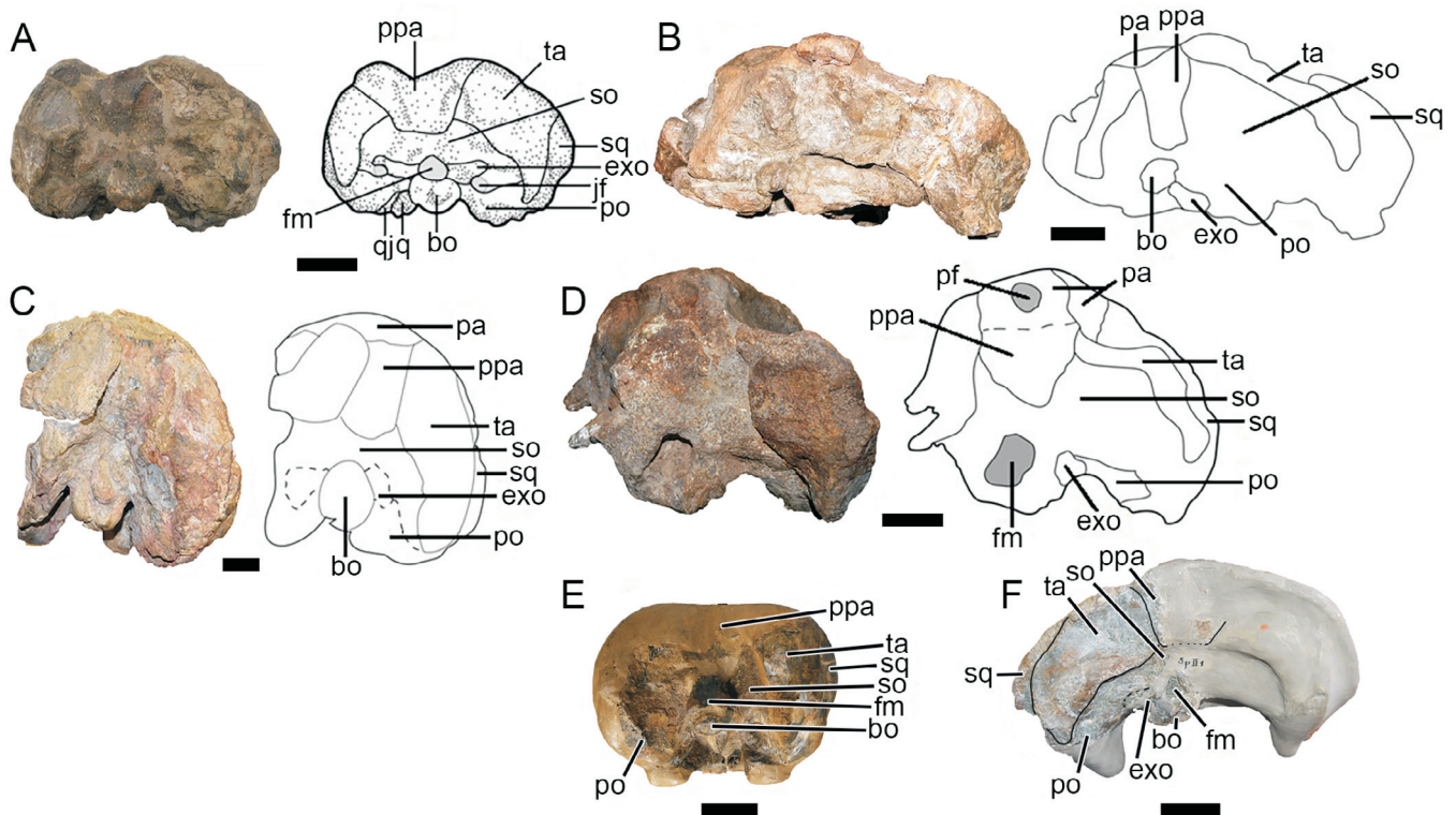
Figure 12. Jonkeria skulls in occipital view. A , FMNH UC 1511; B , SAM-PK-4343; C , SAM-PK-11884; D , TM 212; E , AMNH FARB 5620; F , MB.R.983. Abbreviations: bo, basioccipital; exo, exoccipital; fm, foramen magnum; jf, jugular foramen; pa, parietal; pf, pineal foramen; po, paroccipital process of opisthotic; ppa, postparietal; q, quadrate; qj, quadratojugal; so, supraoccipital; sq, squamosal; ta, tabular. Scale bars represent 10 cm.
