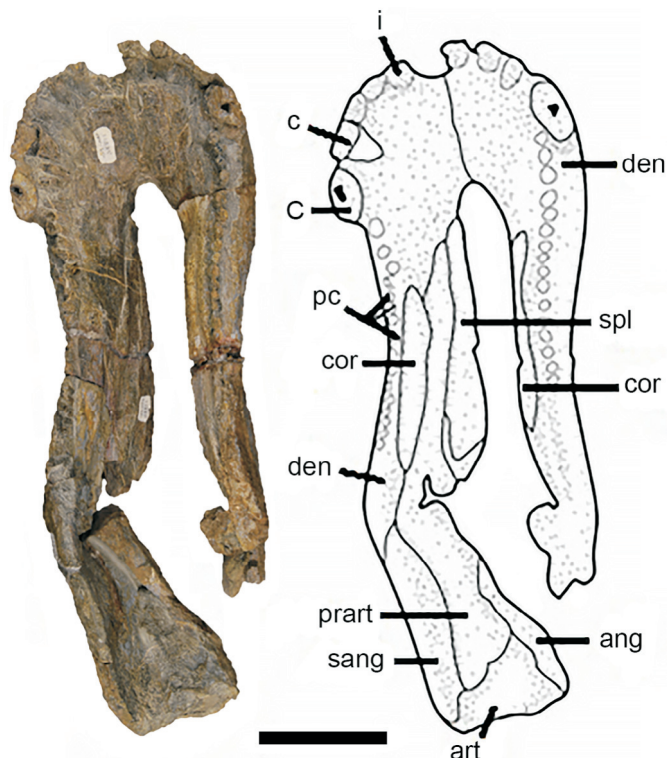
Figure 14. Jonkeria mandible SAM-PK-11884 in dorsal view. Abbreviations: ang, angular; art, articular; C, upper canine; c, lower canine; cor, coronoid bone; den, dentary; i, lower incisor; pc, low postcanine; prart, prearticular; sang, surangular; spl, splenial. Scale bar represents 10 cm.
