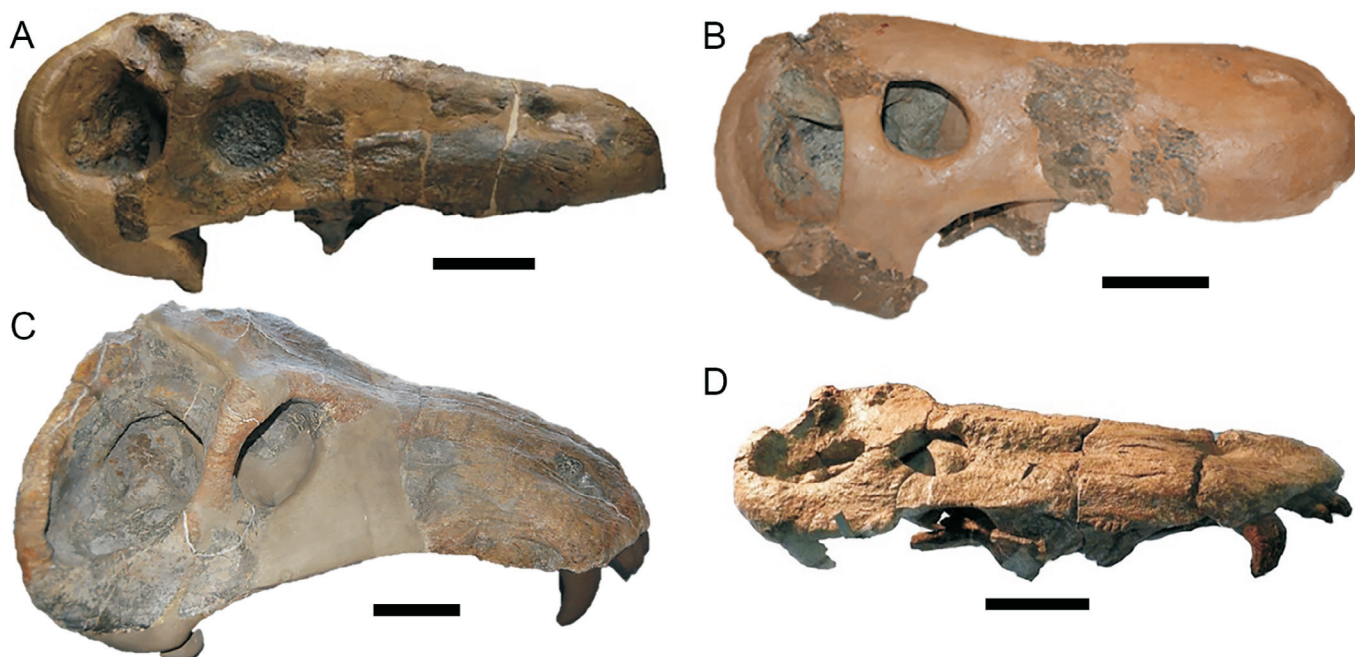
Figure 5. Jonkeria skulls in lateral view. A , Holotype of Jonkeria vanderbyli (AMNH FARB 5620); B , holotype of Jonkeria ingens (AMNH FARB 5634); less than 50% of the skull is preserved; the remainder is reconstructed with plaster of Paris; C , holotype of Jonkeria boonstrai (MB.R.983); the skull is distorted, with two-thirds of the ventral surface and the teeth missing (reconstructed in plaster of Paris); D , holotype of Jonkeria haughtoni (SAM-PK-4343). Specimen in D in right lateral view; specimens in A–C in left lateral view but mirrored for comparison. Scale bars represent 10 cm.
